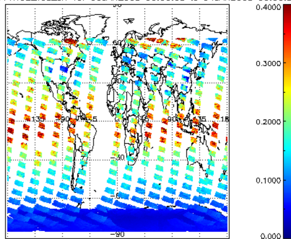
SCIOL2P_NADUV1NO2_vcd_err for 03JAN2008 00:00:00 to 04JAN2008 00:00:00
