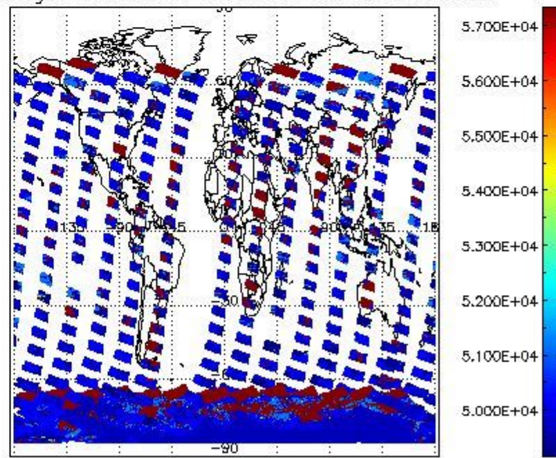
cloud_flags for 03JAN2008 00:00:00 to 04JAN2008 00:00:00
