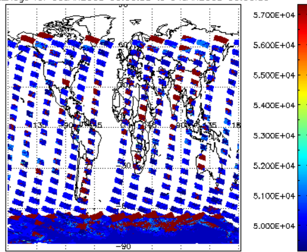
cloud_flags for 03JAN2008 00:00:00 to 04JAN2008 00:00:00
