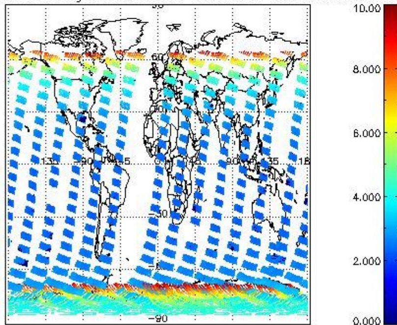
SCIOL2P_NADUV003_amf_gr for 03JAN2008 00:00:00 to 04JAN2008 00:00:00
