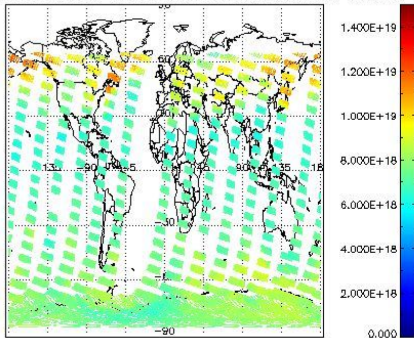
SCIOL2P_NADUV003_vcd for 03JAN2008 00:00:00 to 04JAN2008 00:00:00
