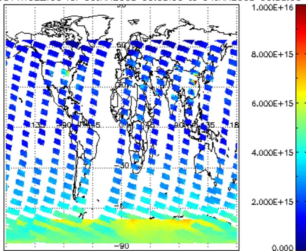
SCIOL2P_NADUV1NO2_vcd for 03JAN2008 00:00:00 to 04JAN2008 00:00:00
