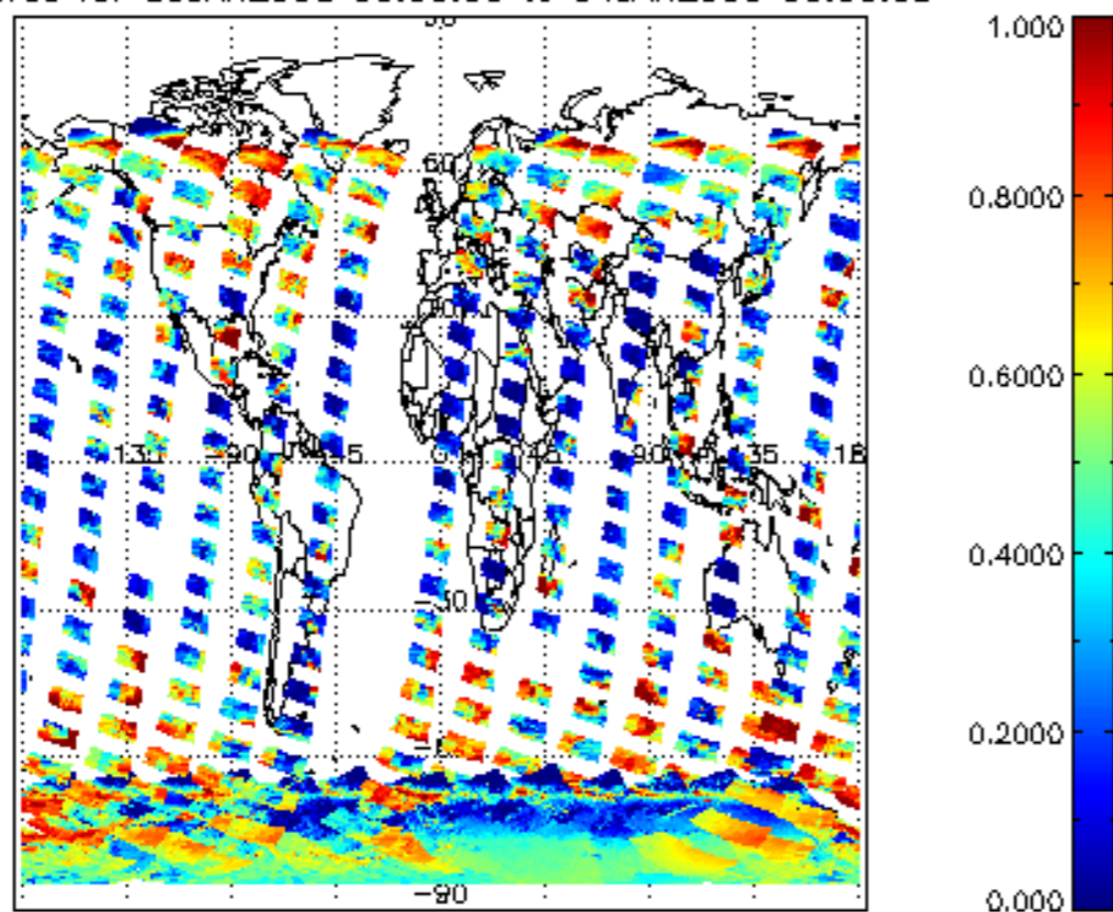
cL_frac for 03JAN2008 00:00:00 to 04JAN2008 00:00:00
