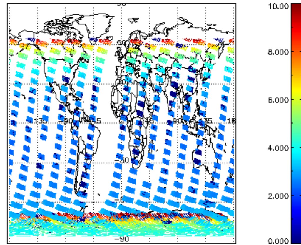
SCIOL2P_NADUV003_amf_cl for 03JAN2008 00:00:00 to 04JAN2008 00:00:00
