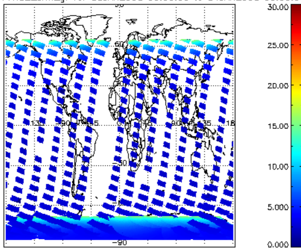
SCIOL2P_NADUV1NO2_amf_gr for 03JAN2008 00:00:00 to 04JAN2008 00:00:00
