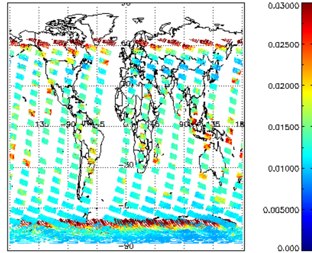
SCIOL2P_NADUV003_vcd_err for 03JAN2008 00:00:00 to 04JAN2008 00:00:00
