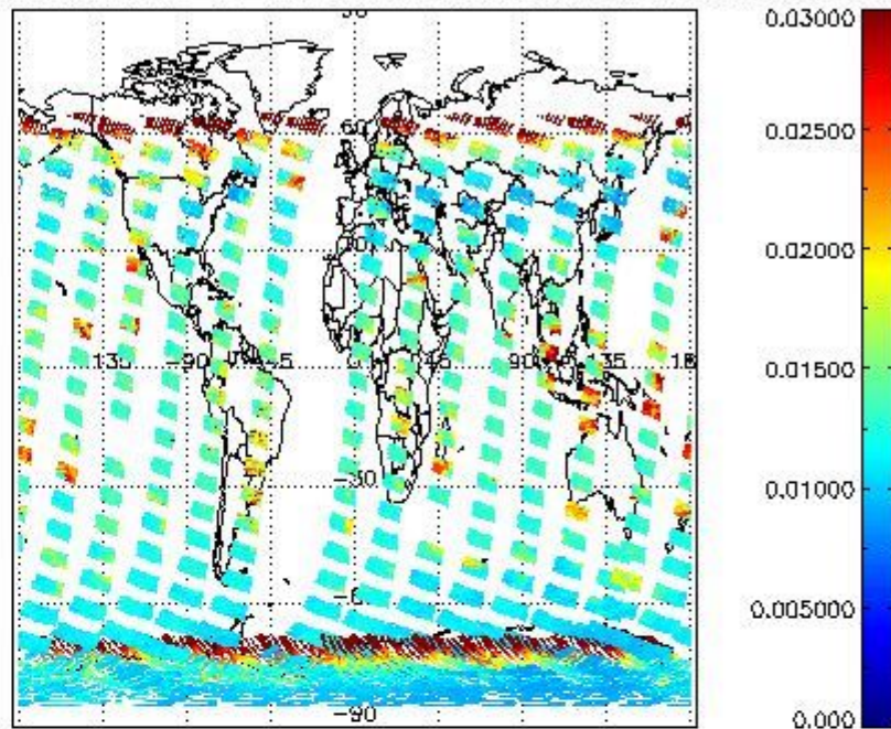
SCIOL2P_NADUV003_vcd_err for 03JAN2008 00:00:00 to 04JAN2008 00:00:00
