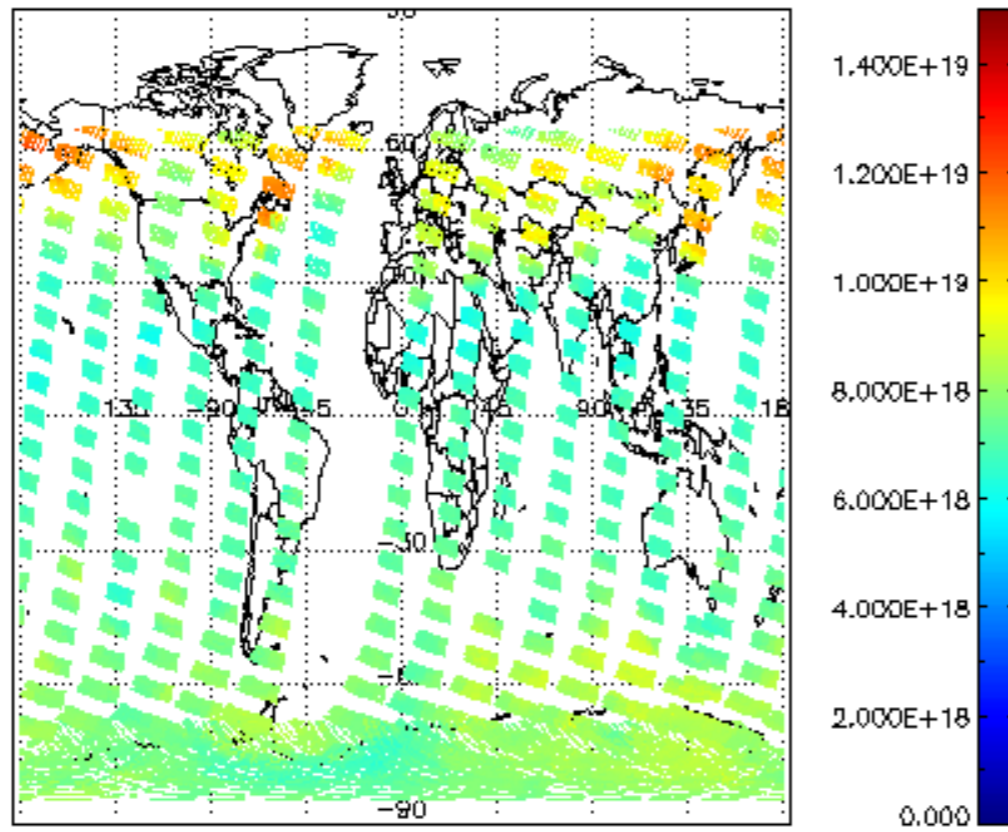
SCIOL2P_NADUV003_vcd for 03JAN2008 00:00:00 to 04JAN2008 00:00:00
