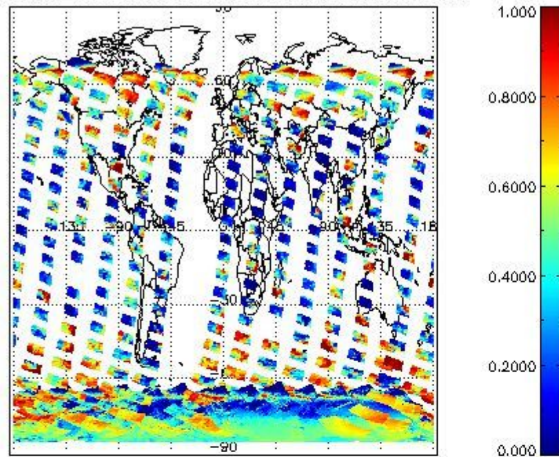
cL_frac for 03JAN2008 00:00:00 to 04JAN2008 00:00:00
