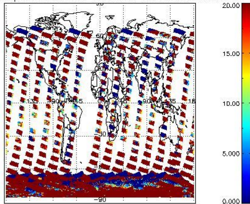
cLopt_depth for 03JAN2008 00:00:00 to 04JAN2008 00:00:00
