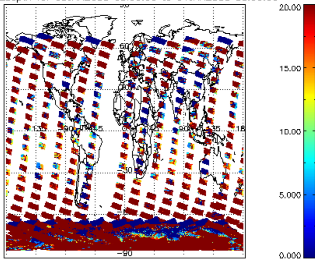
cLopt_depth for 03JAN2008 00:00:00 to 04JAN2008 00:00:00
