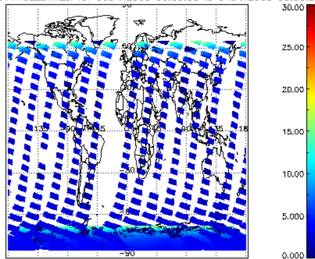
SCIOL2P_NADUV1NO2_amf_cl for 03JAN2008 00:00:00 to 04JAN2008 00:00:00
