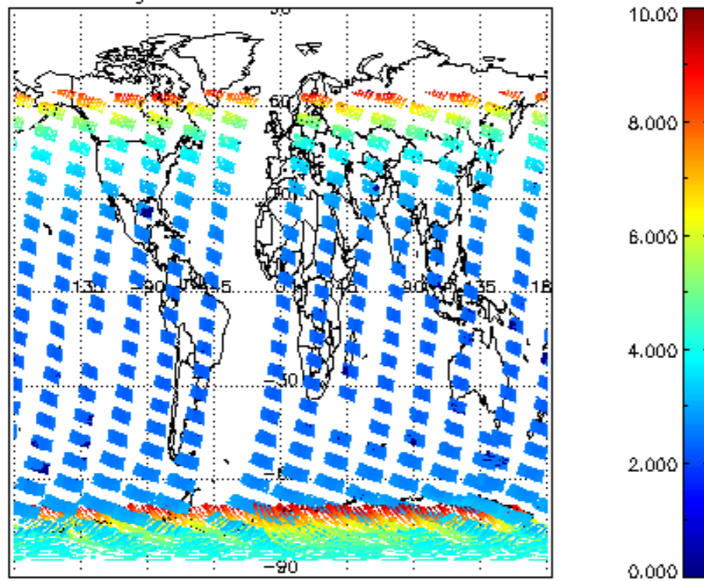
SCIOL2P_NADUV003_amf_gr for 03JAN2008 00:00:00 to 04JAN2008 00:00:00
