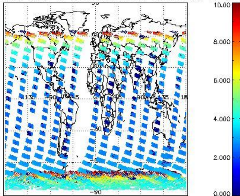
SCIOL2P_NADUV003_amf_cl for 03JAN2008 00:00:00 to 04JAN2008 00:00:00
