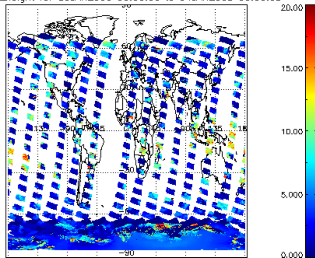
cL_top_height for 03JAN2008 00:00:00 to 04JAN2008 00:00:00
