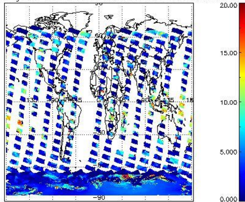
cL_top_height for 03JAN2008 00:00:00 to 04JAN2008 00:00:00
