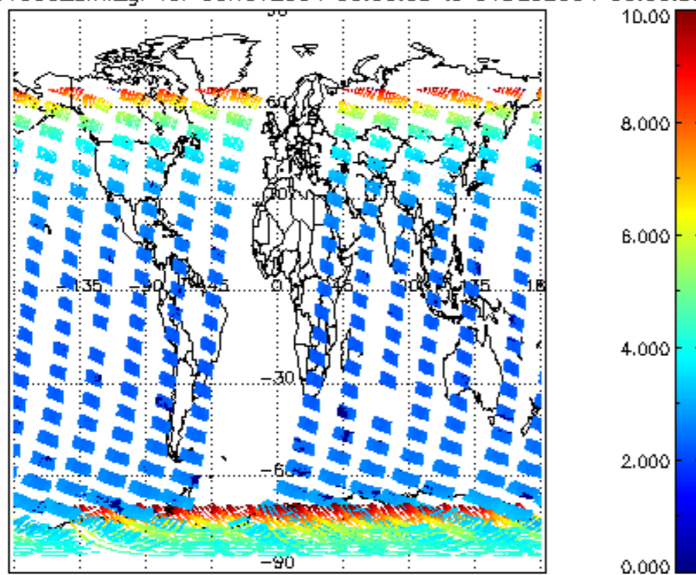
SCIOL2P_NADUV003_amf_gr for 30NOV2004 00:00:00 to 01DEC2004 00:00:00
