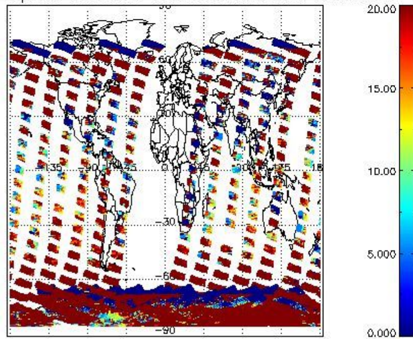
cL_opt_depth for 30NOV2004 00:00:00 to 01DEC2004 00:00:00
