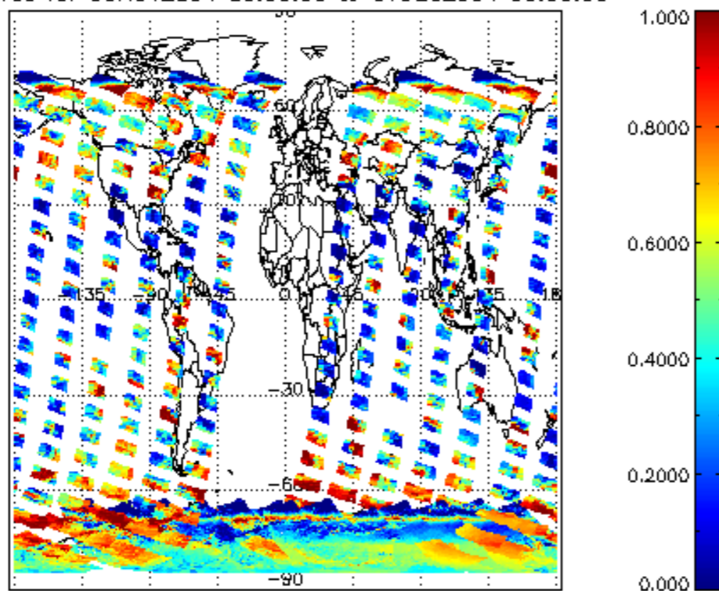
cl_frac for 30NOV2004 00:00:00 to 01DEC2004 00:00:00
