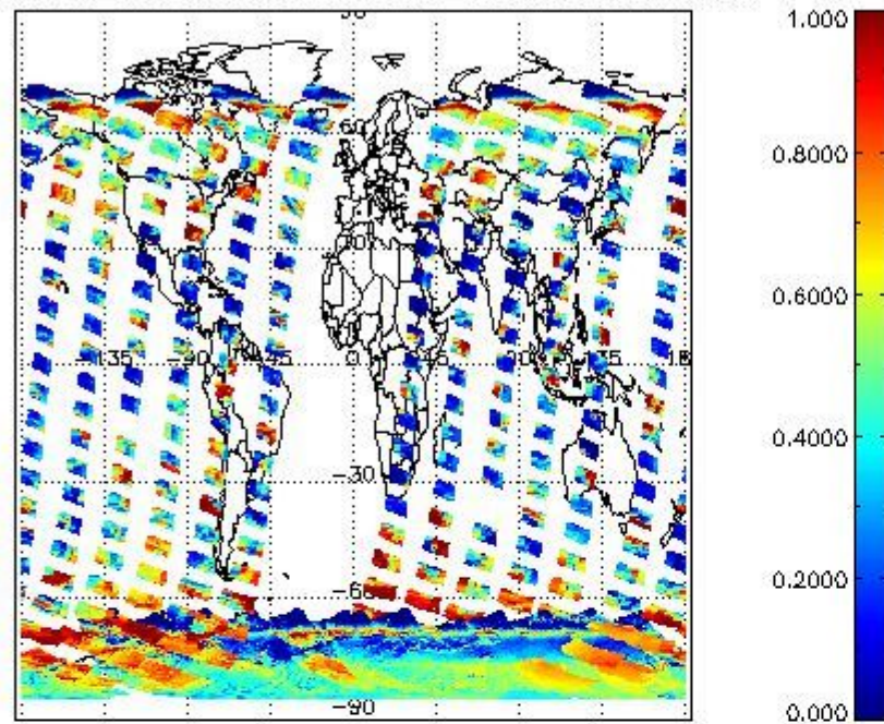
cLfrac for 30NOV2004 00:00:00 to 01DEC2004 00:00:00
