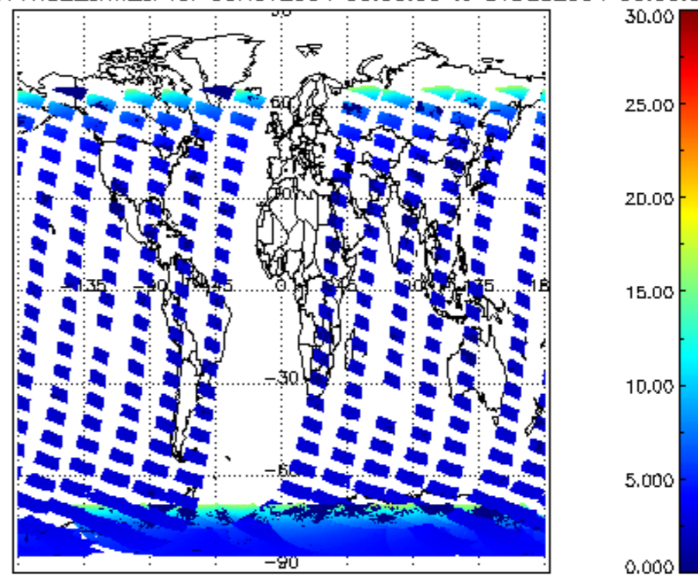
ICIOL2P_NADUV1NO2_amf_cl for 30NOV2004 00:00:00 to 01DEC2004 00:00:00
