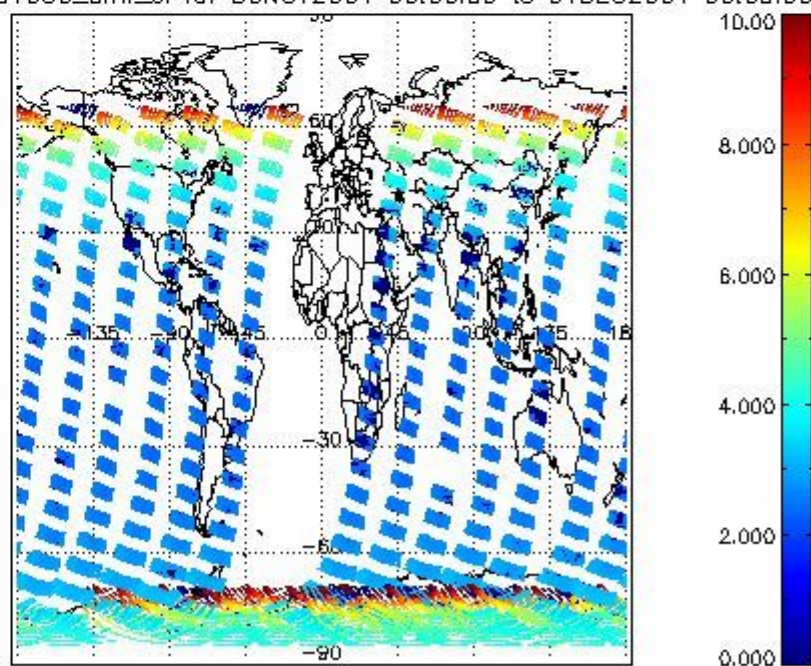
SCIOL2P_NADUV003_amf_sl for 30NOV2004 00:00:00 to 01DEC2004 00:00:00
