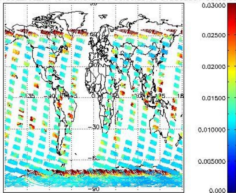
SCIOL2P_NADUV003_vcd_err for 30NOV2004 00:00:00 to 01DEC2004 00:00:00
