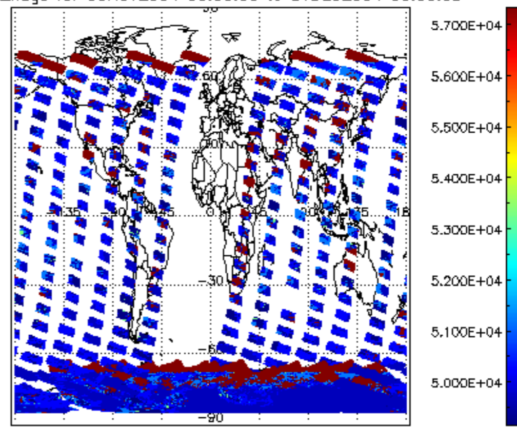
cloud_flags for 30NOV2004 00:00:00 to 01DEC2004 00:00:00
