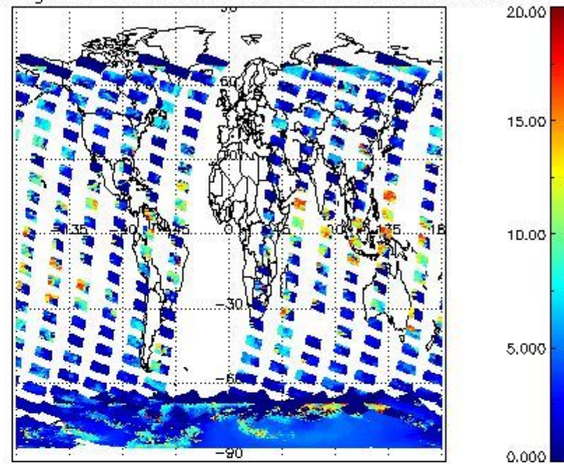
cL_top_height for 30NOV2004 00:00:00 to 01DEC2004 00:00:00
