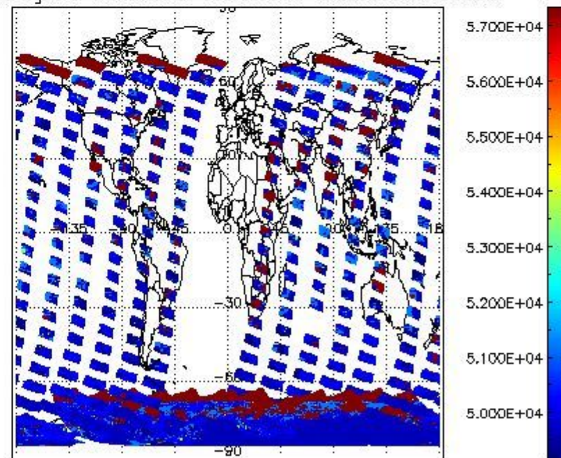
cloud_flags for 30NOV2004 00:00:00 to 01DEC2004 00:00:00
