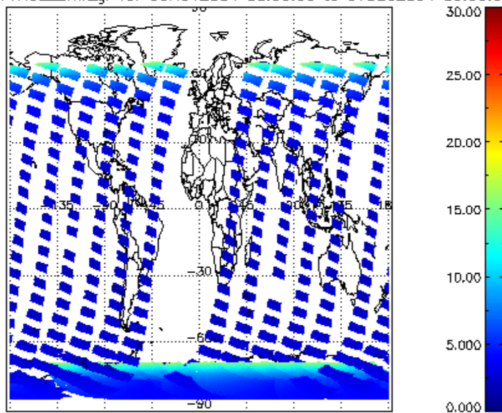
ICIOL2P_NADUV1NO2_amf_gr for 30NOV2004 00:00:00 to 01DEC2004 00:00:00
