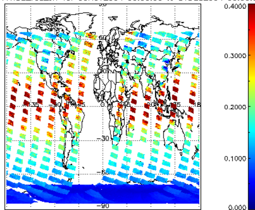
ICIOL2P_NADUV1NO2_vcd_err for 30NOV2004 00:00:00 to 01DEC2004 00:00:00
