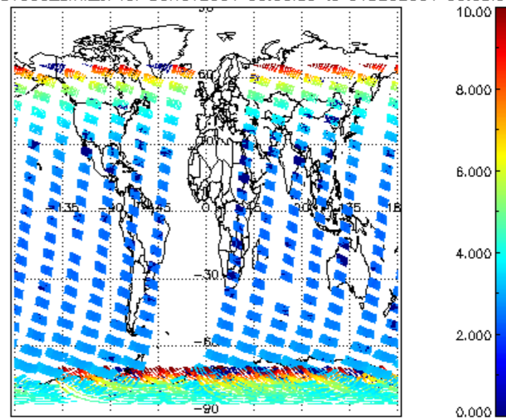
SCIOL2P_NADUV003_amf_cl for 30NOV2004 00:00:00 to 01DEC2004 00:00:00
