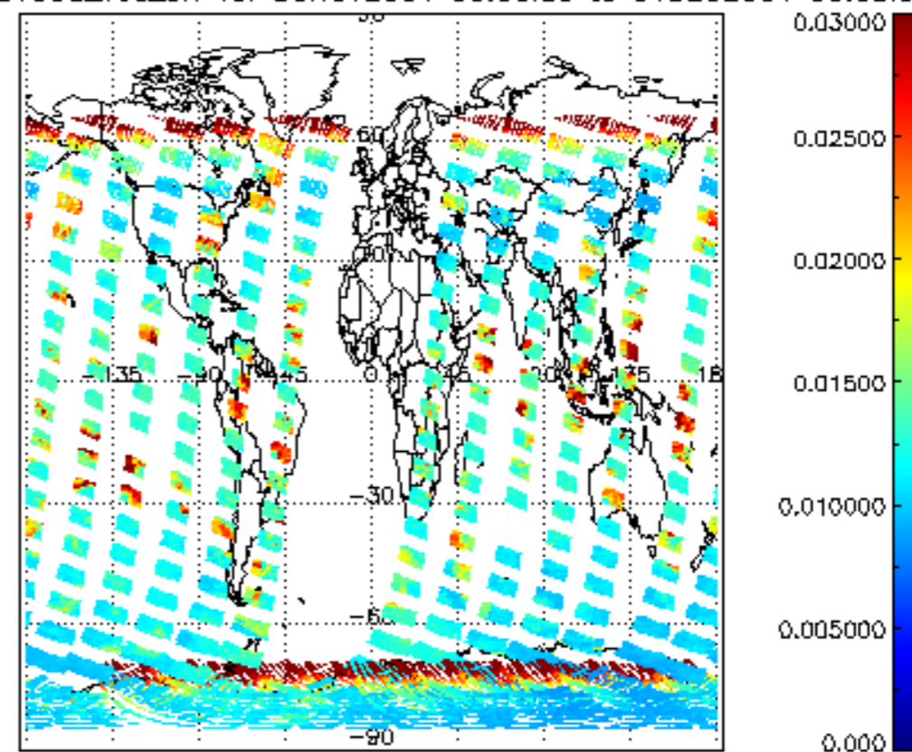
SCIOL2P_NADUV003_vcd_err for 30NOV2004 00:00:00 to 01DEC2004 00:00:00
