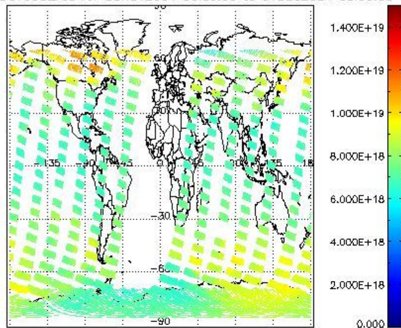
SCIOL2P_NADUV003_vcd for 30NOV2004 00:00:00 to 01DEC2004 00:00:00
