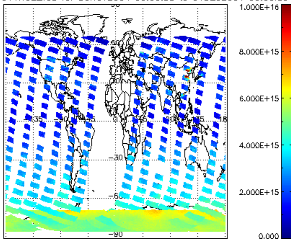
SCIOL2P_NADUV1NO2_vcd for 30NOV2004 00:00:00 to 01DEC2004 00:00:00
