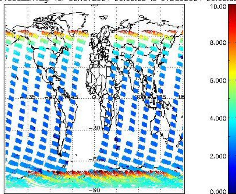
SCIOL2P_NADUV003_amf_gr for 30NOV2004 00:00:00 to 01DEC2004 00:00:00
