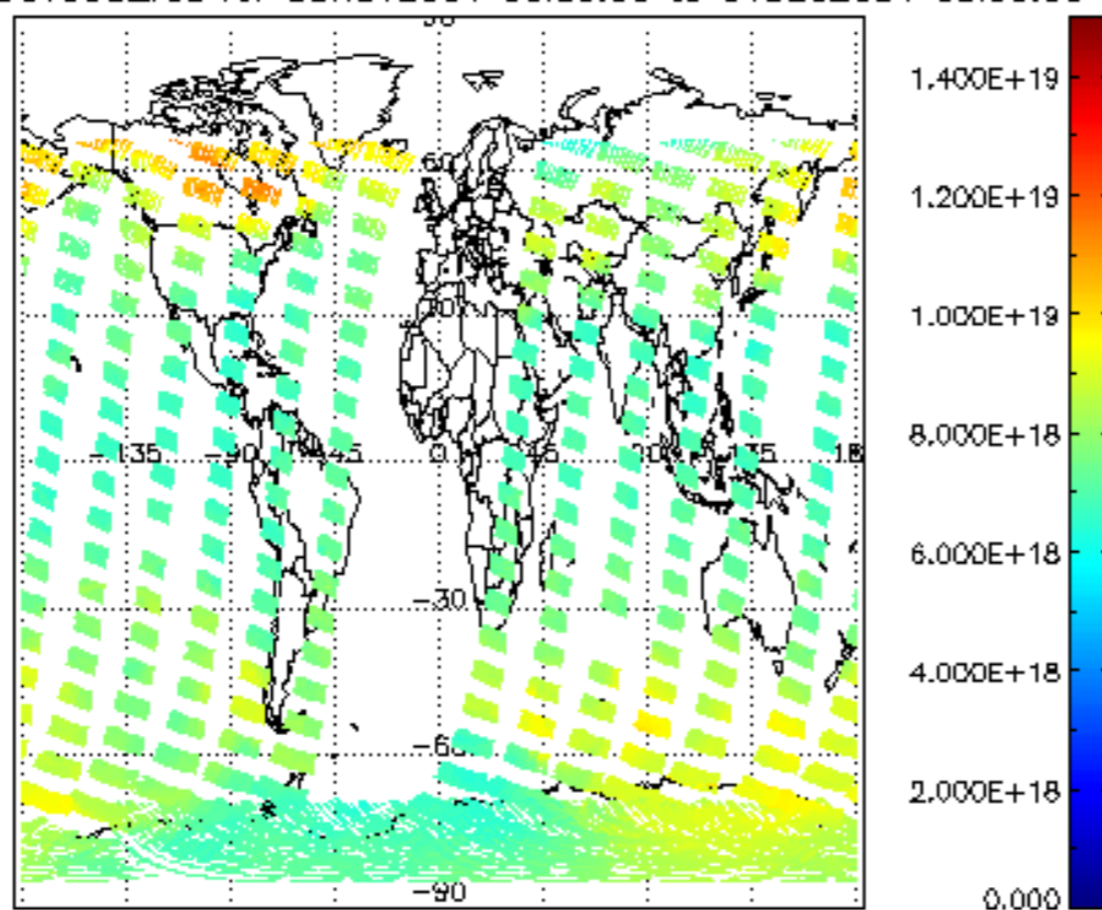
SCIOL2P_NADUV003_vcd for 30NOV2004 00:00:00 to 01DEC2004 00:00:00
