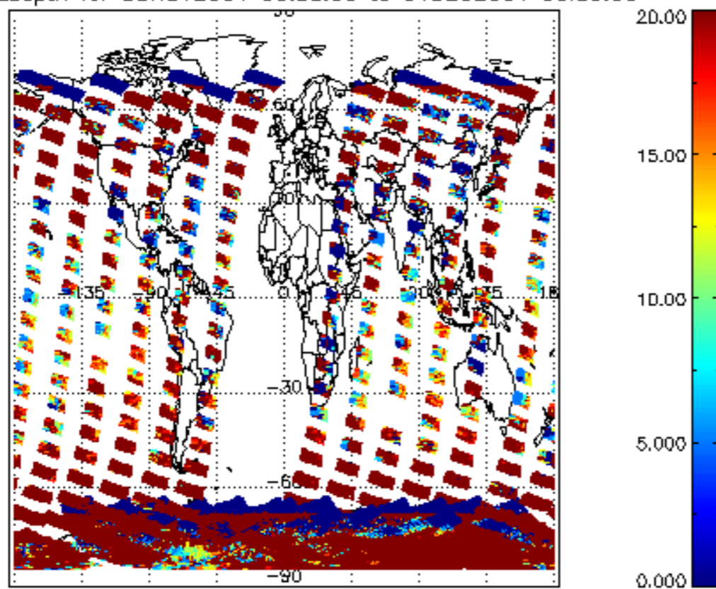
cl_opt_depth for 30NOV2004 00:00:00 to 01DEC2004 00:00:00
