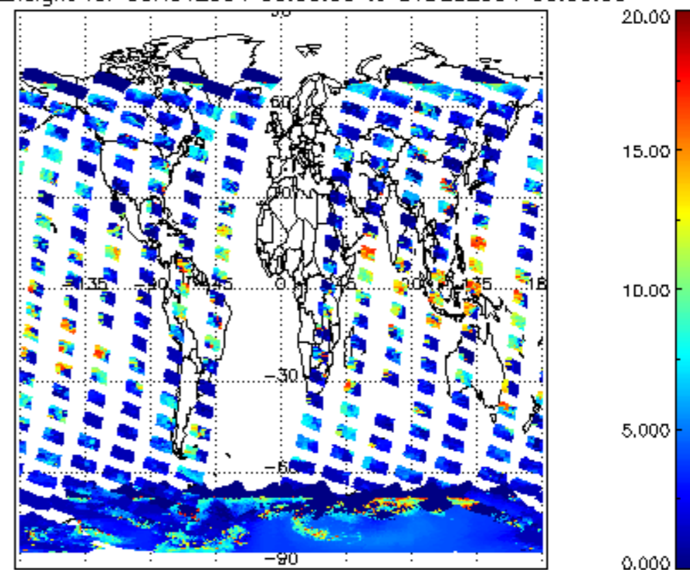
cl_top_height for 30NOV2004 00:00:00 to 01DEC2004 00:00:00
