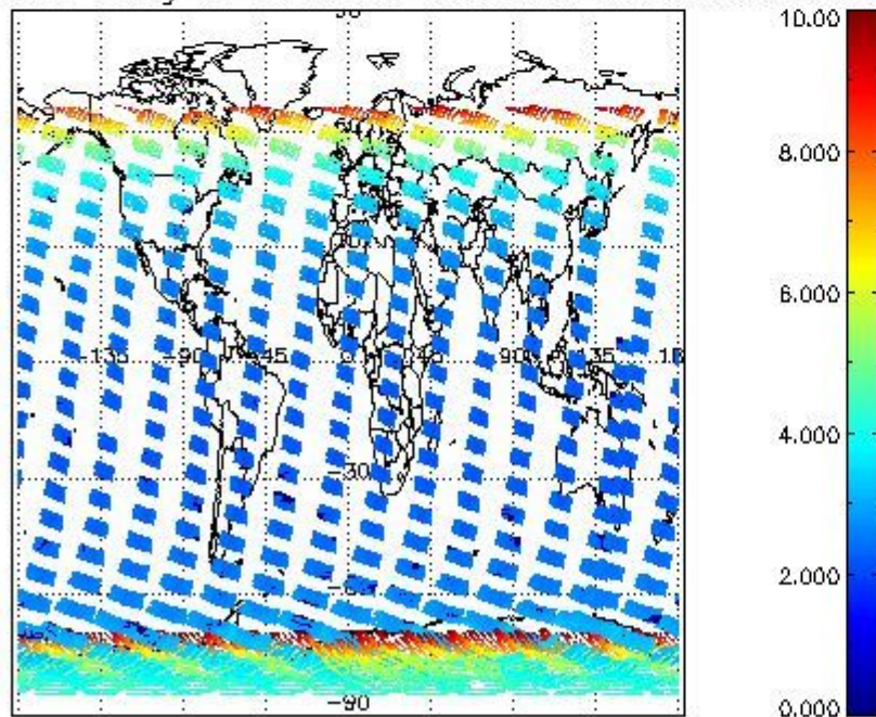
SCIOL2P_NADUV003_amf_gr for 29NOV2004 00:00:00 to 30NOV2004 00:00:00
