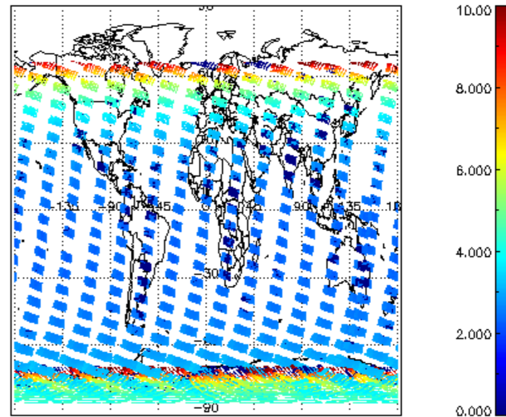
SCIOL2P_NADUV003_amf_cl for 29NOV2004 00:00:00 to 30NOV2004 00:00:00
