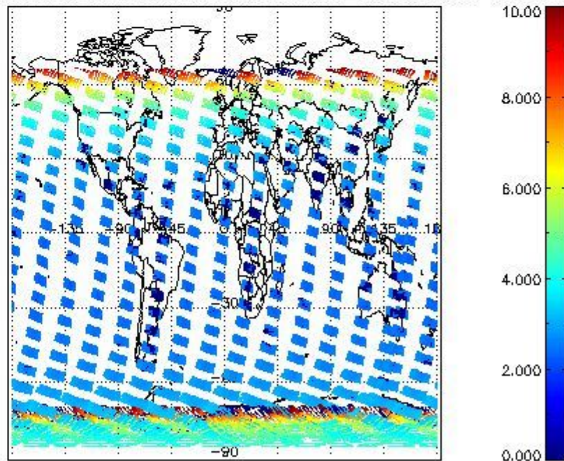
SCIOL2P_NADUV003_amf_cl for 29NOV2004 00:00:00 to 30NOV2004 00:00:00
