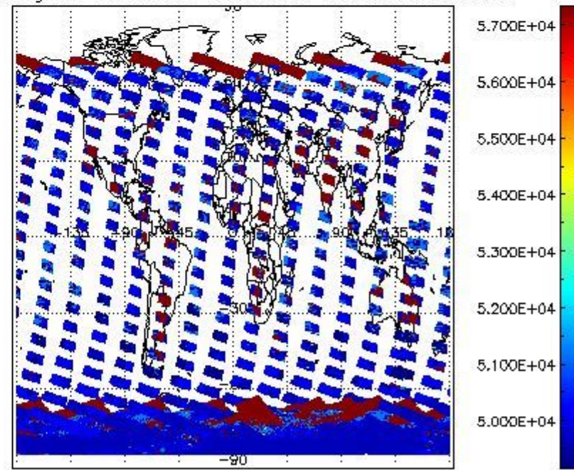
cloud_flags for 29NOV2004 00:00:00 to 30NOV2004 00:00:00
