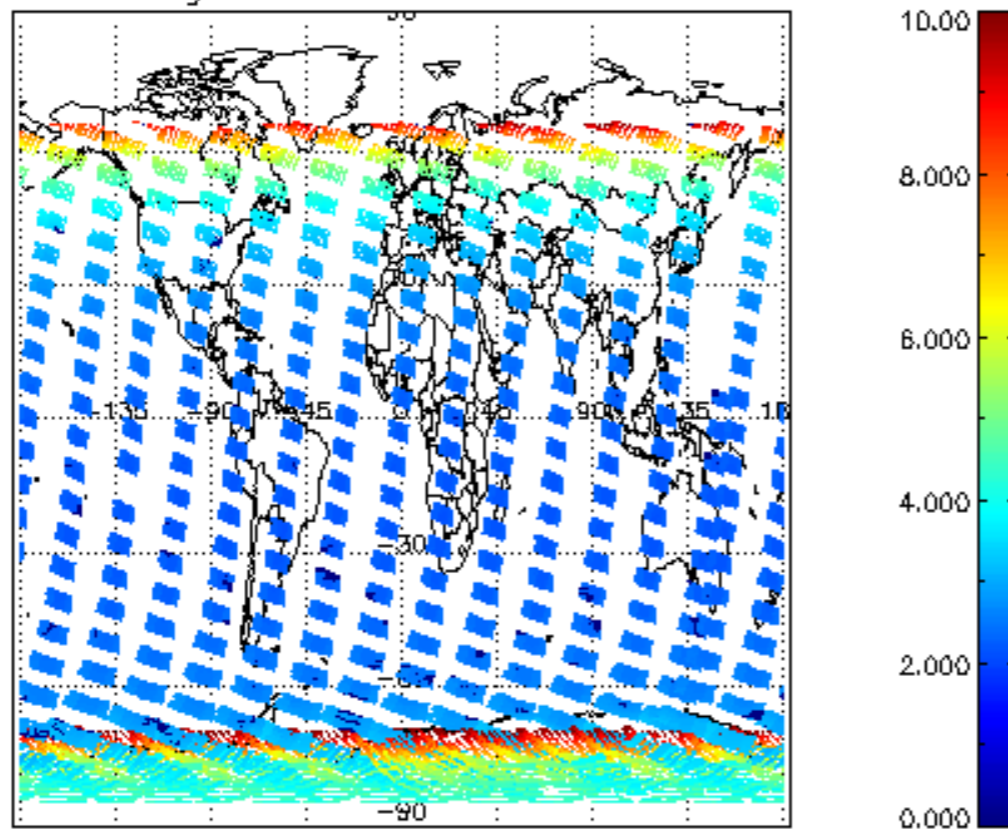
SCIOL2P_NADUV003_amf_gr for 29NOV2004 00:00:00 to 30NOV2004 00:00:00
