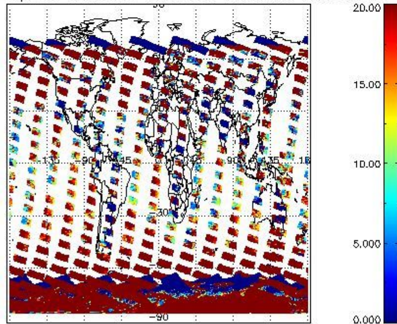
cLopt_depth for 29NOV2004 00:00:00 to 30NOV2004 00:00:00
