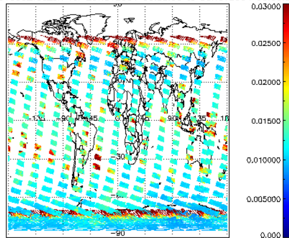
SCIOL2P_NADUV003_vcd_err for 29NOV2004 00:00:00 to 30NOV2004 00:00:00
