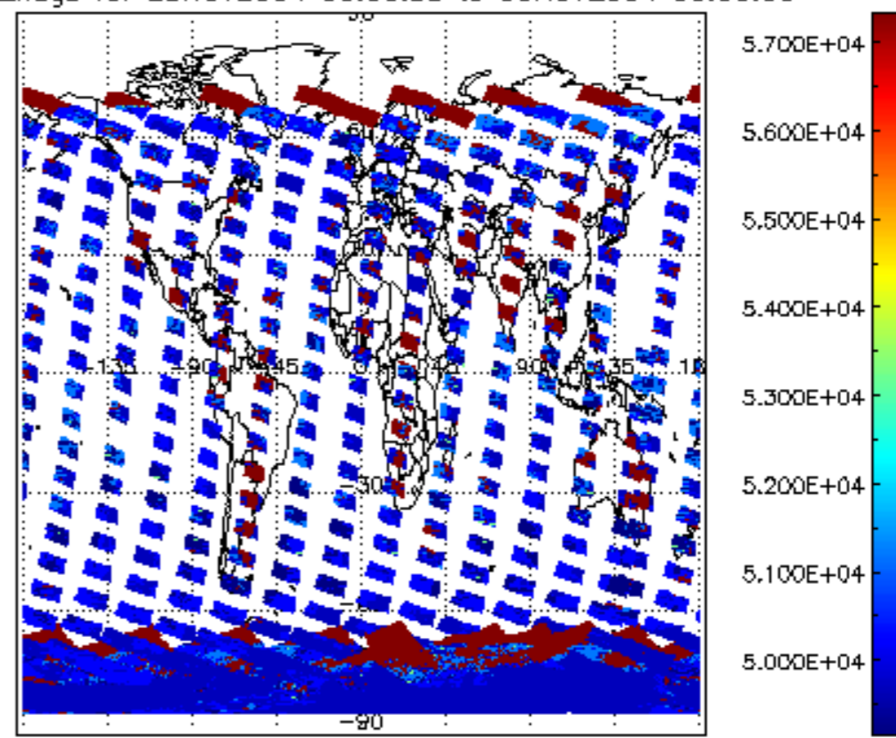
cloud_flags for 29NOV2004 00:00:00 to 30NOV2004 00:00:00
