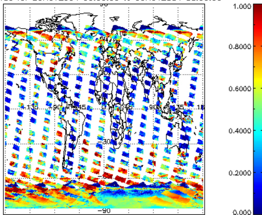
cLfrac for 29NOV2004 00:00:00 to 30NOV2004 00:00:00
