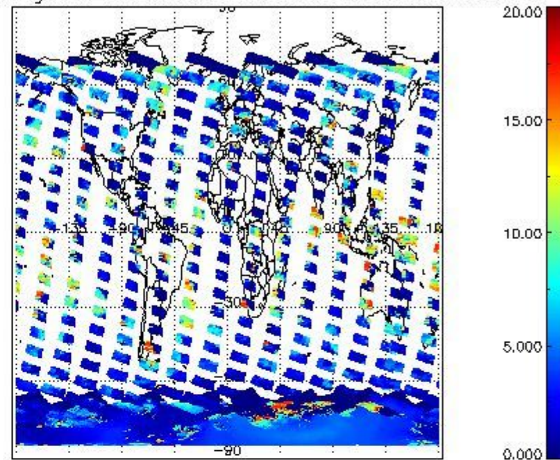
cL_top_height for 29NOV2004 00:00:00 to 30NOV2004 00:00:00
