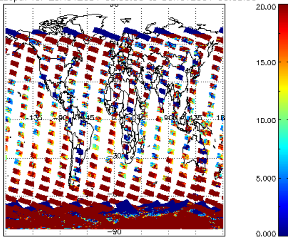
cL_opt_depth for 29NOV2004 00:00:00 to 30NOV2004 00:00:00
