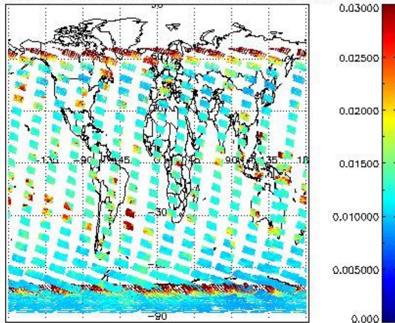
SCIOL2P_NADUV003_vcd_err for 29NOV2004 00:00:00 to 30NOV2004 00:00:00
