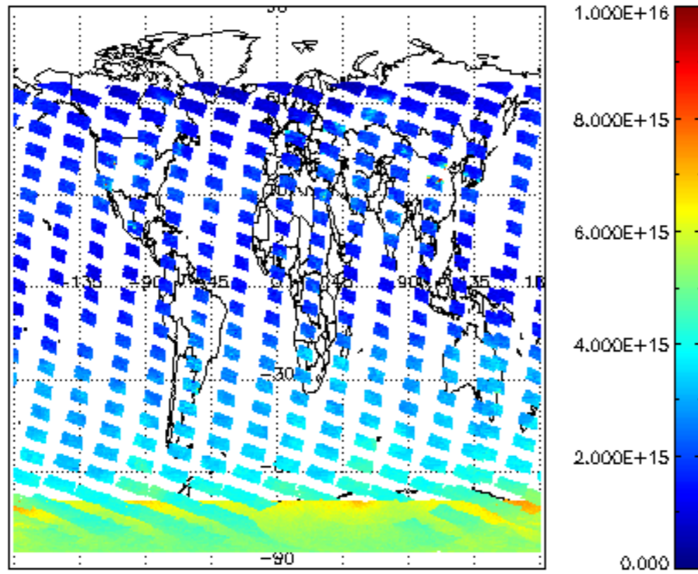
SCIOL2P_NADUV1NO2_vcd for 29NOV2004 00:00:00 to 30NOV2004 00:00:00
