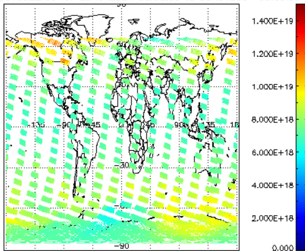
SCIOL2P_NADUV003_vcd for 29NOV2004 00:00:00 to 30NOV2004 00:00:00
