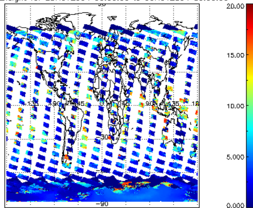
cL_top_height for 29NOV2004 00:00:00 to 30NOV2004 00:00:00
