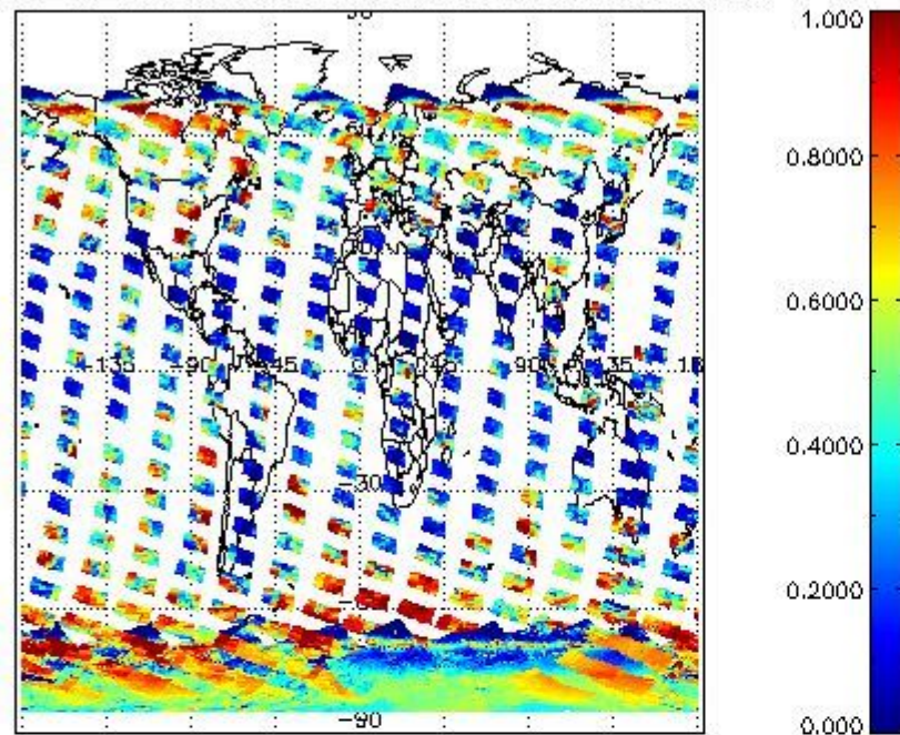
cLfrac for 29NOV2004 00:00:00 to 30NOV2004 00:00:00
