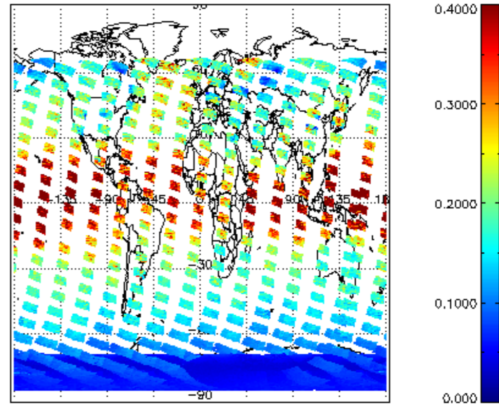
SCIOL2P_NADUV1NO2_vcd_err for 29NOV2004 00:00:00 to 30NOV2004 00:00:00
