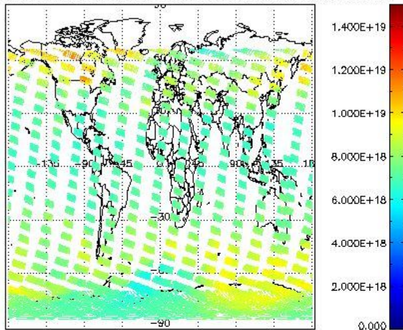
SCIOL2P_NADUV003_vcd for 29NOV2004 00:00:00 to 30NOV2004 00:00:00
