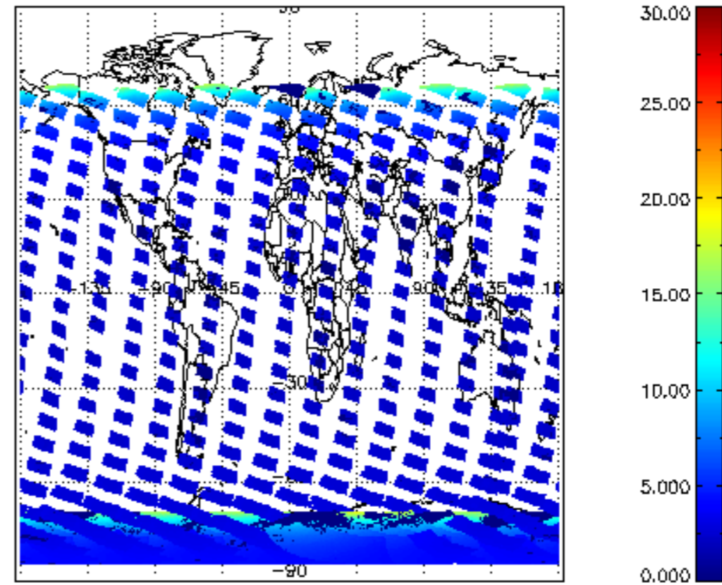
SCIOL2P_NADUV1NO2_amf_cl for 29NOV2004 00:00:00 to 30NOV2004 00:00:00
