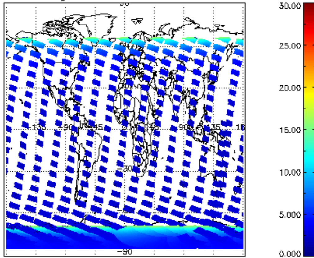
SCIOL2P_NADUV1NO2_amf_gr for 29NOV2004 00:00:00 to 30NOV2004 00:00:00
