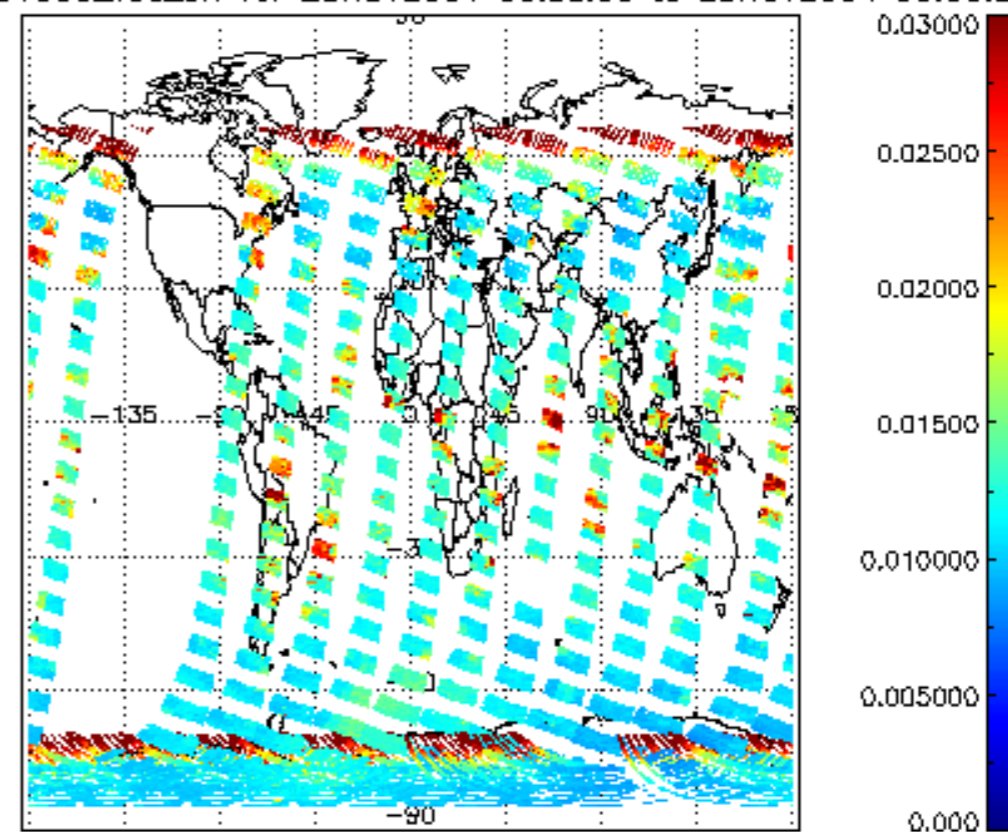
SCIOL2P_NADUV003_vcd_err for 28NOV2004 00:00:00 to 29NOV2004 00:00:00
