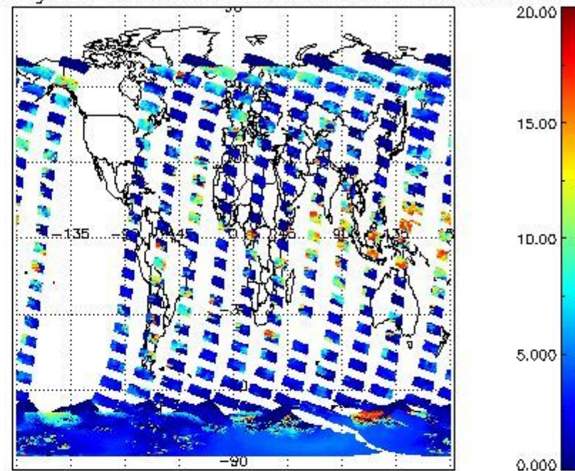
cL_top_height for 28NOV2004 00:00:00 to 29NOV2004 00:00:00
