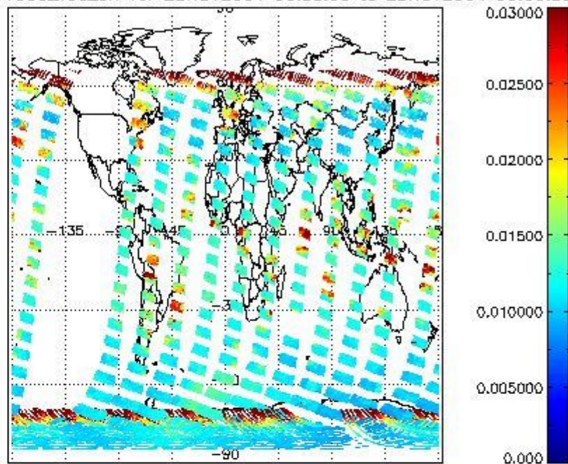
SCIOL2P_NADUV003_vcd_err for 28NOV2004 00:00:00 to 29NOV2004 00:00:00
