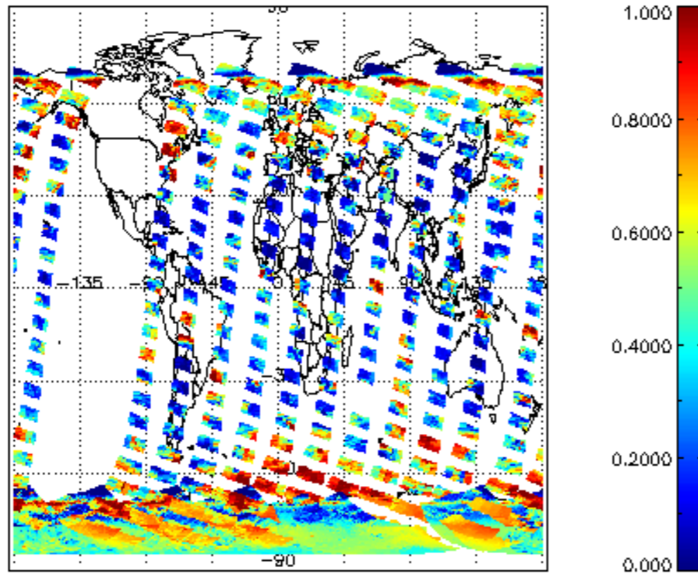
cLfrac for 28NOV2004 00:00:00 to 29NOV2004 00:00:00
