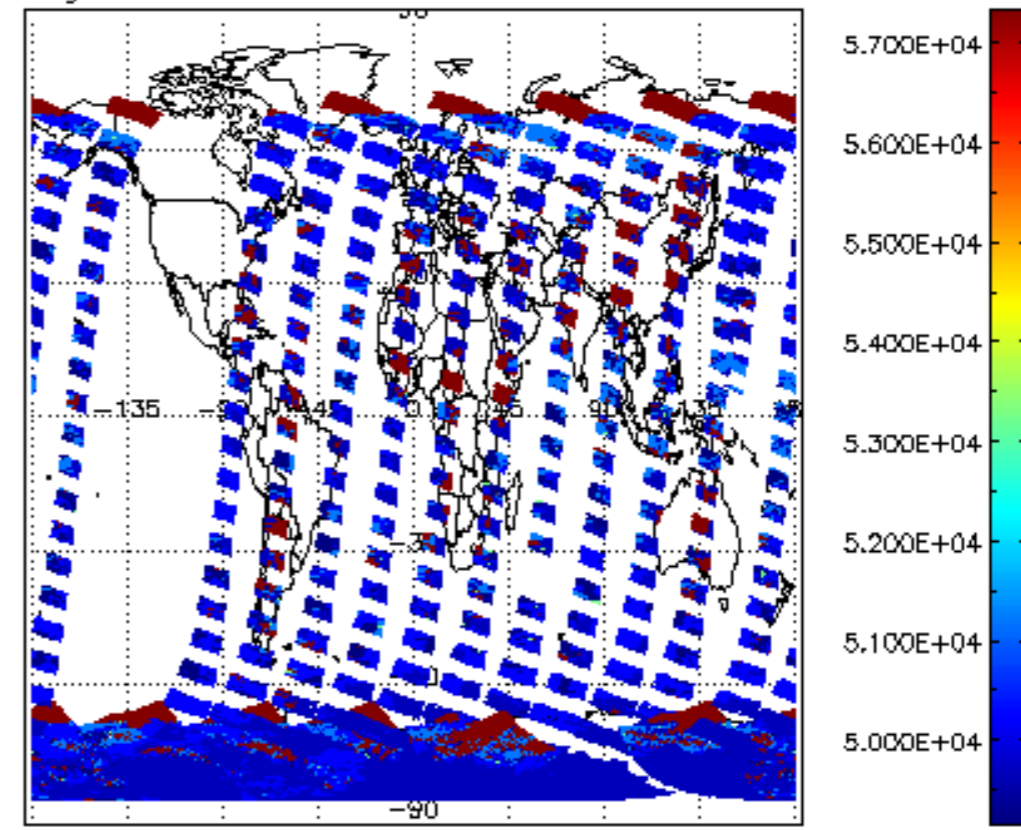
cloud_flags for 28NOV2004 00:00:00 to 29NOV2004 00:00:00
