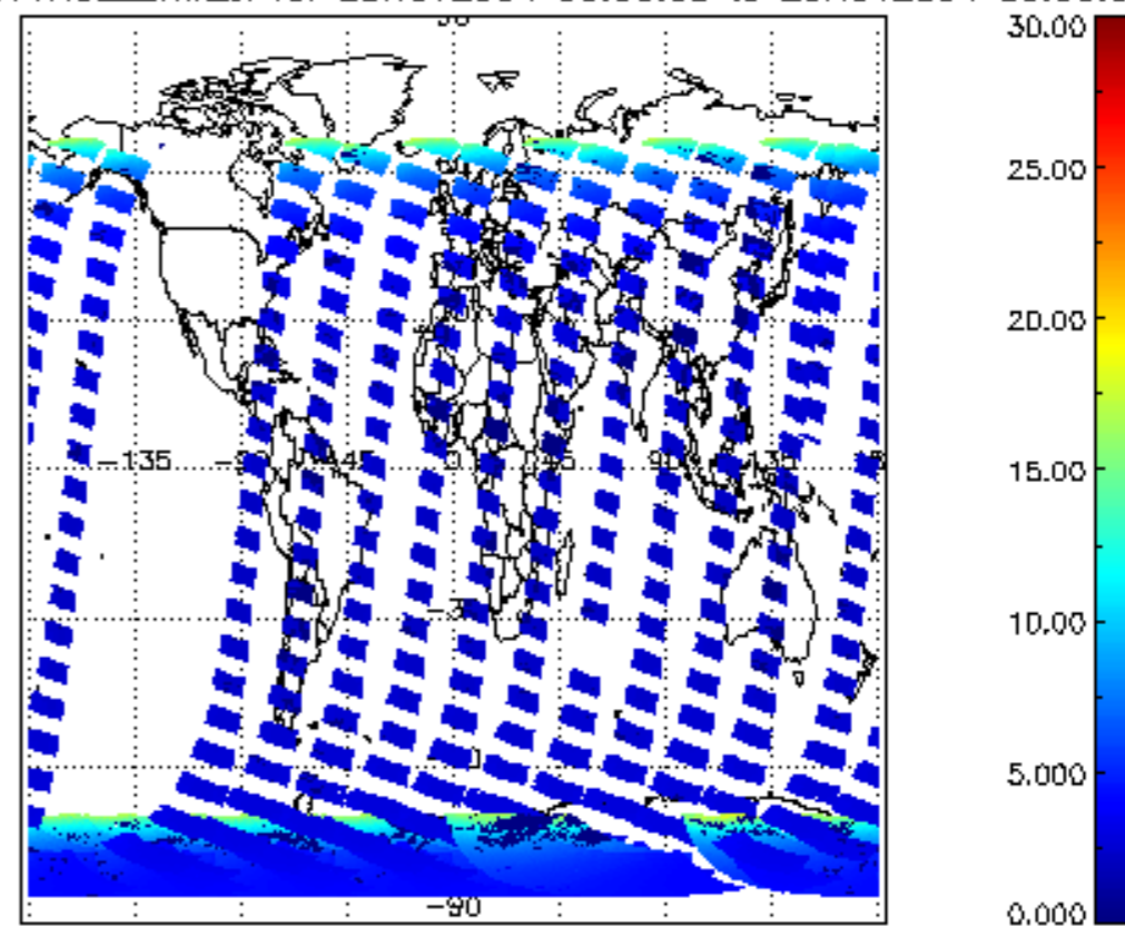
SCIOL2P_NADUV1NO2_amf_cl for 28NOV2004 00:00:00 to 29NOV2004 00:00:00
