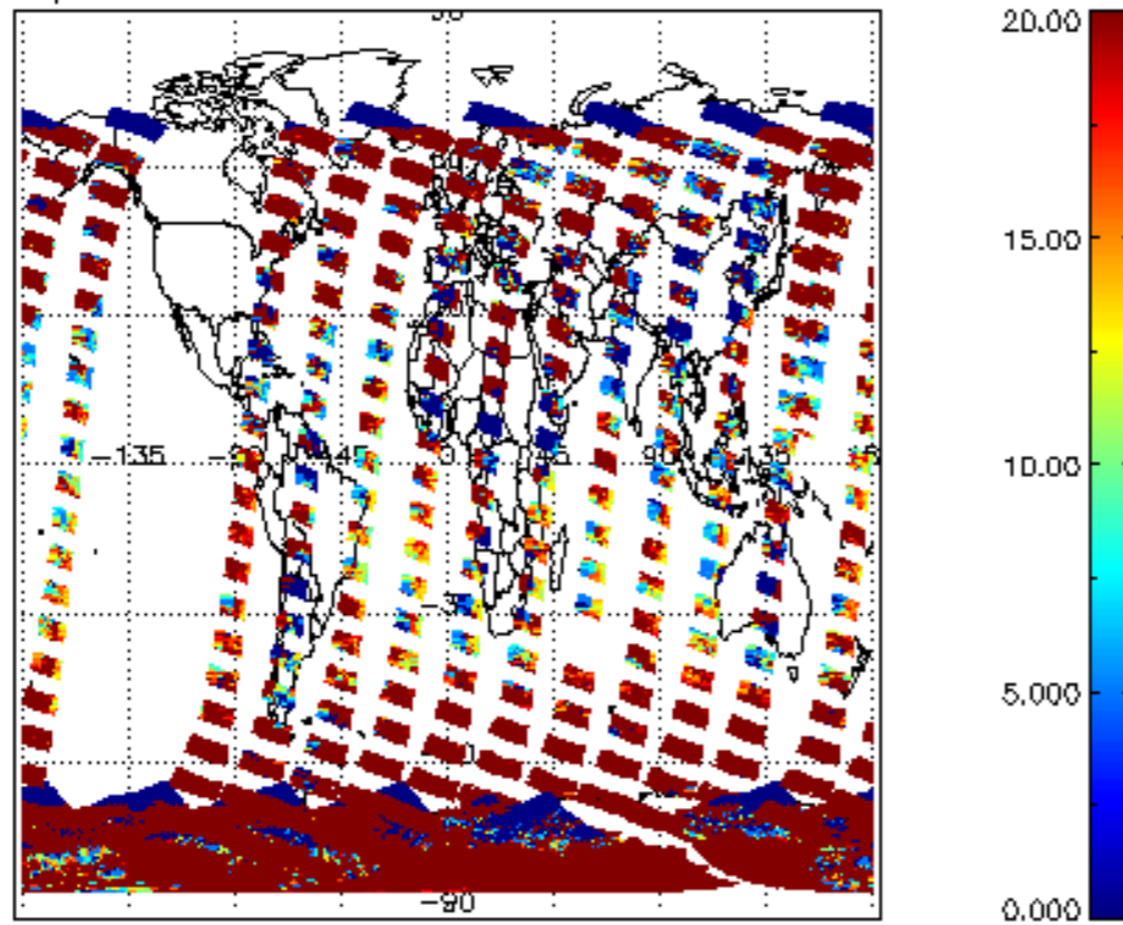
cL_opt_depth for 28NOV2004 00:00:00 to 29NOV2004 00:00:00
