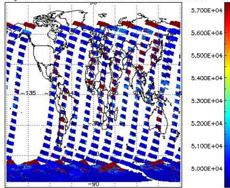
cloud_flags for 28NOV2004 00:00:00 to 29NOV2004 00:00:00
