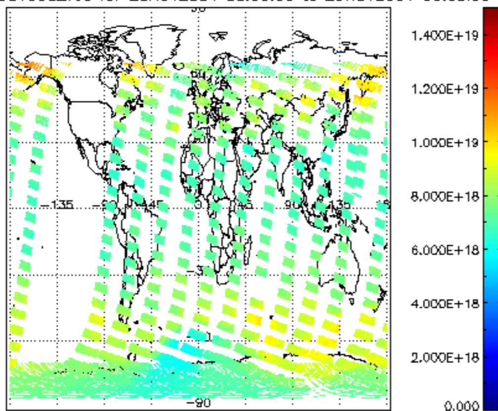
SCIOL2P_NADUV003_vcd for 28NOV2004 00:00:00 to 29NOV2004 00:00:00
