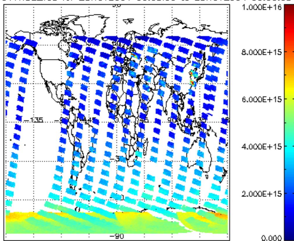
SCIOL2P_NADUV1NO2_vcd for 28NOV2004 00:00:00 to 29NOV2004 00:00:00
