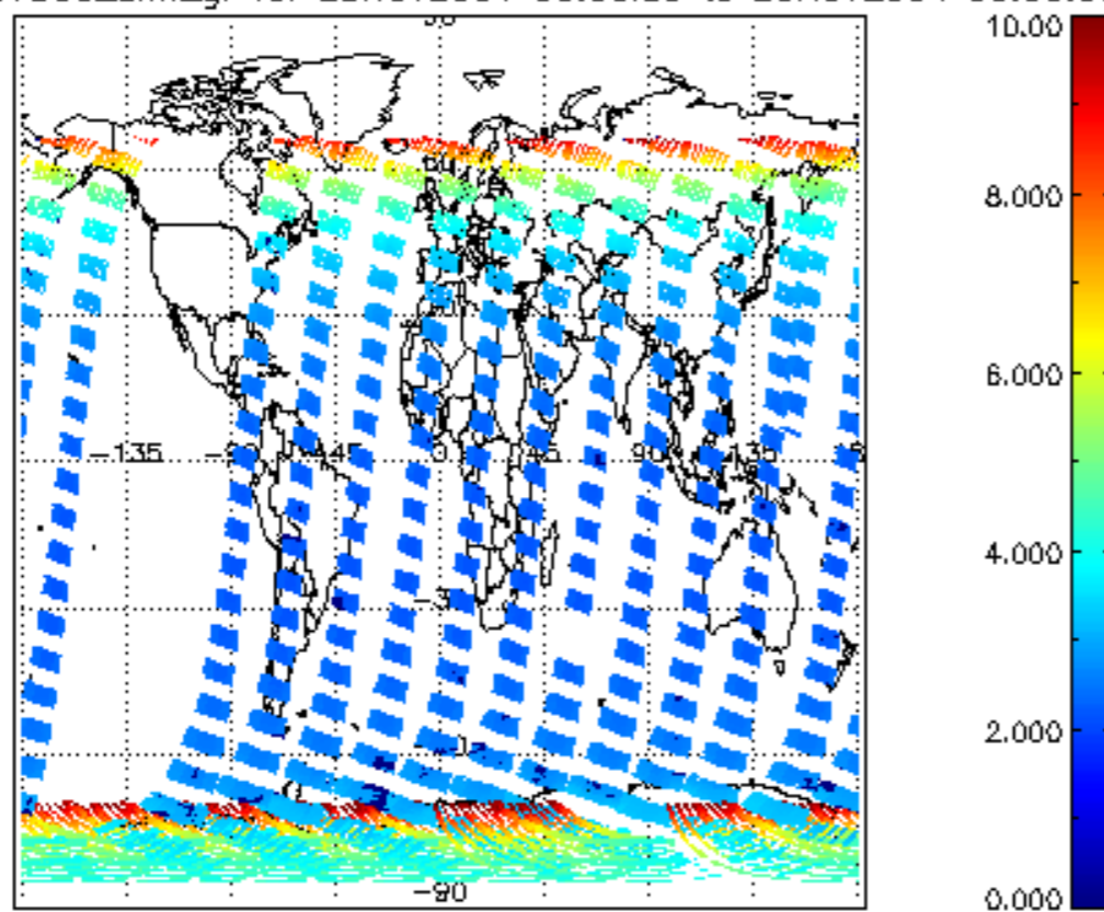
SCIOL2P_NADUV003_amf_gr for 28NOV2004 00:00:00 to 29NOV2004 00:00:00
