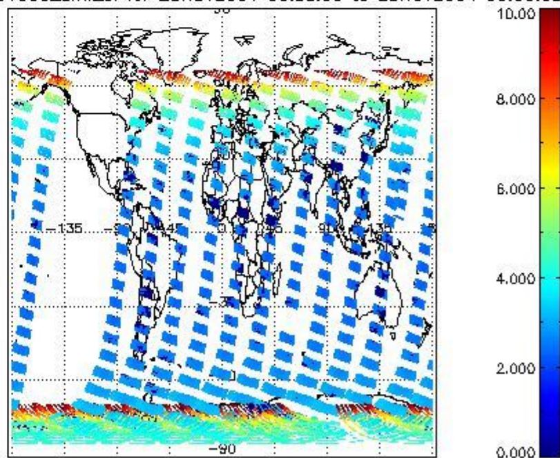
SCIOL2P_NADUV003_amf_cl for 28NOV2004 00:00:00 to 29NOV2004 00:00:00
