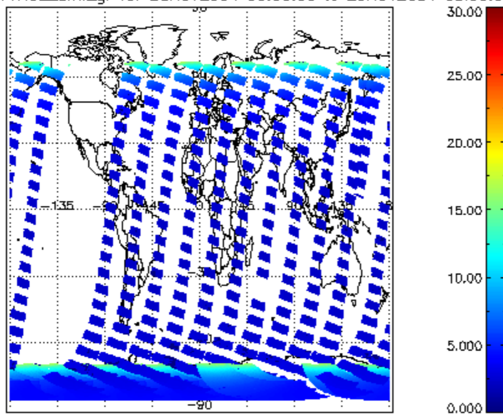
SCIOL2P_NADUV1NO2_amf_gr for 28NOV2004 00:00:00 to 29NOV2004 00:00:00
