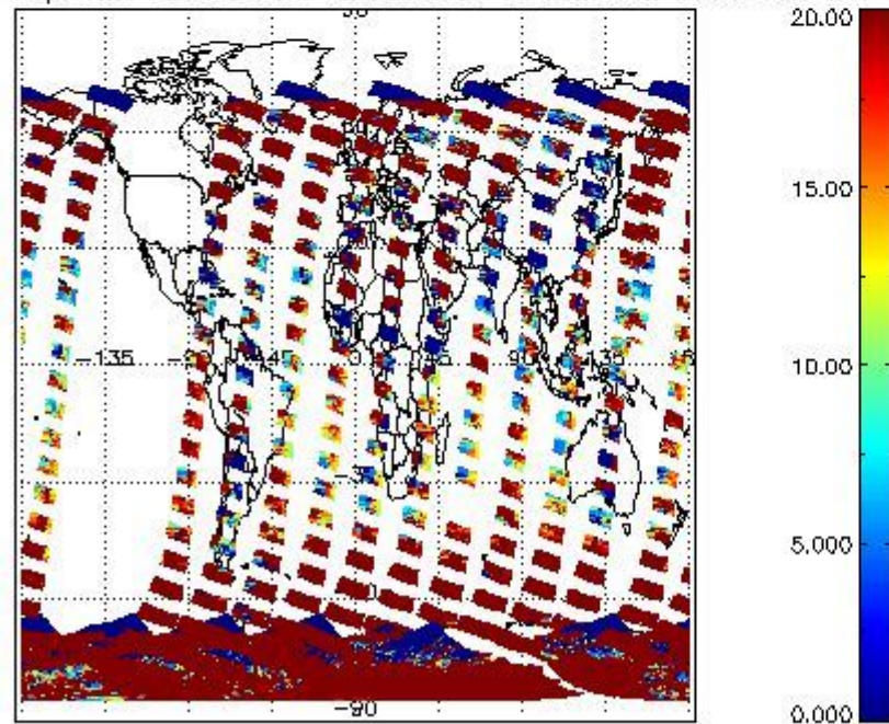
cLopt_depth for 28NOV2004 00:00:00 to 29NOV2004 00:00:00
