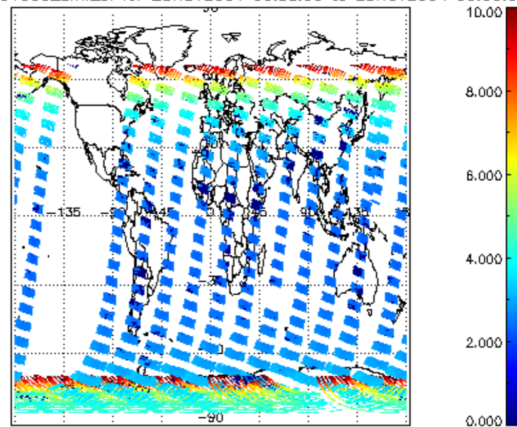
SCIOL2P_NADUV003_amf_cl for 28NOV2004 00:00:00 to 29NOV2004 00:00:00
