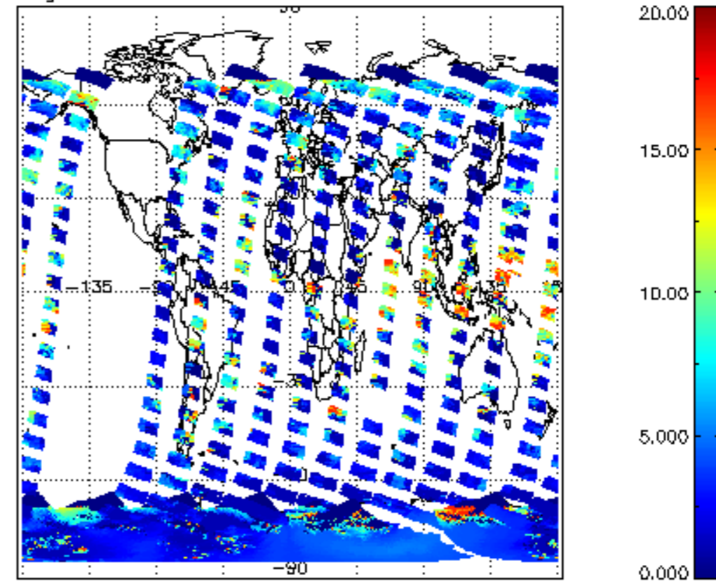
cL_top_height for 28NOV2004 00:00:00 to 29NOV2004 00:00:00
