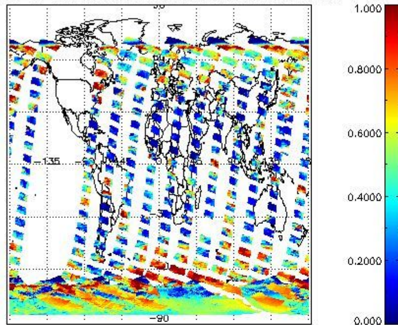
cLfrac for 28NOV2004 00:00:00 to 29NOV2004 00:00:00
