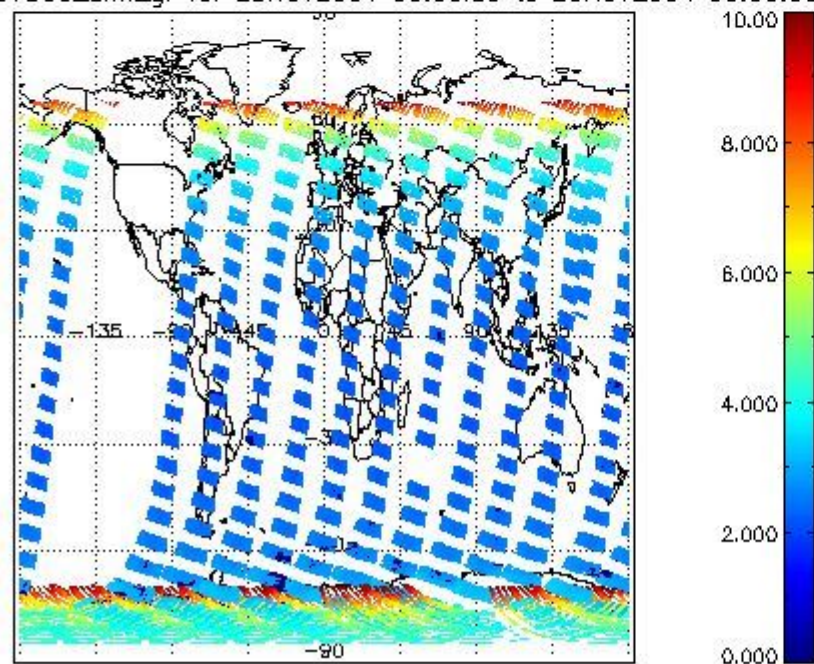
SCIOL2P_NADUV003_amf_gr for 28NOV2004 00:00:00 to 29NOV2004 00:00:00
