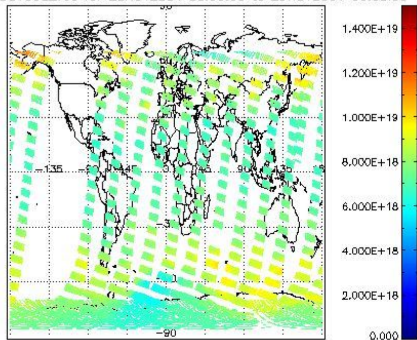
SCIOL2P_NADUV003_vcd for 28NOV2004 00:00:00 to 29NOV2004 00:00:00
