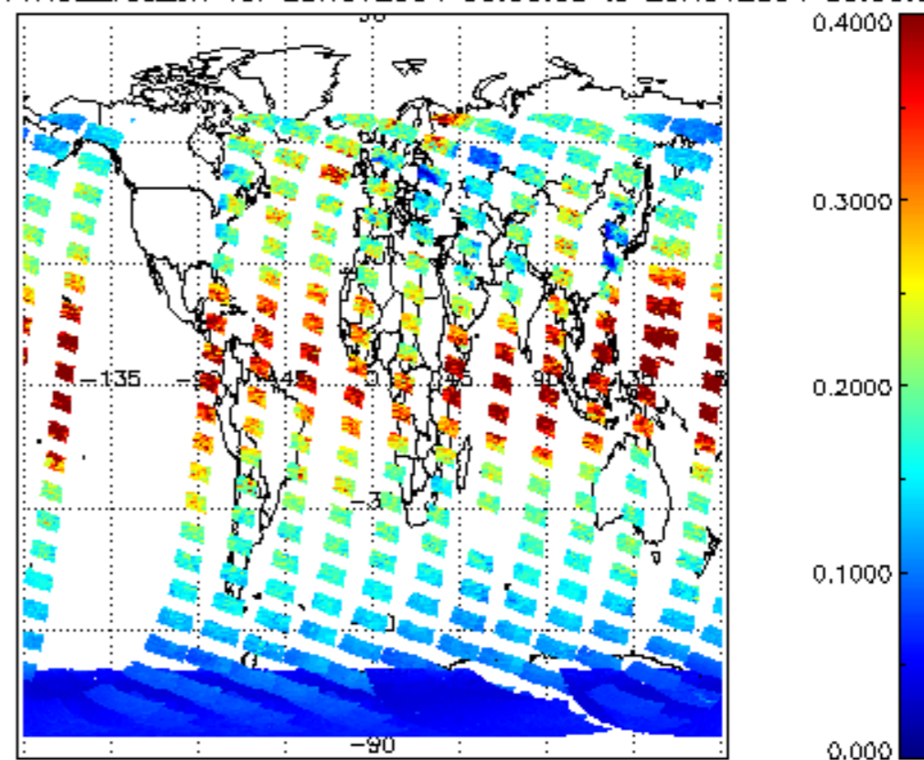
SCIOL2P_NADUV1NO2_vcd_err for 28NOV2004 00:00:00 to 29NOV2004 00:00:00
