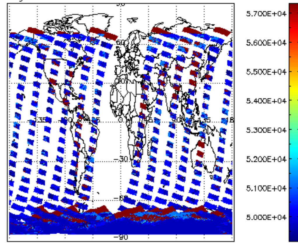
cloud_flags for 27NOV2004 00:00:00 to 28NOV2004 00:00:00
