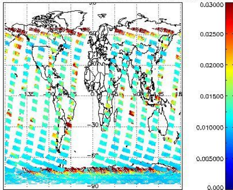
SCIOL2P_NADUV003_vcd_err for 27NOV2004 00:00:00 to 28NOV2004 00:00:00
