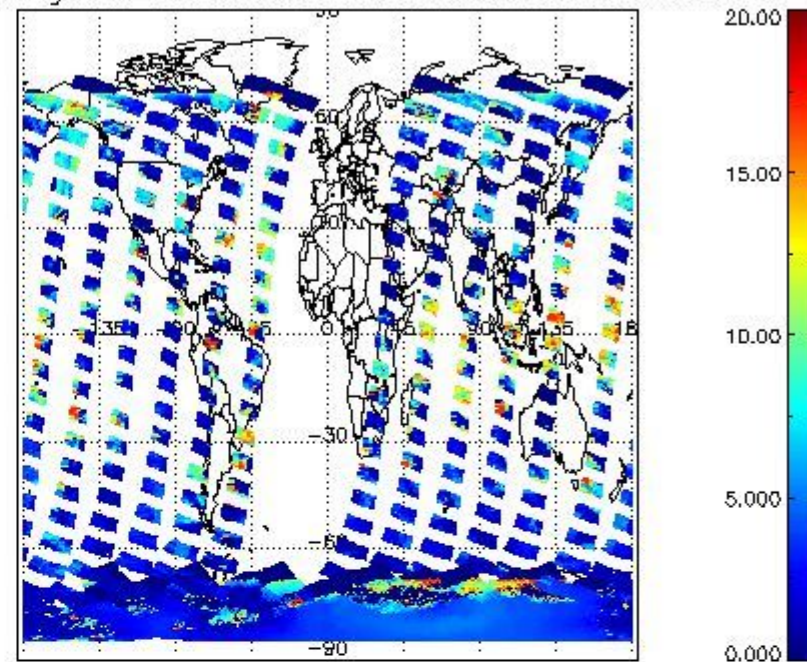
cL_top_height for 27NOV2004 00:00:00 to 28NOV2004 00:00:00
