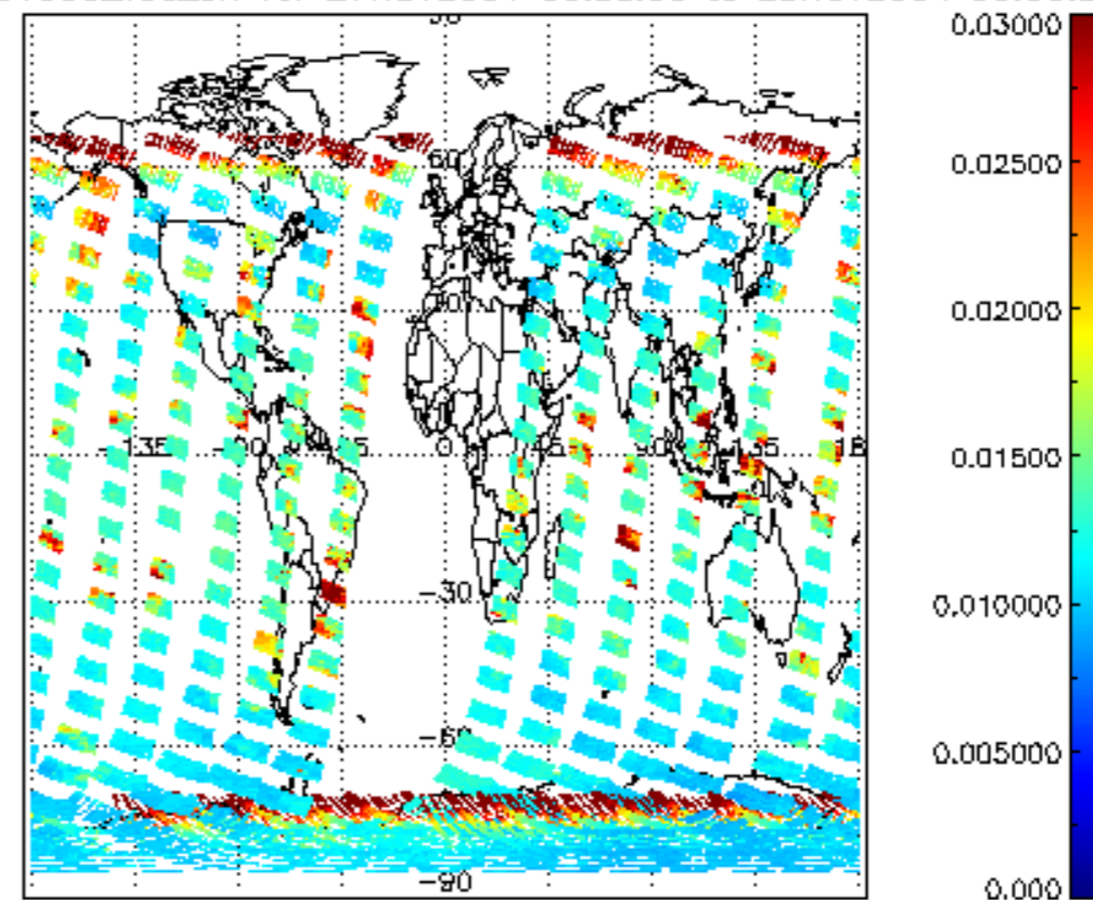
SCIOL2P_NADUV003_vcd_err for 27NOV2004 00:00:00 to 28NOV2004 00:00:00
