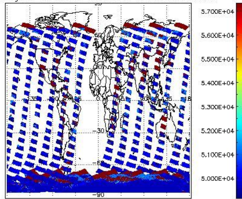
cloud_flags for 27NOV2004 00:00:00 to 28NOV2004 00:00:00
