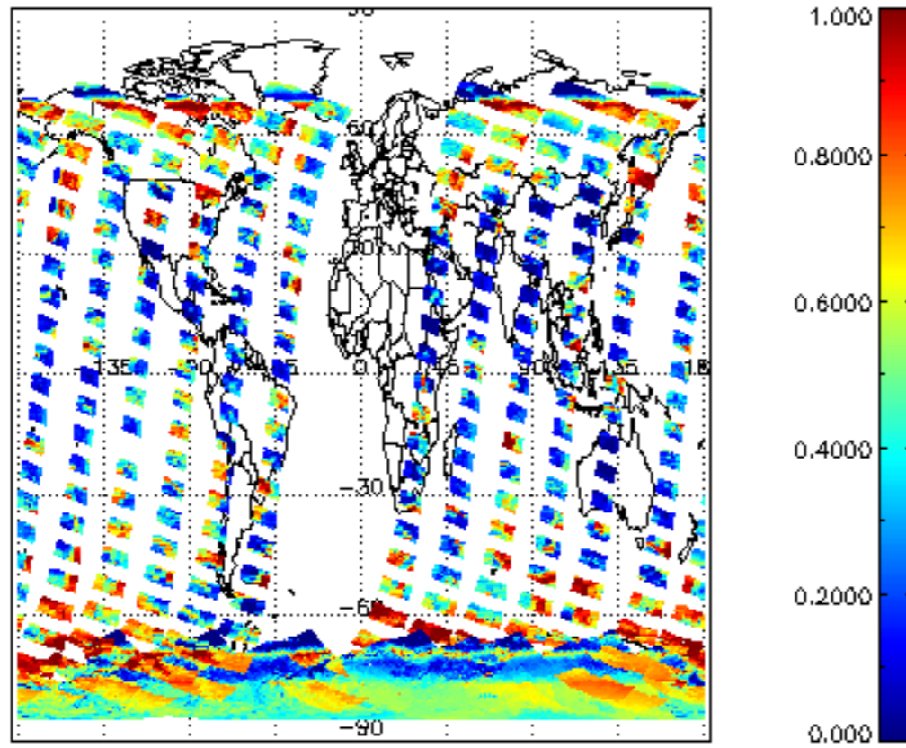
cLfrac for 27NOV2004 00:00:00 to 28NOV2004 00:00:00
