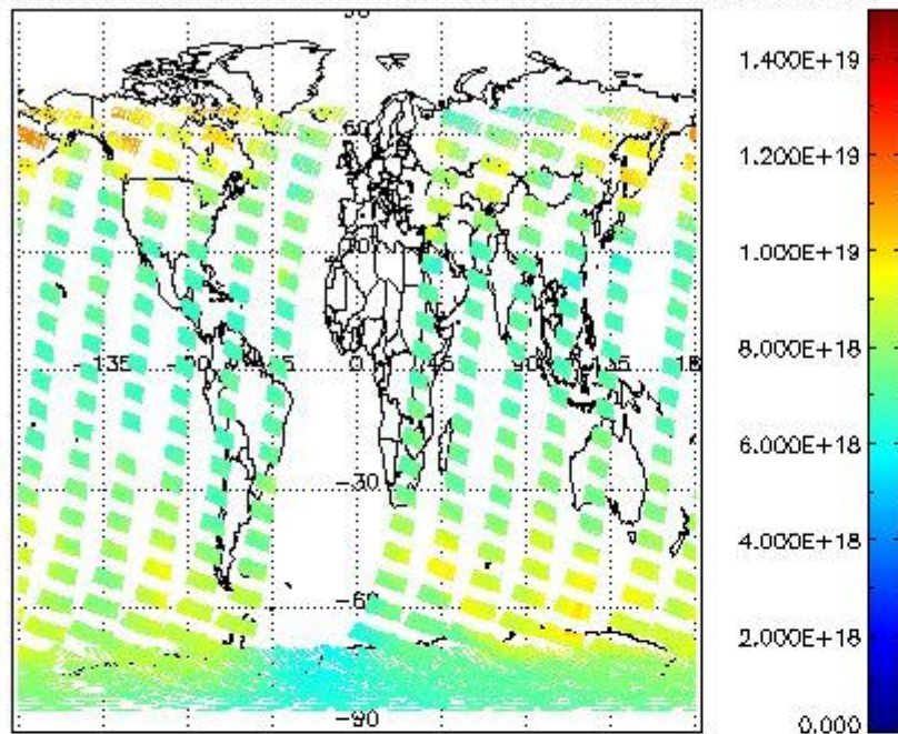
SCIOL2P_NADUV003_vcd for 27NOV2004 00:00:00 to 28NOV2004 00:00:00
