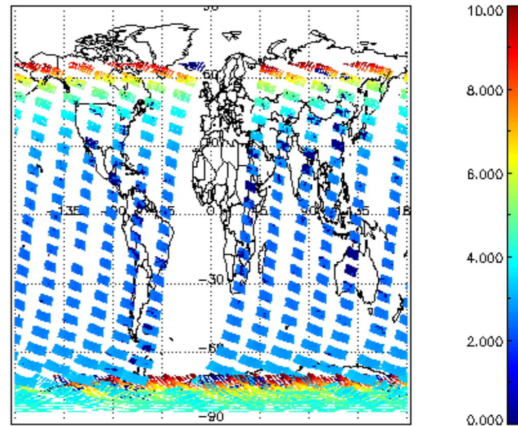
SCIOL2P_NADUV003_amf_cl for 27NOV2004 00:00:00 to 28NOV2004 00:00:00
