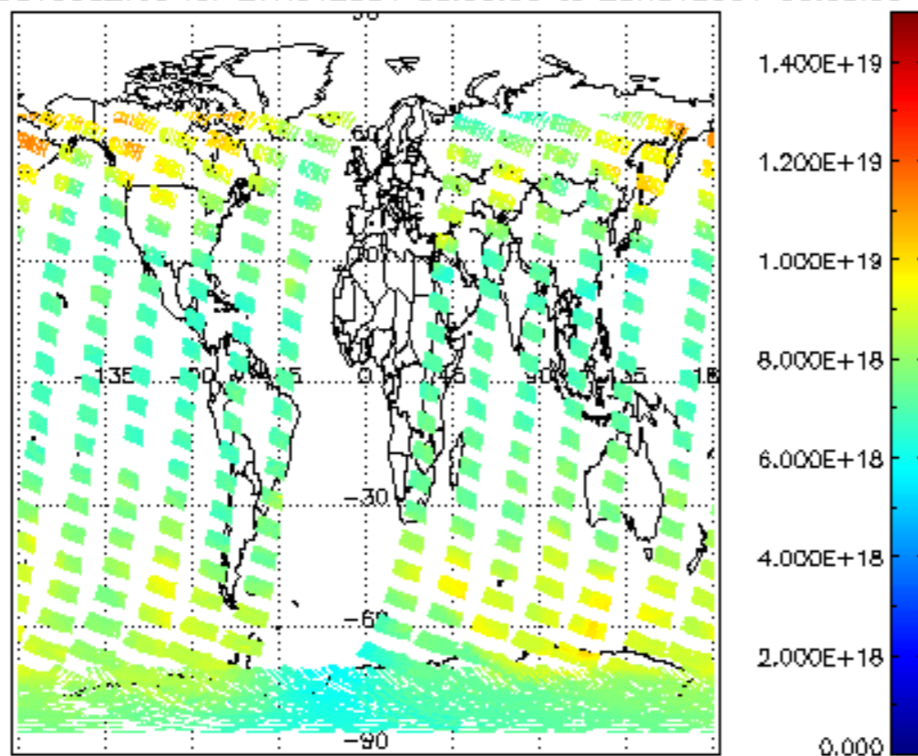
SCIOL2P_NADUV003_vcd for 27NOV2004 00:00:00 to 28NOV2004 00:00:00
