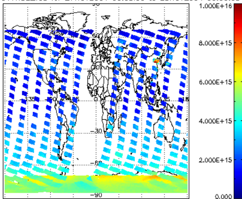
SCIOL2P_NADUV1NO2_vcd for 27NOV2004 00:00:00 to 28NOV2004 00:00:00
