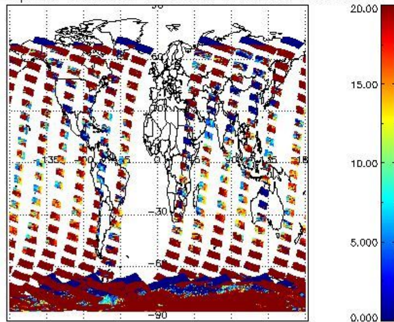
cLopt_depth for 27NOV2004 00:00:00 to 28NOV2004 00:00:00
