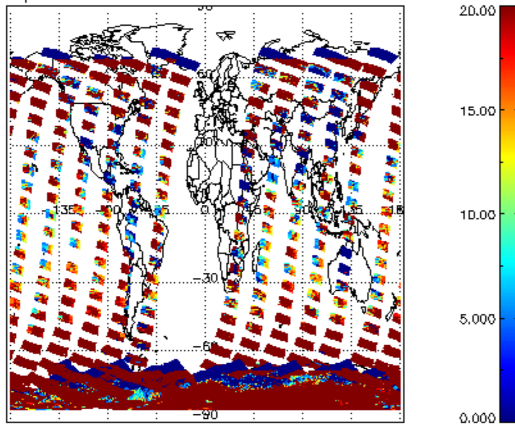
cL_opt_depth for 27NOV2004 00:00:00 to 28NOV2004 00:00:00
