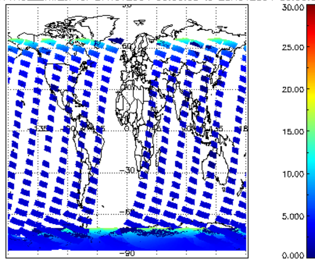
SCIOL2P_NADUV1NO2_amf_cl for 27NOV2004 00:00:00 to 28NOV2004 00:00:00
