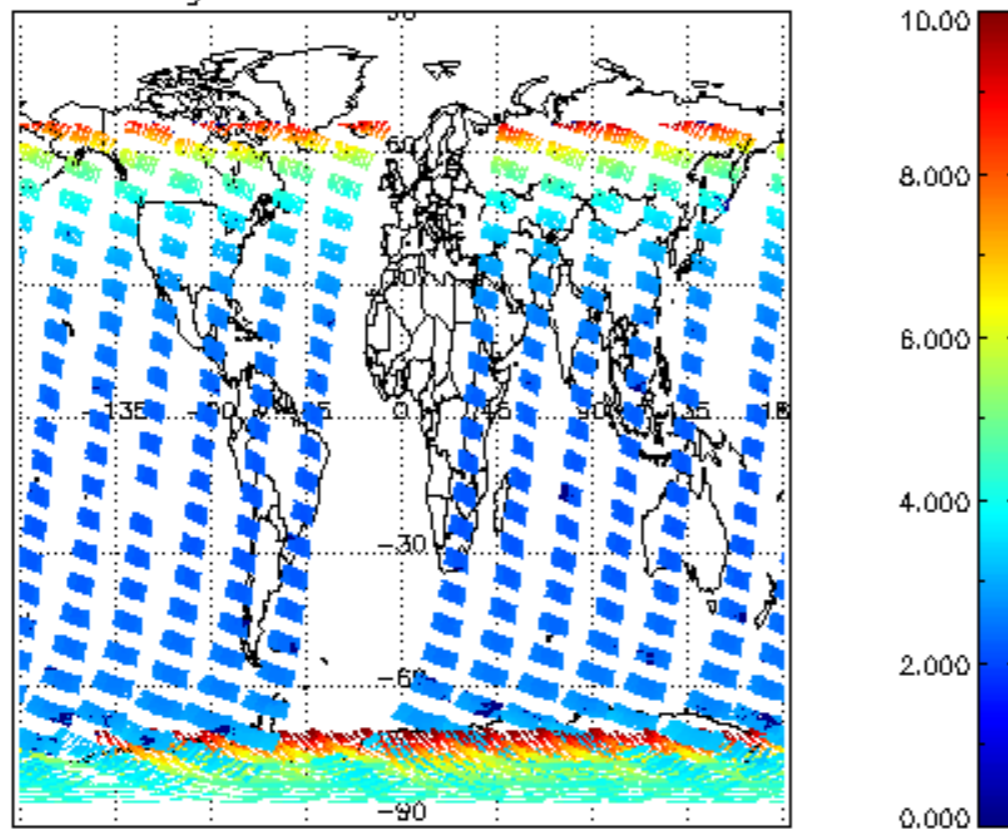
SCIOL2P_NADUV003_amf_gr for 27NOV2004 00:00:00 to 28NOV2004 00:00:00
