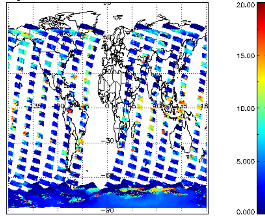
cL_top_height for 27NOV2004 00:00:00 to 28NOV2004 00:00:00
