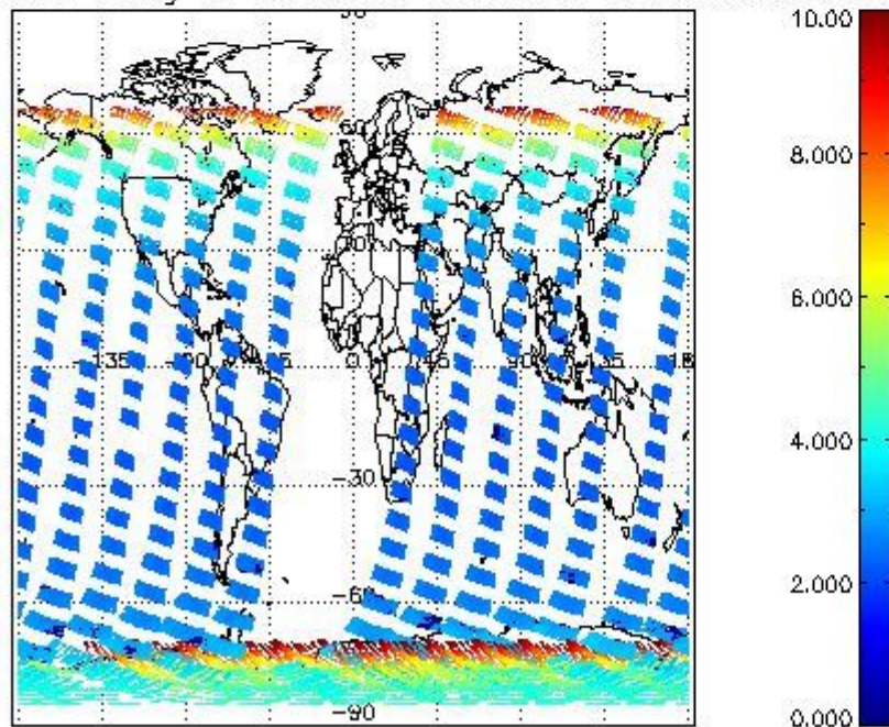
SCIOL2P_NADUV003_amf_gr for 27NOV2004 00:00:00 to 28NOV2004 00:00:00
