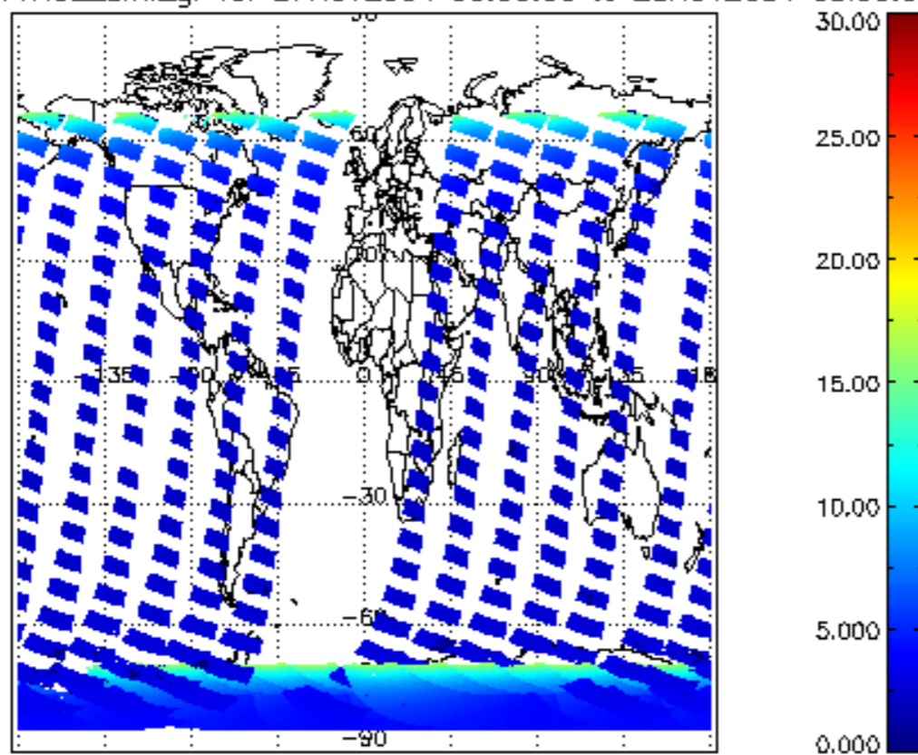
SCIOL2P_NADUV1NO2_amf_gr for 27NOV2004 00:00:00 to 28NOV2004 00:00:00
