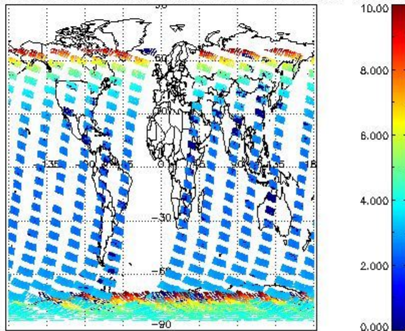
SCIOL2P_NADUV003_amf_cl for 27NOV2004 00:00:00 to 28NOV2004 00:00:00
