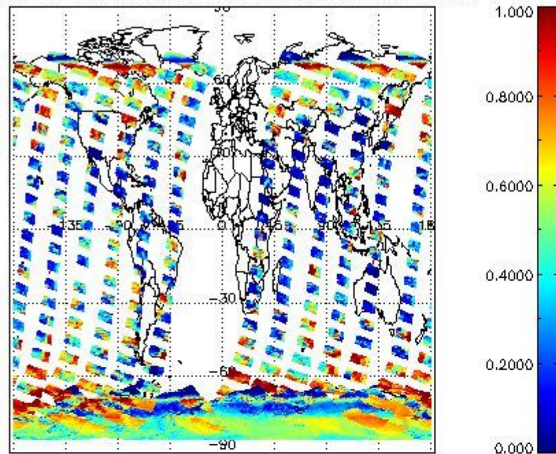
cLfrac for 27NOV2004 00:00:00 to 28NOV2004 00:00:00
