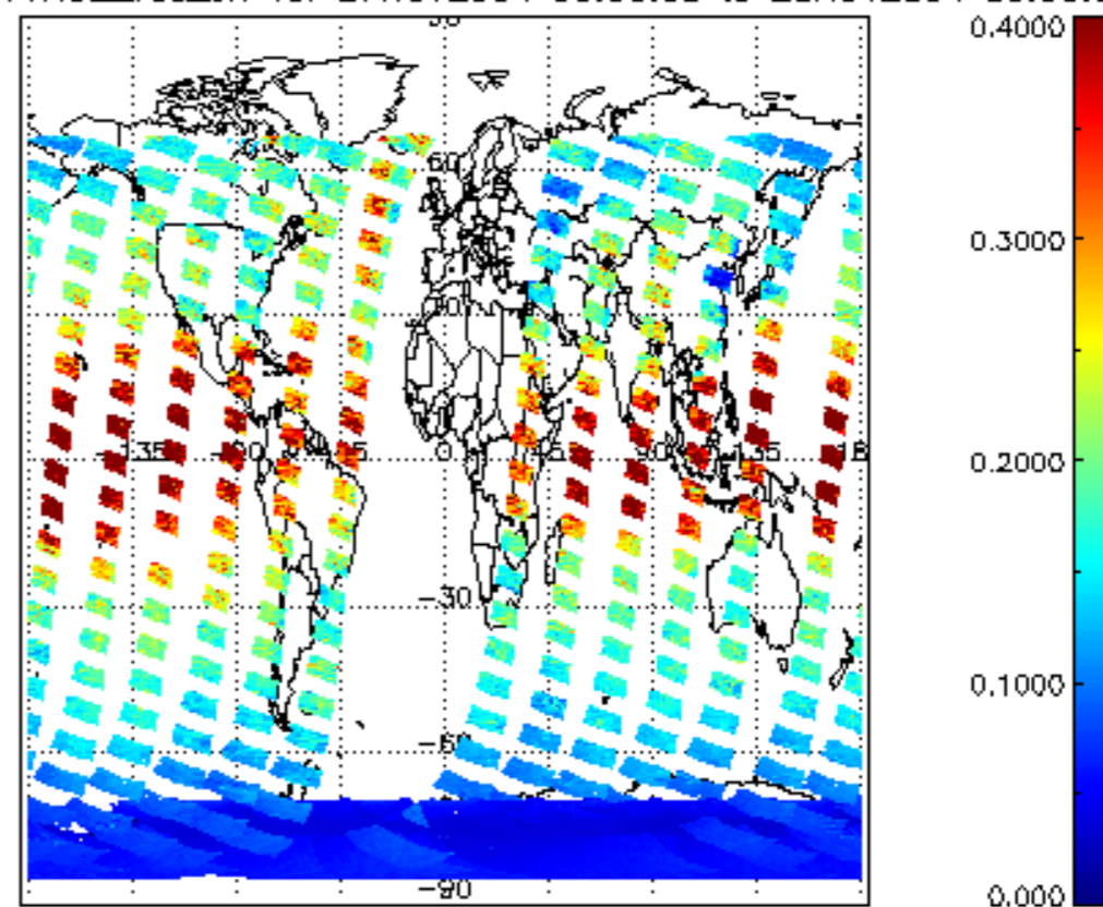
SCIOL2P_NADUV1NO2_vcd_err for 27NOV2004 00:00:00 to 28NOV2004 00:00:00
