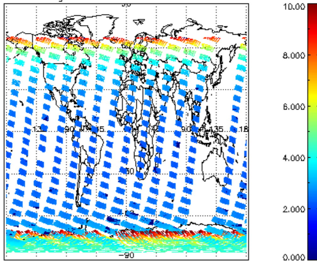
SCIOL2P_NADUV003_amf_gr for 23NOV2004 00:00:00 to 24NOV2004 00:00:00
