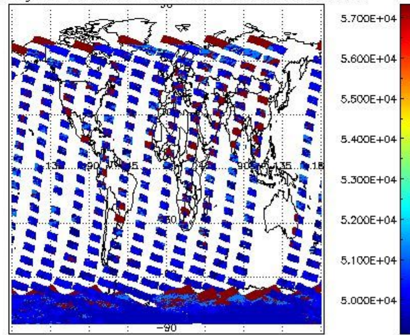
cloud_flags for 23NOV2004 00:00:00 to 24NOV2004 00:00:00
