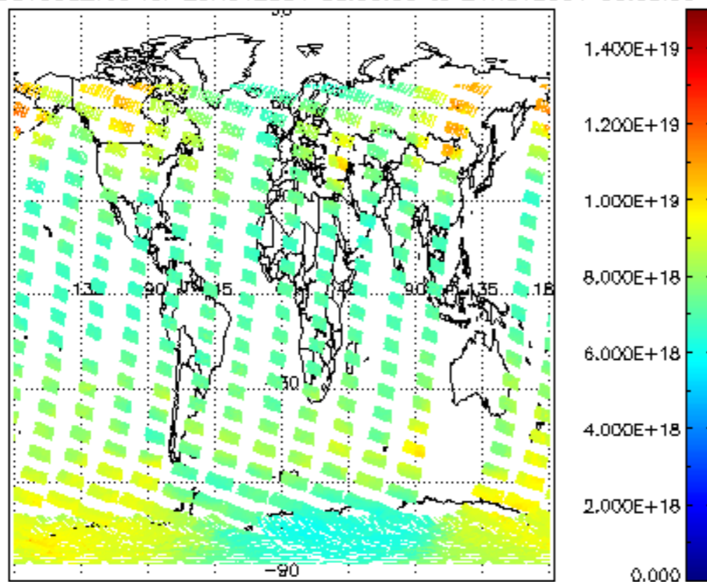
SCIOL2P_NADUV003_vcd for 23NOV2004 00:00:00 to 24NOV2004 00:00:00
