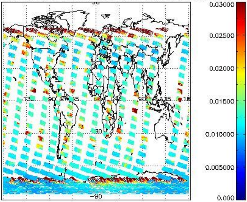
SCIOL2P_NADUV003_vcd_err for 23NOV2004 00:00:00 to 24NOV2004 00:00:00
