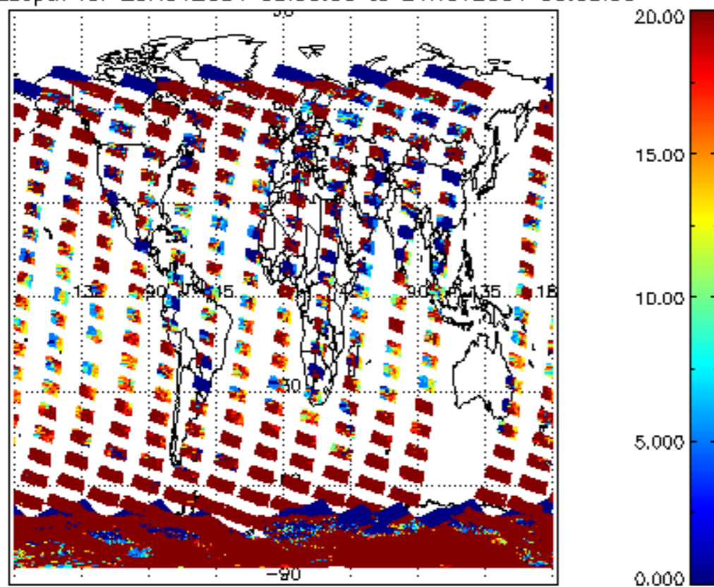
cL_opt_depth for 23NOV2004 00:00:00 to 24NOV2004 00:00:00
