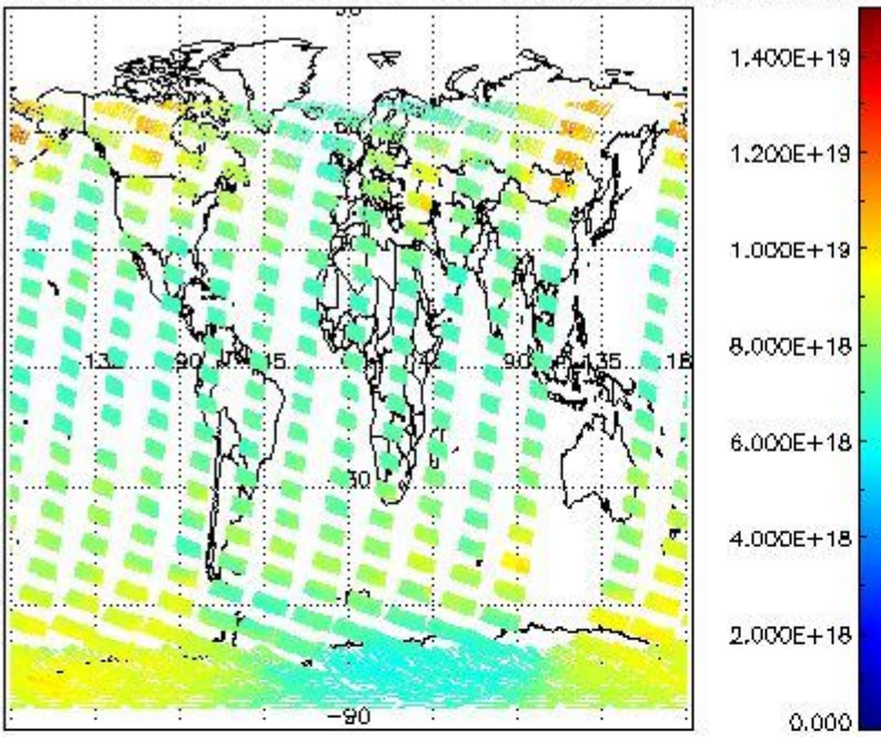
SCIOL2P_NADUV003_vcd for 23NOV2004 00:00:00 to 24NOV2004 00:00:00
