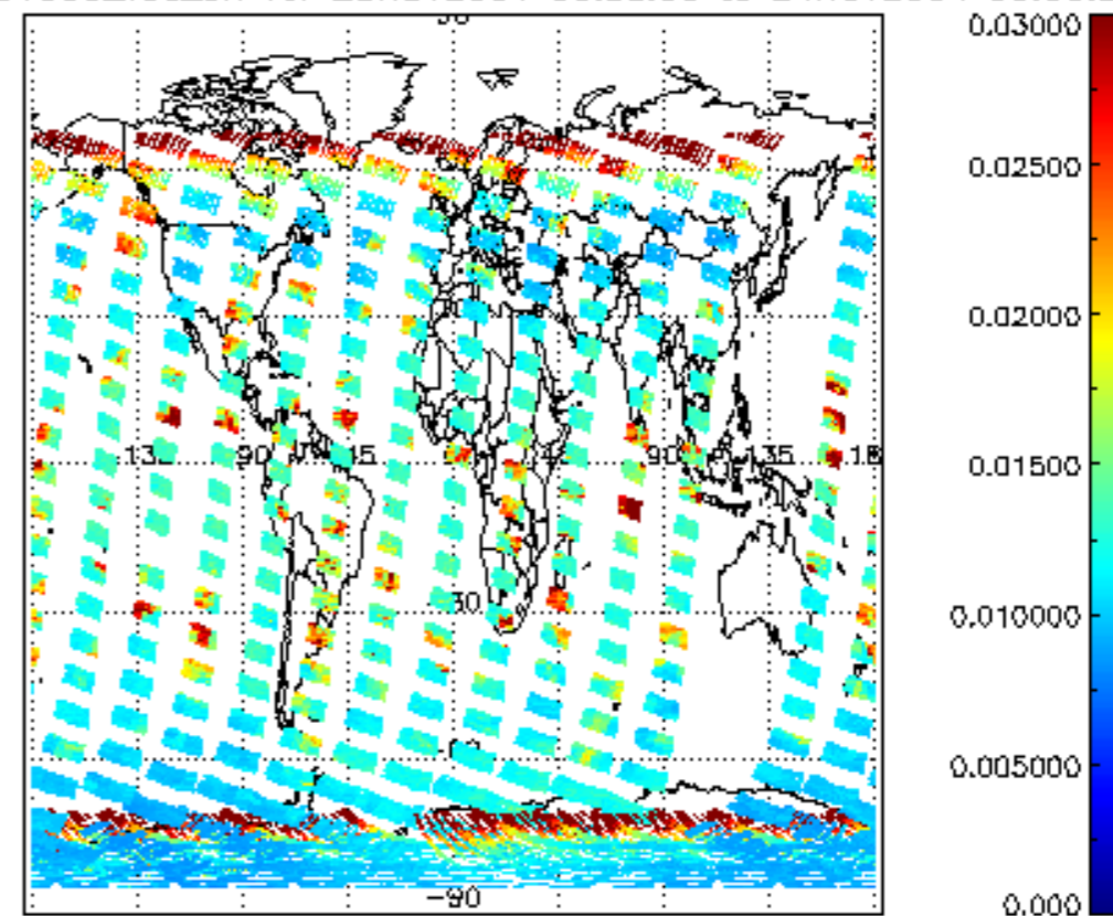
SCIOL2P_NADUV003_vcd_err for 23NOV2004 00:00:00 to 24NOV2004 00:00:00
