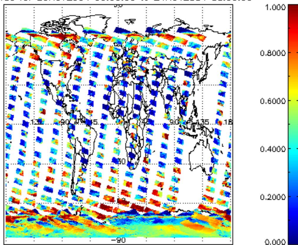
cLfrac for 23NOV2004 00:00:00 to 24NOV2004 00:00:00
