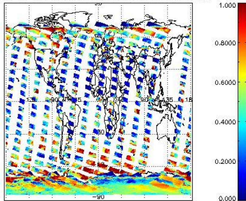
cLfrac for 23NOV2004 00:00:00 to 24NOV2004 00:00:00
