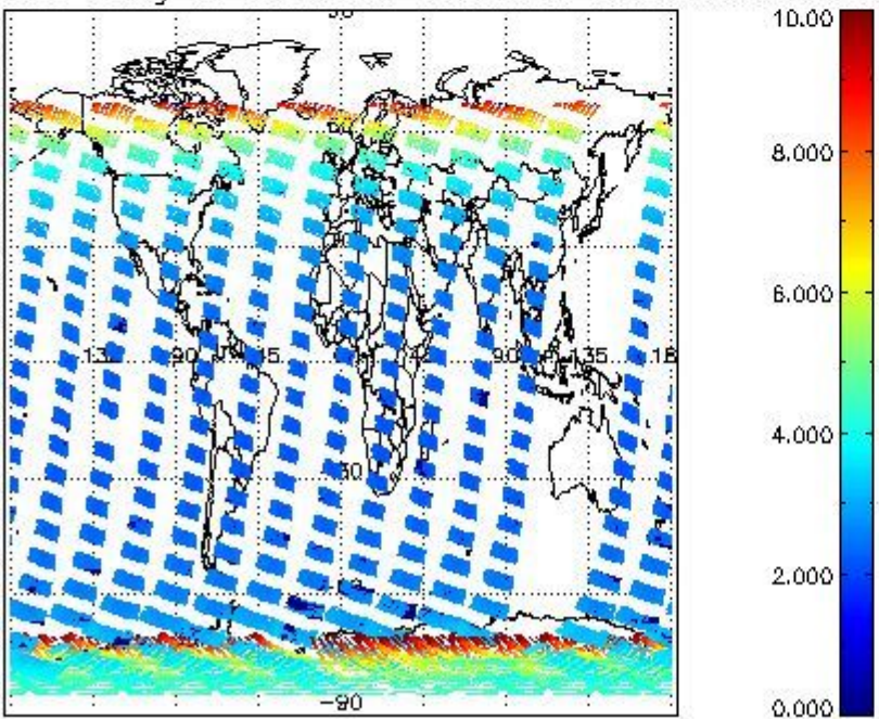
SCIOL2P_NADUV003_amf_gr for 23NOV2004 00:00:00 to 24NOV2004 00:00:00
