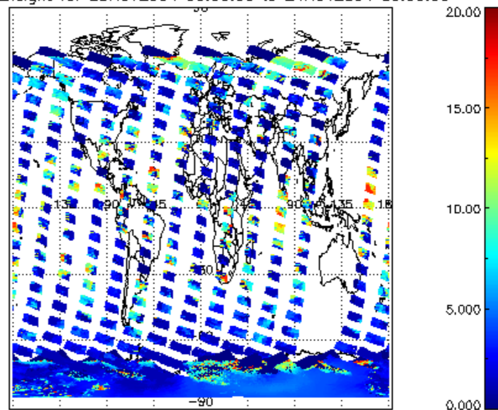
cL_top_height for 23NOV2004 00:00:00 to 24NOV2004 00:00:00
