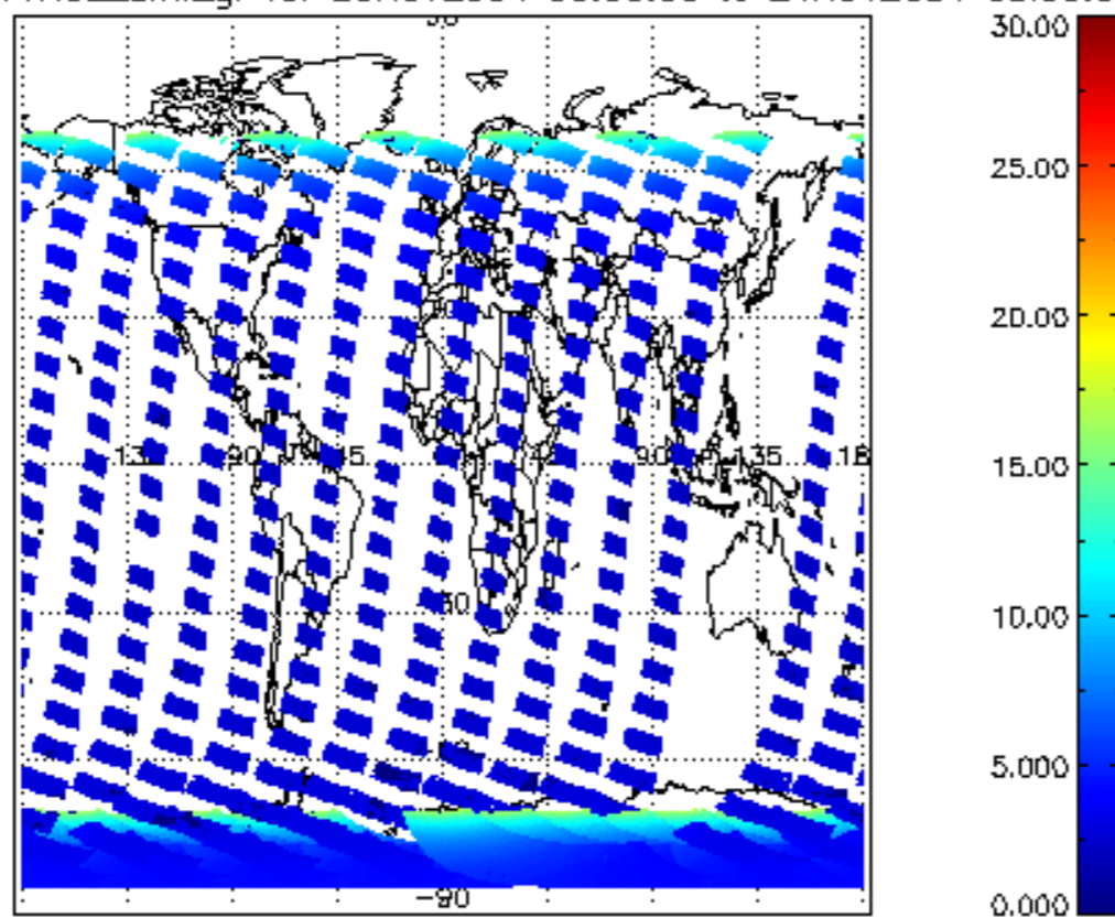
SCIOL2P_NADUV1NO2_amf_gr for 23NOV2004 00:00:00 to 24NOV2004 00:00:00
