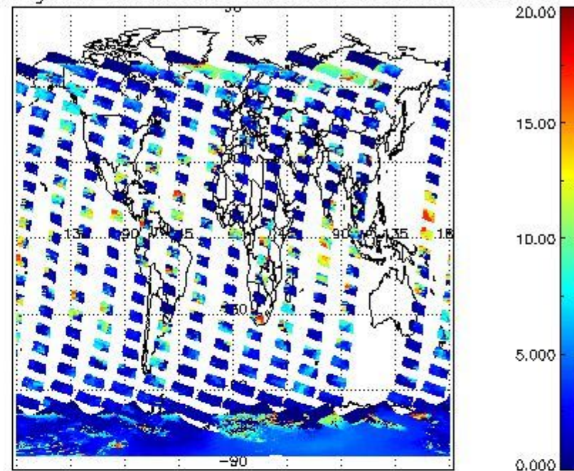
cL_top_height for 23NOV2004 00:00:00 to 24NOV2004 00:00:00
