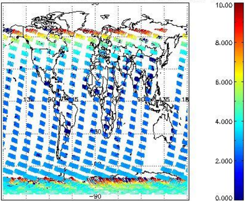
SCIOL2P_NADUV003_amf_cl for 23NOV2004 00:00:00 to 24NOV2004 00:00:00
