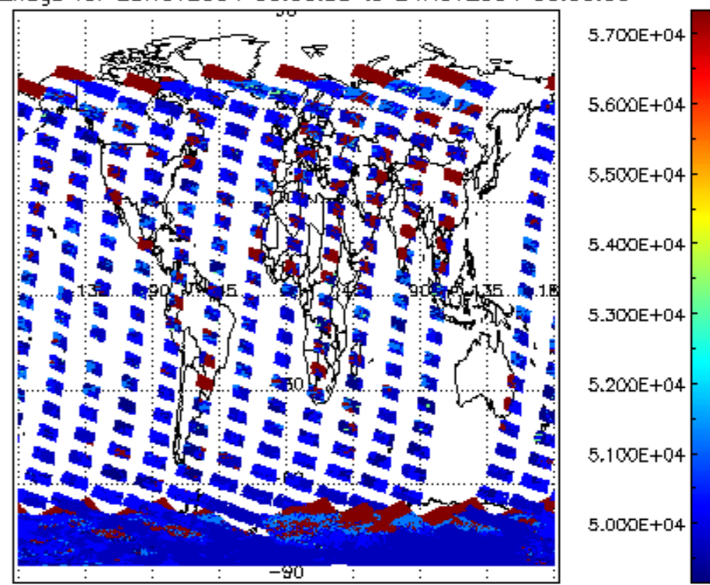
cloud_flags for 23NOV2004 00:00:00 to 24NOV2004 00:00:00
