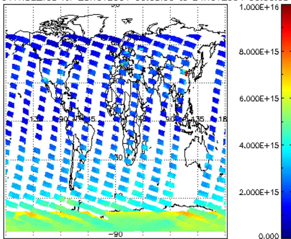
SCIOL2P_NADUV1NO2_vcd for 23NOV2004 00:00:00 to 24NOV2004 00:00:00
