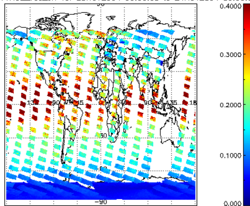
SCIOL2P_NADUV1NO2_vcd_err for 23NOV2004 00:00:00 to 24NOV2004 00:00:00
