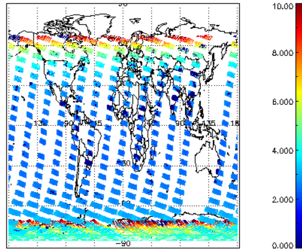
SCIOL2P_NADUV003_amf_cl for 23NOV2004 00:00:00 to 24NOV2004 00:00:00
