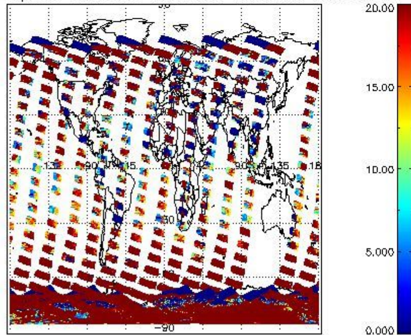
cLopt_depth for 23NOV2004 00:00:00 to 24NOV2004 00:00:00
