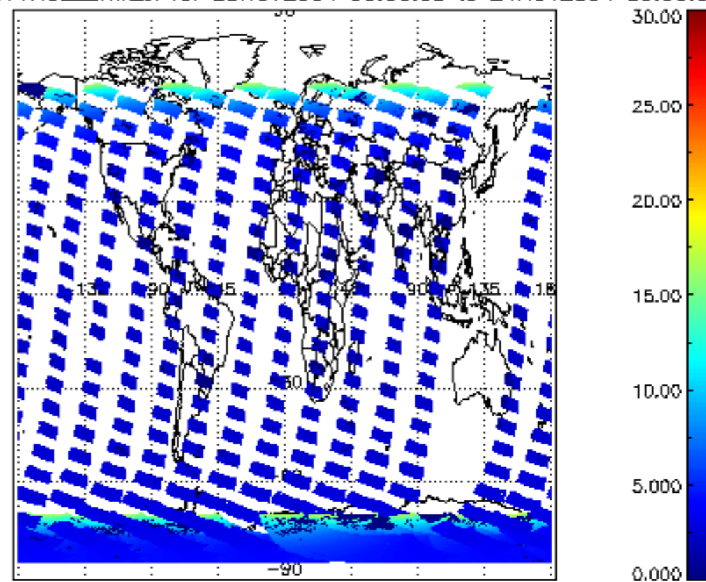
SCIOL2P_NADUV1NO2_amf_cl for 23NOV2004 00:00:00 to 24NOV2004 00:00:00
