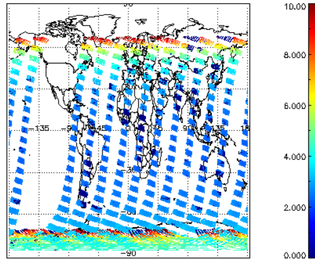
SCIOL2P_NADUV003_amf_cl for 22NOV2004 00:00:00 to 23NOV2004 00:00:00
