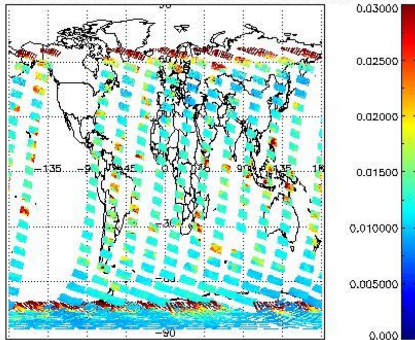
SCIOL2P_NADUV003_vcd_err for 22NOV2004 00:00:00 to 23NOV2004 00:00:00
