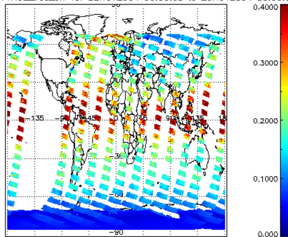
SCIOL2P_NADUV1NO2_vcd_err for 22NOV2004 00:00:00 to 23NOV2004 00:00:00
