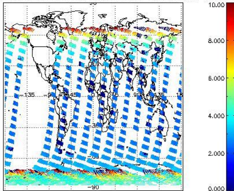
SCIOL2P_NADUV003_amf_cl for 22NOV2004 00:00:00 to 23NOV2004 00:00:00
