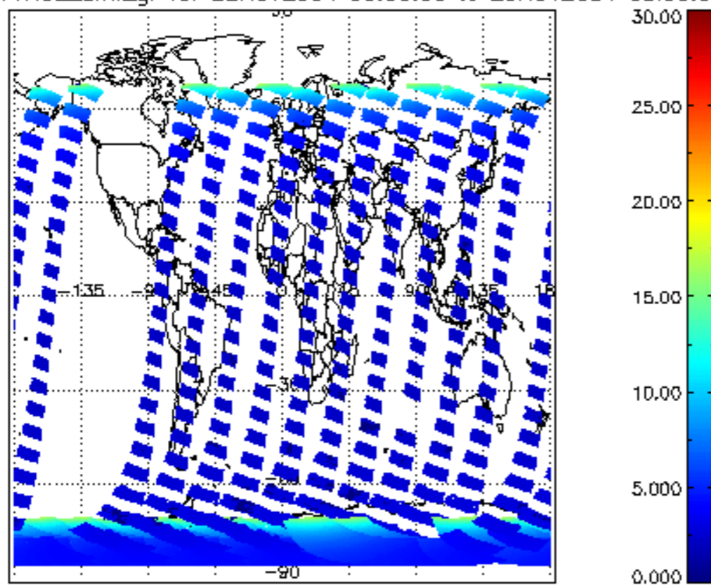
SCIOL2P_NADUV1NO2_amf_gr for 22NOV2004 00:00:00 to 23NOV2004 00:00:00
