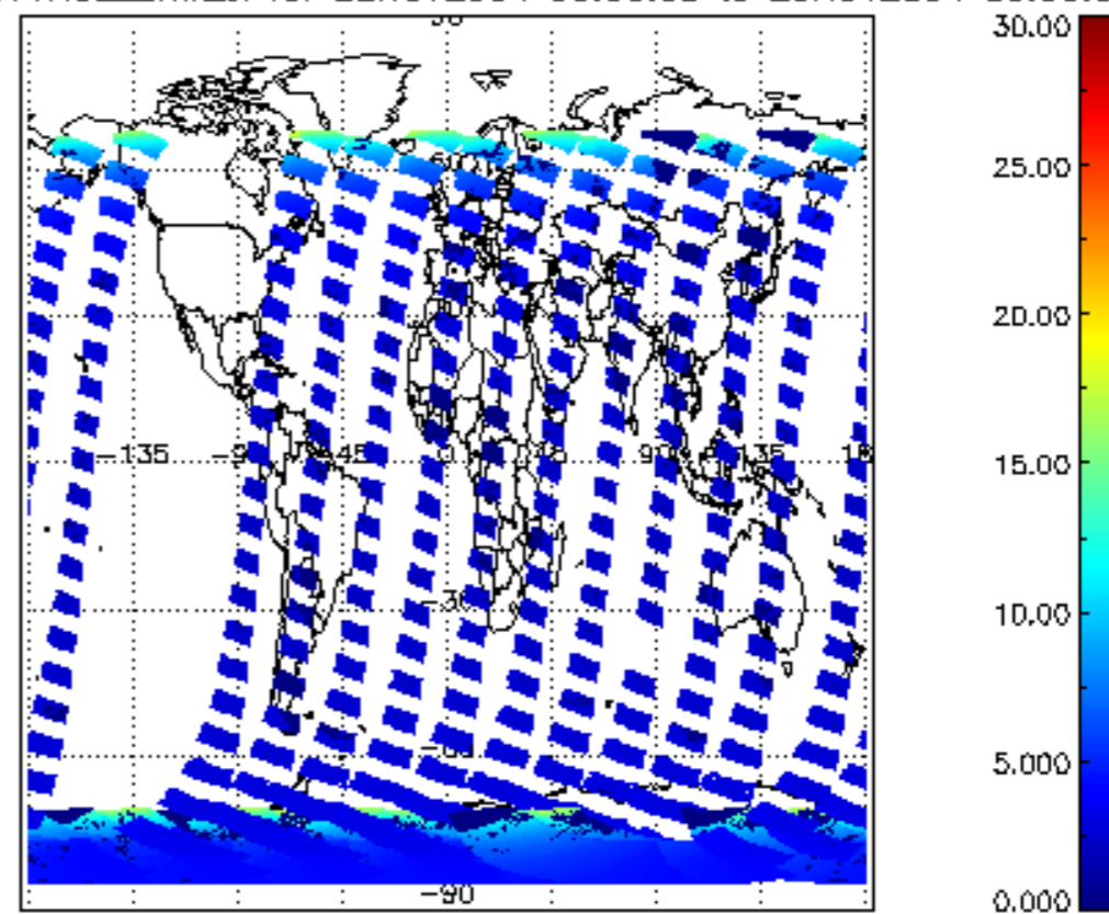
SCIOL2P_NADUV1NO2_amf_cl for 22NOV2004 00:00:00 to 23NOV2004 00:00:00
