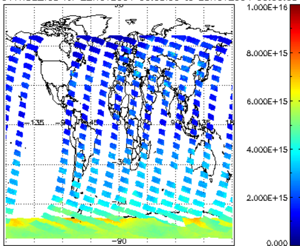
SCIOL2P_NADUV1NO2_vcd for 22NOV2004 00:00:00 to 23NOV2004 00:00:00
