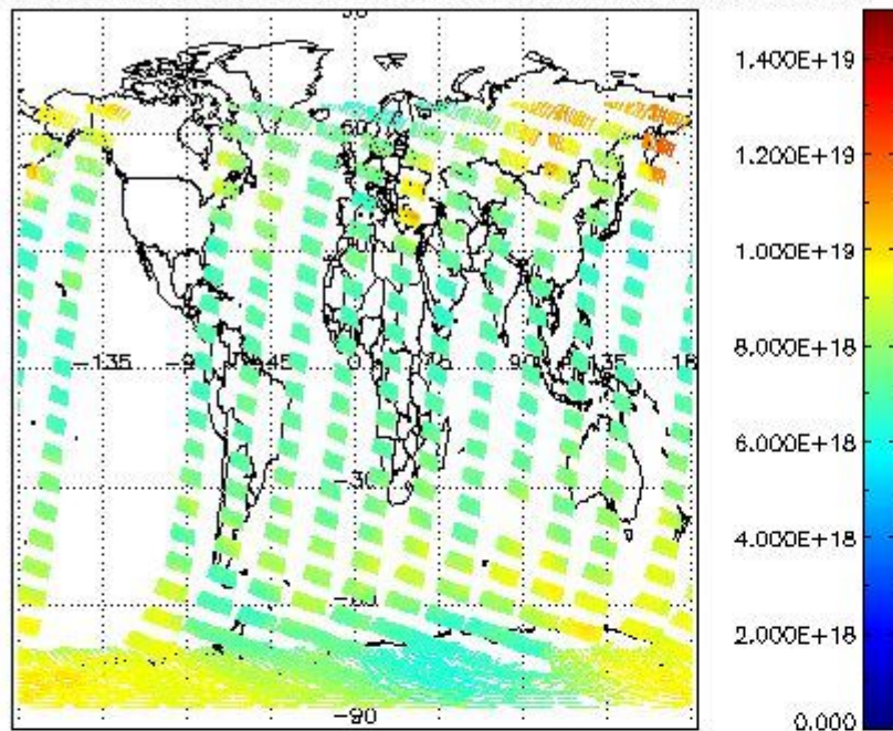
SCIOL2P_NADUV003_vcd for 22NOV2004 00:00:00 to 23NOV2004 00:00:00
