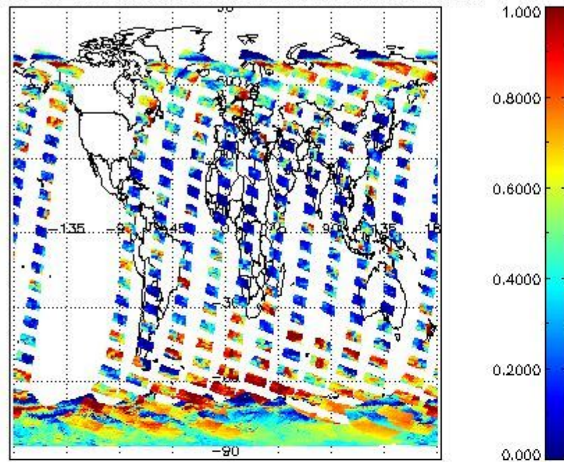
cLfrac for 22NOV2004 00:00:00 to 23NOV2004 00:00:00
