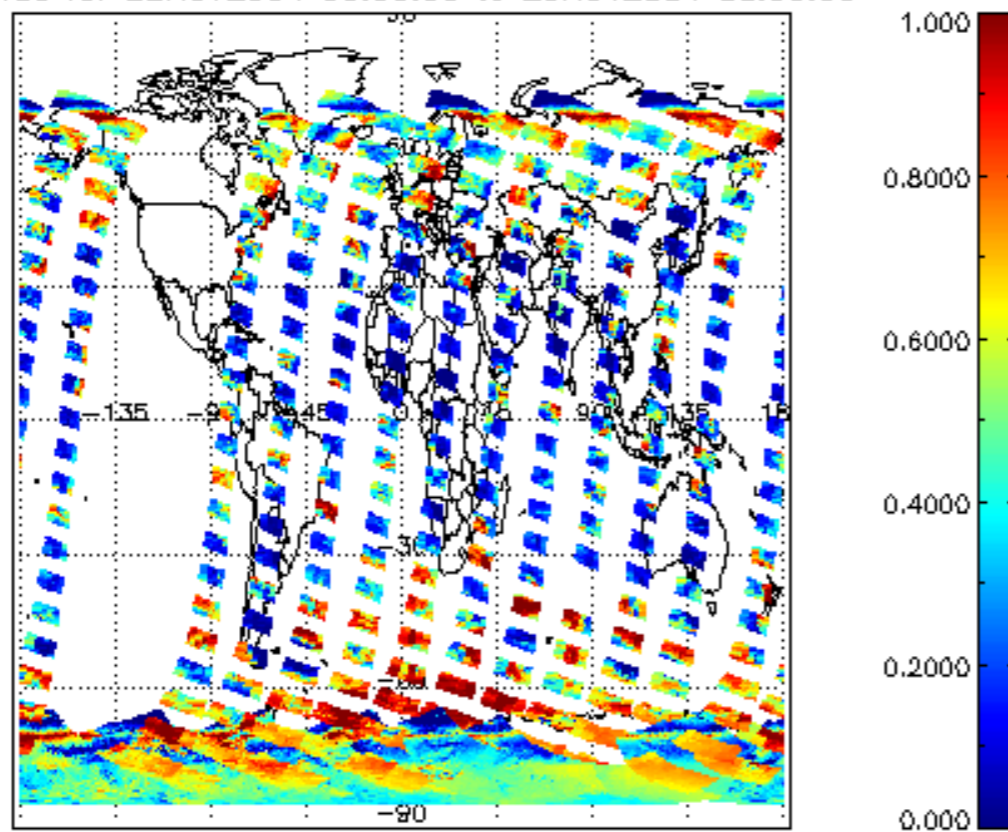
cLfrac for 22NOV2004 00:00:00 to 23NOV2004 00:00:00
