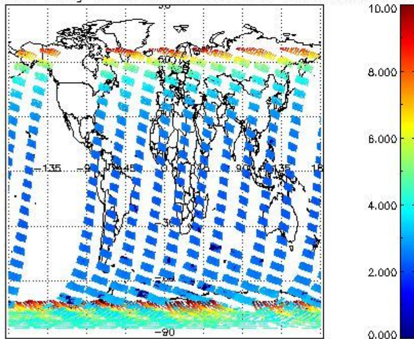
SCIOL2P_NADUV003_amf_gr for 22NOV2004 00:00:00 to 23NOV2004 00:00:00
