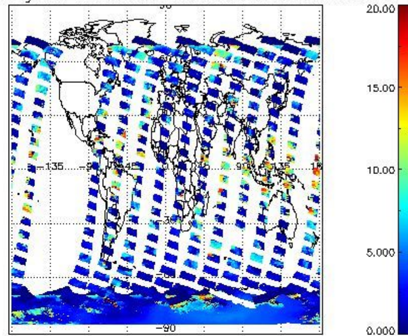
cL_top_height for 22NOV2004 00:00:00 to 23NOV2004 00:00:00
