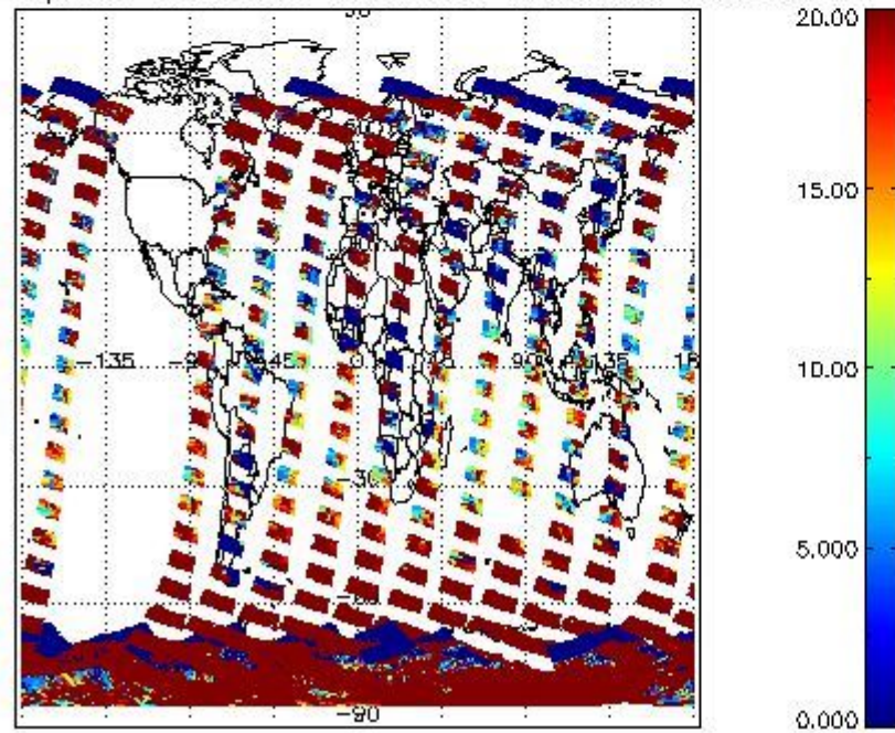
cLopt_depth for 22NOV2004 00:00:00 to 23NOV2004 00:00:00
