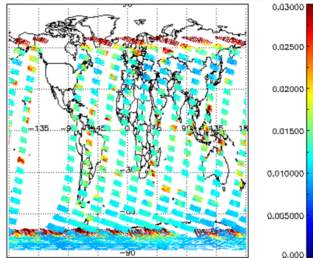
SCIOL2P_NADUV003_vcd_err for 22NOV2004 00:00:00 to 23NOV2004 00:00:00
