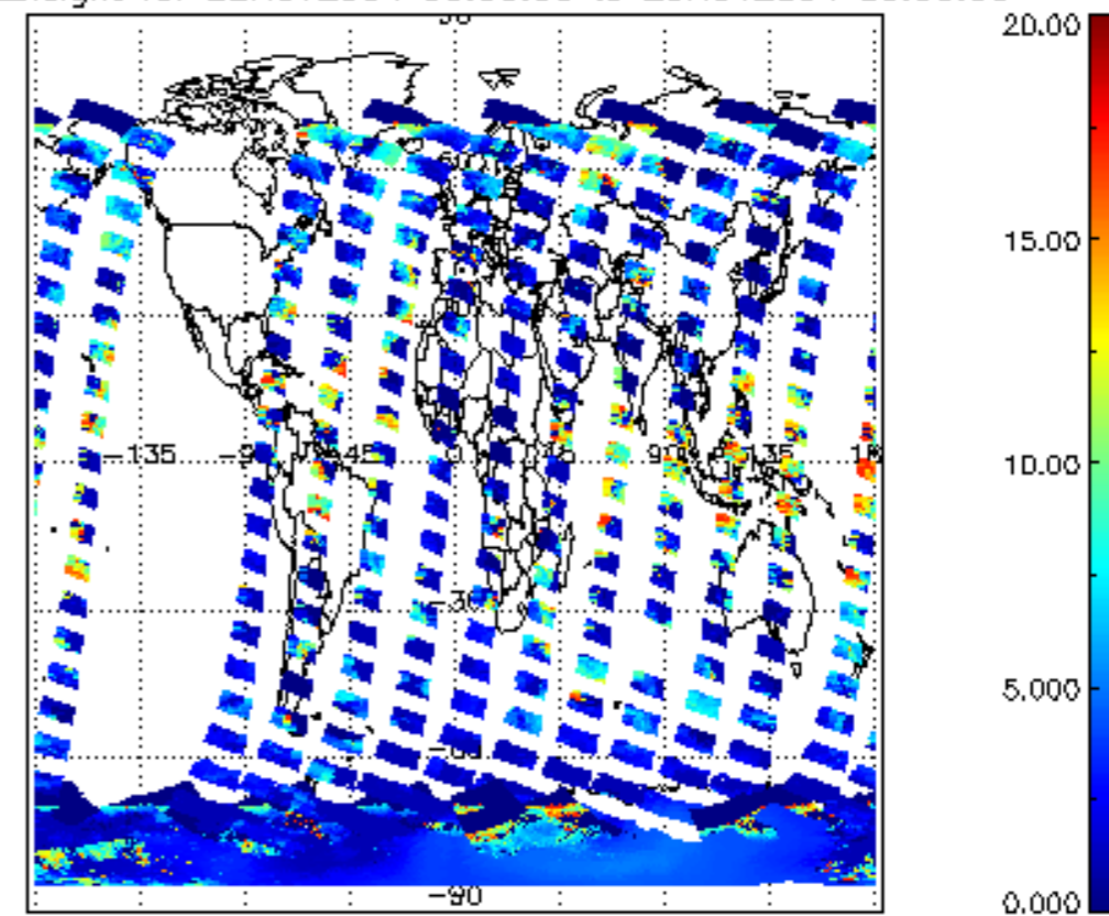
cL_top_height for 22NOV2004 00:00:00 to 23NOV2004 00:00:00
