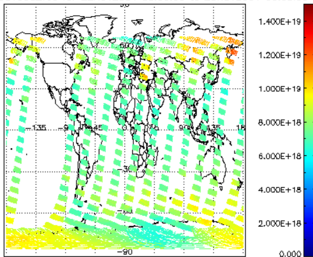
SCIOL2P_NADUV003_vcd for 22NOV2004 00:00:00 to 23NOV2004 00:00:00
