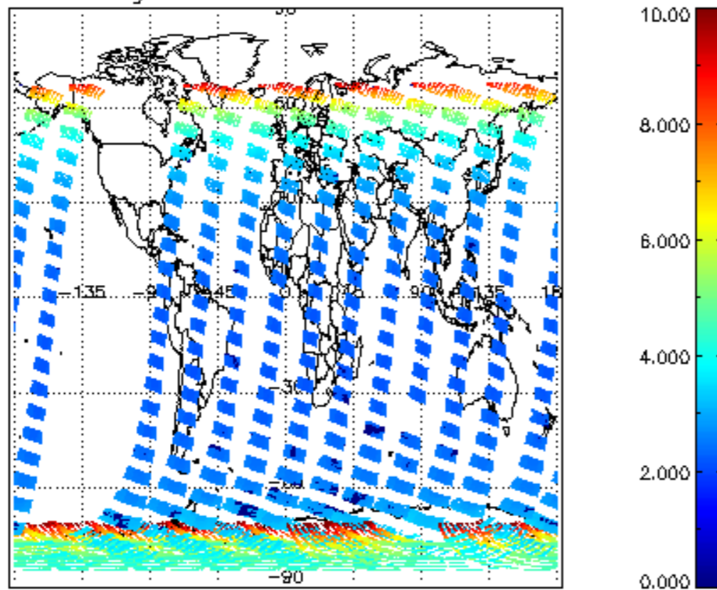
SCIOL2P_NADUV003_amf_gr for 22NOV2004 00:00:00 to 23NOV2004 00:00:00
