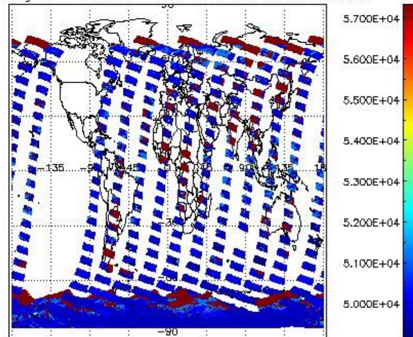
cloud_flags for 22NOV2004 00:00:00 to 23NOV2004 00:00:00
