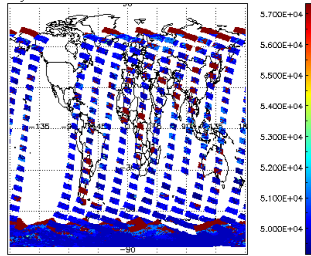
cloud_flags for 22NOV2004 00:00:00 to 23NOV2004 00:00:00
