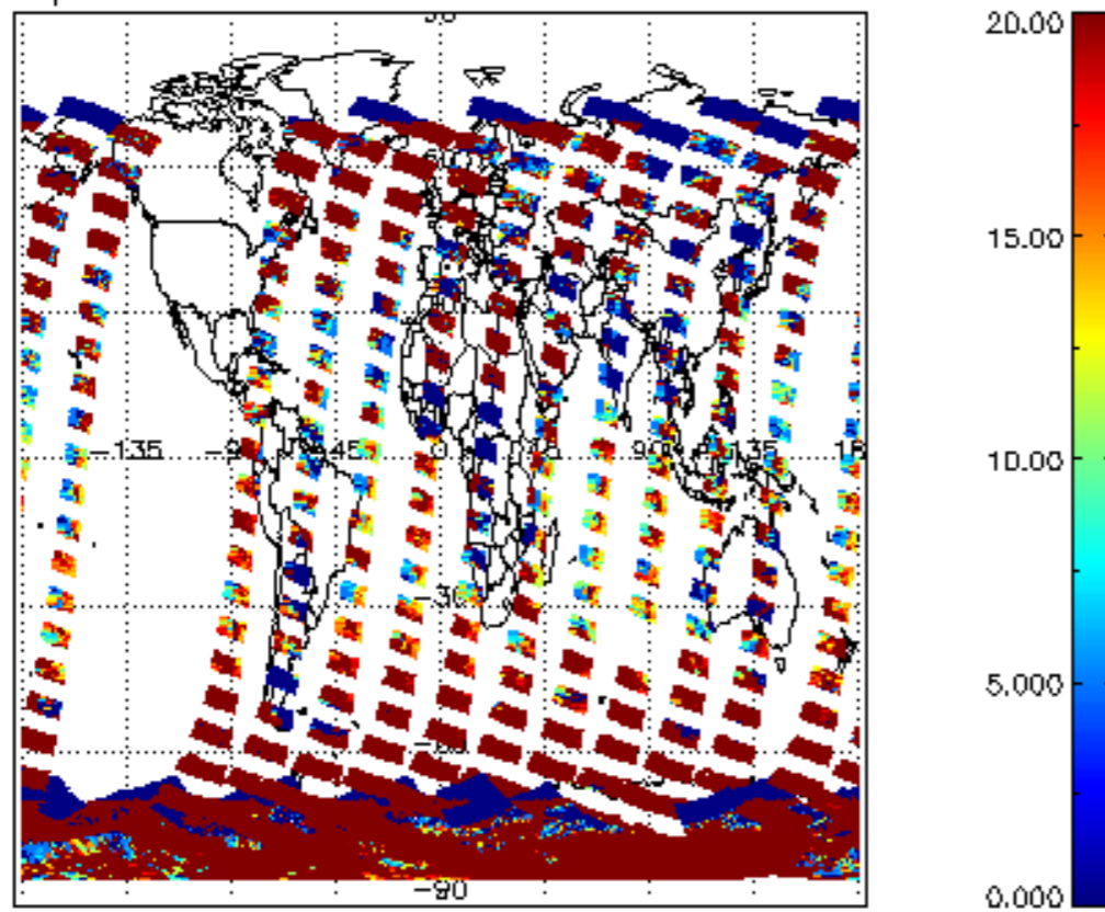
cL_opt_depth for 22NOV2004 00:00:00 to 23NOV2004 00:00:00
