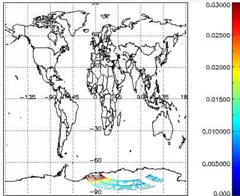
SCIOL2P_NADUV003_vcd_err for 17NOV2004 00:00:00 to 18NOV2004 00:00:00
