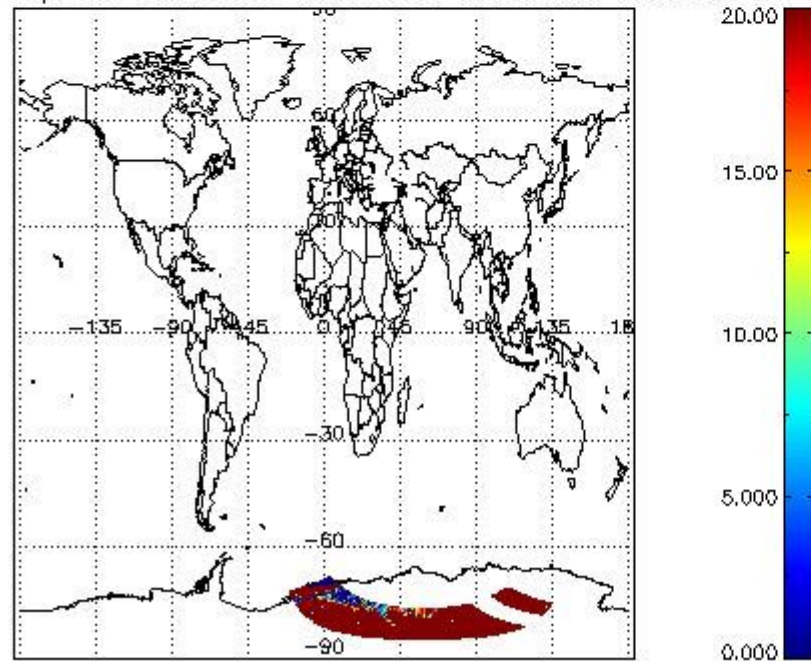
cLopt_depth for 17NOV2004 00:00:00 to 18NOV2004 00:00:00
