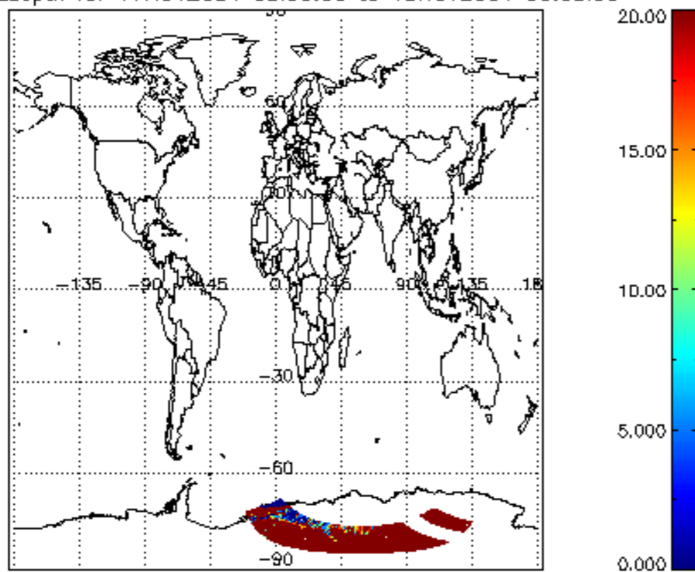
cl_opt_depth for 17NOV2004 00:00:00 to 18NOV2004 00:00:00
