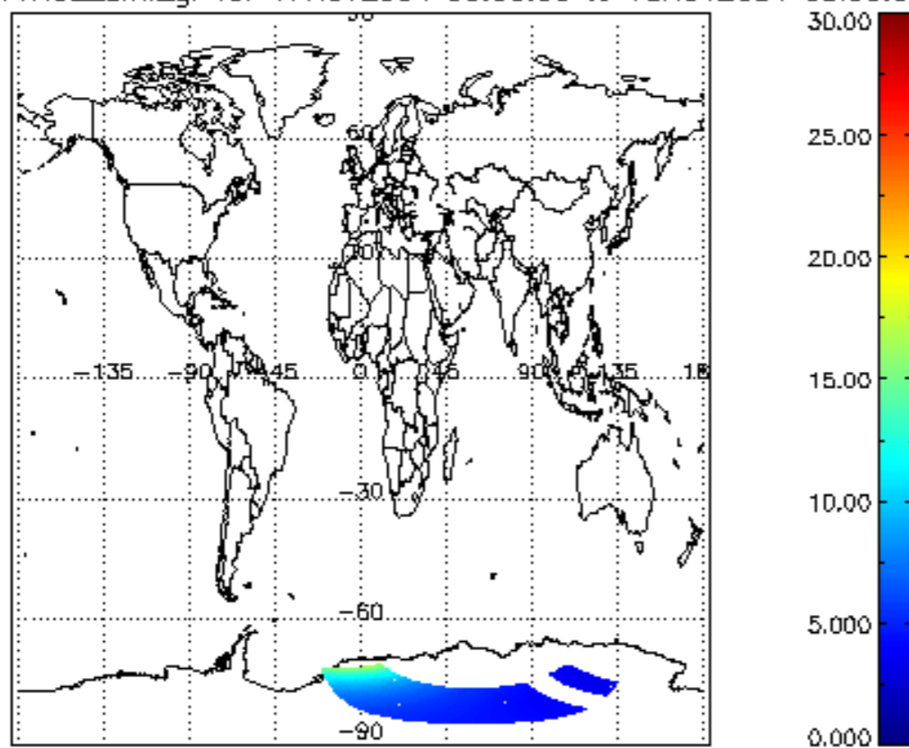
SCIOL2P_NADUV1NO2_amf_gr for 17NOV2004 00:00:00 to 18NOV2004 00:00:00
