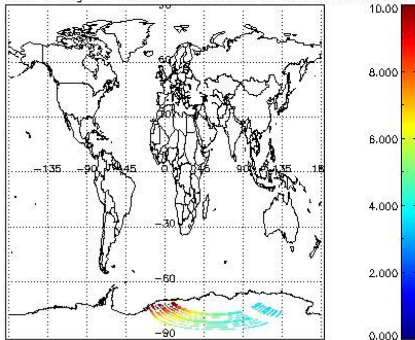
SCIOL2P_NADUV003_amf_gr for 17NOV2004 00:00:00 to 18NOV2004 00:00:00
