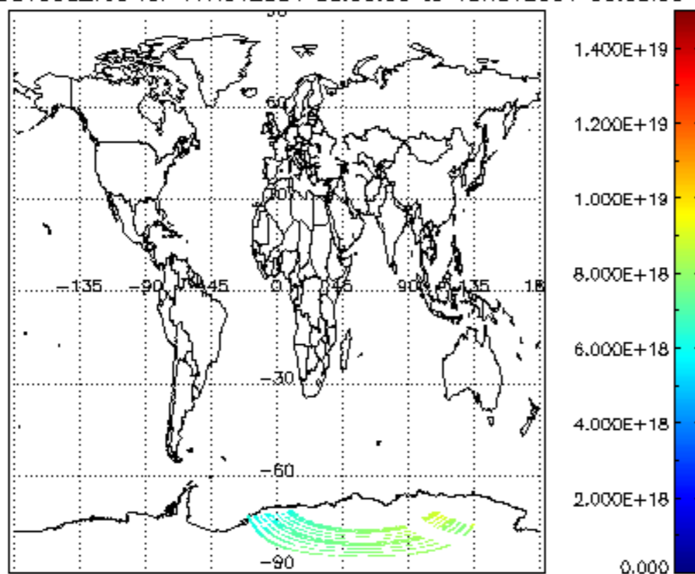
SCIOL2P_NADUV003_vcd for 17NOV2004 00:00:00 to 18NOV2004 00:00:00
