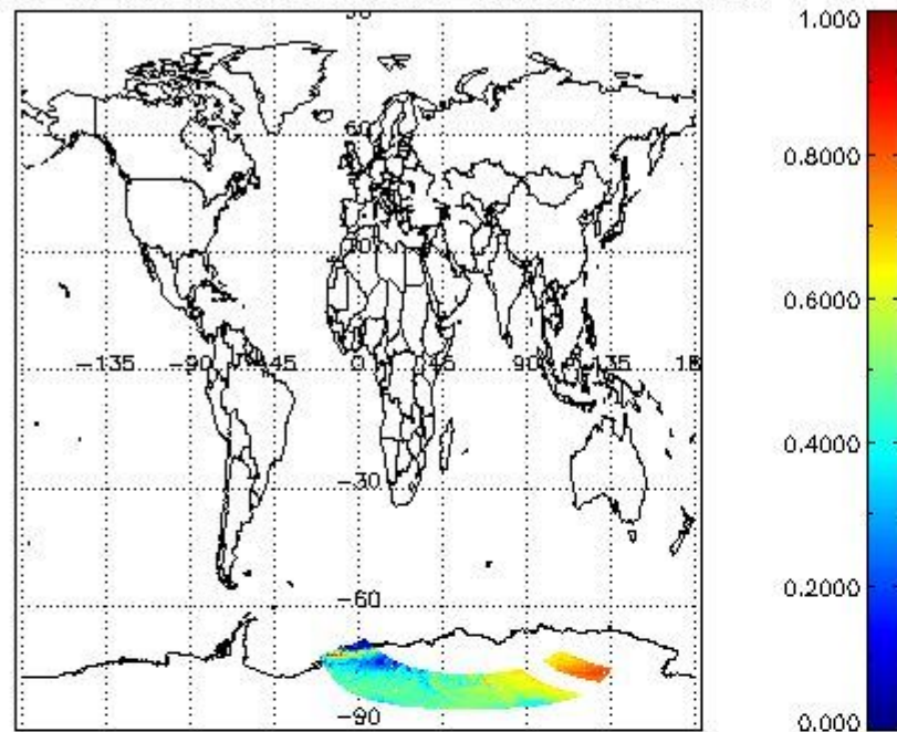
cLfrac for 17NOV2004 00:00:00 to 18NOV2004 00:00:00
