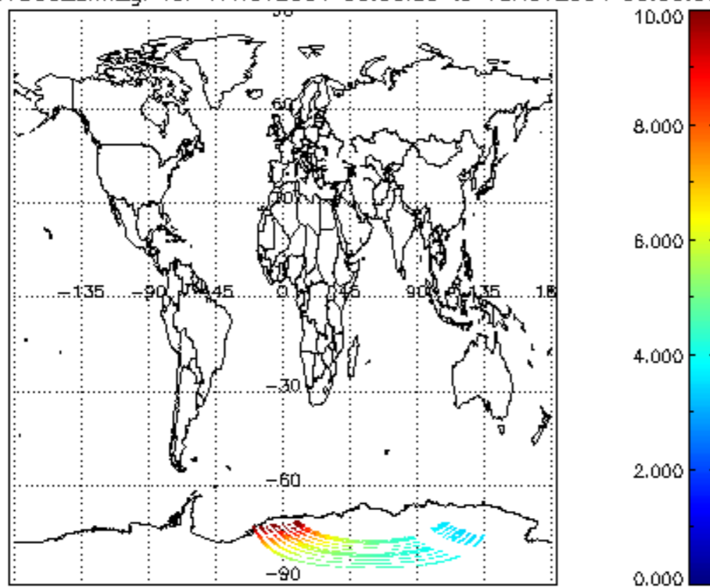
SCIOL2P_NADUV003_amf_gr for 17NOV2004 00:00:00 to 18NOV2004 00:00:00
