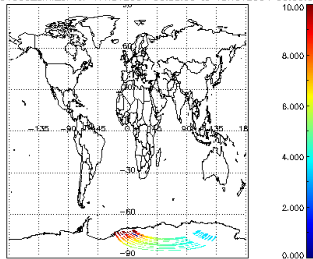
SCIOL2P_NADUV003_amf_cl for 17NOV2004 00:00:00 to 18NOV2004 00:00:00
