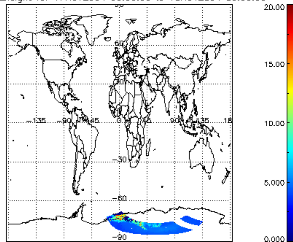
cl_top_height for 17NOV2004 00:00:00 to 18NOV2004 00:00:00
