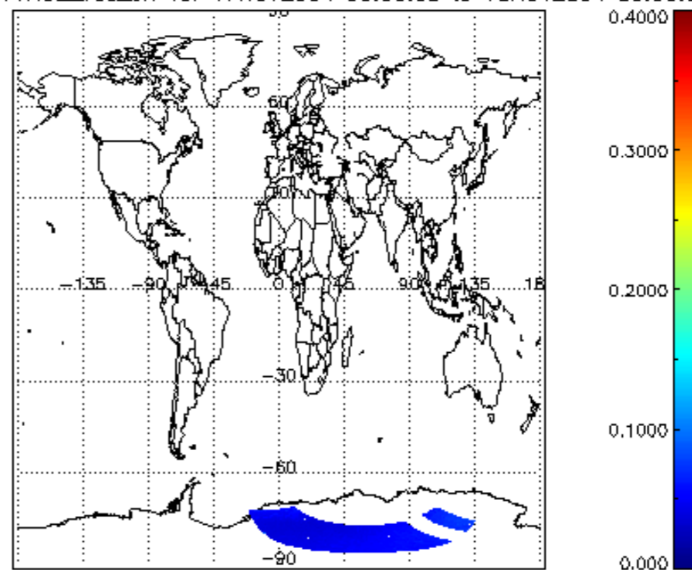
SCIOL2P_NADUV1NO2_vcd_err for 17NOV2004 00:00:00 to 18NOV2004 00:00:00
