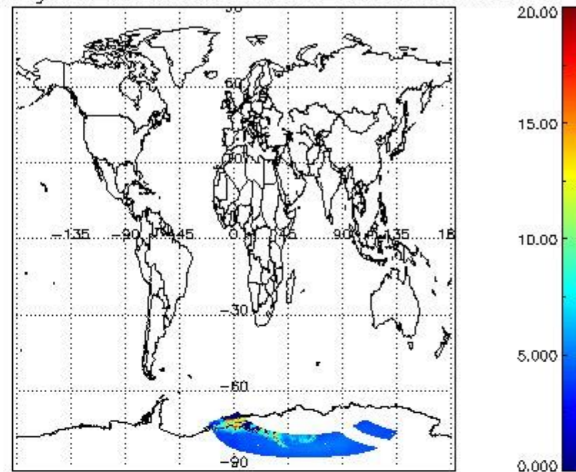
cL_top_height for 17NOV2004 00:00:00 to 18NOV2004 00:00:00
