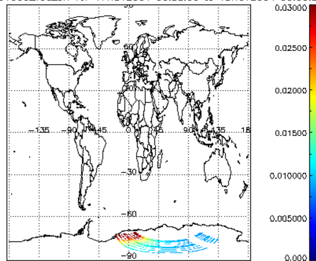
SCIOL2P_NADUV003_vcd_err for 17NOV2004 00:00:00 to 18NOV2004 00:00:00
