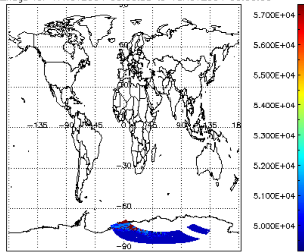
cloud_flags for 17NOV2004 00:00:00 to 18NOV2004 00:00:00
