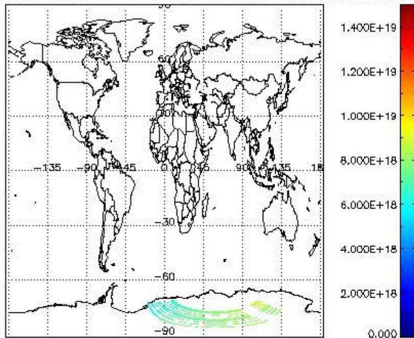
SCIOL2P_NADUV003_vcd for 17NOV2004 00:00:00 to 18NOV2004 00:00:00
