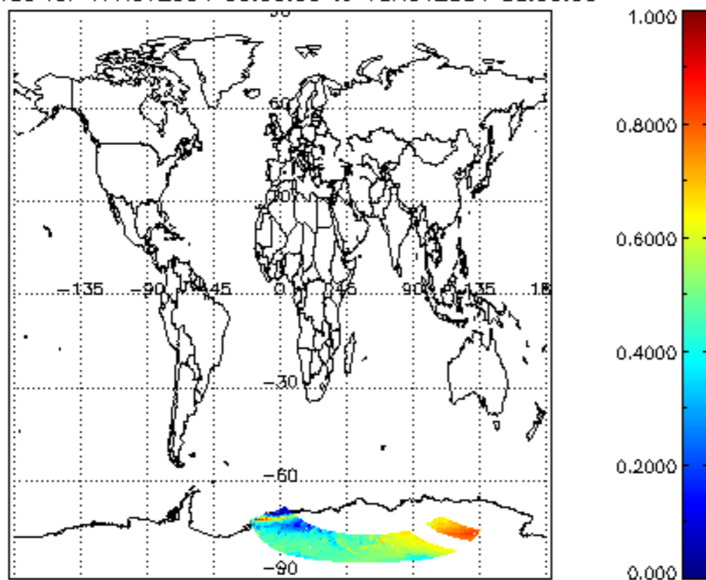
cLfrac for 17NOV2004 00:00:00 to 18NOV2004 00:00:00
