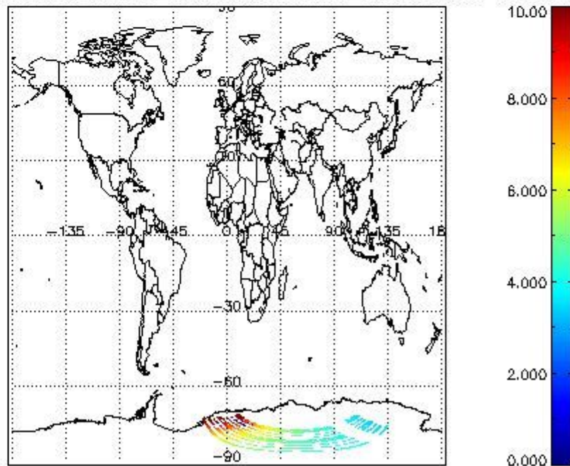
SCIOL2P_NADUV003_amf_cl for 17NOV2004 00:00:00 to 18NOV2004 00:00:00
