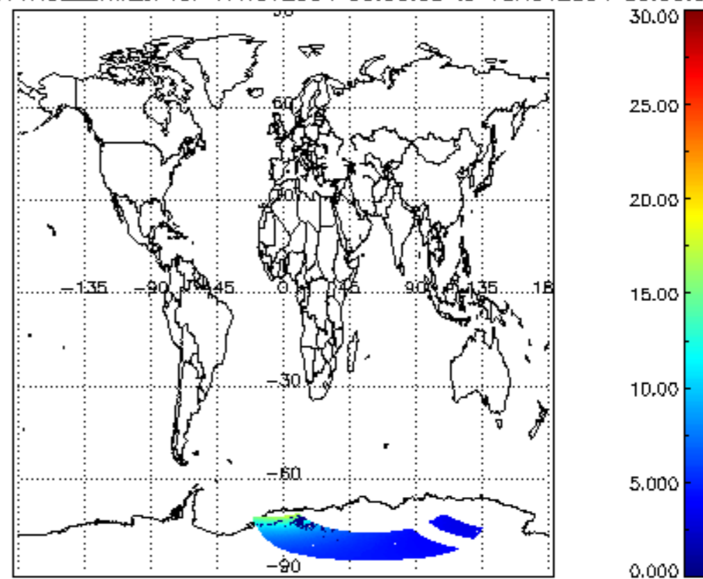
SCIOL2P_NADUV1NO2_amf_cl for 17NOV2004 00:00:00 to 18NOV2004 00:00:00
