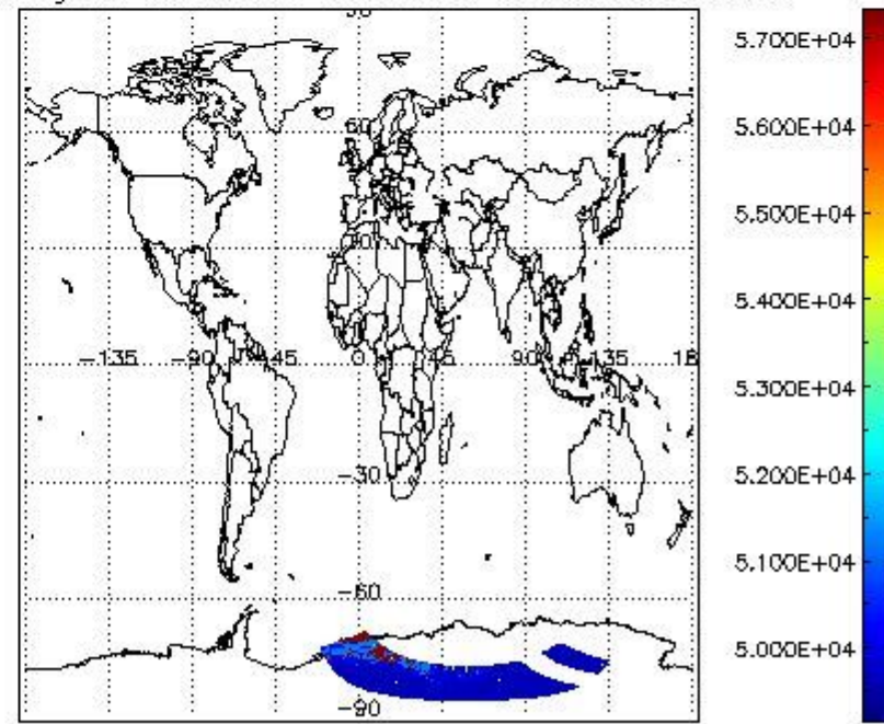
cloud_flags for 17NOV2004 00:00:00 to 18NOV2004 00:00:00
