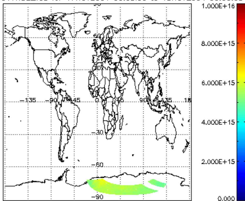
SCIOL2P_NADUV1NO2_vcd for 17NOV2004 00:00:00 to 18NOV2004 00:00:00
