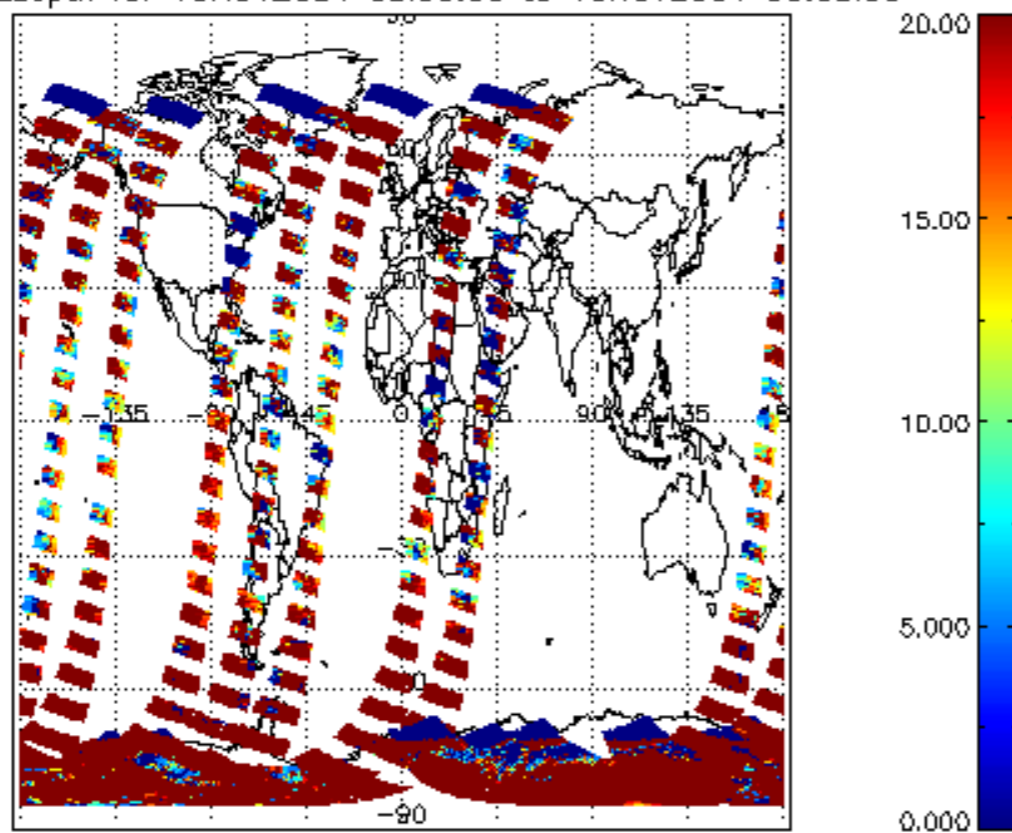
cL_opt_depth for 15NOV2004 00:00:00 to 16NOV2004 00:00:00
