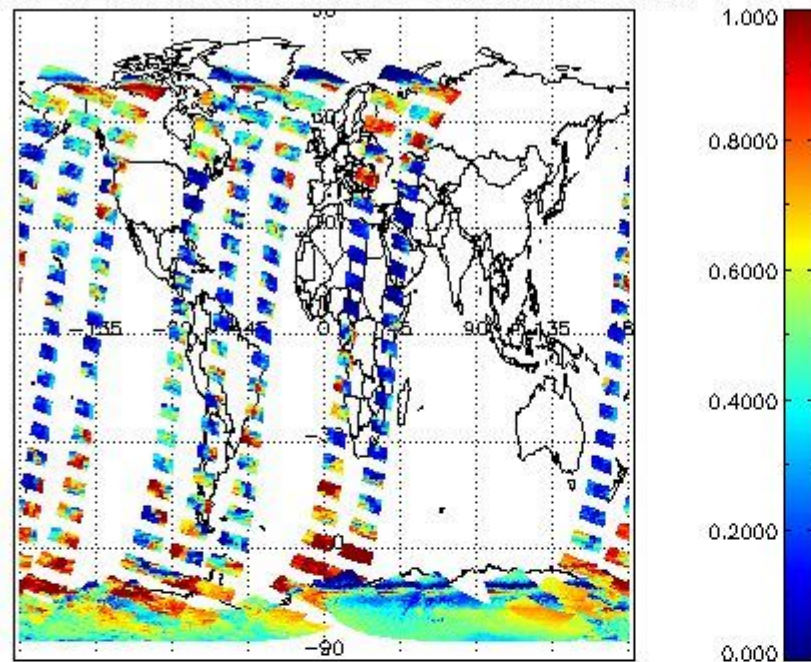
cLfrac for 15NOV2004 00:00:00 to 16NOV2004 00:00:00
