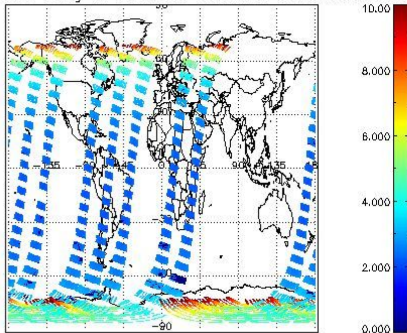
SCIOL2P_NADUV003_amf_gr for 15NOV2004 00:00:00 to 16NOV2004 00:00:00
