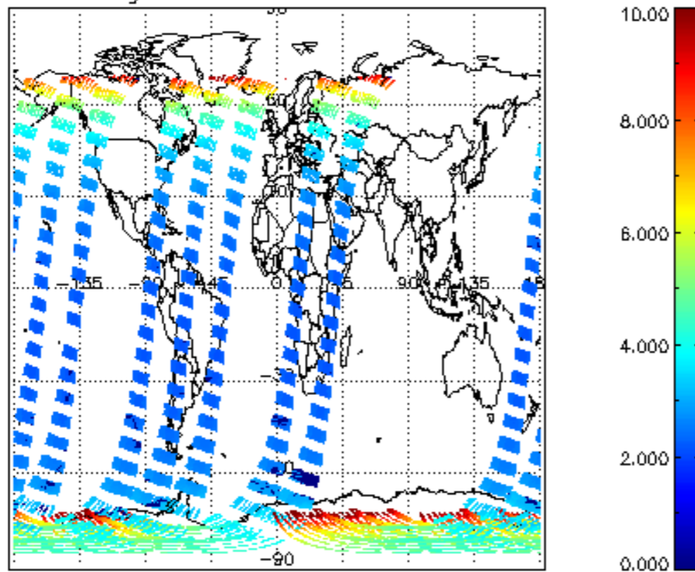
SCIOL2P_NADUV003_amf_gr for 15NOV2004 00:00:00 to 16NOV2004 00:00:00
