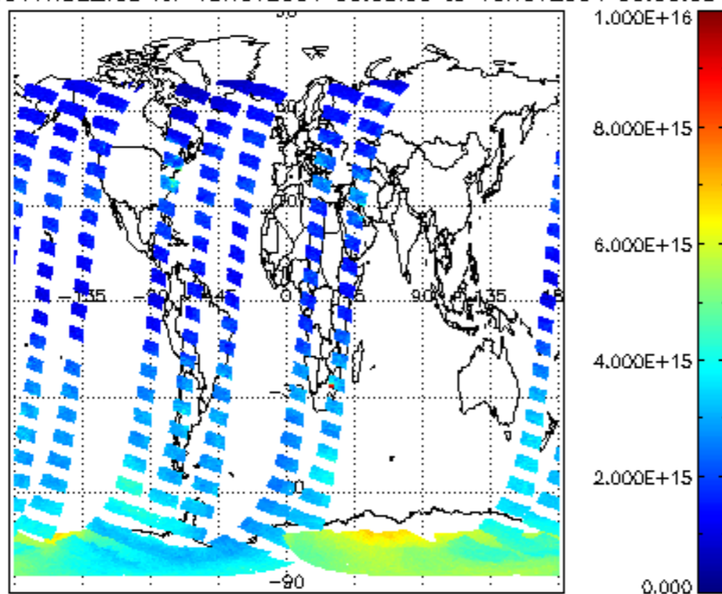
SCIOL2P_NADUV1NO2_vcd for 15NOV2004 00:00:00 to 16NOV2004 00:00:00
