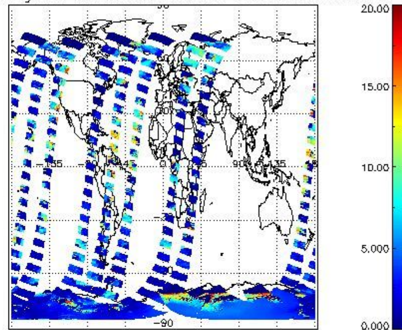
cL_top_height for 15NOV2004 00:00:00 to 16NOV2004 00:00:00
