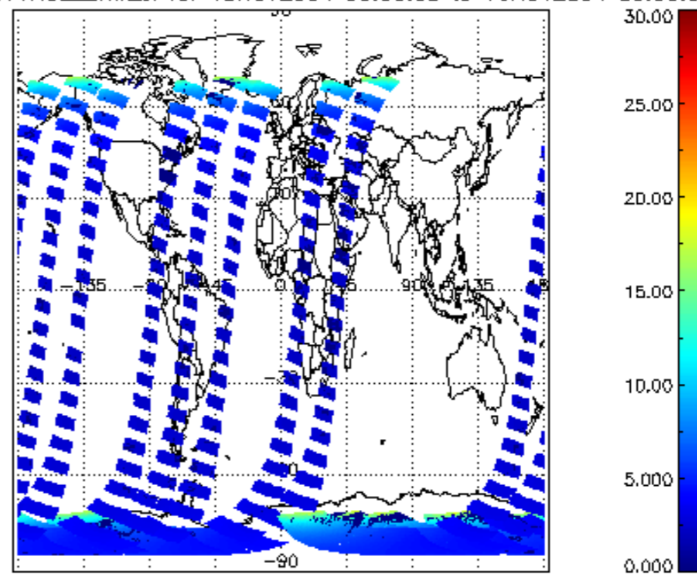
SCIOL2P_NADUV1NO2_amf_cl for 15NOV2004 00:00:00 to 16NOV2004 00:00:00
