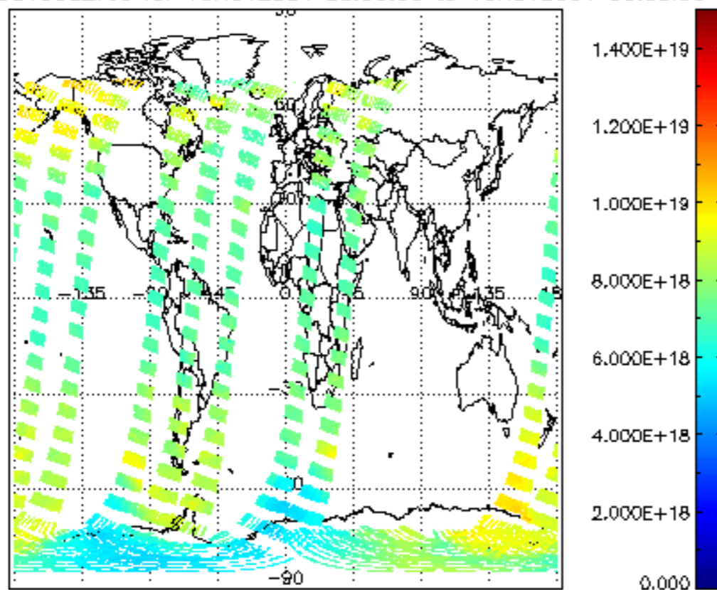
SCIOL2P_NADUV003_vcd for 15NOV2004 00:00:00 to 16NOV2004 00:00:00
