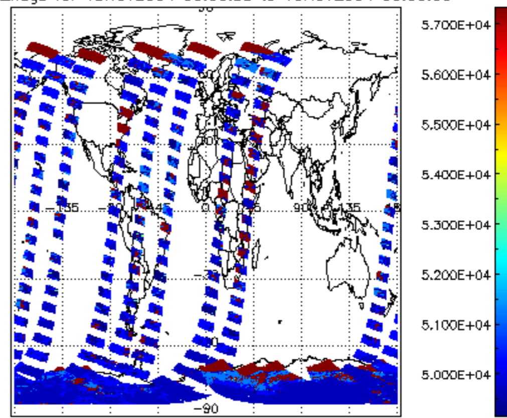
cloud_flags for 15NOV2004 00:00:00 to 16NOV2004 00:00:00
