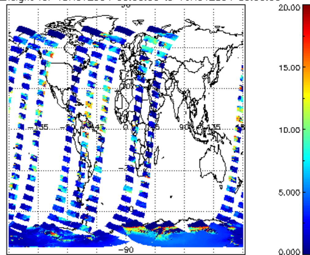
cL_top_height for 15NOV2004 00:00:00 to 16NOV2004 00:00:00
