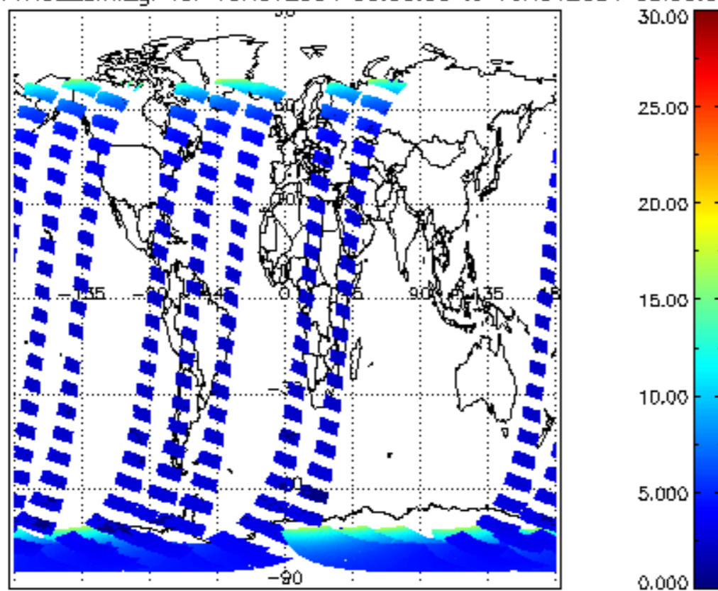
SCIOL2P_NADUV1NO2_amf_gr for 15NOV2004 00:00:00 to 16NOV2004 00:00:00
