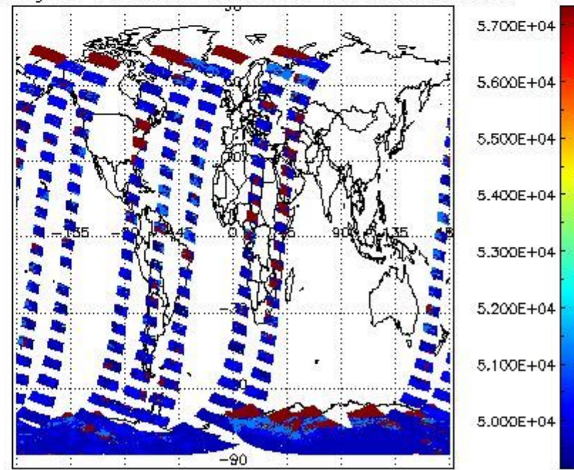
cloud_flags for 15NOV2004 00:00:00 to 16NOV2004 00:00:00
