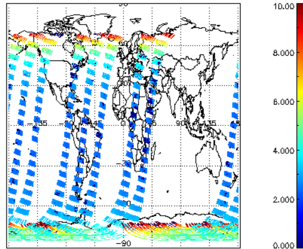
SCIOL2P_NADUV003_amf_cl for 15NOV2004 00:00:00 to 16NOV2004 00:00:00
