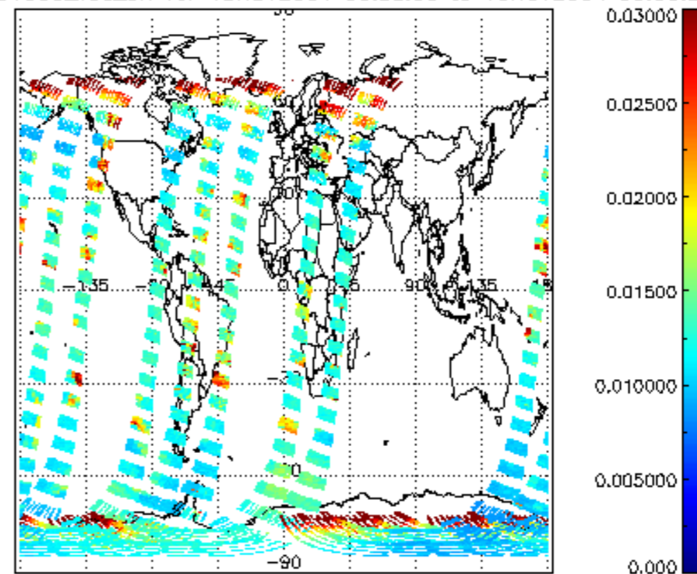
SCIOL2P_NADUV003_vcd_err for 15NOV2004 00:00:00 to 16NOV2004 00:00:00
