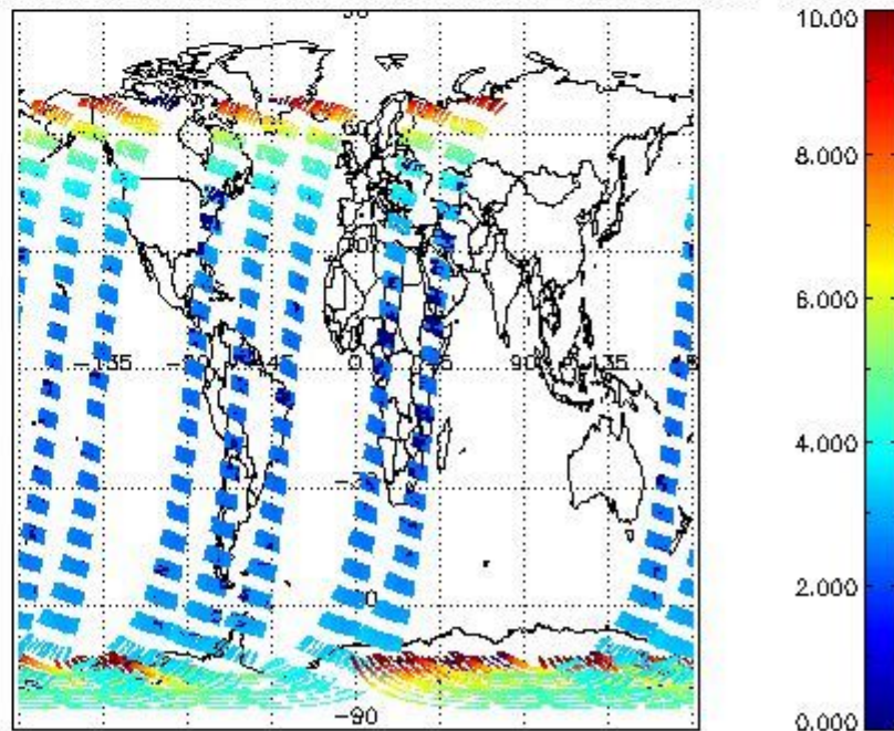
SCIOL2P_NADUV003_amf_cl for 15NOV2004 00:00:00 to 16NOV2004 00:00:00
