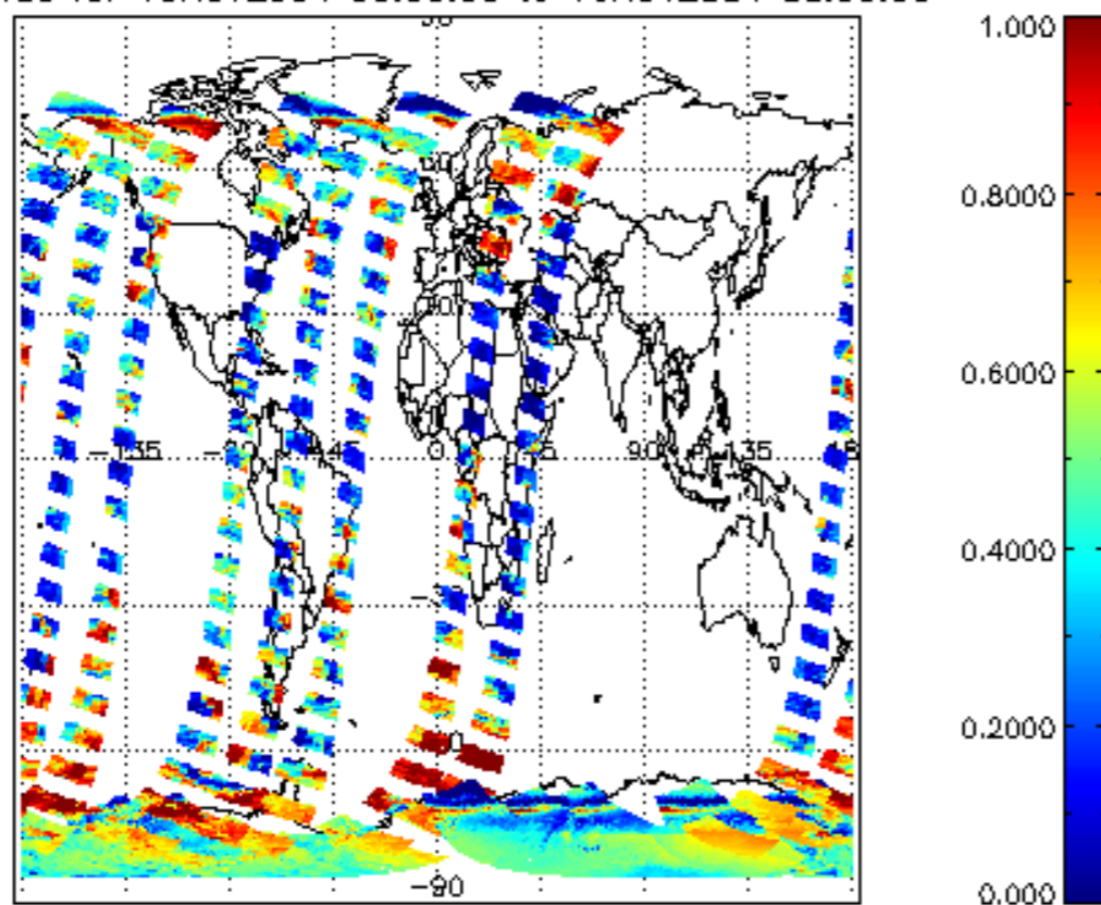
cLfrac for 15NOV2004 00:00:00 to 16NOV2004 00:00:00
