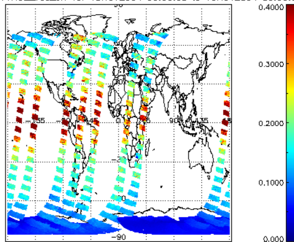
SCIOL2P_NADUV1NO2_vcd_err for 15NOV2004 00:00:00 to 16NOV2004 00:00:00
