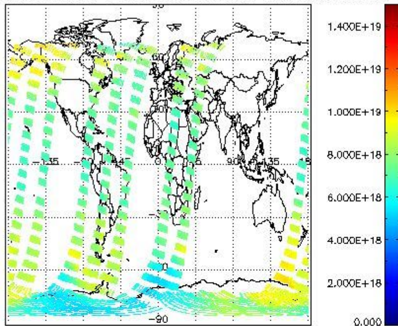
SCIOL2P_NADUV003_vcd for 15NOV2004 00:00:00 to 16NOV2004 00:00:00
