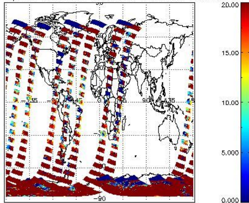
cLopt_depth for 15NOV2004 00:00:00 to 16NOV2004 00:00:00
