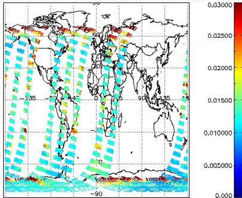
SCIOL2P_NADUV003_vcd_err for 15NOV2004 00:00:00 to 16NOV2004 00:00:00
