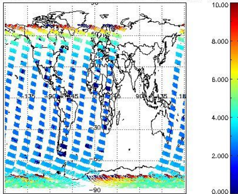
SCIOL2P_NADUV003_amf_cl for 10NOV2004 00:00:00 to 11NOV2004 00:00:00
