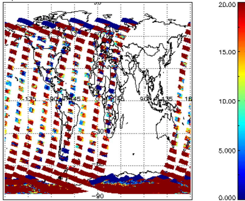
cL_opt_depth for 10NOV2004 00:00:00 to 11NOV2004 00:00:00
