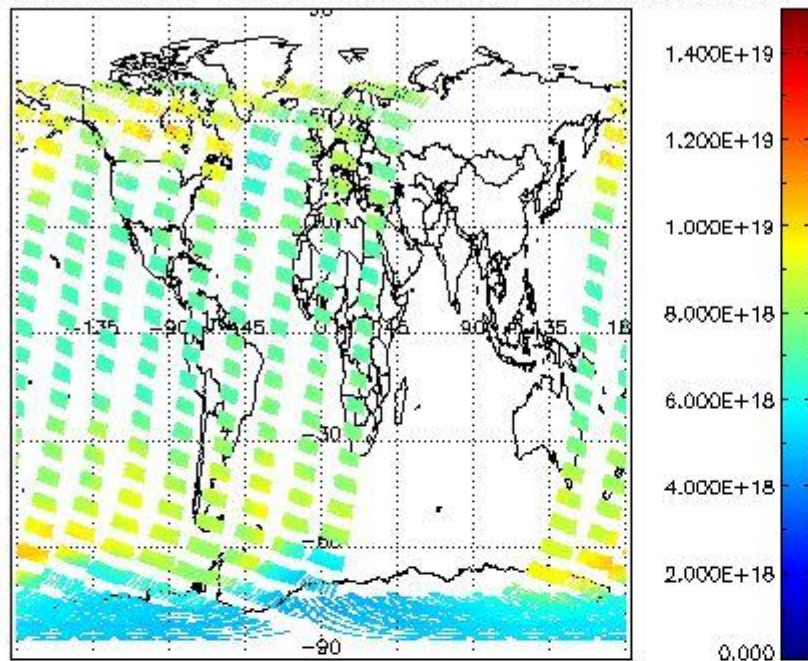
SCIOL2P_NADUV003_vcd for 10NOV2004 00:00:00 to 11NOV2004 00:00:00
