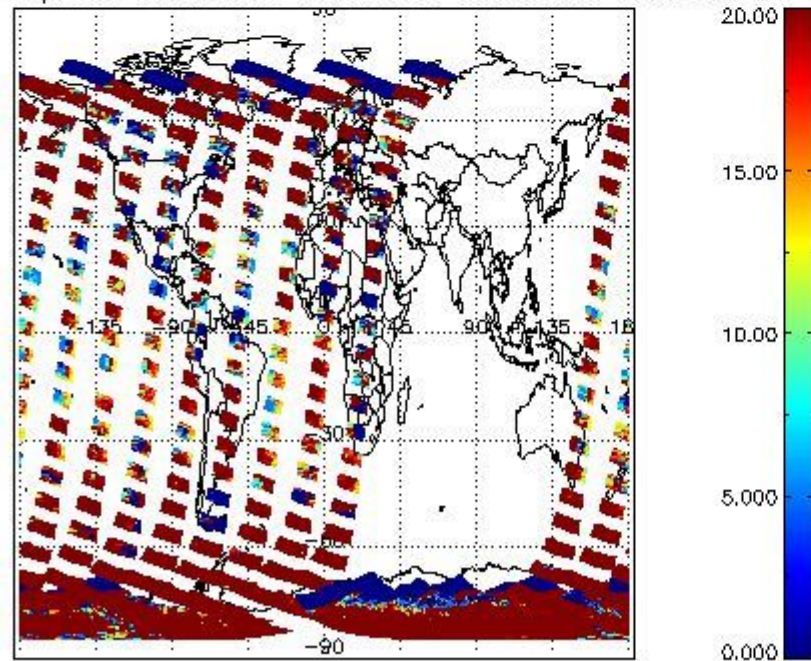
cLopt_depth for 10NOV2004 00:00:00 to 11NOV2004 00:00:00
