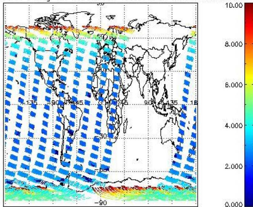
SCIOL2P_NADUV003_amf_gr for 10NOV2004 00:00:00 to 11NOV2004 00:00:00
