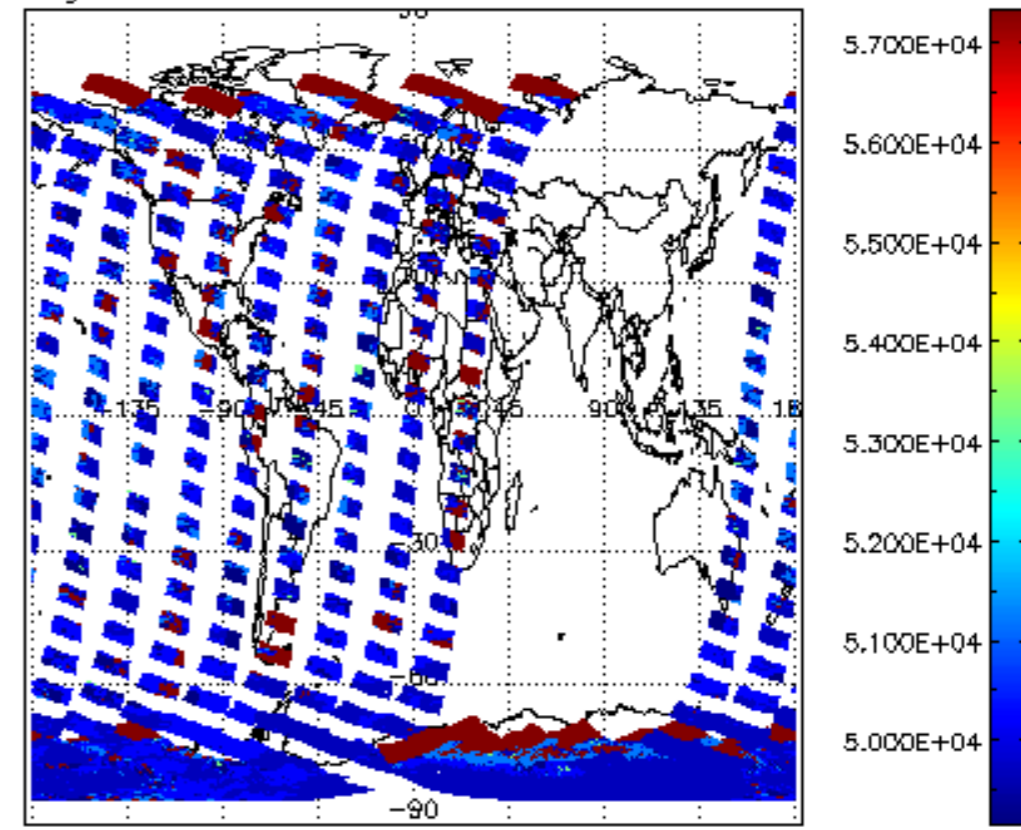
cloud_flags for 10NOV2004 00:00:00 to 11NOV2004 00:00:00
