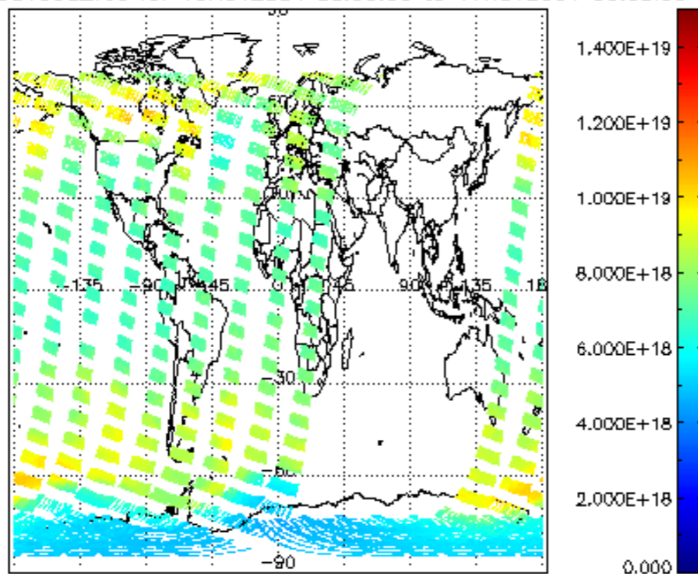
SCIOL2P_NADUV003_vcd for 10NOV2004 00:00:00 to 11NOV2004 00:00:00
