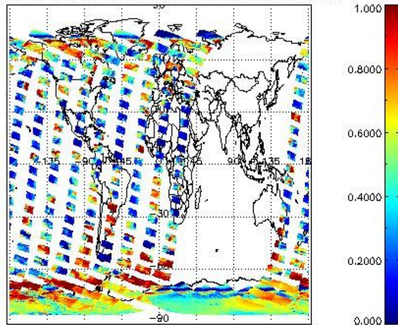
cLfrac for 10NOV2004 00:00:00 to 11NOV2004 00:00:00
