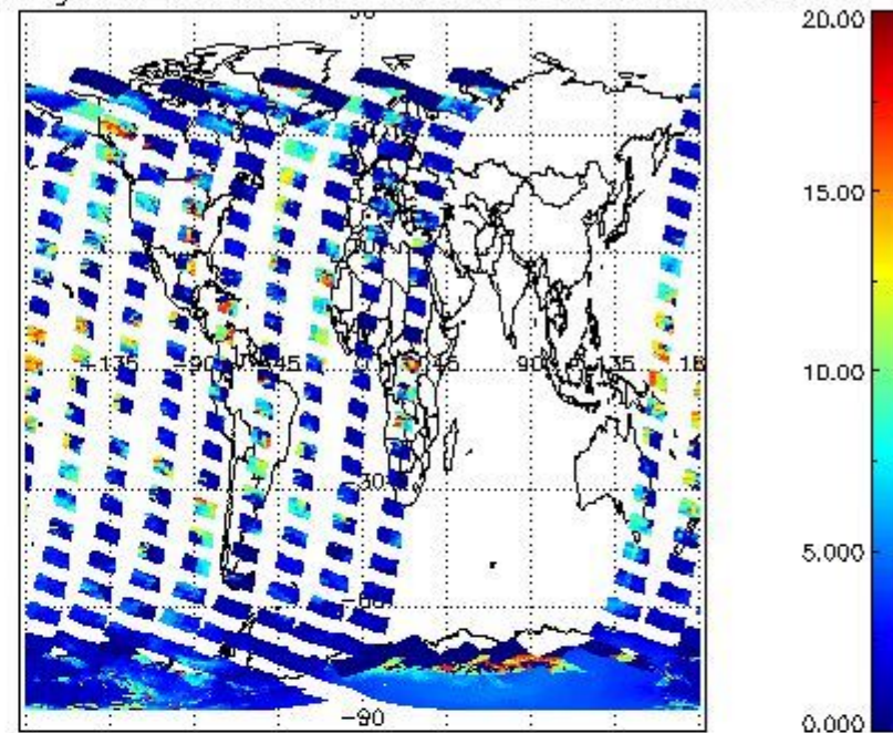
cL_top_height for 10NOV2004 00:00:00 to 11NOV2004 00:00:00
