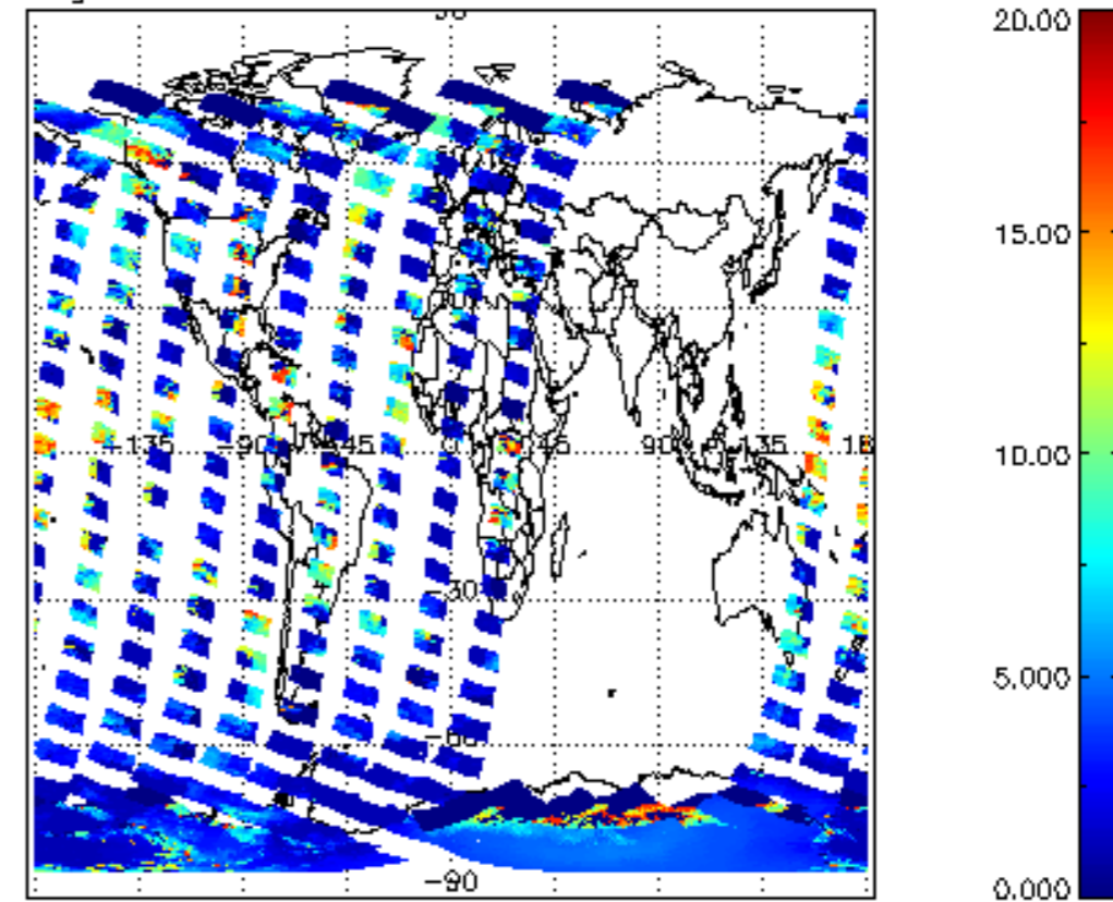
cL_top_height for 10NOV2004 00:00:00 to 11NOV2004 00:00:00
