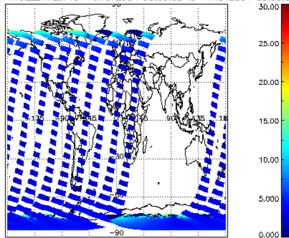
SCIOL2P_NADUV1NO2_amf_cl for 10NOV2004 00:00:00 to 11NOV2004 00:00:00
