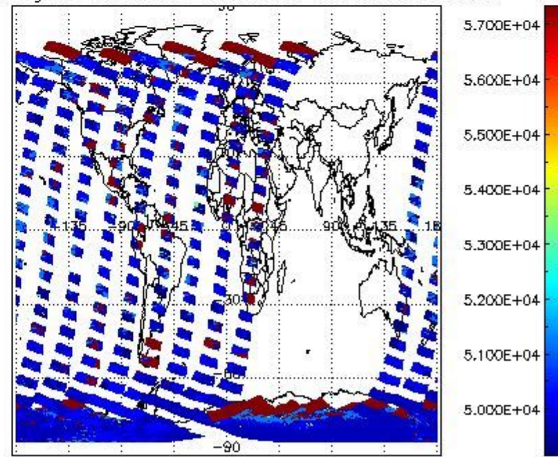
cloud_flags for 10NOV2004 00:00:00 to 11NOV2004 00:00:00
