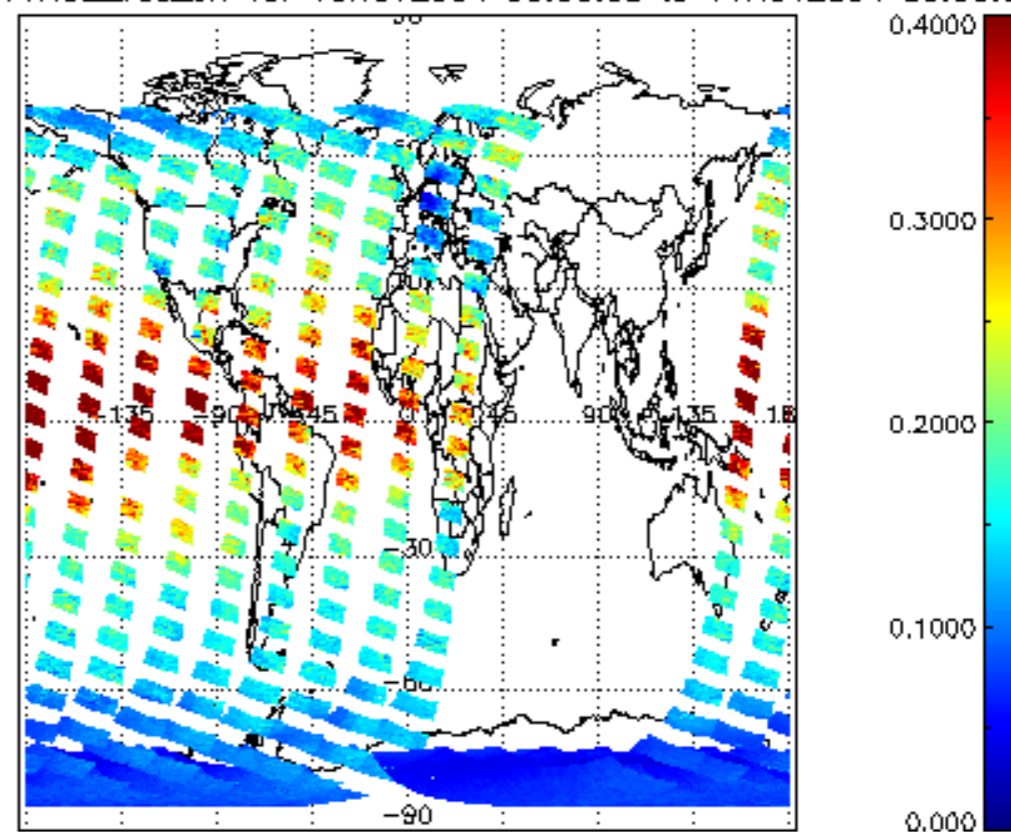
SCIOL2P_NADUV1NO2_vcd_err for 10NOV2004 00:00:00 to 11NOV2004 00:00:00
