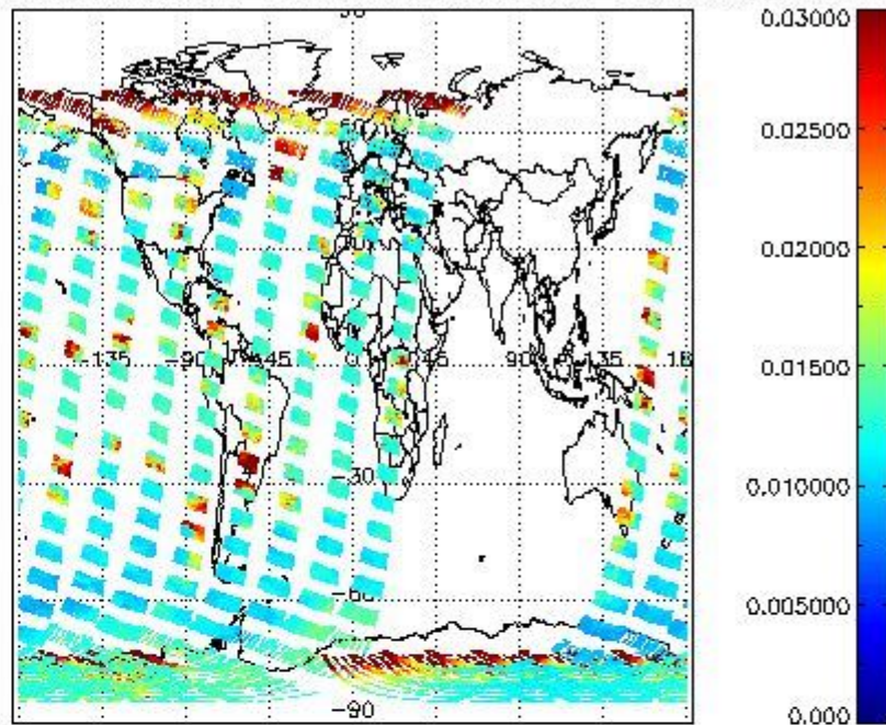
SCIOL2P_NADUV003_vcd_err for 10NOV2004 00:00:00 to 11NOV2004 00:00:00
