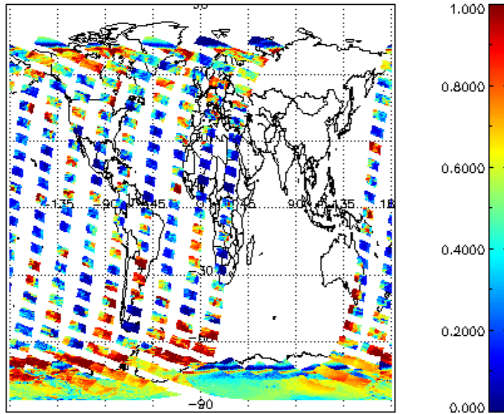
cLfrac for 10NOV2004 00:00:00 to 11NOV2004 00:00:00
