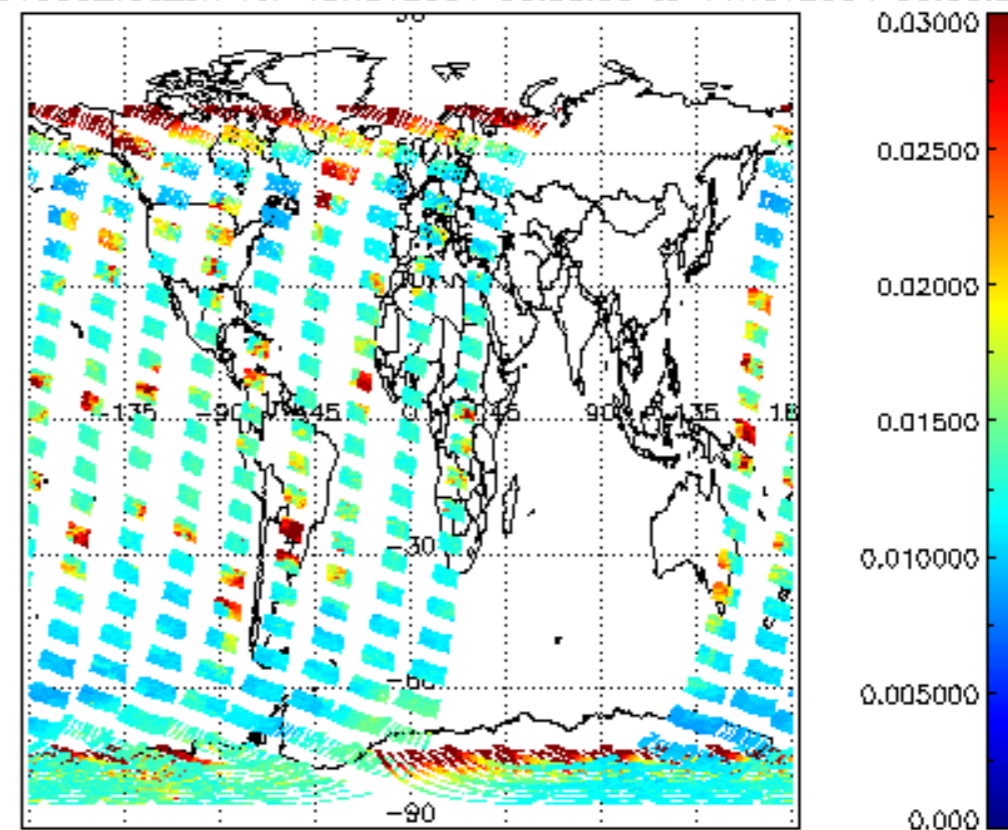
SCIOL2P_NADUV003_vcd_err for 10NOV2004 00:00:00 to 11NOV2004 00:00:00
