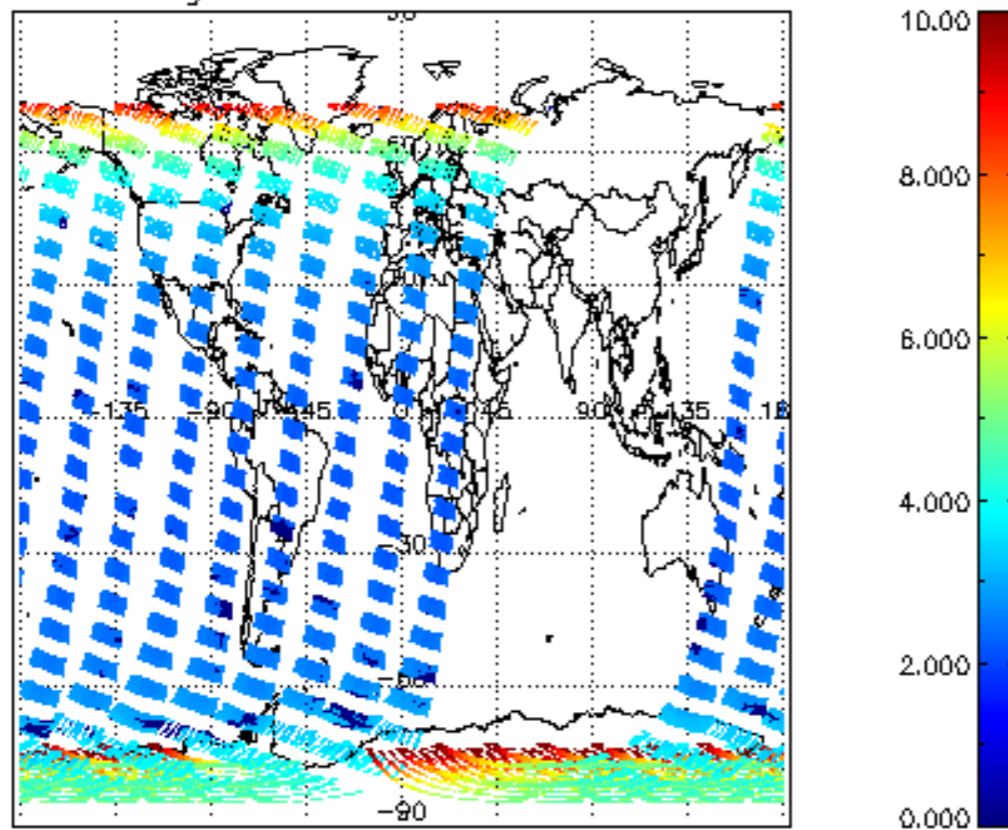
SCIOL2P_NADUV003_amf_gr for 10NOV2004 00:00:00 to 11NOV2004 00:00:00
