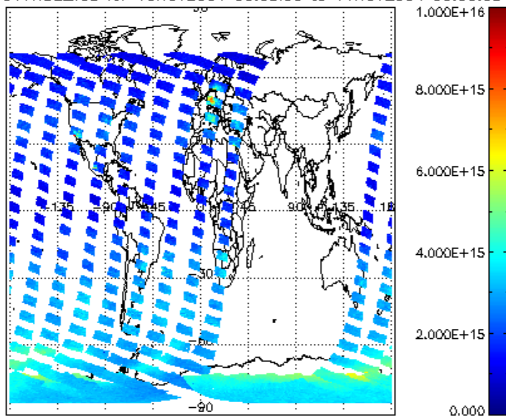
SCIOL2P_NADUV1NO2_vcd for 10NOV2004 00:00:00 to 11NOV2004 00:00:00
