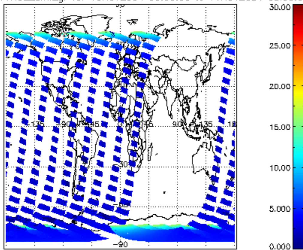
SCIOL2P_NADUV1NO2_amf_gr for 10NOV2004 00:00:00 to 11NOV2004 00:00:00
