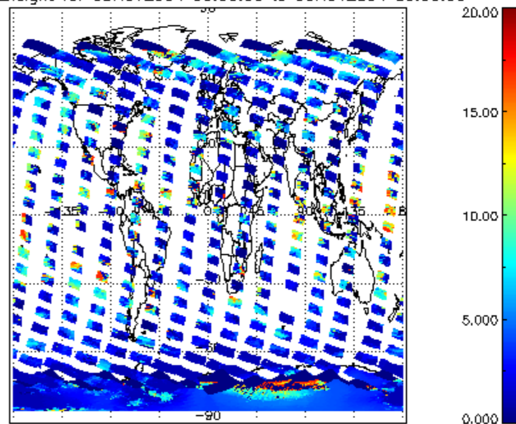
cL_top_height for 08NOV2004 00:00:00 to 09NOV2004 00:00:00
