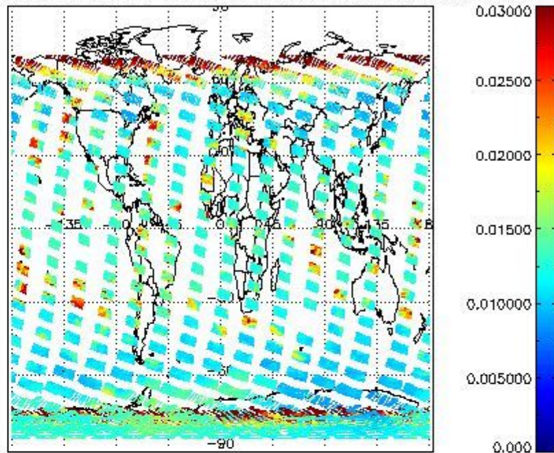
SCIOL2P_NADUV003_vcd_err for 08NOV2004 00:00:00 to 09NOV2004 00:00:00
