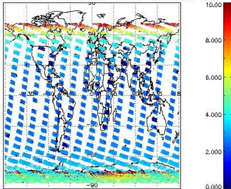
SCIOL2P_NADUV003_amf_cl for 08NOV2004 00:00:00 to 09NOV2004 00:00:00
