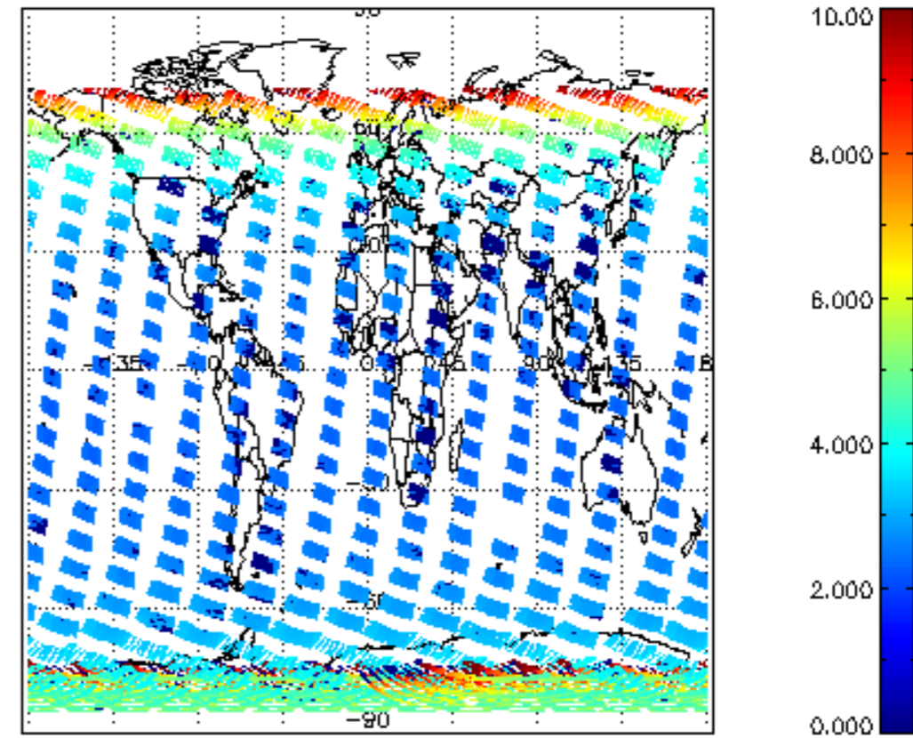
SCIOL2P_NADUV003_amf_cl for 08NOV2004 00:00:00 to 09NOV2004 00:00:00
