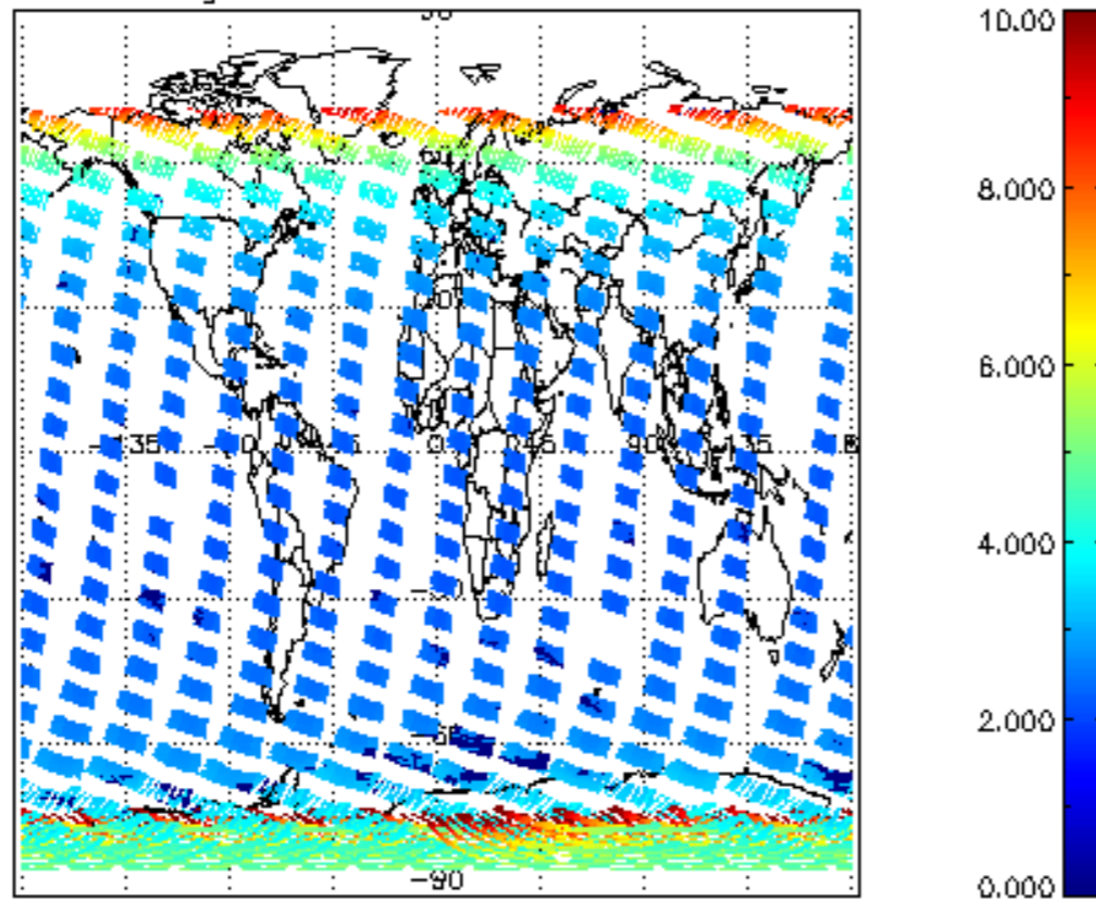
SCIOL2P_NADUV003_amf_gr for 08NOV2004 00:00:00 to 09NOV2004 00:00:00
