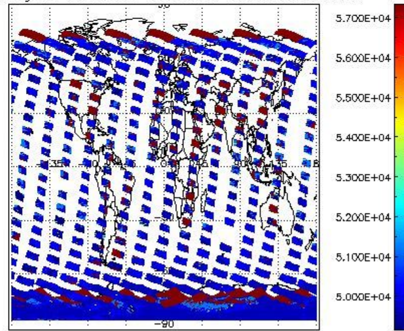
cloud_flags for 08NOV2004 00:00:00 to 09NOV2004 00:00:00
