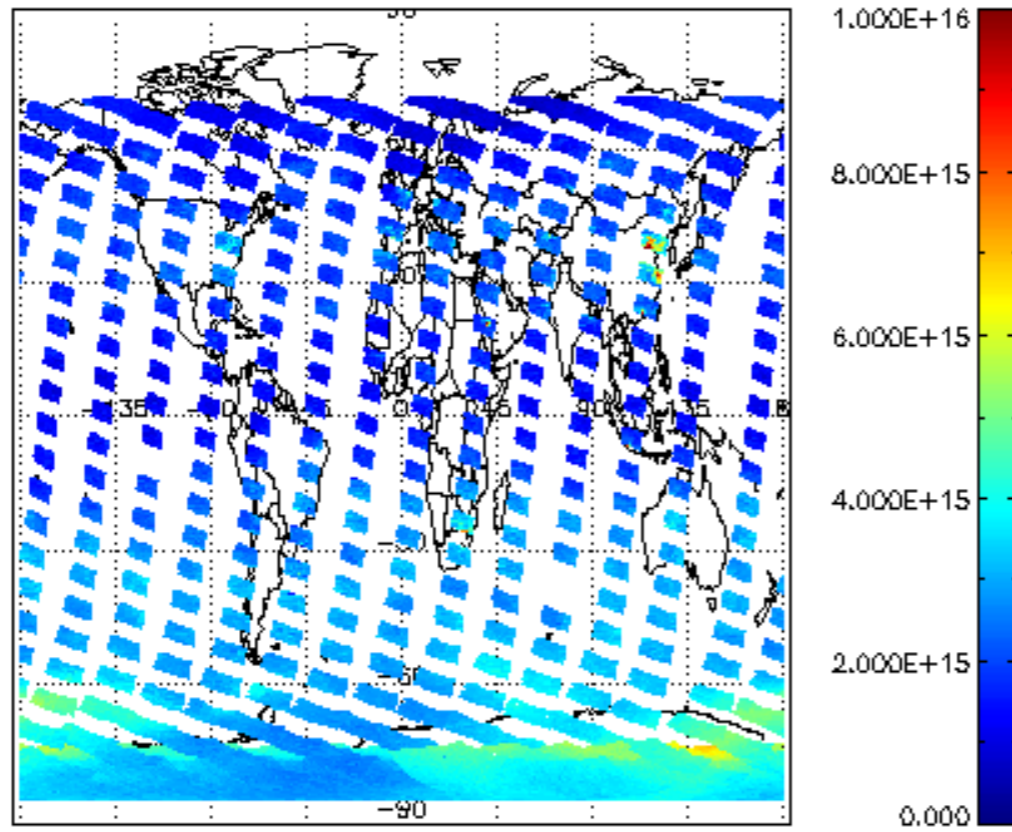
SCIOL2P_NADUV1NO2_vcd for 08NOV2004 00:00:00 to 09NOV2004 00:00:00
