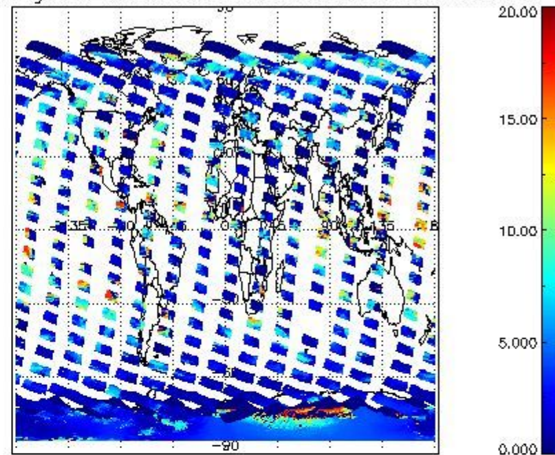
cL_top_height for 08NOV2004 00:00:00 to 09NOV2004 00:00:00
