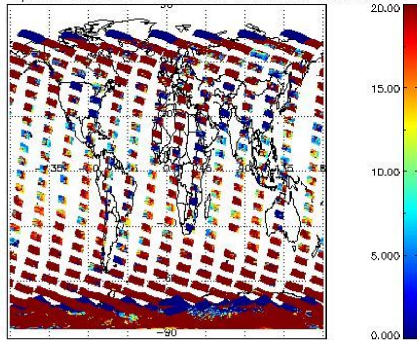
cLopt_depth for 08NOV2004 00:00:00 to 09NOV2004 00:00:00
