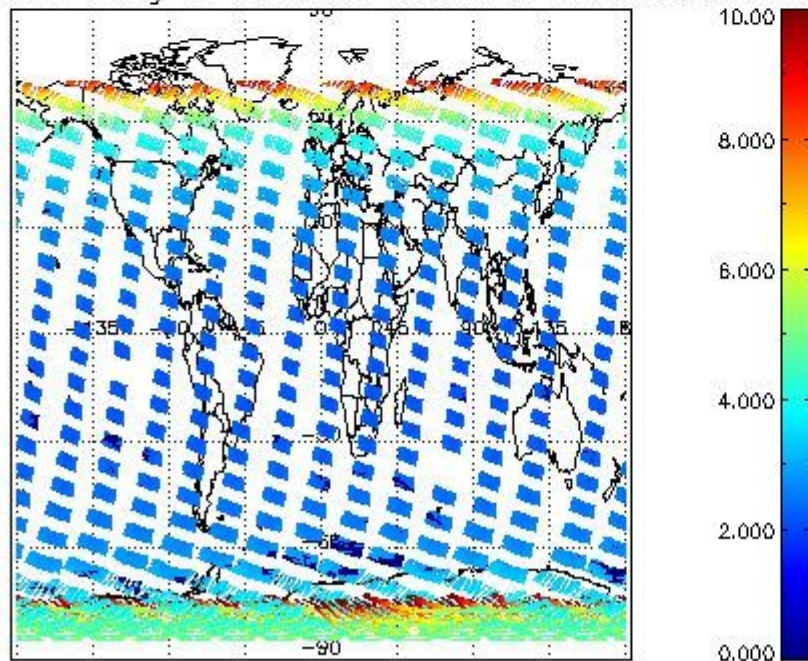
SCIOL2P_NADUV003_amf_gr for 08NOV2004 00:00:00 to 09NOV2004 00:00:00
