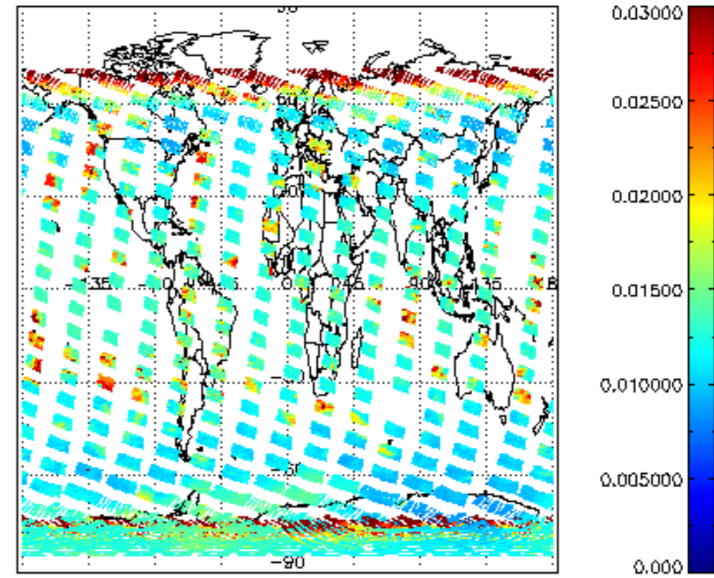
SCIOL2P_NADUV003_vcd_err for 08NOV2004 00:00:00 to 09NOV2004 00:00:00
