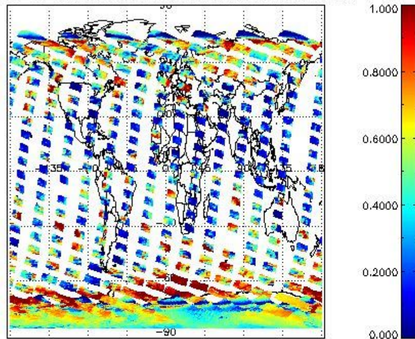
cLfrac for 08NOV2004 00:00:00 to 09NOV2004 00:00:00
