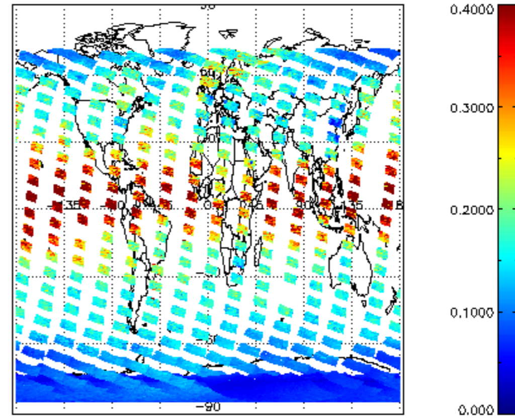
SCIOL2P_NADUV1NO2_vcd_err for 08NOV2004 00:00:00 to 09NOV2004 00:00:00
