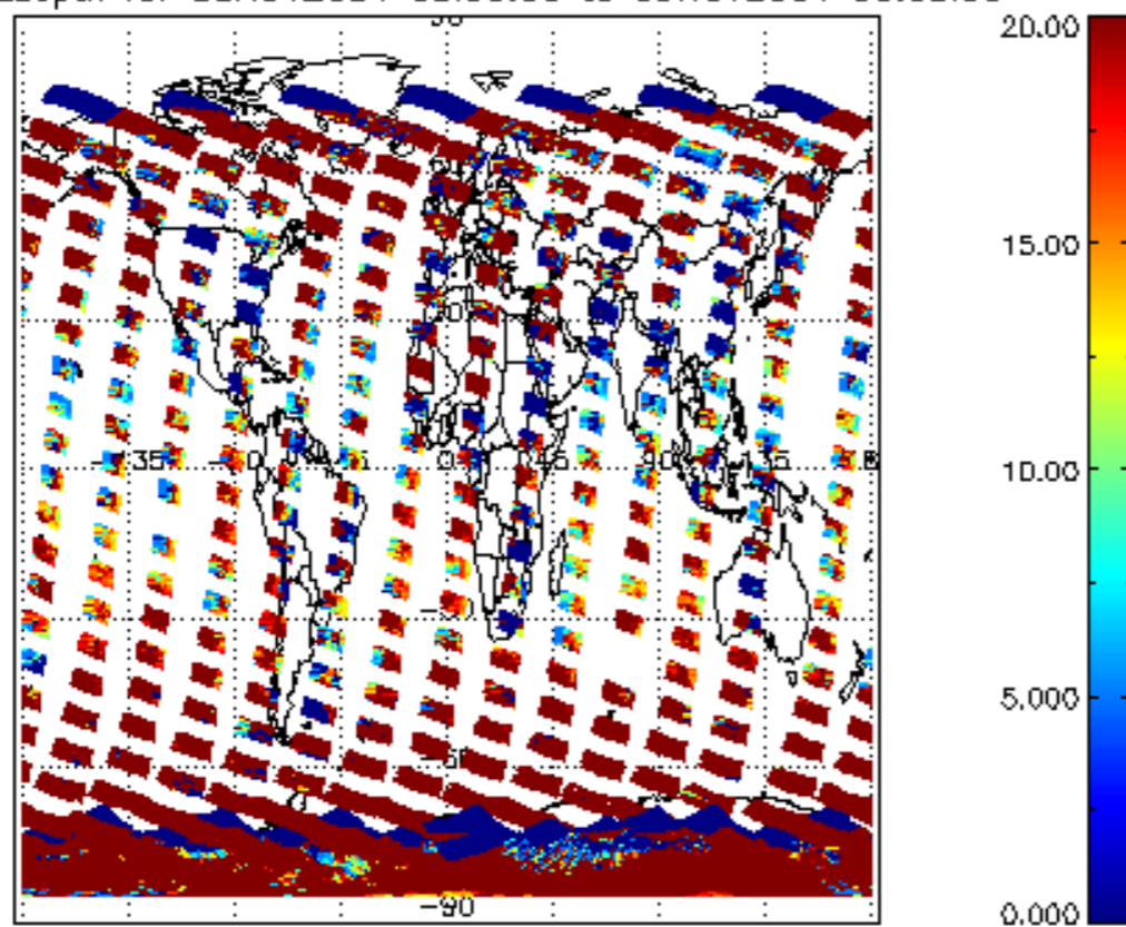
cL_opt_depth for 08NOV2004 00:00:00 to 09NOV2004 00:00:00
