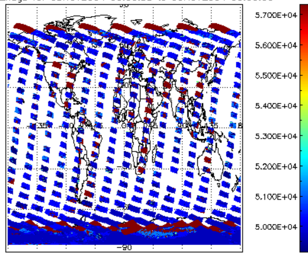
cloud_flags for 08NOV2004 00:00:00 to 09NOV2004 00:00:00
