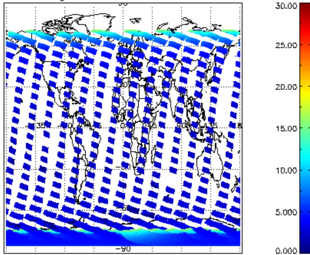
SCIOL2P_NADUV1NO2_amf_gr for 08NOV2004 00:00:00 to 09NOV2004 00:00:00
