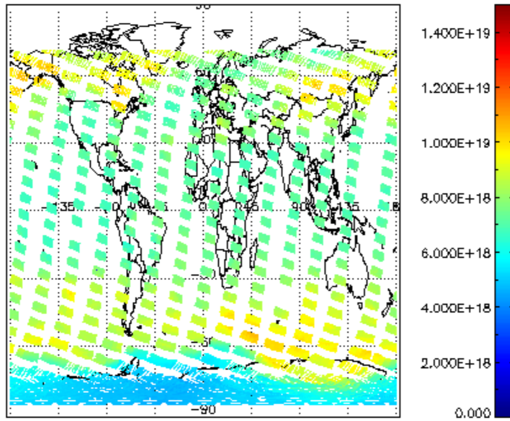
SCIOL2P_NADUV003_vcd for 08NOV2004 00:00:00 to 09NOV2004 00:00:00
