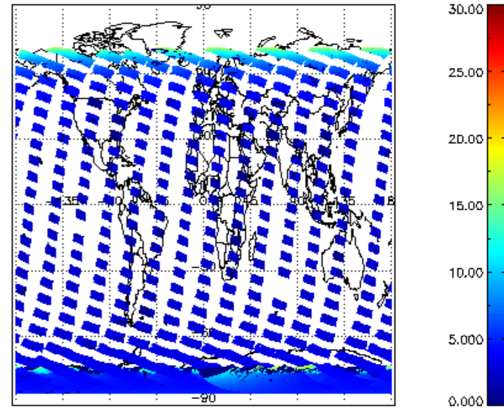
SCIOL2P_NADUV1NO2_amf_cl for 08NOV2004 00:00:00 to 09NOV2004 00:00:00
