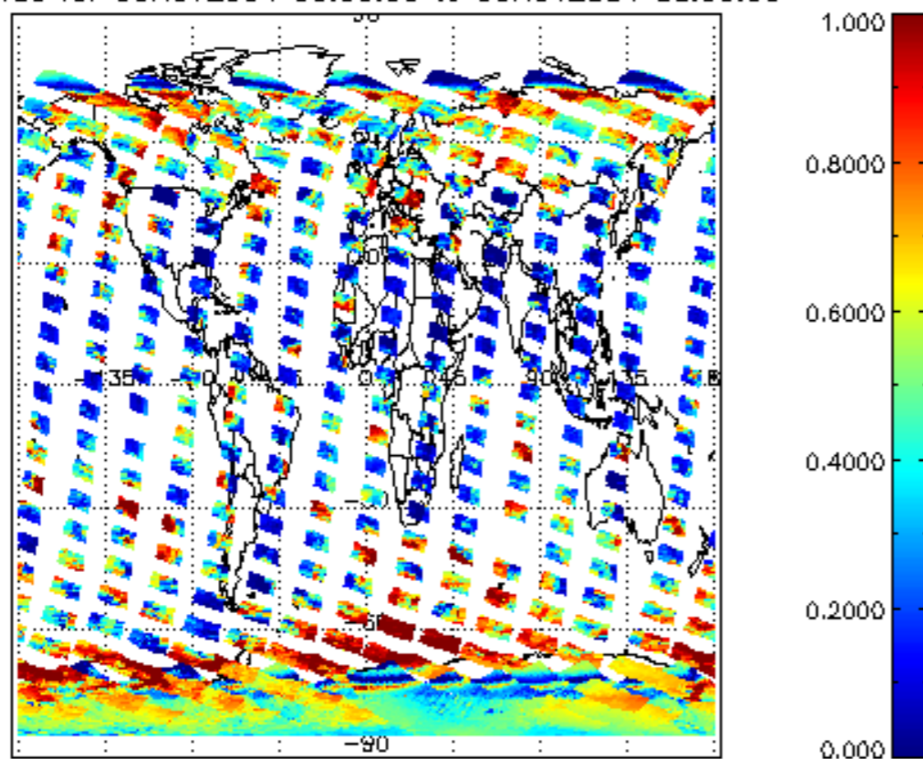
cLfrac for 08NOV2004 00:00:00 to 09NOV2004 00:00:00
