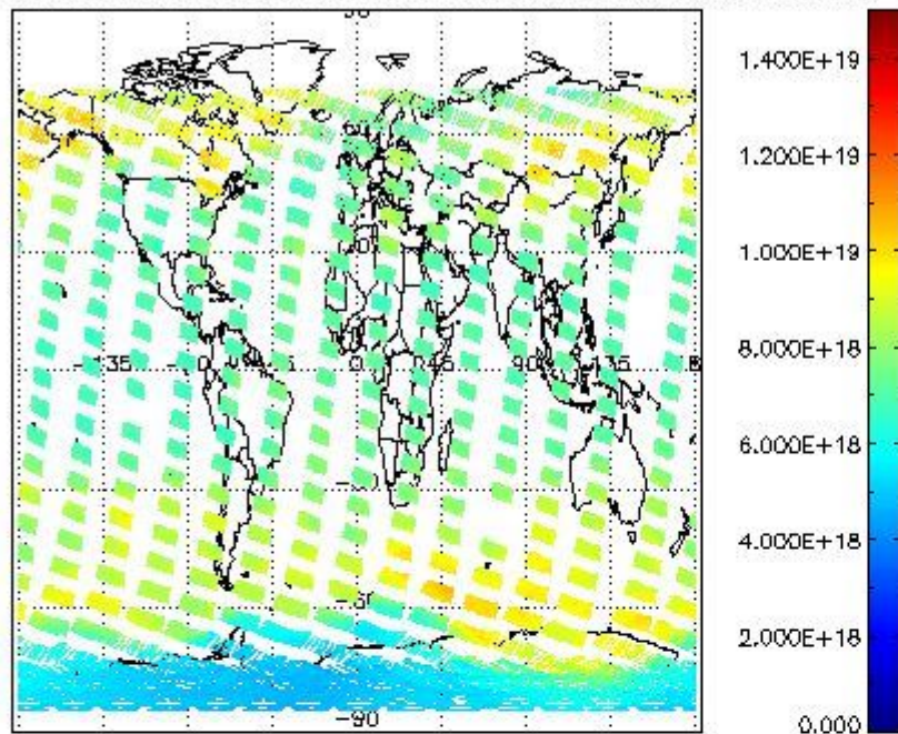
SCIOL2P_NADUV003_vcd for 08NOV2004 00:00:00 to 09NOV2004 00:00:00
