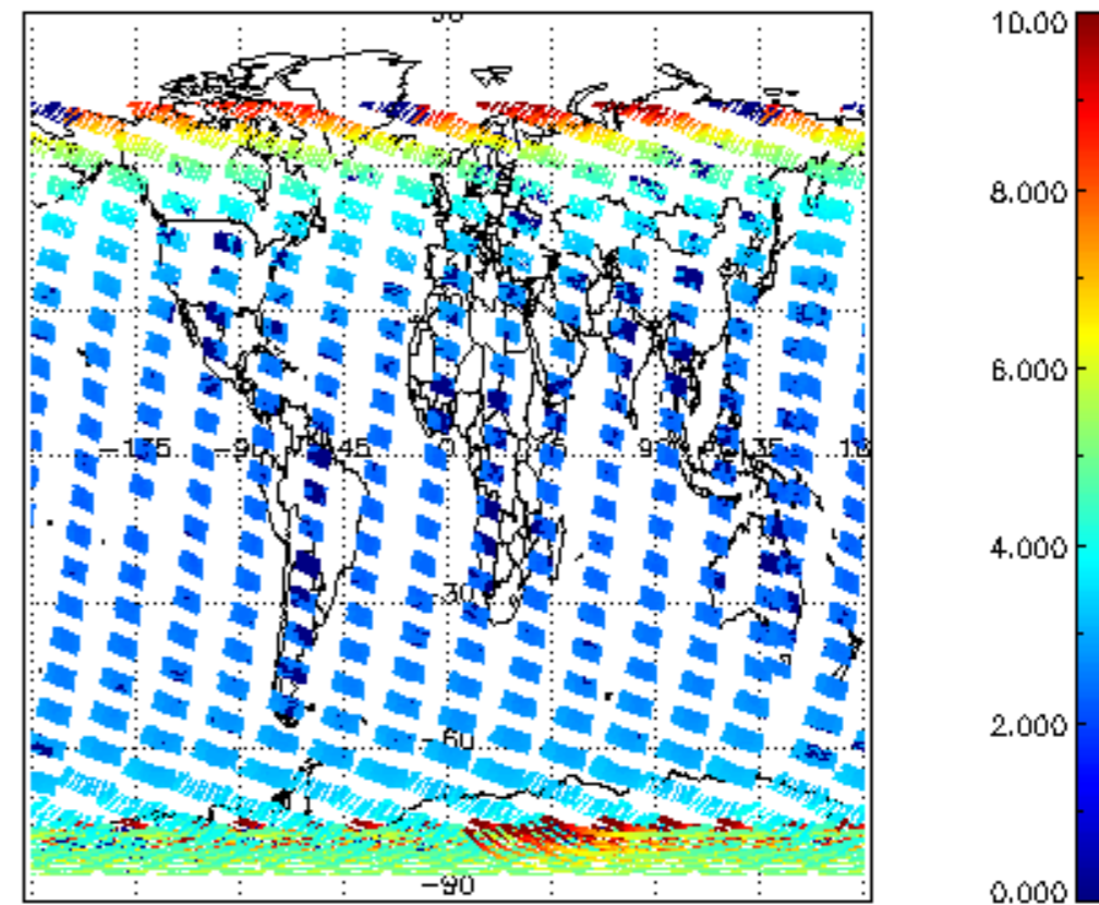
SCIOL2P_NADUV003_amf_cl for 03NOV2004 00:00:00 to 04NOV2004 00:00:00
