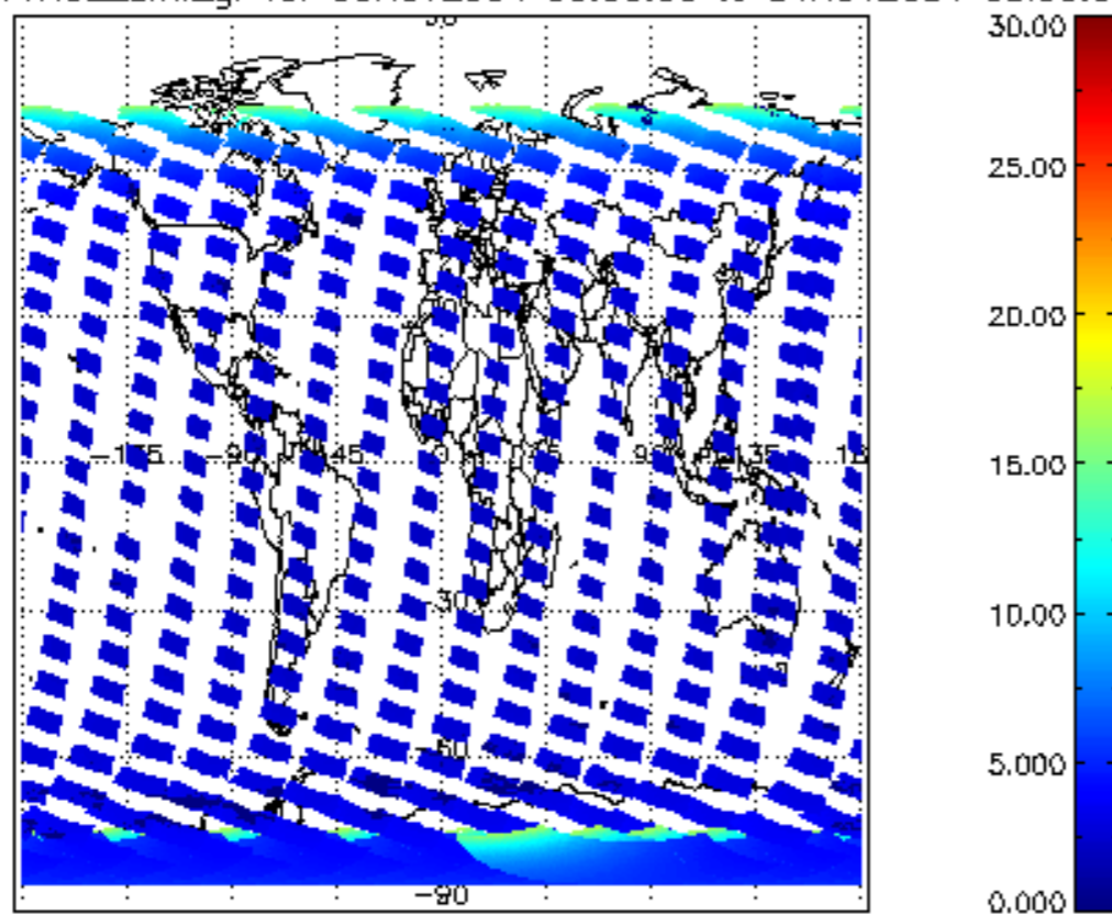
SCIOL2P_NADUV1NO2_amf_gr for 03NOV2004 00:00:00 to 04NOV2004 00:00:00
