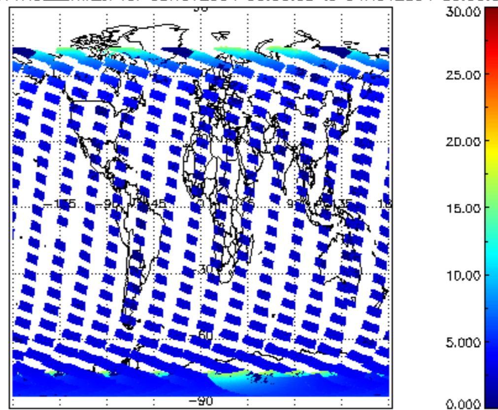
SCIOL2P_NADUV1NO2_amf_cl for 03NOV2004 00:00:00 to 04NOV2004 00:00:00
