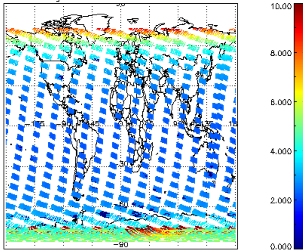
SCIOL2P_NADUV003_amf_gr for 03NOV2004 00:00:00 to 04NOV2004 00:00:00
