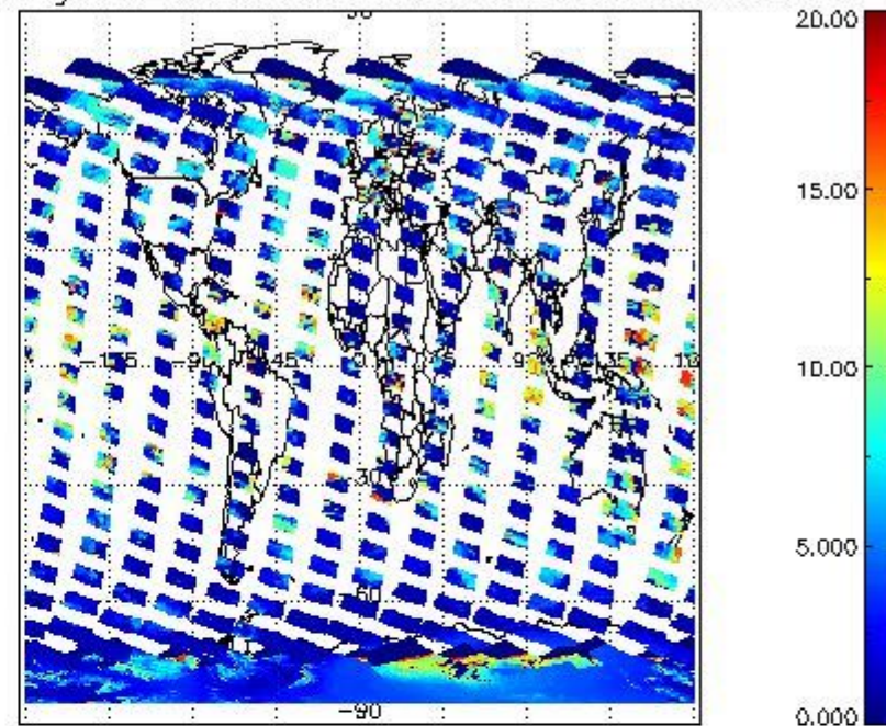
cL_top_height for 03NOV2004 00:00:00 to 04NOV2004 00:00:00
