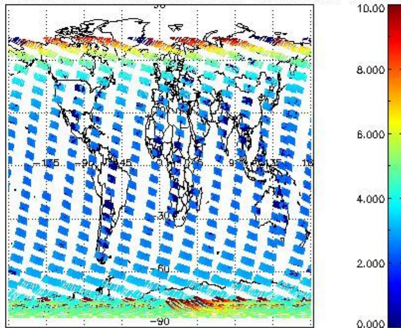
SCIOL2P_NADUV003_amf_cl for 03NOV2004 00:00:00 to 04NOV2004 00:00:00
