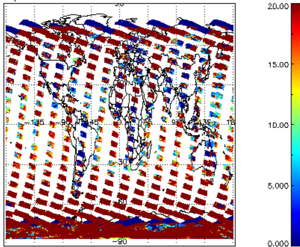
cL_opt_depth for 03NOV2004 00:00:00 to 04NOV2004 00:00:00
