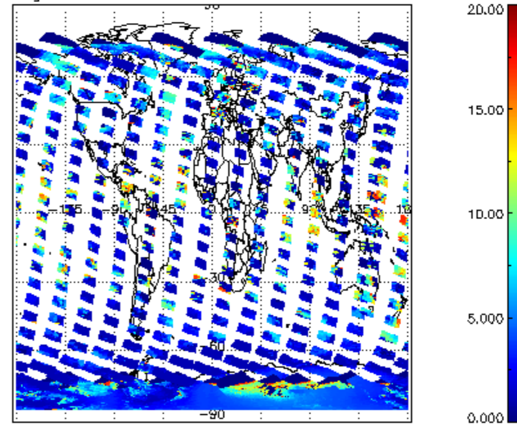
cL_top_height for 03NOV2004 00:00:00 to 04NOV2004 00:00:00
