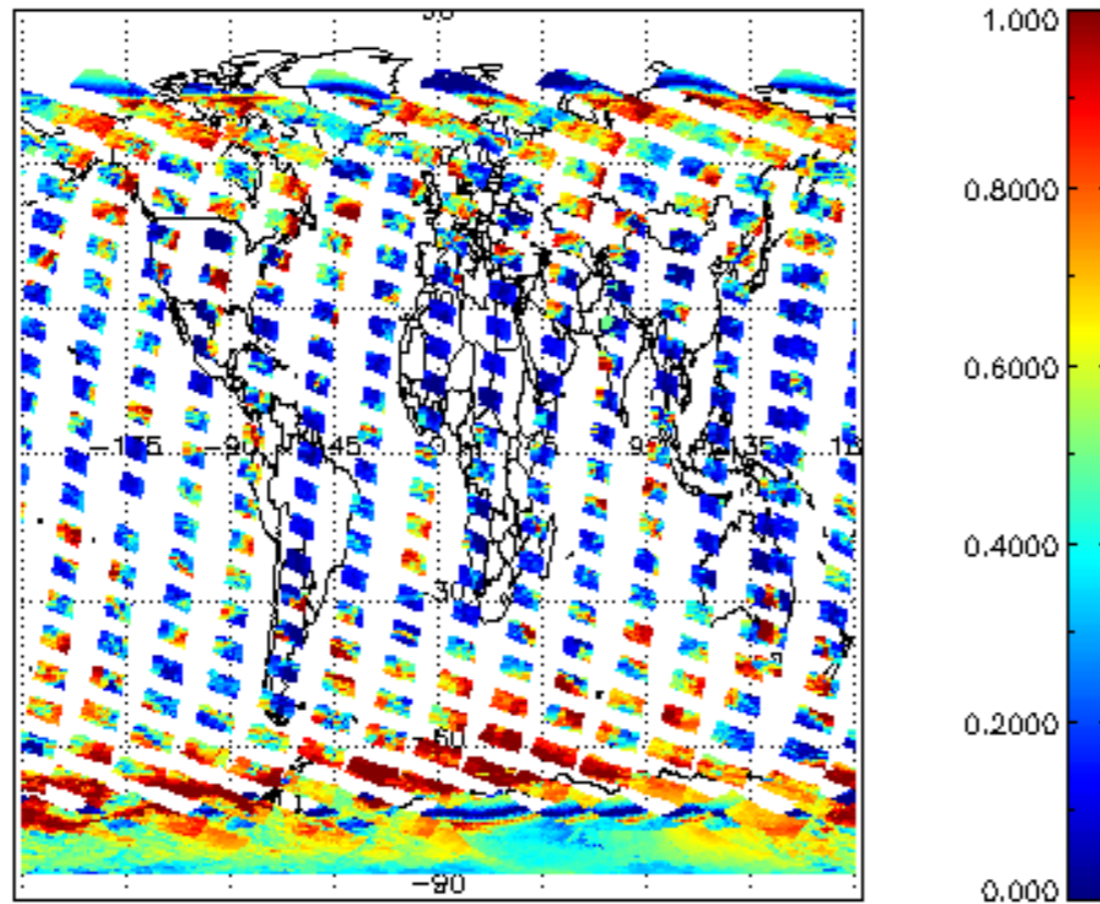
cLfrac for 03NOV2004 00:00:00 to 04NOV2004 00:00:00
