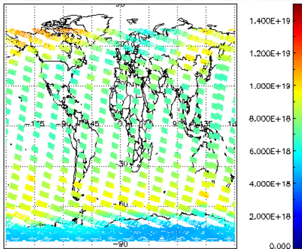
SCIOL2P_NADUV003_vcd for 03NOV2004 00:00:00 to 04NOV2004 00:00:00
