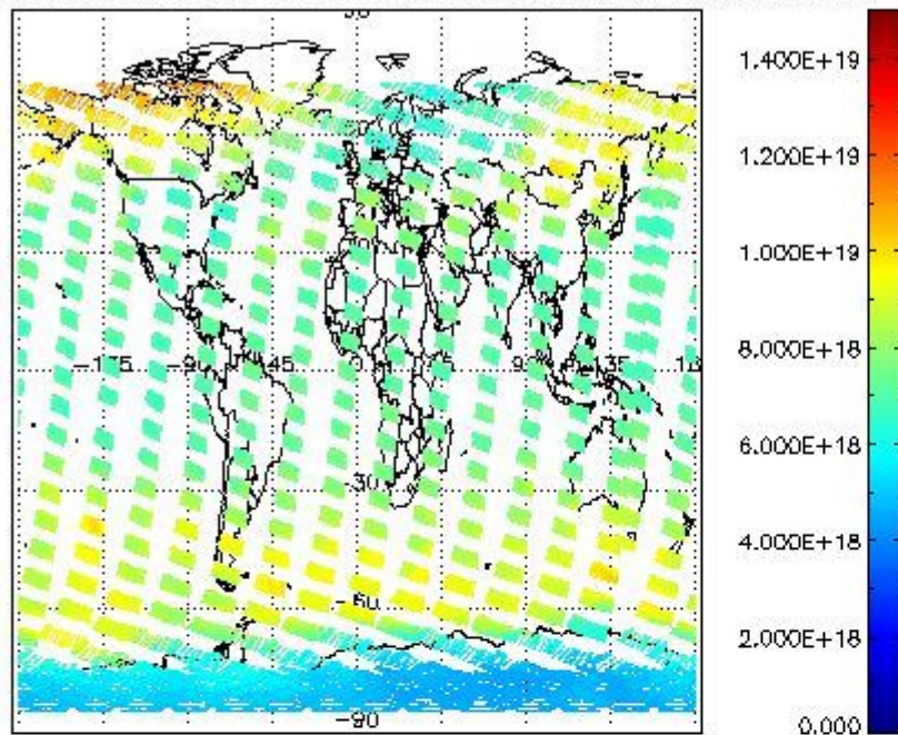
SCIOL2P_NADUV003_vcd for 03NOV2004 00:00:00 to 04NOV2004 00:00:00
