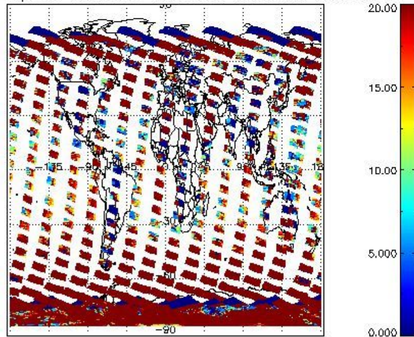
cLopt_depth for 03NOV2004 00:00:00 to 04NOV2004 00:00:00
