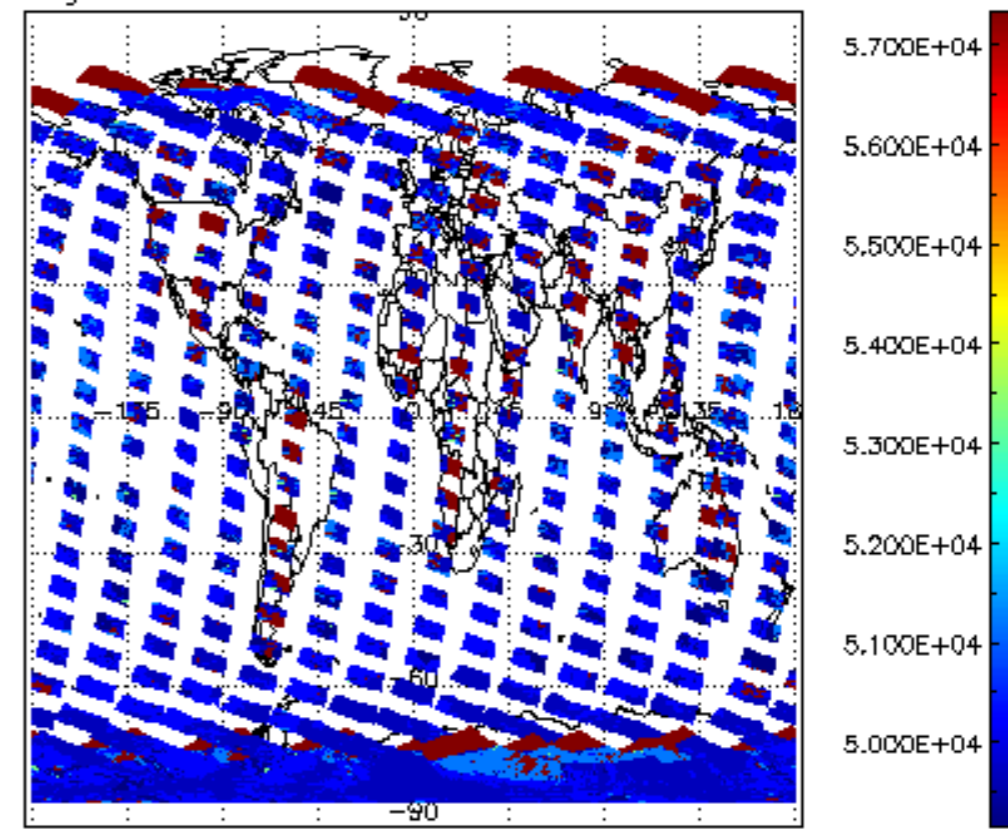
cloud_flags for 03NOV2004 00:00:00 to 04NOV2004 00:00:00
