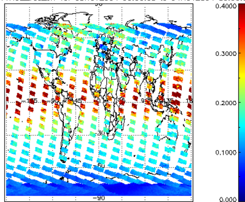
SCIOL2P_NADUV1NO2_vcd_err for 03NOV2004 00:00:00 to 04NOV2004 00:00:00
