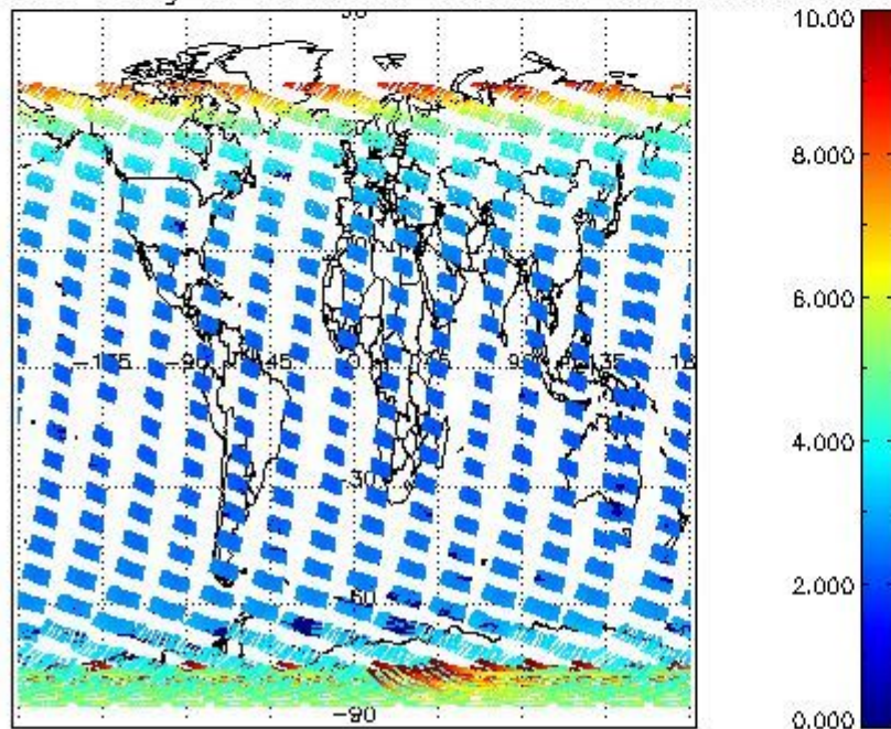
SCIOL2P_NADUV003_amf_gr for 03NOV2004 00:00:00 to 04NOV2004 00:00:00
