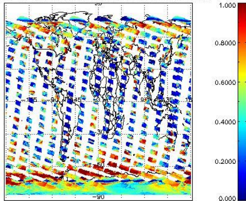
cLfrac for 03NOV2004 00:00:00 to 04NOV2004 00:00:00
