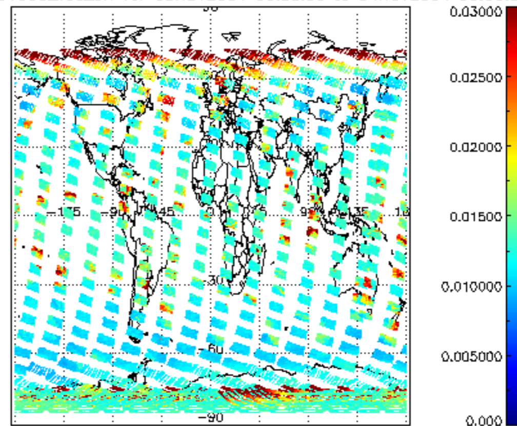
SCIOL2P_NADUV003_vcd_err for 03NOV2004 00:00:00 to 04NOV2004 00:00:00
