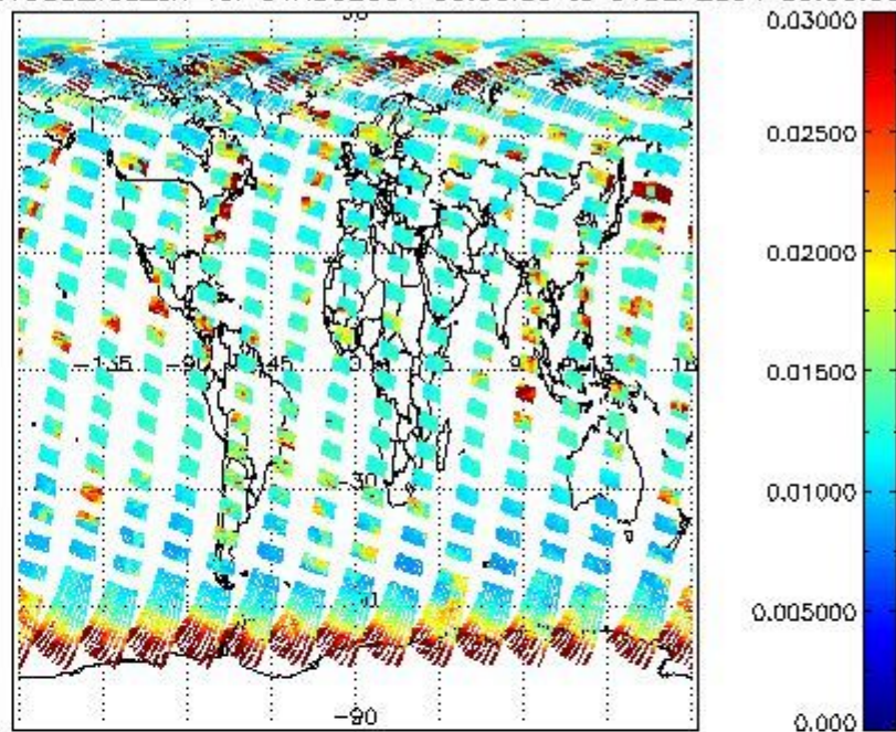
SCIOL2P_NADUV003_vcd_err for 31AUG2004 00:00:00 to 01SEP2004 00:00:00
