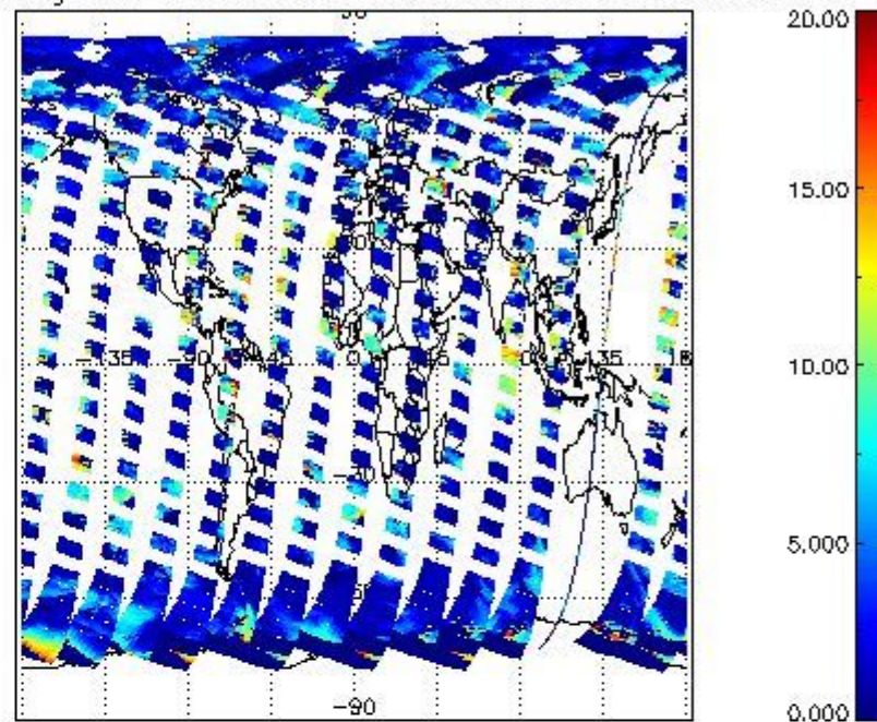
cL_top_height for 30AUG2004 00:00:00 to 31AUG2004 00:00:00
