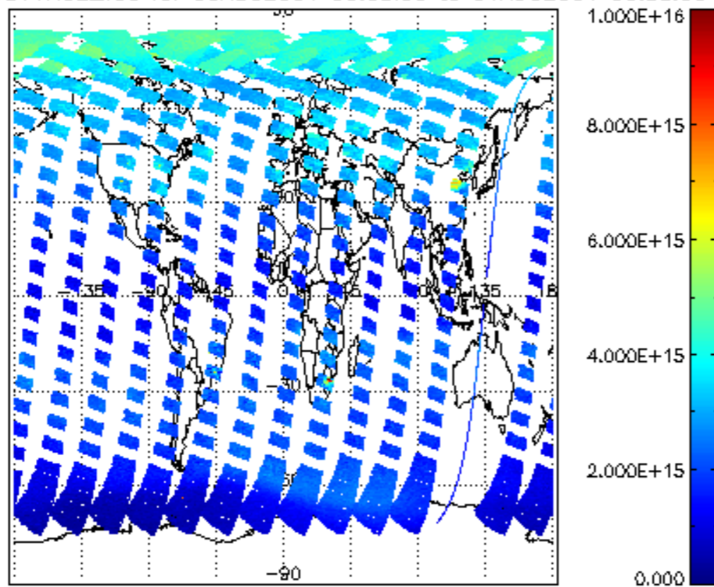
SCIOL2P_NADUV1NO2_vcd for 30AUG2004 00:00:00 to 31AUG2004 00:00:00
