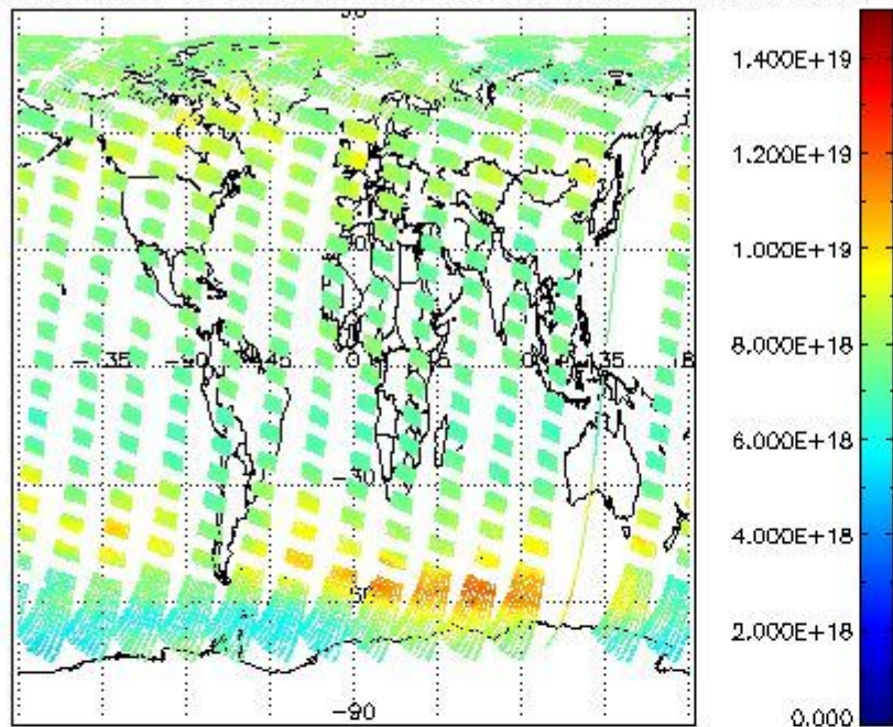
SCIOL2P_NADUV003_vcd for 30AUG2004 00:00:00 to 31AUG2004 00:00:00
