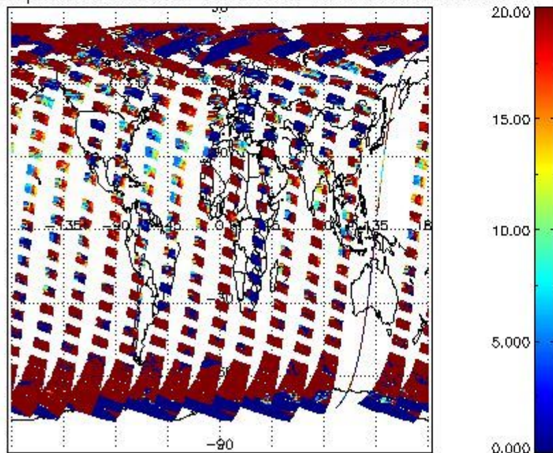
cL_opt_depth for 30AUG2004 00:00:00 to 31AUG2004 00:00:00
