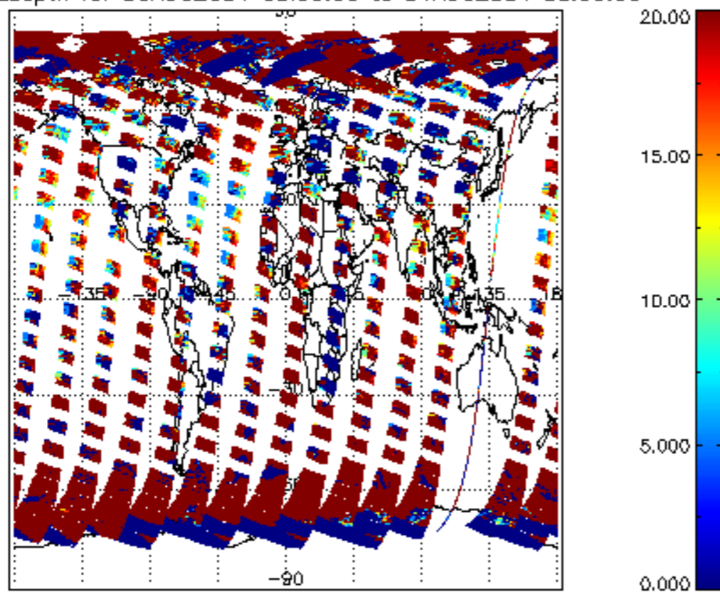
cL_opt_depth for 30AUG2004 00:00:00 to 31AUG2004 00:00:00
