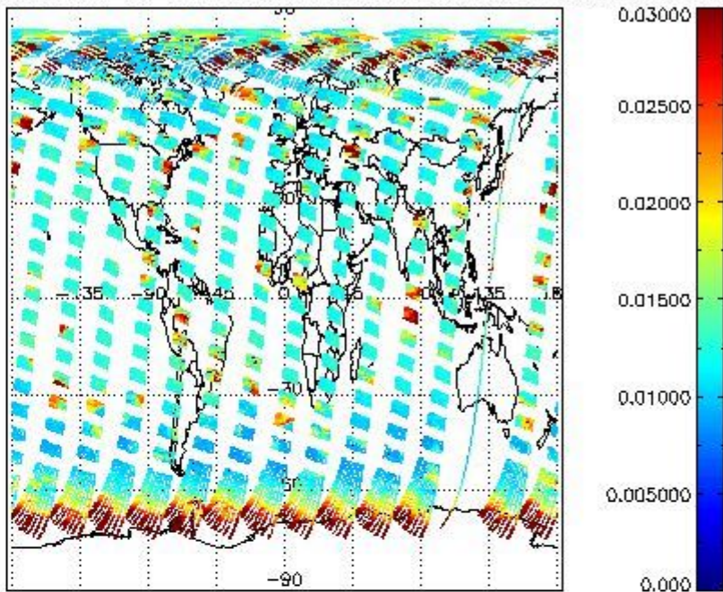
SCIOL2P_NADUV003_vcd_err for 30AUG2004 00:00:00 to 31AUG2004 00:00:00
