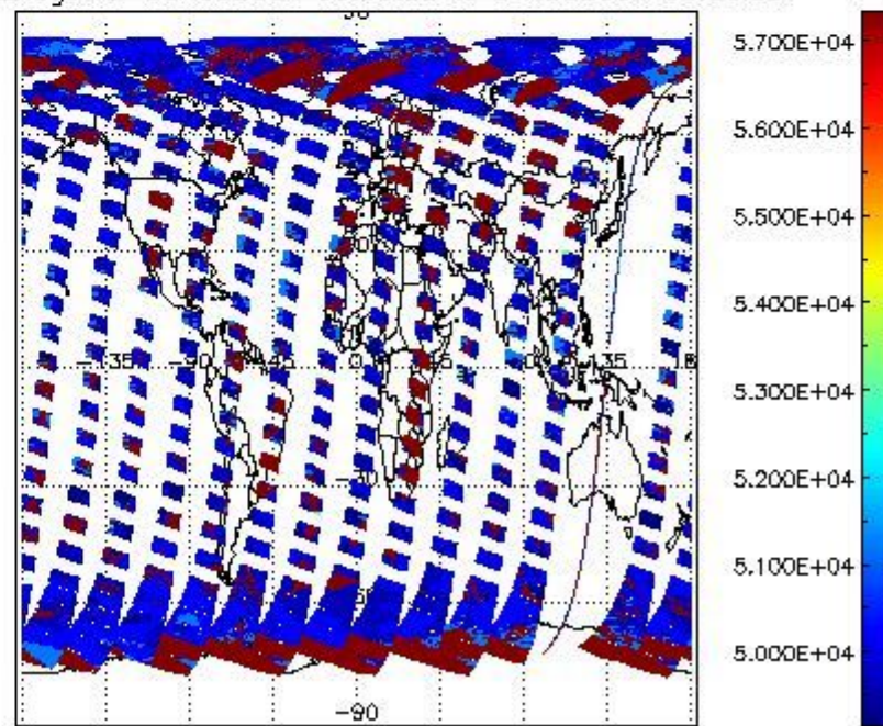
cloud_flags for 30AUG2004 00:00:00 to 31AUG2004 00:00:00
