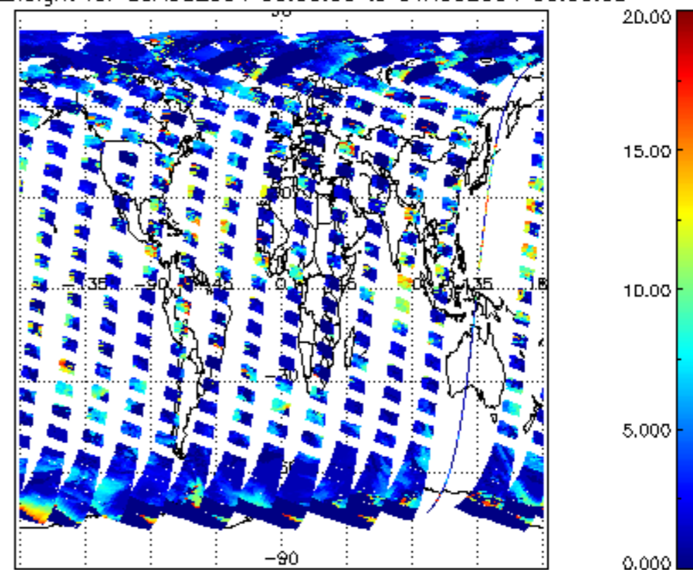
cL_top_height for 30AUG2004 00:00:00 to 31AUG2004 00:00:00
