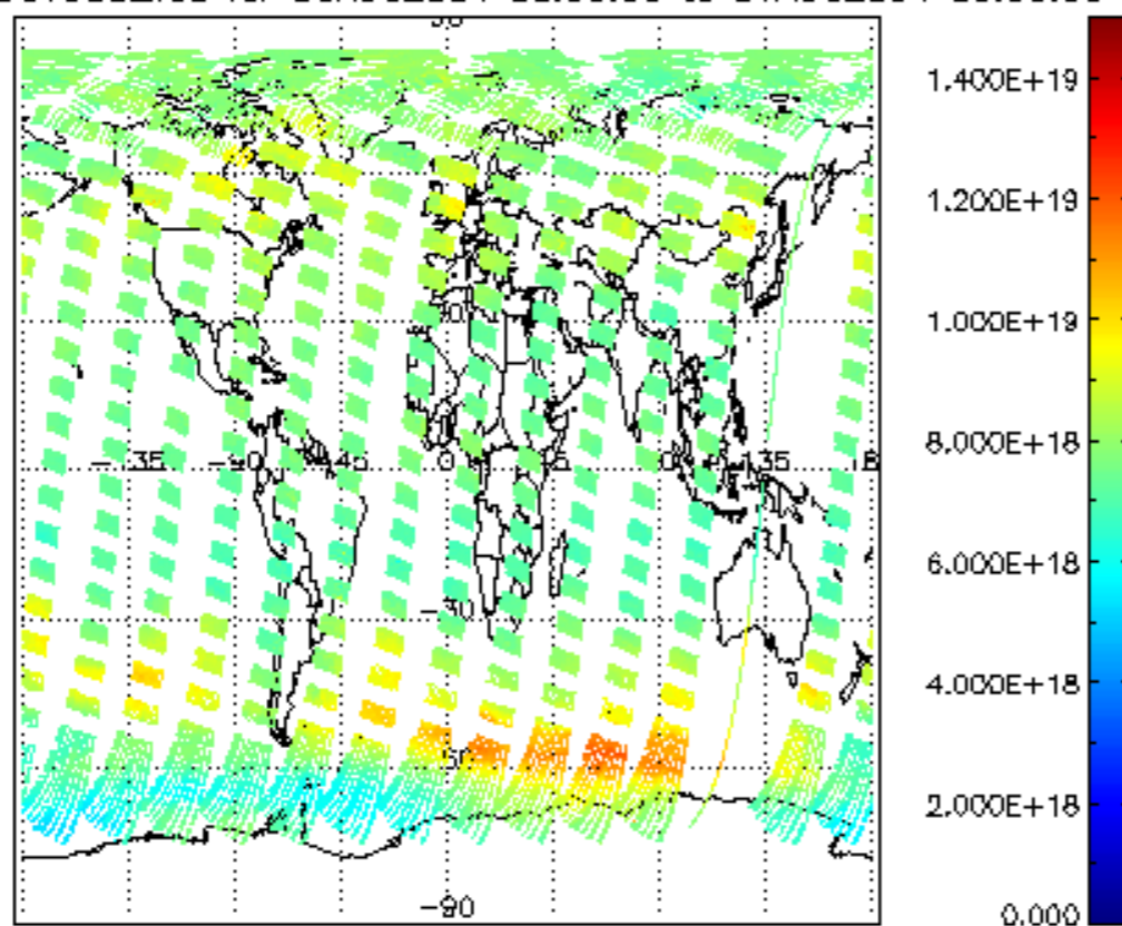
SCIOL2P_NADUV003_vcd for 30AUG2004 00:00:00 to 31AUG2004 00:00:00
