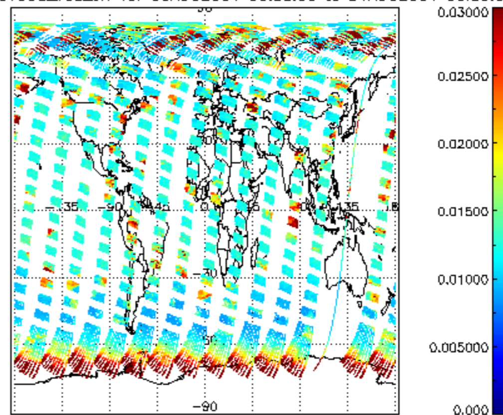
SCIOL2P_NADUV003_vcd_err for 30AUG2004 00:00:00 to 31AUG2004 00:00:00
