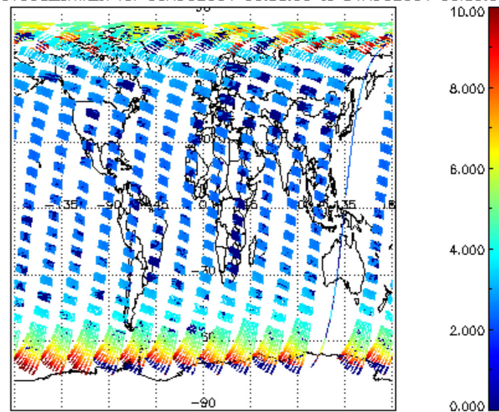
SCIOL2P_NADUV003_amf_cl for 30AUG2004 00:00:00 to 31AUG2004 00:00:00
