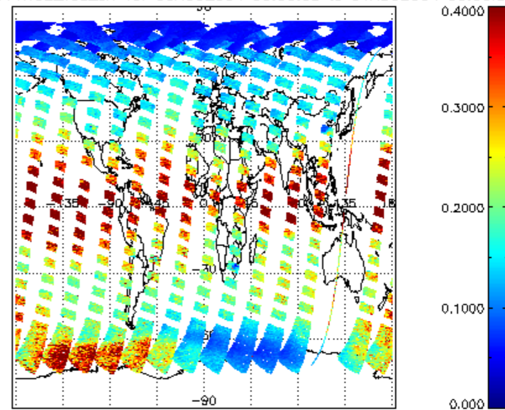
SCIOL2P_NADUV1NO2_vcd_err for 30AUG2004 00:00:00 to 31AUG2004 00:00:00
