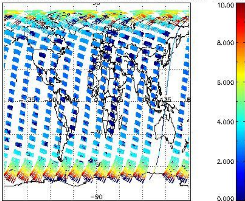
SCIOL2P_NADUV003_amf_cl for 30AUG2004 00:00:00 to 31AUG2004 00:00:00
