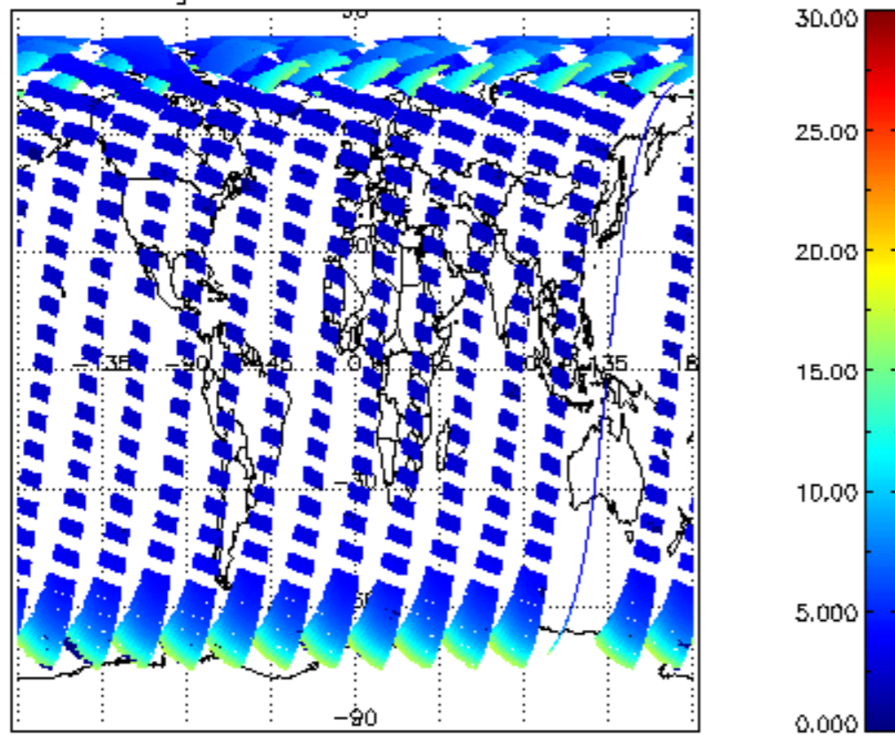
SCIOL2P_NADUV1NO2_amf_gr for 30AUG2004 00:00:00 to 31AUG2004 00:00:00
