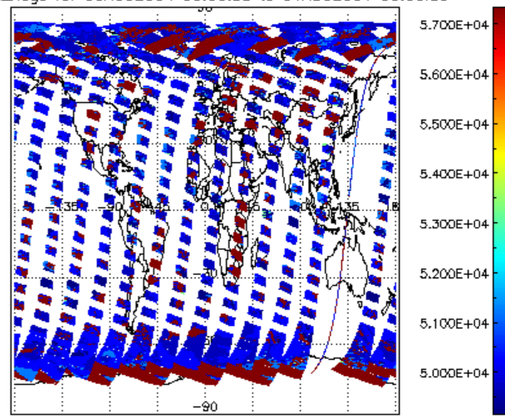
cloud_flags for 30AUG2004 00:00:00 to 31AUG2004 00:00:00
