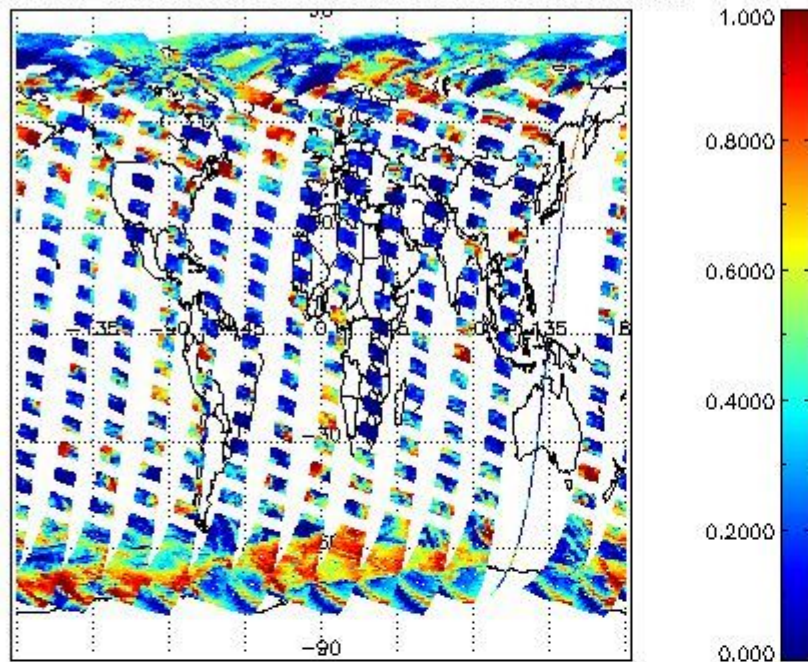
cL_frac for 30AUG2004 00:00:00 to 31AUG2004 00:00:00
