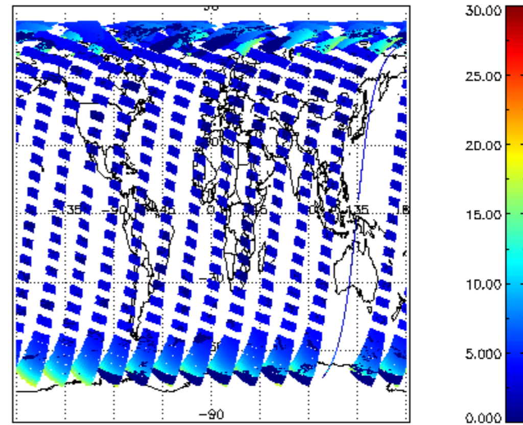
SCIOL2P_NADUV1NO2_amf_cl for 30AUG2004 00:00:00 to 31AUG2004 00:00:00
