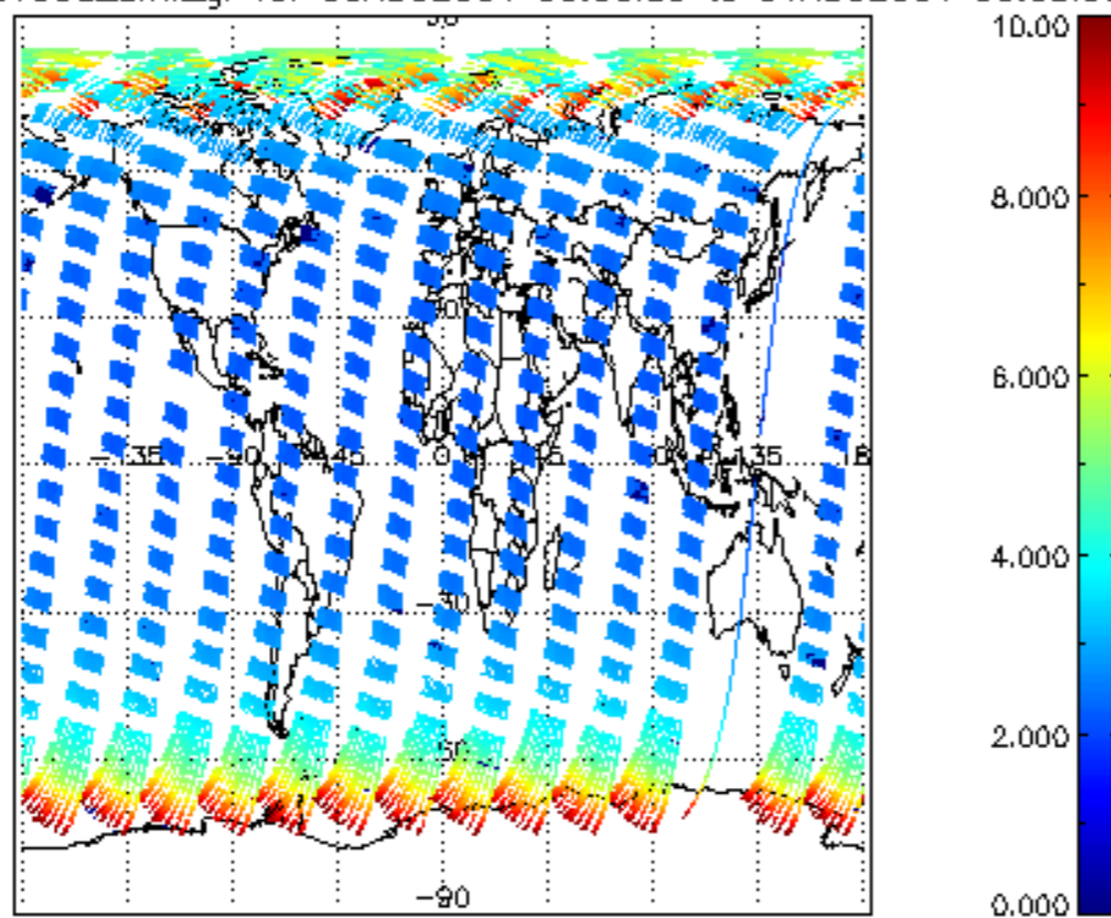
SCIOL2P_NADUV003_amf_gr for 30AUG2004 00:00:00 to 31AUG2004 00:00:00
