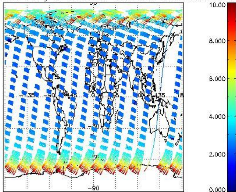
SCIOL2P_NADUV003_amf_gr for 30AUG2004 00:00:00 to 31AUG2004 00:00:00
