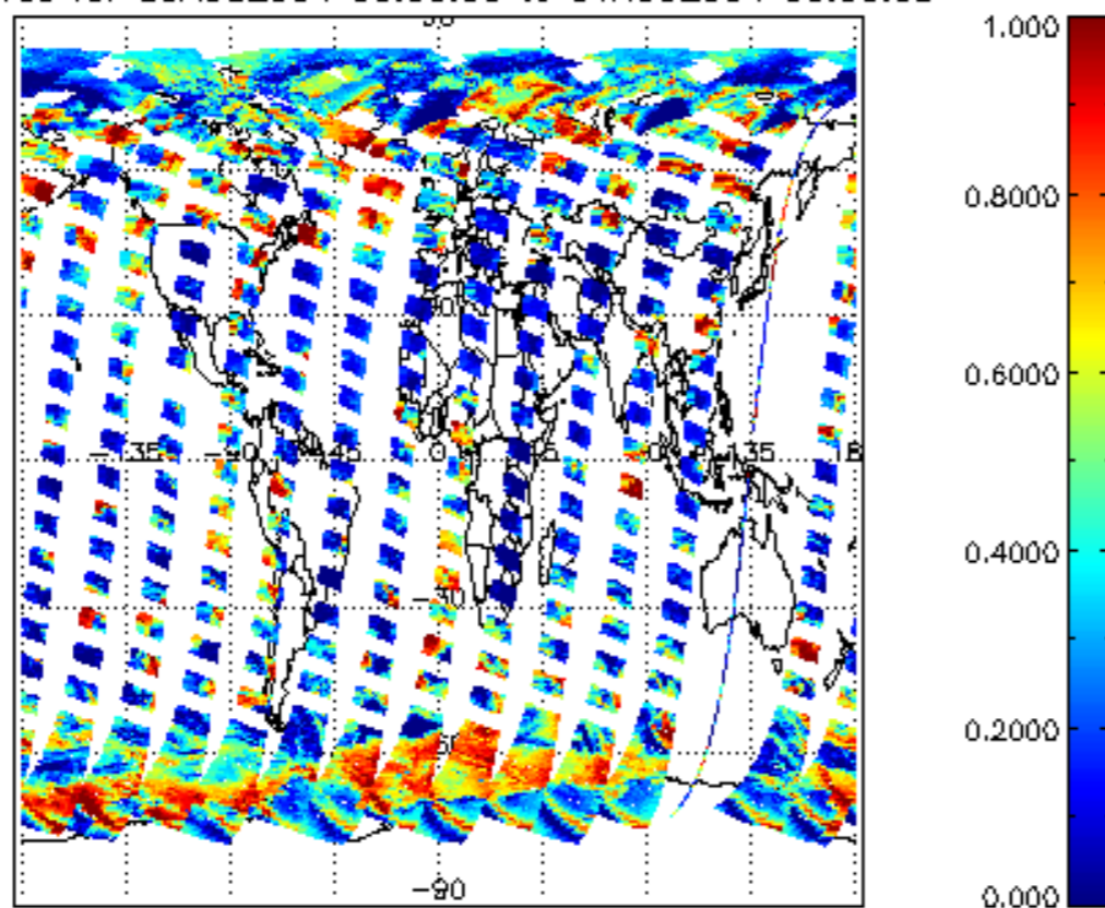
cL_frac for 30AUG2004 00:00:00 to 31AUG2004 00:00:00
