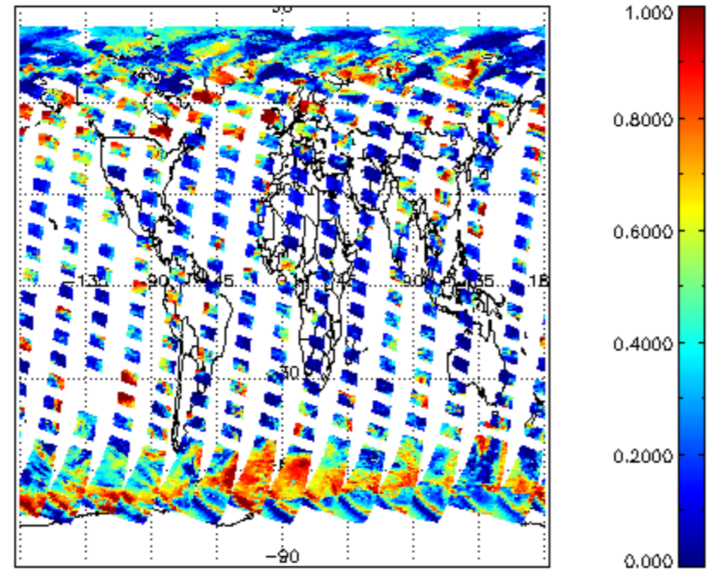
cI_frac for 26AUG2004 00:00:00 to 27AUG2004 00:00:00
