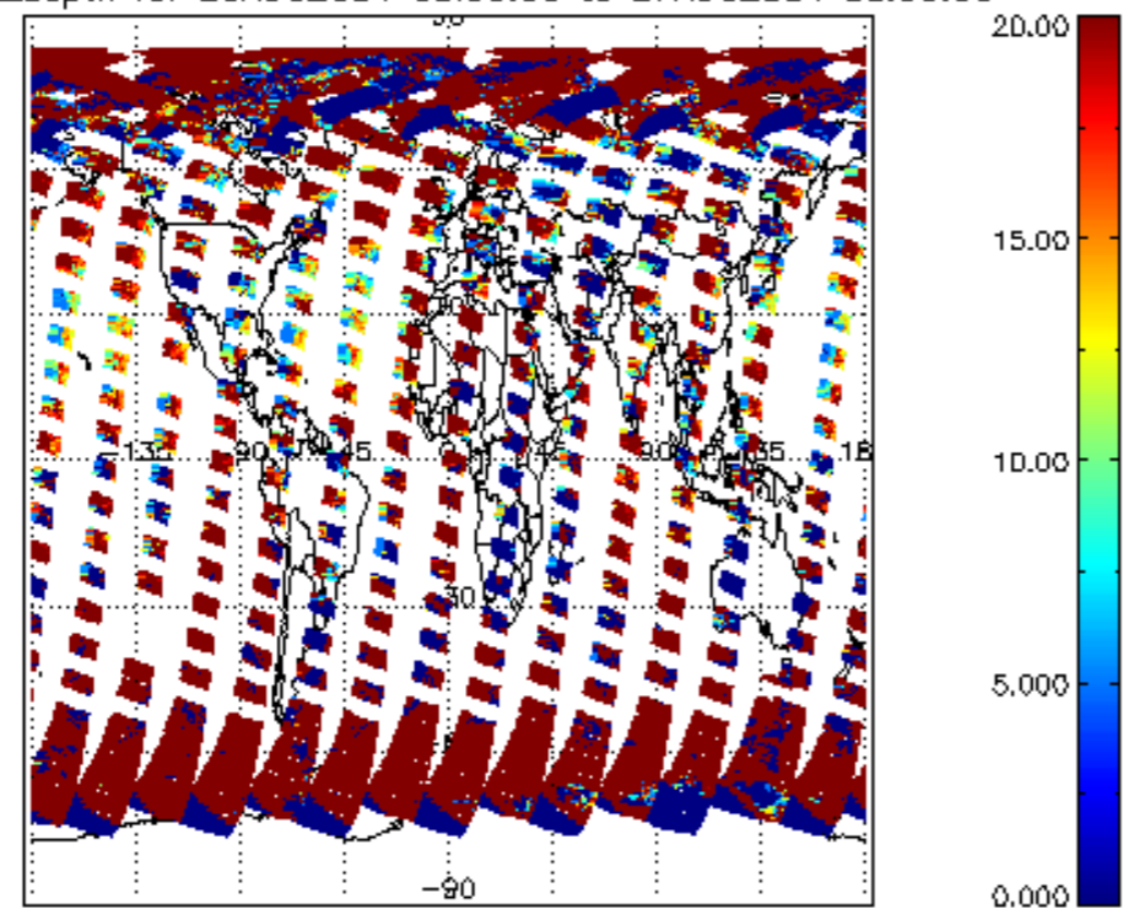
cI_opt_depth for 26AUG2004 00:00:00 to 27AUG2004 00:00:00
