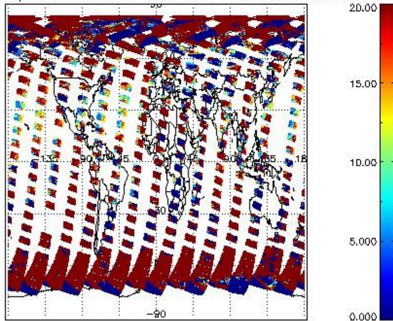
cL_opt_depth for 26AUG2004 00:00:00 to 27AUG2004 00:00:00
