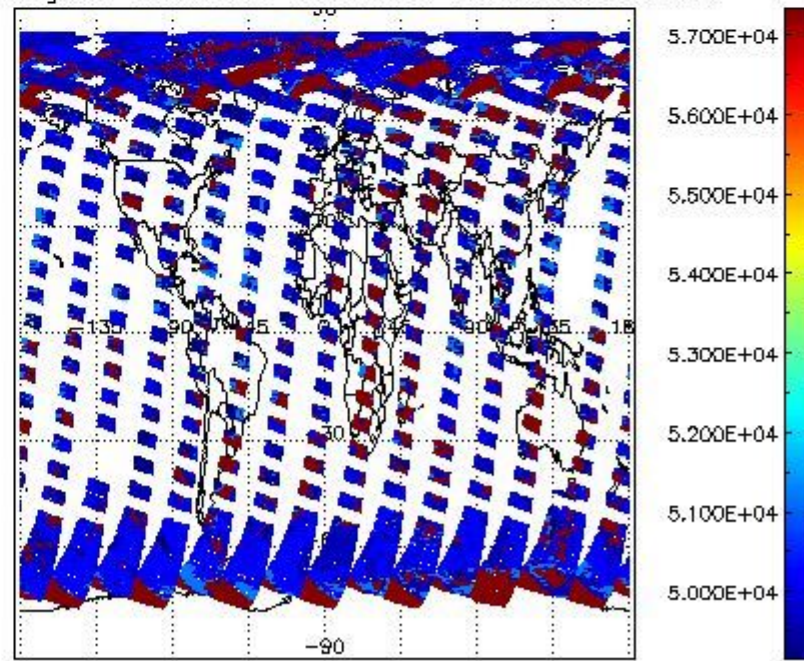
cloud_flags for 26AUG2004 00:00:00 to 27AUG2004 00:00:00
