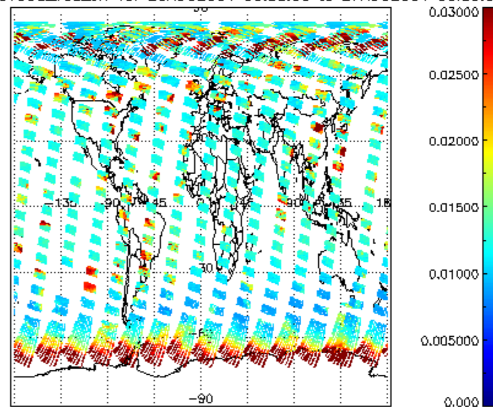
SCIOL2P_NADUV003_vcd_err for 26AUG2004 00:00:00 to 27AUG2004 00:00:00
