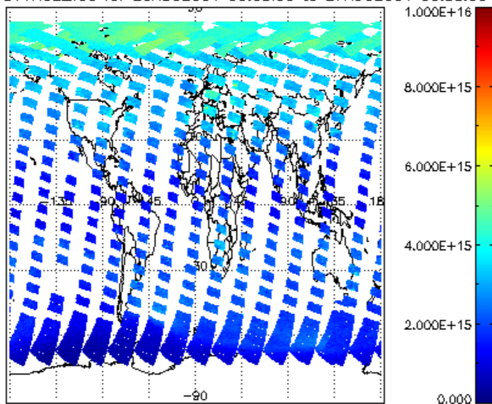
SCIOL2P_NADUV1NO2_vcd for 26AUG2004 00:00:00 to 27AUG2004 00:00:00
