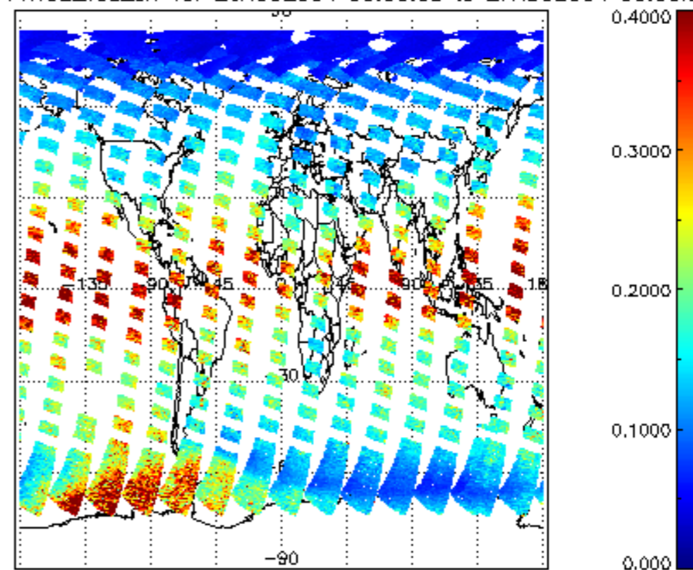
SCIOL2P_NADUV1NO2_vcd_err for 26AUG2004 00:00:00 to 27AUG2004 00:00:00
