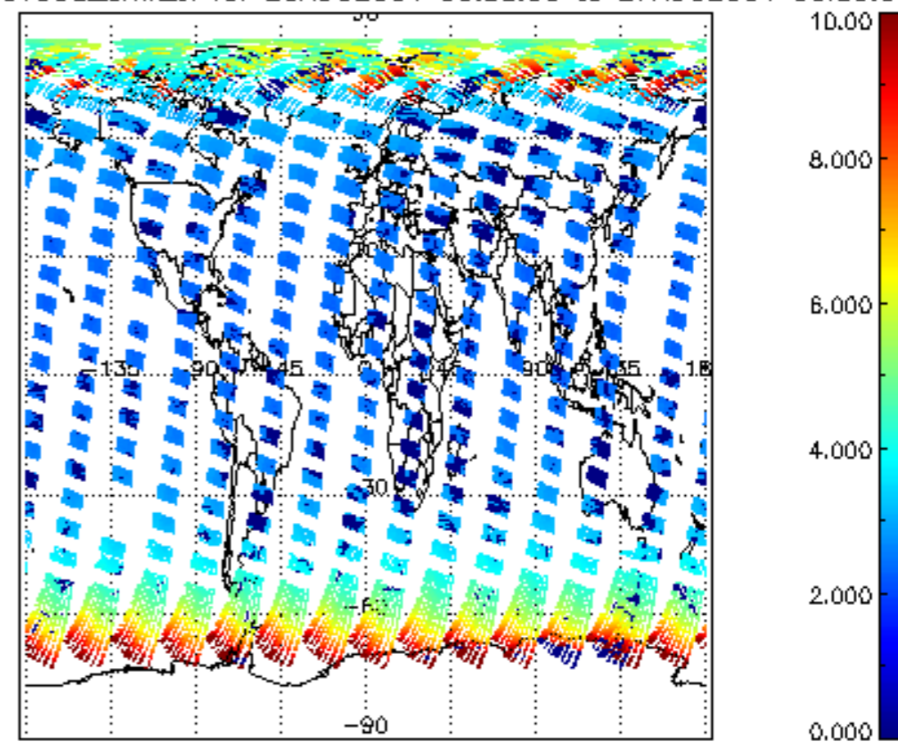
SCIOL2P_NADUV003_amf_cl for 26AUG2004 00:00:00 to 27AUG2004 00:00:00
