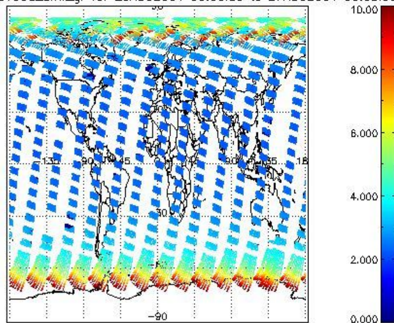
SCIOL2P_NADUV003_amf_gr for 26AUG2004 00:00:00 to 27AUG2004 00:00:00
