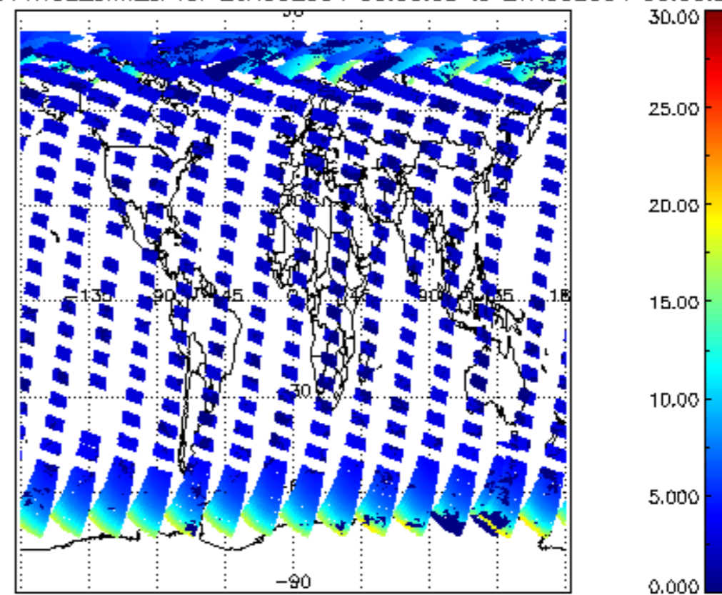
SCIOL2P_NADUV1NO2_amf_cl for 26AUG2004 00:00:00 to 27AUG2004 00:00:00
