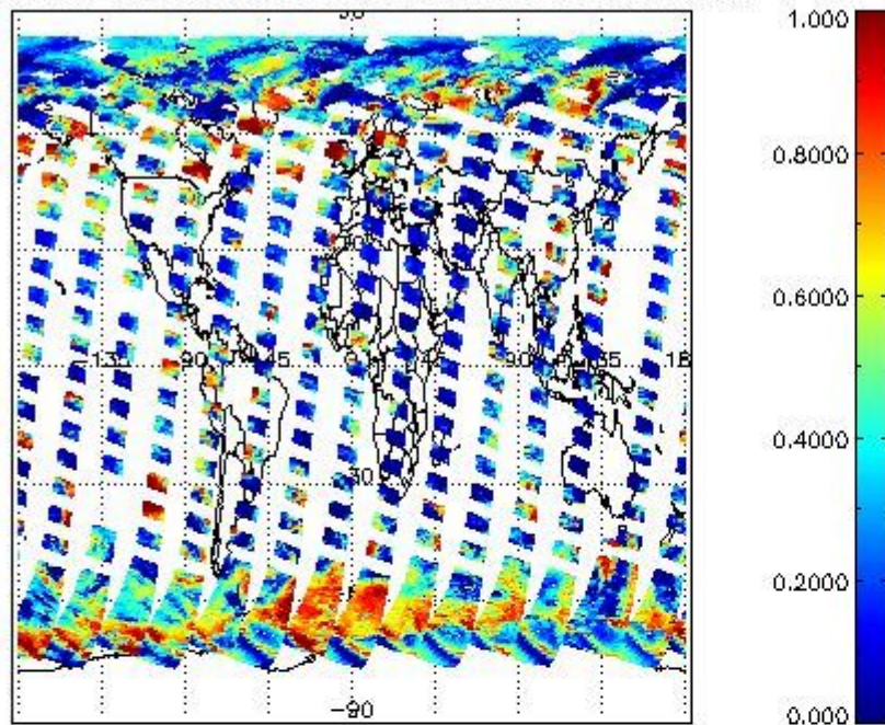
cL_frac for 26AUG2004 00:00:00 to 27AUG2004 00:00:00
