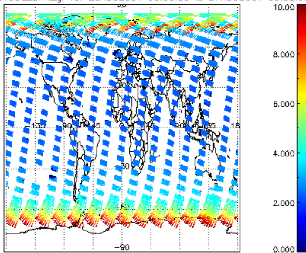
SCIOL2P_NADUV003_amf_gr for 26AUG2004 00:00:00 to 27AUG2004 00:00:00
