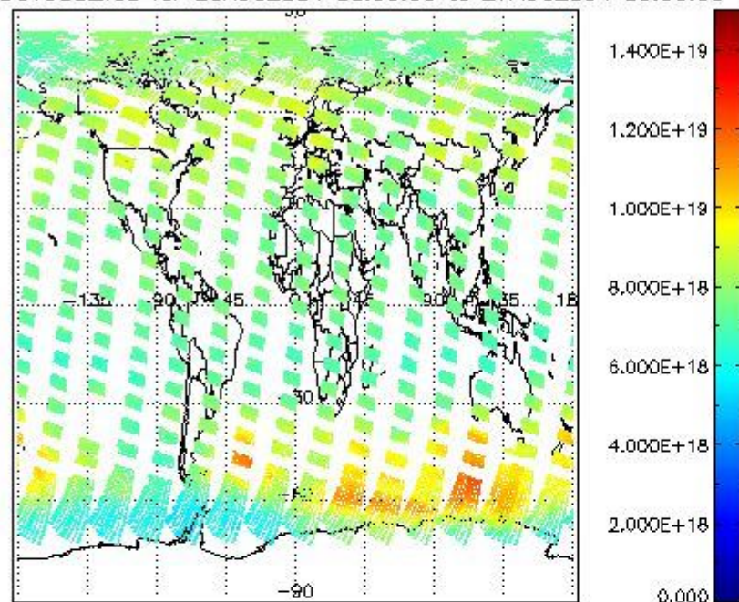
SCIOL2P_NADUV003_vcd for 26AUG2004 00:00:00 to 27AUG2004 00:00:00
