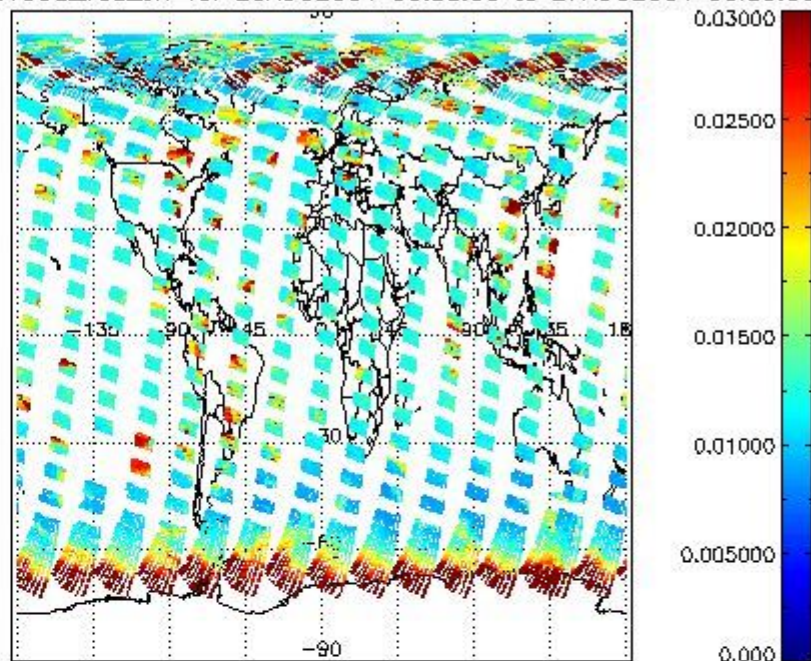
SCIOL2P_NADUV003_vcd_err for 26AUG2004 00:00:00 to 27AUG2004 00:00:00
