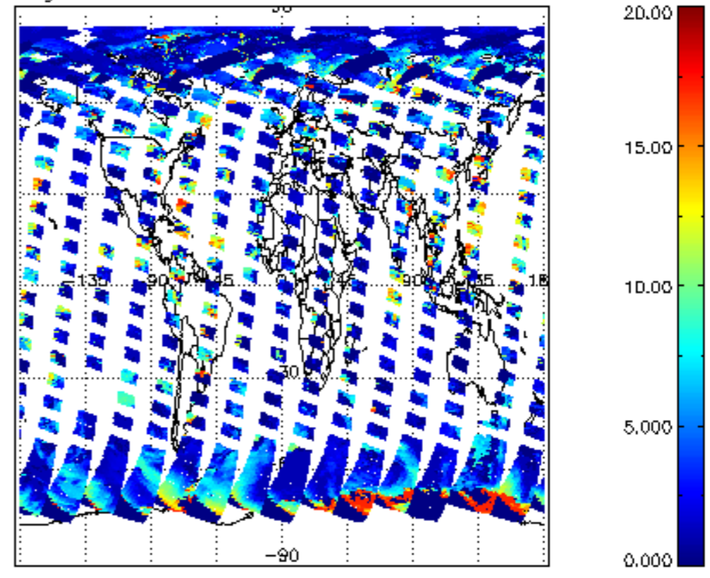
cI_top_height for 26AUG2004 00:00:00 to 27AUG2004 00:00:00
