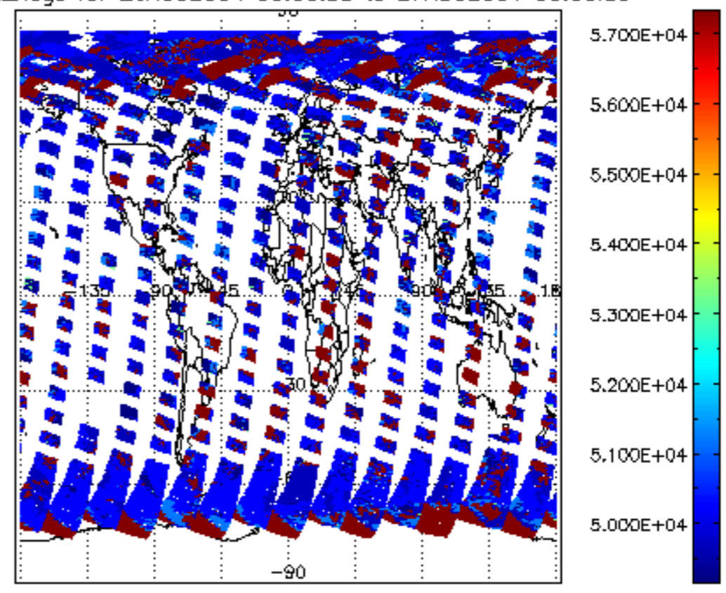
cloud_flags for 26AUG2004 00:00:00 to 27AUG2004 00:00:00
