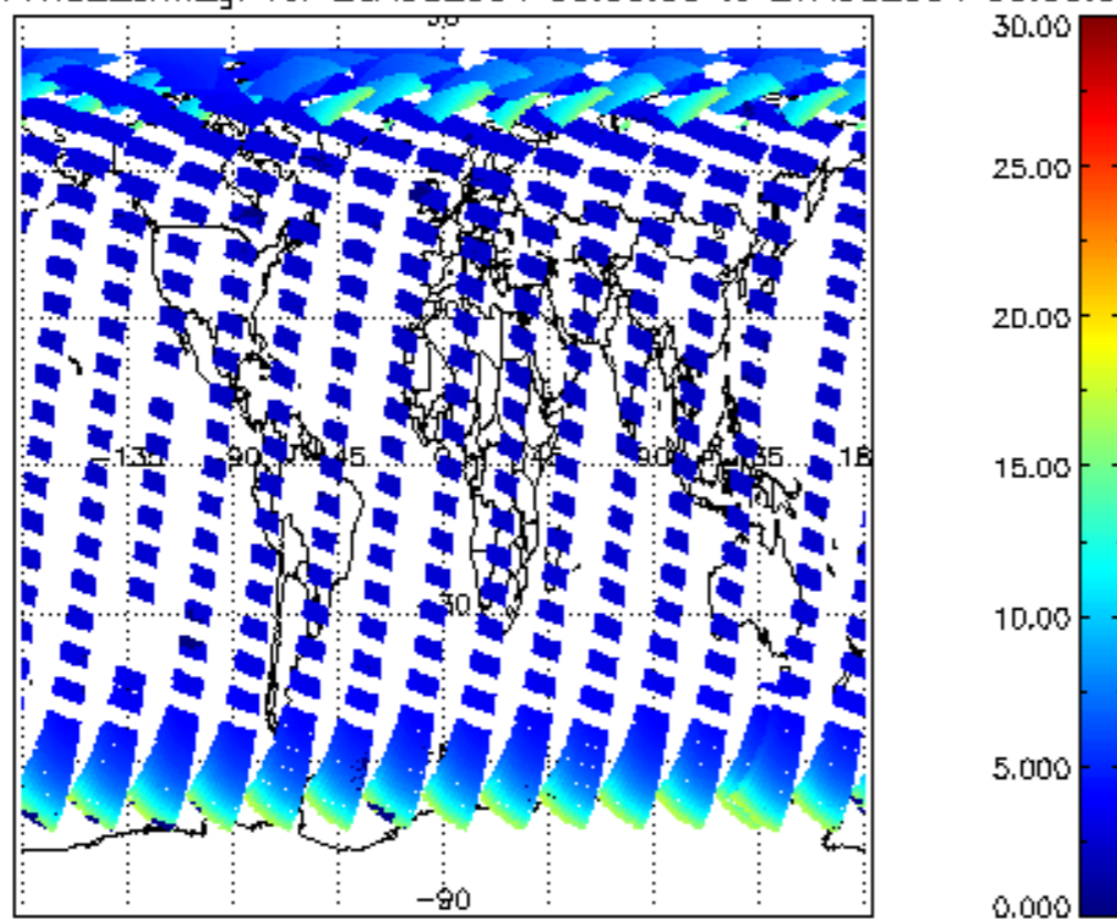
SCIOL2P_NADUV1NO2_amf_gr for 26AUG2004 00:00:00 to 27AUG2004 00:00:00
