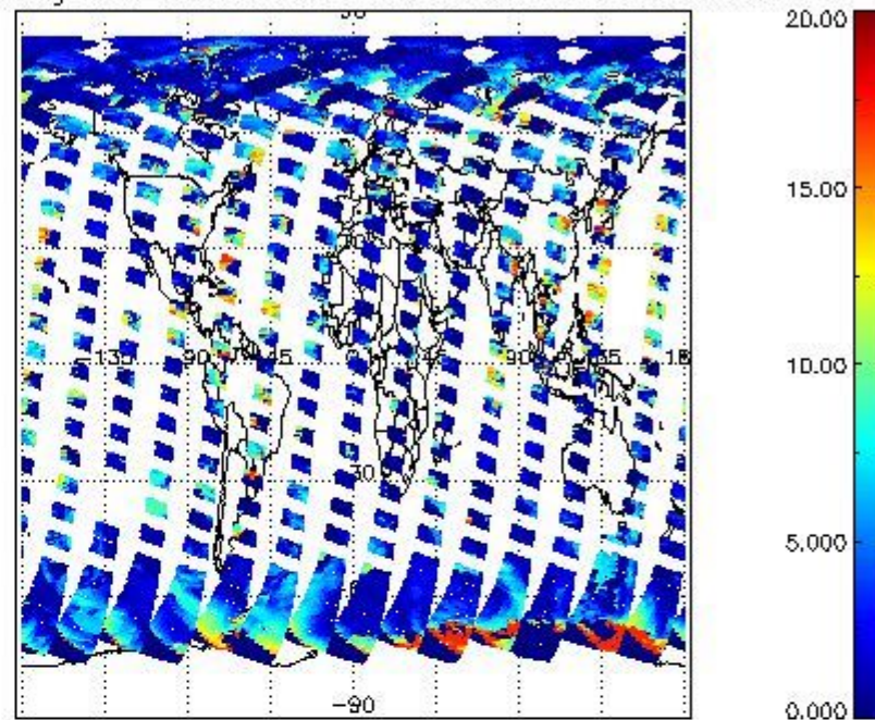
cL_top_height for 26AUG2004 00:00:00 to 27AUG2004 00:00:00
