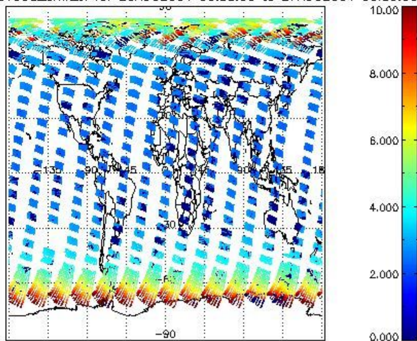
SCIOL2P_NADUV003_amf_cl for 26AUG2004 00:00:00 to 27AUG2004 00:00:00
