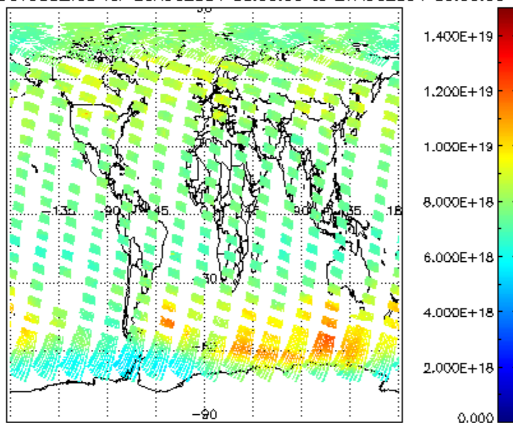
SCIOL2P_NADUV003_vcd for 26AUG2004 00:00:00 to 27AUG2004 00:00:00
