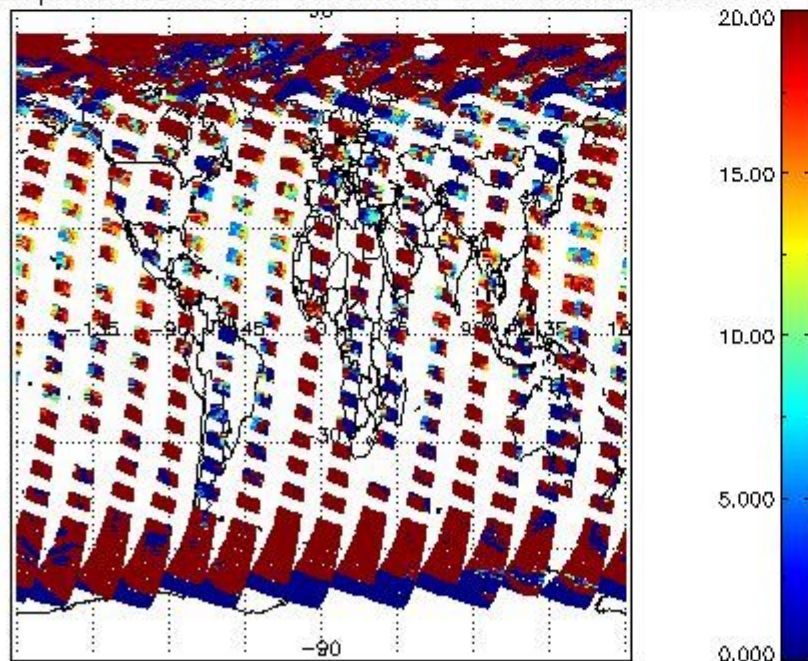
cL_opt_depth for 25AUG2004 00:00:00 to 26AUG2004 00:00:00
