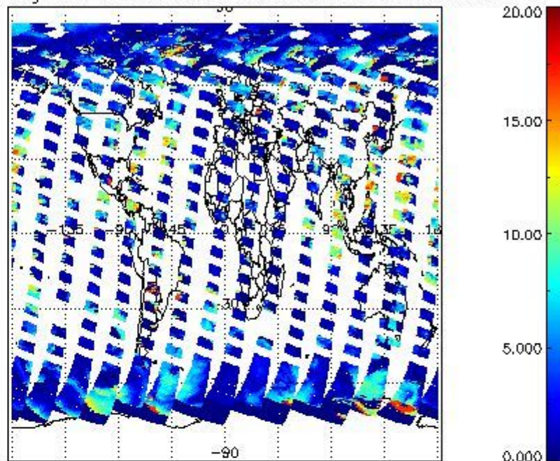
cL_top_height for 25AUG2004 00:00:00 to 26AUG2004 00:00:00
