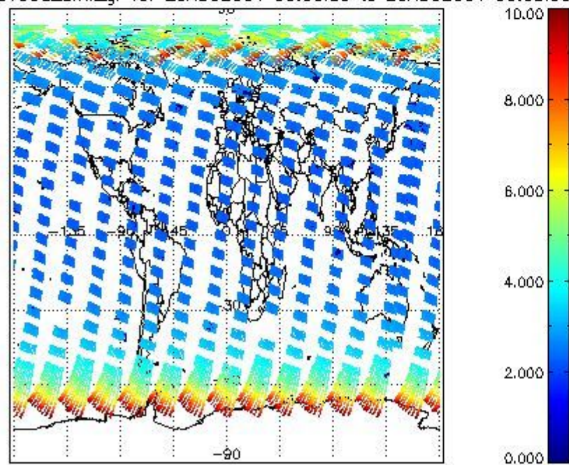
SCIOL2P_NADUV003_amf_gr for 25AUG2004 00:00:00 to 26AUG2004 00:00:00
