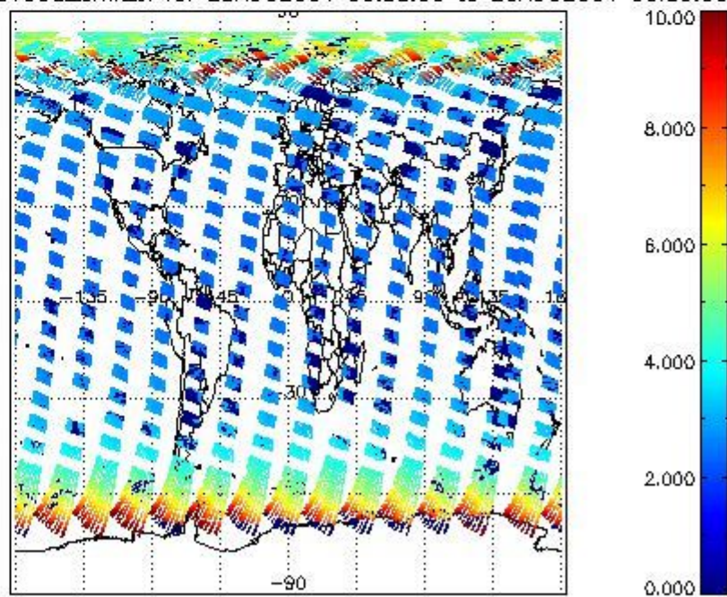
SCIOL2P_NADUV003_amf_sl for 25AUG2004 00:00:00 to 26AUG2004 00:00:00
