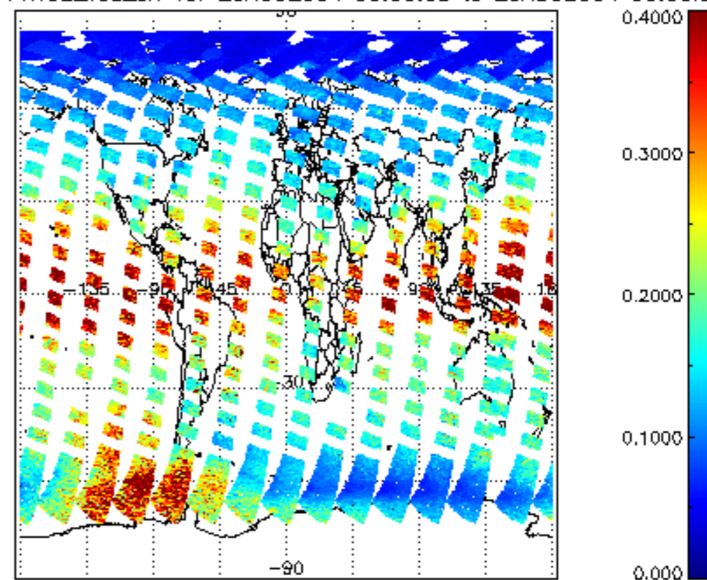
SCIOL2P_NADUV1NO2_vcd_err for 25AUG2004 00:00:00 to 26AUG2004 00:00:00
