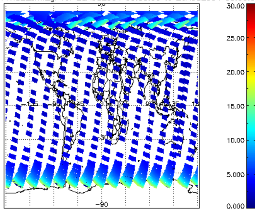
SCIOL2P_NADUV1NO2_amf_gr for 25AUG2004 00:00:00 to 26AUG2004 00:00:00
