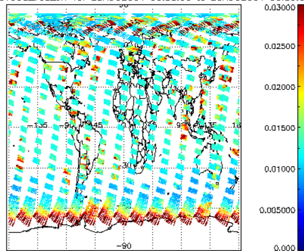
SCIOL2P_NADUV003_vcd_err for 25AUG2004 00:00:00 to 26AUG2004 00:00:00
