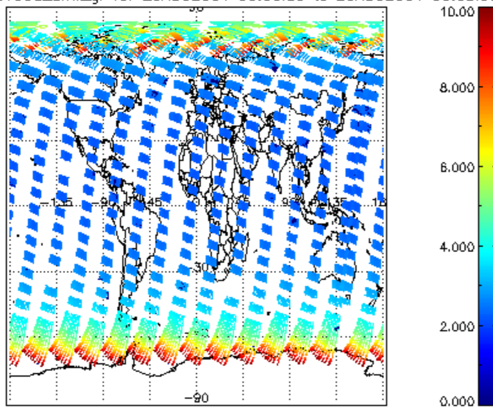
SCIOL2P_NADUV003_amf_gr for 25AUG2004 00:00:00 to 26AUG2004 00:00:00
