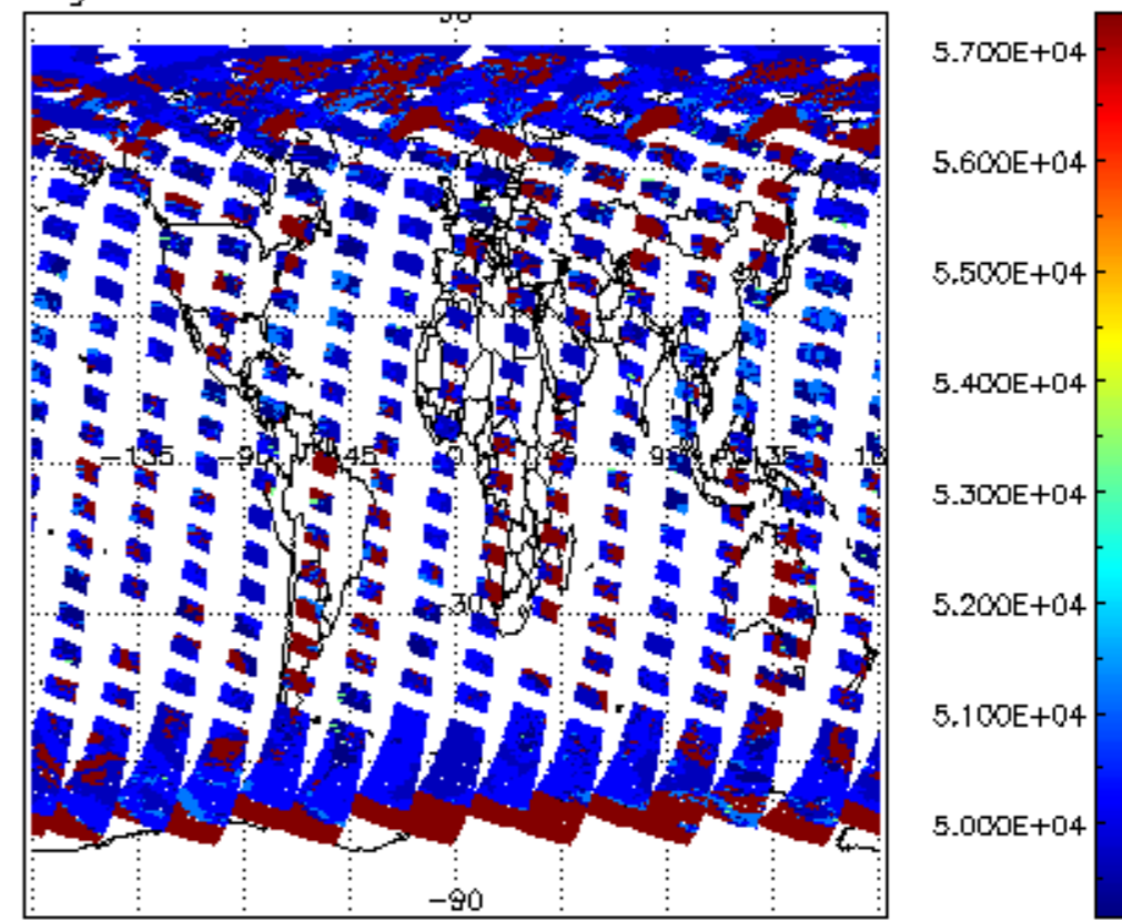
cloud_flags for 25AUG2004 00:00:00 to 26AUG2004 00:00:00
