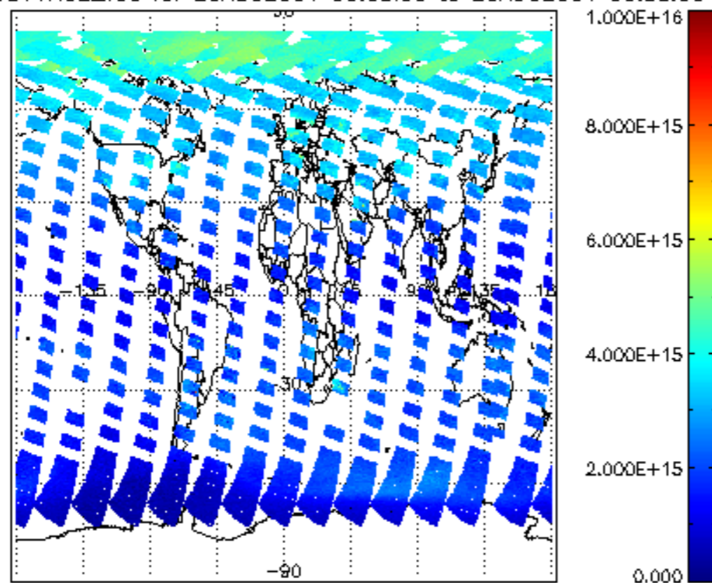
SCIOL2P_NADUV1NO2_vcd for 25AUG2004 00:00:00 to 26AUG2004 00:00:00
