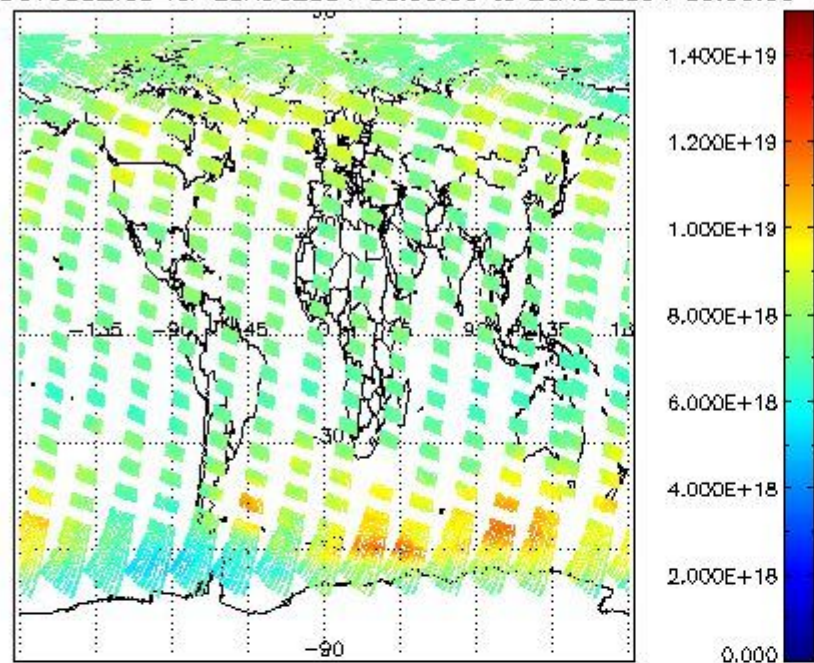
SCIOL2P_NADUV003_vcd for 25AUG2004 00:00:00 to 26AUG2004 00:00:00
