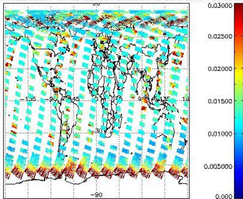
SCIOL2P_NADUV003_vcd_err for 25AUG2004 00:00:00 to 26AUG2004 00:00:00
