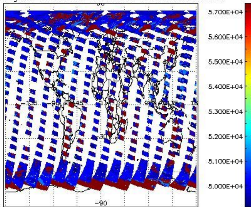
cloud_flags for 25AUG2004 00:00:00 to 26AUG2004 00:00:00
