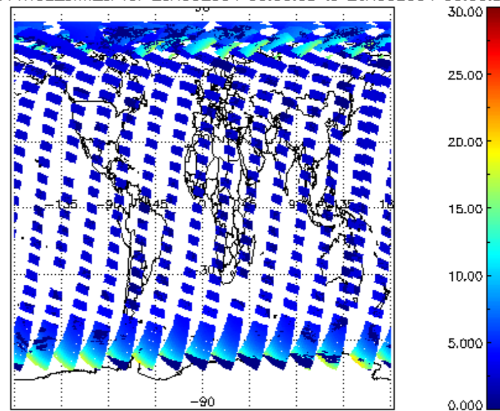
SCIOL2P_NADUV1NO2_amf_cl for 25AUG2004 00:00:00 to 26AUG2004 00:00:00
