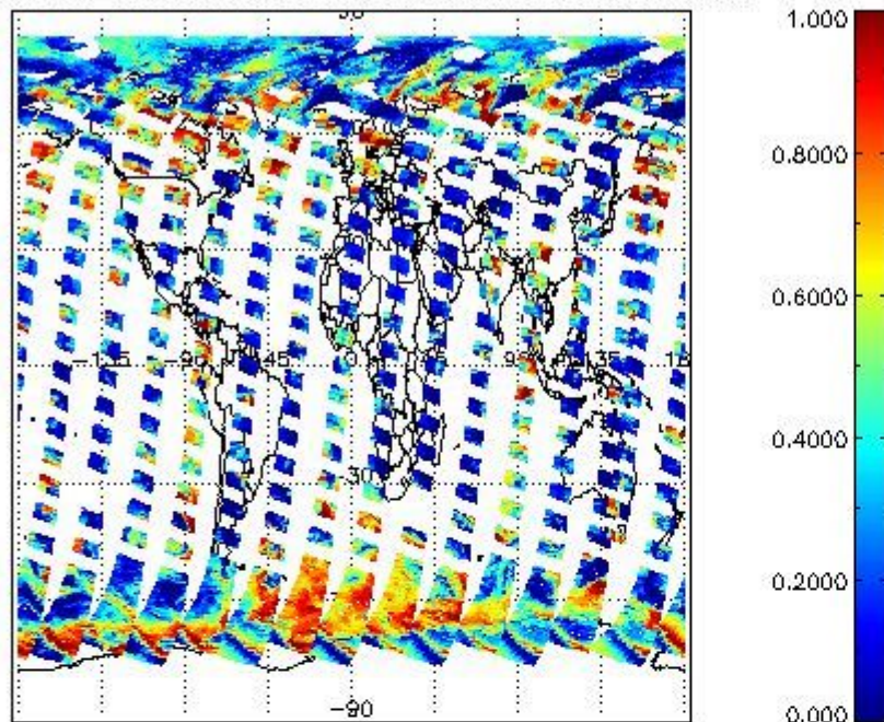
cL_frac for 25AUG2004 00:00:00 to 26AUG2004 00:00:00
