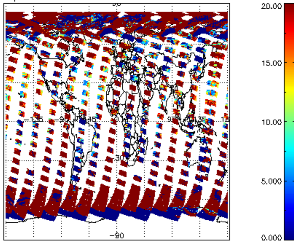
cL_opt_depth for 25AUG2004 00:00:00 to 26AUG2004 00:00:00
