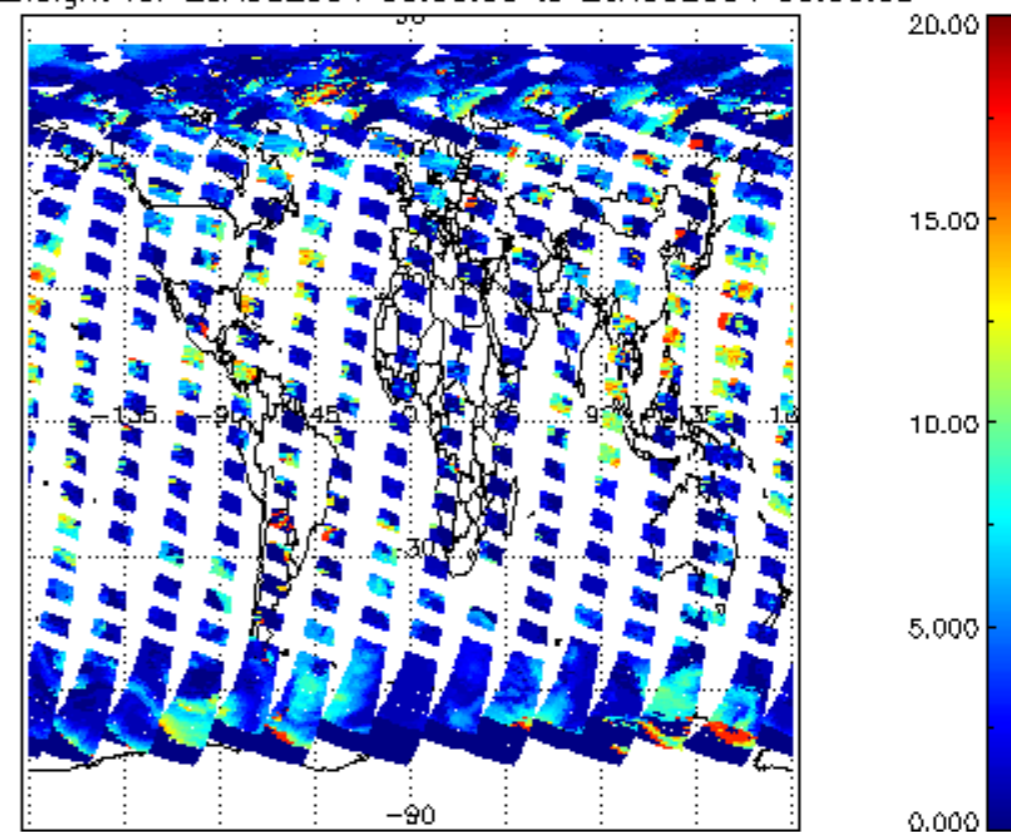
cL_top_height for 25AUG2004 00:00:00 to 26AUG2004 00:00:00
