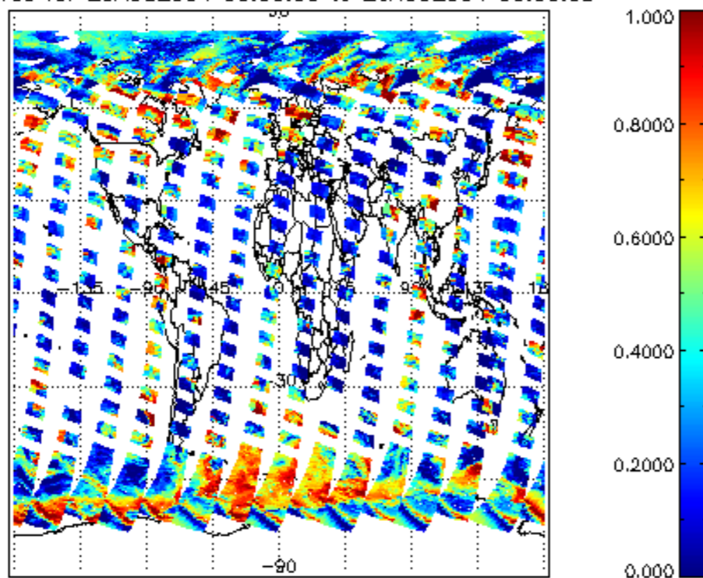
cL_frac for 25AUG2004 00:00:00 to 26AUG2004 00:00:00
