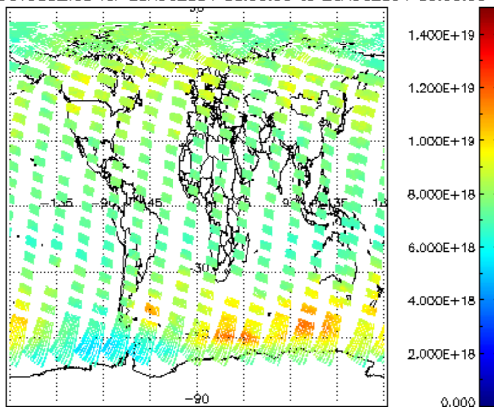
SCIOL2P_NADUV003_vcd for 25AUG2004 00:00:00 to 26AUG2004 00:00:00
