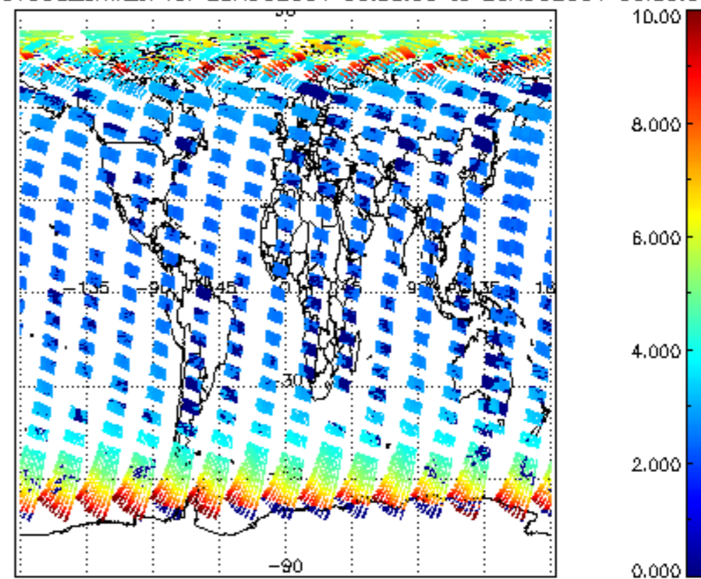
SCIOL2P_NADUV003_amf_cl for 25AUG2004 00:00:00 to 26AUG2004 00:00:00
