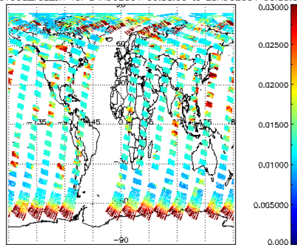
SCIOL2P_NADUV003_vcd_err for 24AUG2004 00:00:00 to 25AUG2004 00:00:00
