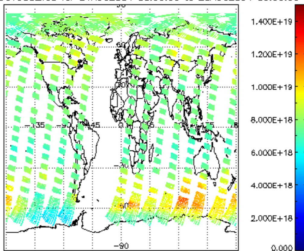
SCIOL2P_NADUV003_vcd for 24AUG2004 00:00:00 to 25AUG2004 00:00:00
