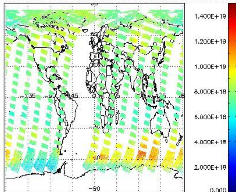
SCIOL2P_NADUV003_vcd for 24AUG2004 00:00:00 to 25AUG2004 00:00:00
