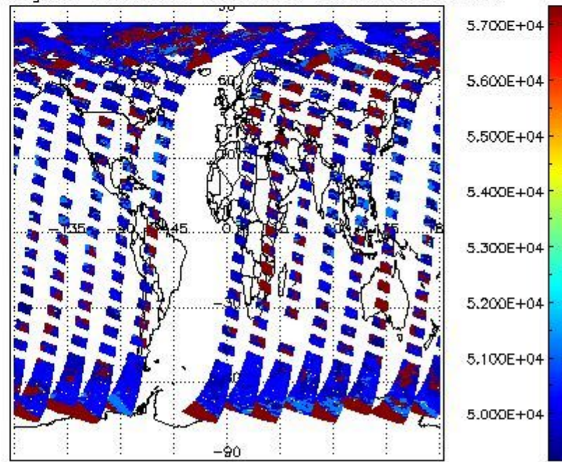
cloud_flags for 24AUG2004 00:00:00 to 25AUG2004 00:00:00
