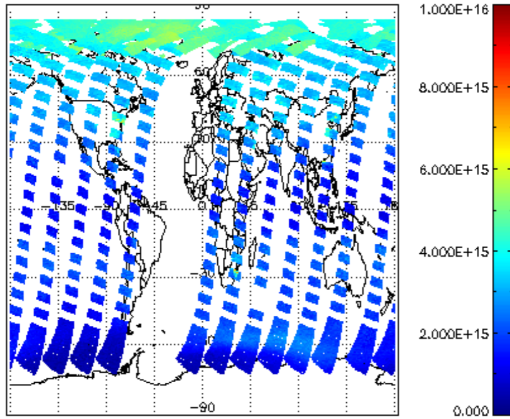
SCIOL2P_NADUV1NO2_vcd for 24AUG2004 00:00:00 to 25AUG2004 00:00:00
