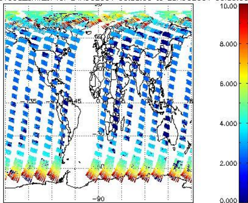
SCIOL2P_NADUV003_amf_cl for 24AUG2004 00:00:00 to 25AUG2004 00:00:00
