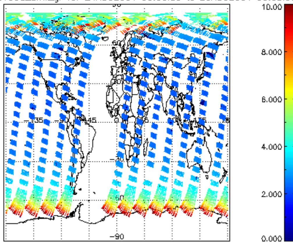
SCIOL2P_NADUV003_amf_gr for 24AUG2004 00:00:00 to 25AUG2004 00:00:00
