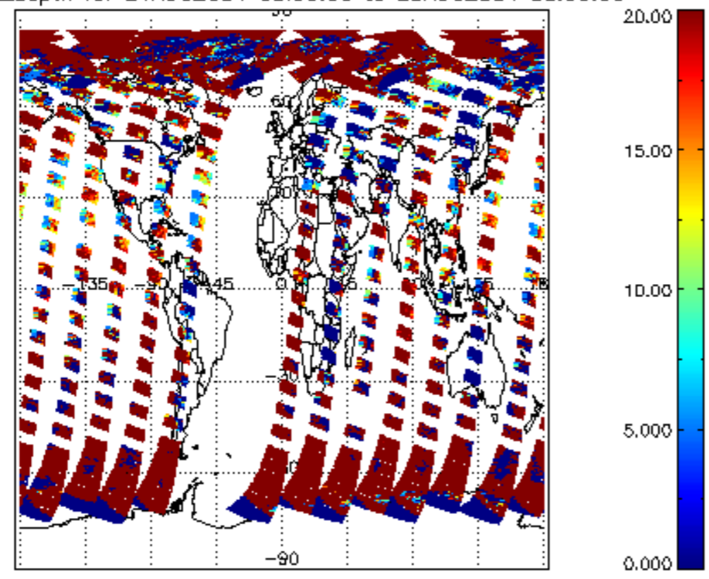
cL_opt_depth for 24AUG2004 00:00:00 to 25AUG2004 00:00:00
