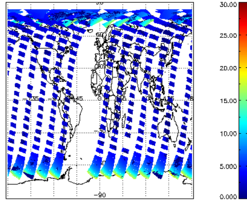
SCIOL2P_NADUV1NO2_amf_cl for 24AUG2004 00:00:00 to 25AUG2004 00:00:00
