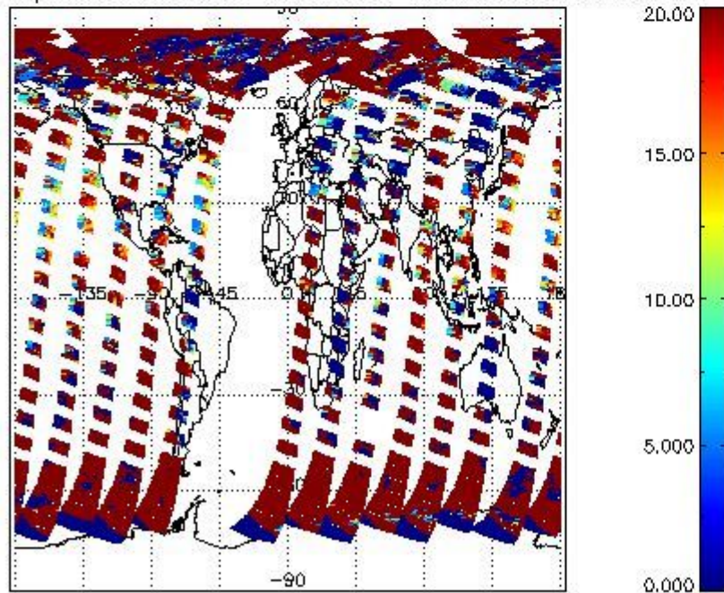
cL_opt_depth for 24AUG2004 00:00:00 to 25AUG2004 00:00:00
