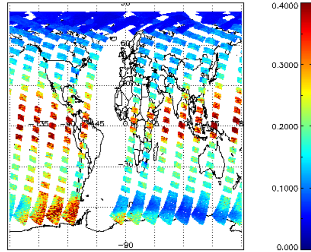
SCIOL2P_NADUV1NO2_vcd_err for 24AUG2004 00:00:00 to 25AUG2004 00:00:00
