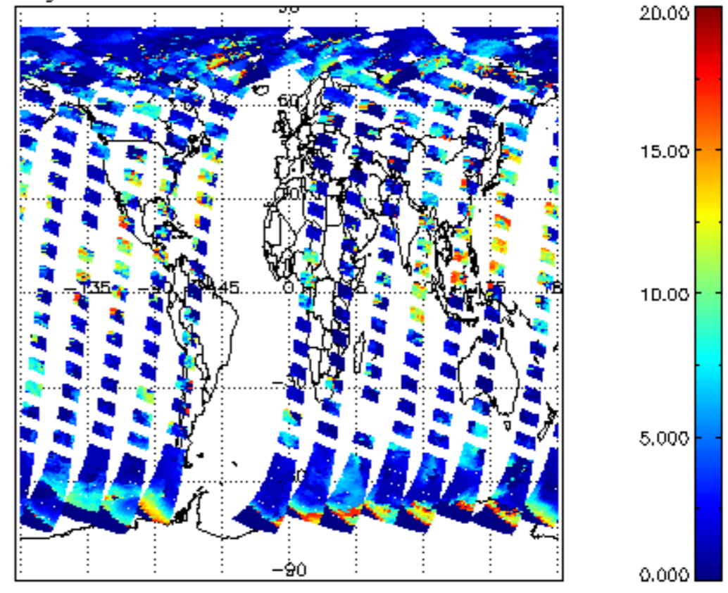
cL_top_height for 24AUG2004 00:00:00 to 25AUG2004 00:00:00
