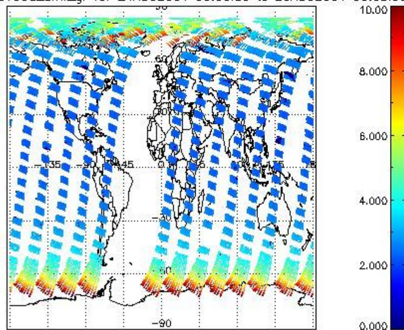
SCIOL2P_NADUV003_amf_gr for 24AUG2004 00:00:00 to 25AUG2004 00:00:00
