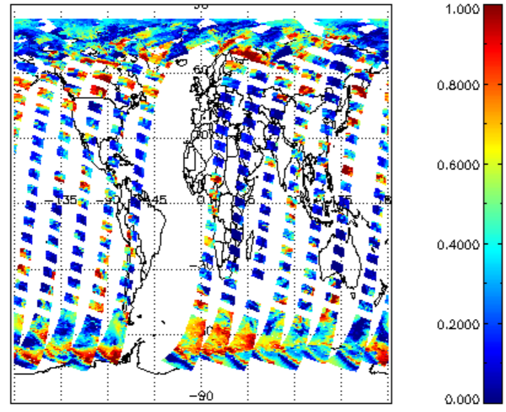
cL_frac for 24AUG2004 00:00:00 to 25AUG2004 00:00:00
