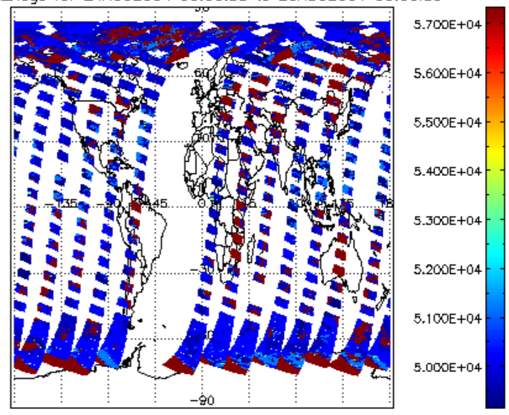
cloud_flags for 24AUG2004 00:00:00 to 25AUG2004 00:00:00
