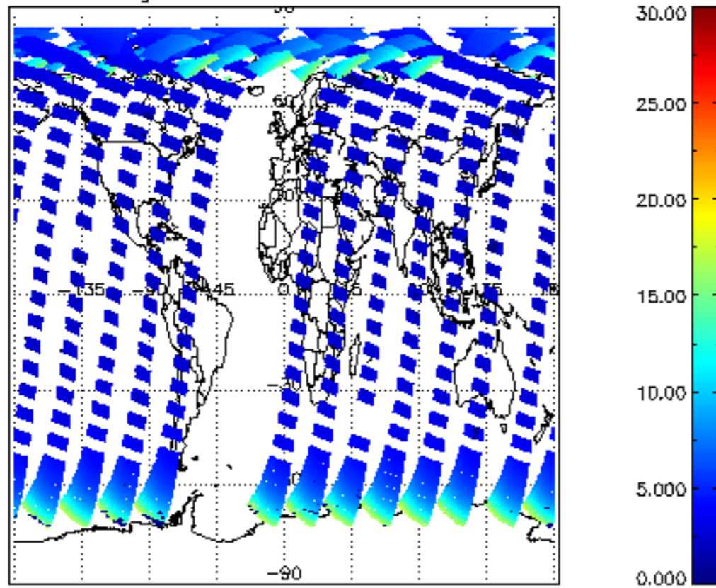
SCIOL2P_NADUV1NO2_amf_gr for 24AUG2004 00:00:00 to 25AUG2004 00:00:00
