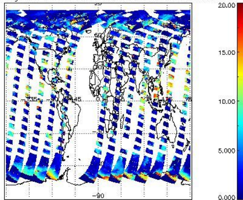
cL_top_height for 24AUG2004 00:00:00 to 25AUG2004 00:00:00
