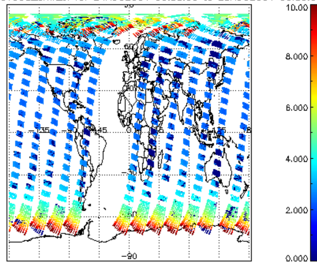
SCIOL2P_NADUV003_amf_cl for 24AUG2004 00:00:00 to 25AUG2004 00:00:00
