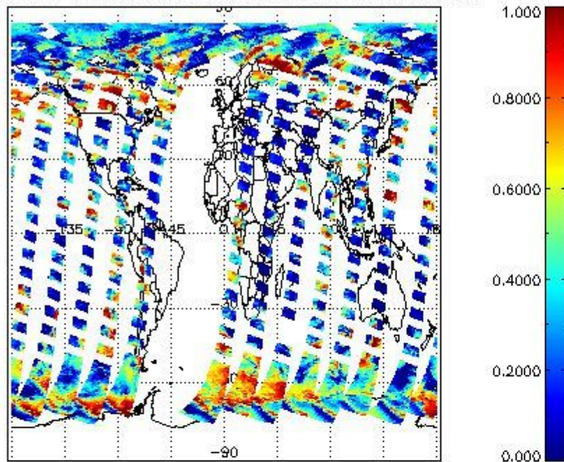
cL_frac for 24AUG2004 00:00:00 to 25AUG2004 00:00:00
