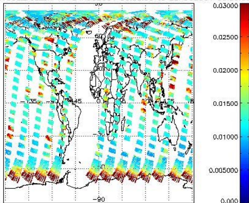
SCIOL2P_NADUV003_vcd_err for 24AUG2004 00:00:00 to 25AUG2004 00:00:00
