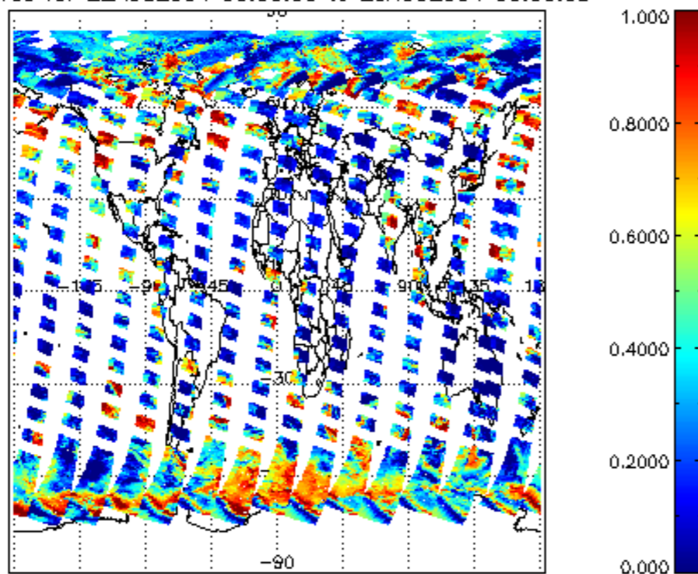
cl_frac for 22AUG2004 00:00:00 to 23AUG2004 00:00:00
