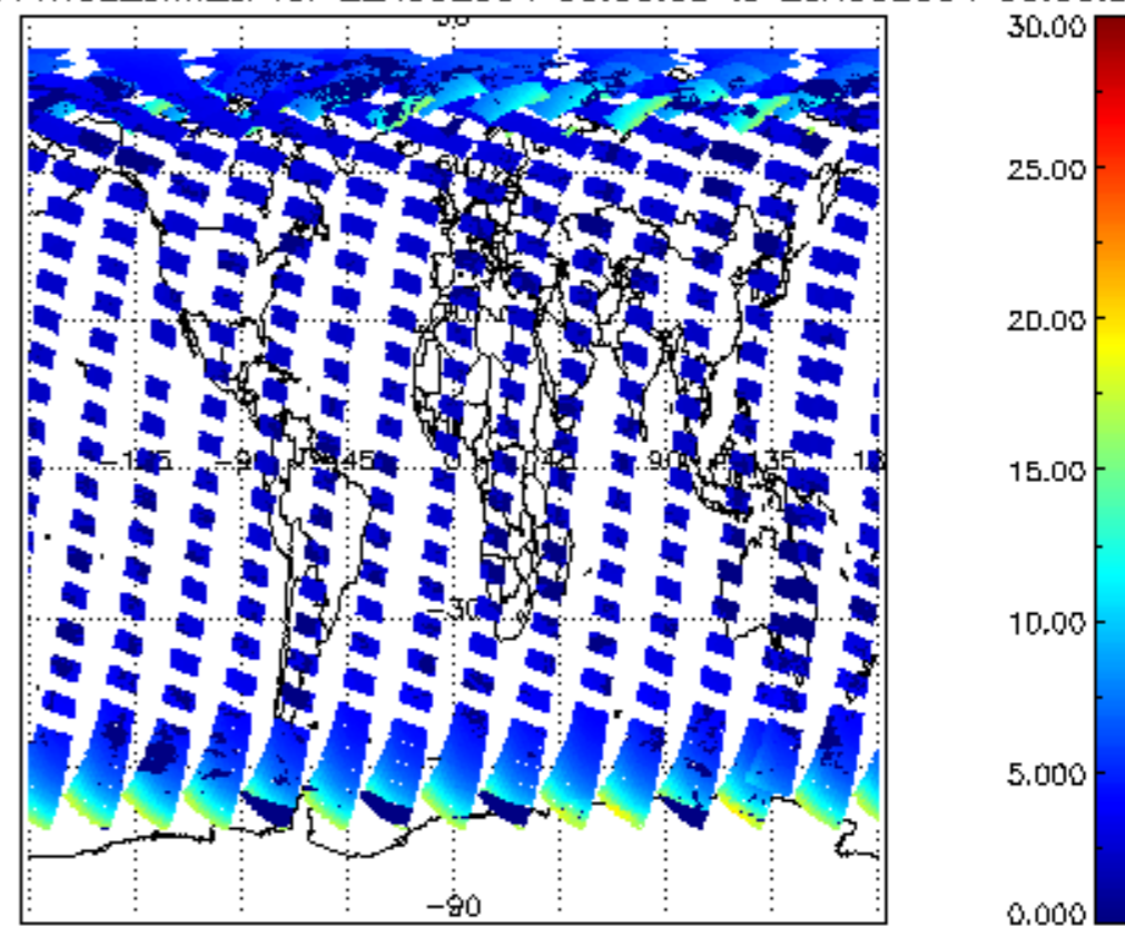
SCIOL2P_NADUV1NO2_amf_cl for 22AUG2004 00:00:00 to 23AUG2004 00:00:00
