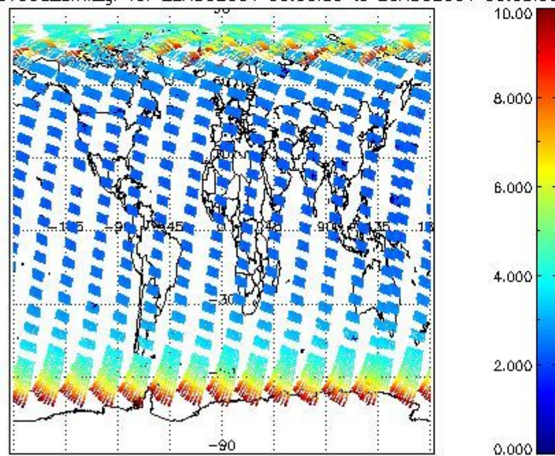
SCIOL2P_NADUV003_amf_gr for 22AUG2004 00:00:00 to 23AUG2004 00:00:00
