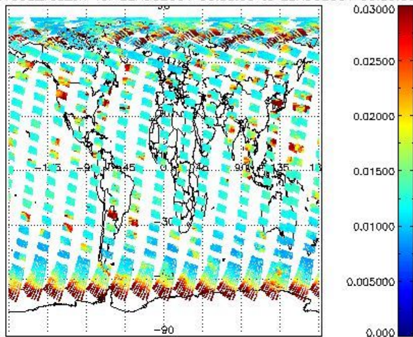
SCIOL2P_NADUV003_vcd_err for 22AUG2004 00:00:00 to 23AUG2004 00:00:00
