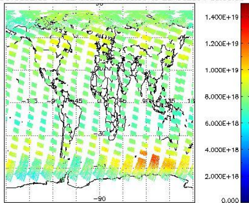
SCIOL2P_NADUV003_vcd for 22AUG2004 00:00:00 to 23AUG2004 00:00:00
