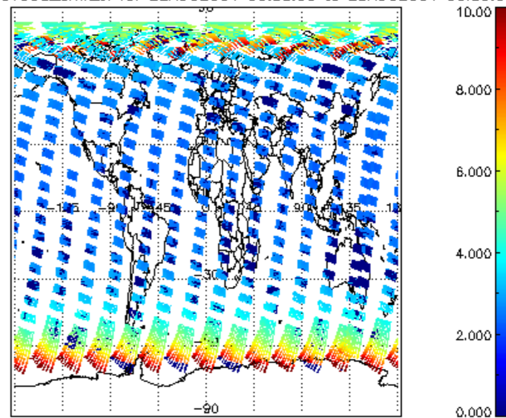
SCIOL2P_NADUV003_amf_cl for 22AUG2004 00:00:00 to 23AUG2004 00:00:00
