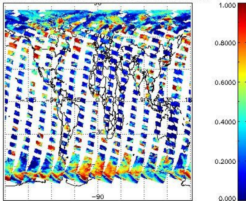
cL_frac for 22AUG2004 00:00:00 to 23AUG2004 00:00:00
