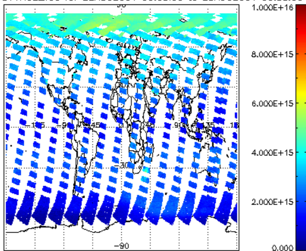
SCIOL2P_NADUV1NO2_vcd for 22AUG2004 00:00:00 to 23AUG2004 00:00:00
