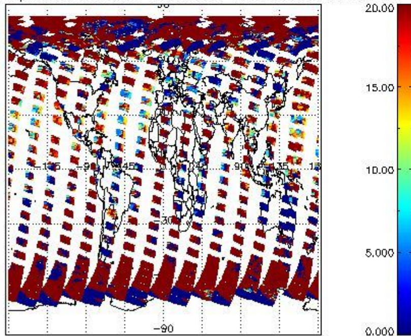
cL_opt_depth for 22AUG2004 00:00:00 to 23AUG2004 00:00:00
