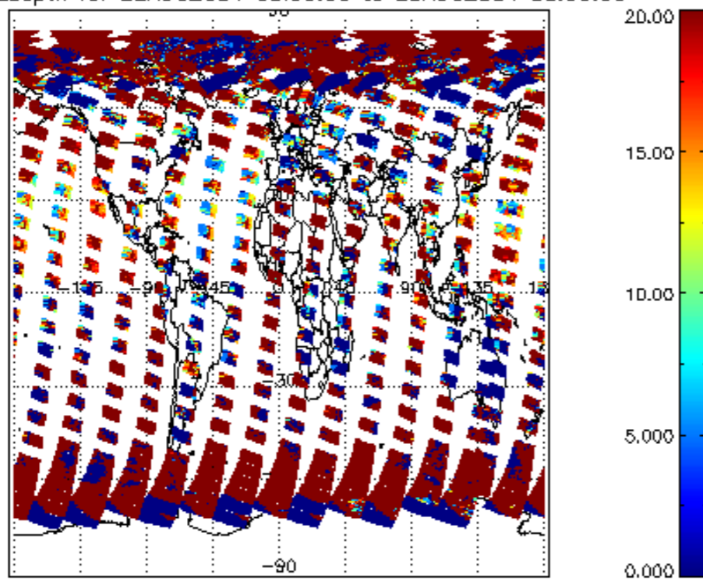
cl_opt_depth for 22AUG2004 00:00:00 to 23AUG2004 00:00:00
