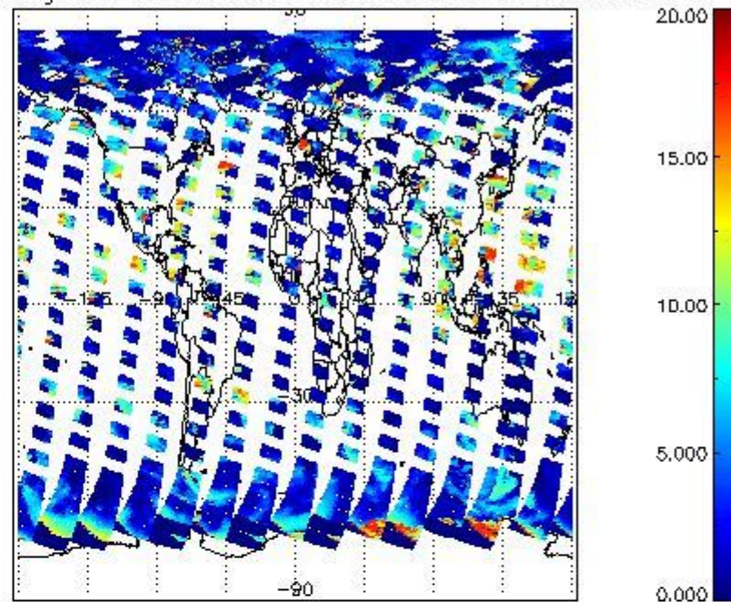
cL_top_height for 22AUG2004 00:00:00 to 23AUG2004 00:00:00
