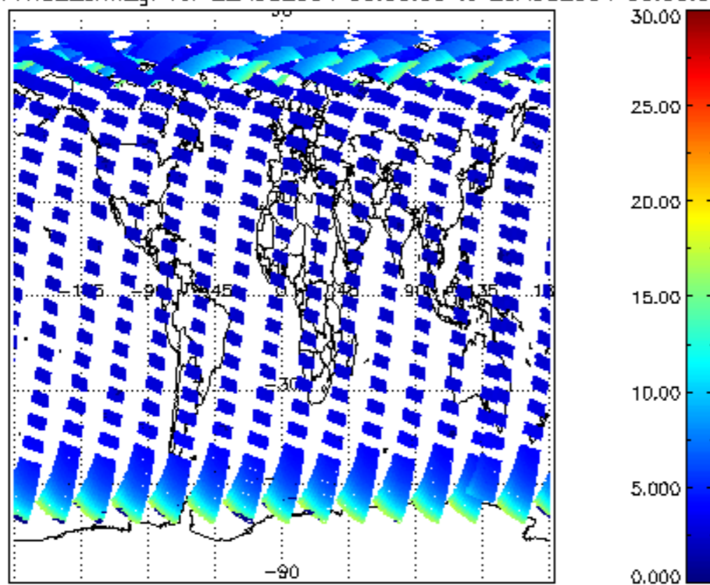
SCIOL2P_NADUV1NO2_amf_gr for 22AUG2004 00:00:00 to 23AUG2004 00:00:00
