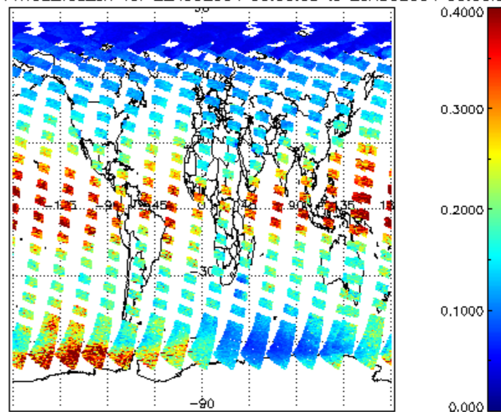
SCIOL2P_NADUV1NO2_vcd_err for 22AUG2004 00:00:00 to 23AUG2004 00:00:00
