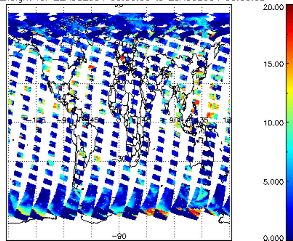
cl_top_height for 22AUG2004 00:00:00 to 23AUG2004 00:00:00
