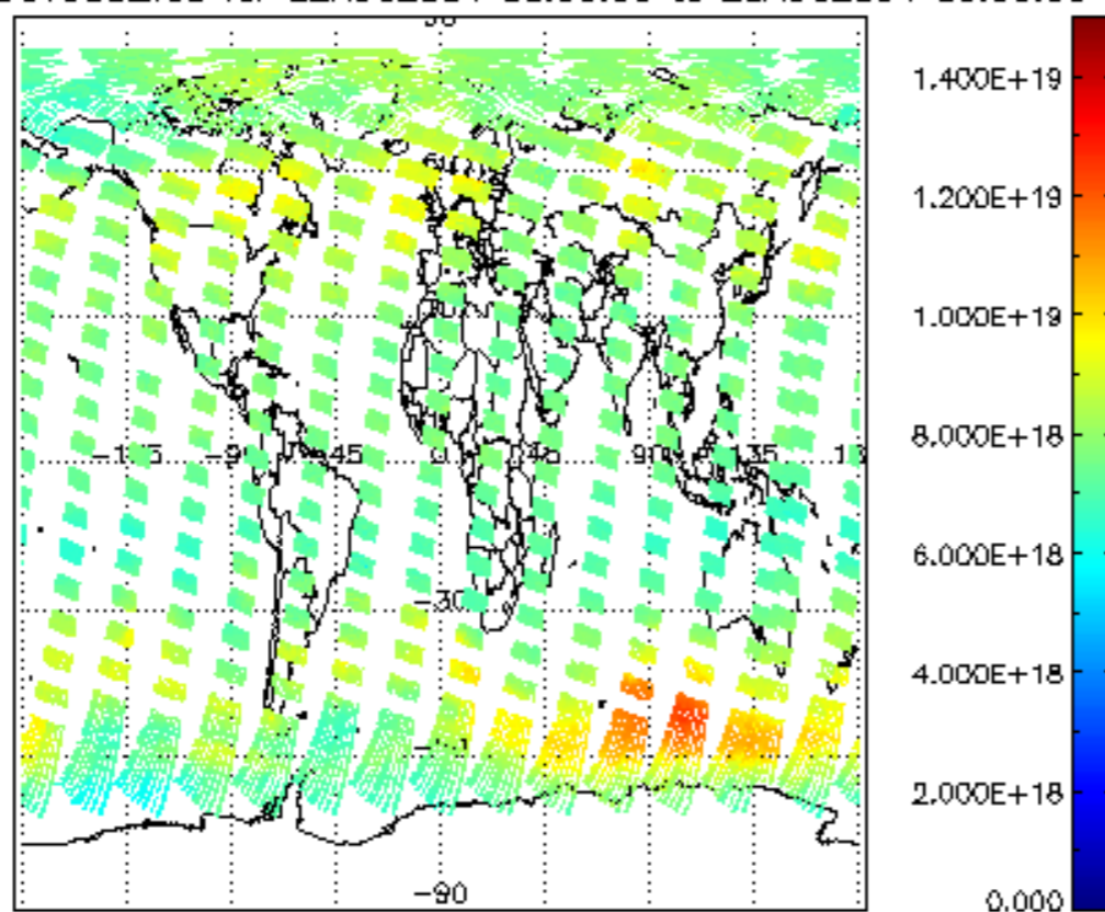
SCIOL2P_NADUV003_vcd for 22AUG2004 00:00:00 to 23AUG2004 00:00:00
