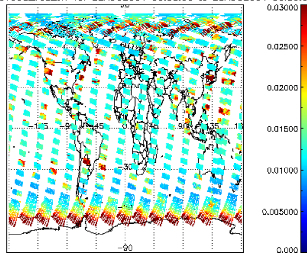
SCIOL2P_NADUV003_vcd_err for 22AUG2004 00:00:00 to 23AUG2004 00:00:00
