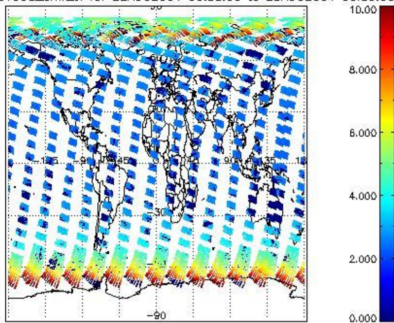
SCIOL2P_NADUV003_amf_cl for 22AUG2004 00:00:00 to 23AUG2004 00:00:00
