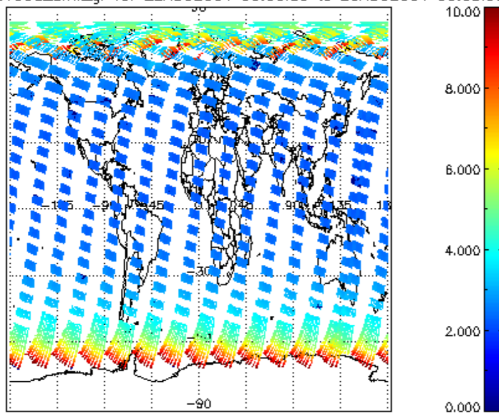
SCIOL2P_NADUV003_amf_gr for 22AUG2004 00:00:00 to 23AUG2004 00:00:00
