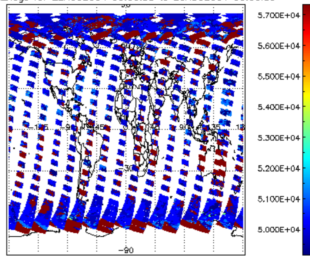
cloud_flags for 22AUG2004 00:00:00 to 23AUG2004 00:00:00
