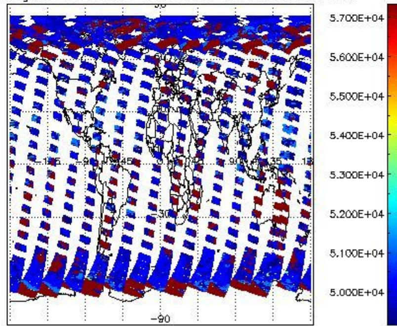
cloud_flags for 22AUG2004 00:00:00 to 23AUG2004 00:00:00
