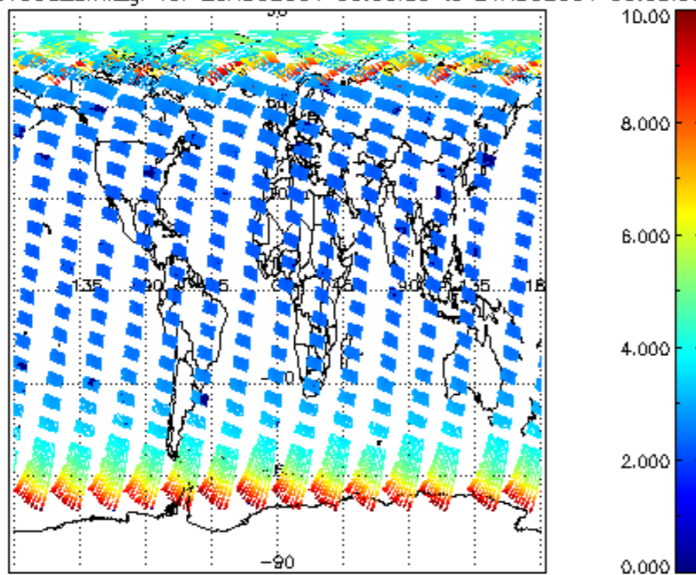
SCIOL2P_NADUV003_amf_gr for 20AUG2004 00:00:00 to 21AUG2004 00:00:00
