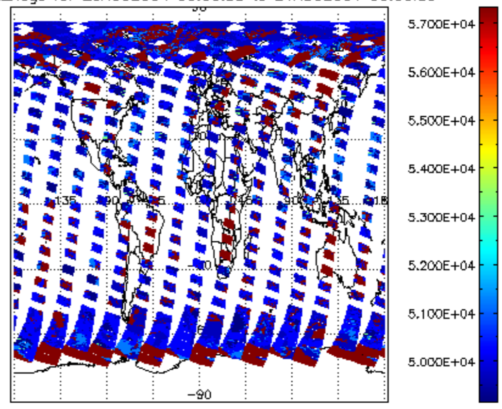
cloud_flags for 20AUG2004 00:00:00 to 21AUG2004 00:00:00
