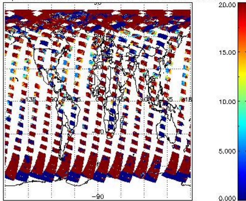
cL_opt_depth for 20AUG2004 00:00:00 to 21AUG2004 00:00:00
