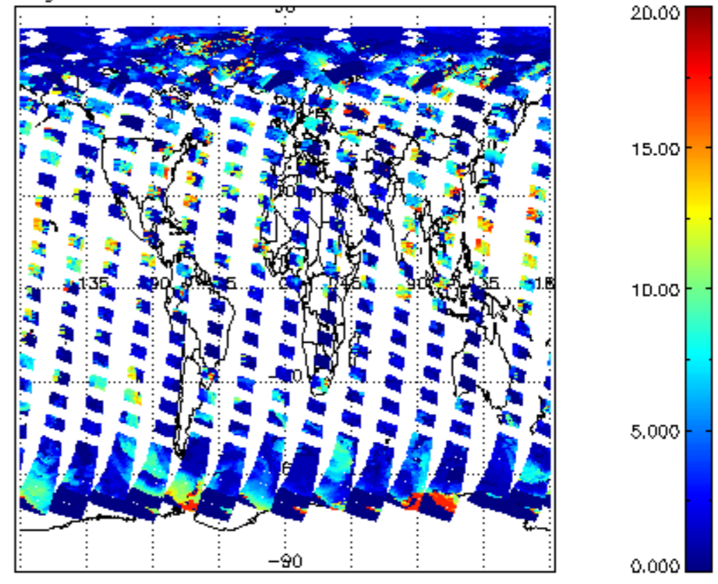
cL_top_height for 20AUG2004 00:00:00 to 21AUG2004 00:00:00
