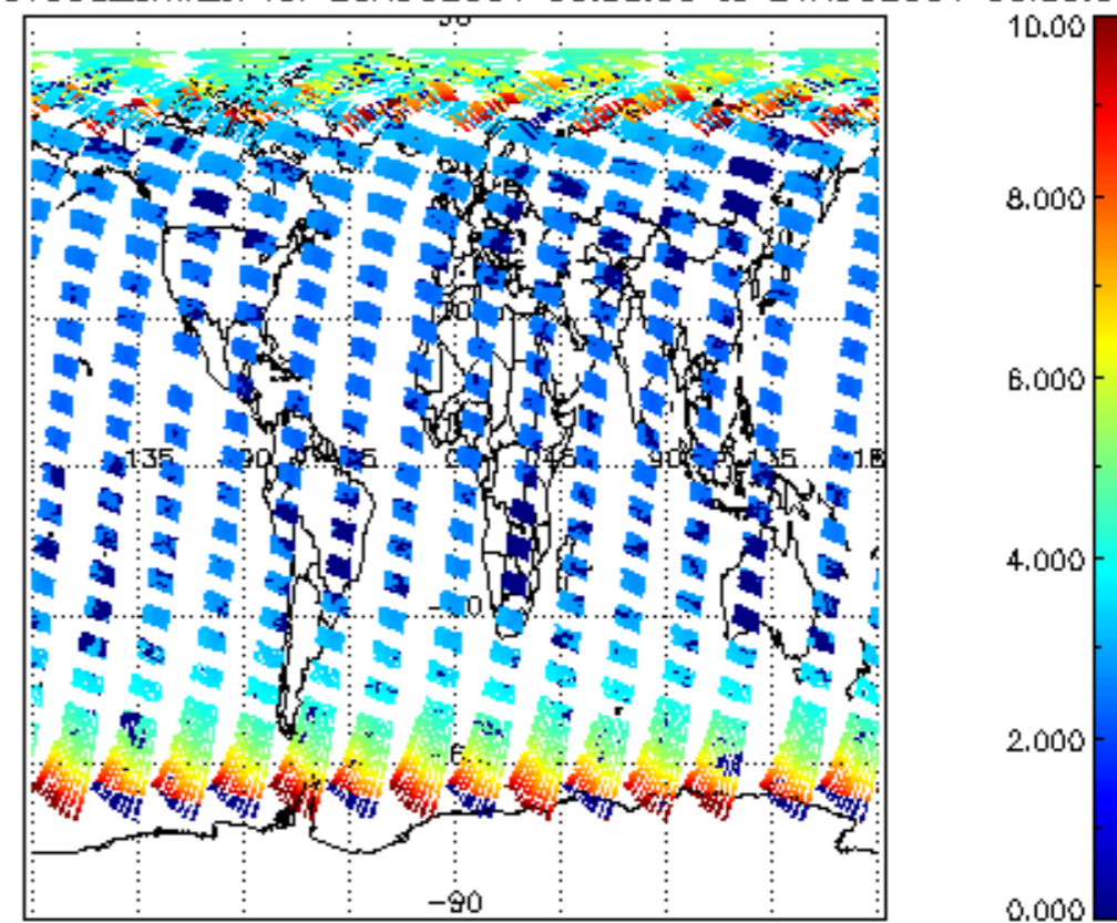
SCIOL2P_NADUV003_amf_cl for 20AUG2004 00:00:00 to 21AUG2004 00:00:00
