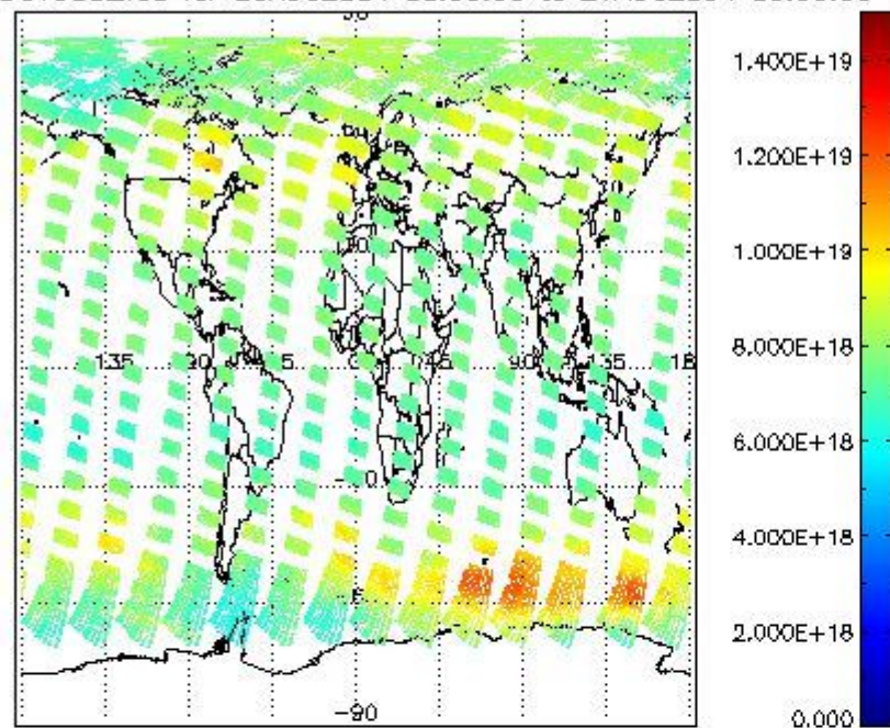
SCIOL2P_NADUV003_vcd for 20AUG2004 00:00:00 to 21AUG2004 00:00:00
