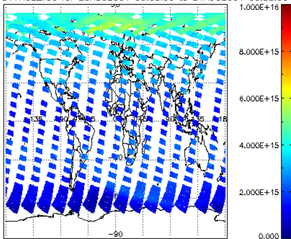
SCIOL2P_NADUV1NO2_vcd for 20AUG2004 00:00:00 to 21AUG2004 00:00:00
