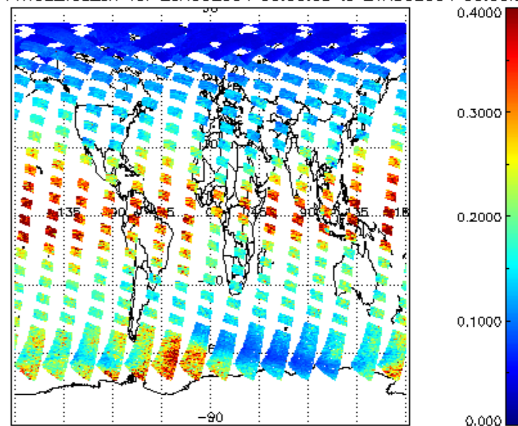
SCIOL2P_NADUV1NO2_vcd_err for 20AUG2004 00:00:00 to 21AUG2004 00:00:00
