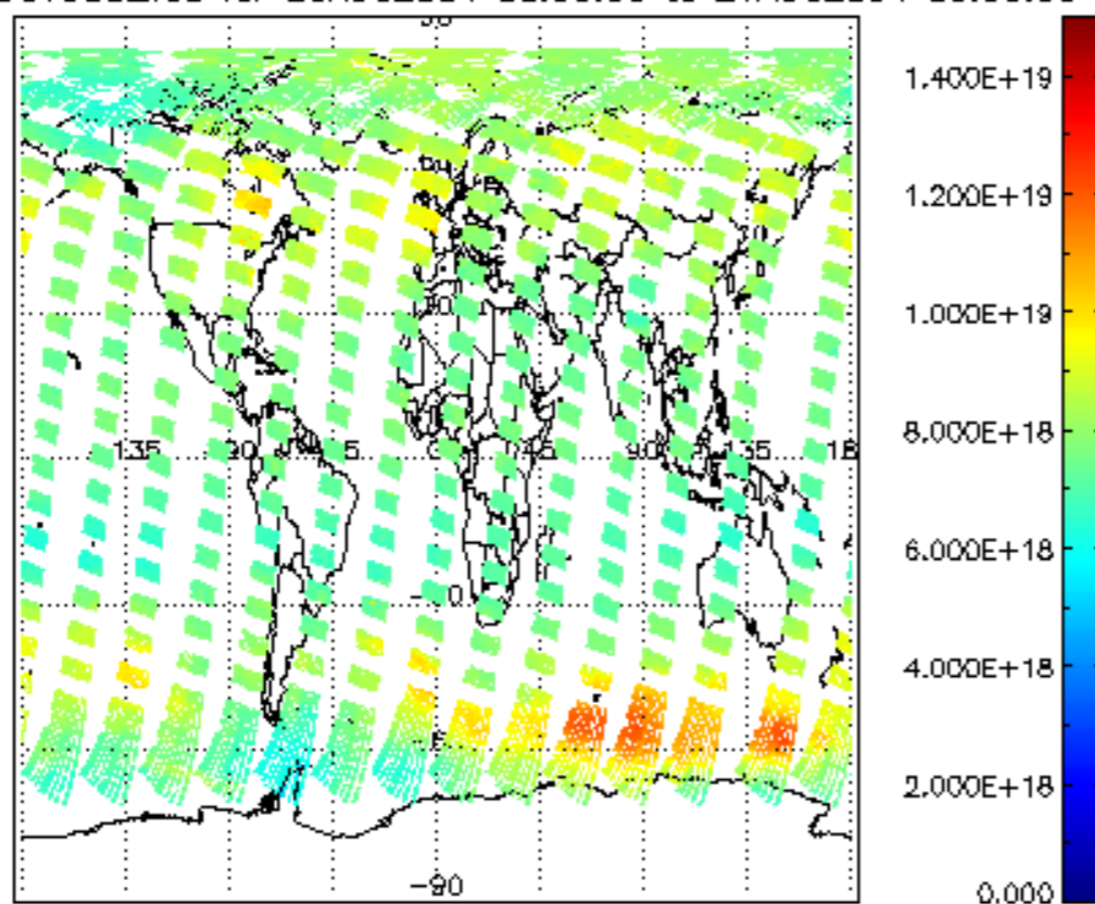
SCIOL2P_NADUV003_vcd for 20AUG2004 00:00:00 to 21AUG2004 00:00:00
