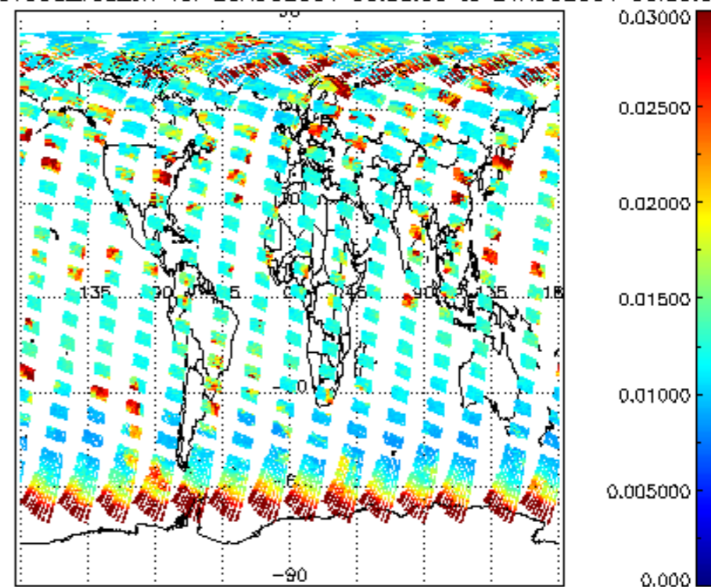
SCIOL2P_NADUV003_vcd_err for 20AUG2004 00:00:00 to 21AUG2004 00:00:00
