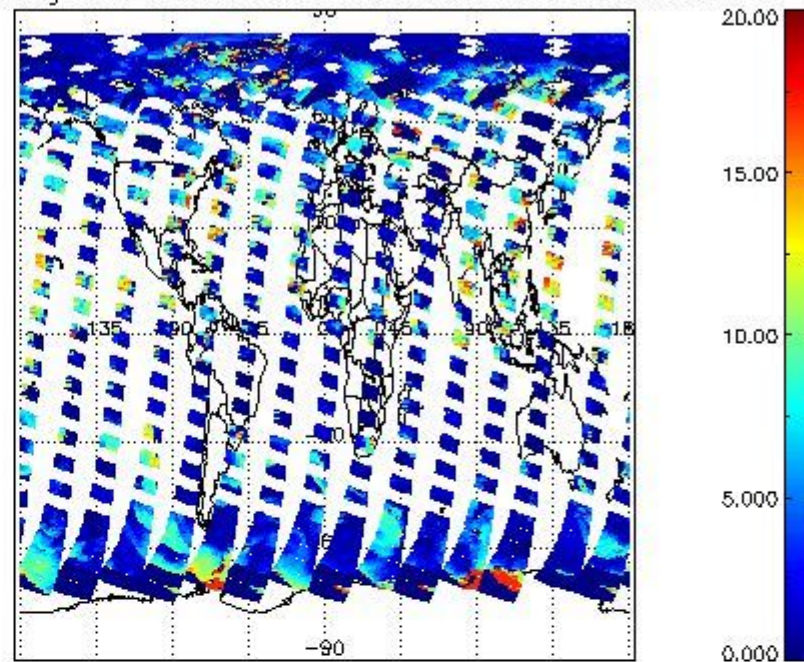
cL_top_height for 20AUG2004 00:00:00 to 21AUG2004 00:00:00
