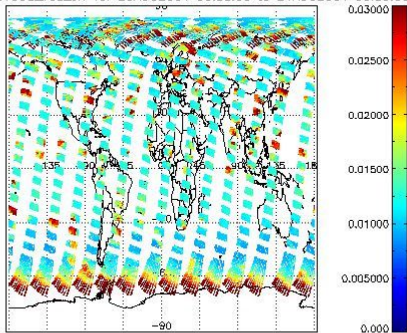
SCIOL2P_NADUV003_vcd_err for 20AUG2004 00:00:00 to 21AUG2004 00:00:00
