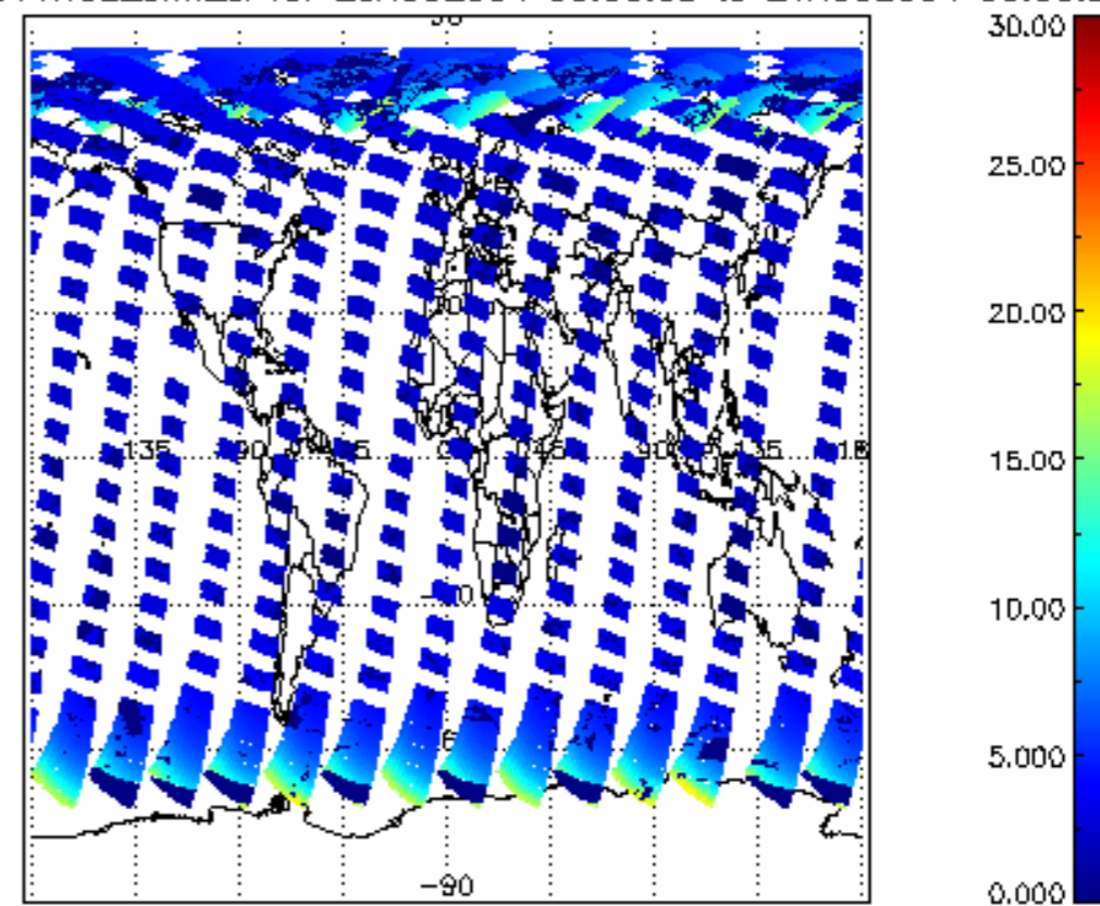
SCIOL2P_NADUV1NO2_amf_cl for 20AUG2004 00:00:00 to 21AUG2004 00:00:00
