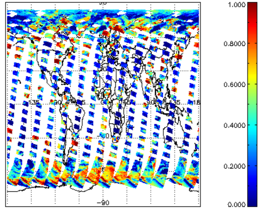
cL_frac for 20AUG2004 00:00:00 to 21AUG2004 00:00:00
