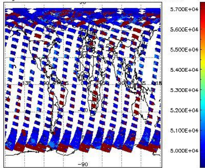
cloud_flags for 20AUG2004 00:00:00 to 21AUG2004 00:00:00
