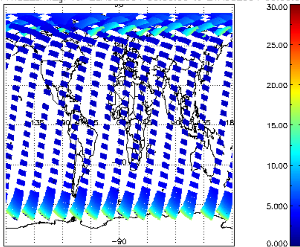
SCIOL2P_NADUV1NO2_amf_gr for 20AUG2004 00:00:00 to 21AUG2004 00:00:00
