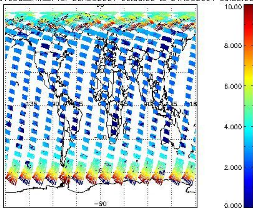
SCIOL2P_NADUV003_amf_cl for 20AUG2004 00:00:00 to 21AUG2004 00:00:00
