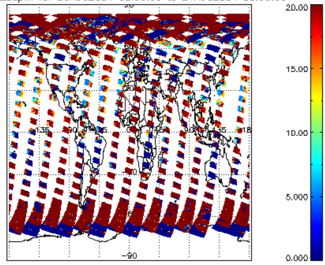
cL_opt_depth for 20AUG2004 00:00:00 to 21AUG2004 00:00:00
