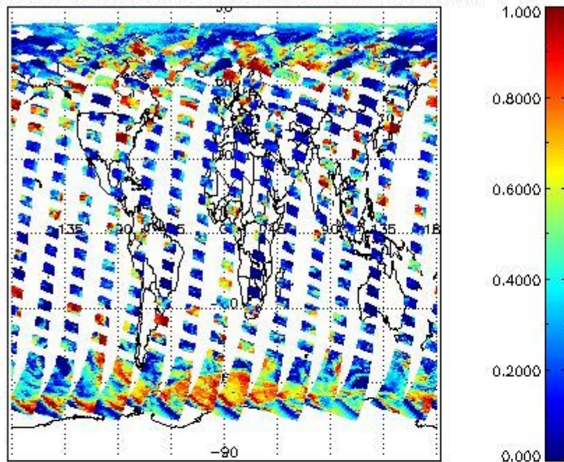
cL_frac for 20AUG2004 00:00:00 to 21AUG2004 00:00:00
