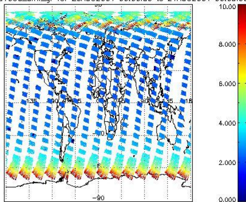
SCIOL2P_NADUV003_amf_gr for 20AUG2004 00:00:00 to 21AUG2004 00:00:00
