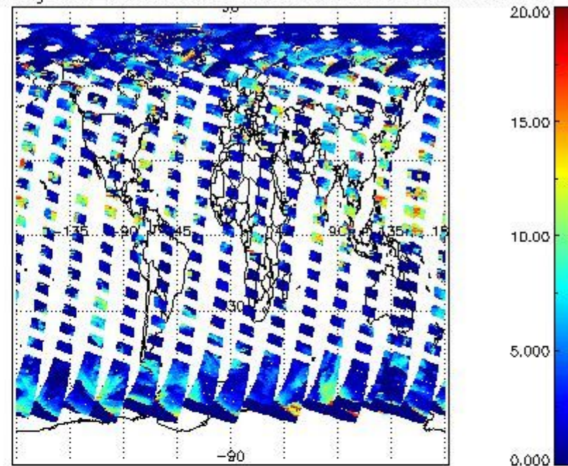
cL_top_height for 19AUG2004 00:00:00 to 20AUG2004 00:00:00
