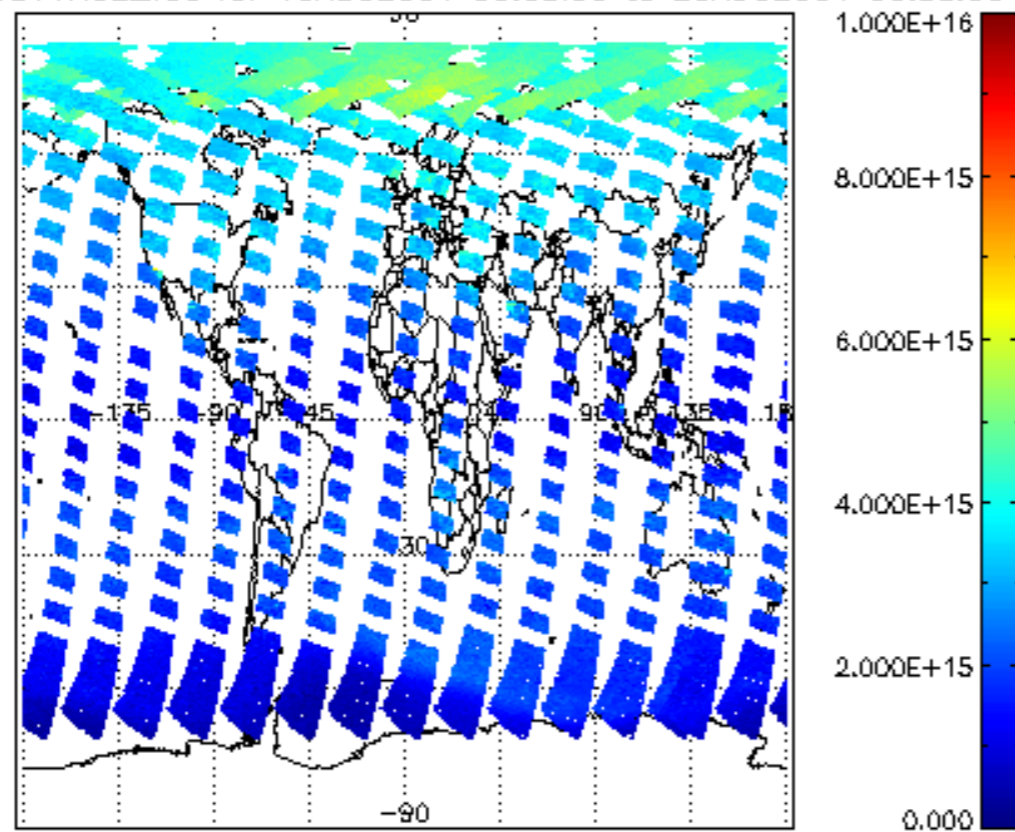
SCIOL2P_NADUV1NO2_vcd for 19AUG2004 00:00:00 to 20AUG2004 00:00:00
