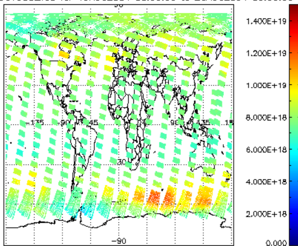
SCIOL2P_NADUV003_vcd for 19AUG2004 00:00:00 to 20AUG2004 00:00:00
