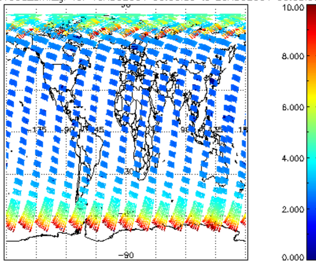
SCIOL2P_NADUV003_amf_gr for 19AUG2004 00:00:00 to 20AUG2004 00:00:00
