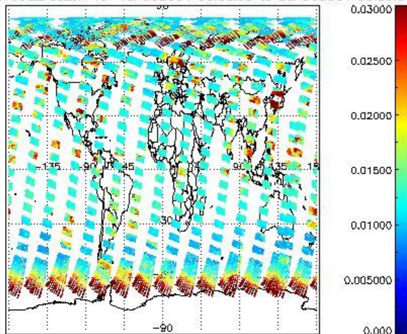
SCIOL2P_NADUV003_vcd_err for 19AUG2004 00:00:00 to 20AUG2004 00:00:00
