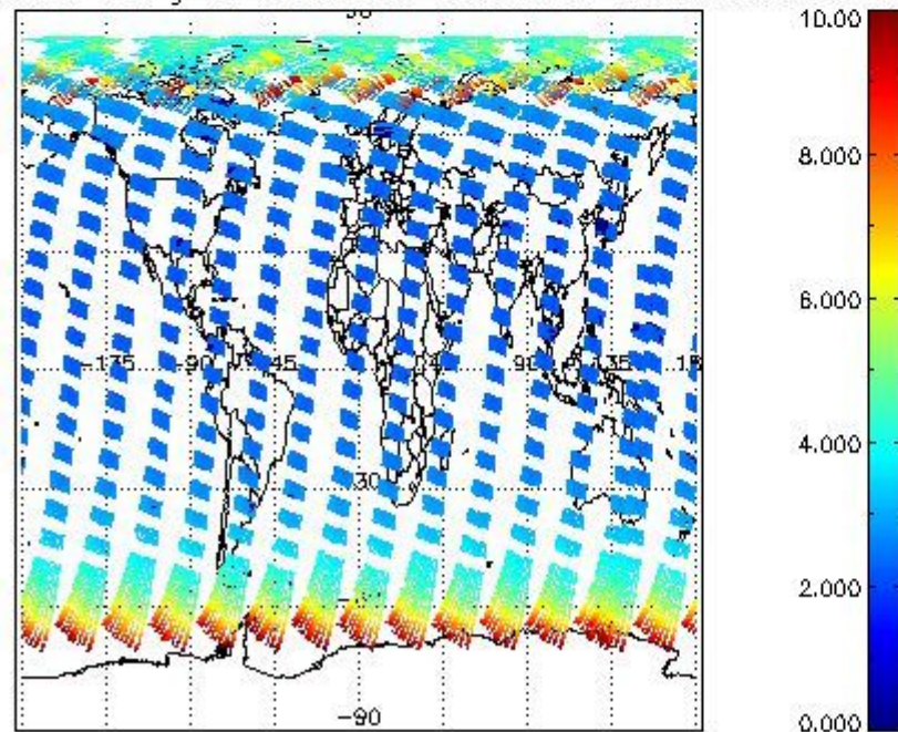
SCIOL2P_NADUV003_amf_gr for 19AUG2004 00:00:00 to 20AUG2004 00:00:00
