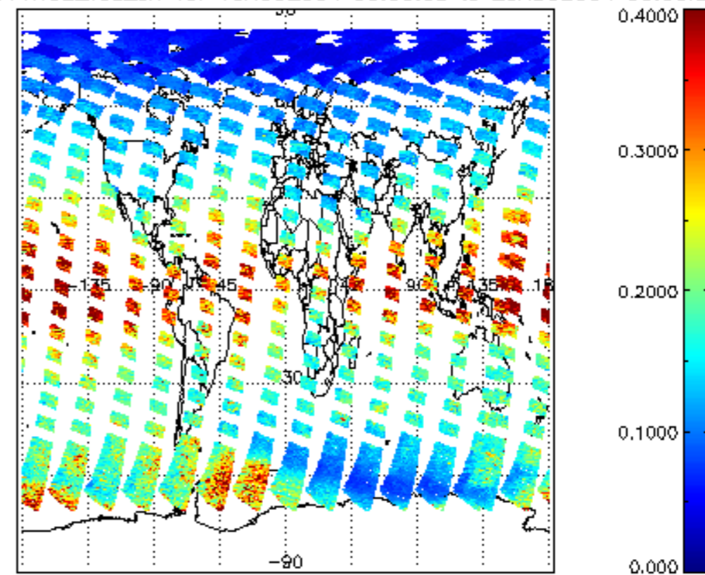
SCIOL2P_NADUV1NO2_vcd_err for 19AUG2004 00:00:00 to 20AUG2004 00:00:00
