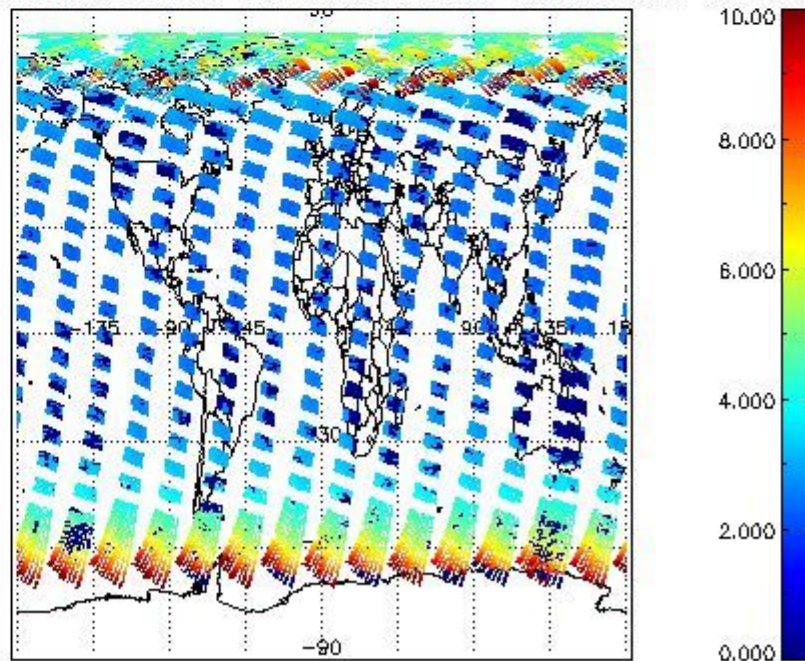
SCIOL2P_NADUV003_amf_cl for 19AUG2004 00:00:00 to 20AUG2004 00:00:00
