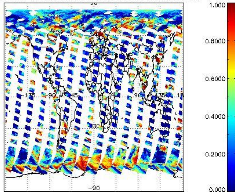
cL_frac for 19AUG2004 00:00:00 to 20AUG2004 00:00:00
