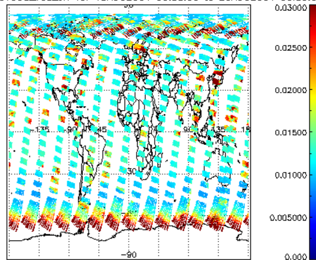
SCIOL2P_NADUV003_vcd_err for 19AUG2004 00:00:00 to 20AUG2004 00:00:00
