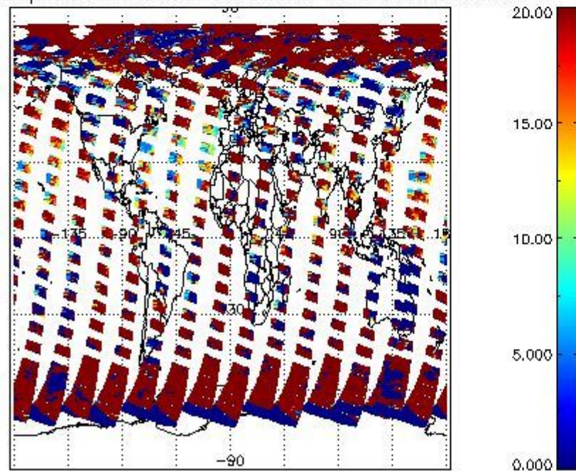
cL_opt_depth for 19AUG2004 00:00:00 to 20AUG2004 00:00:00
