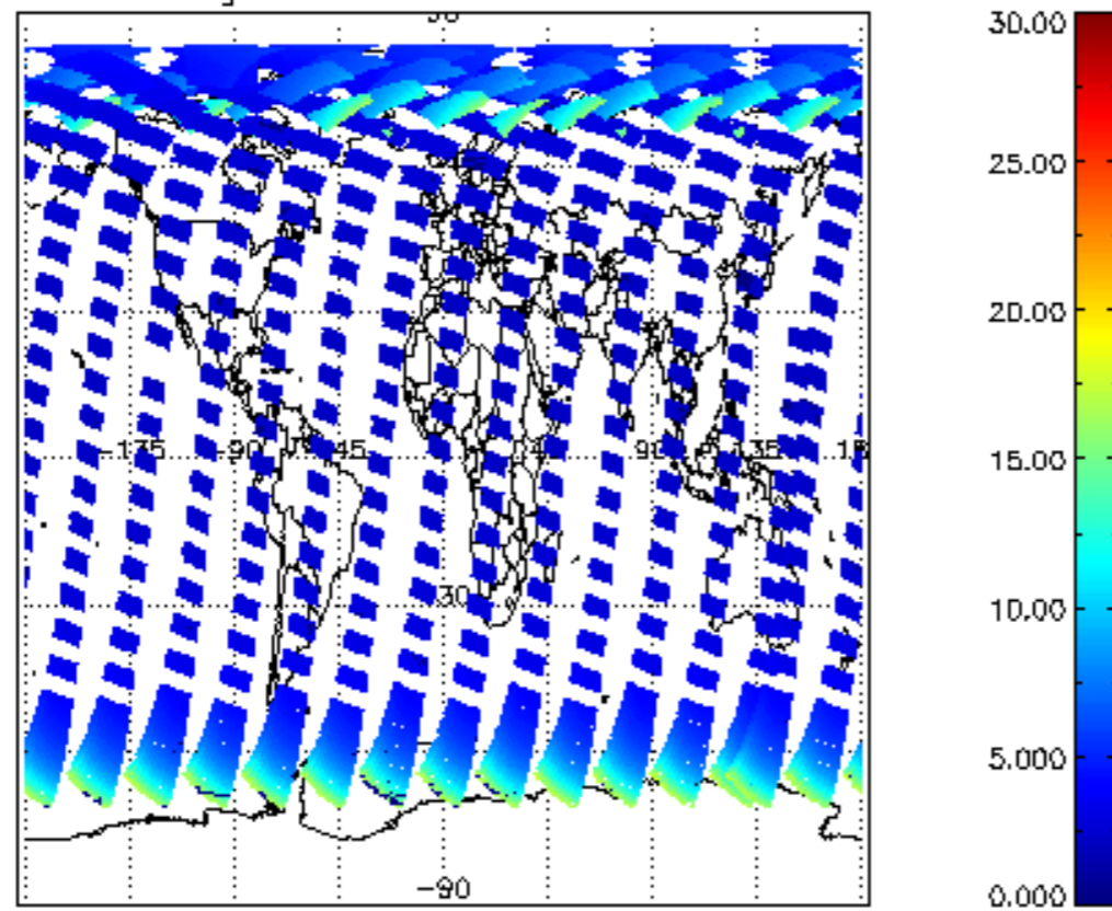
SCIOL2P_NADUV1NO2_amf_gr for 19AUG2004 00:00:00 to 20AUG2004 00:00:00
