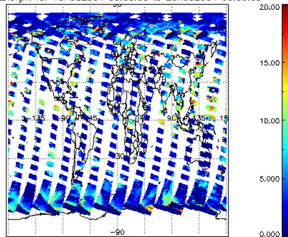
cL_top_height for 19AUG2004 00:00:00 to 20AUG2004 00:00:00
