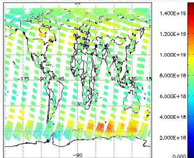
SCIOL2P_NADUV003_vcd for 19AUG2004 00:00:00 to 20AUG2004 00:00:00
