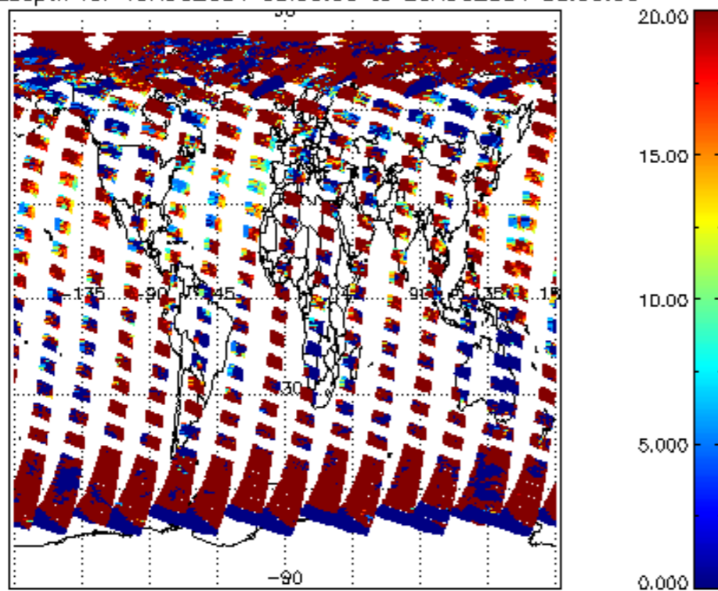
cL_opt_depth for 19AUG2004 00:00:00 to 20AUG2004 00:00:00
