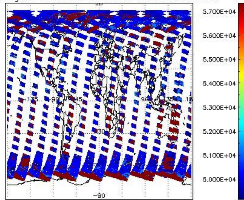
cloud_flags for 19AUG2004 00:00:00 to 20AUG2004 00:00:00
