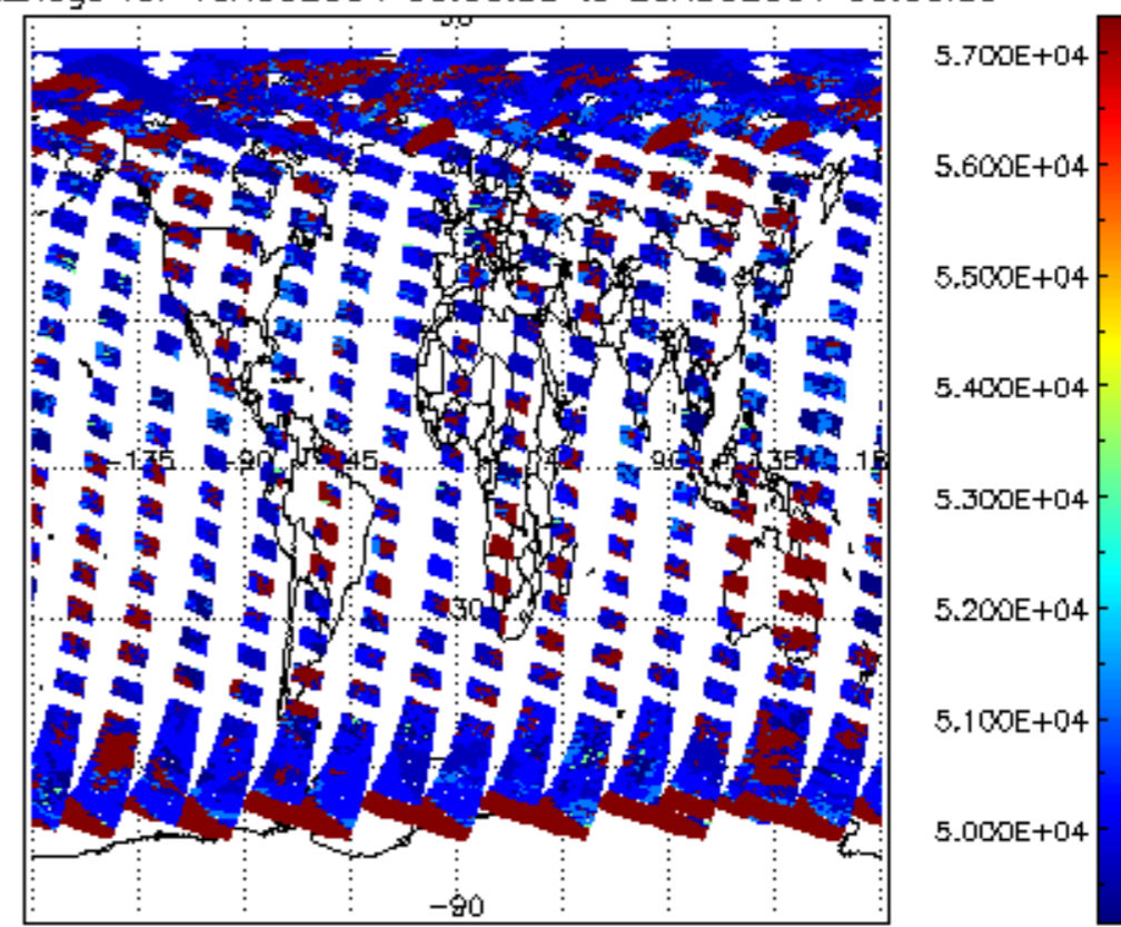
cloud_flags for 19AUG2004 00:00:00 to 20AUG2004 00:00:00
