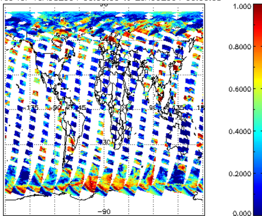
cL_frac for 19AUG2004 00:00:00 to 20AUG2004 00:00:00
