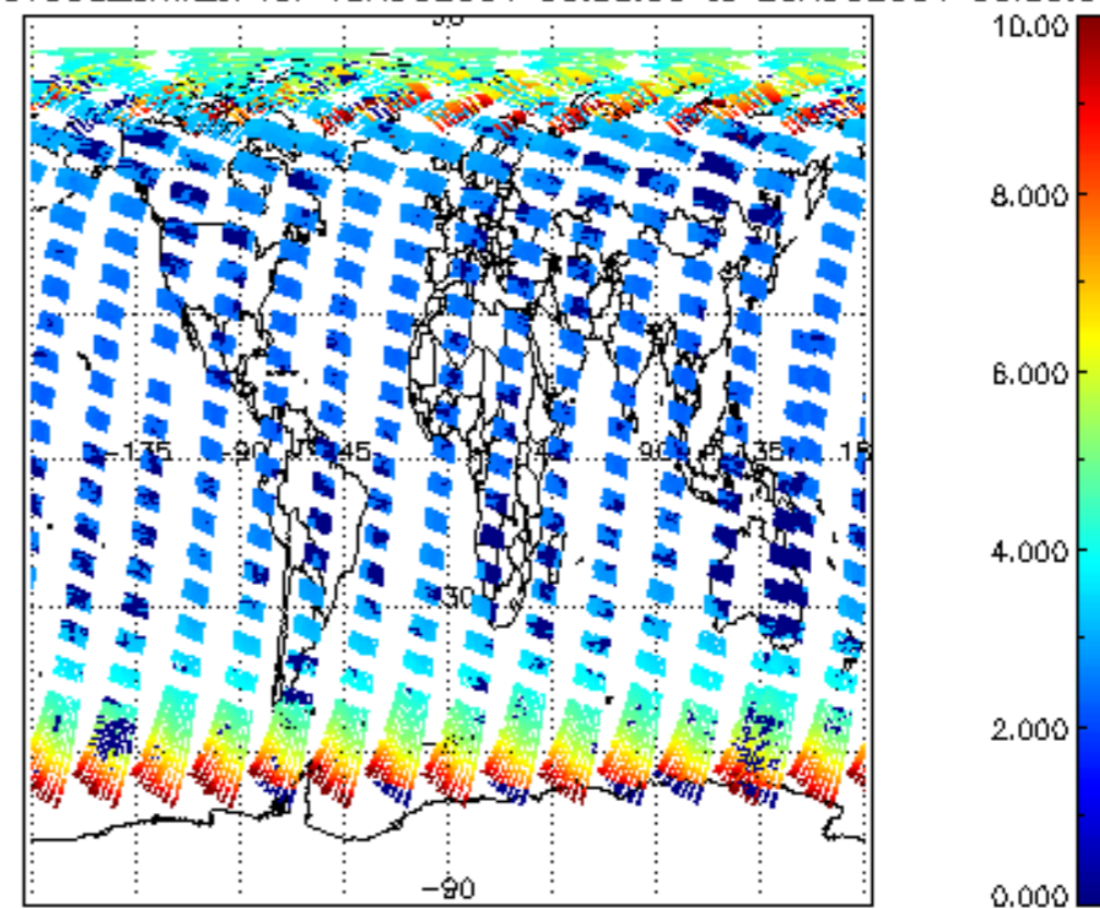
SCIOL2P_NADUV003_amf_cl for 19AUG2004 00:00:00 to 20AUG2004 00:00:00
