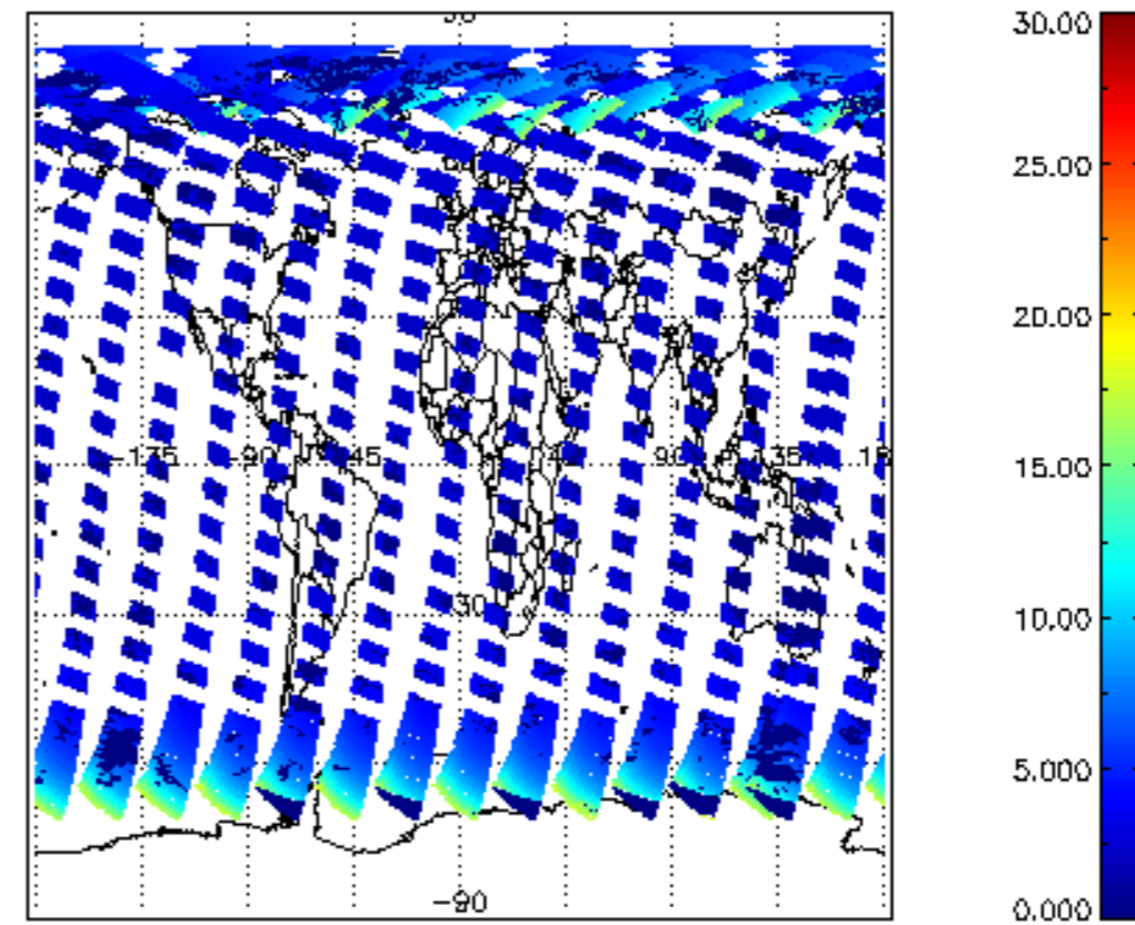
SCIOL2P_NADUV1NO2_amf_cl for 19AUG2004 00:00:00 to 20AUG2004 00:00:00
