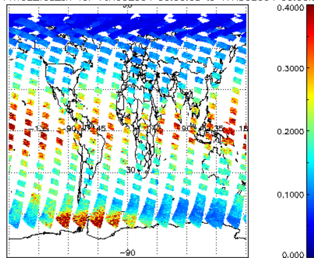
SCIOL2P_NADUV1NO2_vcd_err for 16AUG2004 00:00:00 to 17AUG2004 00:00:00
