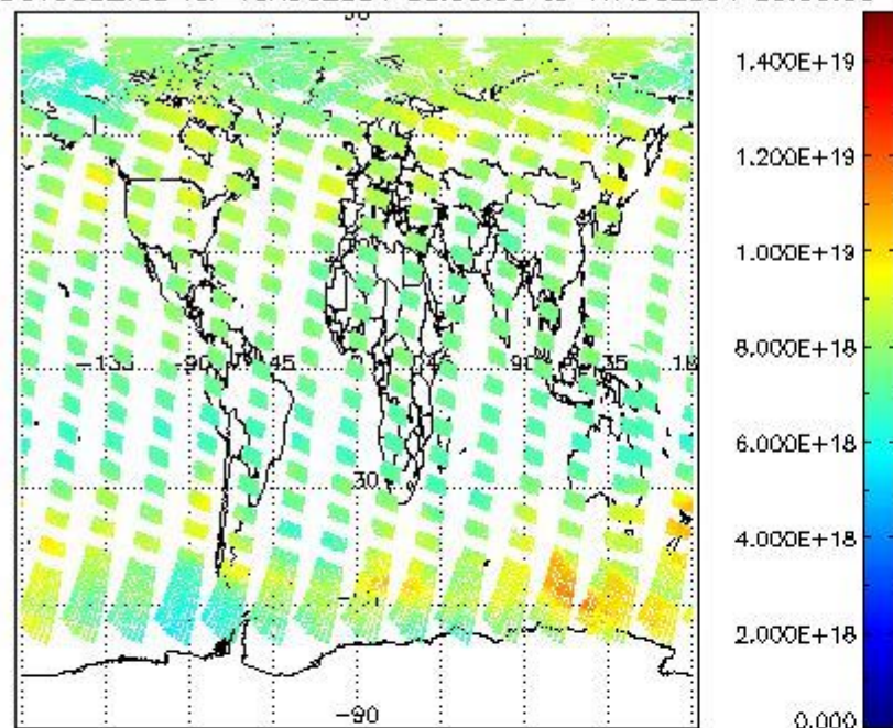
SCIOL2P_NADUV003_vcd for 16AUG2004 00:00:00 to 17AUG2004 00:00:00
