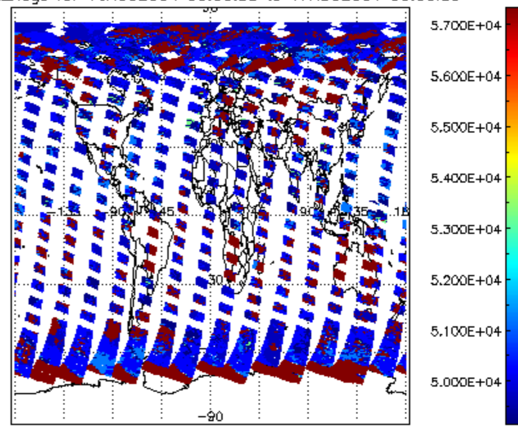
cloud_flags for 16AUG2004 00:00:00 to 17AUG2004 00:00:00
