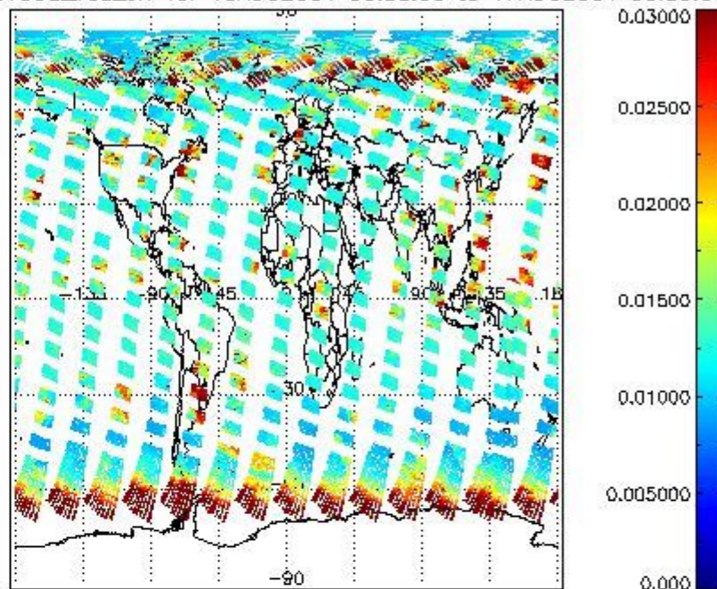
SCIOL2P_NADUV003_vcd_err for 16AUG2004 00:00:00 to 17AUG2004 00:00:00
