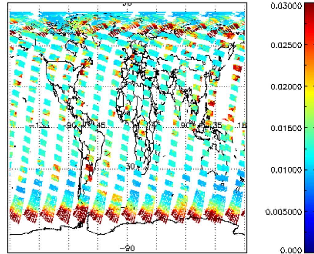
SCIOL2P_NADUV003_vcd_err for 16AUG2004 00:00:00 to 17AUG2004 00:00:00
