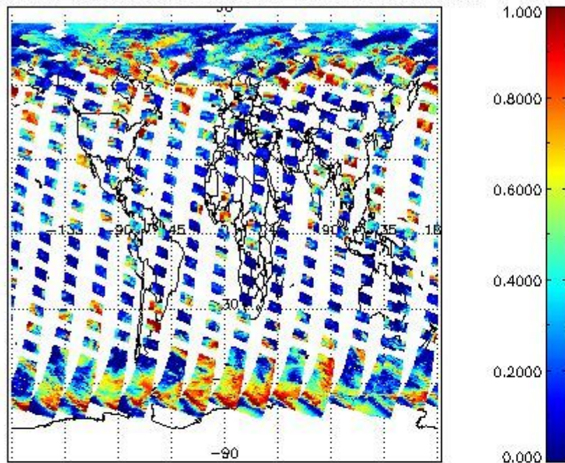
cL_frac for 16AUG2004 00:00:00 to 17AUG2004 00:00:00
