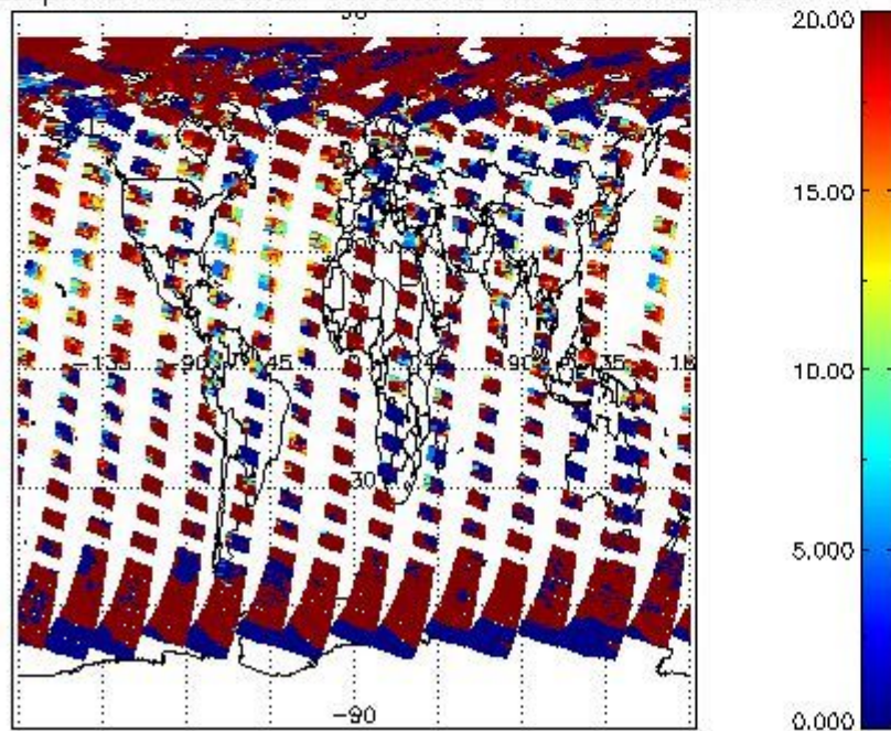
cL_opt_depth for 16AUG2004 00:00:00 to 17AUG2004 00:00:00
