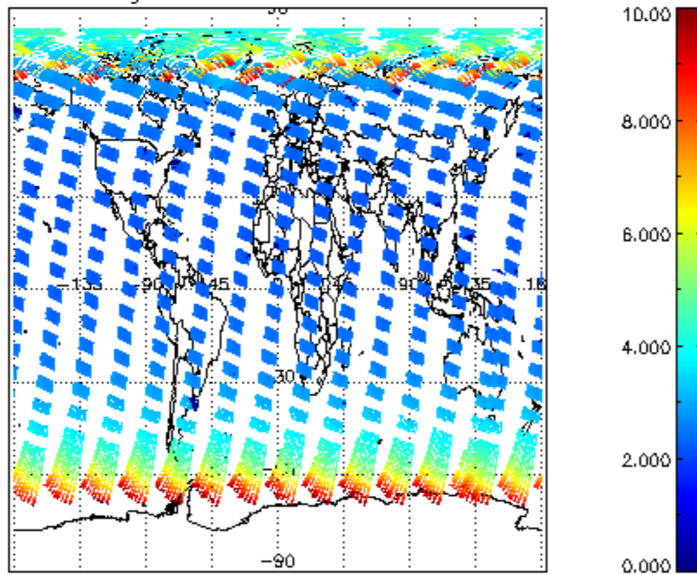
SCIOL2P_NADUV003_amf_gr for 16AUG2004 00:00:00 to 17AUG2004 00:00:00
