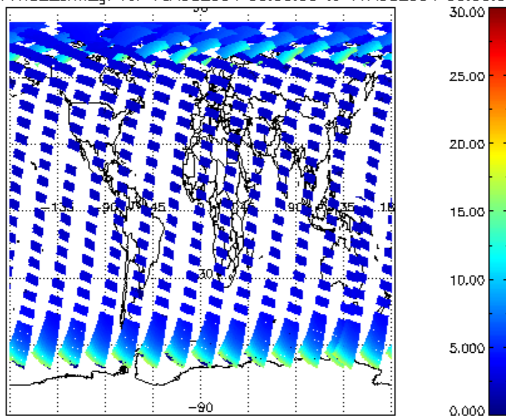
SCIOL2P_NADUV1NO2_amf_gr for 16AUG2004 00:00:00 to 17AUG2004 00:00:00
