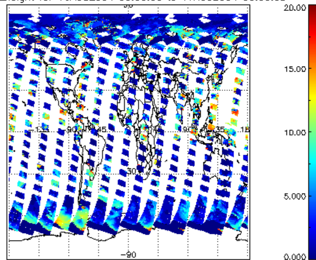
cL_top_height for 16AUG2004 00:00:00 to 17AUG2004 00:00:00
