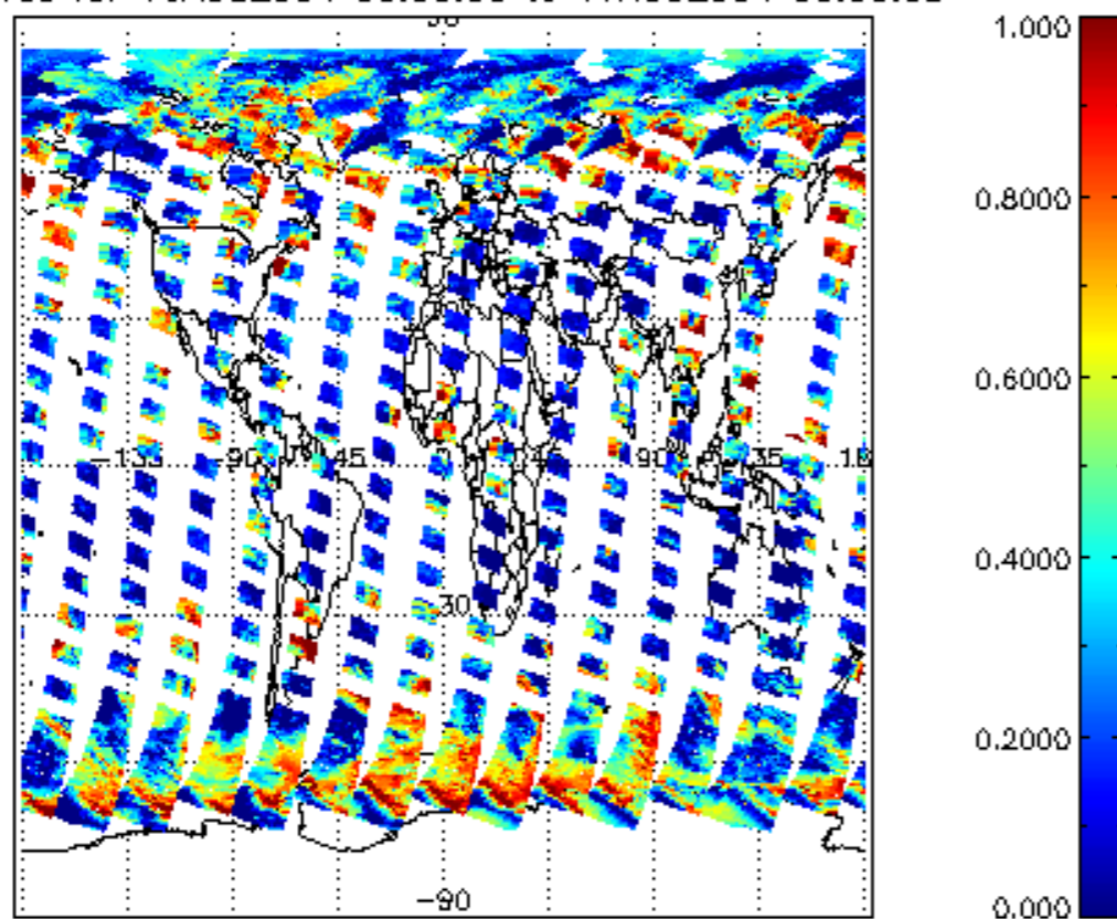
cL_frac for 16AUG2004 00:00:00 to 17AUG2004 00:00:00
