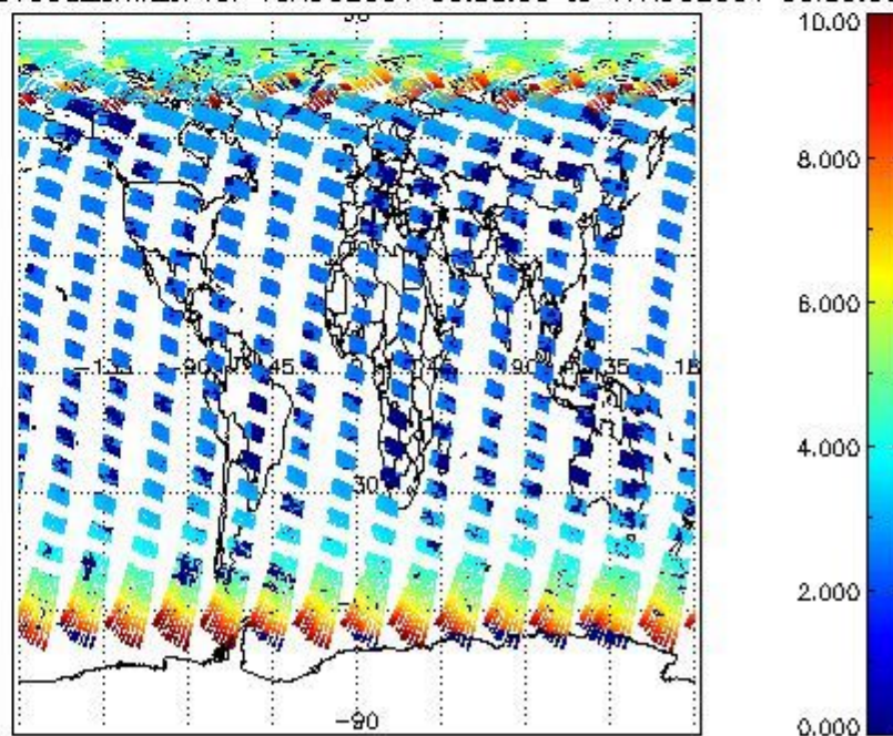
SCIOL2P_NADUV003_amf_sl for 16AUG2004 00:00:00 to 17AUG2004 00:00:00
