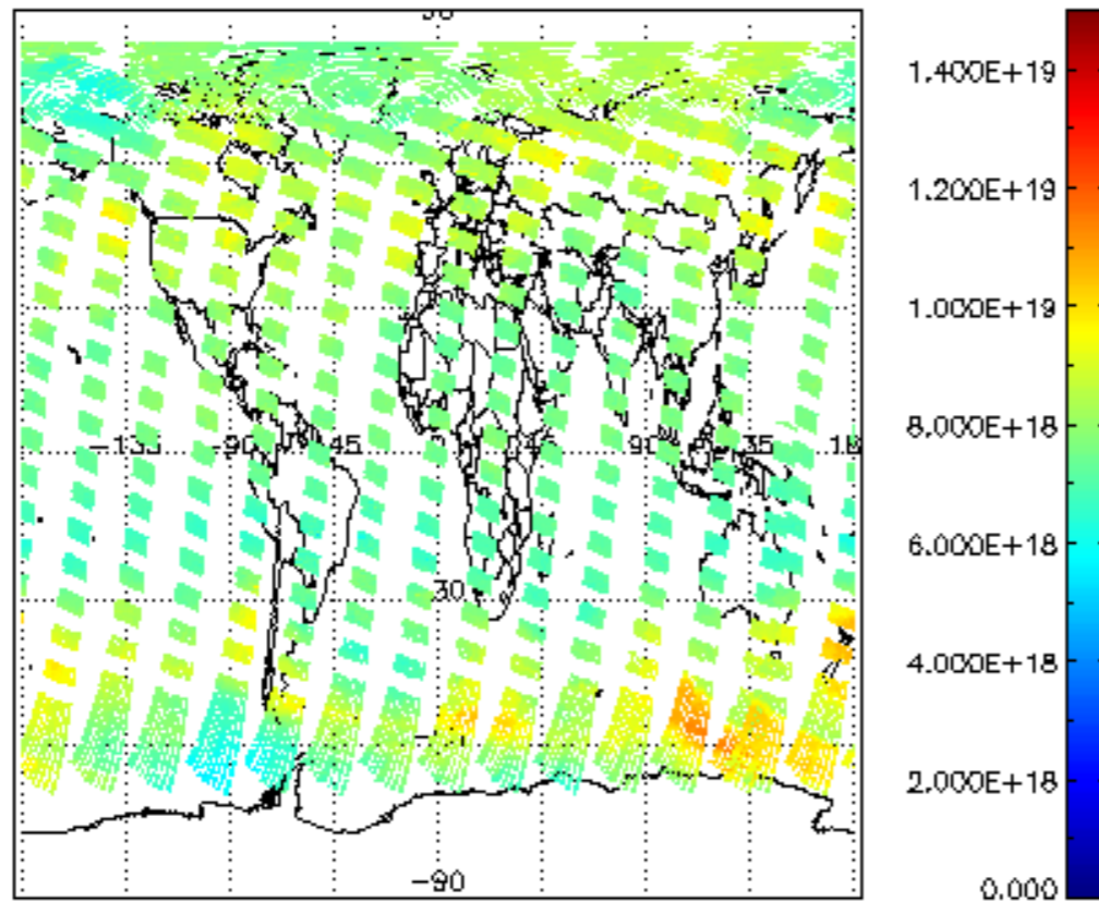
SCIOL2P_NADUV003_vcd for 16AUG2004 00:00:00 to 17AUG2004 00:00:00
