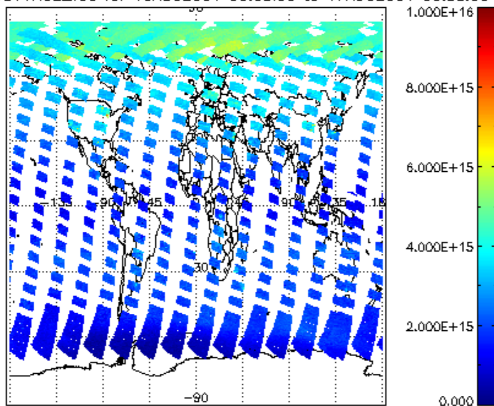
SCIOL2P_NADUV1NO2_vcd for 16AUG2004 00:00:00 to 17AUG2004 00:00:00
