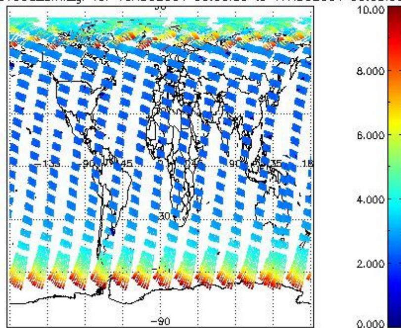
SCIOL2P_NADUV003_amf_gr for 16AUG2004 00:00:00 to 17AUG2004 00:00:00
