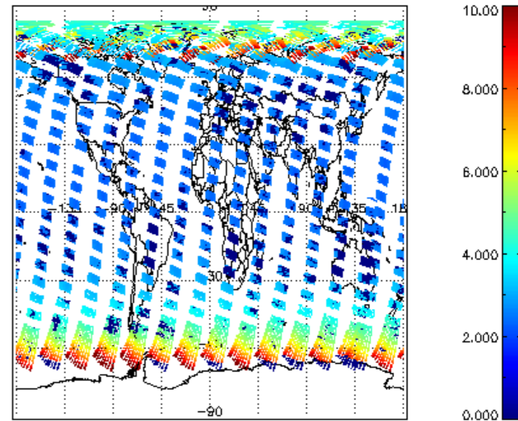
SCIOL2P_NADUV003_amf_cl for 16AUG2004 00:00:00 to 17AUG2004 00:00:00
