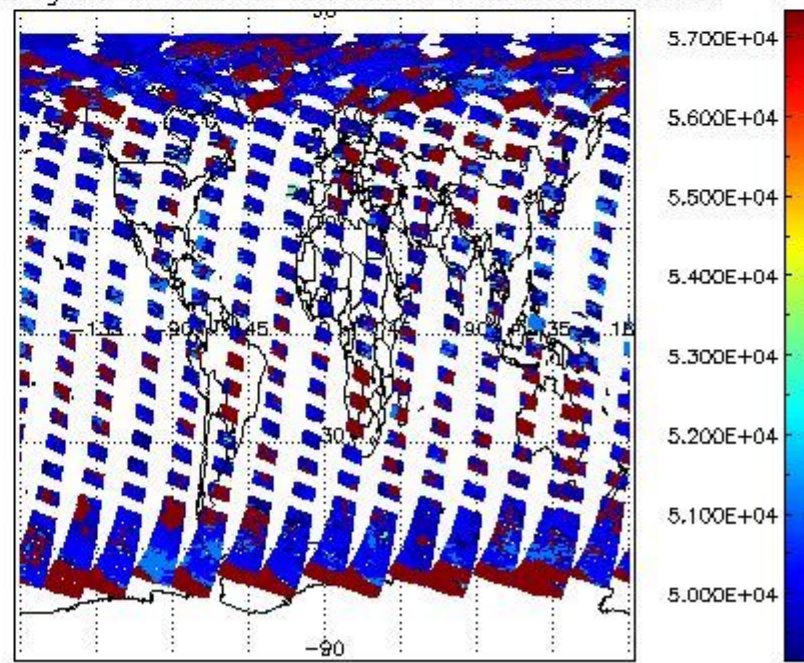
cloud_flags for 16AUG2004 00:00:00 to 17AUG2004 00:00:00
