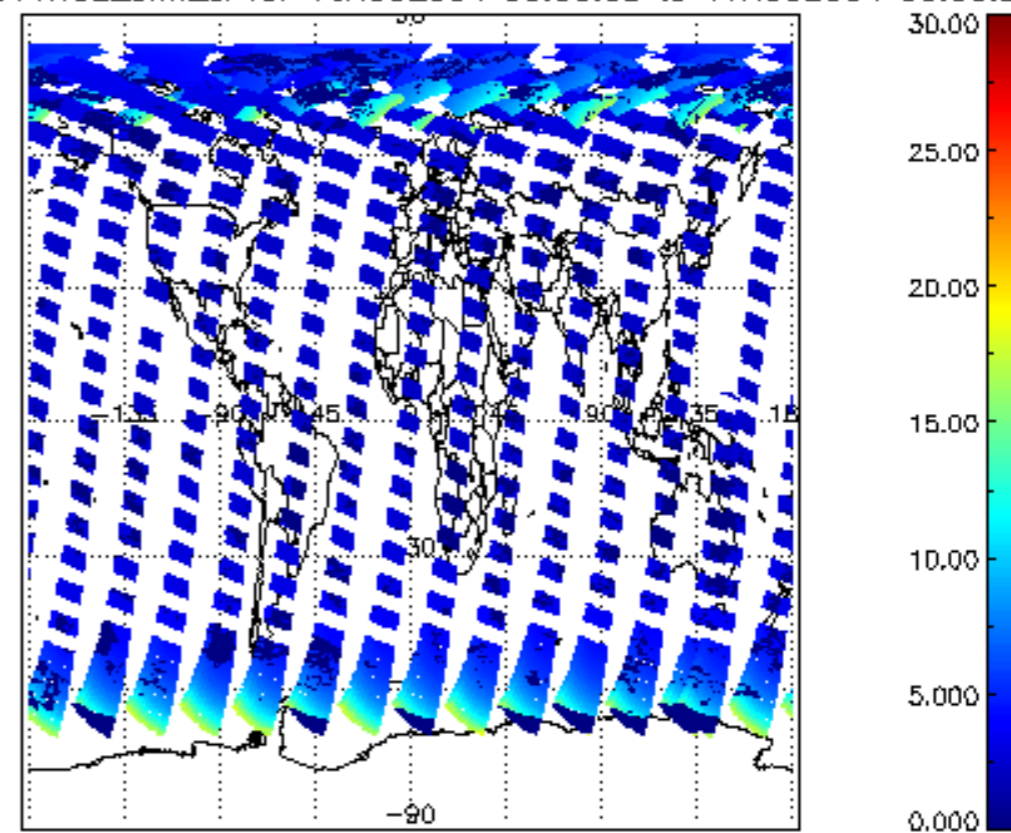
SCIOL2P_NADUV1NO2_amf_cl for 16AUG2004 00:00:00 to 17AUG2004 00:00:00
