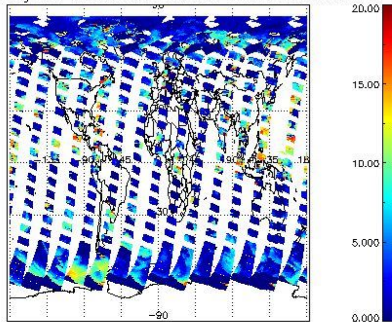
cL_top_height for 16AUG2004 00:00:00 to 17AUG2004 00:00:00
