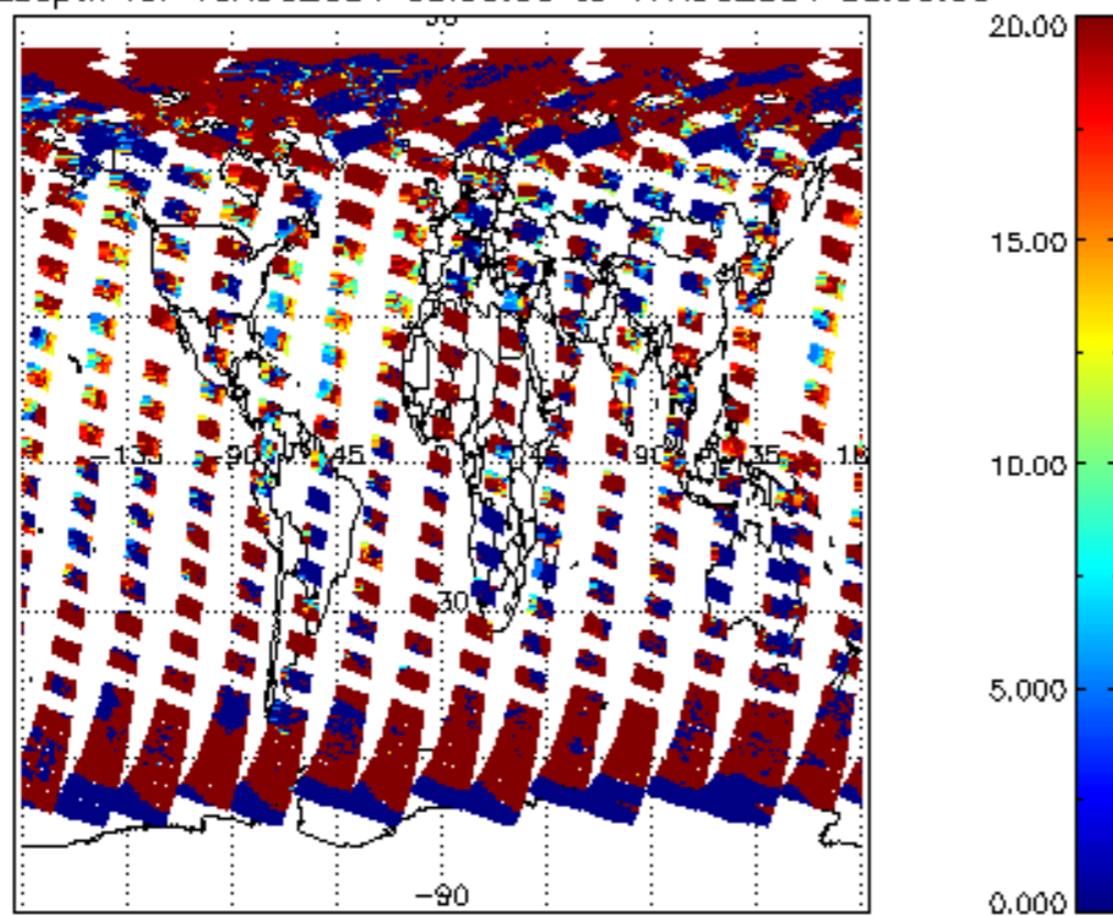
cL_opt_depth for 16AUG2004 00:00:00 to 17AUG2004 00:00:00
