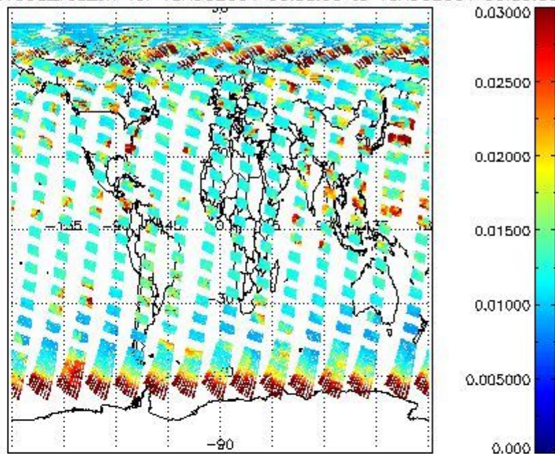
SCIOL2P_NADUV003_vcd_err for 15AUG2004 00:00:00 to 16AUG2004 00:00:00
