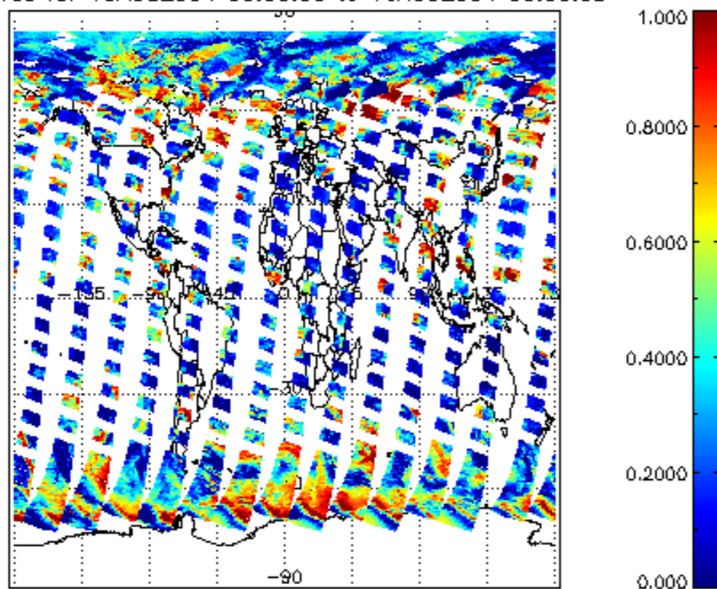
cL_frac for 15AUG2004 00:00:00 to 16AUG2004 00:00:00
