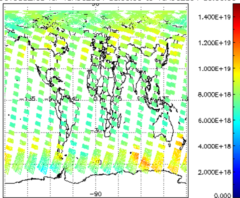
SCIOL2P_NADUV003_vcd for 15AUG2004 00:00:00 to 16AUG2004 00:00:00
