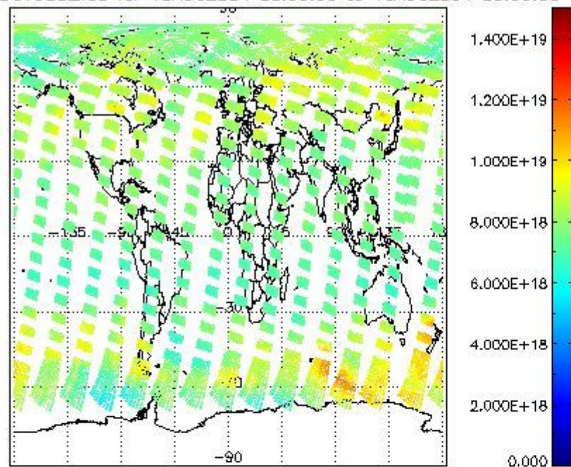
SCIOL2P_NADUV003_vcd for 15AUG2004 00:00:00 to 16AUG2004 00:00:00
