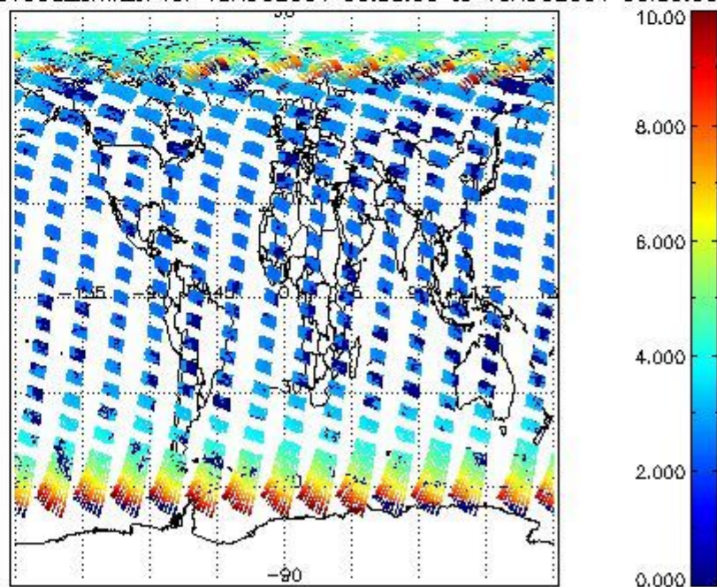
SCIOL2P_NADUV003_amf_cl for 15AUG2004 00:00:00 to 16AUG2004 00:00:00
