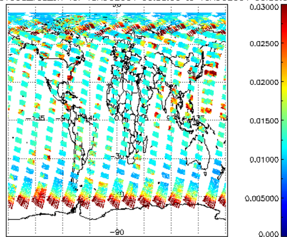
SCIOL2P_NADUV003_vcd_err for 15AUG2004 00:00:00 to 16AUG2004 00:00:00
