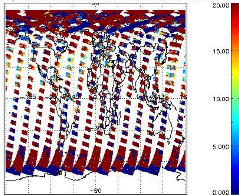
cL_opt_depth for 15AUG2004 00:00:00 to 16AUG2004 00:00:00
