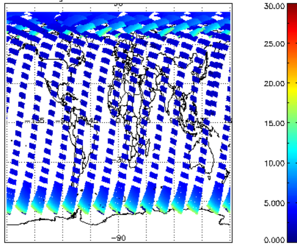
SCIOL2P_NADUV1NO2_amf_gr for 15AUG2004 00:00:00 to 16AUG2004 00:00:00
