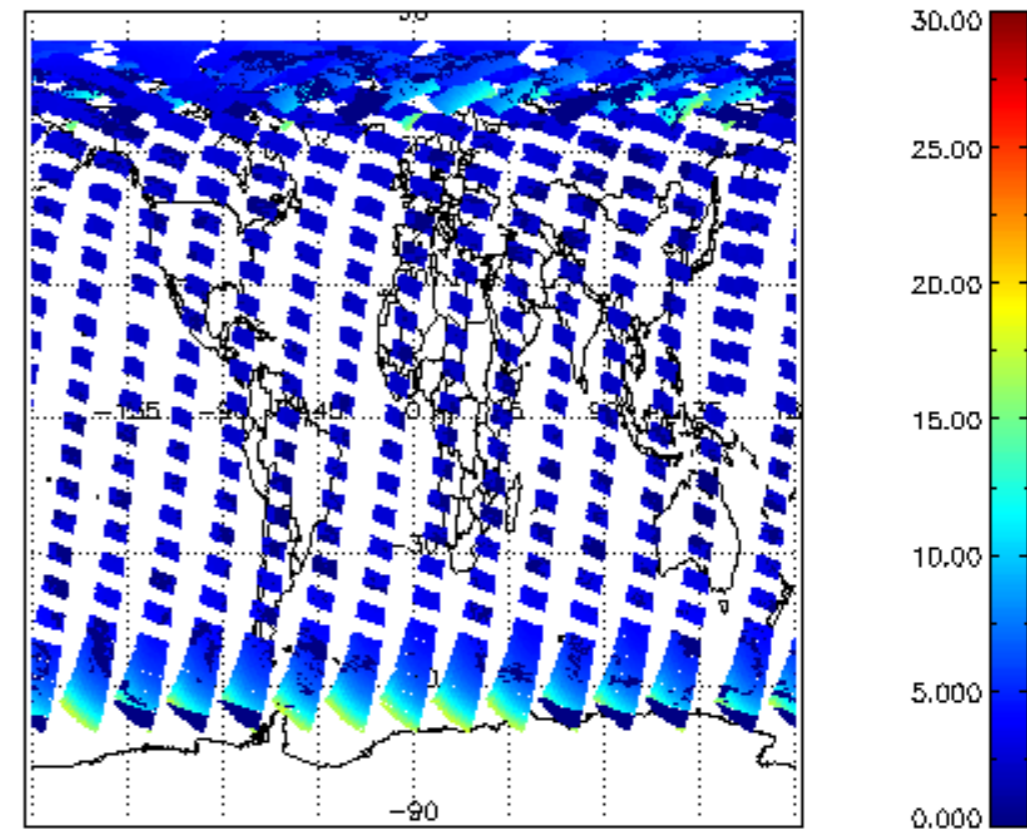
SCIOL2P_NADUV1NO2_amf_cl for 15AUG2004 00:00:00 to 16AUG2004 00:00:00
