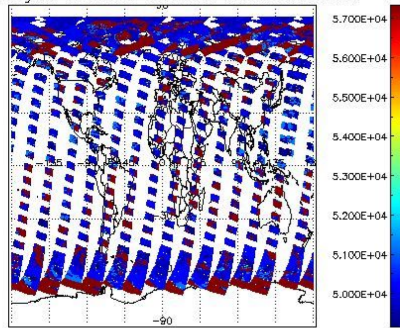
cloud_flags for 15AUG2004 00:00:00 to 16AUG2004 00:00:00
