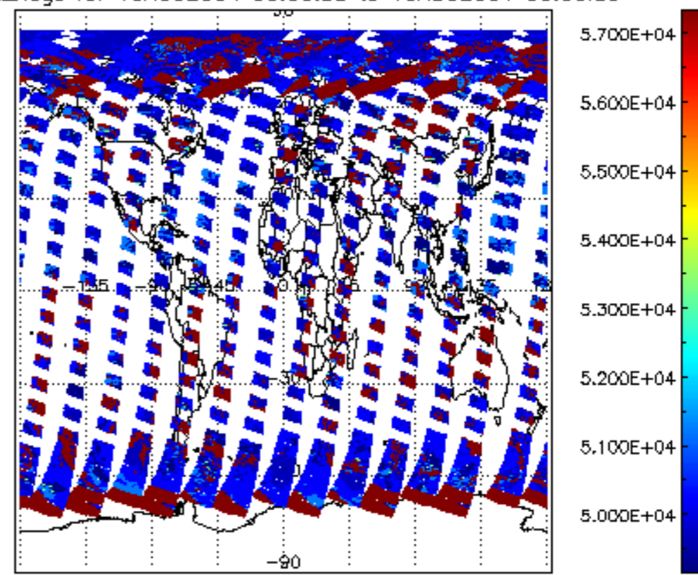
cloud_flags for 15AUG2004 00:00:00 to 16AUG2004 00:00:00
