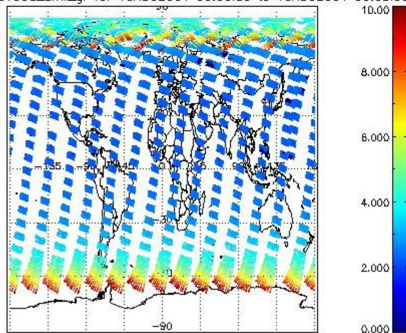
SCIOL2P_NADUV003_amf_gr for 15AUG2004 00:00:00 to 16AUG2004 00:00:00
