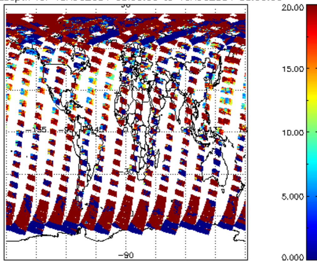
cL_opt_depth for 15AUG2004 00:00:00 to 16AUG2004 00:00:00
