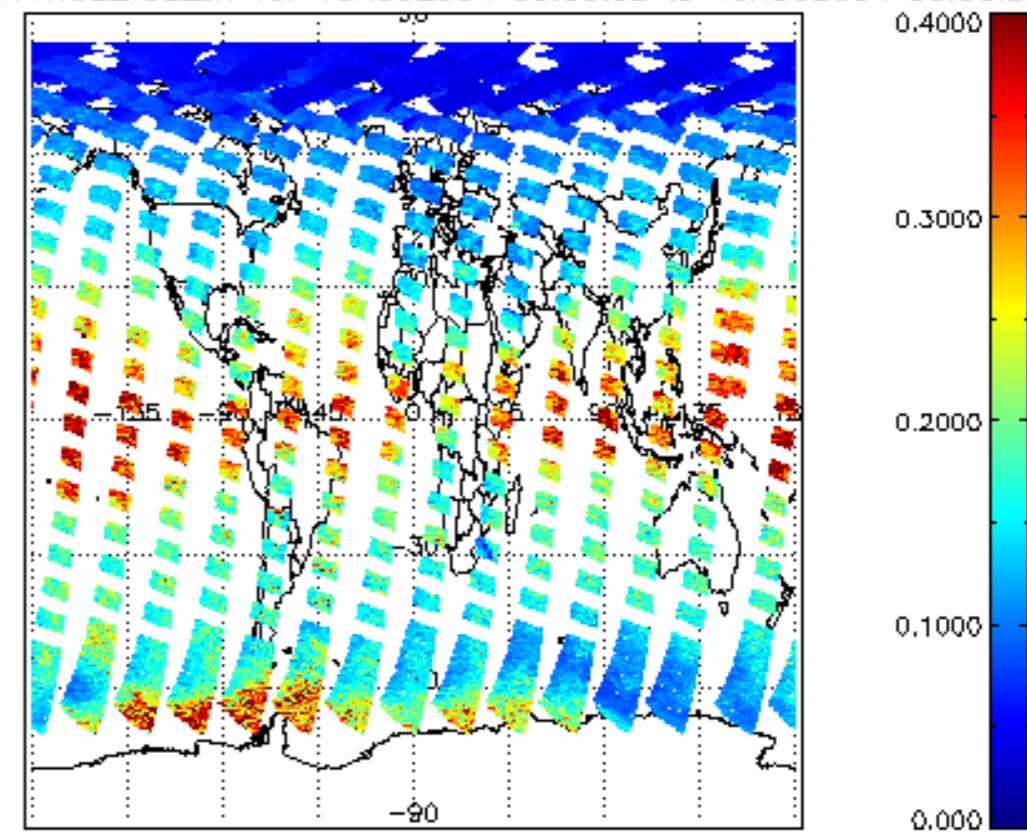
SCIOL2P_NADUV1NO2_vcd_err for 15AUG2004 00:00:00 to 16AUG2004 00:00:00
