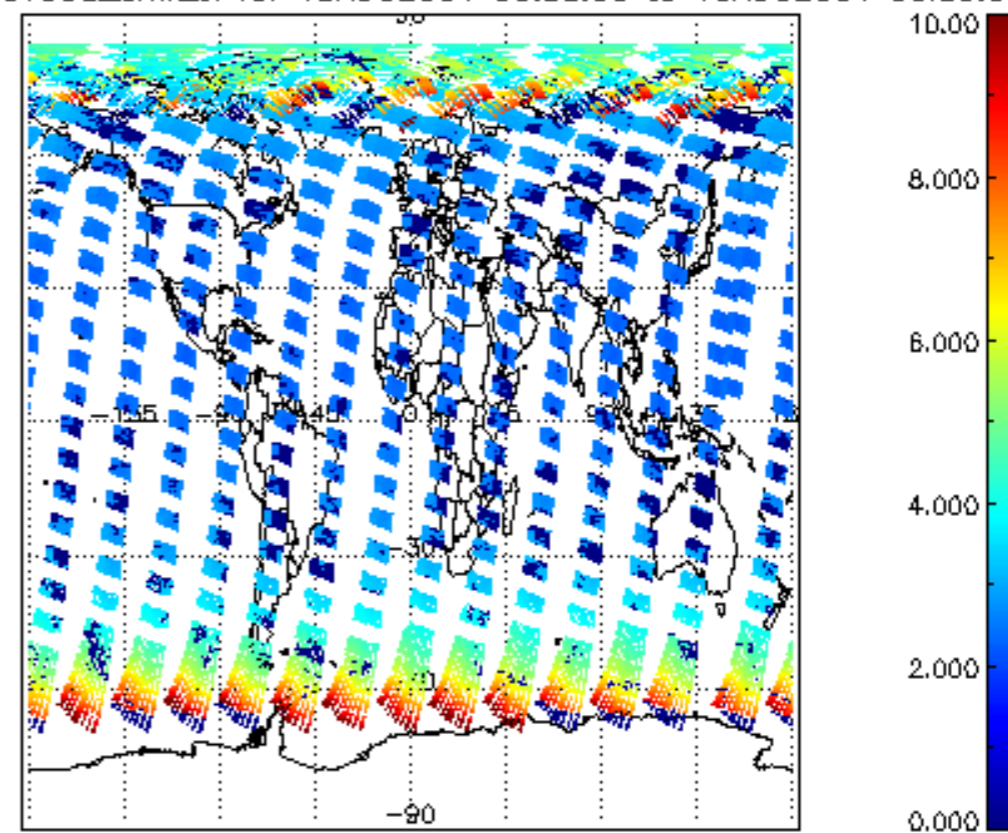
SCIOL2P_NADUV003_amf_cl for 15AUG2004 00:00:00 to 16AUG2004 00:00:00
