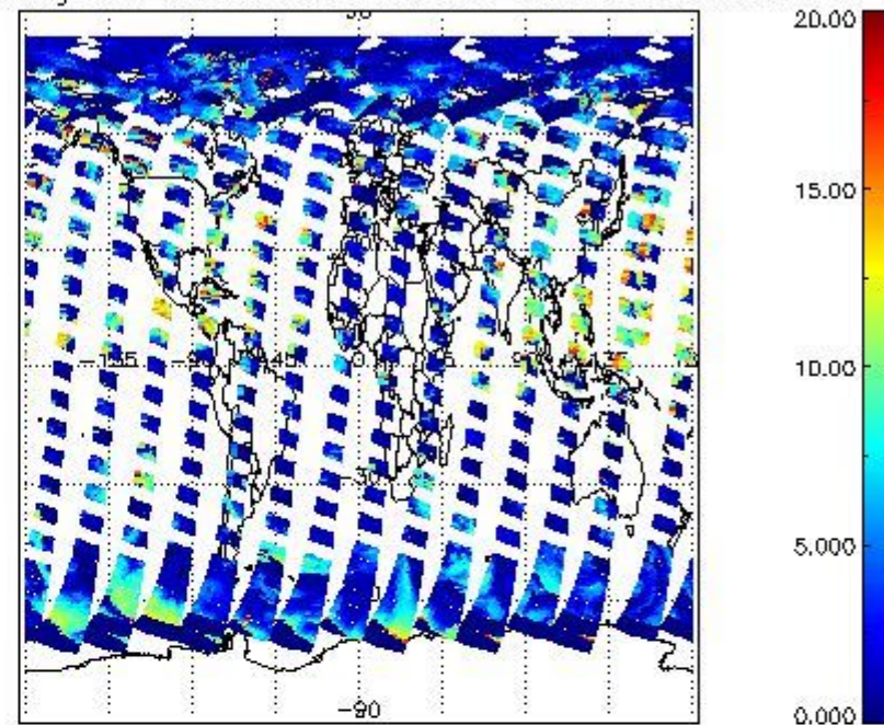
cL_top_height for 15AUG2004 00:00:00 to 16AUG2004 00:00:00
