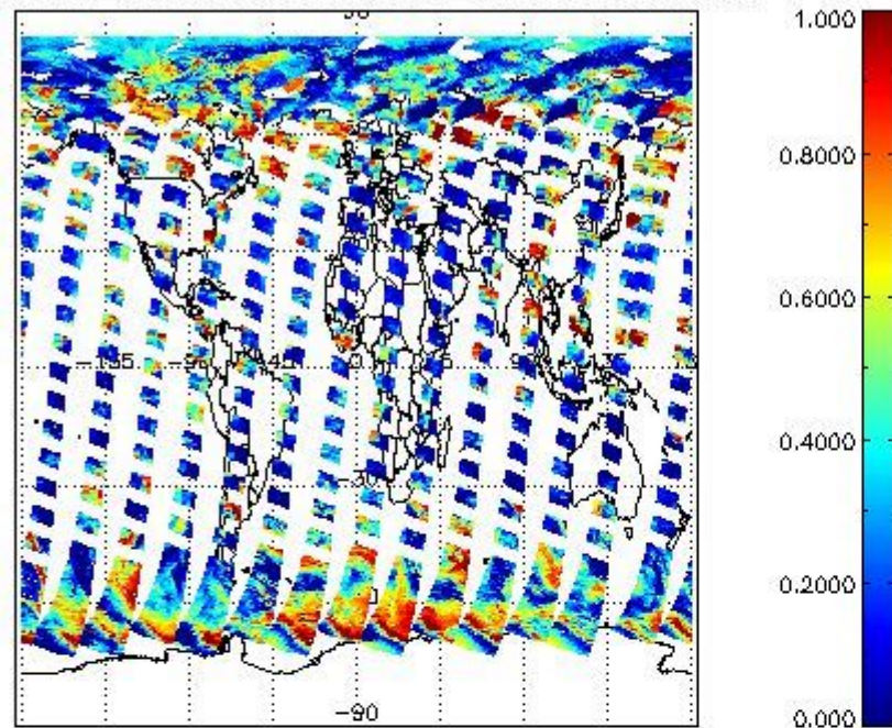
cL_frac for 15AUG2004 00:00:00 to 16AUG2004 00:00:00
