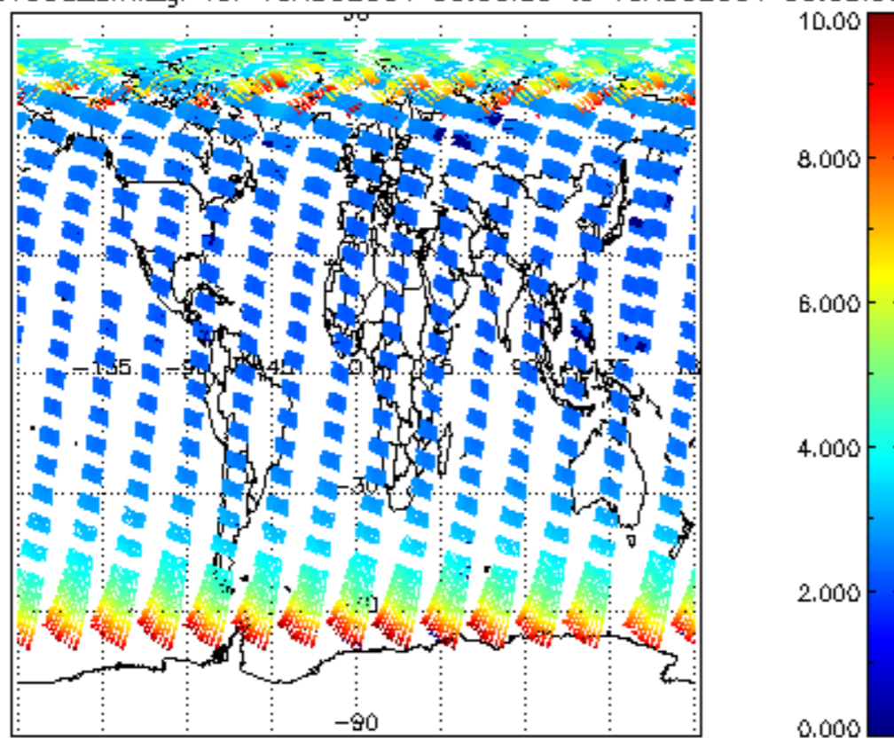
SCIOL2P_NADUV003_amf_gr for 15AUG2004 00:00:00 to 16AUG2004 00:00:00
