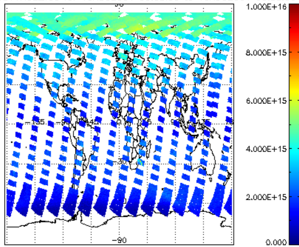
SCIOL2P_NADUV1NO2_vcd for 15AUG2004 00:00:00 to 16AUG2004 00:00:00
