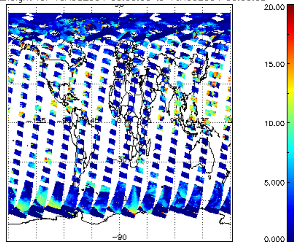
cL_top_height for 15AUG2004 00:00:00 to 16AUG2004 00:00:00
