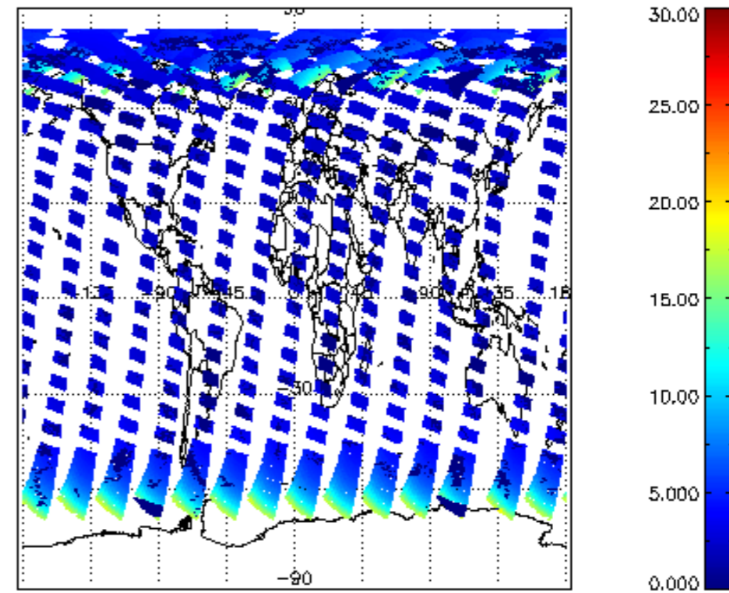
SCIOL2P_NADUV1NO2_amf_cl for 13AUG2004 00:00:00 to 14AUG2004 00:00:00
