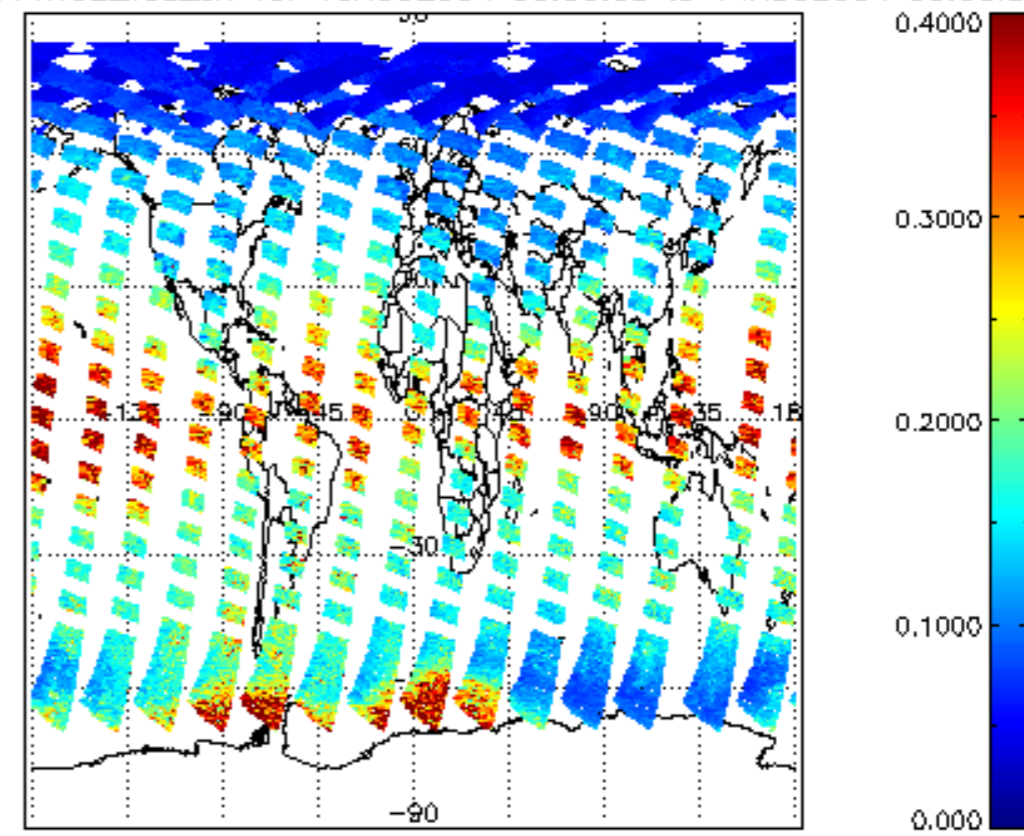
SCIOL2P_NADUV1NO2_vcd_err for 13AUG2004 00:00:00 to 14AUG2004 00:00:00
