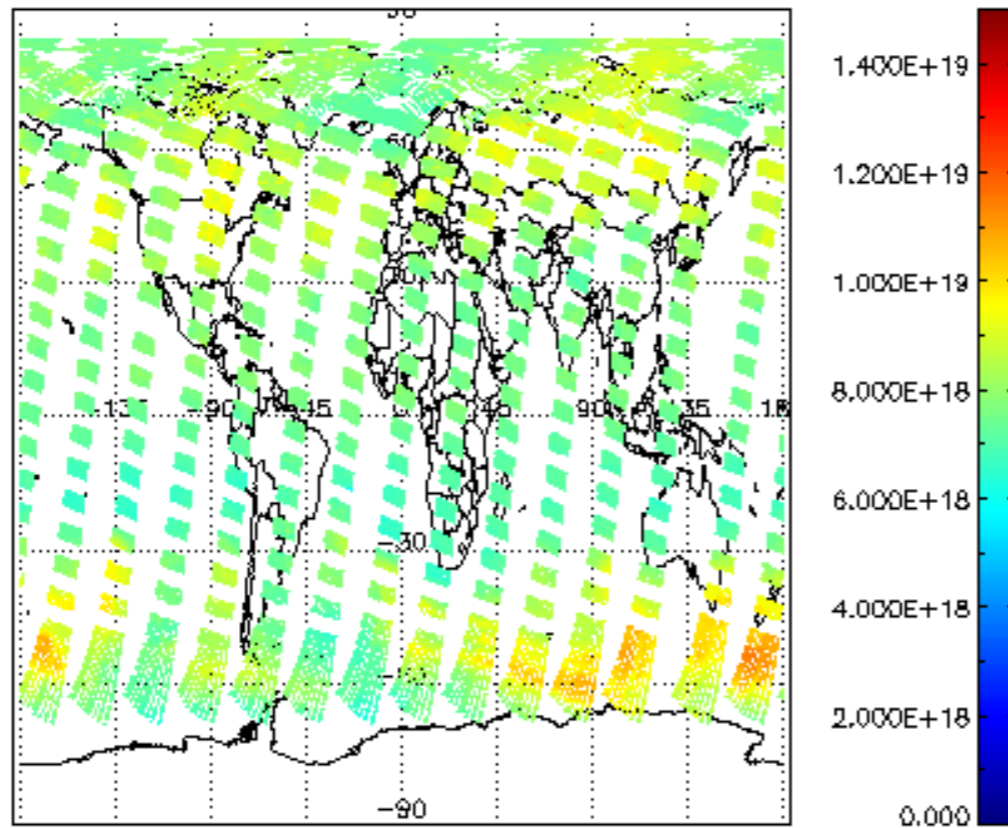
SCIOL2P_NADUV003_vcd for 13AUG2004 00:00:00 to 14AUG2004 00:00:00
