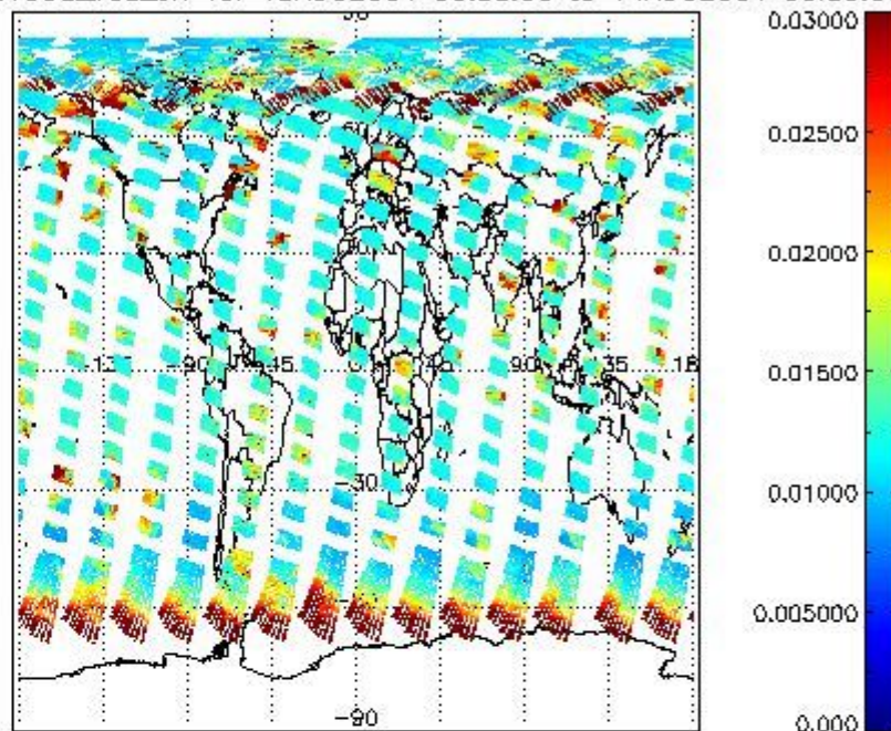
SCIOL2P_NADUV003_vcd_err for 13AUG2004 00:00:00 to 14AUG2004 00:00:00
