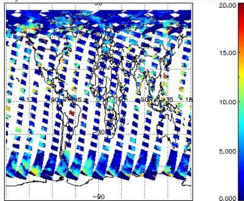
cL_top_height for 13AUG2004 00:00:00 to 14AUG2004 00:00:00
