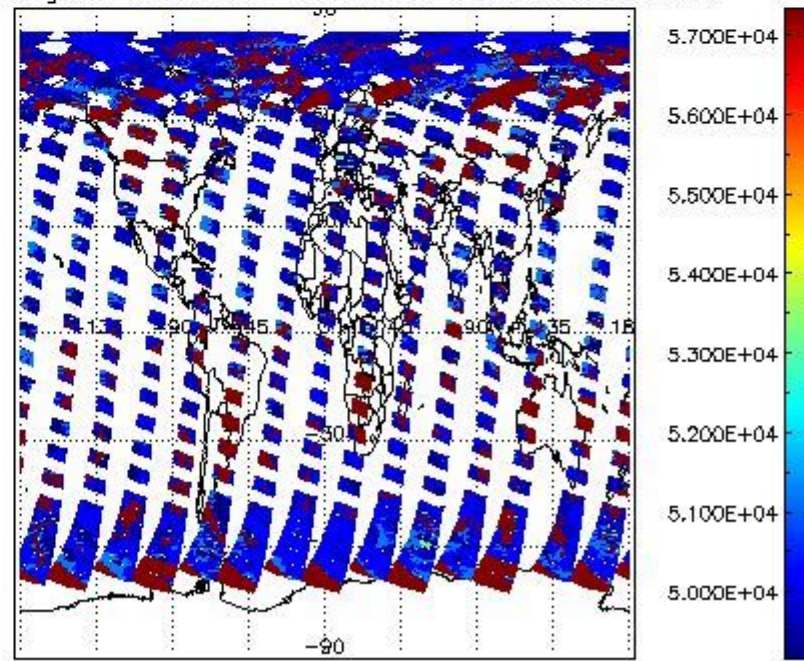
cloud_flags for 13AUG2004 00:00:00 to 14AUG2004 00:00:00
