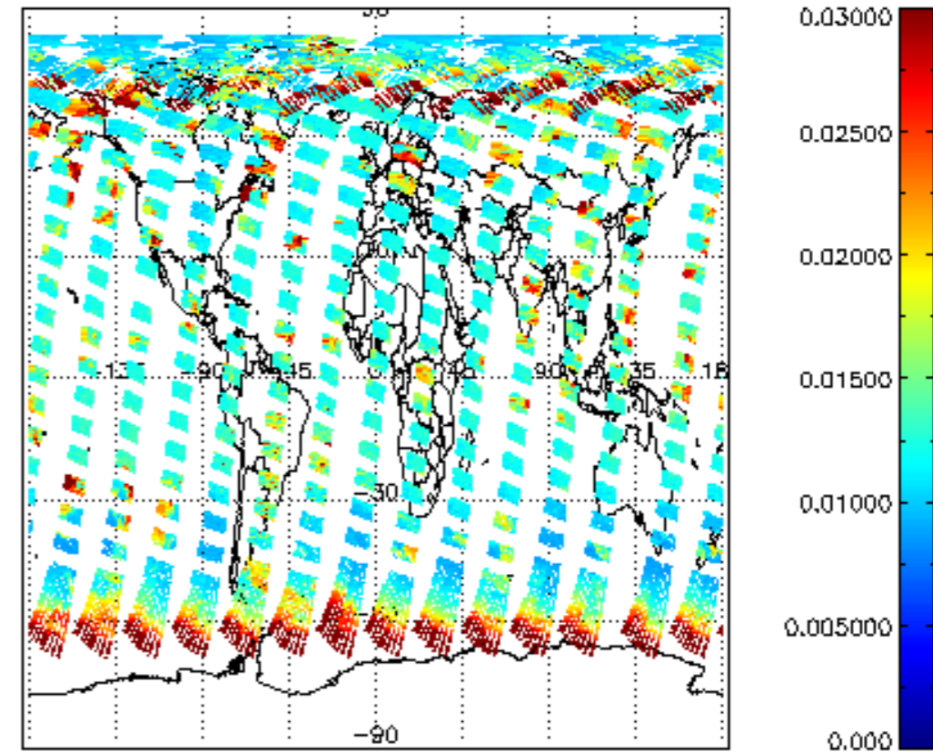
SCIOL2P_NADUV003_vcd_err for 13AUG2004 00:00:00 to 14AUG2004 00:00:00
