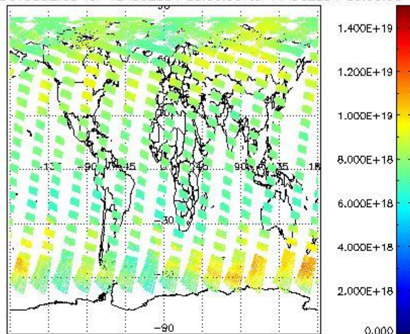
SCIOL2P_NADUV003_vcd for 13AUG2004 00:00:00 to 14AUG2004 00:00:00
