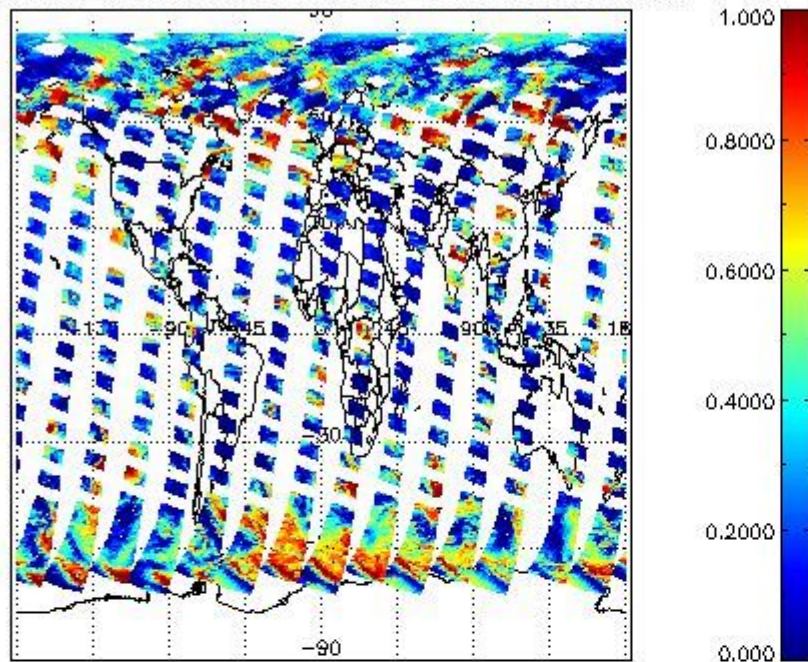
cL_frac for 13AUG2004 00:00:00 to 14AUG2004 00:00:00
