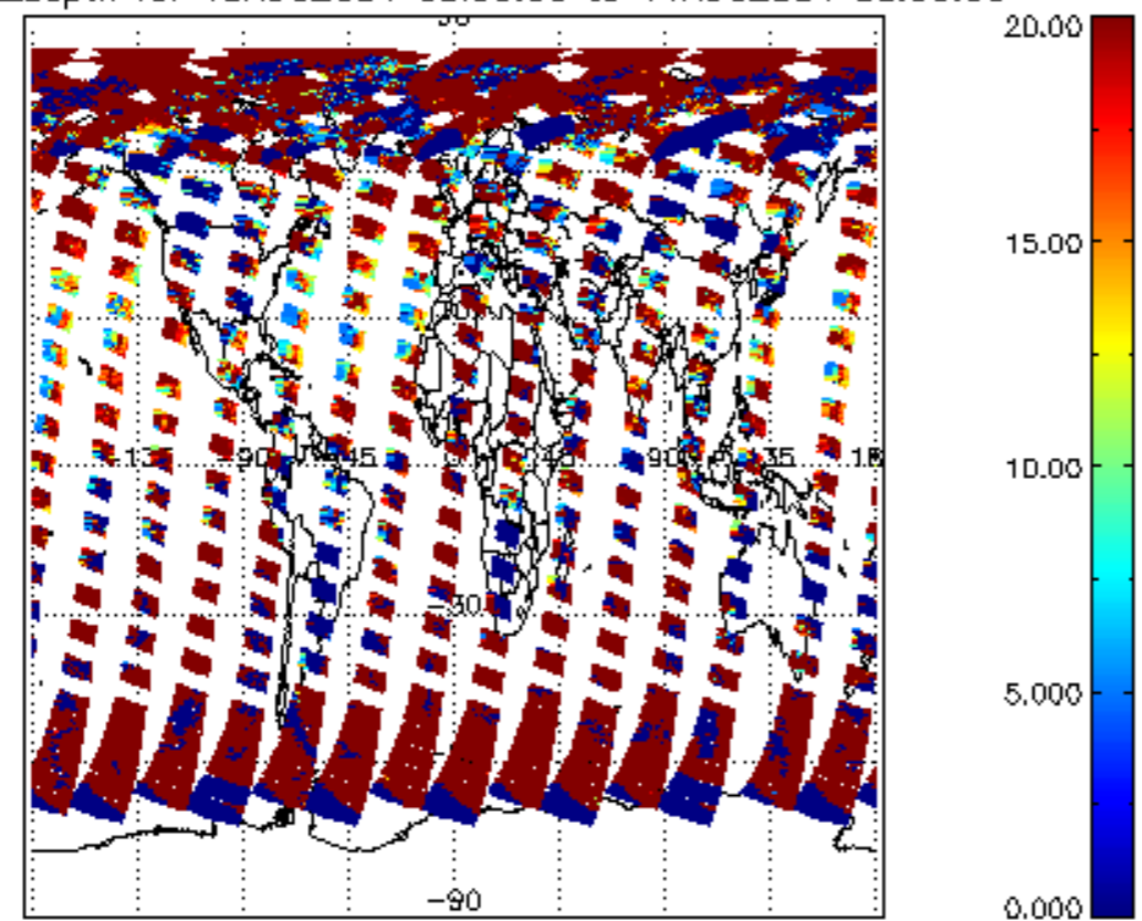
cL_opt_depth for 13AUG2004 00:00:00 to 14AUG2004 00:00:00
