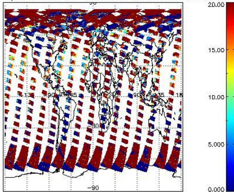
cL_opt_depth for 13AUG2004 00:00:00 to 14AUG2004 00:00:00
