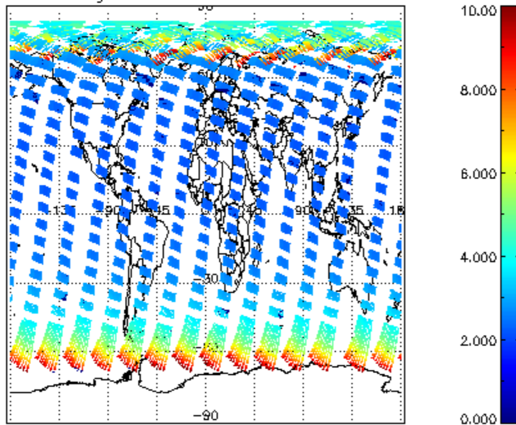
SCIOL2P_NADUV003_amf_gr for 13AUG2004 00:00:00 to 14AUG2004 00:00:00
