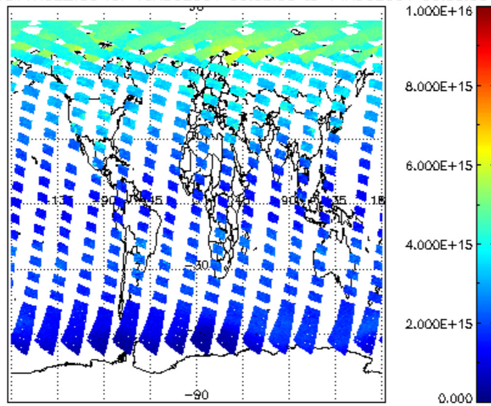
SCIOL2P_NADUV1NO2_vcd for 13AUG2004 00:00:00 to 14AUG2004 00:00:00
