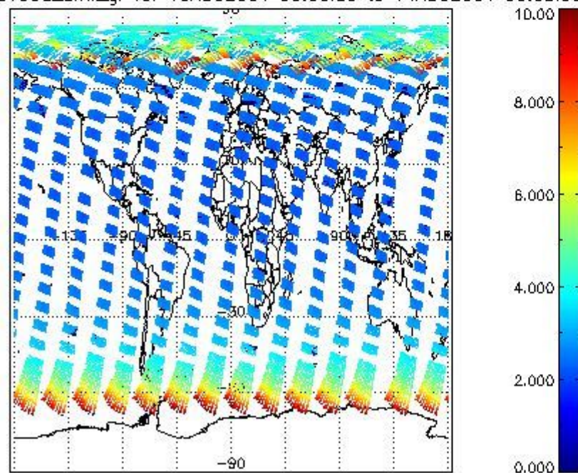
SCIOL2P_NADUV003_amf_gr for 13AUG2004 00:00:00 to 14AUG2004 00:00:00
