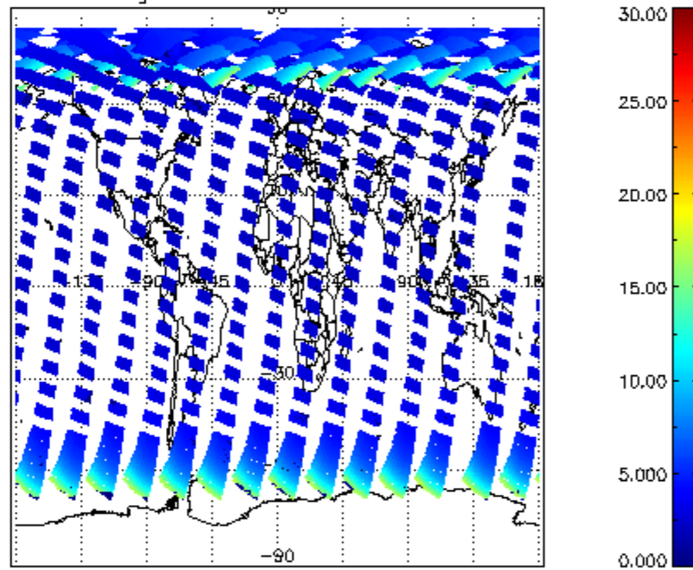
SCIOL2P_NADUV1NO2_amf_gr for 13AUG2004 00:00:00 to 14AUG2004 00:00:00
