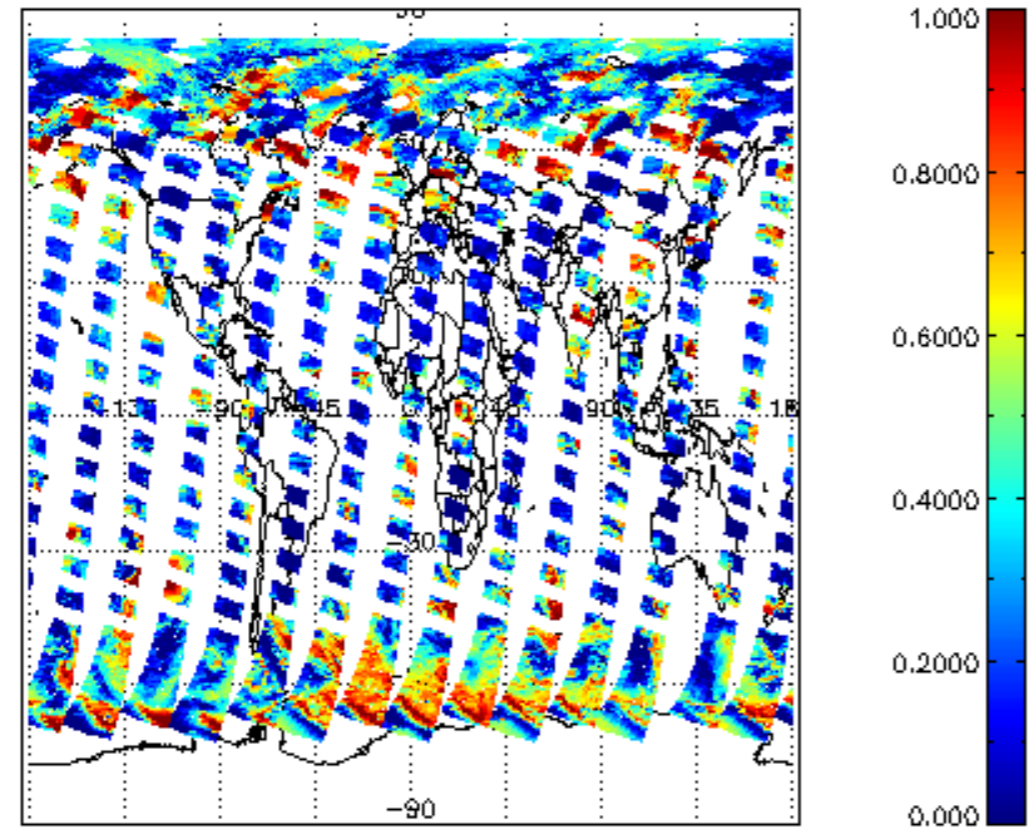
cL_frac for 13AUG2004 00:00:00 to 14AUG2004 00:00:00
