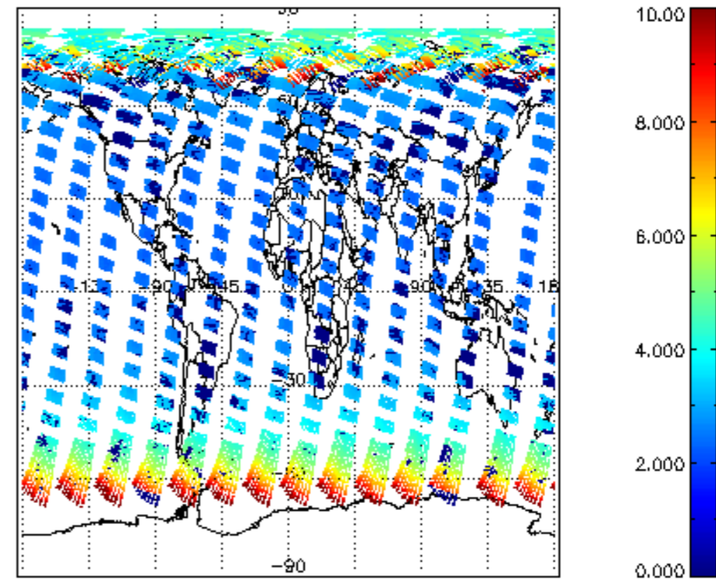
SCIOL2P_NADUV003_amf_cl for 13AUG2004 00:00:00 to 14AUG2004 00:00:00
