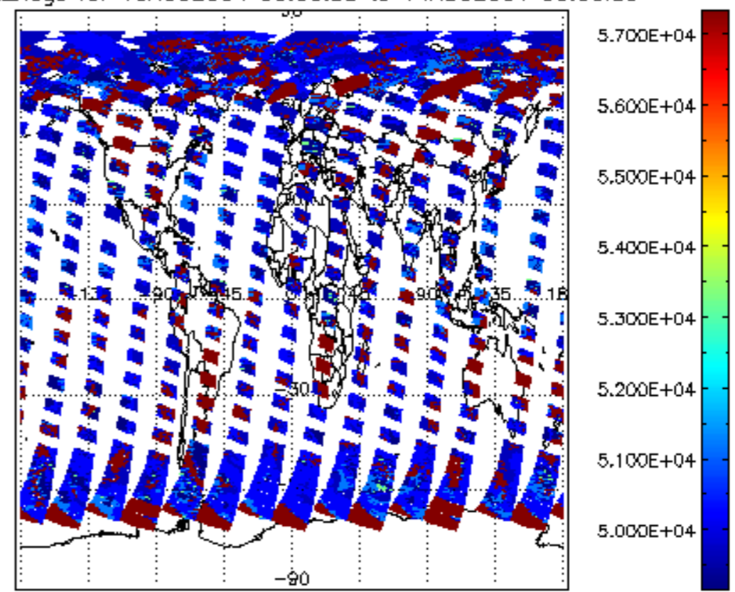
cloud_flags for 13AUG2004 00:00:00 to 14AUG2004 00:00:00
