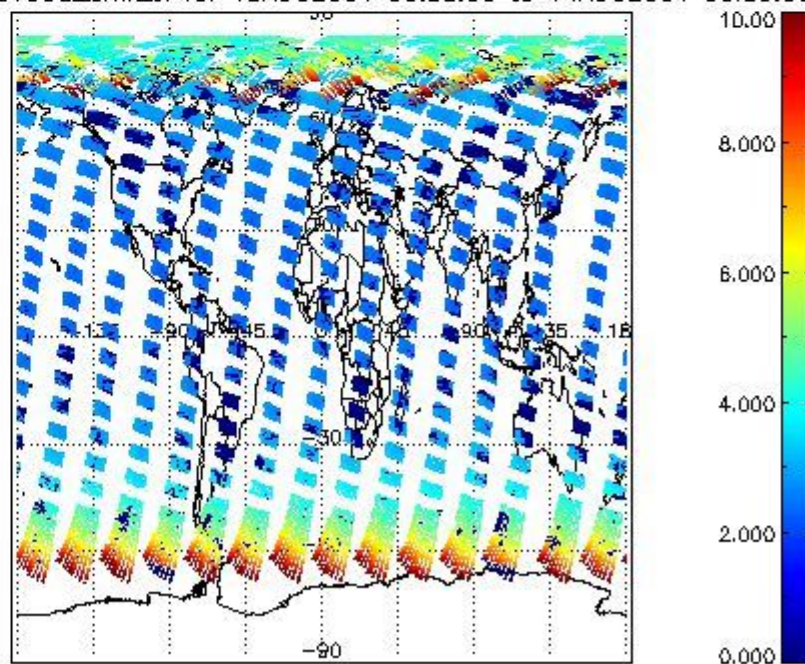
SCIOL2P_NADUV003_amf_cl for 13AUG2004 00:00:00 to 14AUG2004 00:00:00
