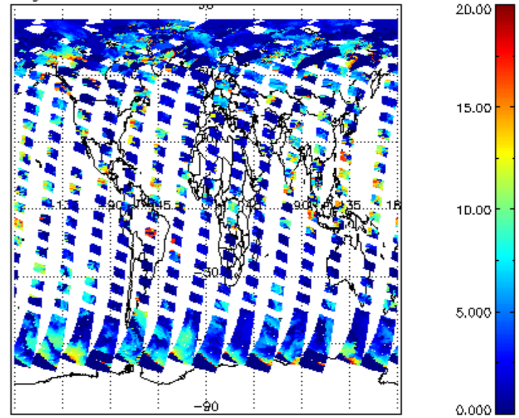
cL_top_height for 13AUG2004 00:00:00 to 14AUG2004 00:00:00
