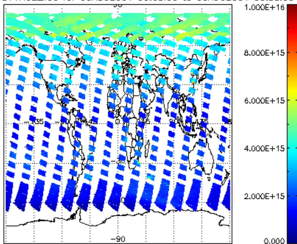
SCIOL2P_NADUV1NO2_vcd for 05AUG2004 00:00:00 to 06AUG2004 00:00:00
