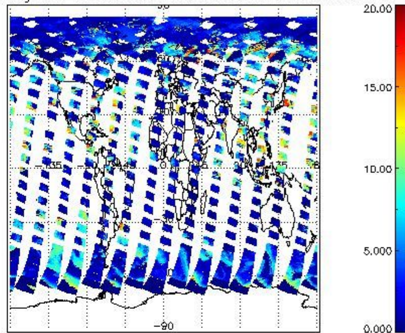
cL_top_height for 05AUG2004 00:00:00 to 06AUG2004 00:00:00
