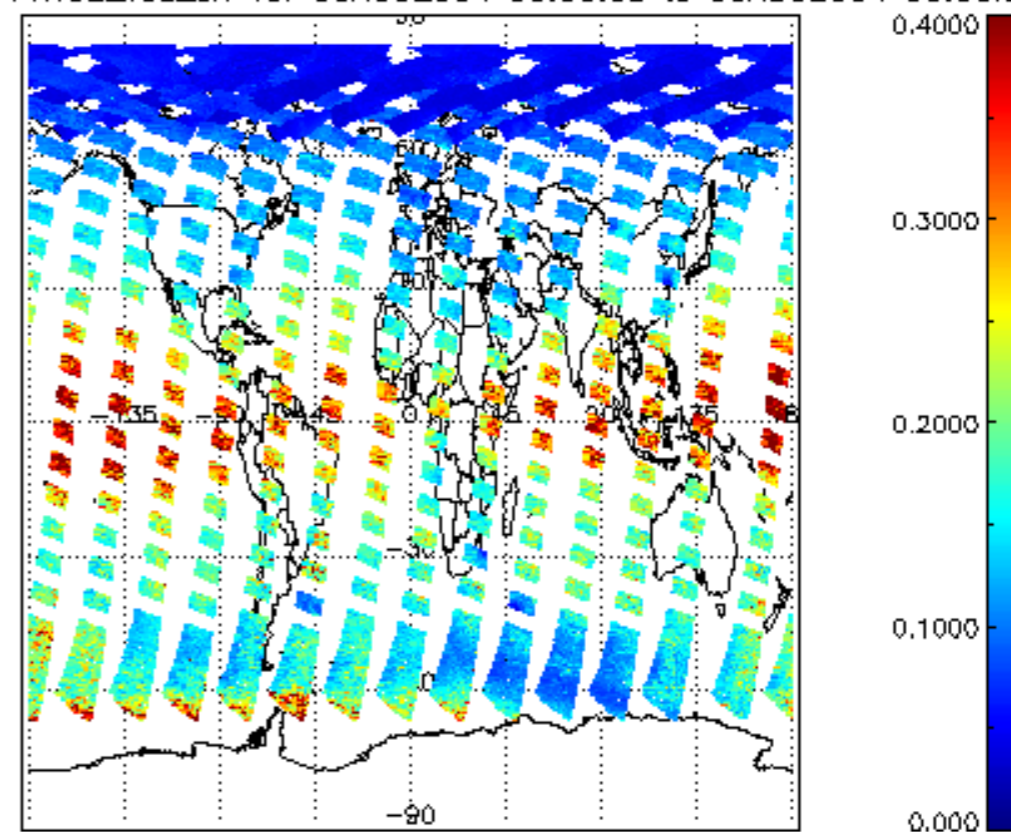
SCIOL2P_NADUV1NO2_vcd_err for 05AUG2004 00:00:00 to 06AUG2004 00:00:00
