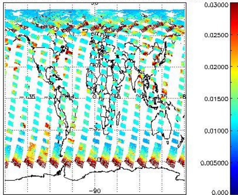
SCIOL2P_NADUV003_vcd_err for 05AUG2004 00:00:00 to 06AUG2004 00:00:00
