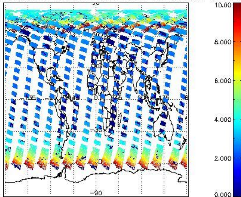
SCIOL2P_NADUV003_amf_cl for 05AUG2004 00:00:00 to 06AUG2004 00:00:00
