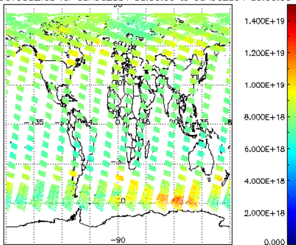
SCIOL2P_NADUV003_vcd for 05AUG2004 00:00:00 to 06AUG2004 00:00:00
