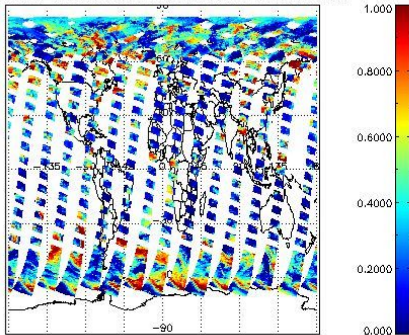
cL_frac for 05AUG2004 00:00:00 to 06AUG2004 00:00:00
