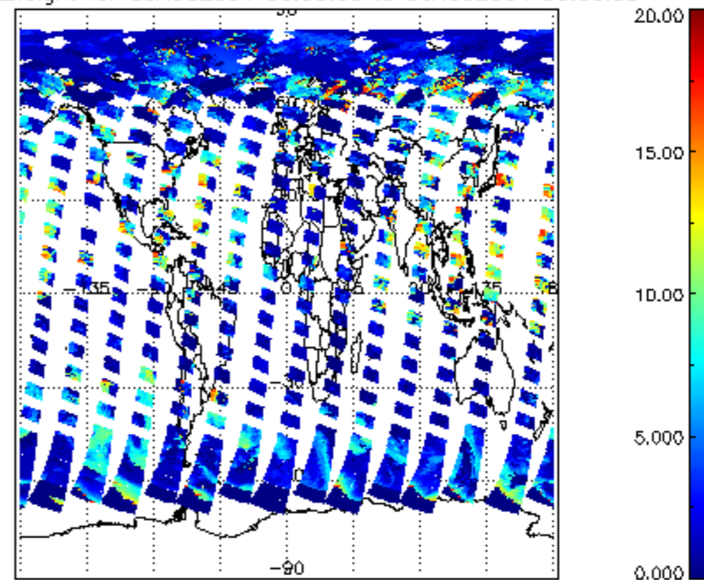
cL_top_height for 05AUG2004 00:00:00 to 06AUG2004 00:00:00
