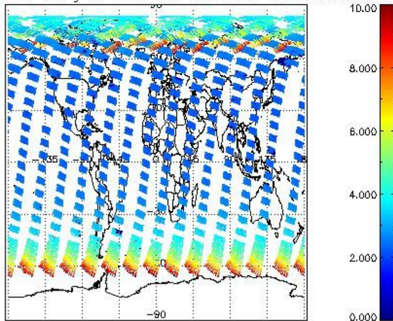
SCIOL2P_NADUV003_amf_gr for 05AUG2004 00:00:00 to 06AUG2004 00:00:00
