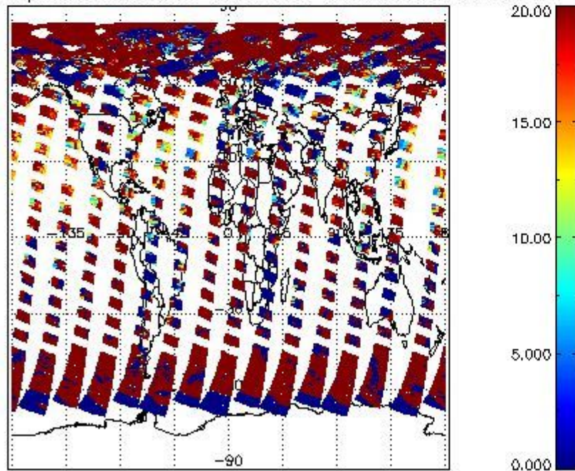
cL_opt_depth for 05AUG2004 00:00:00 to 06AUG2004 00:00:00
