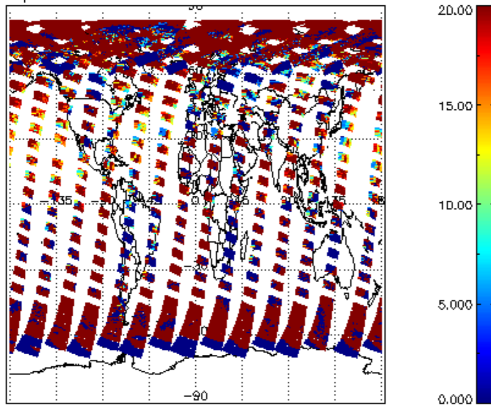
cL_opt_depth for 05AUG2004 00:00:00 to 06AUG2004 00:00:00
