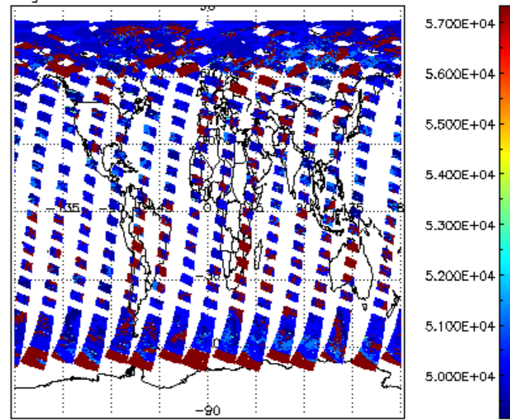
cloud_flags for 05AUG2004 00:00:00 to 06AUG2004 00:00:00
