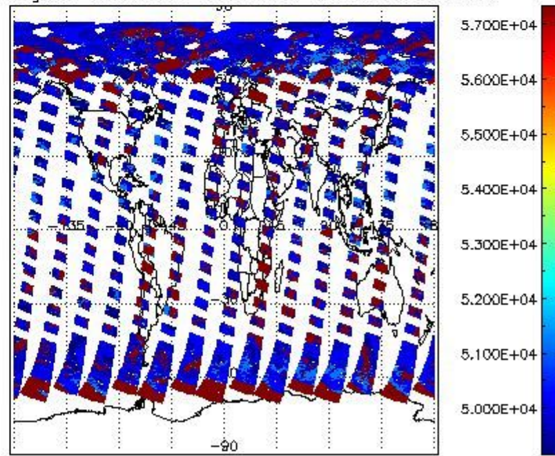
cloud_flags for 05AUG2004 00:00:00 to 06AUG2004 00:00:00
