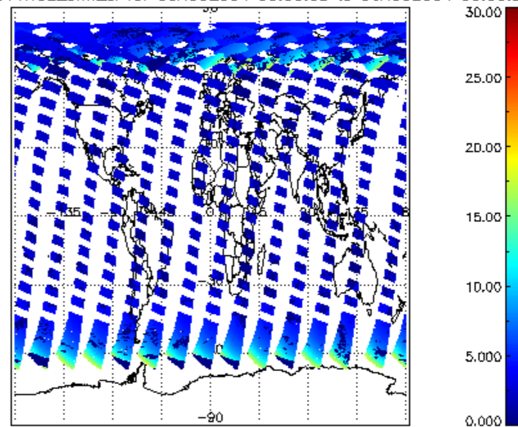
SCIOL2P_NADUV1NO2_amf_cl for 05AUG2004 00:00:00 to 06AUG2004 00:00:00
