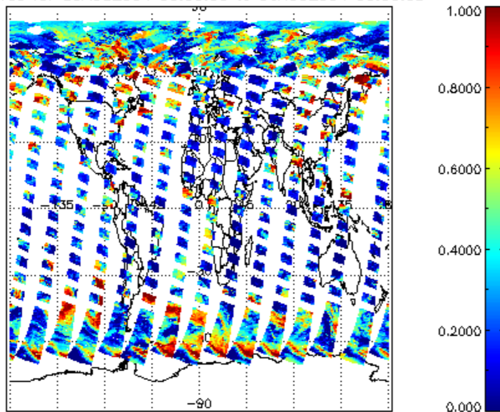
cL_frac for 05AUG2004 00:00:00 to 06AUG2004 00:00:00
