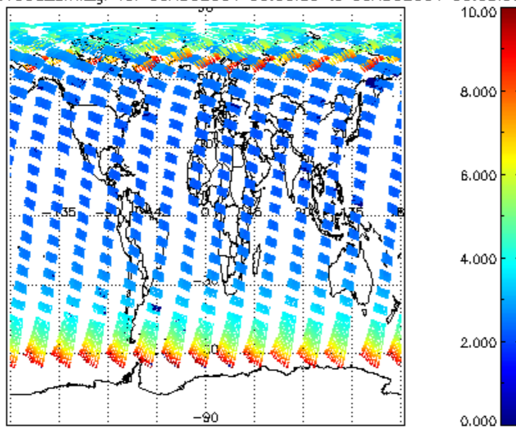
SCIOL2P_NADUV003_amf_gr for 05AUG2004 00:00:00 to 06AUG2004 00:00:00
