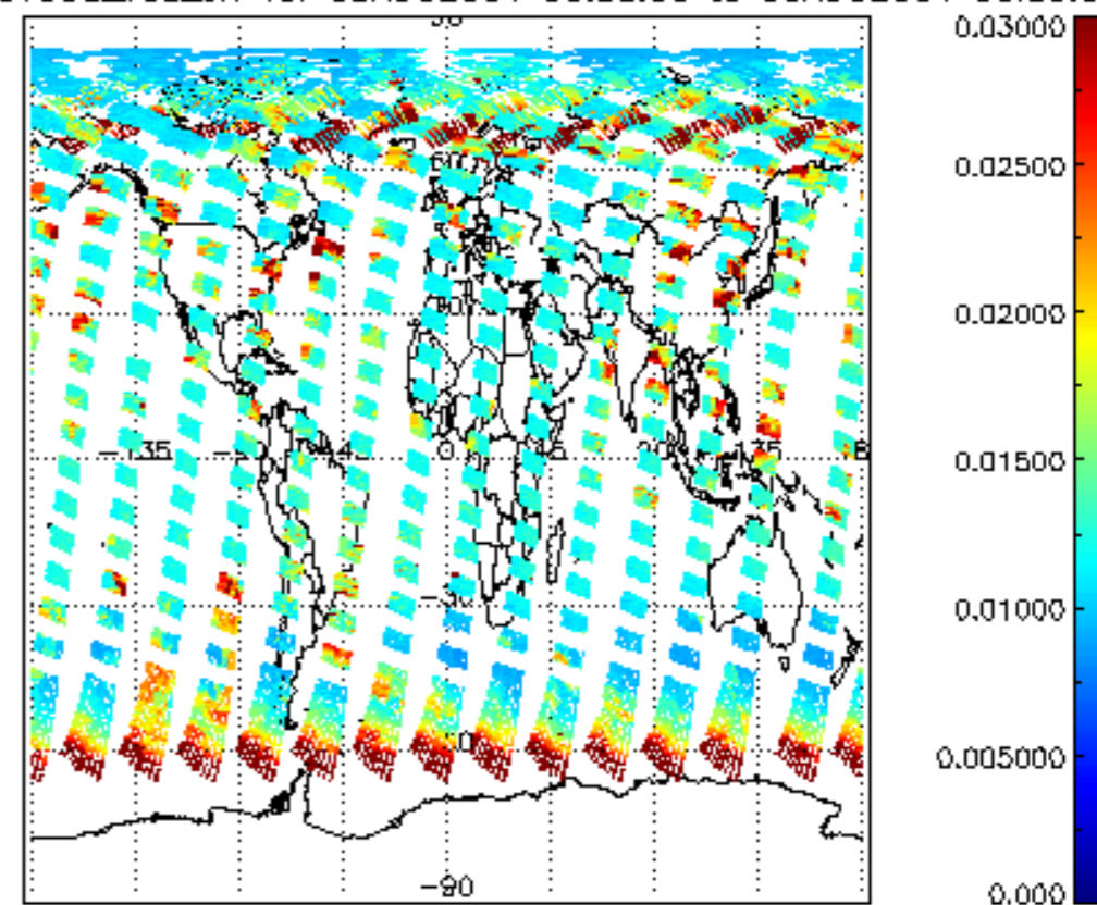
SCIOL2P_NADUV003_vcd_err for 05AUG2004 00:00:00 to 06AUG2004 00:00:00
