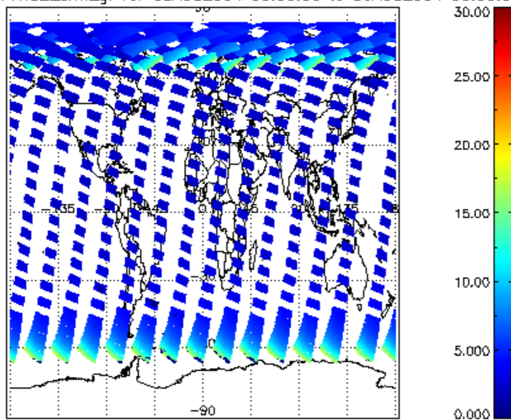
SCIOL2P_NADUV1NO2_amf_gr for 05AUG2004 00:00:00 to 06AUG2004 00:00:00
