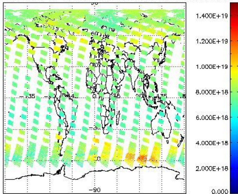
SCIOL2P_NADUV003_vcd for 05AUG2004 00:00:00 to 06AUG2004 00:00:00
