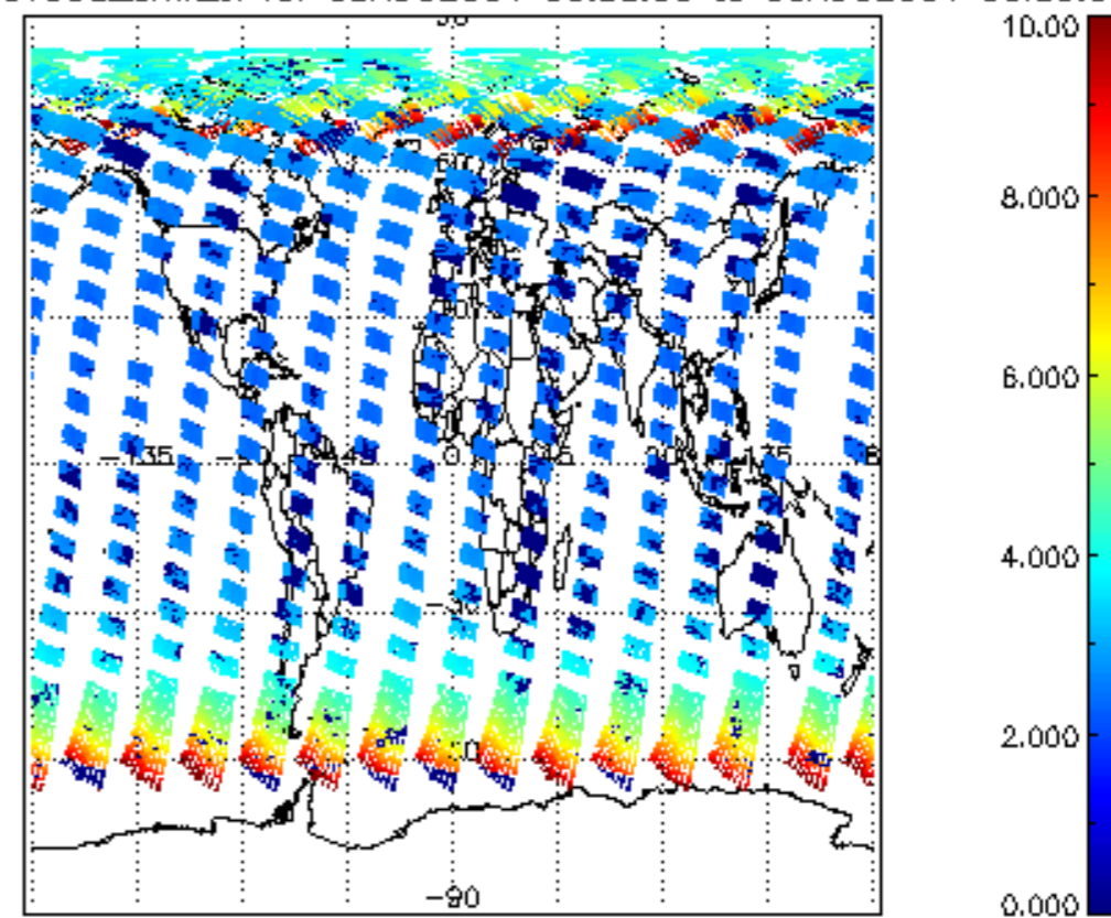
SCIOL2P_NADUV003_amf_cl for 05AUG2004 00:00:00 to 06AUG2004 00:00:00
