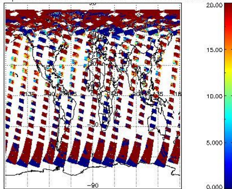
cL_opt_depth for 04AUG2004 00:00:00 to 05AUG2004 00:00:00
