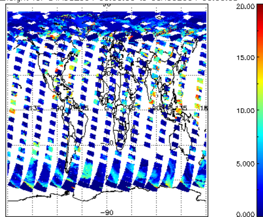
cL_top_height for 04AUG2004 00:00:00 to 05AUG2004 00:00:00
