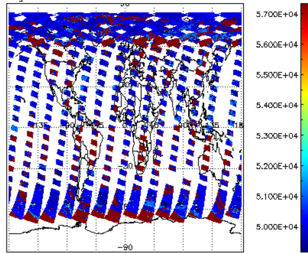
cloud_flags for 04AUG2004 00:00:00 to 05AUG2004 00:00:00
