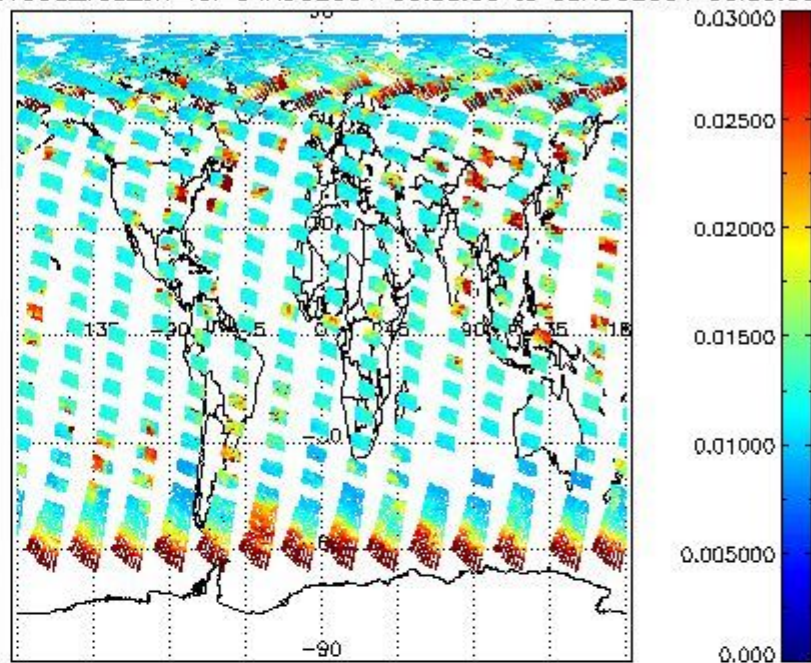
SCIOL2P_NADUV003_vcd_err for 04AUG2004 00:00:00 to 05AUG2004 00:00:00
