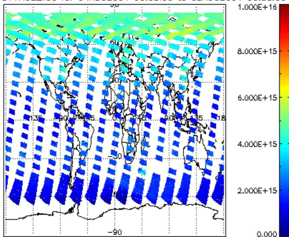
SCIOL2P_NADUV1NO2_vcd for 04AUG2004 00:00:00 to 05AUG2004 00:00:00
