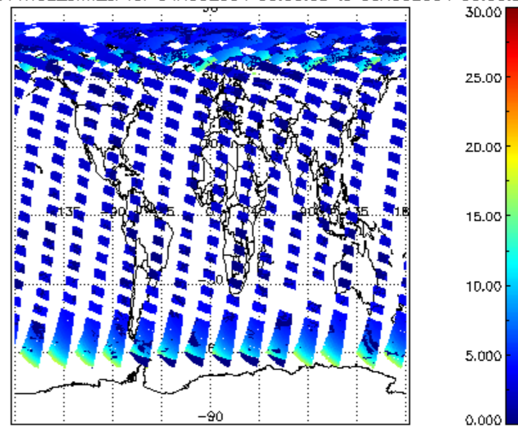
SCIOL2P_NADUV1NO2_amf_cl for 04AUG2004 00:00:00 to 05AUG2004 00:00:00
