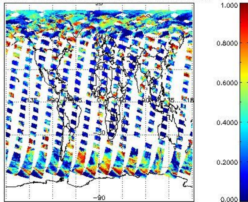
cL_frac for 04AUG2004 00:00:00 to 05AUG2004 00:00:00
