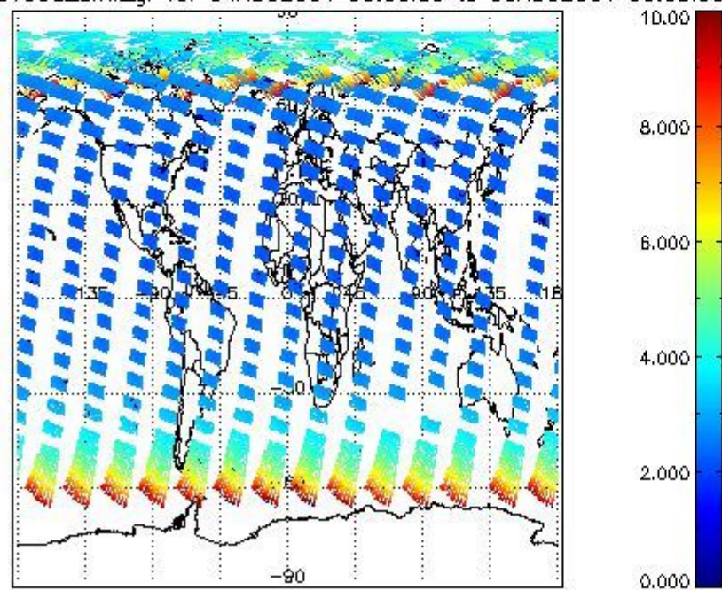
SCIOL2P_NADUV003_amf_gr for 04AUG2004 00:00:00 to 05AUG2004 00:00:00
