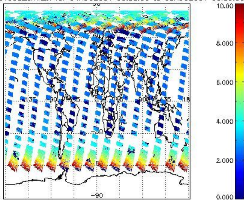
SCIOL2P_NADUV003_amf_cl for 04AUG2004 00:00:00 to 05AUG2004 00:00:00
