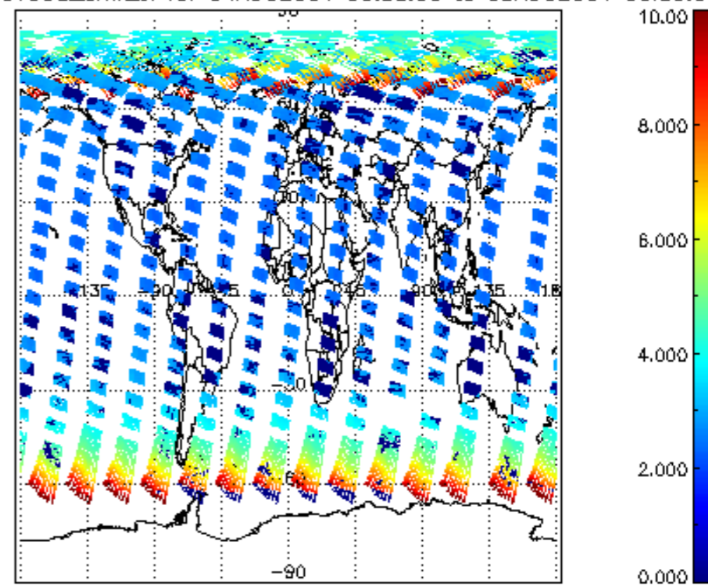
SCIOL2P_NADUV003_amf_cl for 04AUG2004 00:00:00 to 05AUG2004 00:00:00
