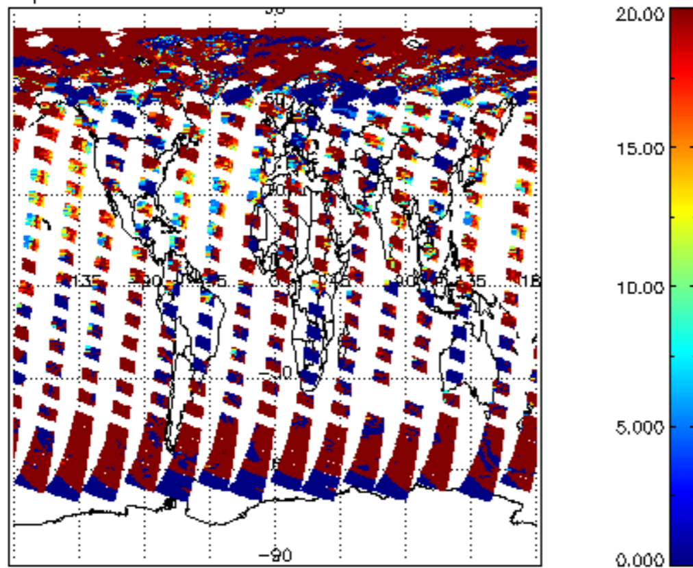
cL_opt_depth for 04AUG2004 00:00:00 to 05AUG2004 00:00:00
