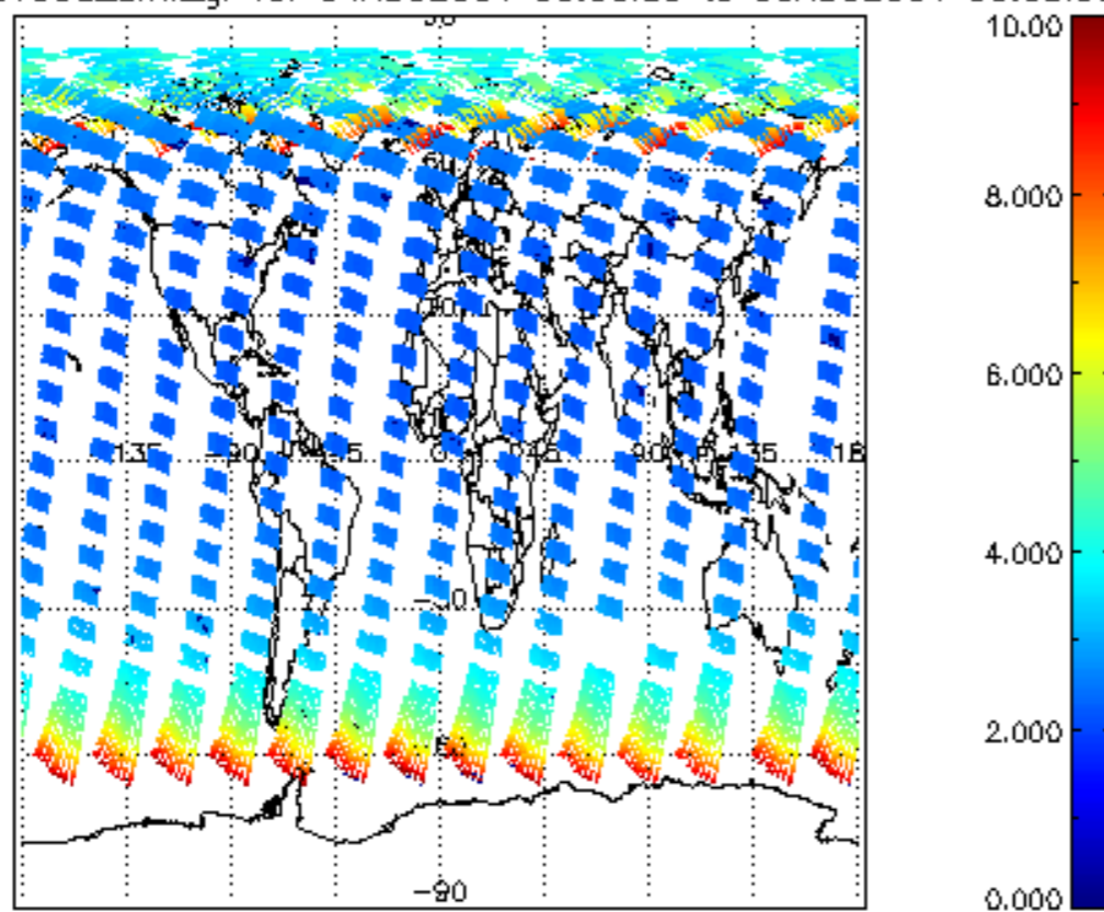
SCIOL2P_NADUV003_amf_gr for 04AUG2004 00:00:00 to 05AUG2004 00:00:00
