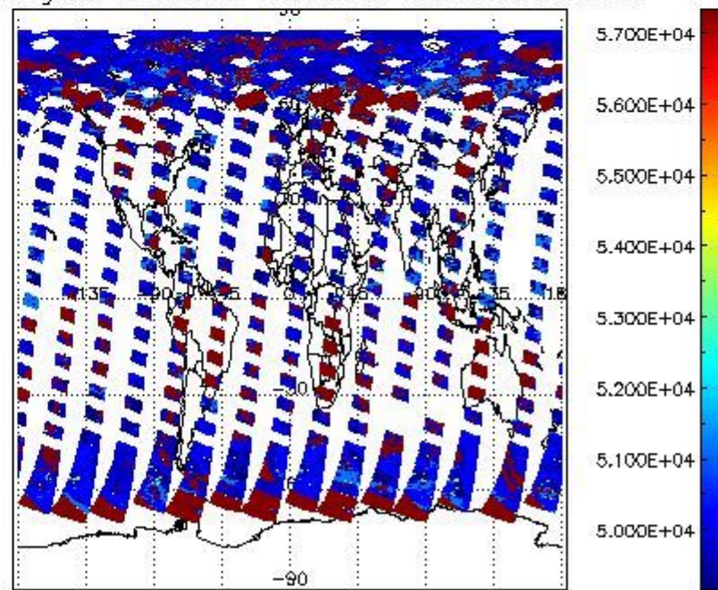
cloud_flags for 04AUG2004 00:00:00 to 05AUG2004 00:00:00
