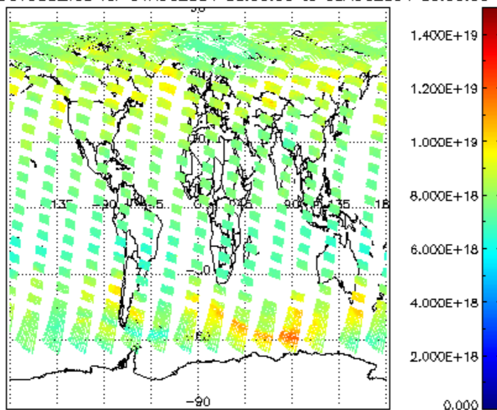
SCIOL2P_NADUV003_vcd for 04AUG2004 00:00:00 to 05AUG2004 00:00:00
