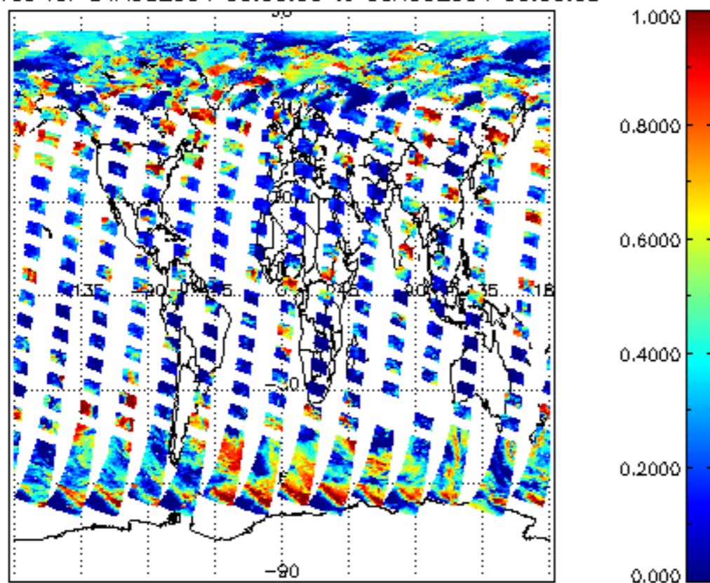
cL_frac for 04AUG2004 00:00:00 to 05AUG2004 00:00:00
