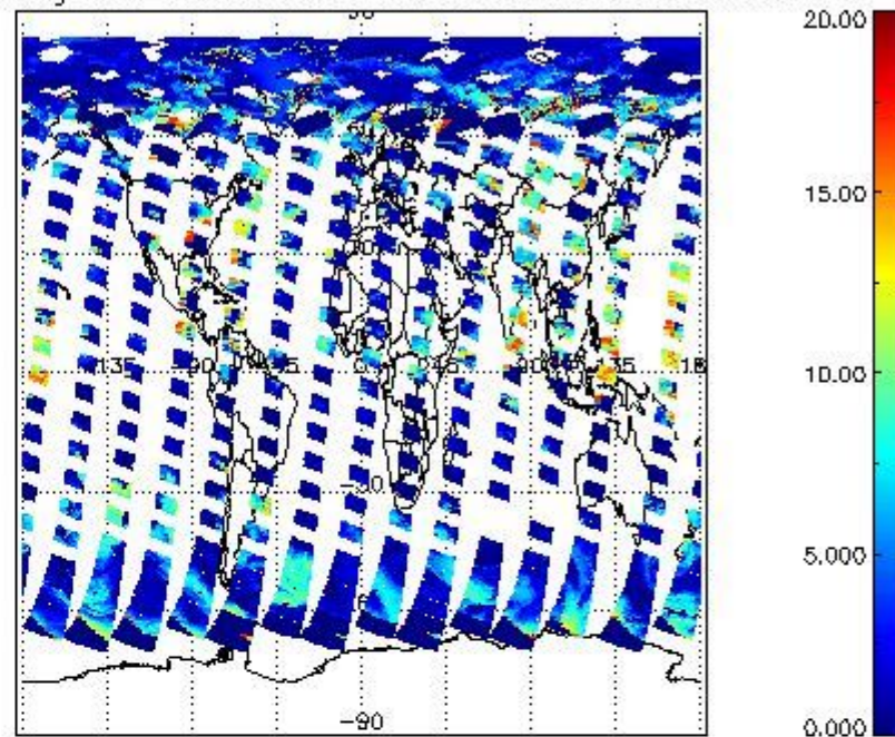
cL_top_height for 04AUG2004 00:00:00 to 05AUG2004 00:00:00
