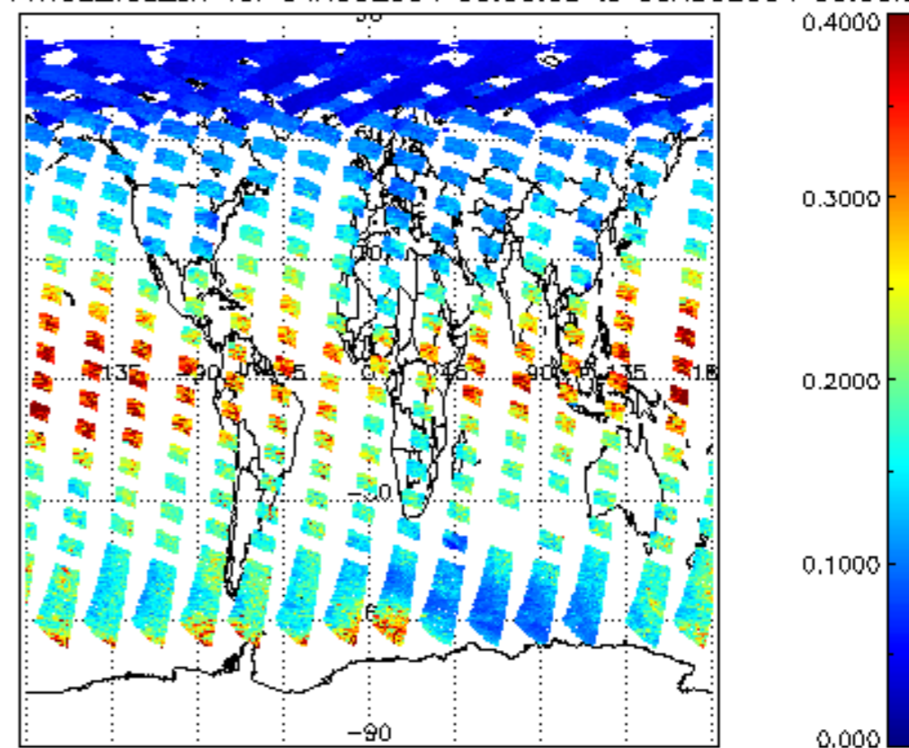
SCIOL2P_NADUV1NO2_vcd_err for 04AUG2004 00:00:00 to 05AUG2004 00:00:00
