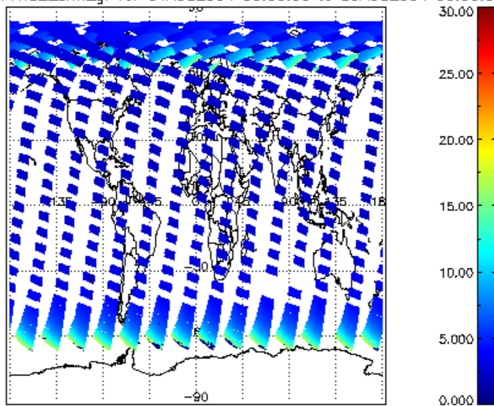
SCIOL2P_NADUV1NO2_amf_gr for 04AUG2004 00:00:00 to 05AUG2004 00:00:00
