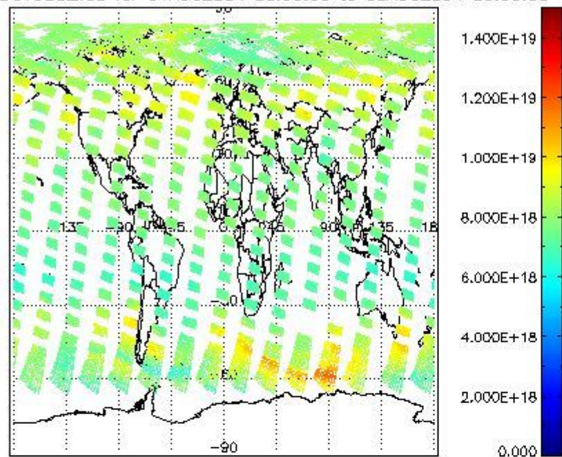
SCIOL2P_NADUV003_vcd for 04AUG2004 00:00:00 to 05AUG2004 00:00:00
