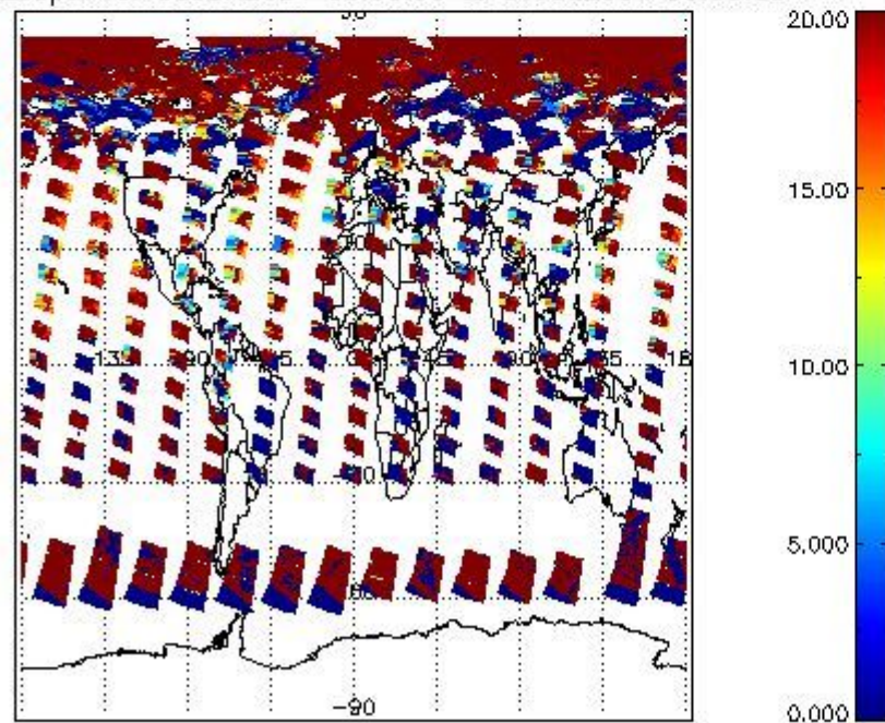
cL_opt_depth for 30JUN2004 00:00:00 to 01JUL2004 00:00:00
