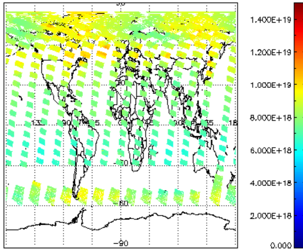
SCIOL2P_NADUV003_vcd for 30JUN2004 00:00:00 to 01JUL2004 00:00:00
