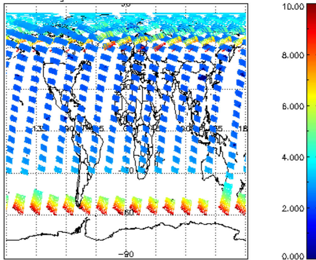
SCIOL2P_NADUV003_amf_gr for 30JUN2004 00:00:00 to 01JUL2004 00:00:00
