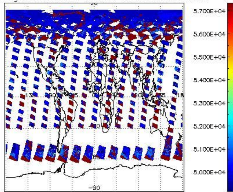
cloud_flags for 30JUN2004 00:00:00 to 01JUL2004 00:00:00
