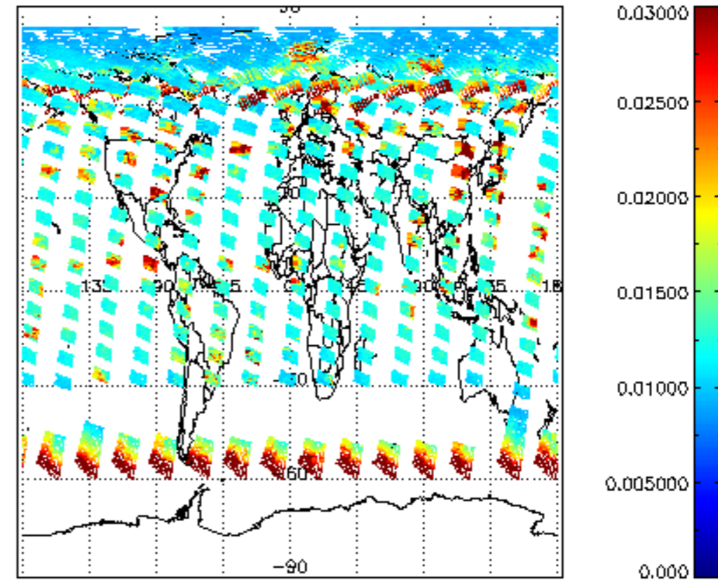
SCIOL2P_NADUV003_vcd_err for 30JUN2004 00:00:00 to 01JUL2004 00:00:00
