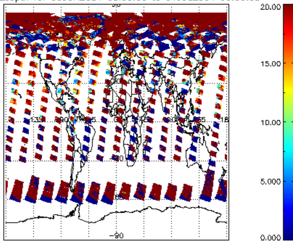
cl_lopt_depth for 30JUN2004 00:00:00 to 01JUL2004 00:00:00
