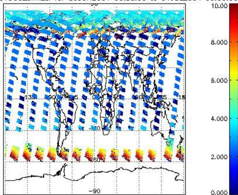
SCIOL2P_NADUV003_amf_cl for 30JUN2004 00:00:00 to 01JUL2004 00:00:00
