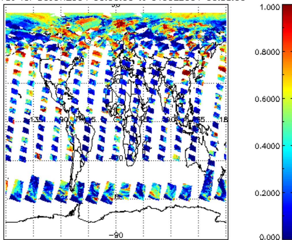
cl_frac for 30JUN2004 00:00:00 to 01JUL2004 00:00:00
