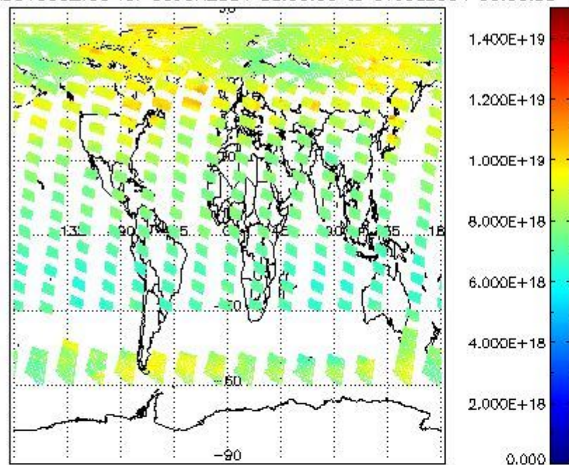
SCIOL2P_NADUV003_vcd for 30JUN2004 00:00:00 to 01JUL2004 00:00:00
