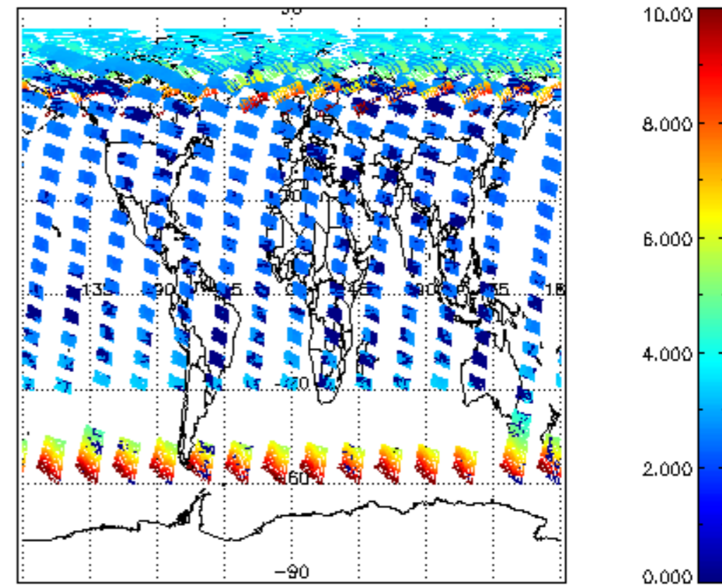
SCIOL2P_NADUV003_amf_cl for 30JUN2004 00:00:00 to 01JUL2004 00:00:00
