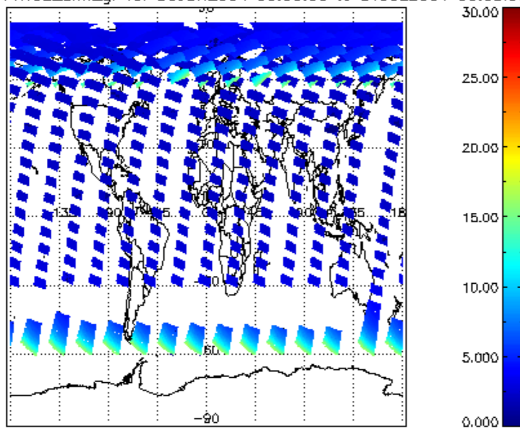
SCIOL2P_NADUV1NO2_amf_gr for 30JUN2004 00:00:00 to 01JUL2004 00:00:00
