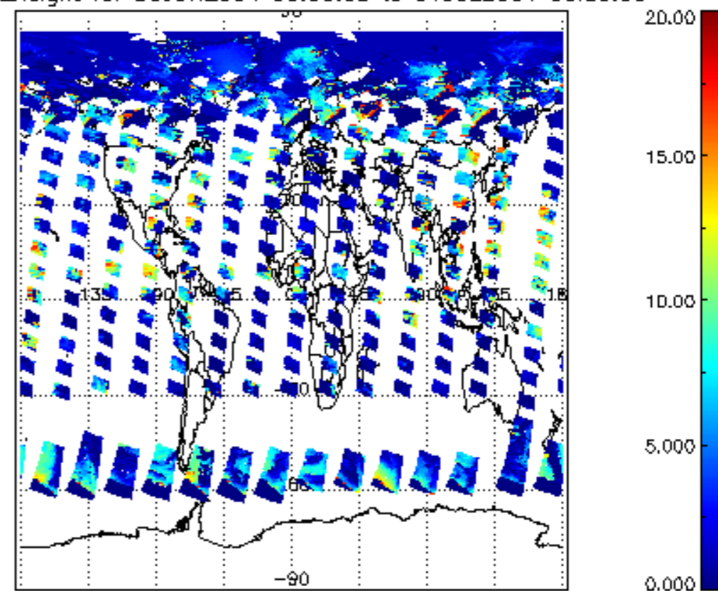
cl_top_height for 30JUN2004 00:00:00 to 01JUL2004 00:00:00
