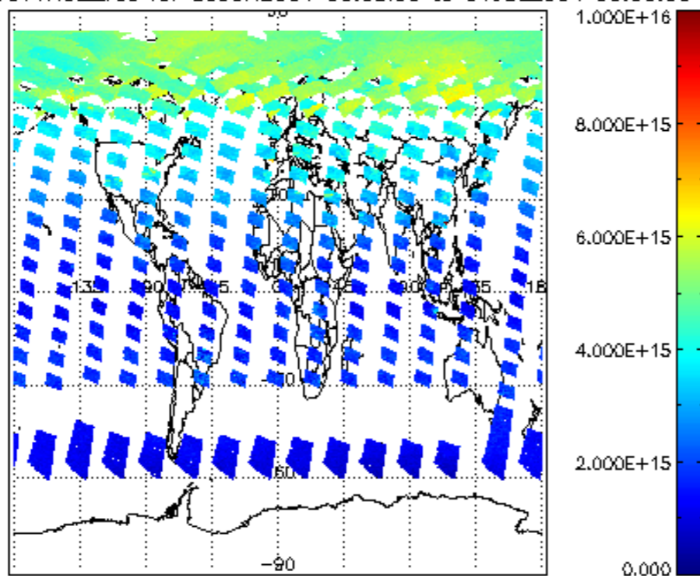
SCIOL2P_NADUV1NO2_vcd for 30JUN2004 00:00:00 to 01JUL2004 00:00:00
