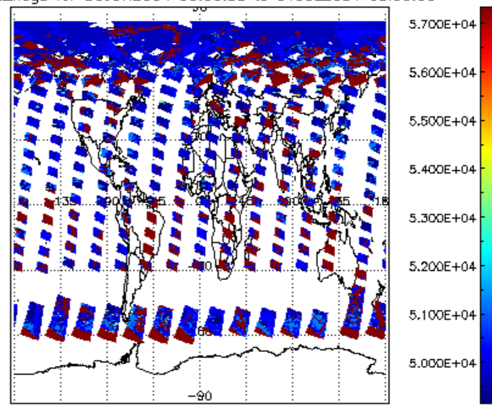
cloud_flags for 30JUN2004 00:00:00 to 01JUL2004 00:00:00
