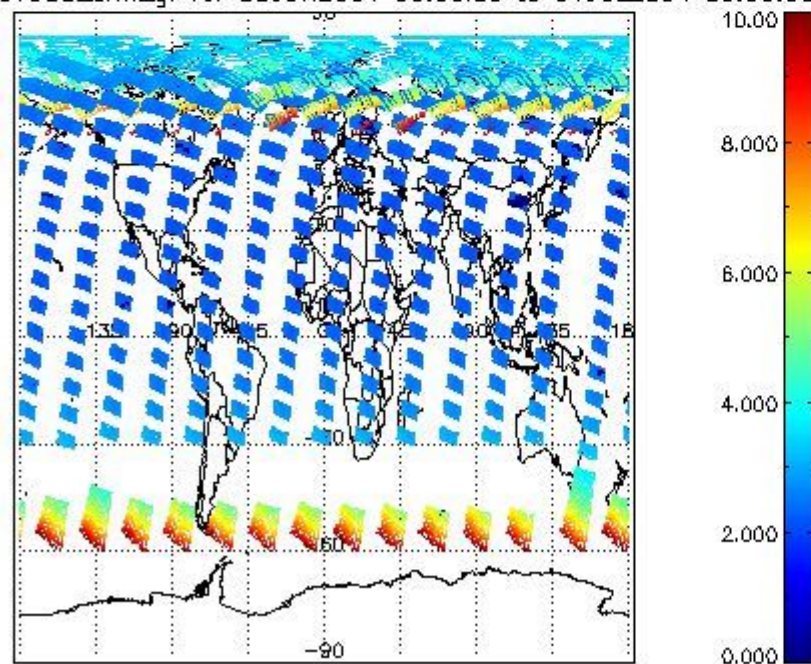
SCIOL2P_NADUV003_amf_gr for 30JUN2004 00:00:00 to 01JUL2004 00:00:00
