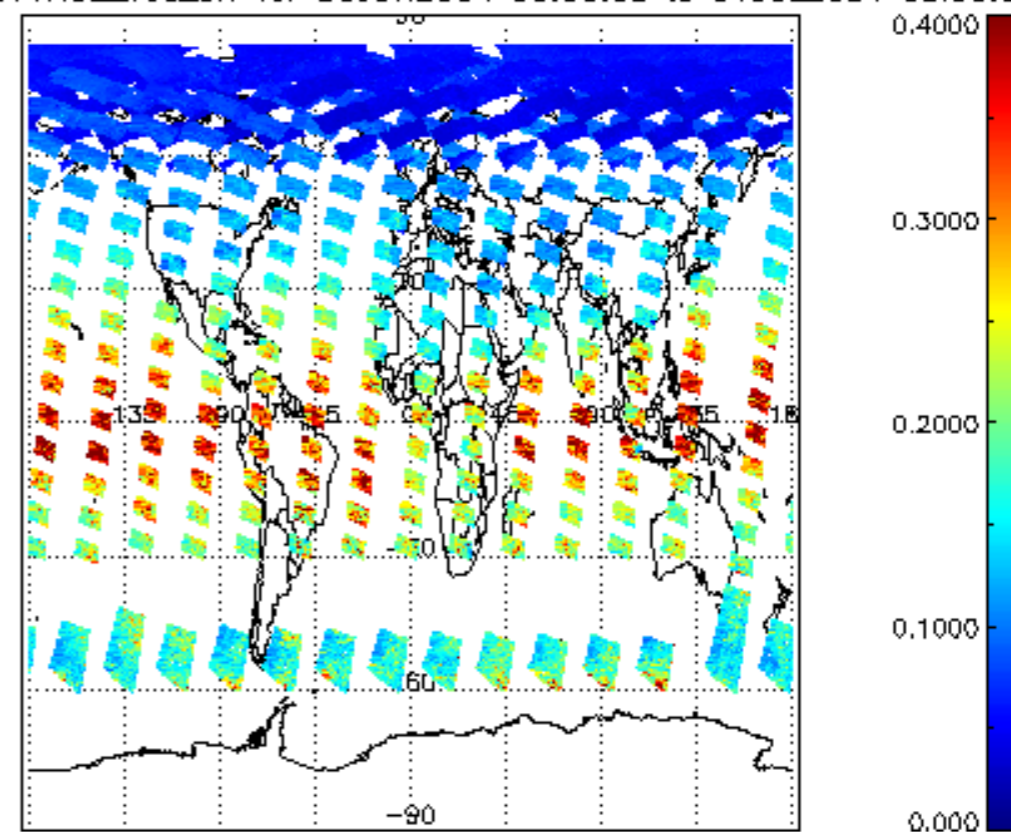
ICIOL2P_NADUV1NO2_vcd_err for 30JUN2004 00:00:00 to 01JUL2004 00:00:00
