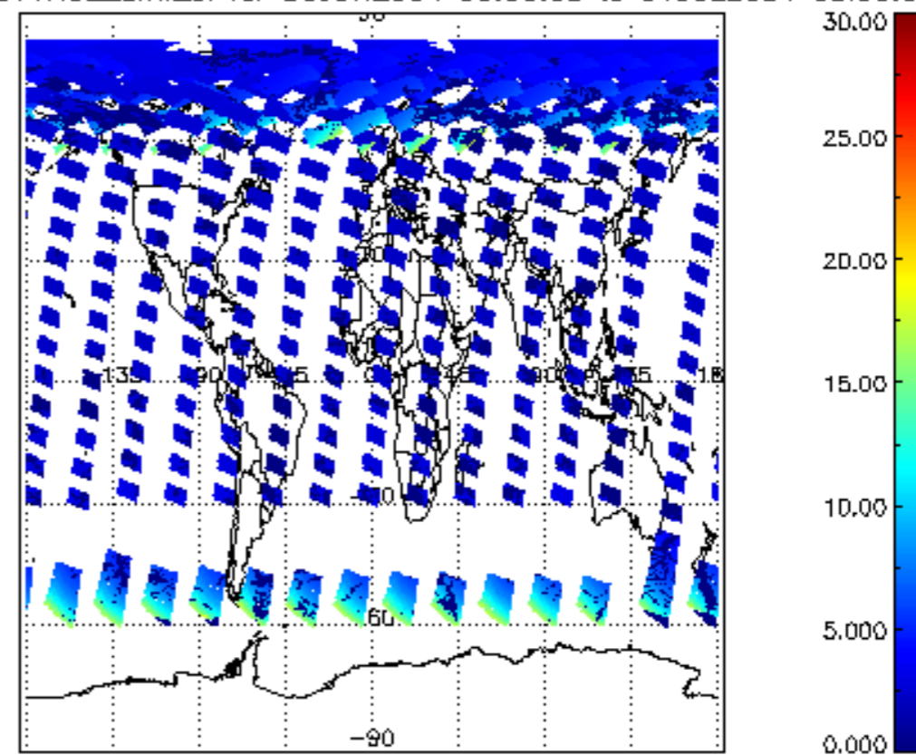
ICIOL2P_NADUV1NO2_amf_cl for 30JUN2004 00:00:00 to 01JUL2004 00:00:00
