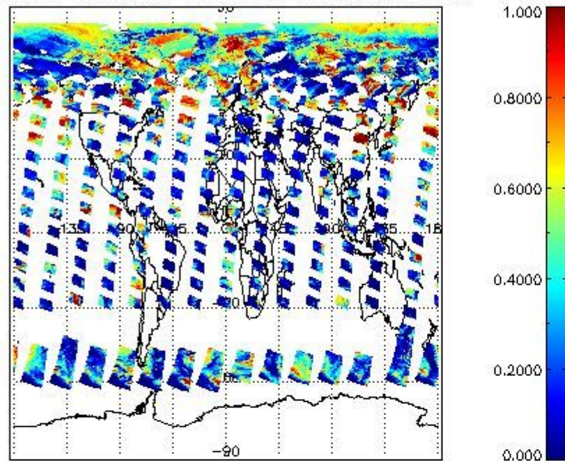
cL_frac for 30JUN2004 00:00:00 to 01JUL2004 00:00:00
