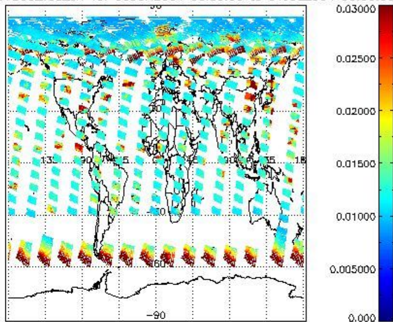
SCIOL2P_NADUV003_vcd_err for 30JUN2004 00:00:00 to 01JUL2004 00:00:00
