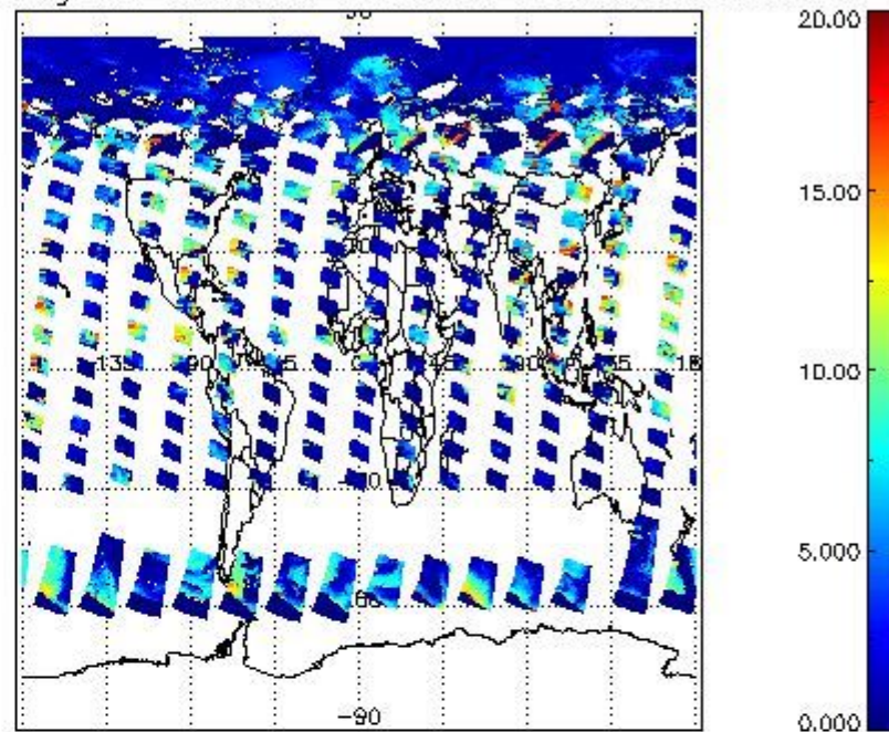
cL_top_height for 30JUN2004 00:00:00 to 01JUL2004 00:00:00
