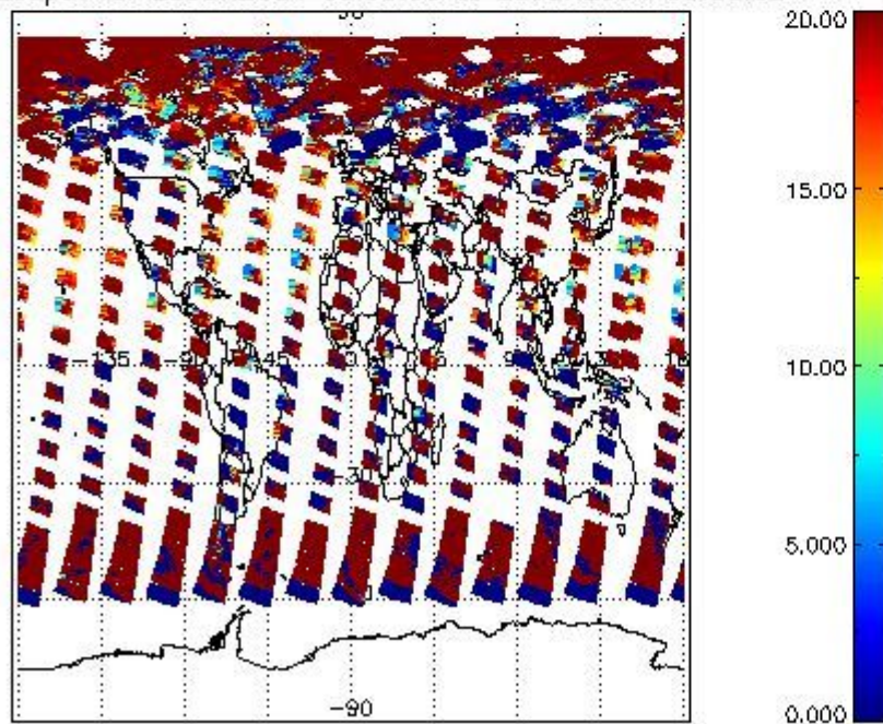
cL_opt_depth for 22JUN2004 00:00:00 to 23JUN2004 00:00:00
