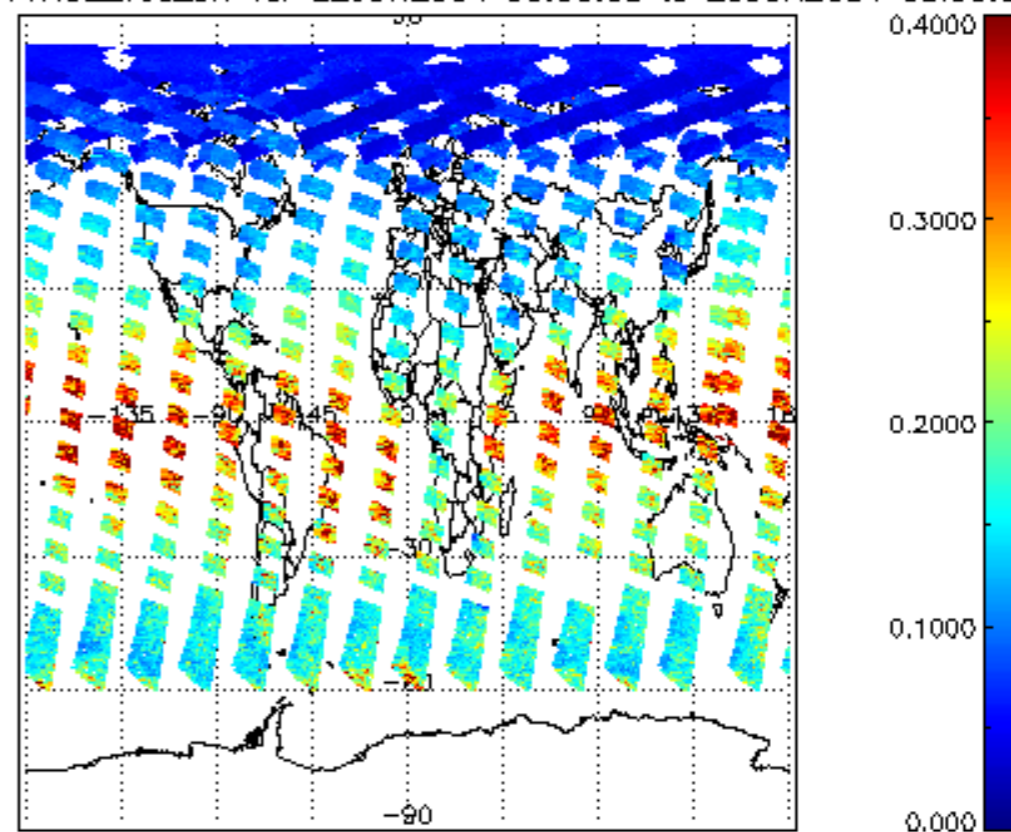
iCIOL2P_NADUV1NO2_vcd_err for 22JUN2004 00:00:00 to 23JUN2004 00:00:00
