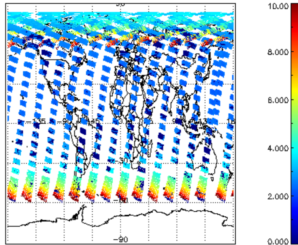
SCIOL2P_NADUV003_amf_cl for 22JUN2004 00:00:00 to 23JUN2004 00:00:00
