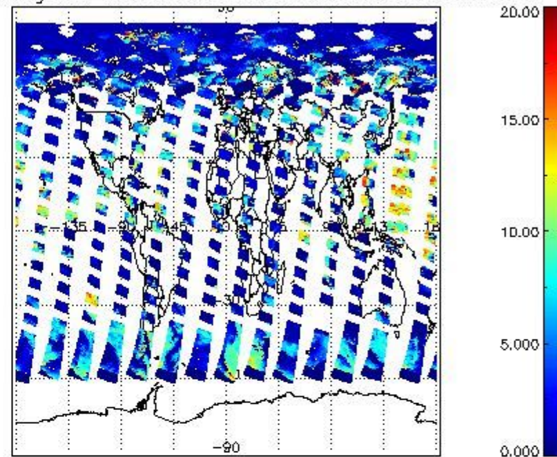
cL_top_height for 22JUN2004 00:00:00 to 23JUN2004 00:00:00
