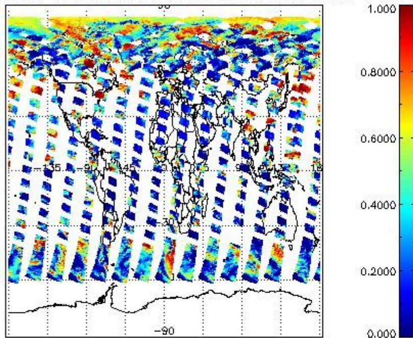
cL_frac for 22JUN2004 00:00:00 to 23JUN2004 00:00:00
