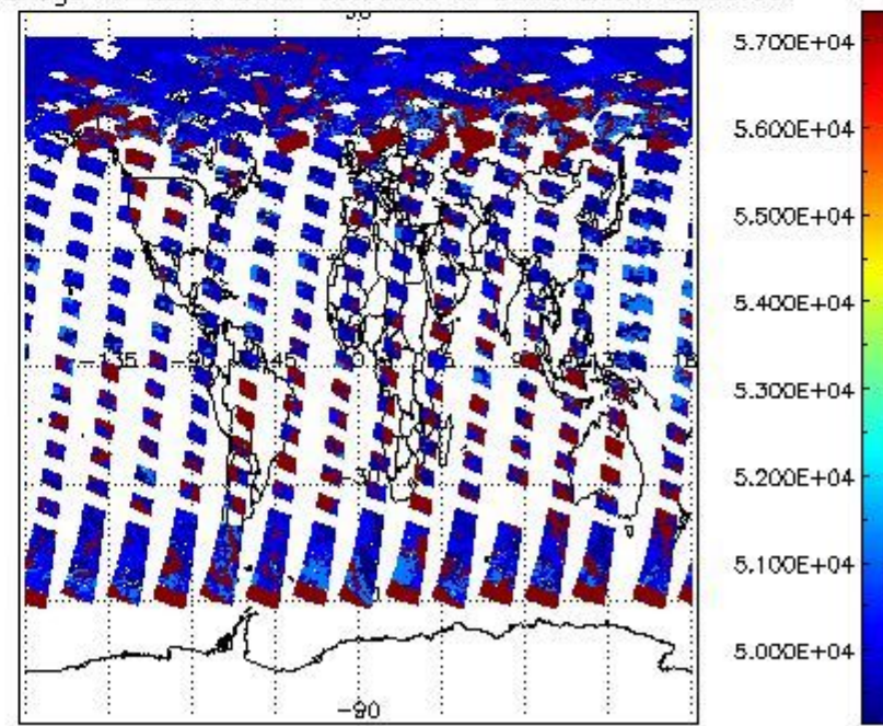
cloud_flags for 22JUN2004 00:00:00 to 23JUN2004 00:00:00
