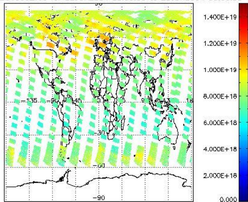
SCIOL2P_NADUV003_vcd for 22JUN2004 00:00:00 to 23JUN2004 00:00:00
