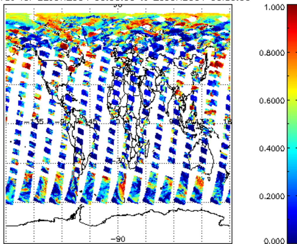
cl_frac for 22JUN2004 00:00:00 to 23JUN2004 00:00:00
