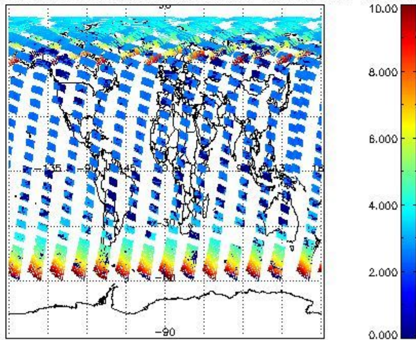
SCIOL2P_NADUV003_amf_cl for 22JUN2004 00:00:00 to 23JUN2004 00:00:00
