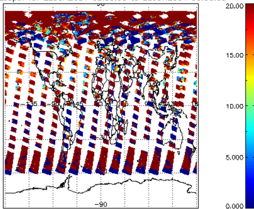
cl_opt_depth for 22JUN2004 00:00:00 to 23JUN2004 00:00:00
