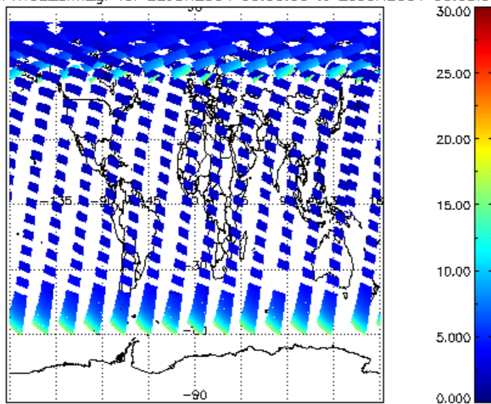
iCIOL2P_NADUV1NO2_amf_gr for 22JUN2004 00:00:00 to 23JUN2004 00:00:00
