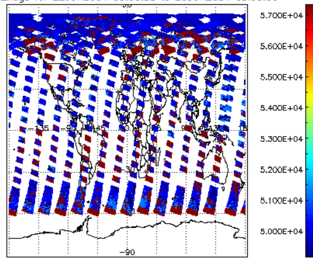
cloud_flags for 22JUN2004 00:00:00 to 23JUN2004 00:00:00
