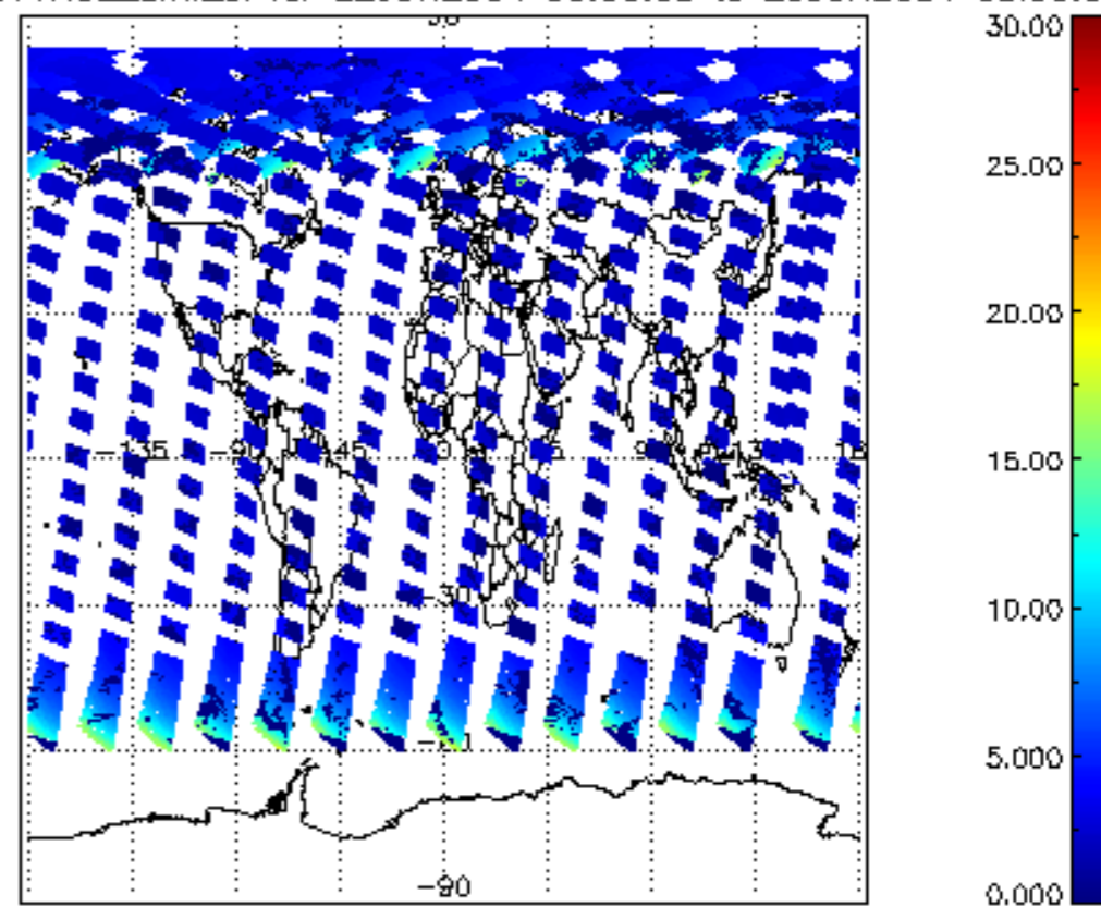
iCIOL2P_NADUV1NO2_amf_cl for 22JUN2004 00:00:00 to 23JUN2004 00:00:00
