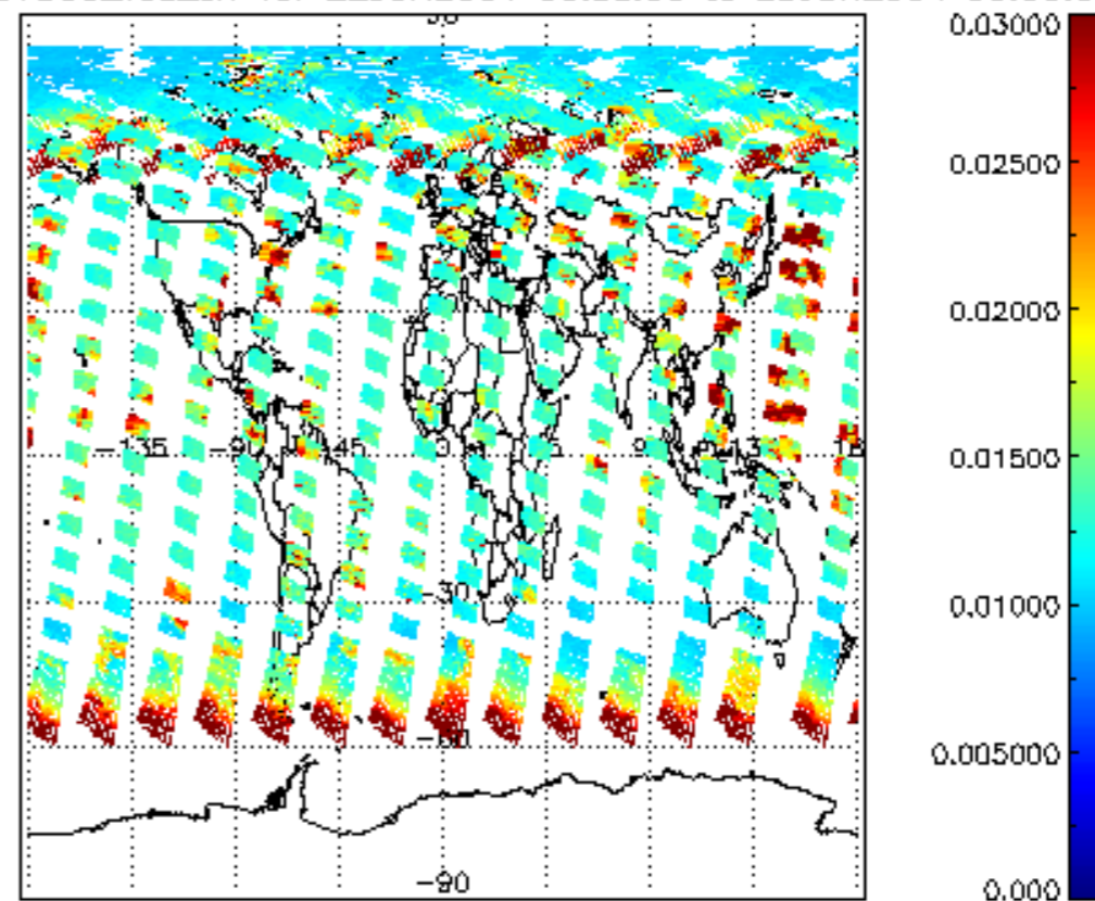
SCIOL2P_NADUV003_vcd_err for 22JUN2004 00:00:00 to 23JUN2004 00:00:00
