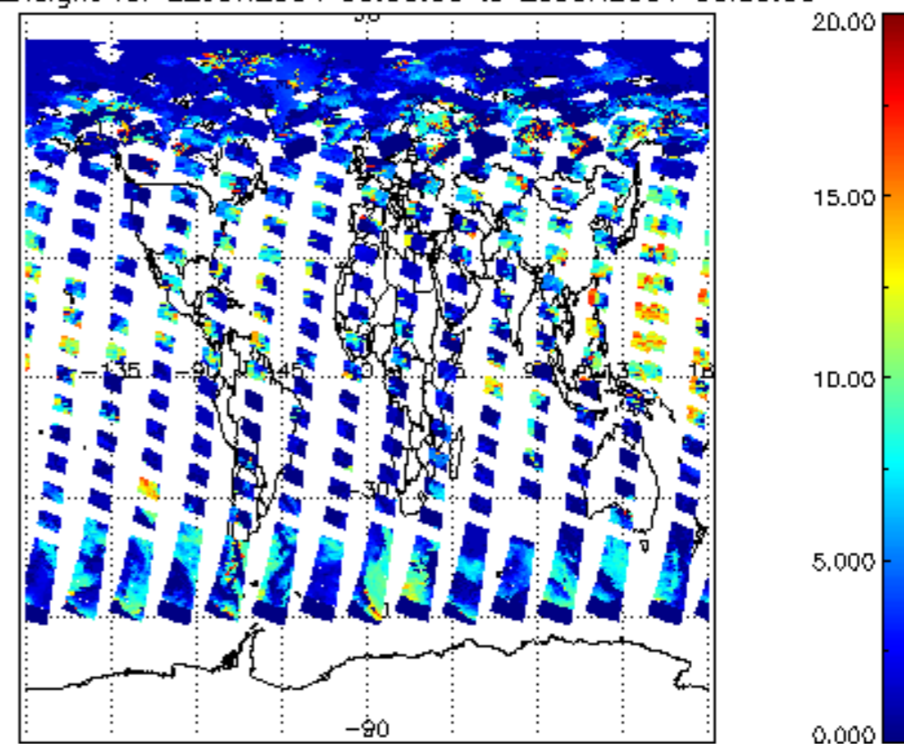
cl_top_height for 22JUN2004 00:00:00 to 23JUN2004 00:00:00
