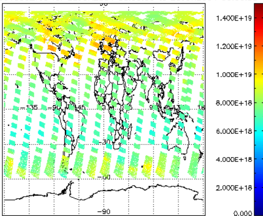
SCIOL2P_NADUV003_vcd for 22JUN2004 00:00:00 to 23JUN2004 00:00:00
