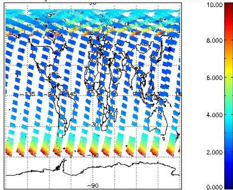
SCIOL2P_NADUV003_amf_gr for 22JUN2004 00:00:00 to 23JUN2004 00:00:00
