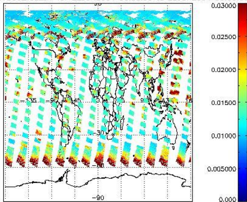
SCIOL2P_NADUV003_vcd_err for 22JUN2004 00:00:00 to 23JUN2004 00:00:00
