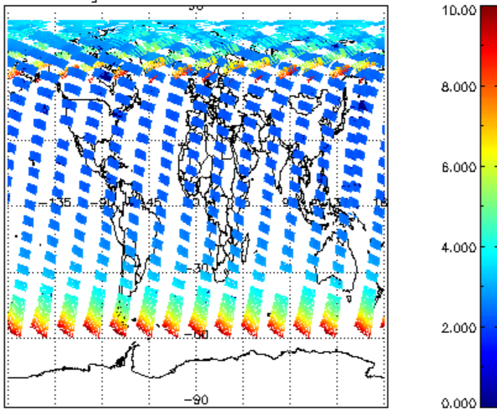
SCIOL2P_NADUV003_amf_gr for 22JUN2004 00:00:00 to 23JUN2004 00:00:00
