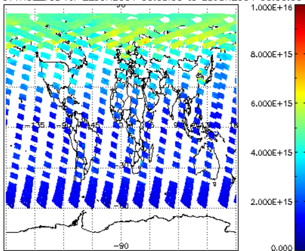
SCIOL2P_NADUV1NO2_vcd for 22JUN2004 00:00:00 to 23JUN2004 00:00:00
