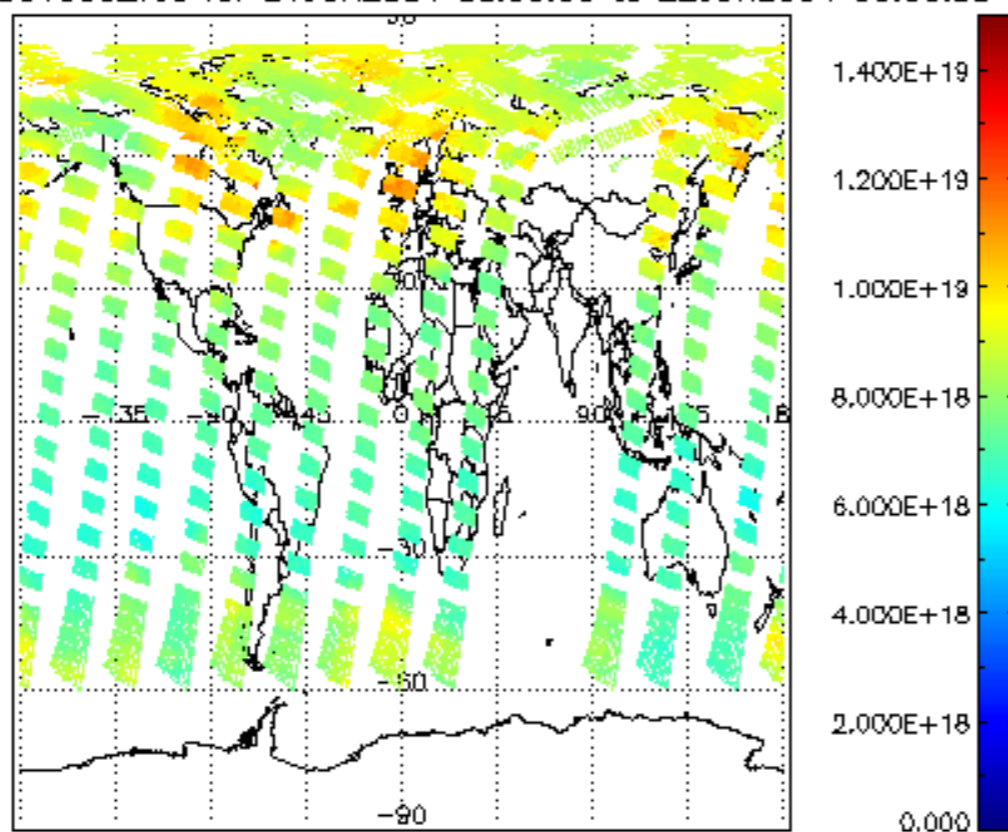
SCIOL2P_NADUV003_vcd for 21JUN2004 00:00:00 to 22JUN2004 00:00:00
