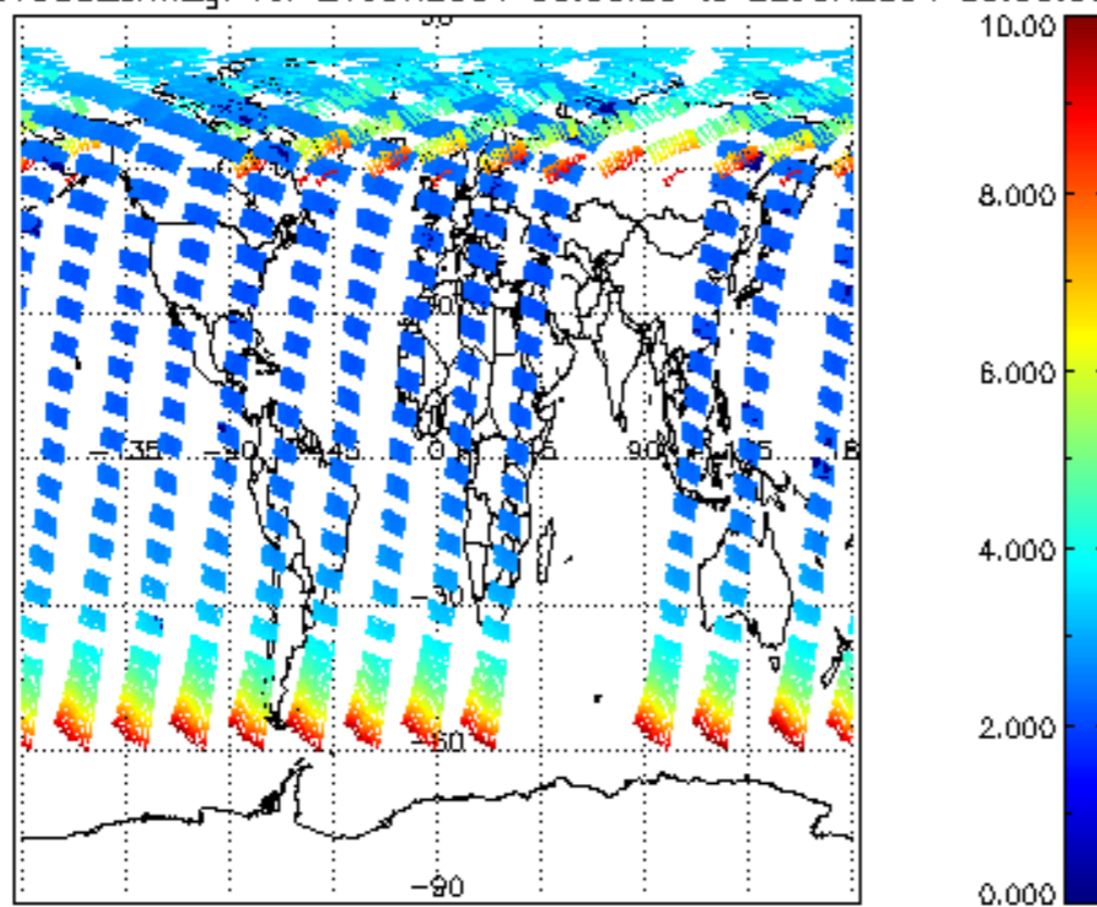
SCIOL2P_NADUV003_amf_gr for 21JUN2004 00:00:00 to 22JUN2004 00:00:00
