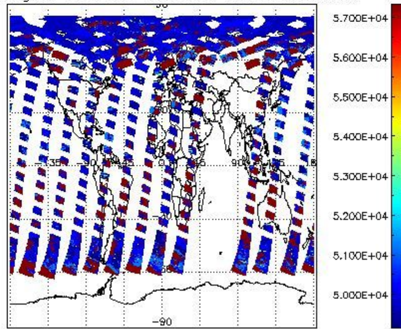
cloud_flags for 21JUN2004 00:00:00 to 22JUN2004 00:00:00
