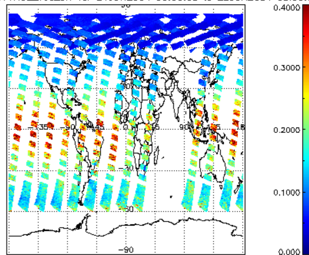
SCIOL2P_NADUV1NO2_vcd for 21JUN2004 00:00:00 to 22JUN2004 00:00:00 iCIOL2P_NADUV1NO2_vcd_err for 21JUN2004 00:00:00 to 22JUN2004 00:00:00
