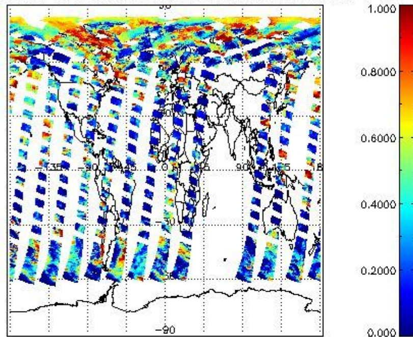
cL_frac for 21JUN2004 00:00:00 to 22JUN2004 00:00:00
