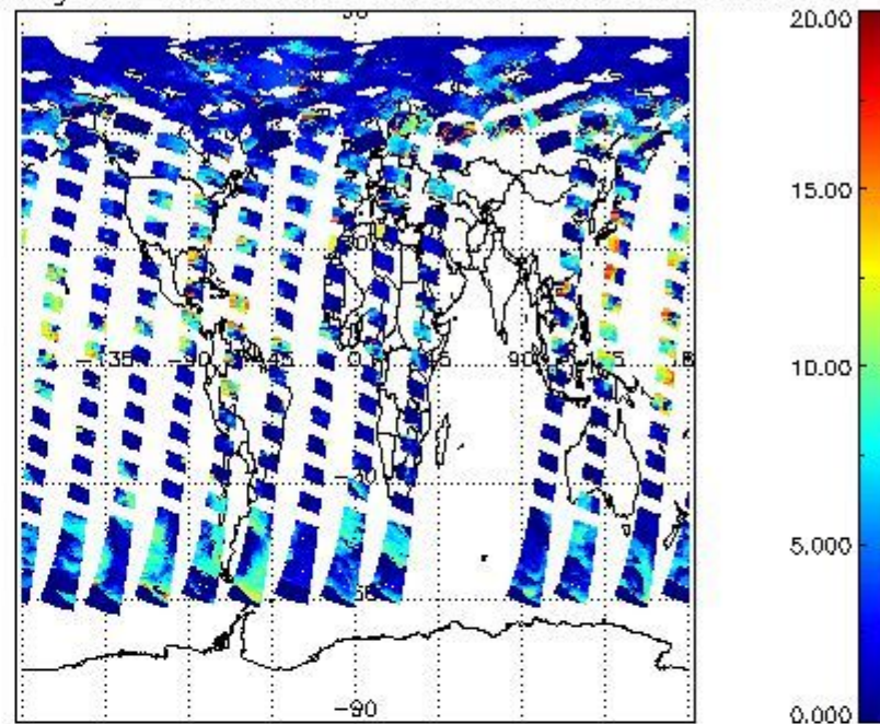
cL_top_height for 21JUN2004 00:00:00 to 22JUN2004 00:00:00
