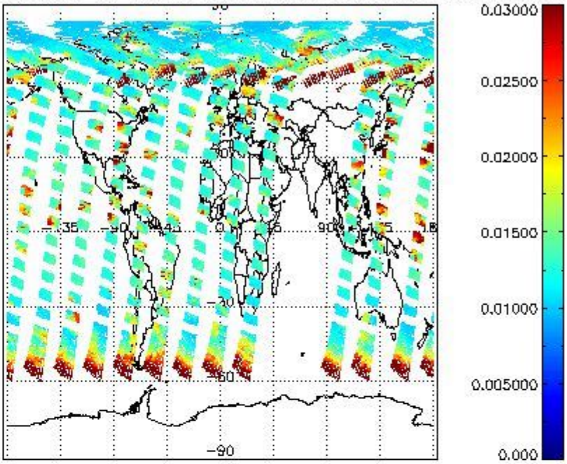
SCIOL2P_NADUV003_vcd_err for 21JUN2004 00:00:00 to 22JUN2004 00:00:00
