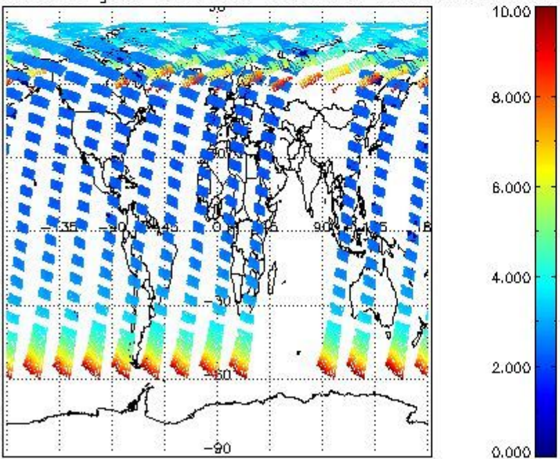
SCIOL2P_NADUV003_amf_gr for 21JUN2004 00:00:00 to 22JUN2004 00:00:00
