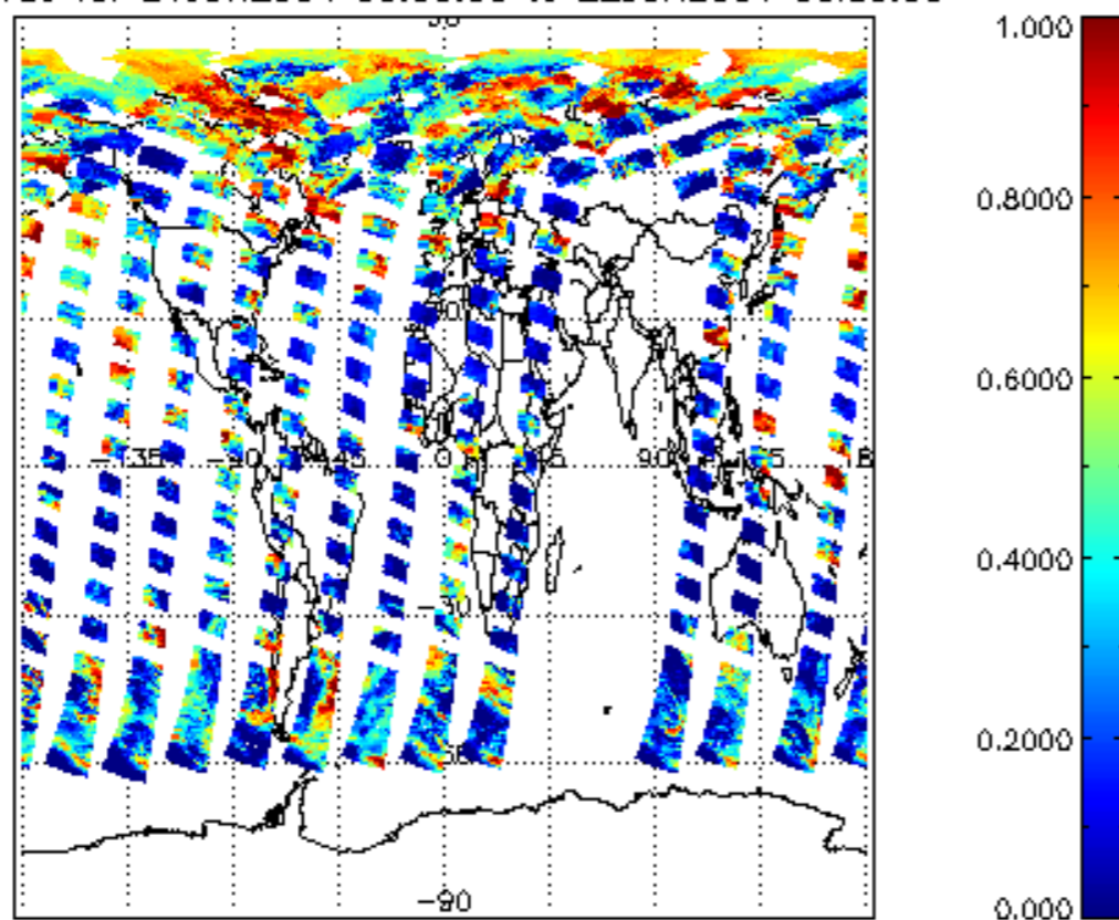
cl_frac for 21JUN2004 00:00:00 to 22JUN2004 00:00:00
