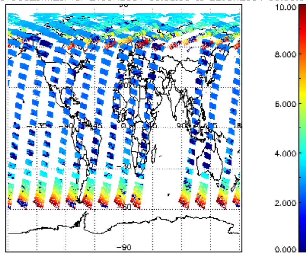
SCIOL2P_NADUV003_amf_cl for 21JUN2004 00:00:00 to 22JUN2004 00:00:00
