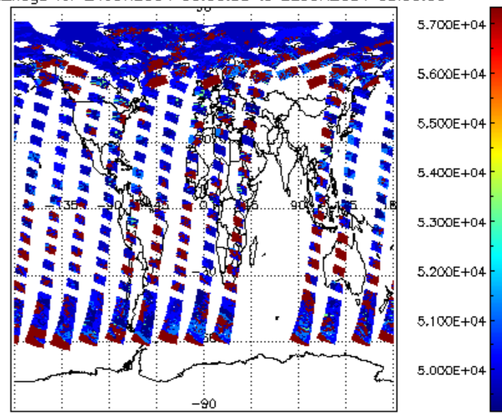
cloud_flags for 21JUN2004 00:00:00 to 22JUN2004 00:00:00
