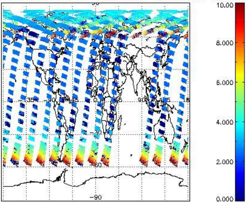
SCIOL2P_NADUV003_amf_cl for 21JUN2004 00:00:00 to 22JUN2004 00:00:00
