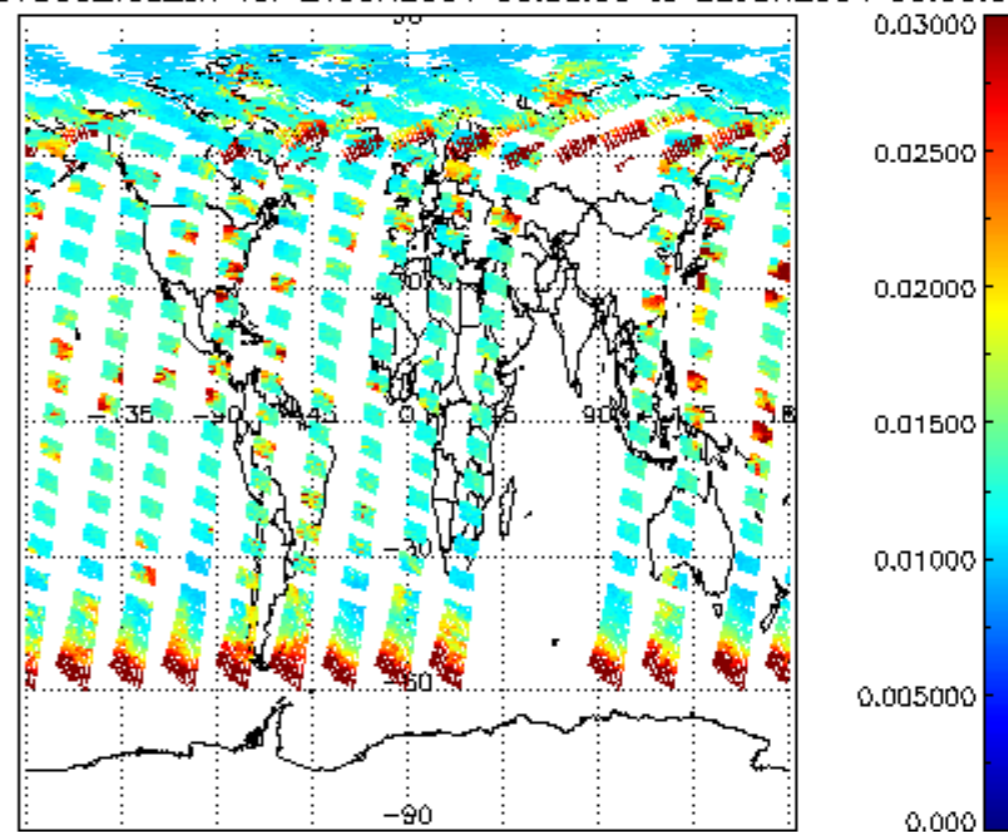
SCIOL2P_NADUV003_vcd_err for 21JUN2004 00:00:00 to 22JUN2004 00:00:00
