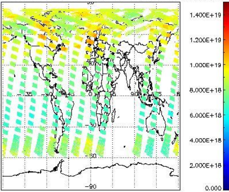
SCIOL2P_NADUV003_vcd for 21JUN2004 00:00:00 to 22JUN2004 00:00:00
