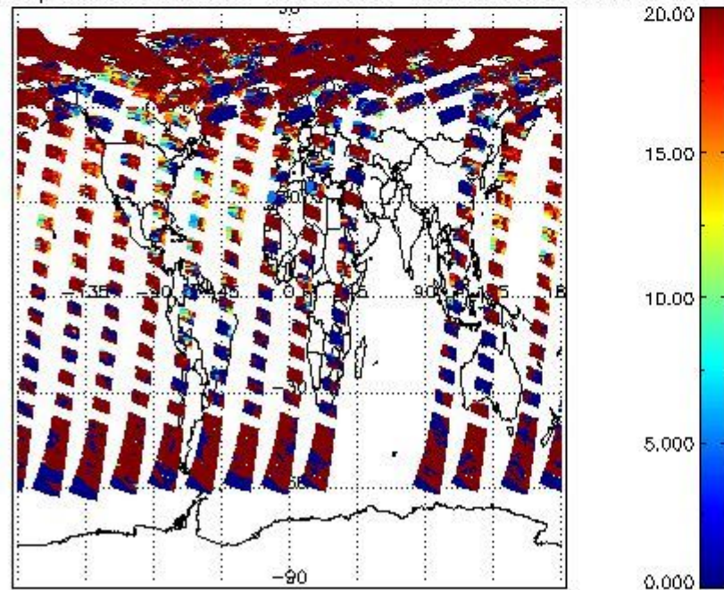
cL_opt_depth for 21JUN2004 00:00:00 to 22JUN2004 00:00:00
