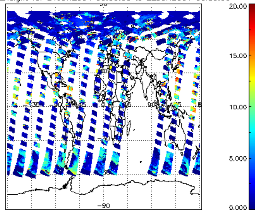
cl_top_height for 21JUN2004 00:00:00 to 22JUN2004 00:00:00
