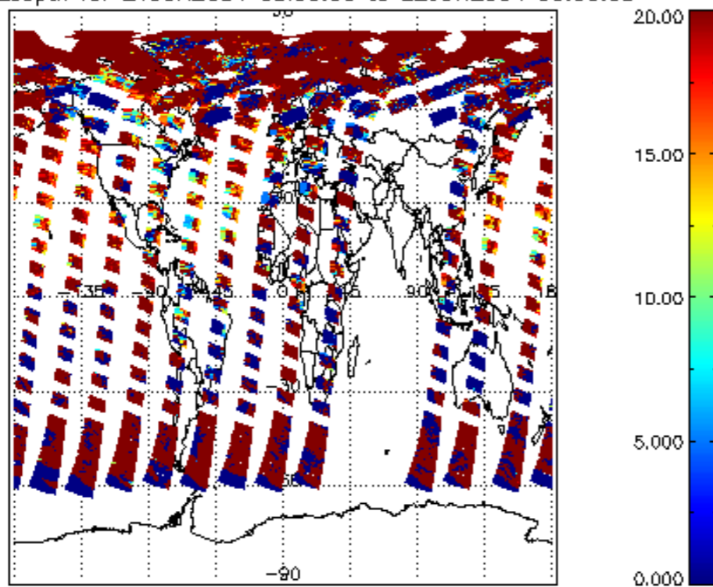
cl_opt_depth for 21JUN2004 00:00:00 to 22JUN2004 00:00:00
