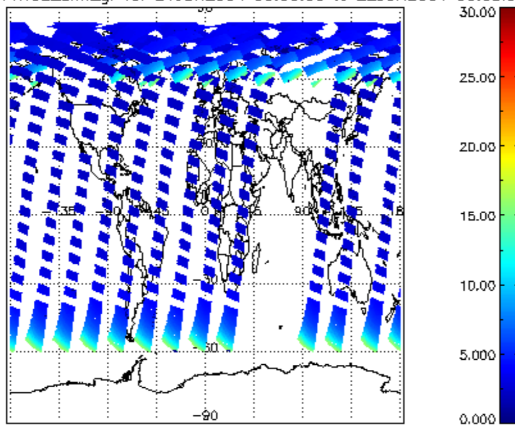
iCIOL2P_NADUV1NO2_amf_gr for 21JUN2004 00:00:00 to 22JUN2004 00:00:00 iCIOL2P_NADUV1NO2_amf_cl for 21JUN2004 00:00:00 to 22JUN2004 00:00:00
