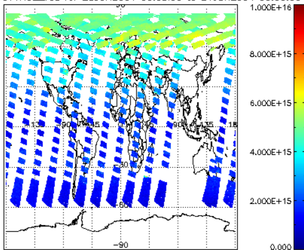
SCIOL2P_NADUV1NO2_vcd for 20JUN2004 00:00:00 to 21JUN2004 00:00:00
