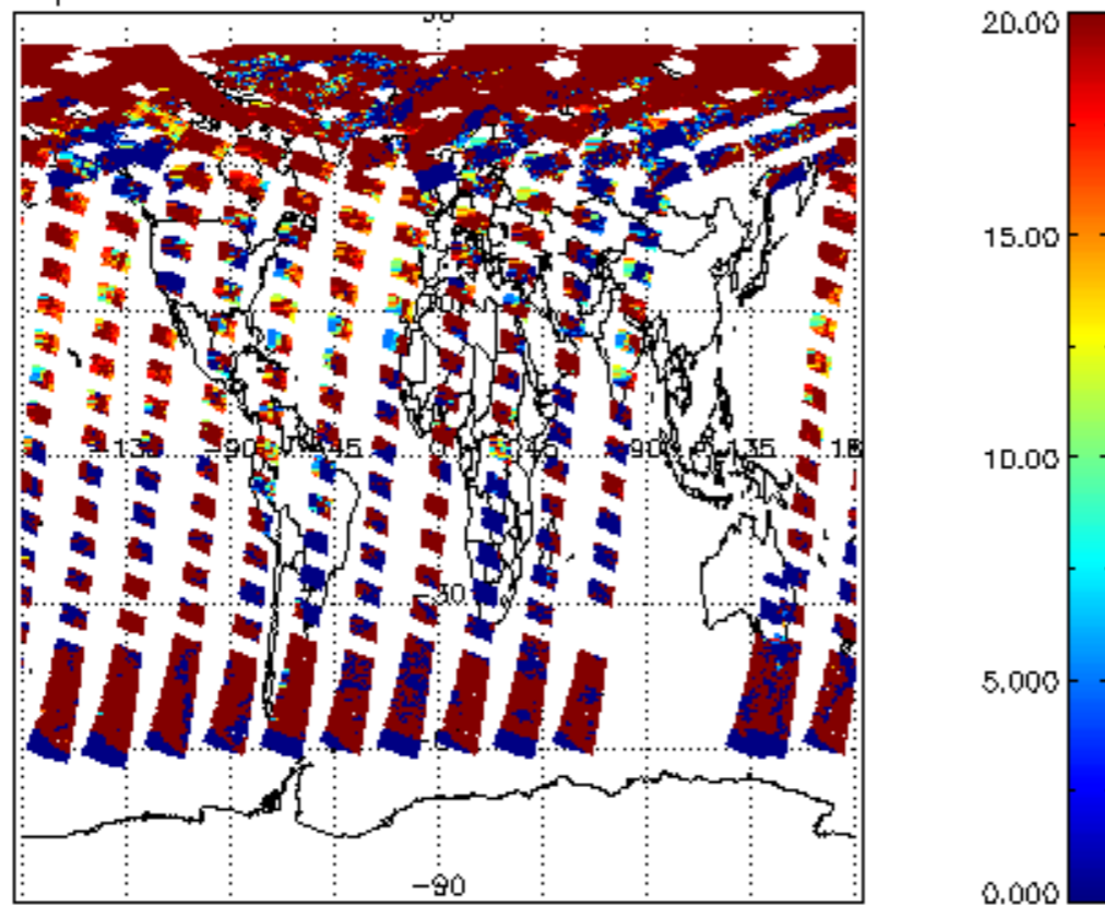
cl_opt_depth for 20JUN2004 00:00:00 to 21JUN2004 00:00:00
