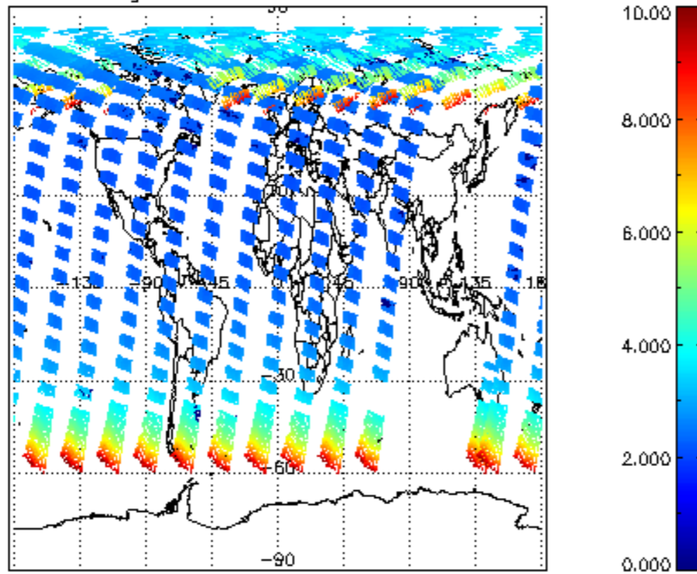
SCIOL2P_NADUV003_amf_gr for 20JUN2004 00:00:00 to 21JUN2004 00:00:00
