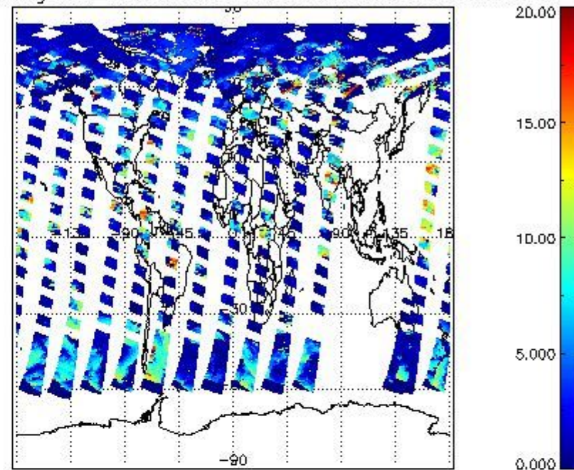
cL_top_height for 20JUN2004 00:00:00 to 21JUN2004 00:00:00
