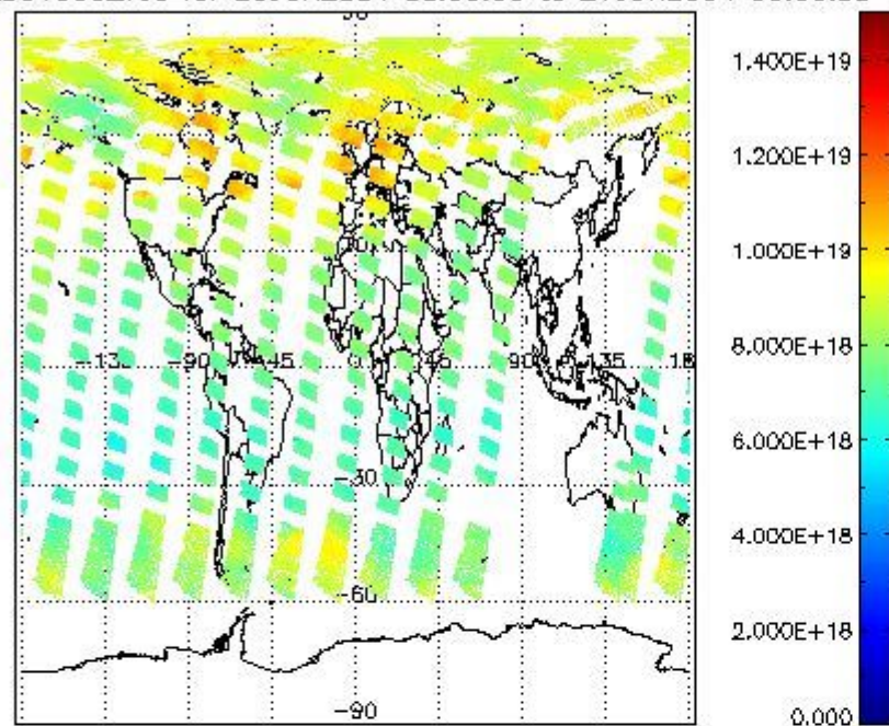
SCIOL2P_NADUV003_vcd for 20JUN2004 00:00:00 to 21JUN2004 00:00:00
