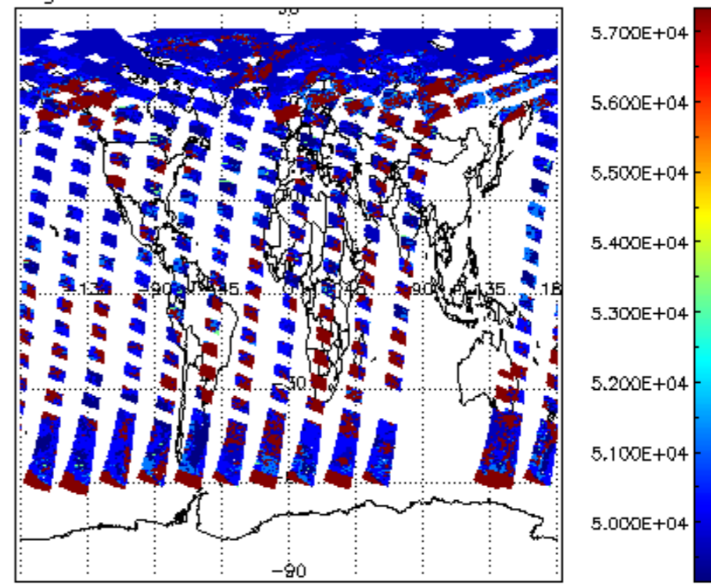
cloud_flags for 20JUN2004 00:00:00 to 21JUN2004 00:00:00
