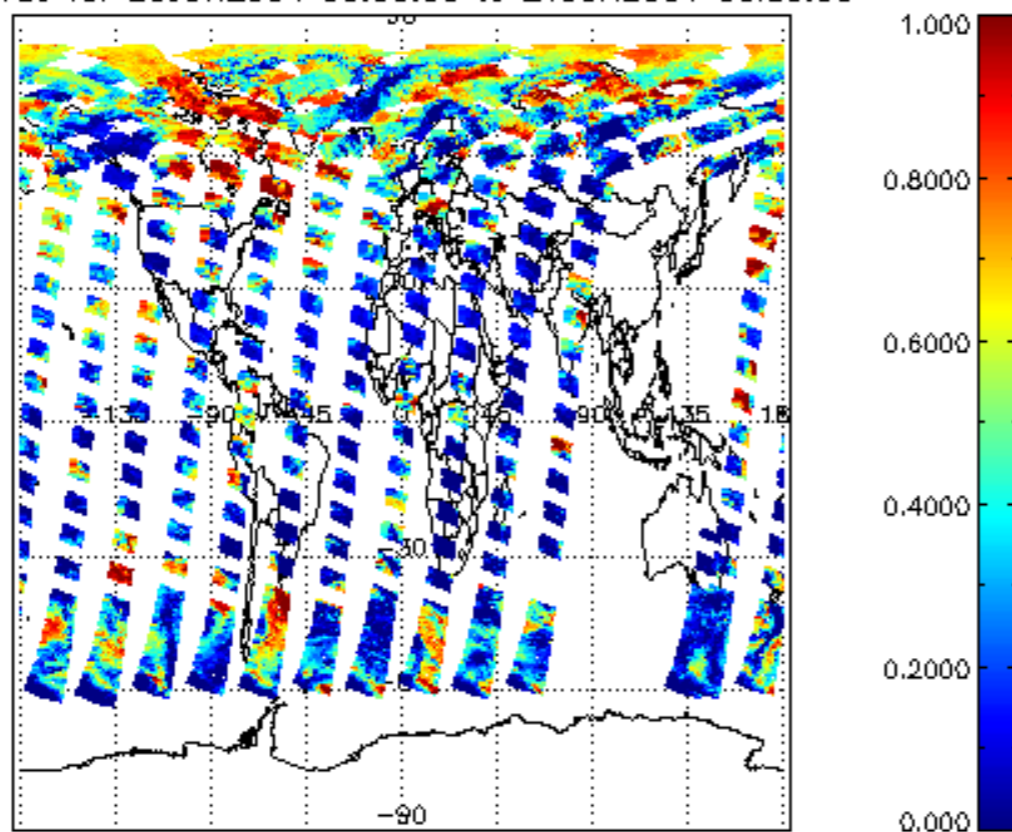
cl_frac for 20JUN2004 00:00:00 to 21JUN2004 00:00:00
