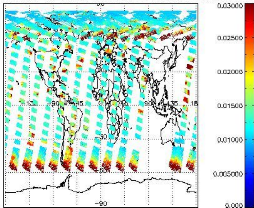
SCIOL2P_NADUV003_vcd_err for 20JUN2004 00:00:00 to 21JUN2004 00:00:00
