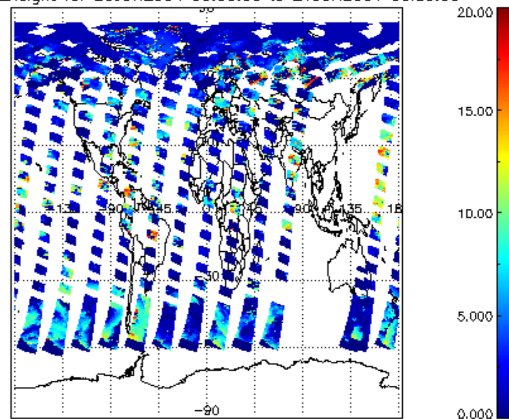
cl_top_height for 20JUN2004 00:00:00 to 21JUN2004 00:00:00
