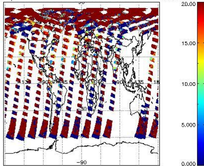
cL_opt_depth for 20JUN2004 00:00:00 to 21JUN2004 00:00:00
