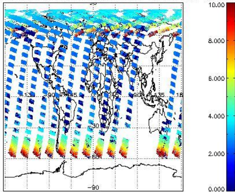
SCIOL2P_NADUV003_amf_cl for 20JUN2004 00:00:00 to 21JUN2004 00:00:00
