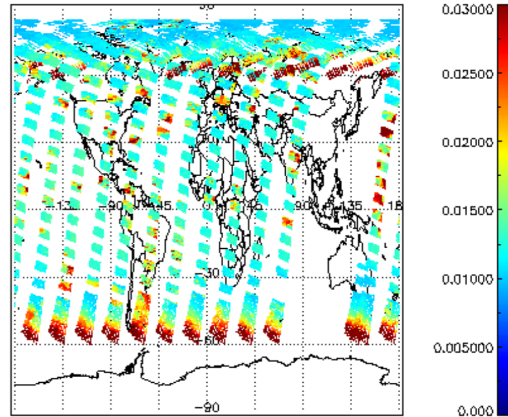
SCIOL2P_NADUV003_vcd_err for 20JUN2004 00:00:00 to 21JUN2004 00:00:00
