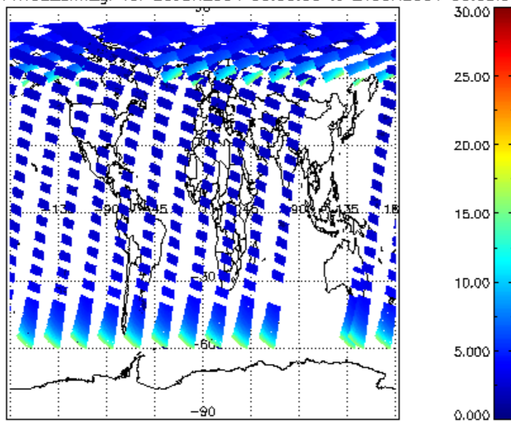
iCIOL2P_NADUV1NO2_amf_gr for 20JUN2004 00:00:00 to 21JUN2004 00:00:00
