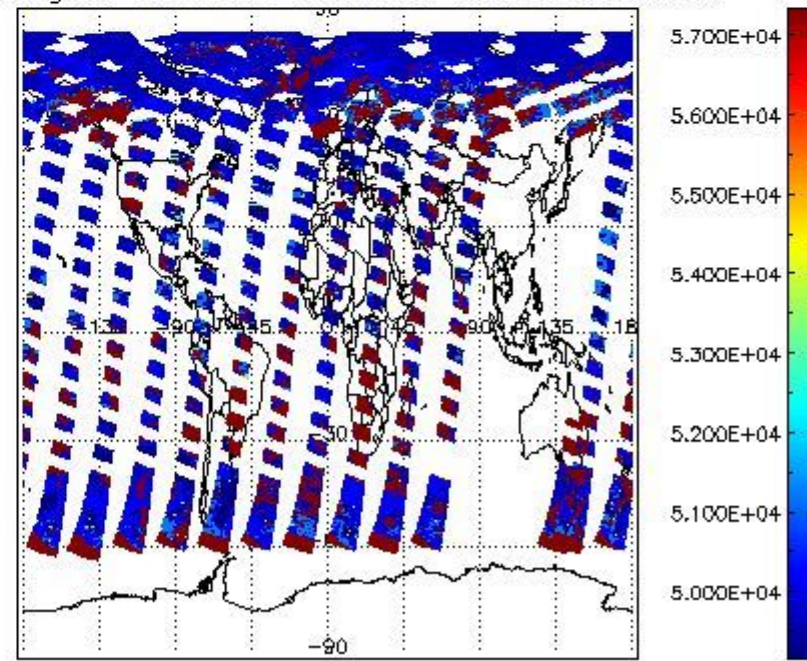
cloud_flags for 20JUN2004 00:00:00 to 21JUN2004 00:00:00
