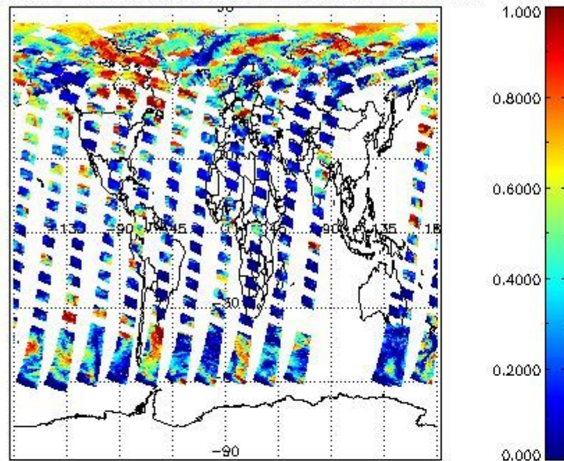
cL_frac for 20JUN2004 00:00:00 to 21JUN2004 00:00:00
