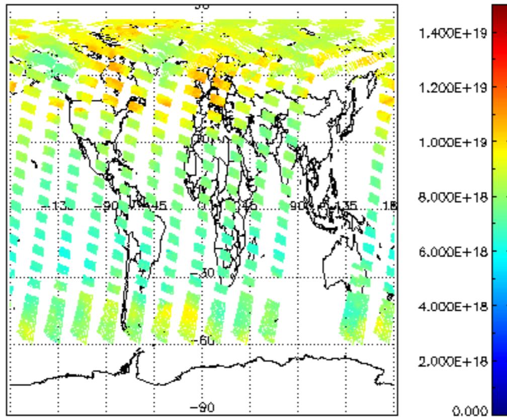
SCIOL2P_NADUV003_vcd for 20JUN2004 00:00:00 to 21JUN2004 00:00:00
