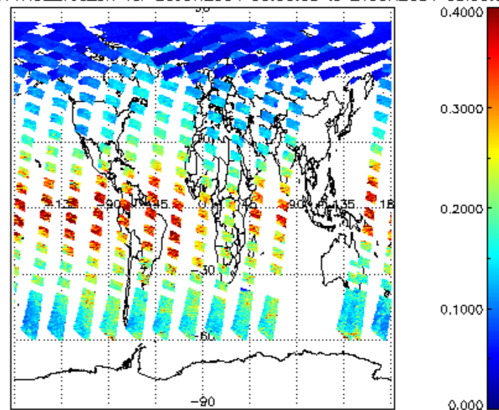
iCIOL2P_NADUV1NO2_vcd_err for 20JUN2004 00:00:00 to 21JUN2004 00:00:00
