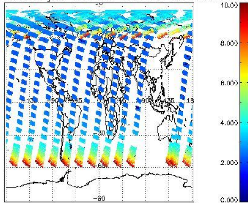
SCIOL2P_NADUV003_amf_gr for 20JUN2004 00:00:00 to 21JUN2004 00:00:00
