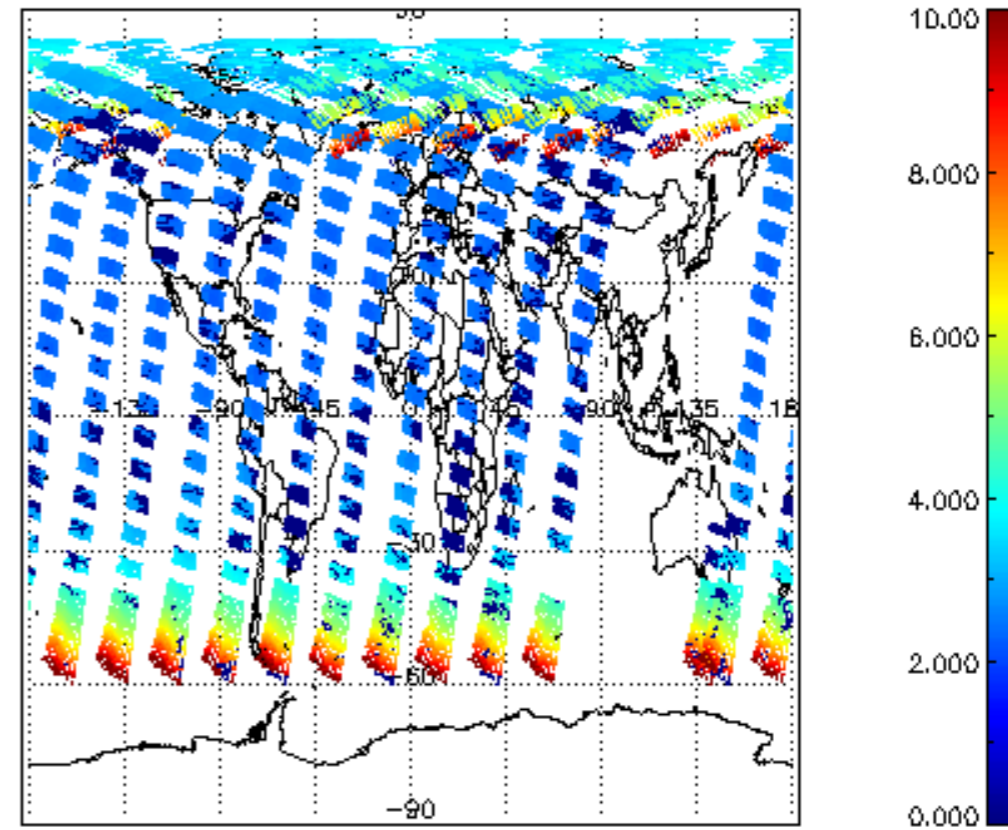
SCIOL2P_NADUV003_amf_cl for 20JUN2004 00:00:00 to 21JUN2004 00:00:00
