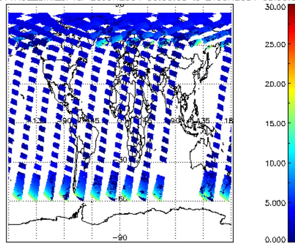
iCIOL2P_NADUV1NO2_amf_cl for 20JUN2004 00:00:00 to 21JUN2004 00:00:00
