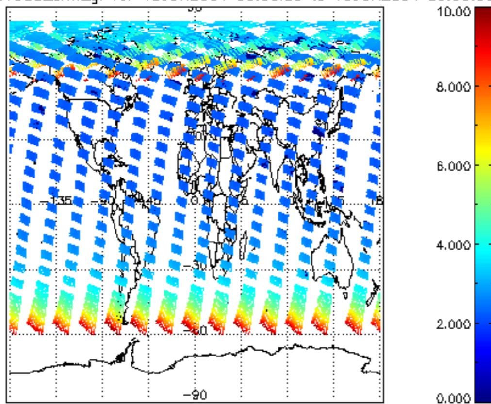
SCIOL2P_NADUV003_amf_gr for 15JUN2004 00:00:00 to 16JUN2004 00:00:00
