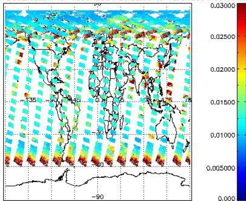
SCIOL2P_NADUV003_vcd_err for 15JUN2004 00:00:00 to 16JUN2004 00:00:00
