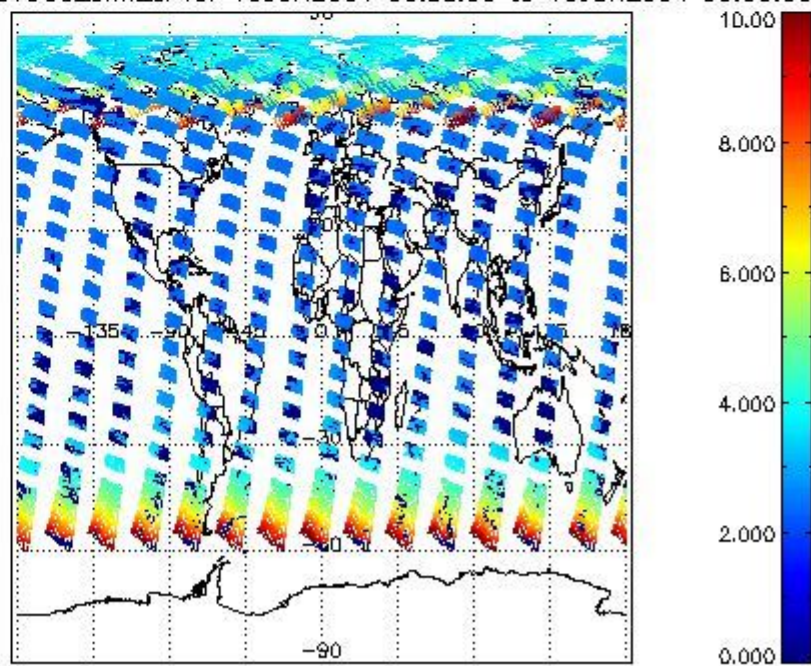
SCIOL2P_NADUV003_amf_cl for 15JUN2004 00:00:00 to 16JUN2004 00:00:00
