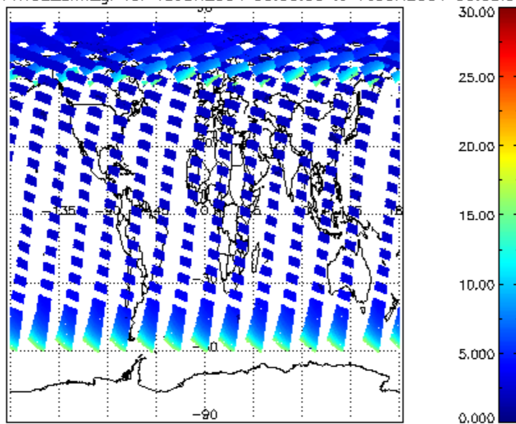
iCIOL2P_NADUV1NO2_amf_gr for 15JUN2004 00:00:00 to 16JUN2004 00:00:00
