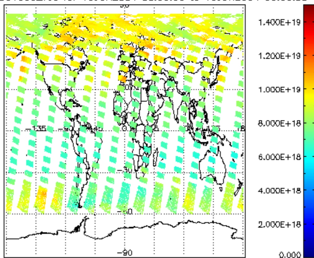
SCIOL2P_NADUV003_vcd for 15JUN2004 00:00:00 to 16JUN2004 00:00:00
