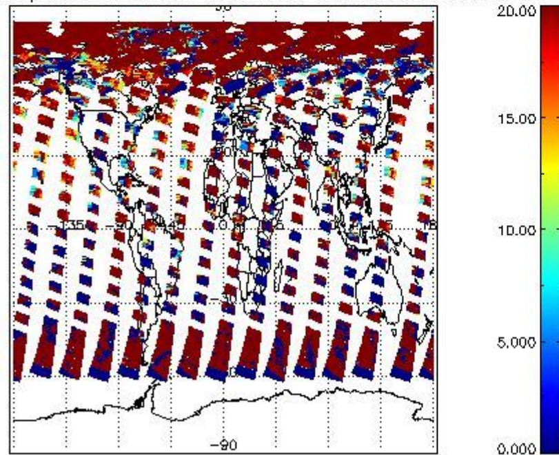
cL_opt_depth for 15JUN2004 00:00:00 to 16JUN2004 00:00:00
