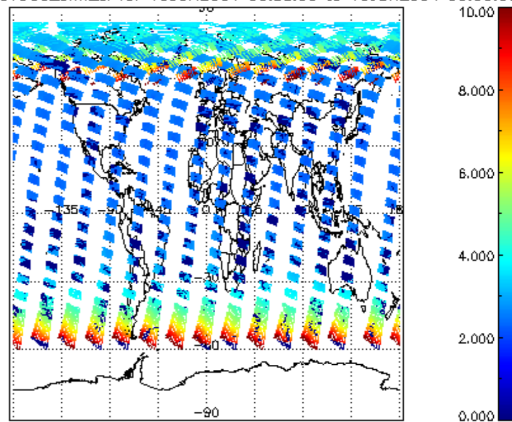
SCIOL2P_NADUV003_amf_cl for 15JUN2004 00:00:00 to 16JUN2004 00:00:00
