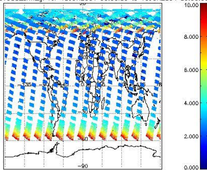
SCIOL2P_NADUV003_amf_gr for 15JUN2004 00:00:00 to 16JUN2004 00:00:00
