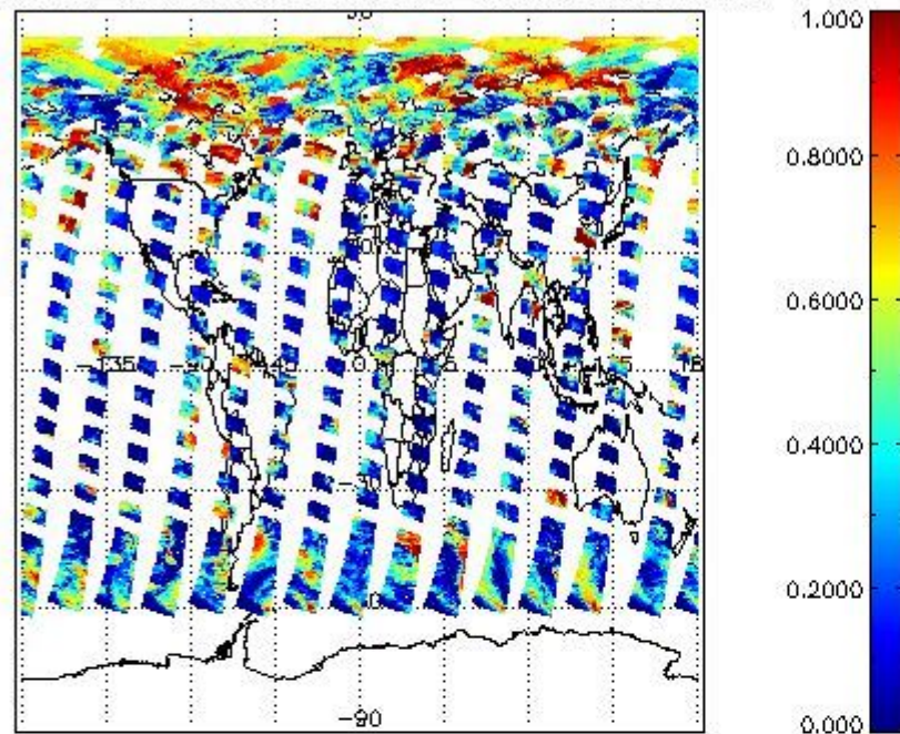
cL_frac for 15JUN2004 00:00:00 to 16JUN2004 00:00:00
