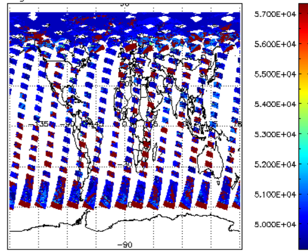
cloud_flags for 15JUN2004 00:00:00 to 16JUN2004 00:00:00
