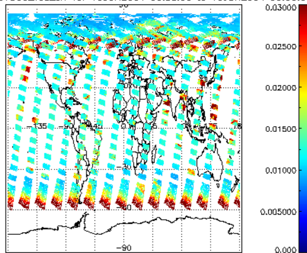
SCIOL2P_NADUV003_vcd_err for 15JUN2004 00:00:00 to 16JUN2004 00:00:00
