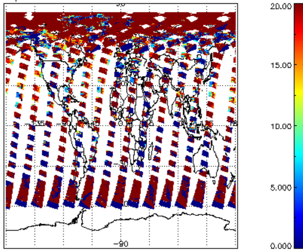
cl_opt_depth for 15JUN2004 00:00:00 to 16JUN2004 00:00:00
