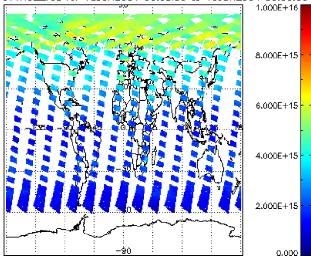
SCIOL2P_NADUV1NO2_vcd for 15JUN2004 00:00:00 to 16JUN2004 00:00:00
