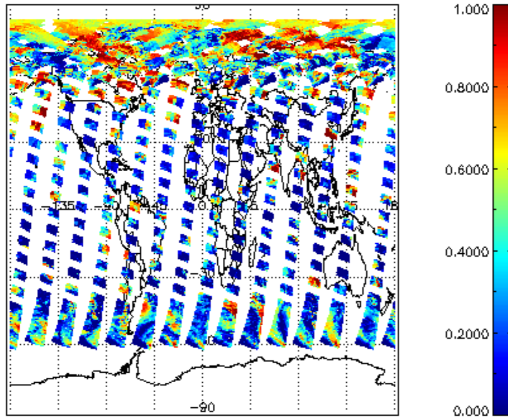
cl_frac for 15JUN2004 00:00:00 to 16JUN2004 00:00:00
