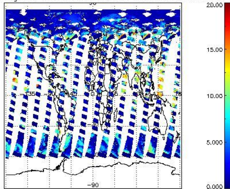
cL_top_height for 15JUN2004 00:00:00 to 16JUN2004 00:00:00
