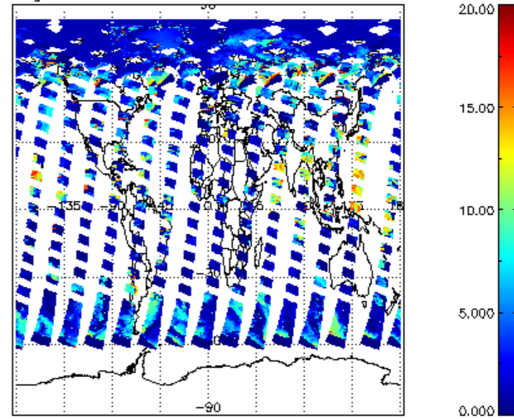
cl_top_height for 15JUN2004 00:00:00 to 16JUN2004 00:00:00
