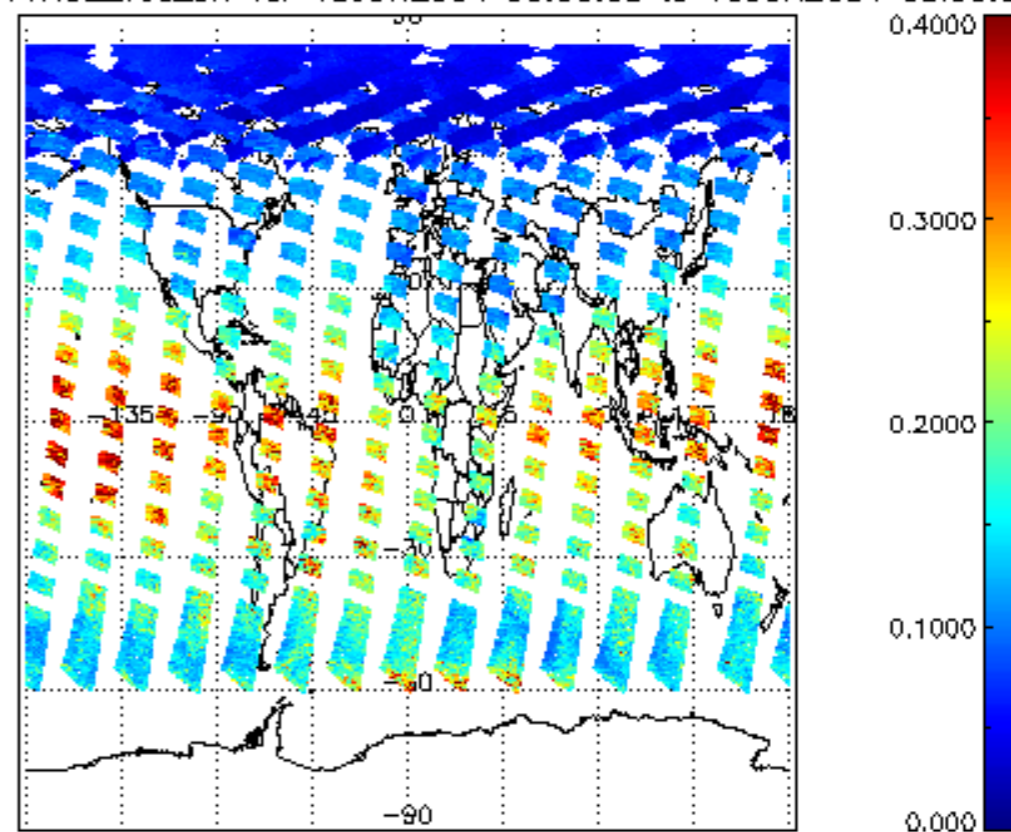
iCIOL2P_NADUV1NO2_vcd_err for 15JUN2004 00:00:00 to 16JUN2004 00:00:00
