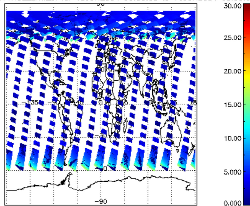
iCIOL2P_NADUV1NO2_amf_cl for 15JUN2004 00:00:00 to 16JUN2004 00:00:00
