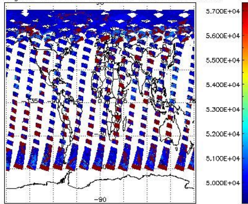
cloud_flags for 15JUN2004 00:00:00 to 16JUN2004 00:00:00
