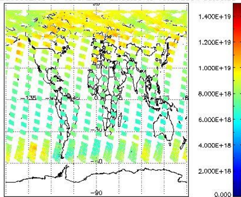
SCIOL2P_NADUV003_vcd for 15JUN2004 00:00:00 to 16JUN2004 00:00:00
