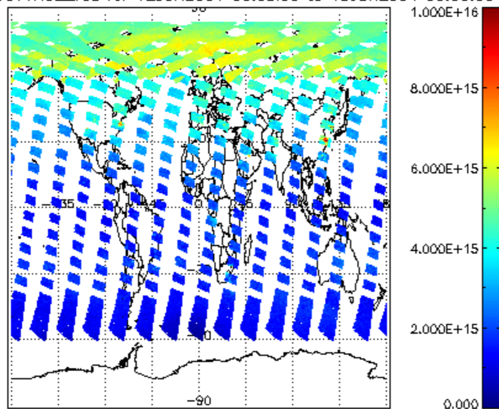
SCIOL2P_NADUV1NO2_vcd for 12JUN2004 00:00:00 to 13JUN2004 00:00:00
