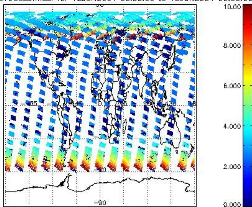
SCIOL2P_NADUV003_amf_cl for 12JUN2004 00:00:00 to 13JUN2004 00:00:00
