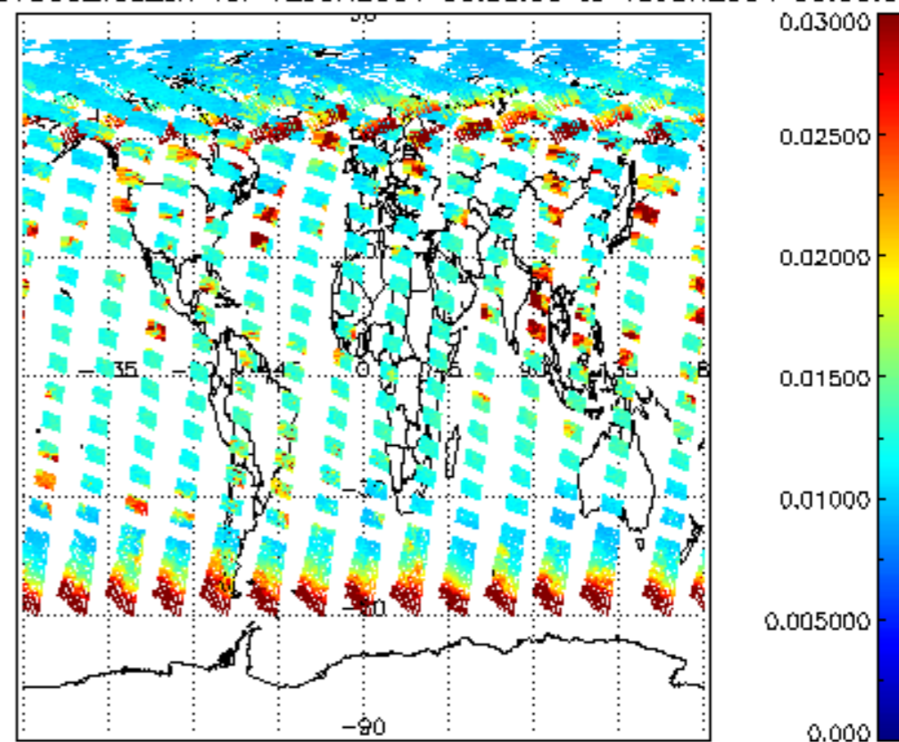
SCIOL2P_NADUV003_vcd_err for 12JUN2004 00:00:00 to 13JUN2004 00:00:00
