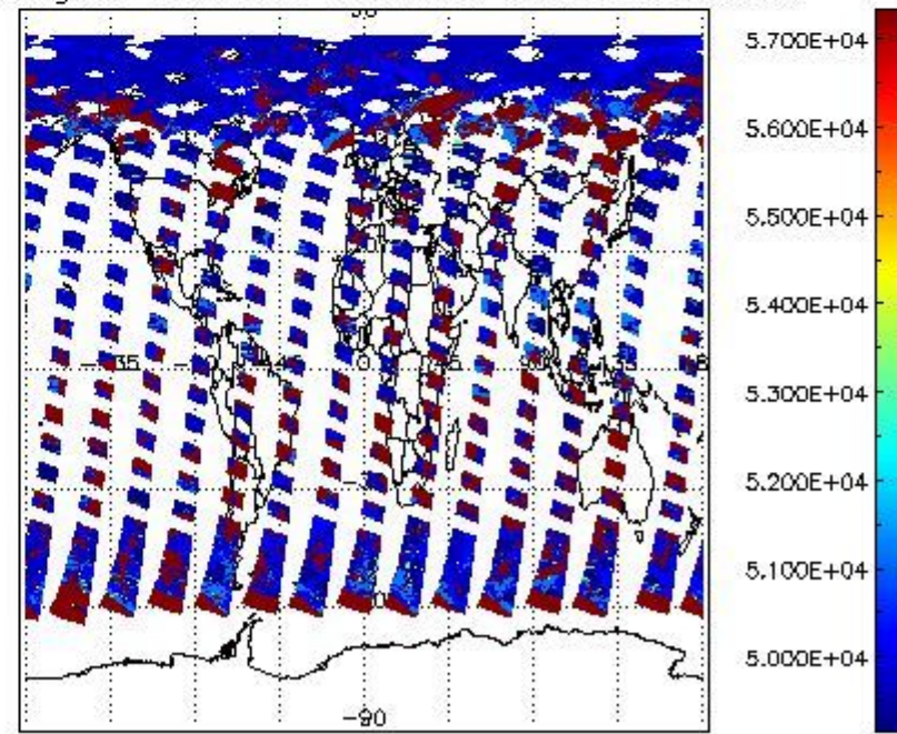
cloud_flags for 12JUN2004 00:00:00 to 13JUN2004 00:00:00
