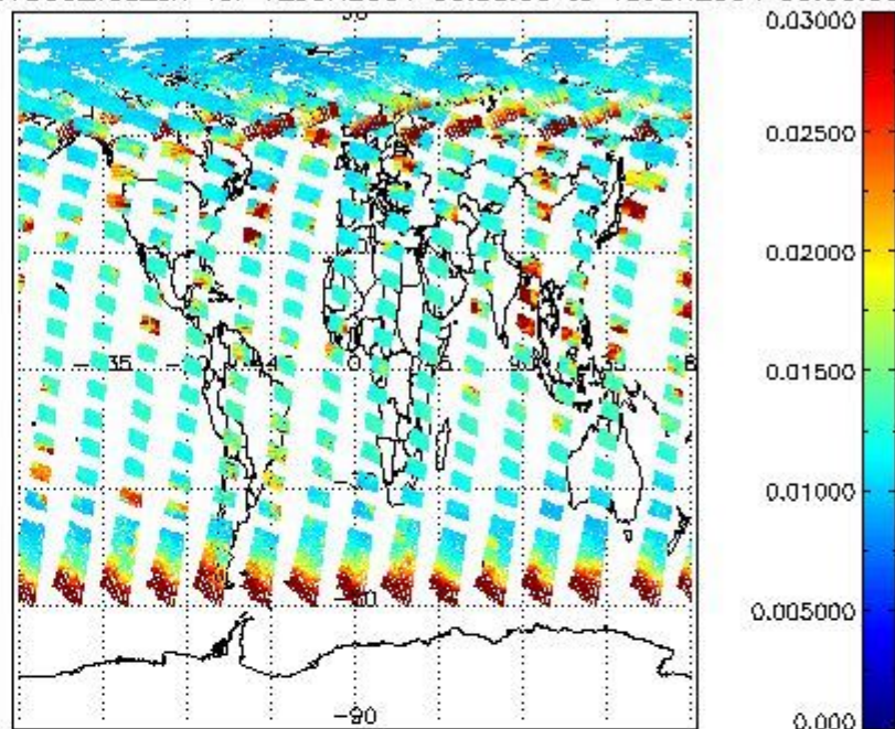
SCIOL2P_NADUV003_vcd_err for 12JUN2004 00:00:00 to 13JUN2004 00:00:00
