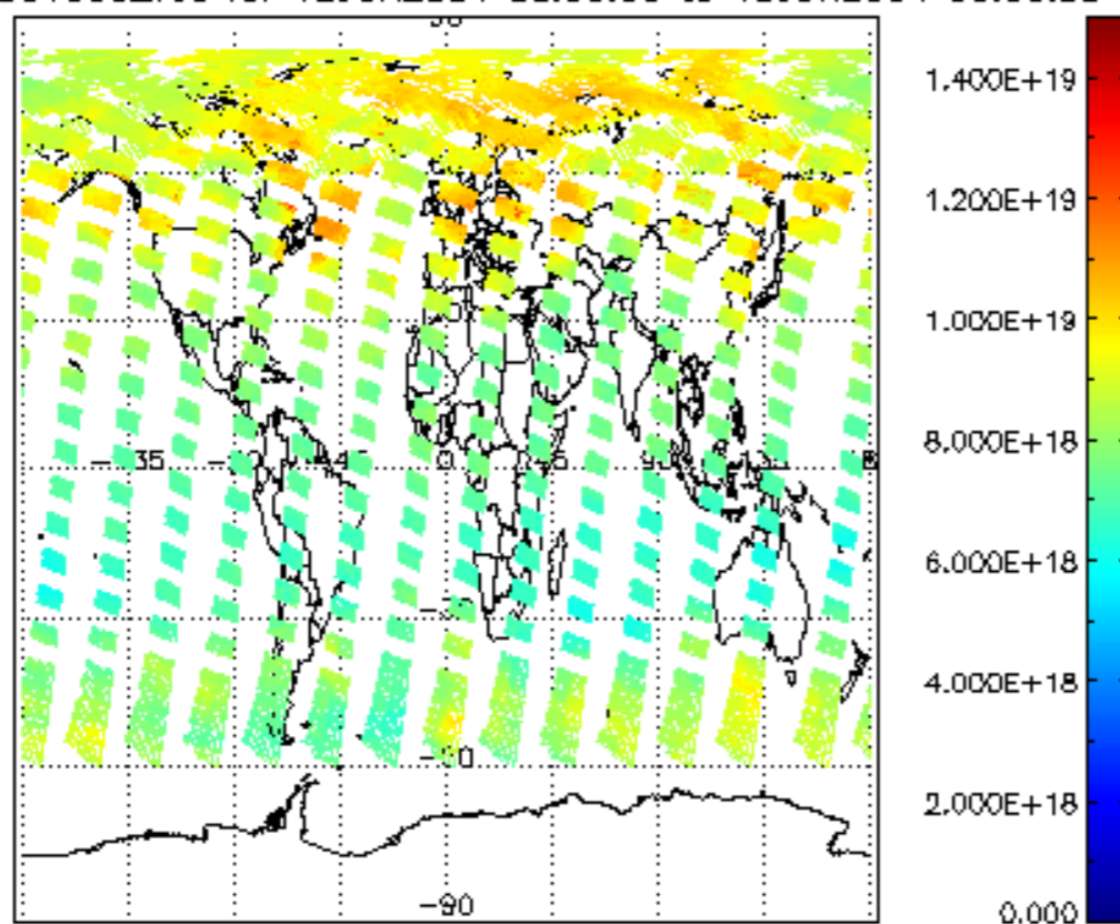
SCIOL2P_NADUV003_vcd for 12JUN2004 00:00:00 to 13JUN2004 00:00:00
