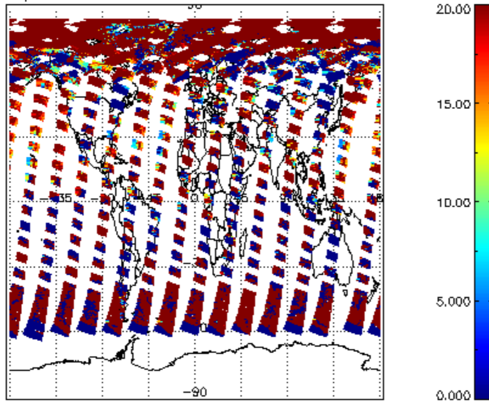
cl_opt_depth for 12JUN2004 00:00:00 to 13JUN2004 00:00:00
