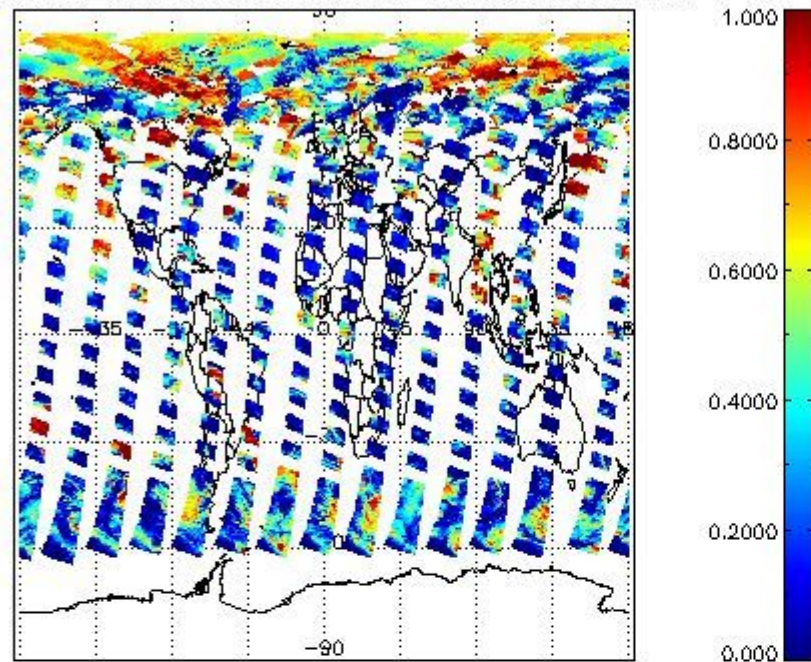
cL_frac for 12JUN2004 00:00:00 to 13JUN2004 00:00:00
