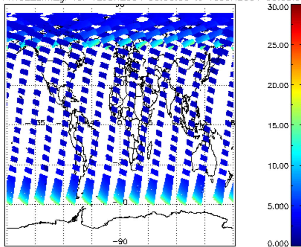
iCIOL2P_NADUV1NO2_amf_gr for 12JUN2004 00:00:00 to 13JUN2004 00:00:00
