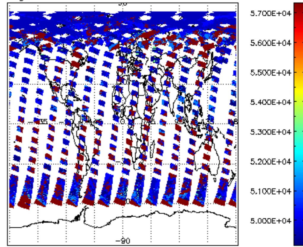
cloud_flags for 12JUN2004 00:00:00 to 13JUN2004 00:00:00
