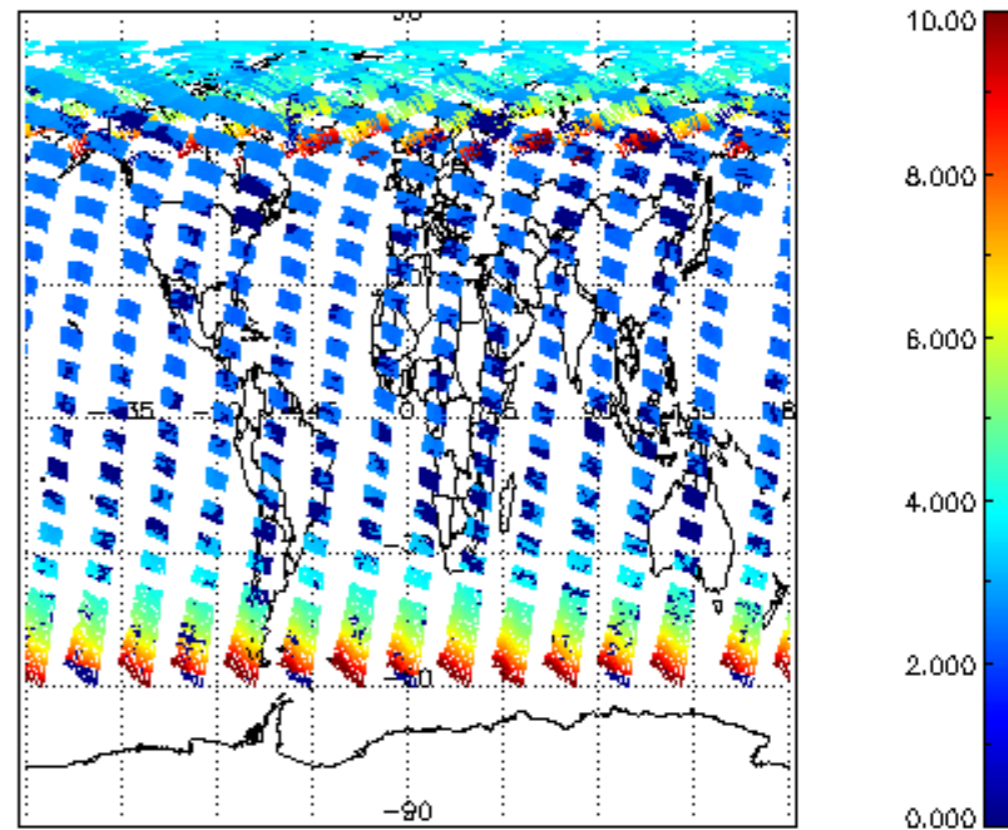
SCIOL2P_NADUV003_amf_cl for 12JUN2004 00:00:00 to 13JUN2004 00:00:00
