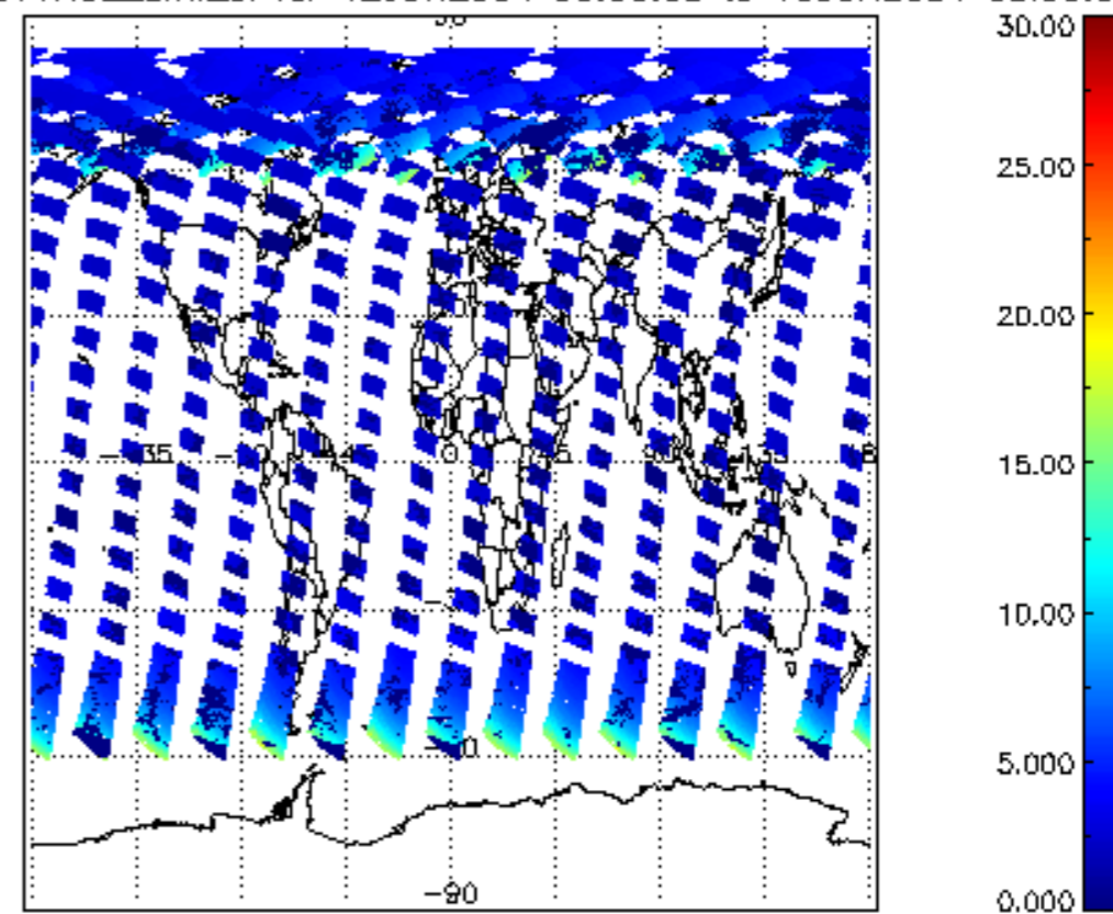
iCIOL2P_NADUV1NO2_amf_cl for 12JUN2004 00:00:00 to 13JUN2004 00:00:00
