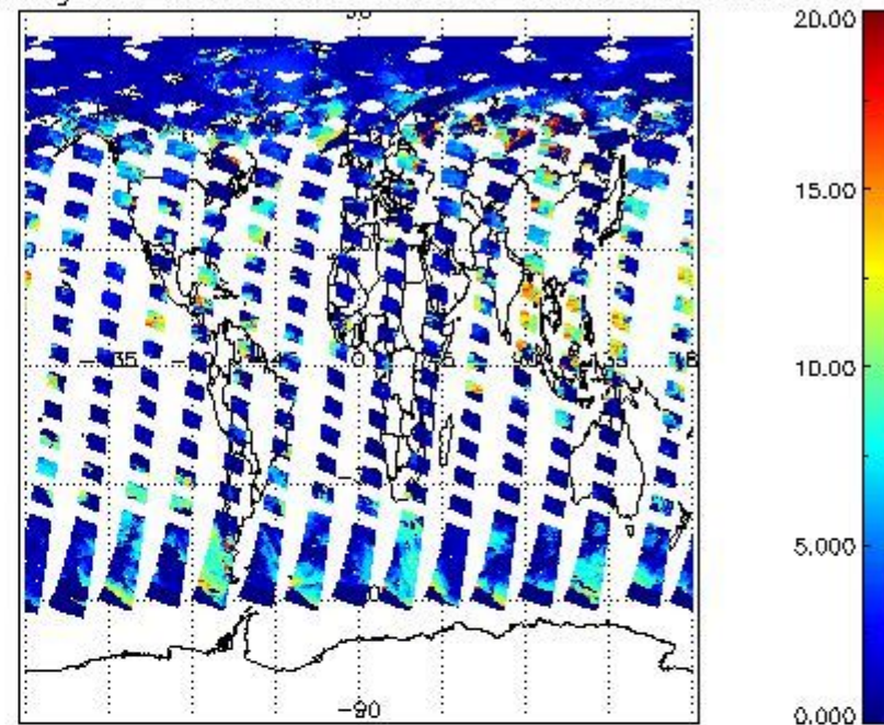
cL_top_height for 12JUN2004 00:00:00 to 13JUN2004 00:00:00
