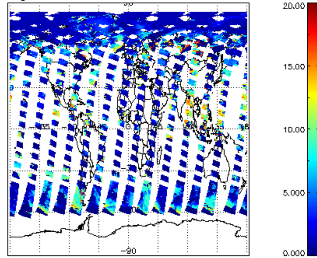
cl_top_height for 12JUN2004 00:00:00 to 13JUN2004 00:00:00
