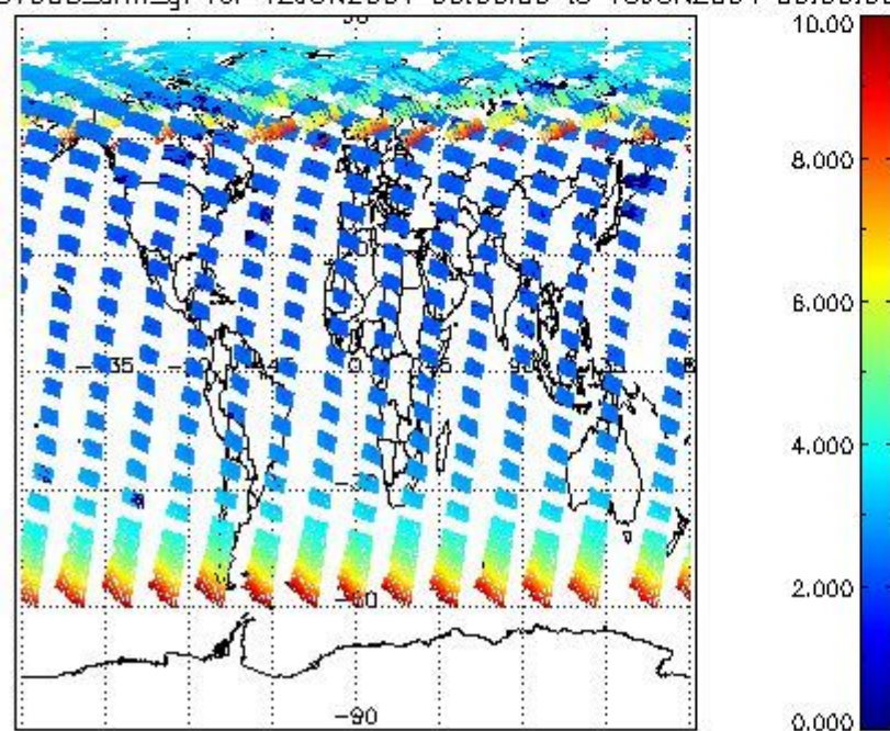
SCIOL2P_NADUV003_amf_gr for 12JUN2004 00:00:00 to 13JUN2004 00:00:00
