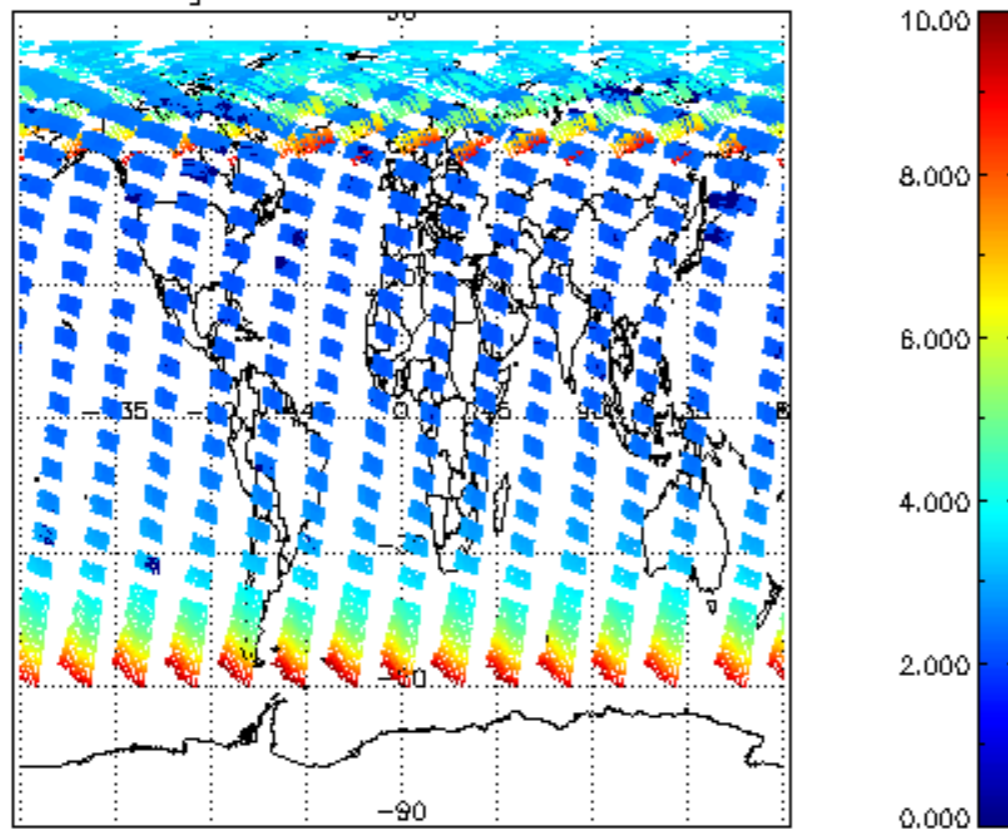
SCIOL2P_NADUV003_amf_gr for 12JUN2004 00:00:00 to 13JUN2004 00:00:00
