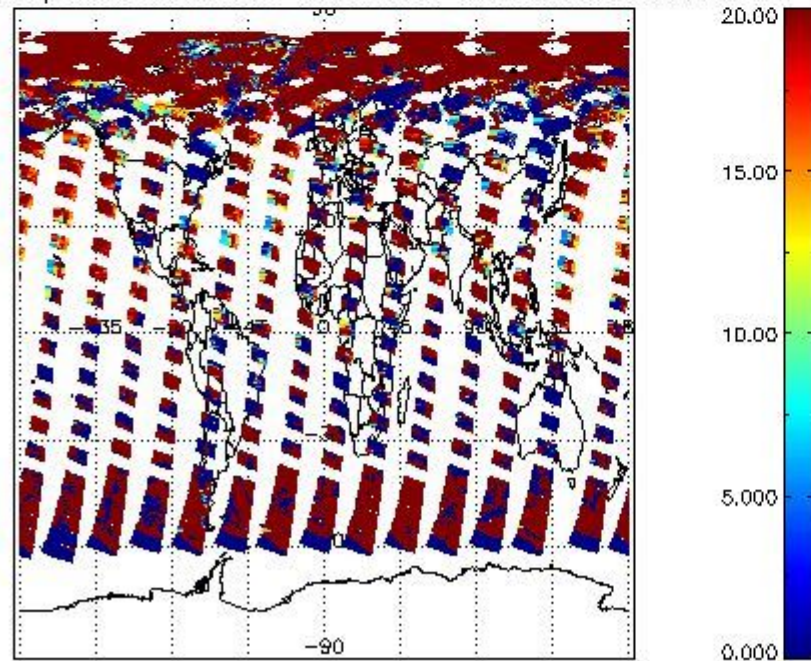
cL_opt_depth for 12JUN2004 00:00:00 to 13JUN2004 00:00:00
