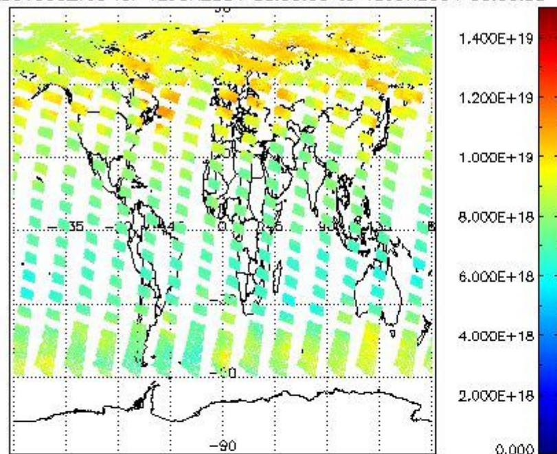
SCIOL2P_NADUV003_vcd for 12JUN2004 00:00:00 to 13JUN2004 00:00:00
