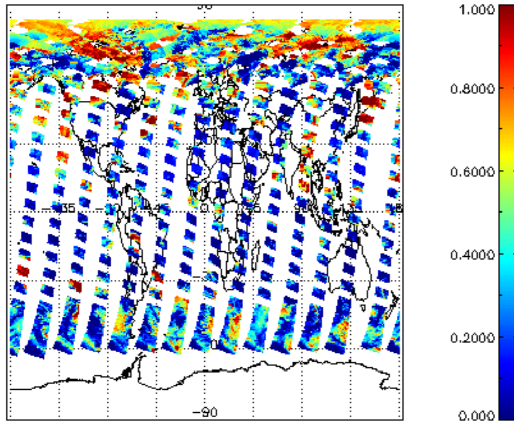
cl_frac for 12JUN2004 00:00:00 to 13JUN2004 00:00:00
