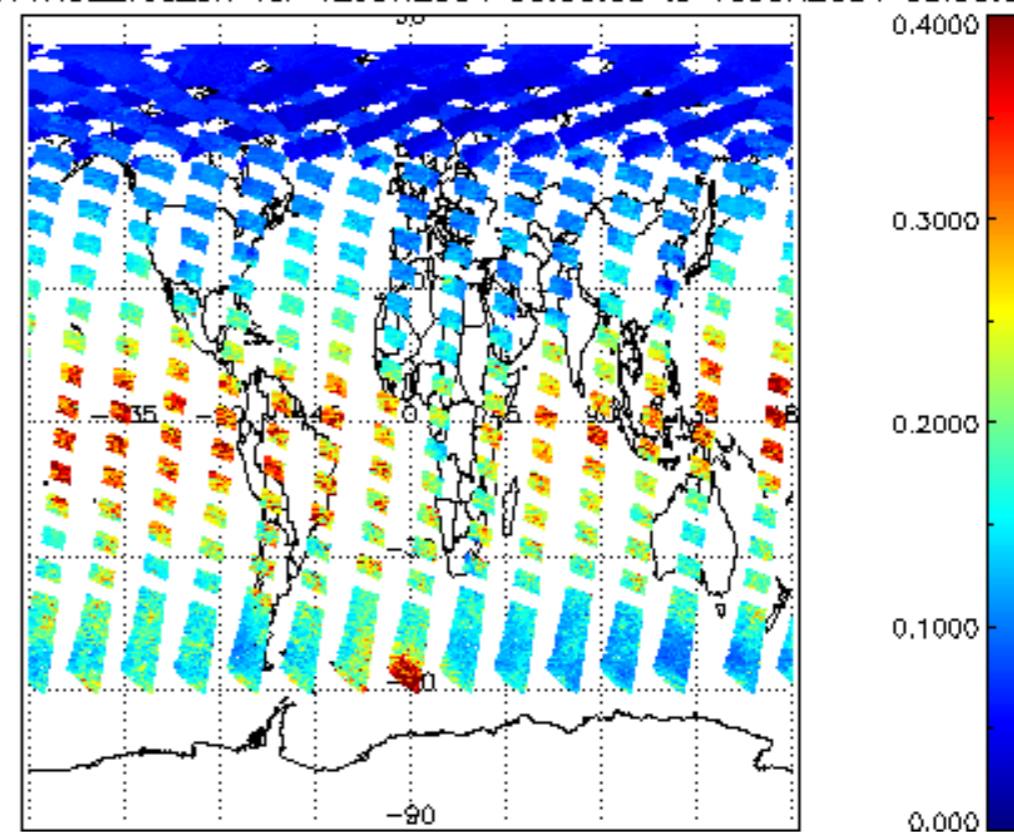
iCIOL2P_NADUV1NO2_vcd_err for 12JUN2004 00:00:00 to 13JUN2004 00:00:00
