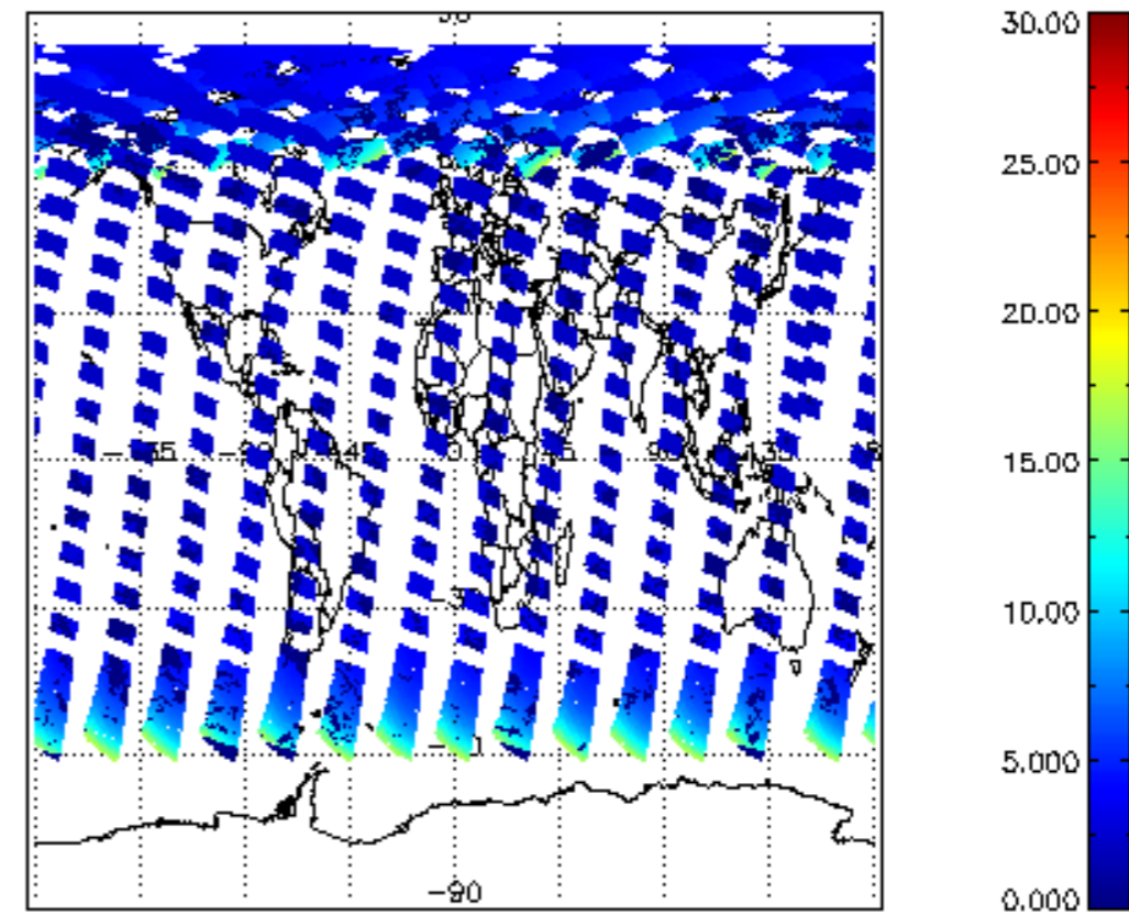
iCIOL2P_NADUV1NO2_amf_cl for 06JUN2004 00:00:00 to 07JUN2004 00:00:00
