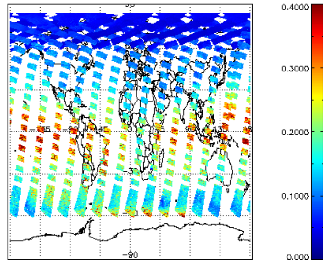
iCIOL2P_NADUV1NO2_vcd_err for 06JUN2004 00:00:00 to 07JUN2004 00:00:00
