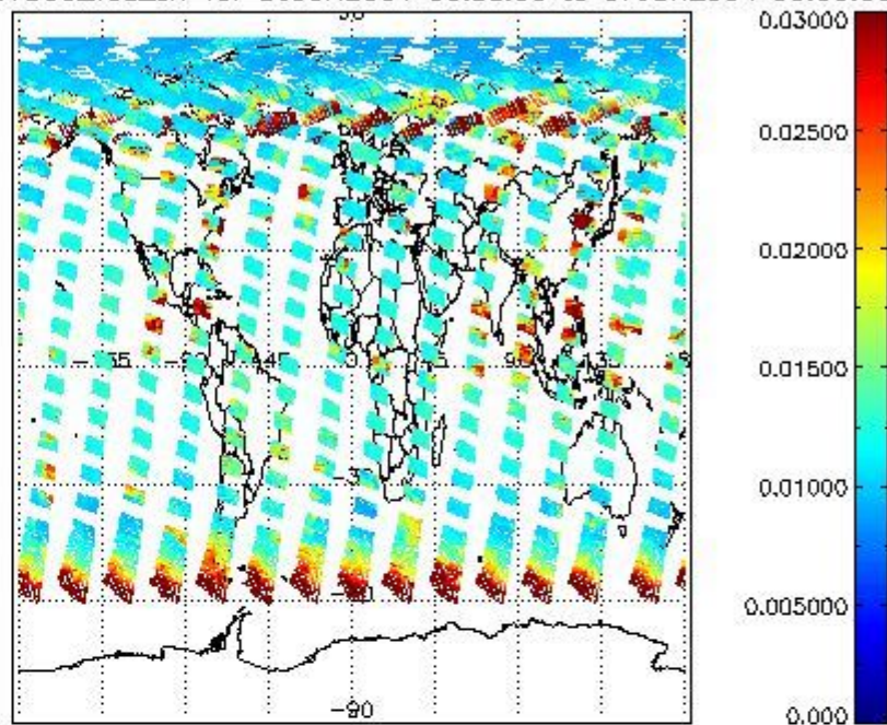
SCIOL2P_NADUV003_vcd_err for 06JUN2004 00:00:00 to 07JUN2004 00:00:00
