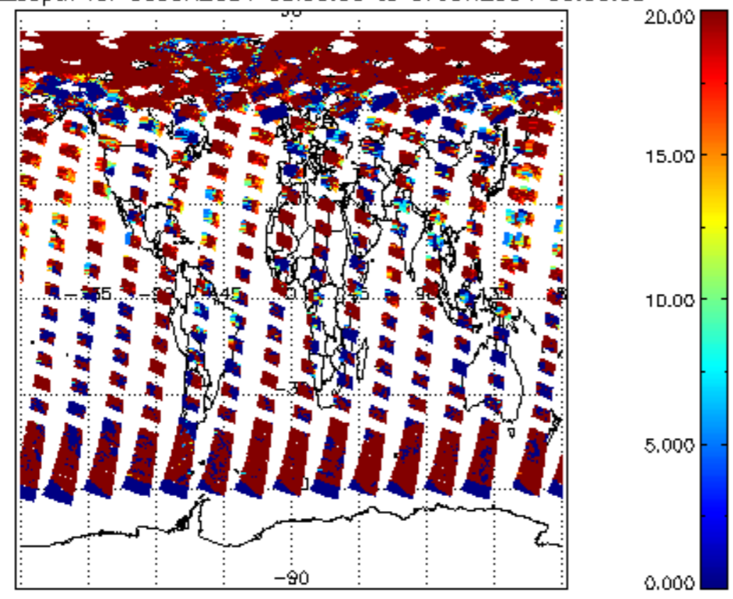
cl_opt_depth for 06JUN2004 00:00:00 to 07JUN2004 00:00:00
