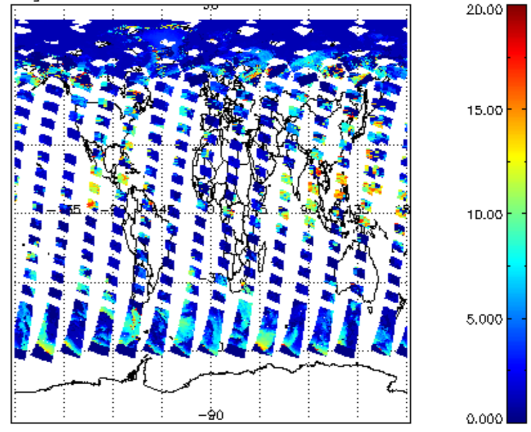
cl_top_height for 06JUN2004 00:00:00 to 07JUN2004 00:00:00
