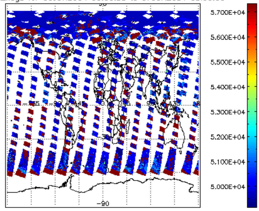
cloud_flags for 06JUN2004 00:00:00 to 07JUN2004 00:00:00
