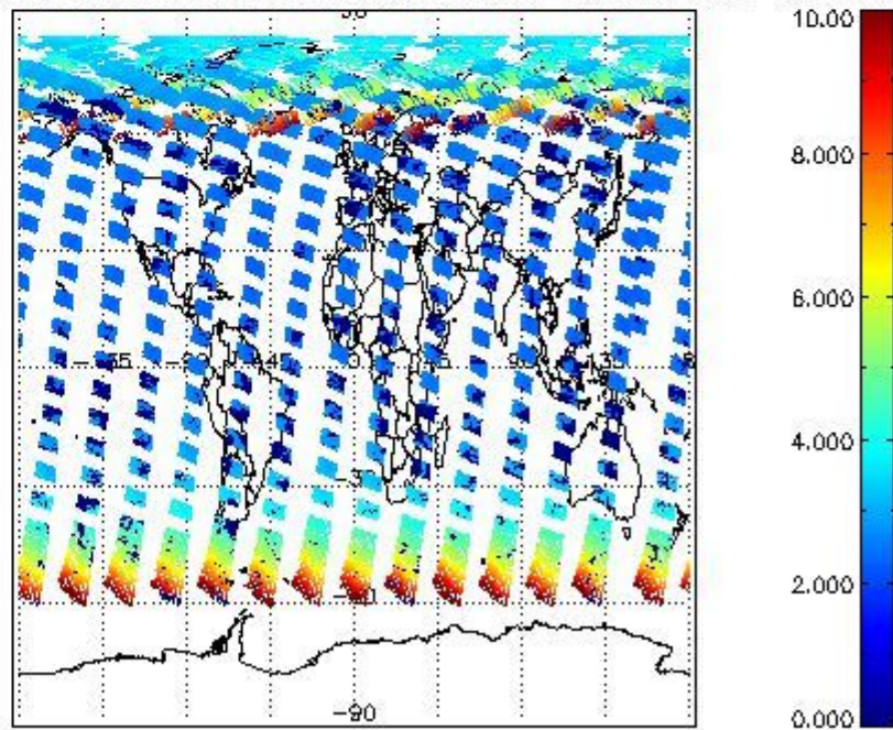
SCIOL2P_NADUV003_amf_cl for 06JUN2004 00:00:00 to 07JUN2004 00:00:00
