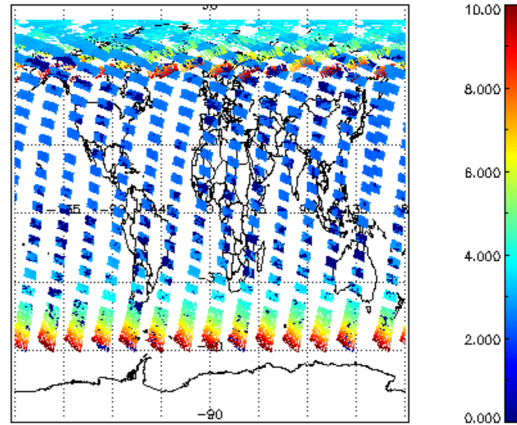
SCIOL2P_NADUV003_amf_cl for 06JUN2004 00:00:00 to 07JUN2004 00:00:00
