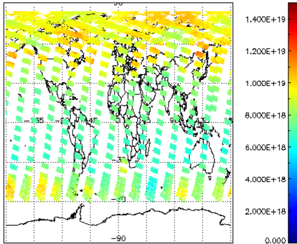
SCIOL2P_NADUV003_vcd for 06JUN2004 00:00:00 to 07JUN2004 00:00:00
