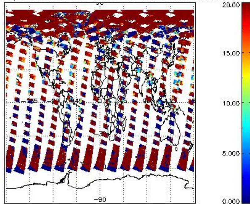
cL_opt_depth for 06JUN2004 00:00:00 to 07JUN2004 00:00:00
