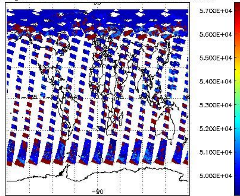
cloud_flags for 06JUN2004 00:00:00 to 07JUN2004 00:00:00
