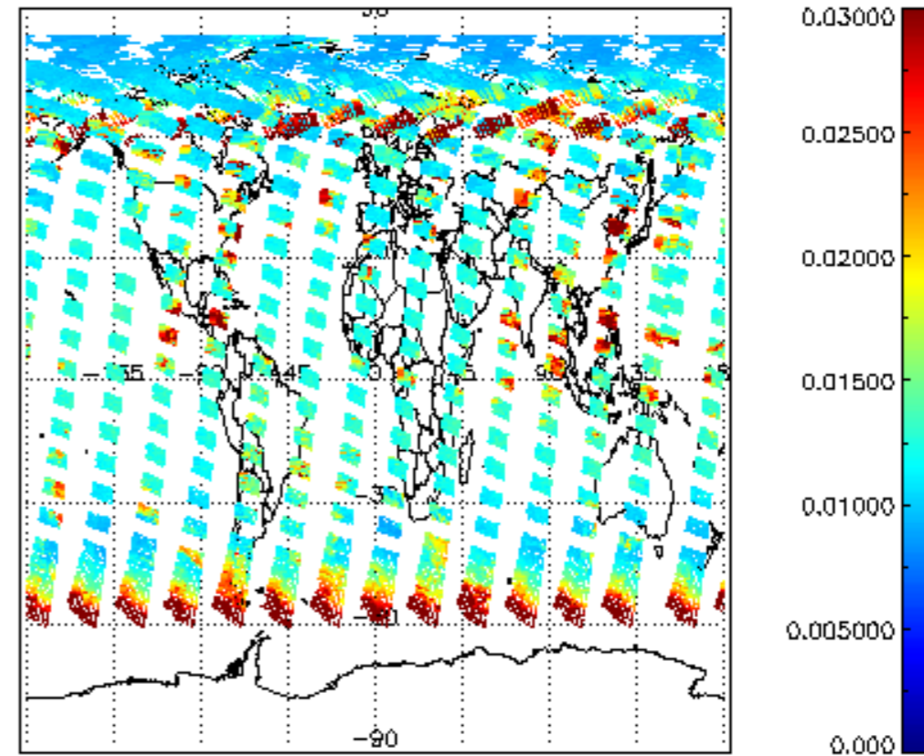
SCIOL2P_NADUV003_vcd_err for 06JUN2004 00:00:00 to 07JUN2004 00:00:00
