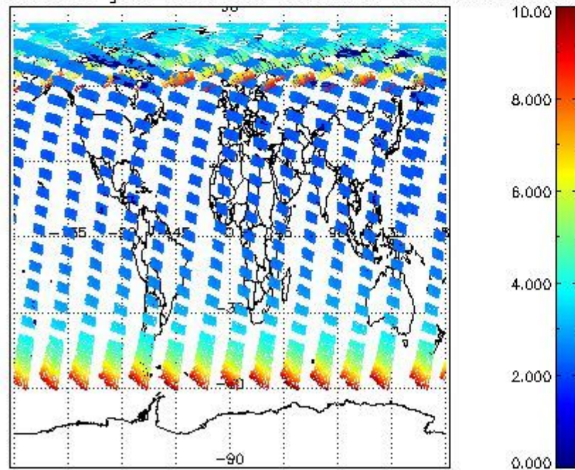
SCIOL2P_NADUV003_amf_gr for 06JUN2004 00:00:00 to 07JUN2004 00:00:00
