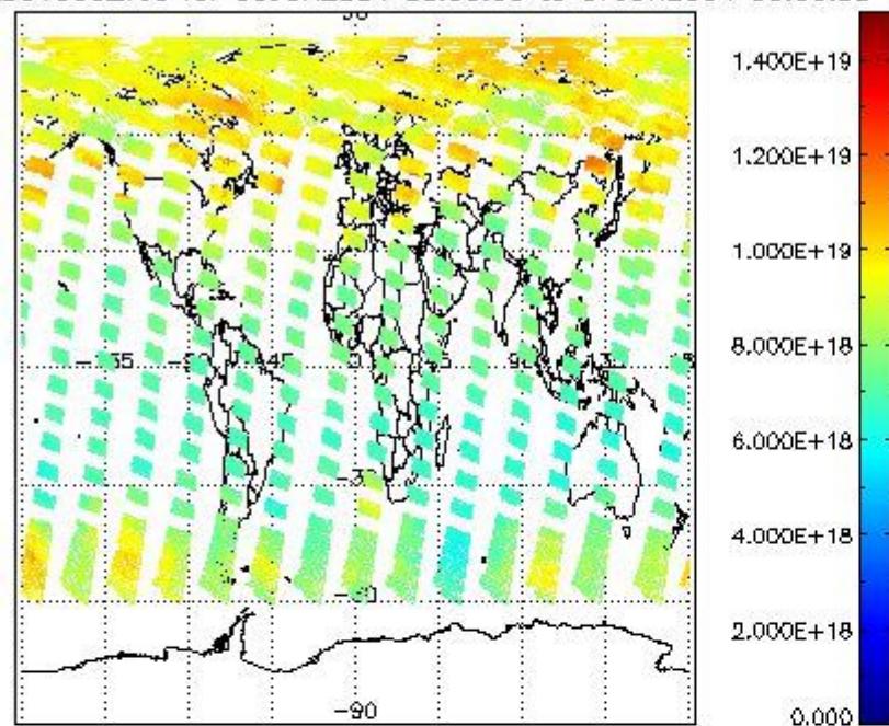
SCIOL2P_NADUV003_vcd for 06JUN2004 00:00:00 to 07JUN2004 00:00:00
