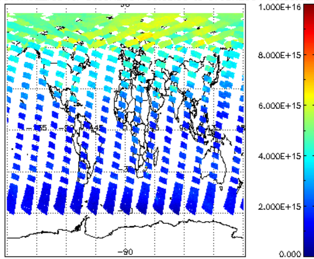
SCIOL2P_NADUV1NO2_vcd for 06JUN2004 00:00:00 to 07JUN2004 00:00:00
