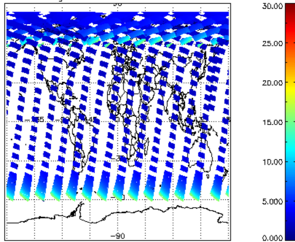
iCIOL2P_NADUV1NO2_amf_gr for 06JUN2004 00:00:00 to 07JUN2004 00:00:00
