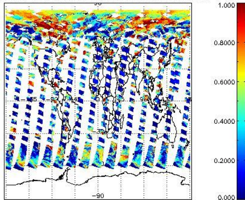
cL_frac for 06JUN2004 00:00:00 to 07JUN2004 00:00:00
