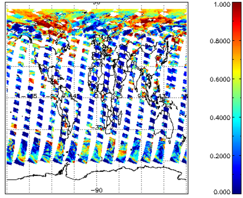
cl_frac for 06JUN2004 00:00:00 to 07JUN2004 00:00:00
