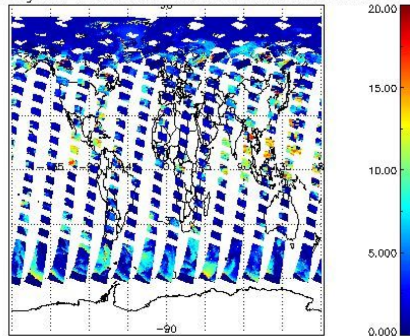
cL_top_height for 06JUN2004 00:00:00 to 07JUN2004 00:00:00
