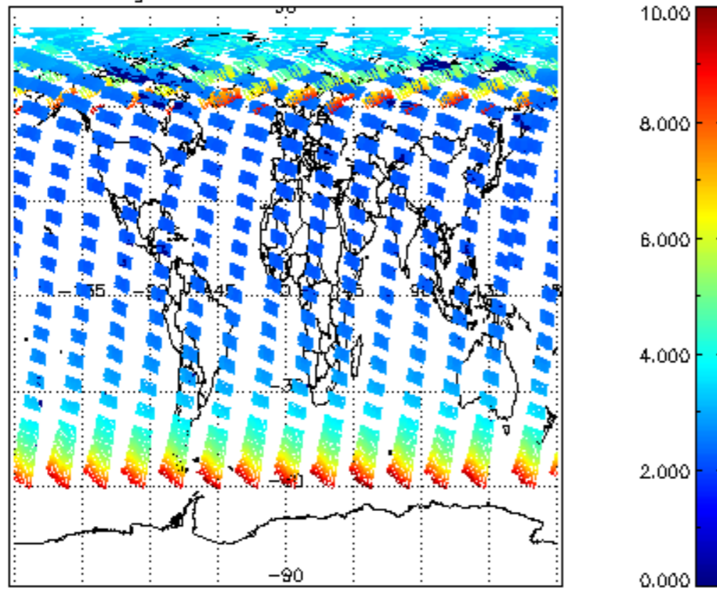
SCIOL2P_NADUV003_amf_gr for 06JUN2004 00:00:00 to 07JUN2004 00:00:00
