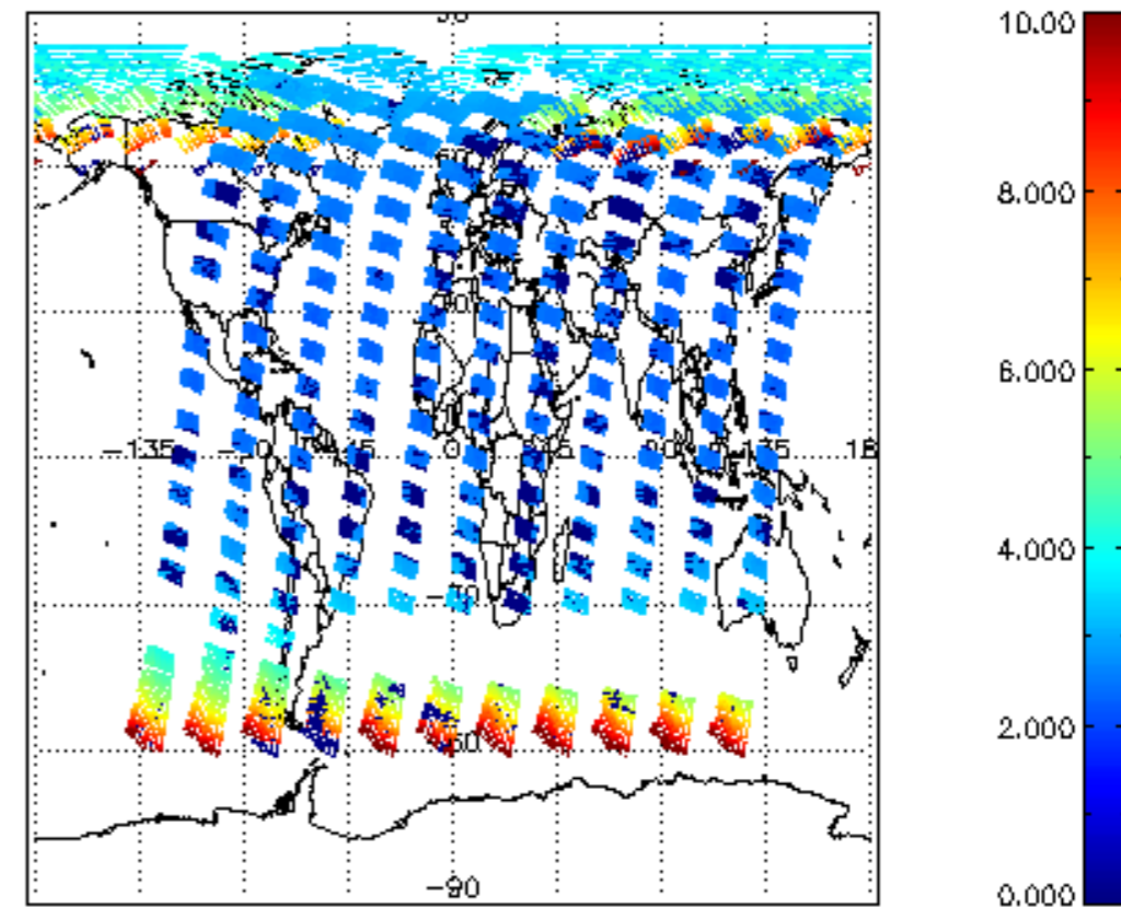
SCIOL2P_NADUV003_amf_cl for 02JUN2004 00:00:00 to 03JUN2004 00:00:00
