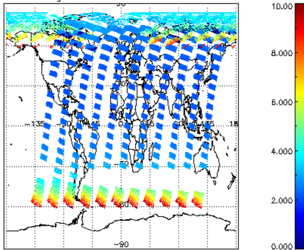
SCIOL2P_NADUV003_amf_gr for 02JUN2004 00:00:00 to 03JUN2004 00:00:00
