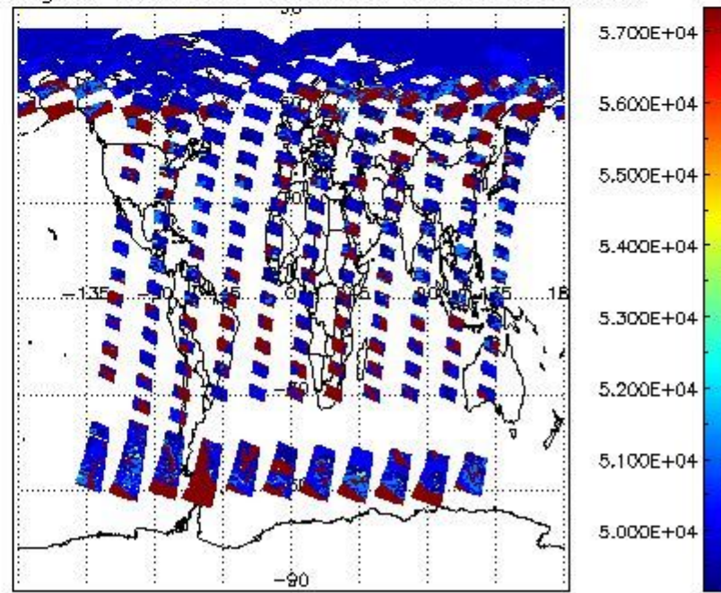
cloud_flags for 02JUN2004 00:00:00 to 03JUN2004 00:00:00
