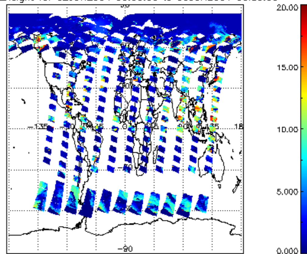
cl_top_height for 02JUN2004 00:00:00 to 03JUN2004 00:00:00
