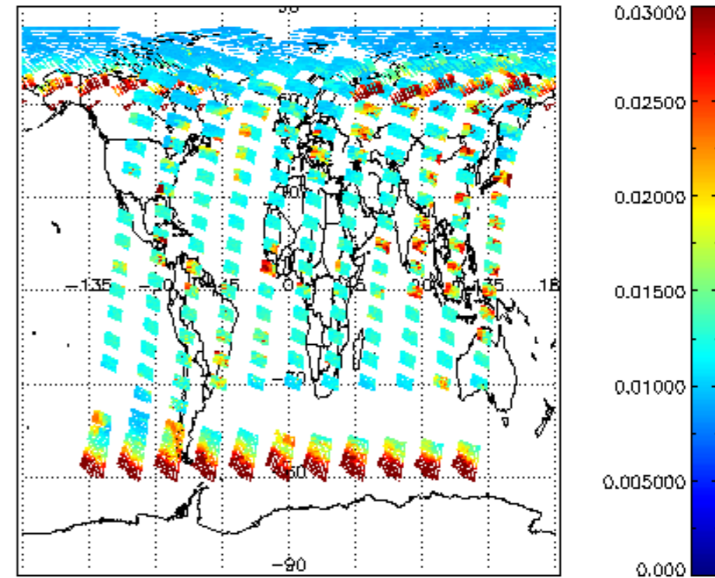
SCIOL2P_NADUV003_vcd_err for 02JUN2004 00:00:00 to 03JUN2004 00:00:00
