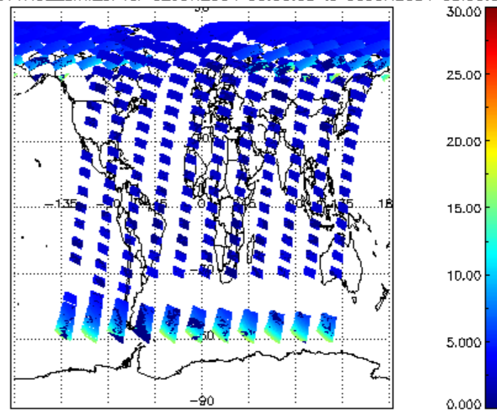
iCIOL2P_NADUV1NO2_amf_cl for 02JUN2004 00:00:00 to 03JUN2004 00:00:00
