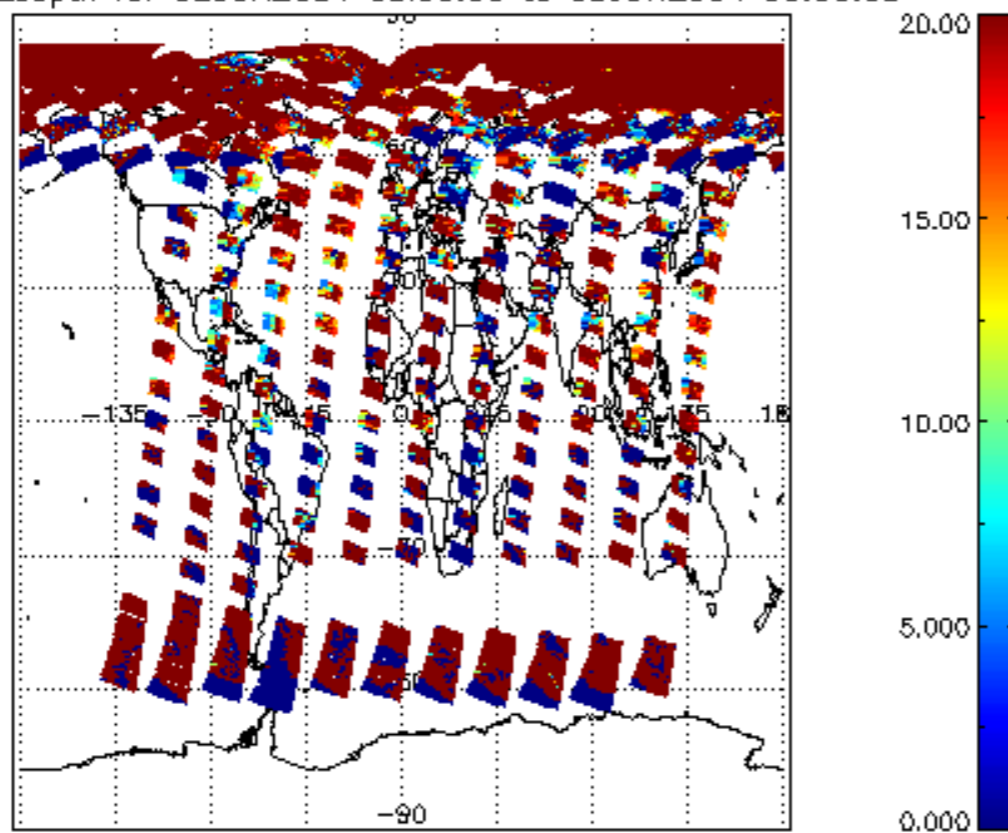
cl_opt_depth for 02JUN2004 00:00:00 to 03JUN2004 00:00:00
