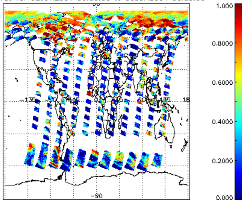
cl_frac for 02JUN2004 00:00:00 to 03JUN2004 00:00:00
