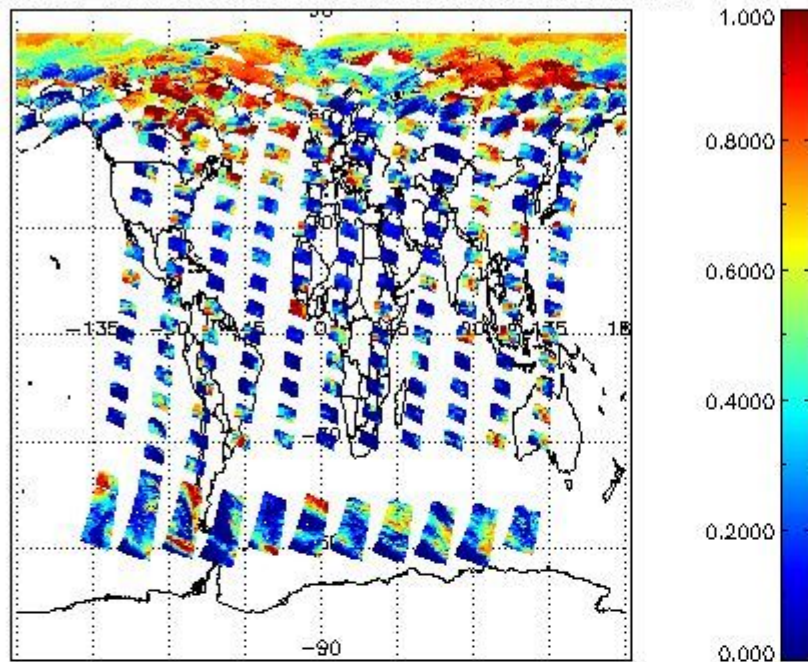
cL_frac for 02JUN2004 00:00:00 to 03JUN2004 00:00:00
