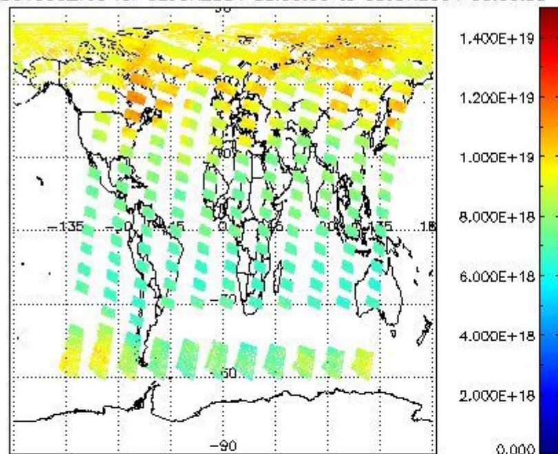
SCIOL2P_NADUV003_vcd for 02JUN2004 00:00:00 to 03JUN2004 00:00:00
