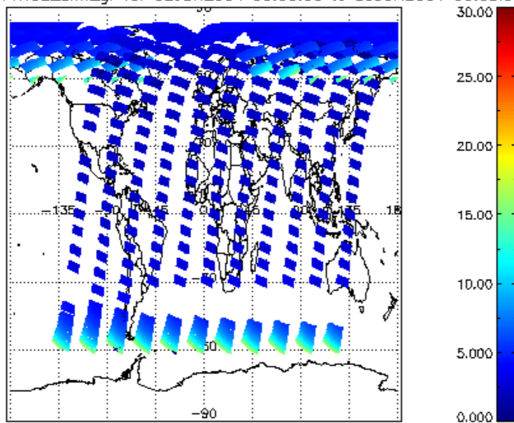
iCIOL2P_NADUV1NO2_amf_gr for 02JUN2004 00:00:00 to 03JUN2004 00:00:00
