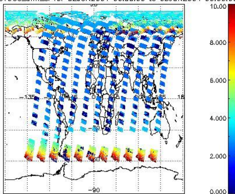
SCIOL2P_NADUV003_amf_cl for 02JUN2004 00:00:00 to 03JUN2004 00:00:00
