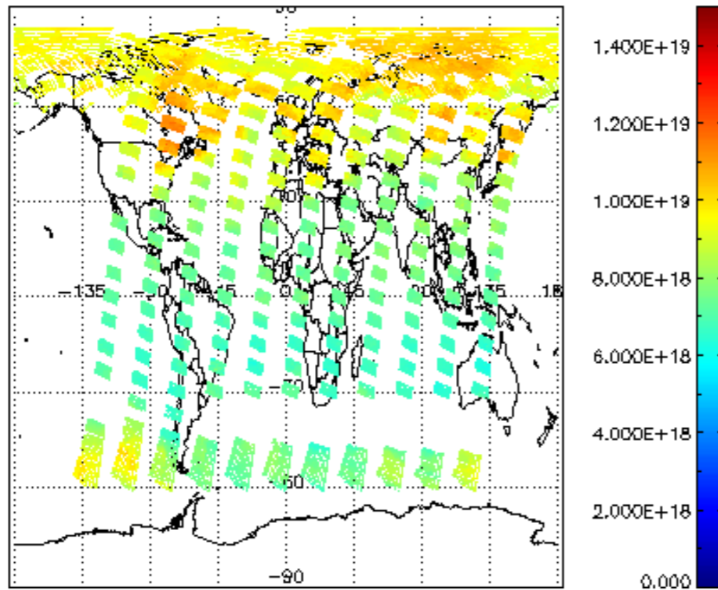
SCIOL2P_NADUV003_vcd for 02JUN2004 00:00:00 to 03JUN2004 00:00:00
