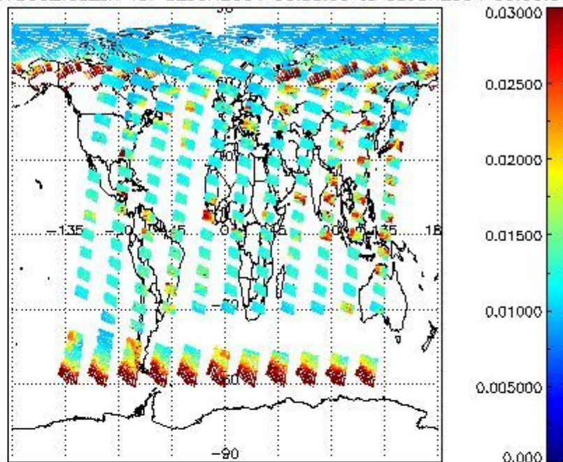
SCIOL2P_NADUV003_vcd_err for 02JUN2004 00:00:00 to 03JUN2004 00:00:00
