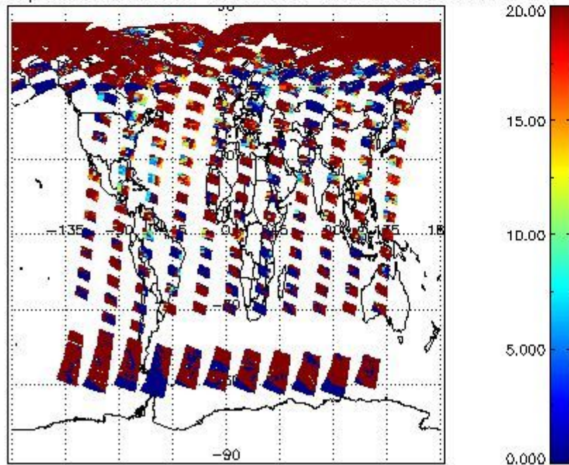
cL_opt_depth for 02JUN2004 00:00:00 to 03JUN2004 00:00:00
