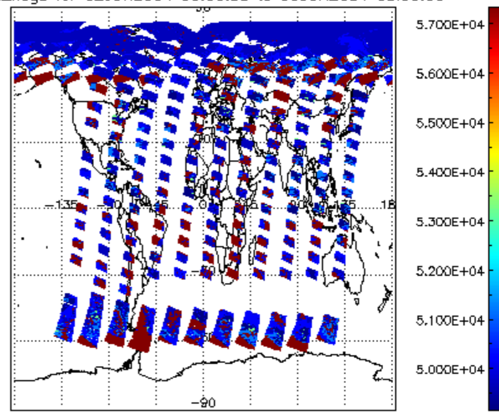
cloud_flags for 02JUN2004 00:00:00 to 03JUN2004 00:00:00
