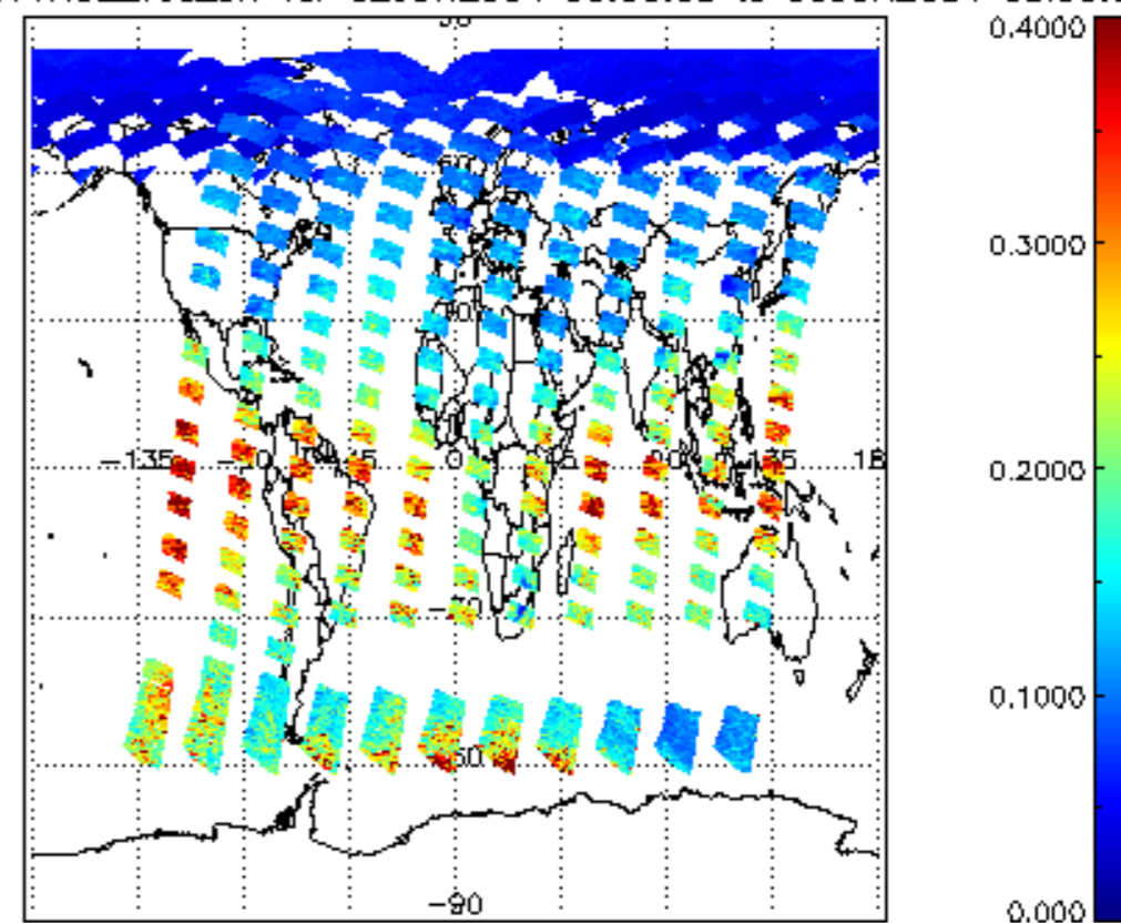
iCIOL2P_NADUV1NO2_vcd_err for 02JUN2004 00:00:00 to 03JUN2004 00:00:00
