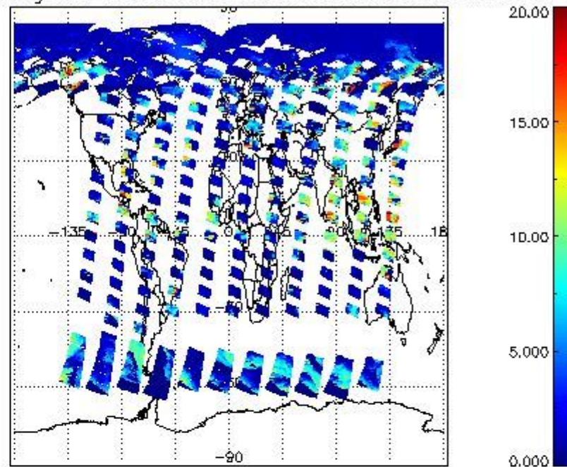
cL_top_height for 02JUN2004 00:00:00 to 03JUN2004 00:00:00
