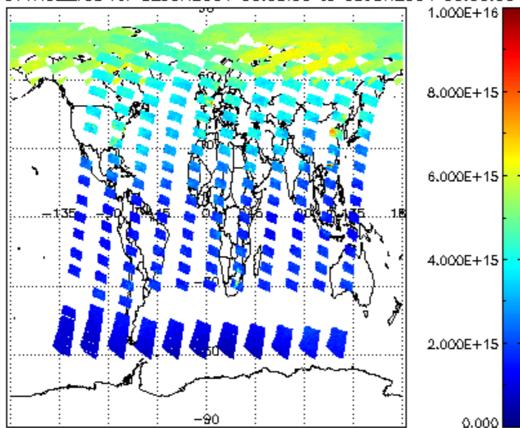
SCIOL2P_NADUV1NO2_vcd for 02JUN2004 00:00:00 to 03JUN2004 00:00:00
