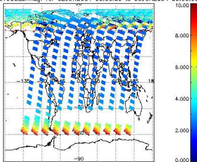
SCIOL2P_NADUV003_amf_gr for 02JUN2004 00:00:00 to 03JUN2004 00:00:00
