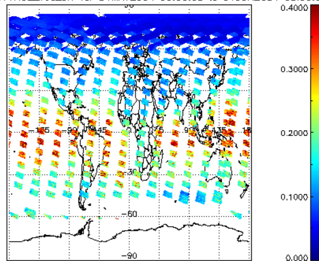
iCIOL2P_NADUV1NO2_vcd_err for 31MAY2004 00:00:00 to 01JUN2004 00:00:00
