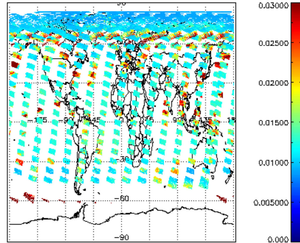
SCIOL2P_NADUV003_vcd_err for 31MAY2004 00:00:00 to 01JUN2004 00:00:00
