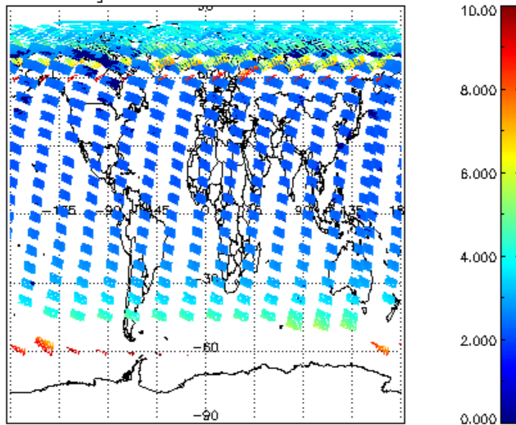
SCIOL2P_NADUV003_amf_gr for 31MAY2004 00:00:00 to 01JUN2004 00:00:00
