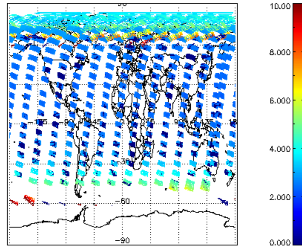
SCIOL2P_NADUV003_amf_cl for 31MAY2004 00:00:00 to 01JUN2004 00:00:00
