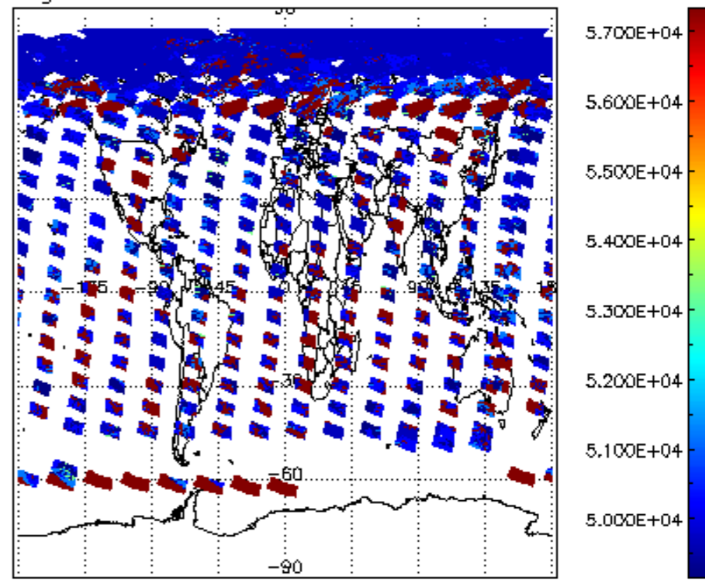
cloud_flags for 31MAY2004 00:00:00 to 01JUN2004 00:00:00
