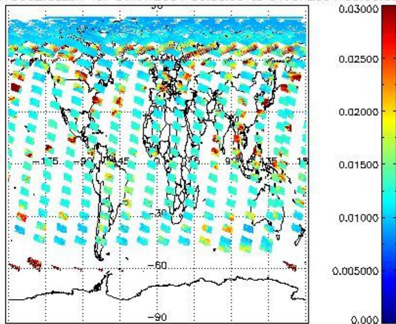
SCIOL2P_NADUV003_vcd_err for 31MAY2004 00:00:00 to 01JUN2004 00:00:00
