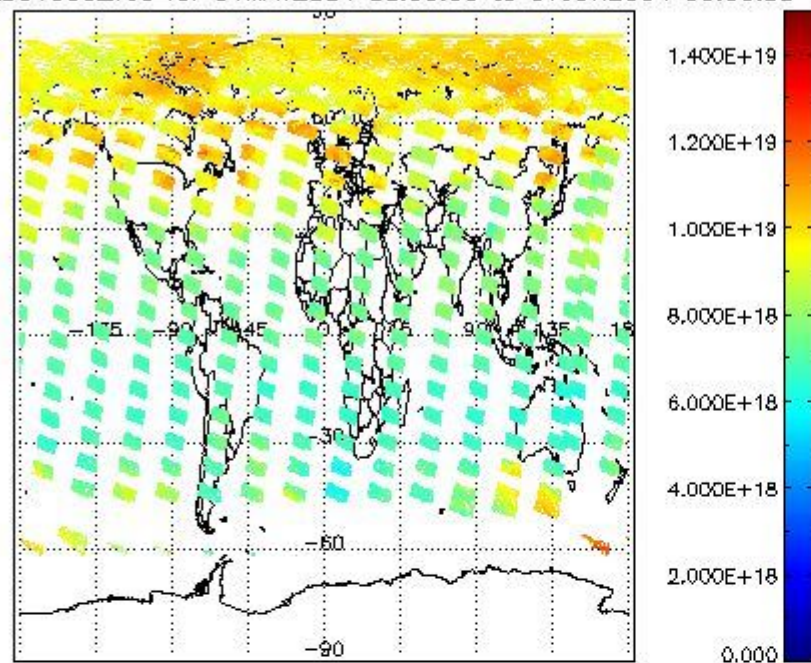
SCIOL2P_NADUV003_vcd for 31MAY2004 00:00:00 to 01JUN2004 00:00:00
