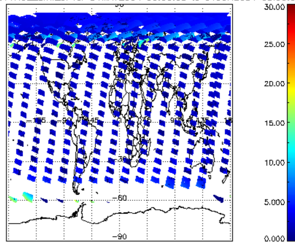
iCIOL2P_NADUV1NO2_amf_cl for 31MAY2004 00:00:00 to 01JUN2004 00:00:00
