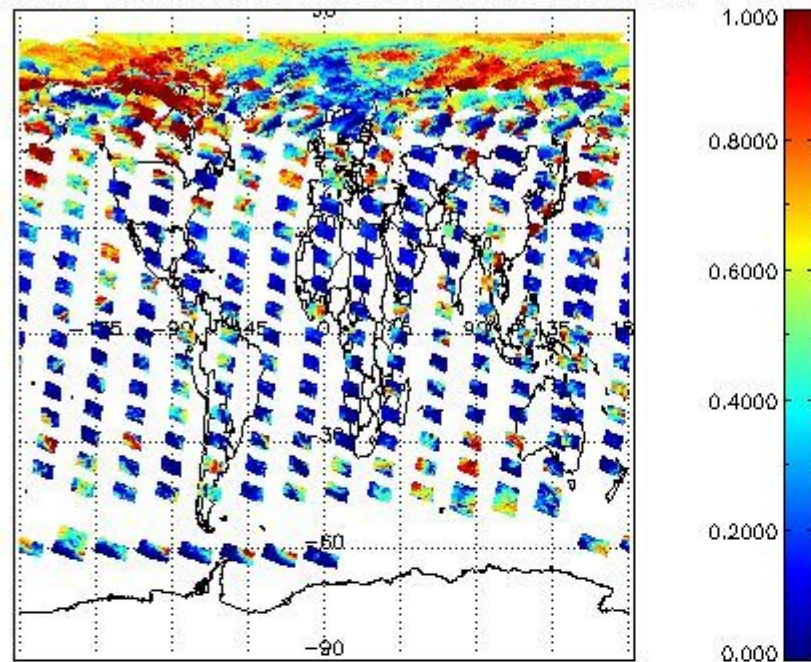
cL_frac for 31MAY2004 00:00:00 to 01JUN2004 00:00:00
