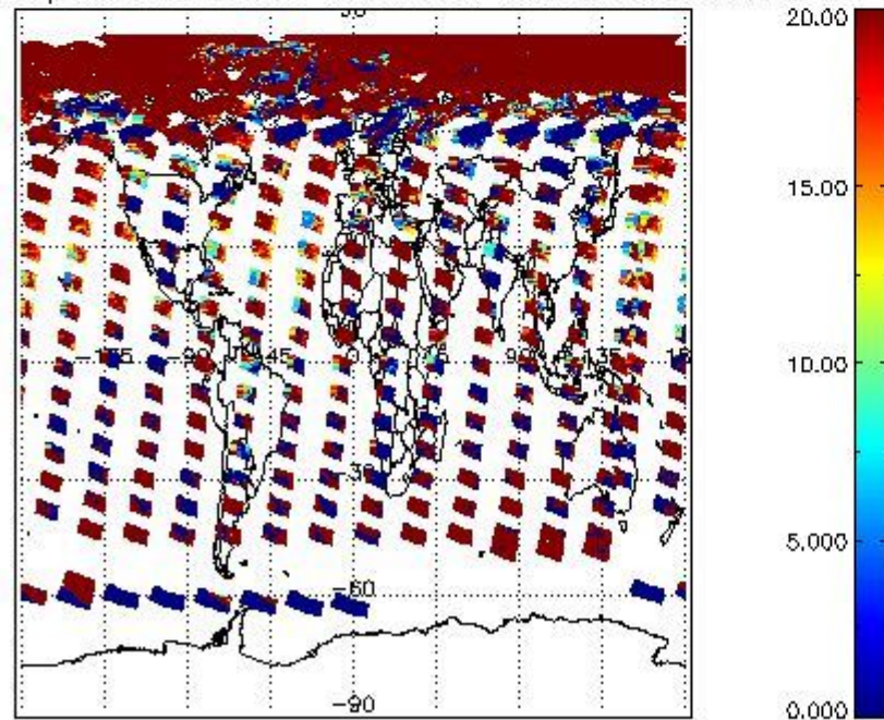
cL_opt_depth for 31MAY2004 00:00:00 to 01JUN2004 00:00:00
