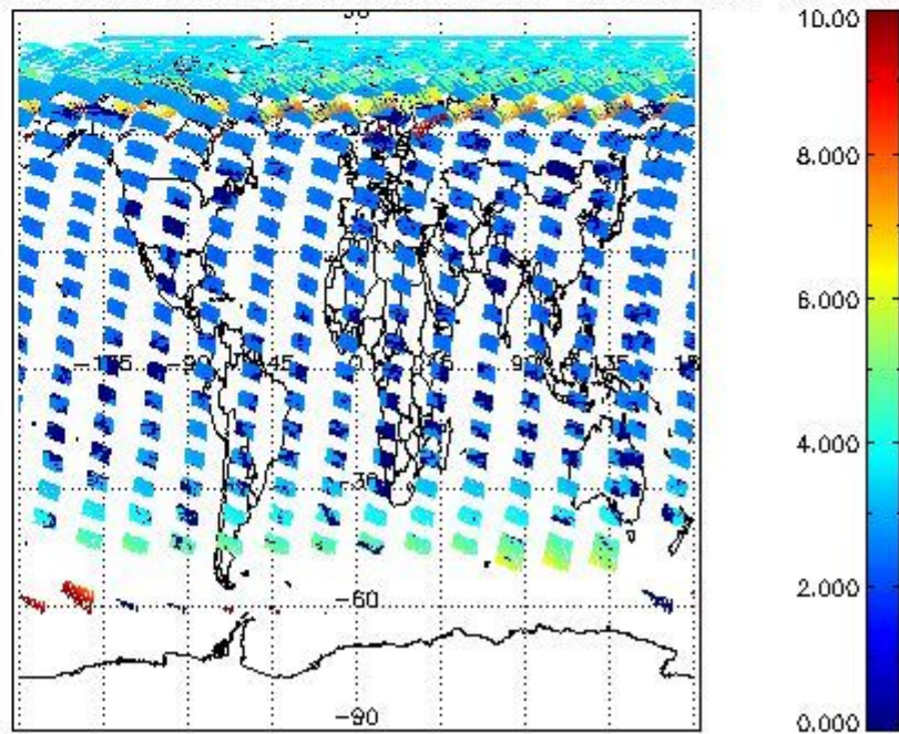
SCIOL2P_NADUV003_amf_cl for 31MAY2004 00:00:00 to 01JUN2004 00:00:00
