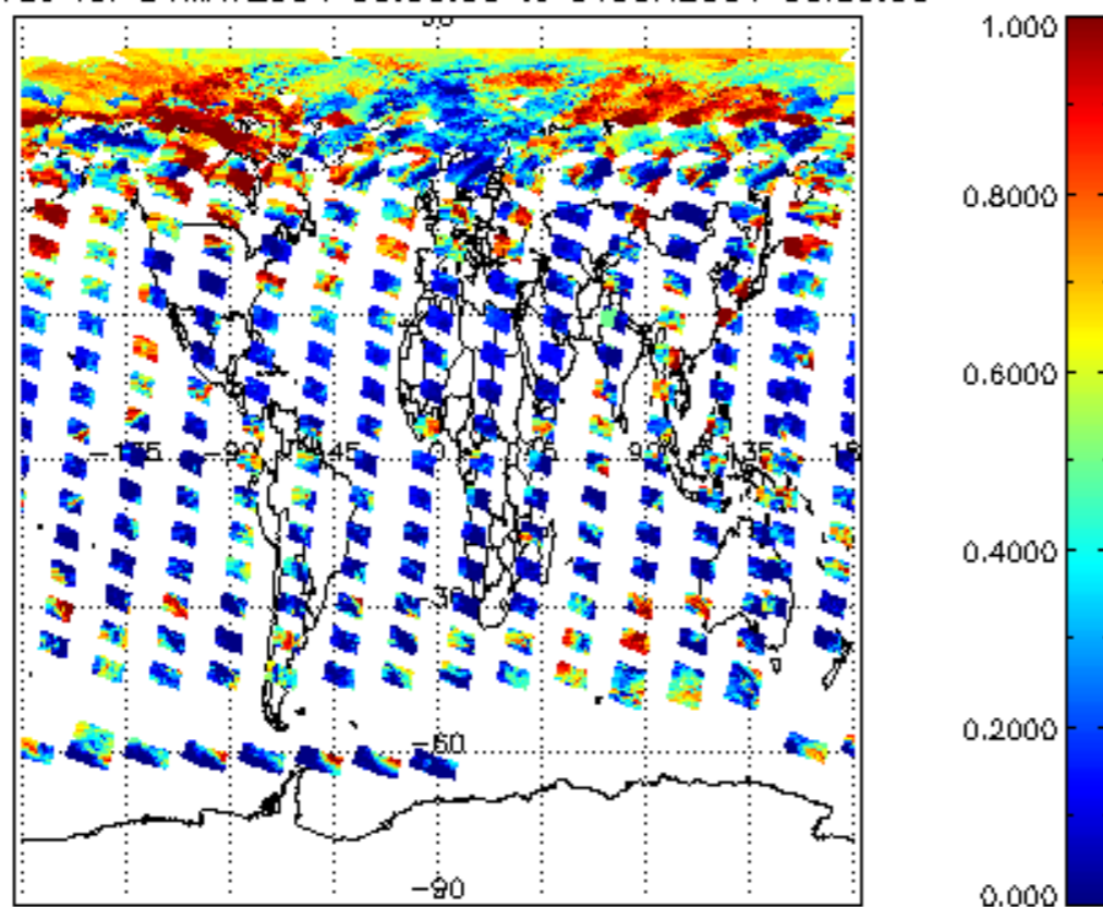
cl_frac for 31MAY2004 00:00:00 to 01JUN2004 00:00:00
