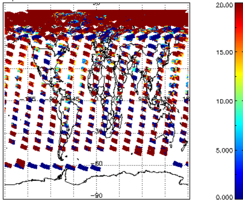
cl_opt_depth for 31MAY2004 00:00:00 to 01JUN2004 00:00:00
