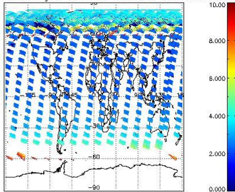
SCIOL2P_NADUV003_amf_gr for 31MAY2004 00:00:00 to 01JUN2004 00:00:00
