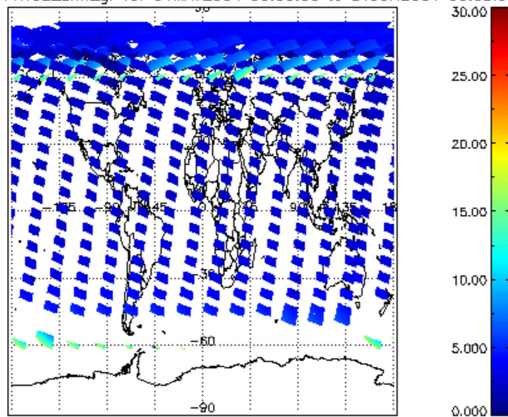
iCIOL2P_NADUV1NO2_amf_gr for 31MAY2004 00:00:00 to 01JUN2004 00:00:00
