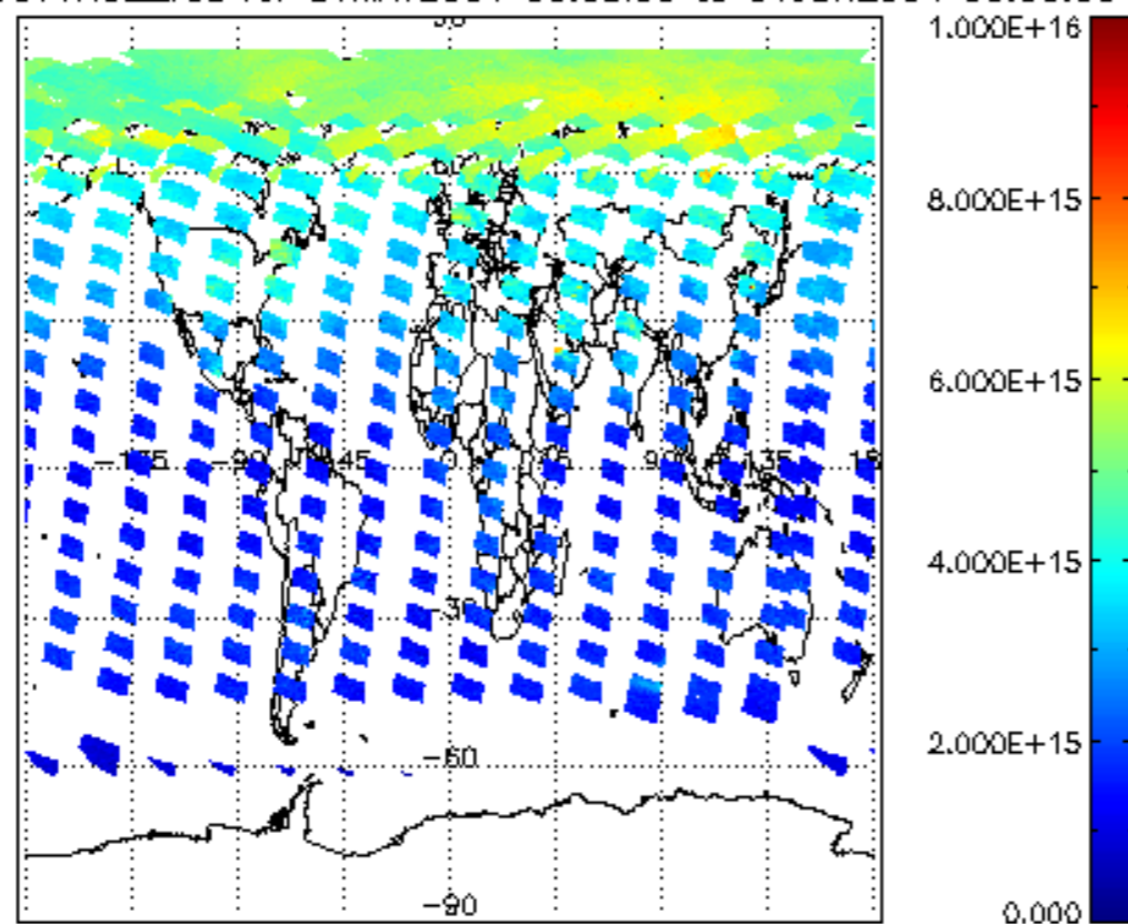
SCIOL2P_NADUV1NO2_vcd for 31MAY2004 00:00:00 to 01JUN2004 00:00:00
