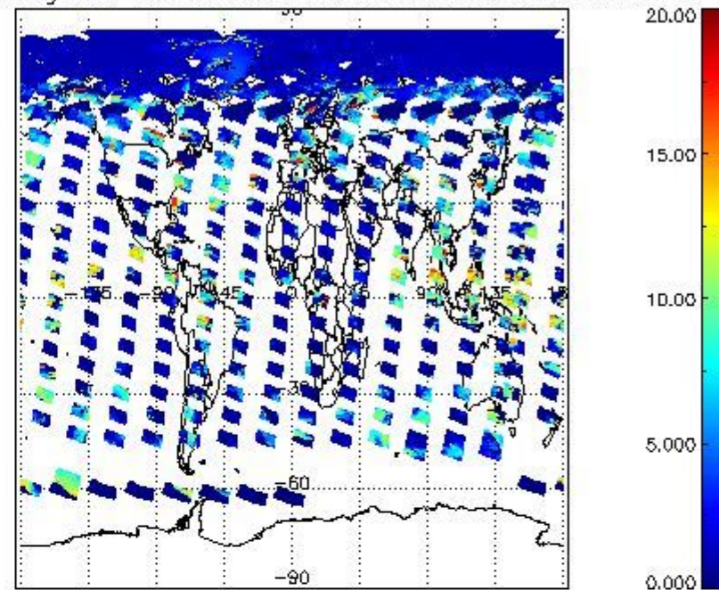
cL_top_height for 31MAY2004 00:00:00 to 01JUN2004 00:00:00
