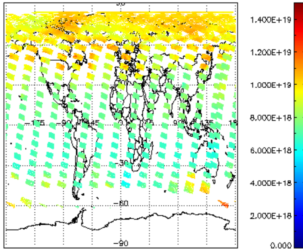
SCIOL2P_NADUV003_vcd for 31MAY2004 00:00:00 to 01JUN2004 00:00:00
