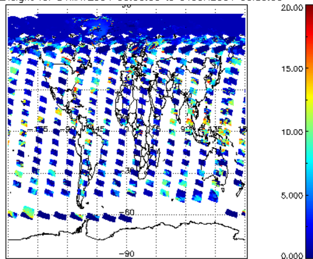
cl_top_height for 31MAY2004 00:00:00 to 01JUN2004 00:00:00
