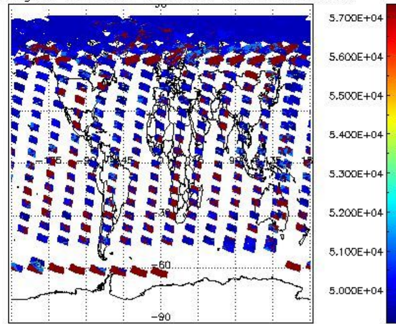
cloud_flags for 31MAY2004 00:00:00 to 01JUN2004 00:00:00
