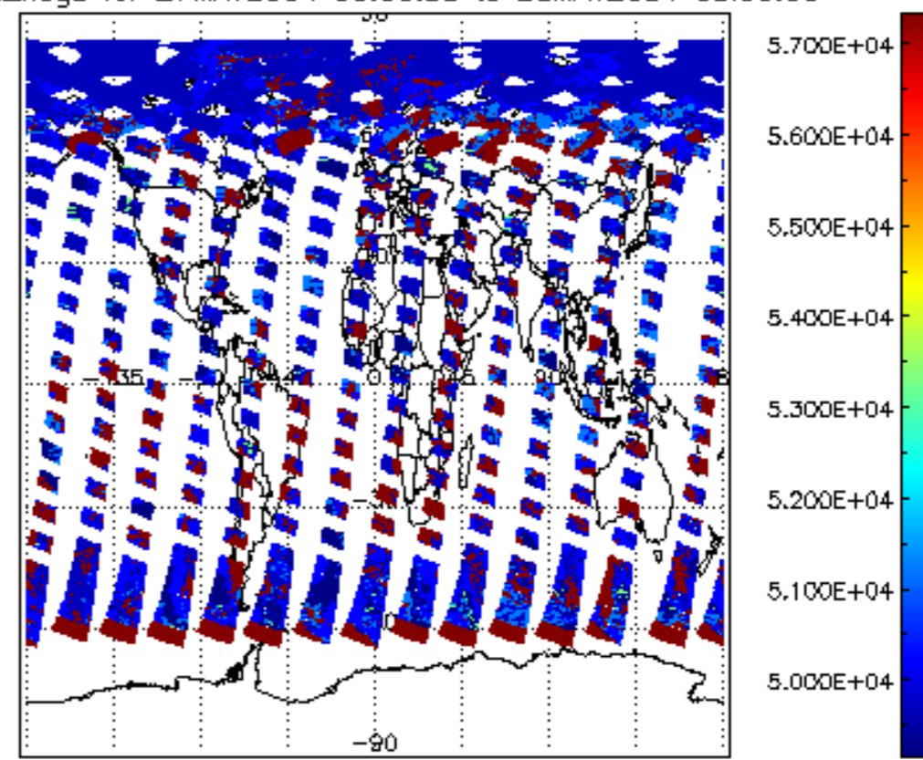
cloud_flags for 27MAY2004 00:00:00 to 28MAY2004 00:00:00
