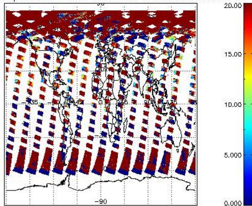
cL_opt_depth for 27MAY2004 00:00:00 to 28MAY2004 00:00:00
