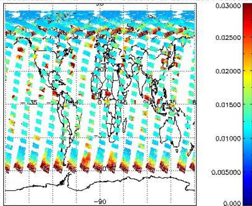
SCIOL2P_NADUV003_vcd_err for 27MAY2004 00:00:00 to 28MAY2004 00:00:00
