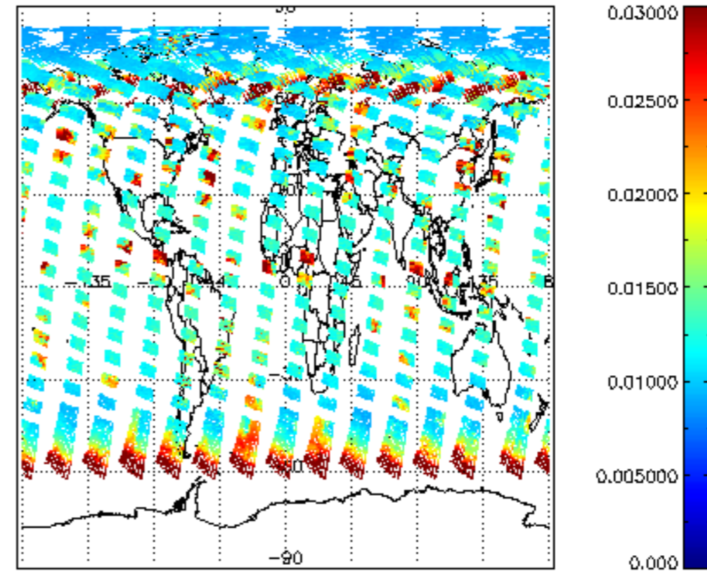
SCIOL2P_NADUV003_vcd_err for 27MAY2004 00:00:00 to 28MAY2004 00:00:00
