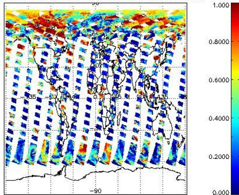
cL_frac for 27MAY2004 00:00:00 to 28MAY2004 00:00:00
