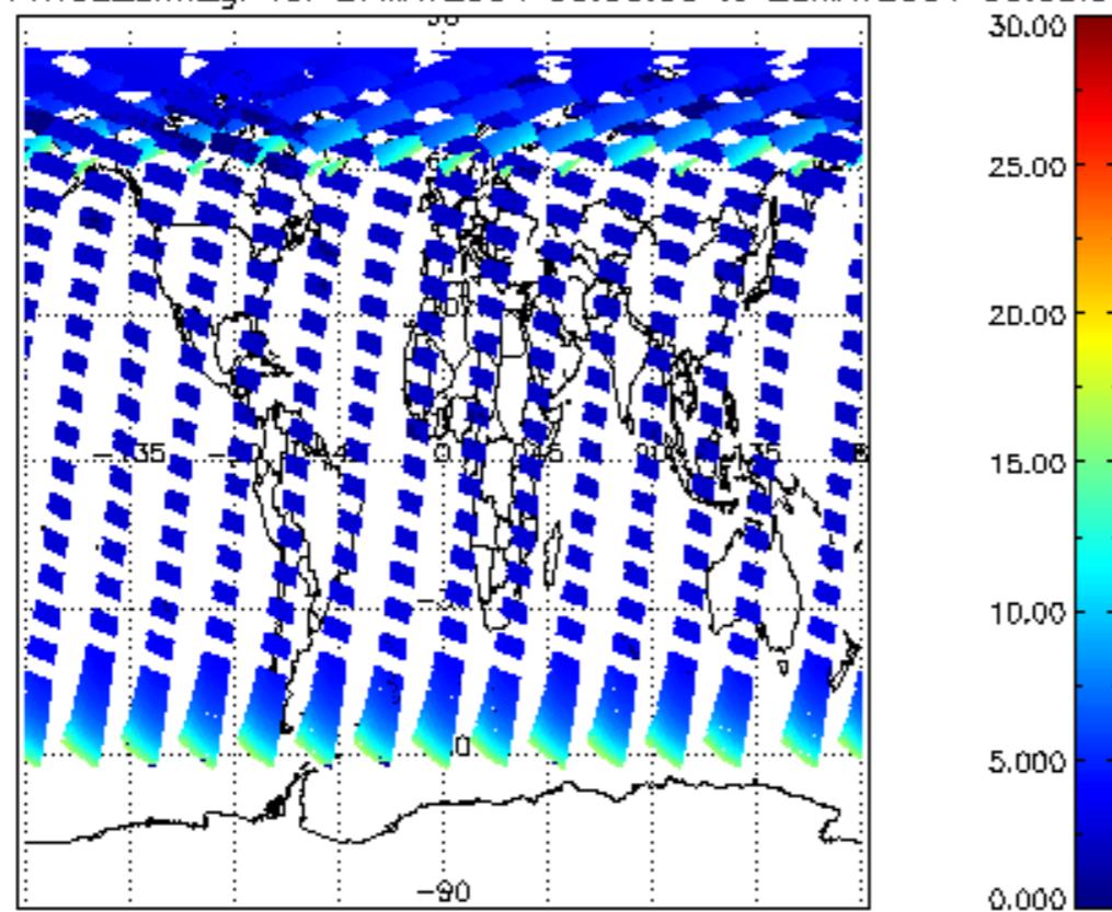
iCIOL2P_NADUV1NO2_amf_gr for 27MAY2004 00:00:00 to 28MAY2004 00:00:00
