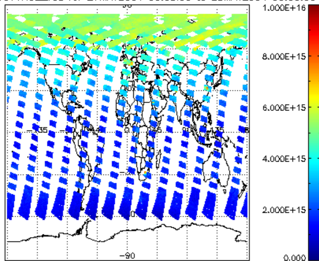
SCIOL2P_NADUV1NO2_vcd for 27MAY2004 00:00:00 to 28MAY2004 00:00:00
