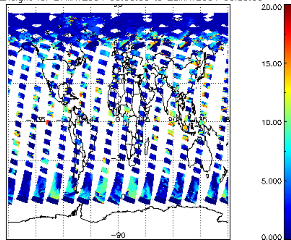
cl_top_height for 27MAY2004 00:00:00 to 28MAY2004 00:00:00
