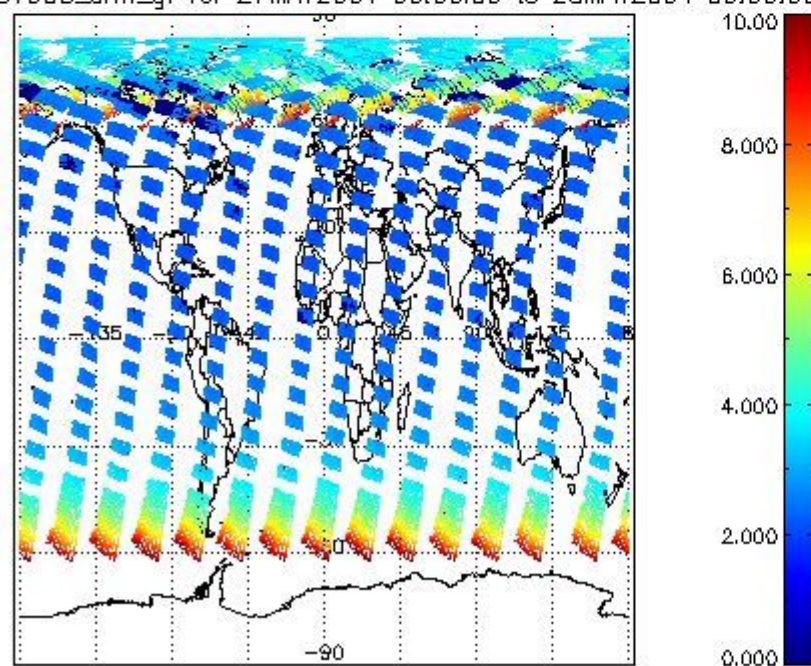
SCIOL2P_NADUV003_amf_gr for 27MAY2004 00:00:00 to 28MAY2004 00:00:00
