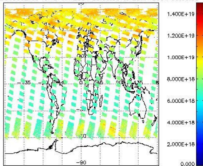
SCIOL2P_NADUV003_vcd for 27MAY2004 00:00:00 to 28MAY2004 00:00:00
