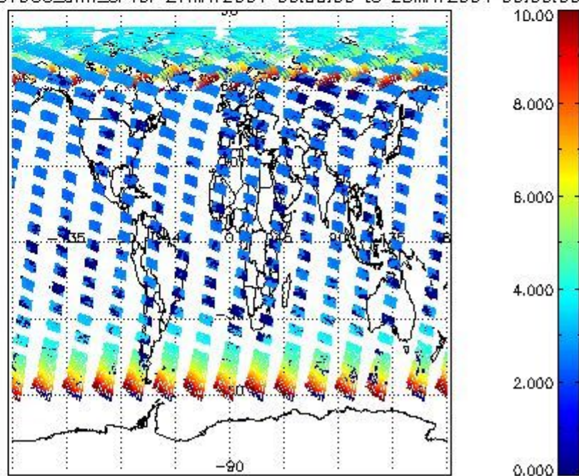
SCIOL2P_NADUV003_amf_cl for 27MAY2004 00:00:00 to 28MAY2004 00:00:00
