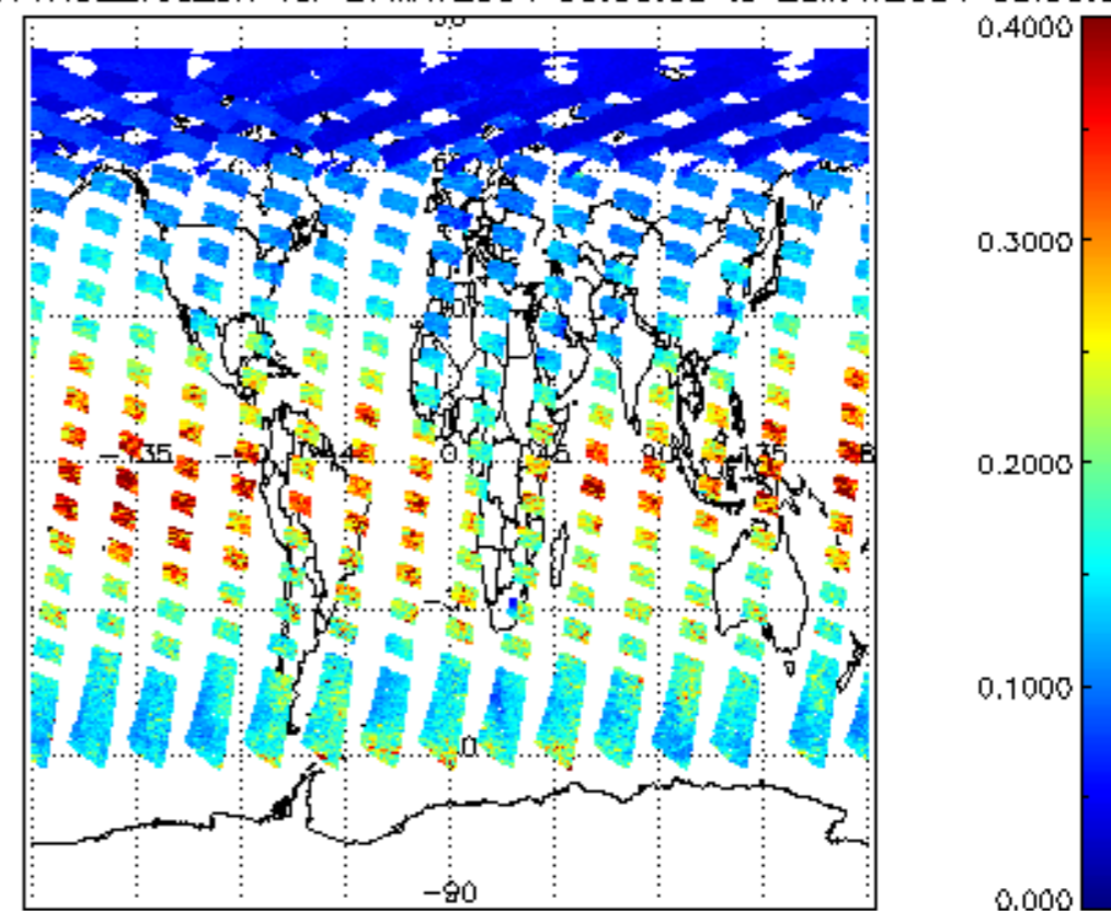
iCIOL2P_NADUV1NO2_vcd_err for 27MAY2004 00:00:00 to 28MAY2004 00:00:00
