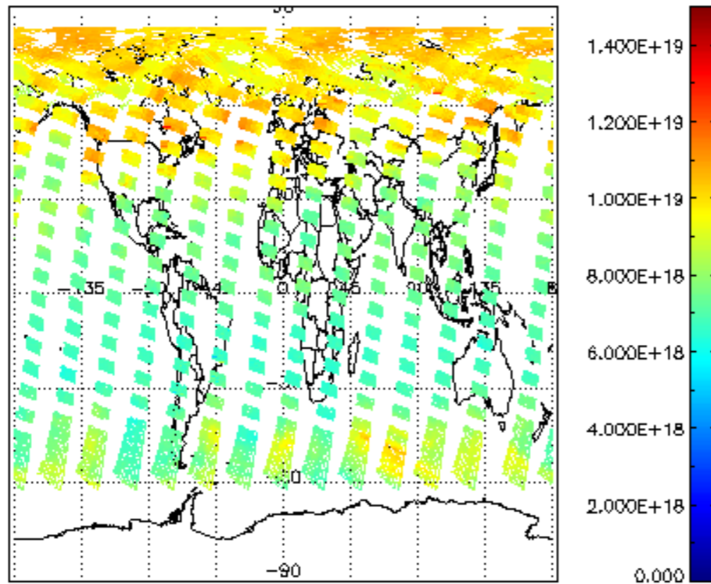
SCIOL2P_NADUV003_vcd for 27MAY2004 00:00:00 to 28MAY2004 00:00:00
