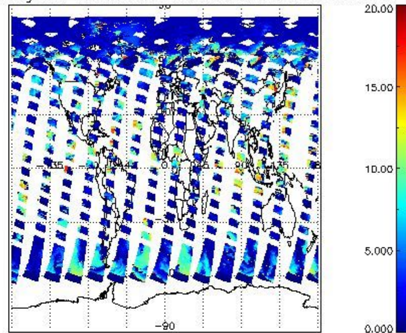
cL_top_height for 27MAY2004 00:00:00 to 28MAY2004 00:00:00
