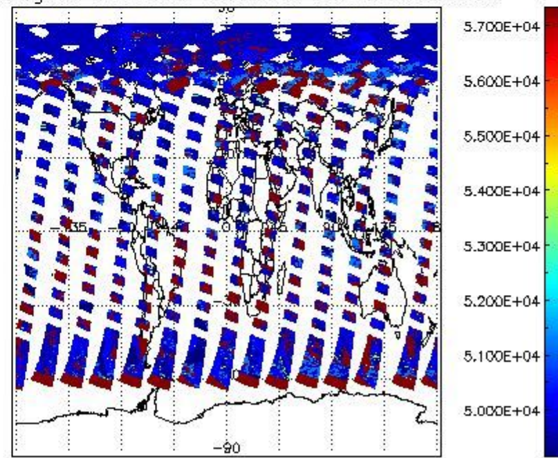
cloud_flags for 27MAY2004 00:00:00 to 28MAY2004 00:00:00
