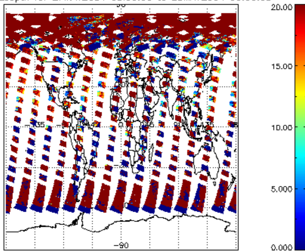
cl_opt_depth for 27MAY2004 00:00:00 to 28MAY2004 00:00:00
