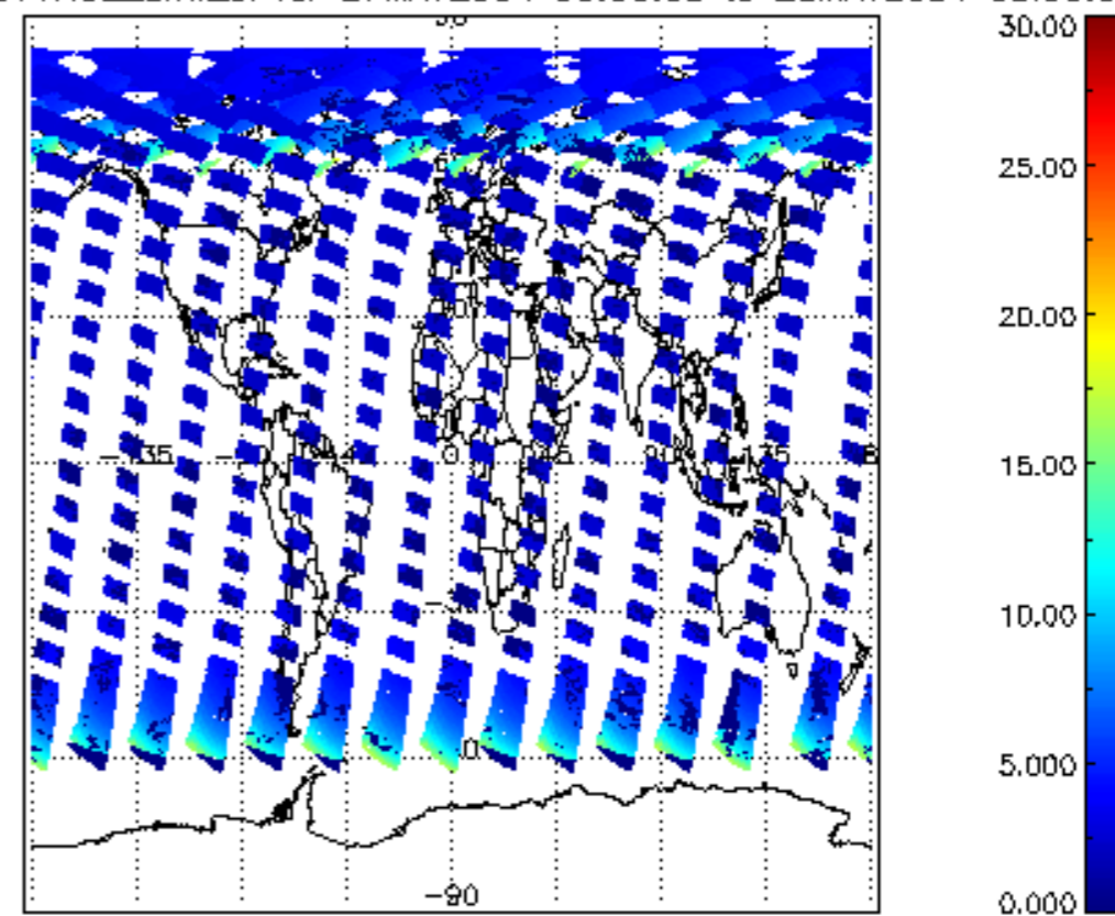
iCIOL2P_NADUV1NO2_amf_cl for 27MAY2004 00:00:00 to 28MAY2004 00:00:00
