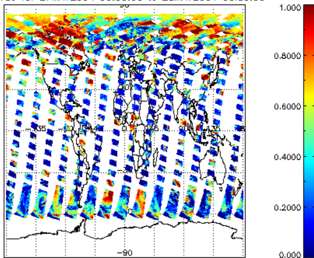
cl_frac for 27MAY2004 00:00:00 to 28MAY2004 00:00:00
