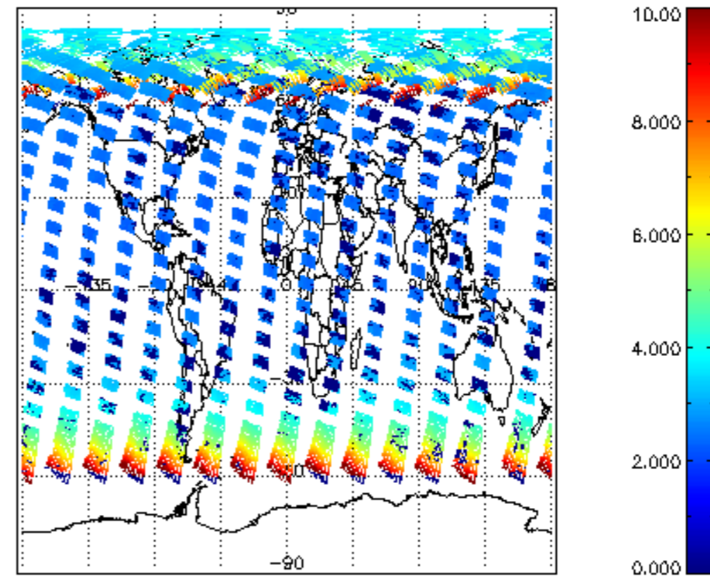
SCIOL2P_NADUV003_amf_cl for 27MAY2004 00:00:00 to 28MAY2004 00:00:00
