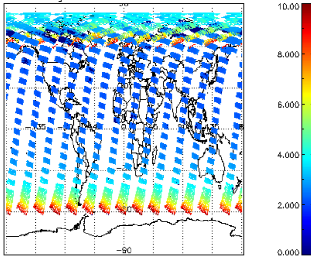
SCIOL2P_NADUV003_amf_gr for 27MAY2004 00:00:00 to 28MAY2004 00:00:00
