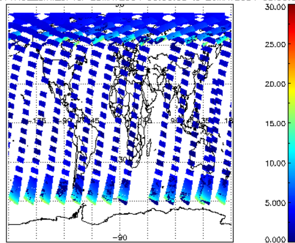
iCIOL2P_NADUV1NO2_amf_cl for 25MAY2004 00:00:00 to 26MAY2004 00:00:00
