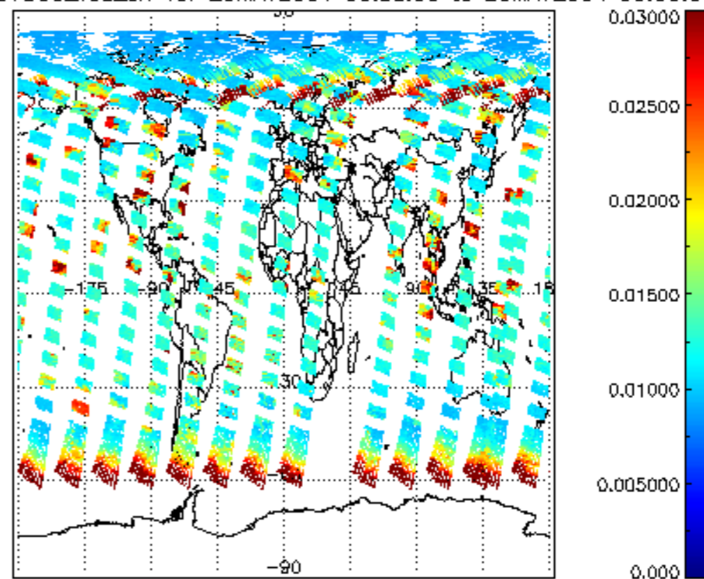
SCIOL2P_NADUV003_vcd_err for 25MAY2004 00:00:00 to 26MAY2004 00:00:00
