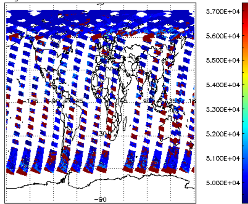
cloud_flags for 25MAY2004 00:00:00 to 26MAY2004 00:00:00
