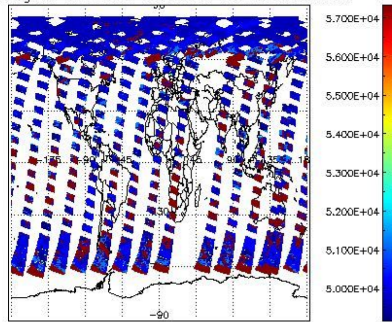
cloud_flags for 25MAY2004 00:00:00 to 26MAY2004 00:00:00
