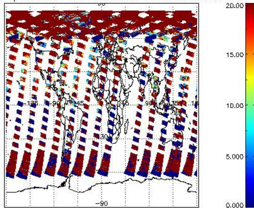
cL_opt_depth for 25MAY2004 00:00:00 to 26MAY2004 00:00:00
