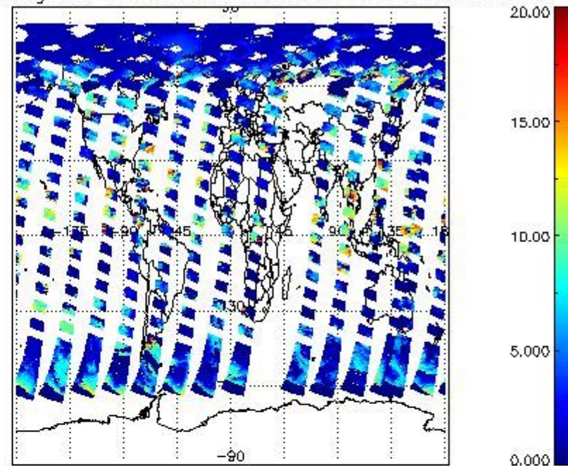
cL_top_height for 25MAY2004 00:00:00 to 26MAY2004 00:00:00
