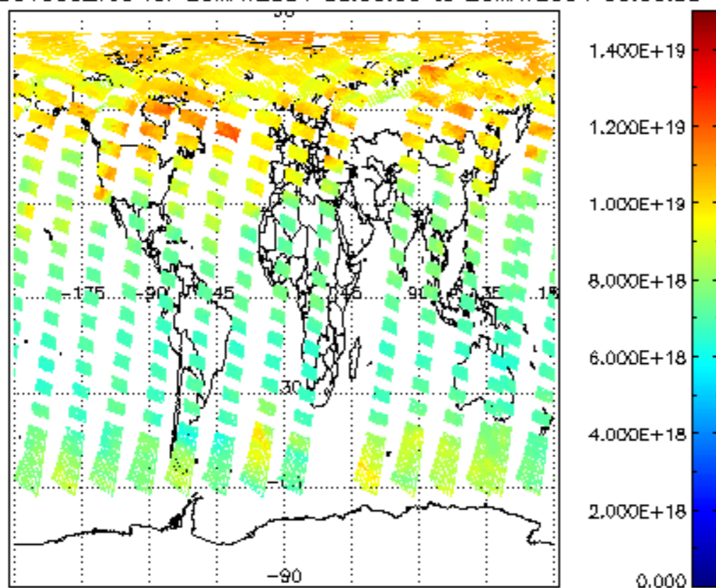
SCIOL2P_NADUV003_vcd for 25MAY2004 00:00:00 to 26MAY2004 00:00:00
