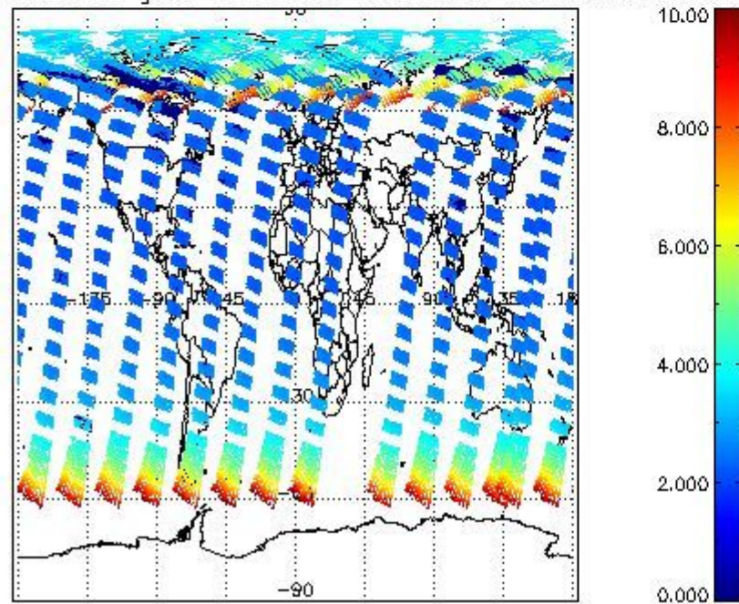
SCIOL2P_NADUV003_amf_gr for 25MAY2004 00:00:00 to 26MAY2004 00:00:00
