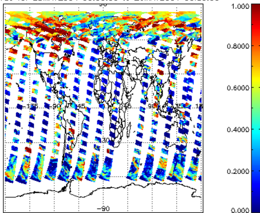
cl_frac for 25MAY2004 00:00:00 to 26MAY2004 00:00:00
