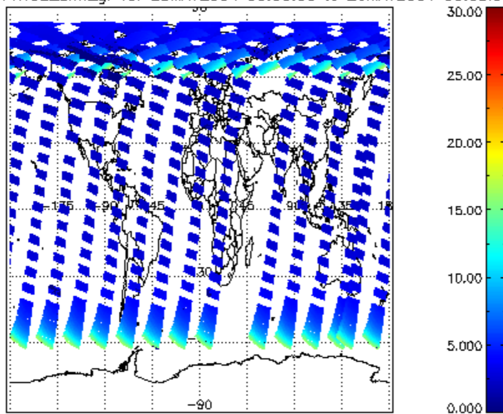
iCIOL2P_NADUV1NO2_amf_gr for 25MAY2004 00:00:00 to 26MAY2004 00:00:00
