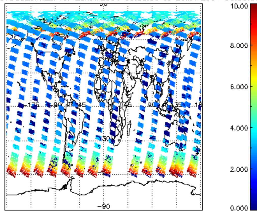
SCIOL2P_NADUV003_amf_cl for 25MAY2004 00:00:00 to 26MAY2004 00:00:00
