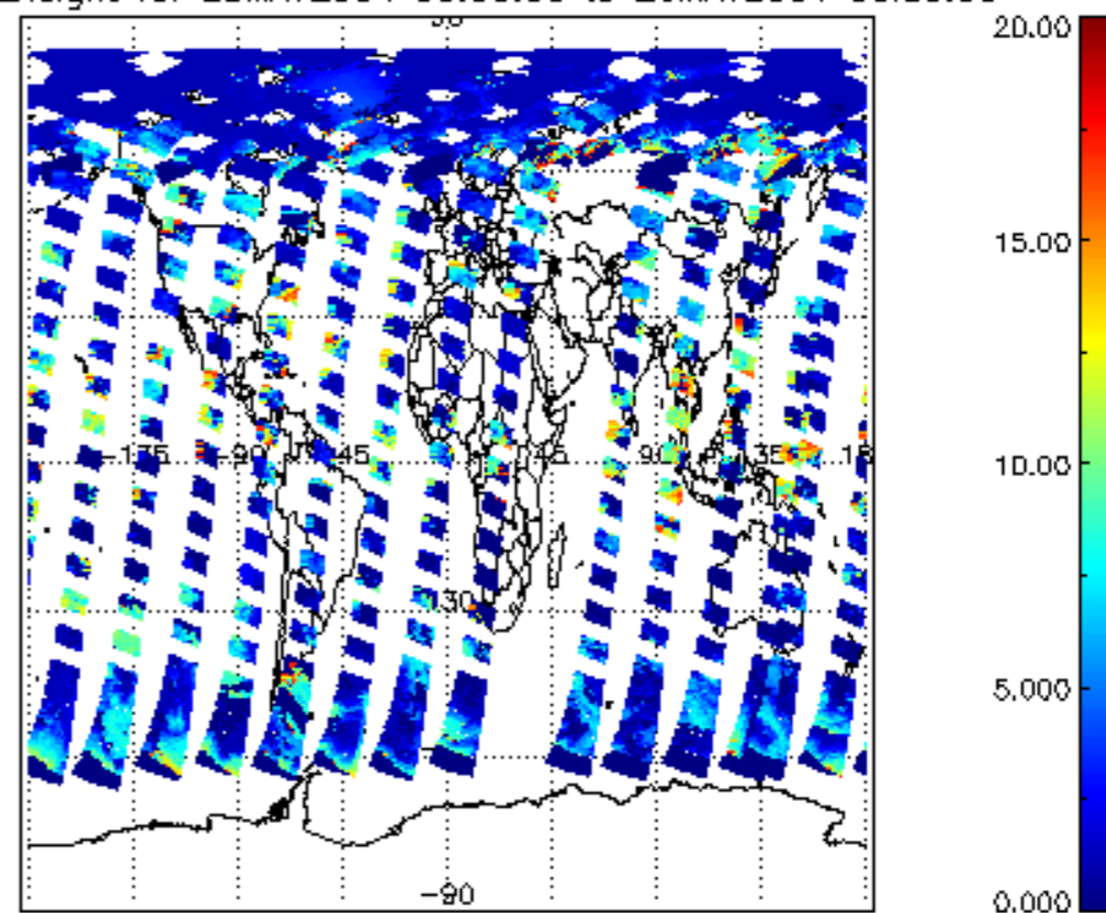
cl_top_height for 25MAY2004 00:00:00 to 26MAY2004 00:00:00
