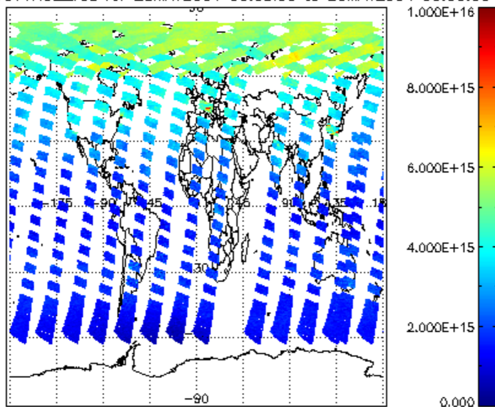
SCIOL2P_NADUV1NO2_vcd for 25MAY2004 00:00:00 to 26MAY2004 00:00:00
