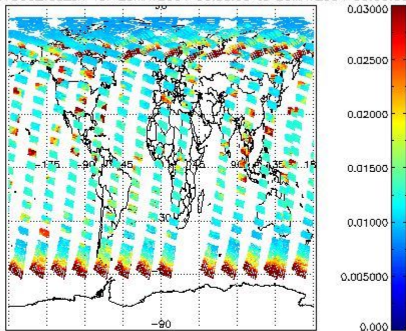
SCIOL2P_NADUV003_vcd_err for 25MAY2004 00:00:00 to 26MAY2004 00:00:00
