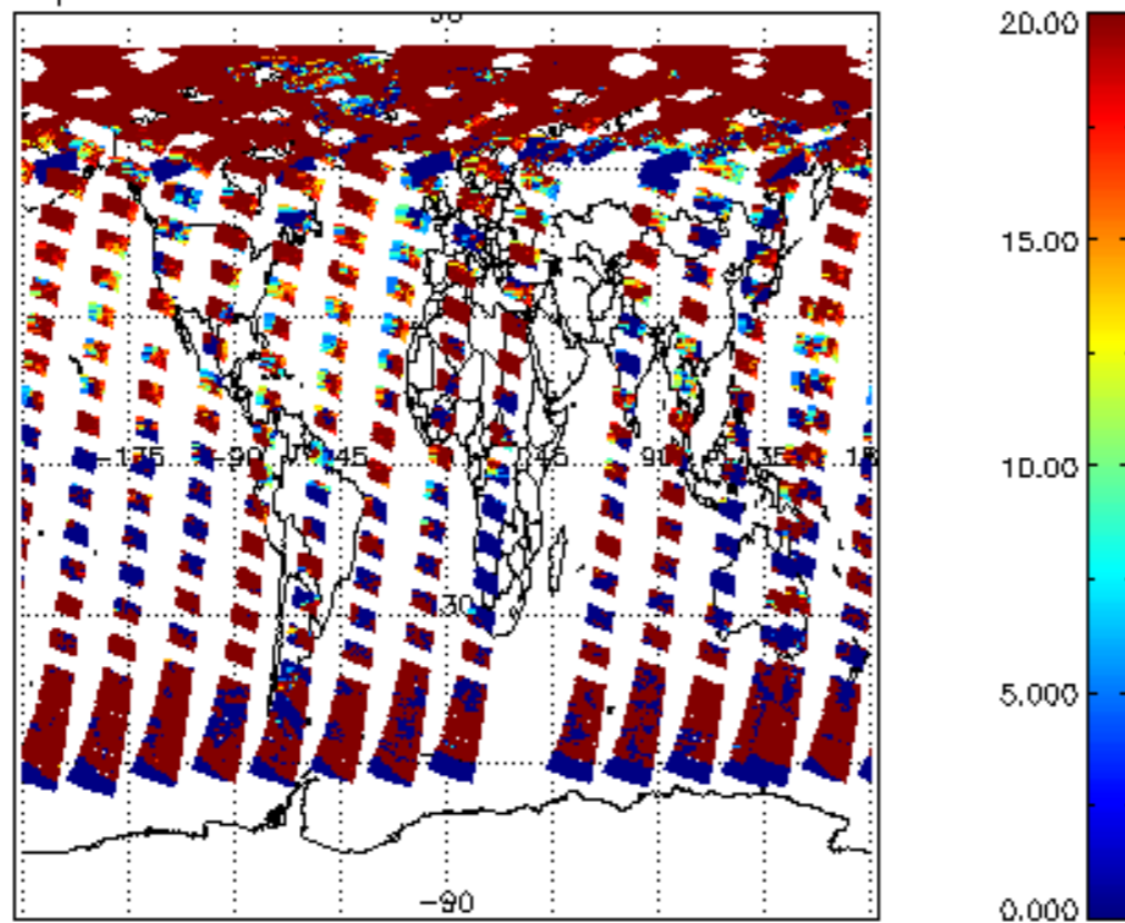
cl_opt_depth for 25MAY2004 00:00:00 to 26MAY2004 00:00:00
