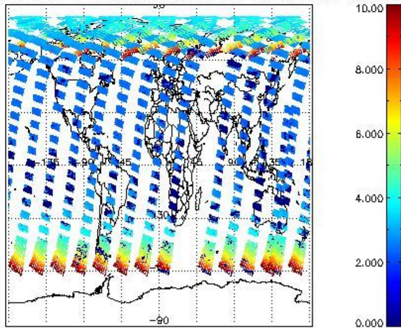
SCIOL2P_NADUV003_amf_cl for 25MAY2004 00:00:00 to 26MAY2004 00:00:00
