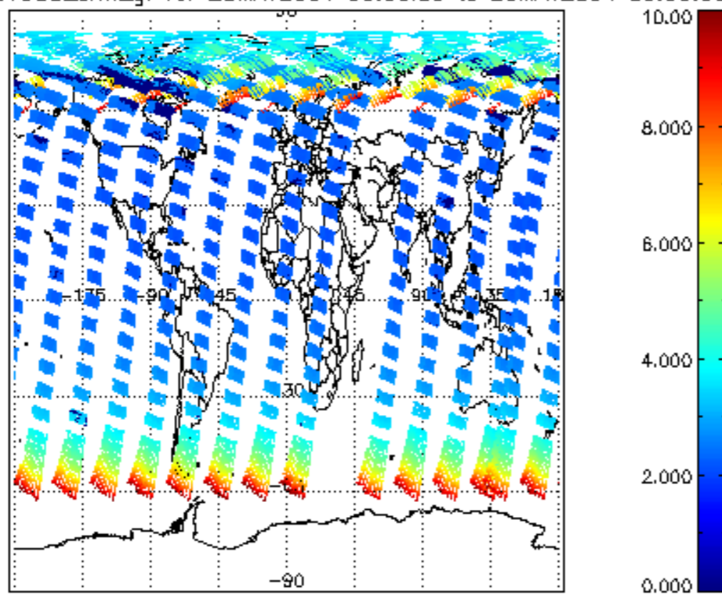
SCIOL2P_NADUV003_amf_gr for 25MAY2004 00:00:00 to 26MAY2004 00:00:00
