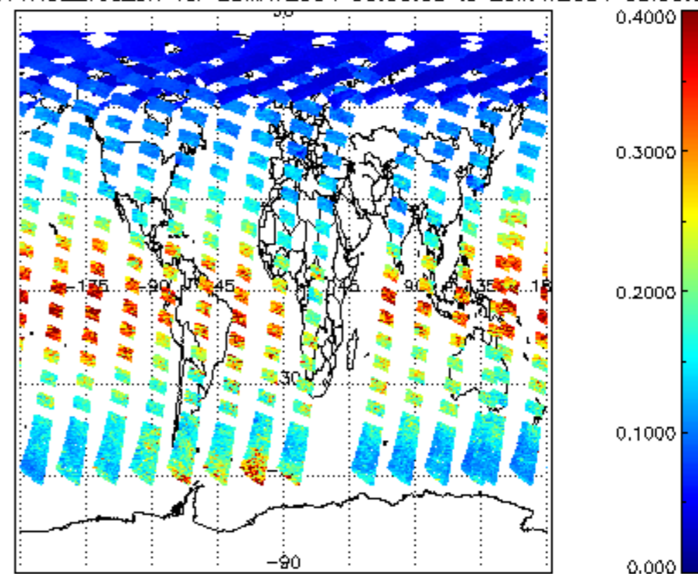
iCIOL2P_NADUV1NO2_vcd_err for 25MAY2004 00:00:00 to 26MAY2004 00:00:00
