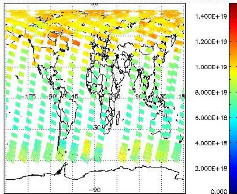
SCIOL2P_NADUV003_vcd for 25MAY2004 00:00:00 to 26MAY2004 00:00:00
