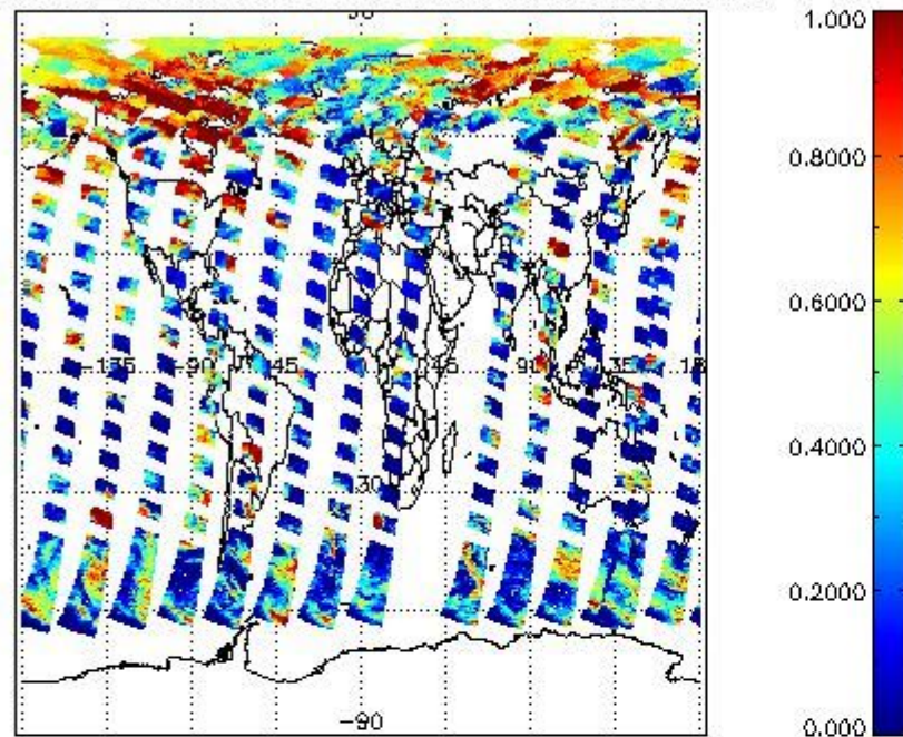
cL_frac for 25MAY2004 00:00:00 to 26MAY2004 00:00:00
