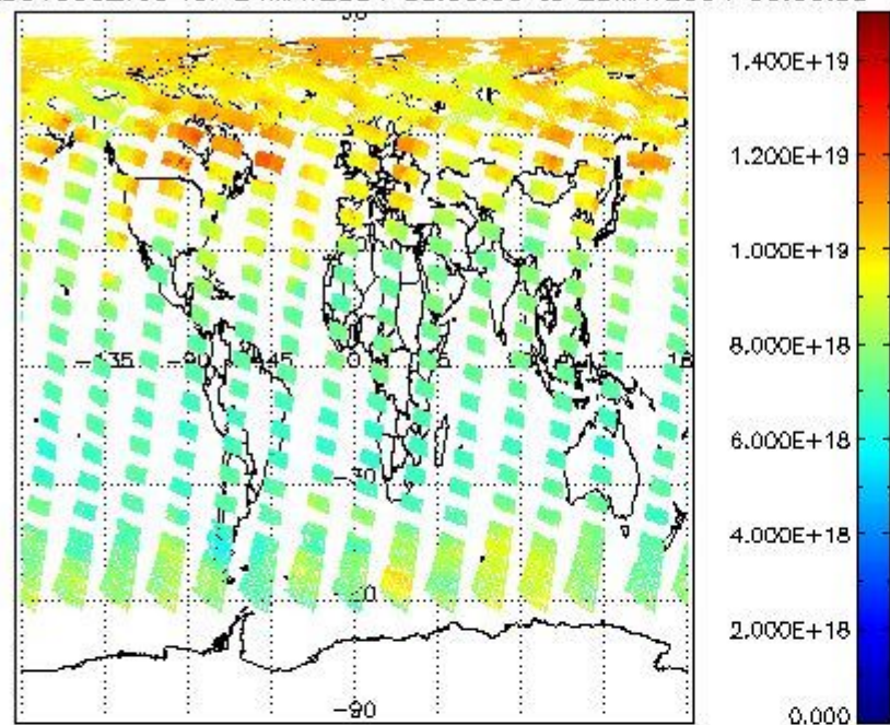
SCIOL2P_NADUV003_vcd for 24MAY2004 00:00:00 to 25MAY2004 00:00:00
