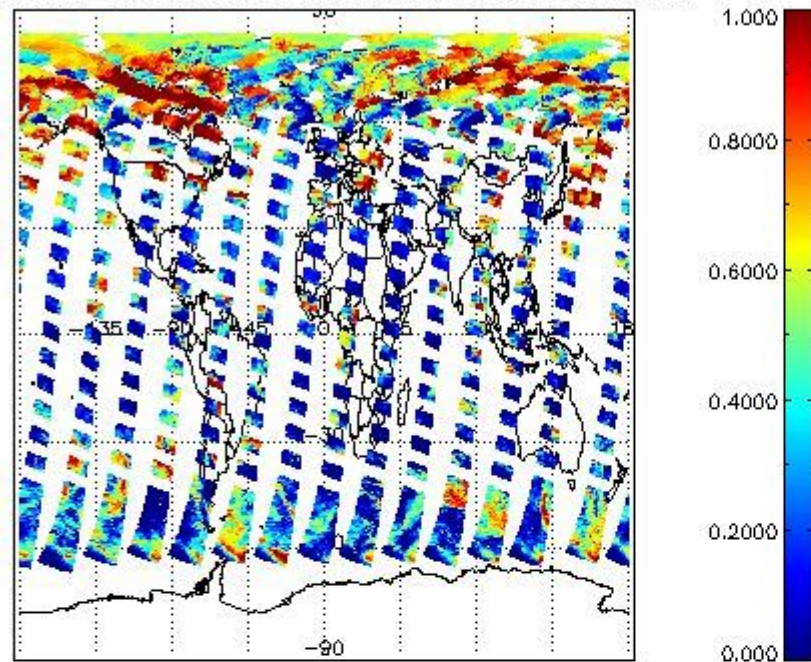
cL_frac for 24MAY2004 00:00:00 to 25MAY2004 00:00:00
