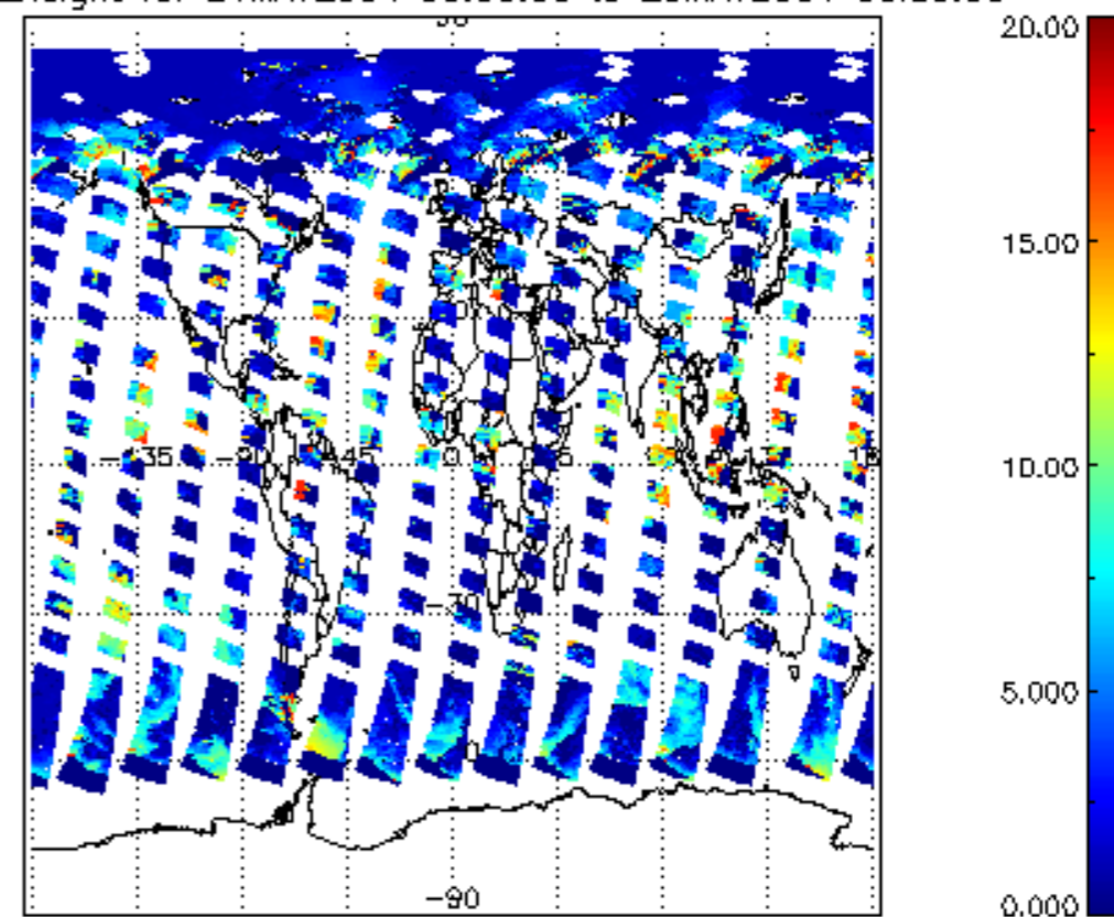
cl_top_height for 24MAY2004 00:00:00 to 25MAY2004 00:00:00
