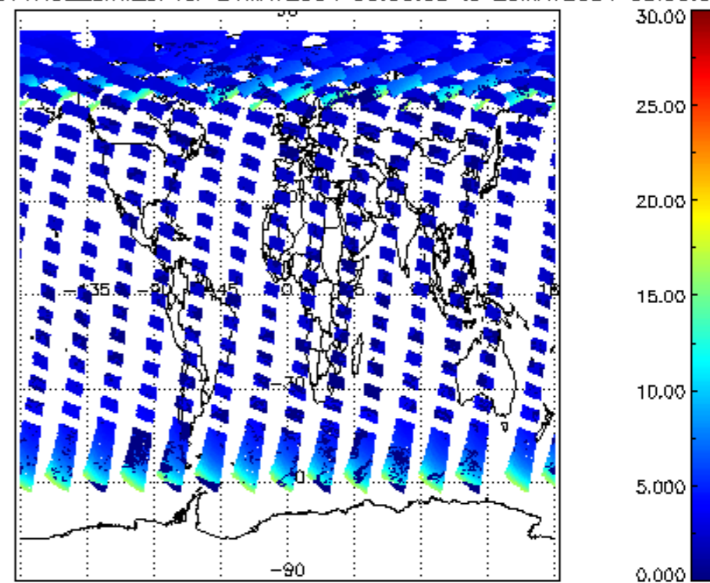
iCIOL2P_NADUV1NO2_amf_cl for 24MAY2004 00:00:00 to 25MAY2004 00:00:00
