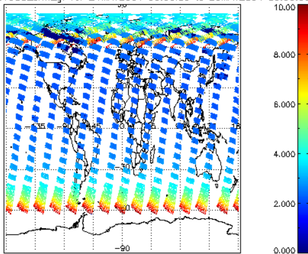
SCIOL2P_NADUV003_amf_gr for 24MAY2004 00:00:00 to 25MAY2004 00:00:00
