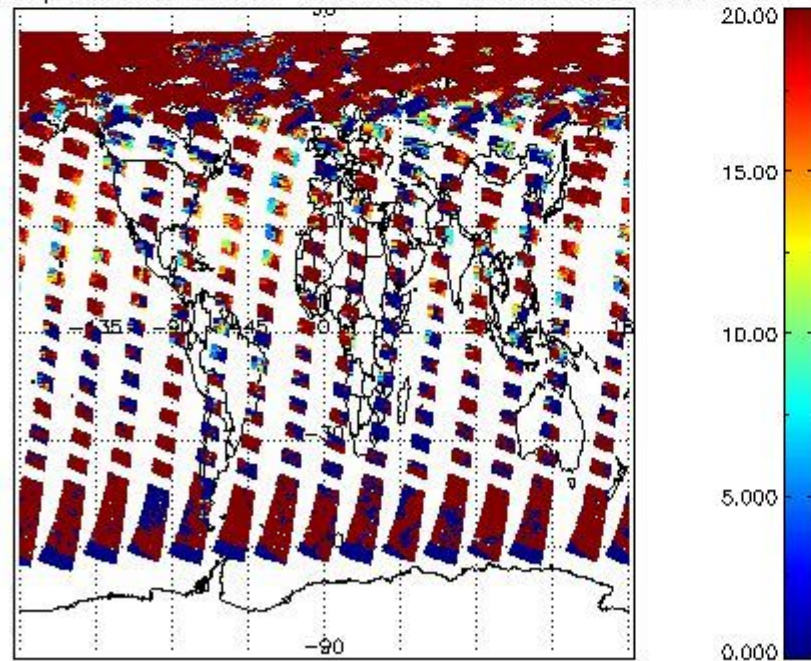
cL_opt_depth for 24MAY2004 00:00:00 to 25MAY2004 00:00:00
