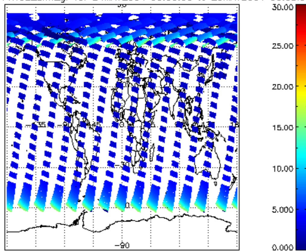
iCIOL2P_NADUV1NO2_amf_gr for 24MAY2004 00:00:00 to 25MAY2004 00:00:00
