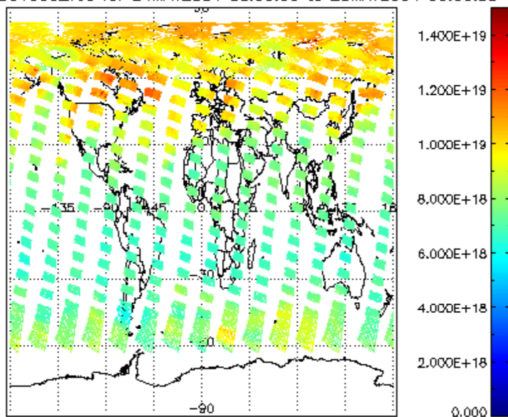
SCIOL2P_NADUV003_vcd for 24MAY2004 00:00:00 to 25MAY2004 00:00:00
