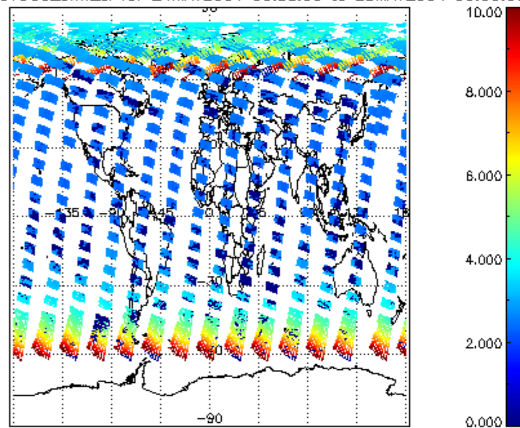
SCIOL2P_NADUV003_amf_cl for 24MAY2004 00:00:00 to 25MAY2004 00:00:00
