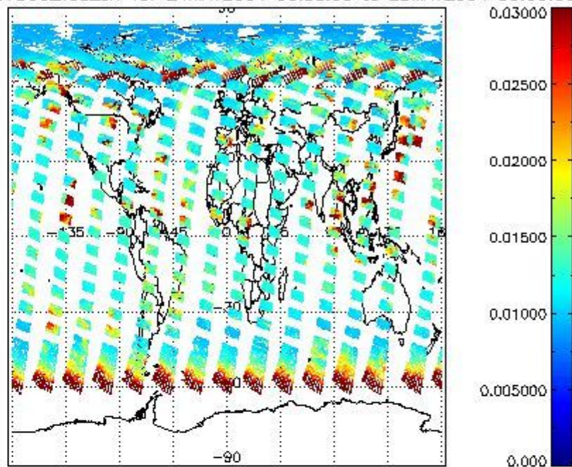
SCIOL2P_NADUV003_vcd_err for 24MAY2004 00:00:00 to 25MAY2004 00:00:00
