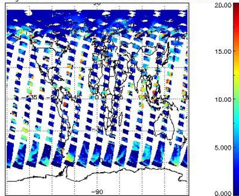
cL_top_height for 24MAY2004 00:00:00 to 25MAY2004 00:00:00
