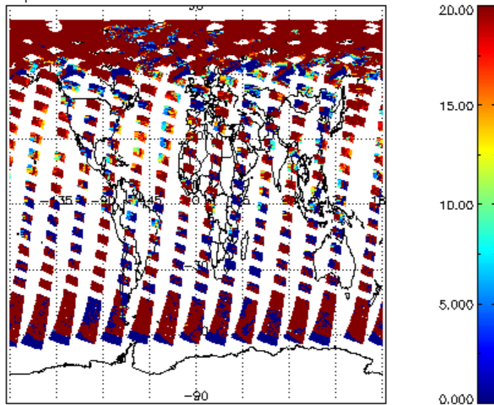
cl_opt_depth for 24MAY2004 00:00:00 to 25MAY2004 00:00:00
