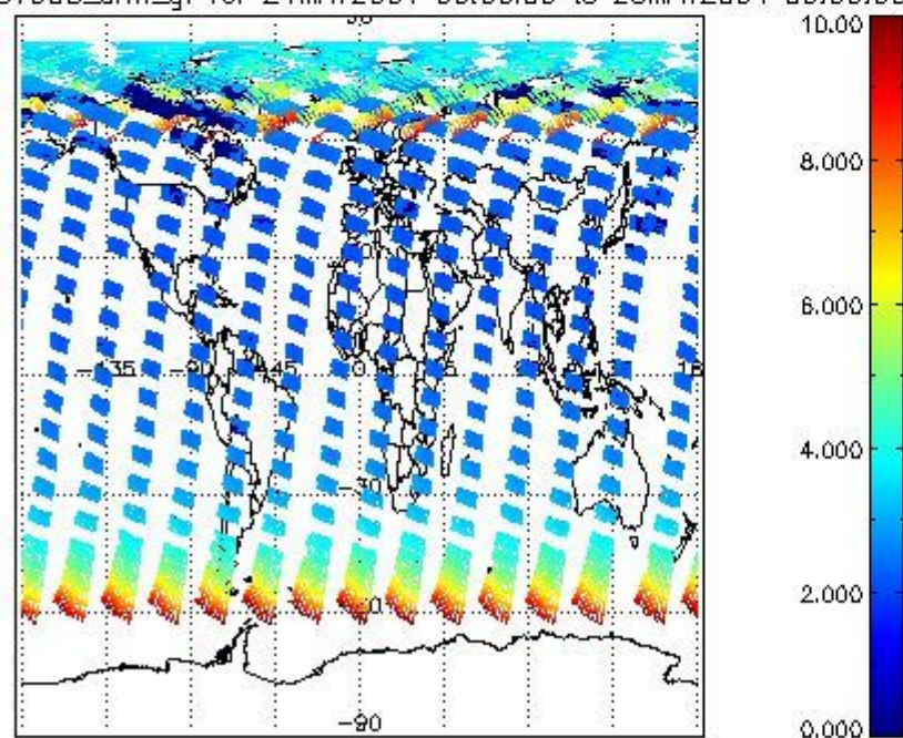
SCIOL2P_NADUV003_amf_gr for 24MAY2004 00:00:00 to 25MAY2004 00:00:00
