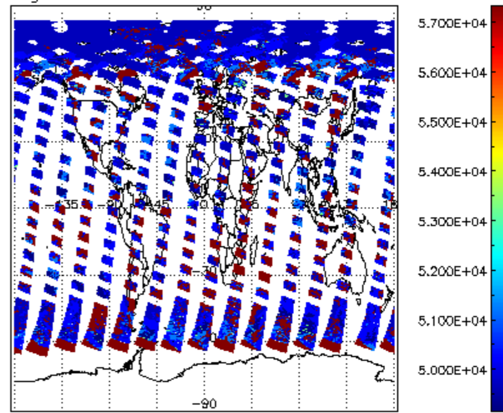
cloud_flags for 24MAY2004 00:00:00 to 25MAY2004 00:00:00
