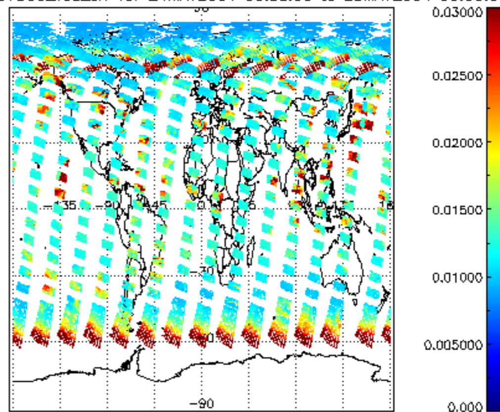
SCIOL2P_NADUV003_vcd_err for 24MAY2004 00:00:00 to 25MAY2004 00:00:00
