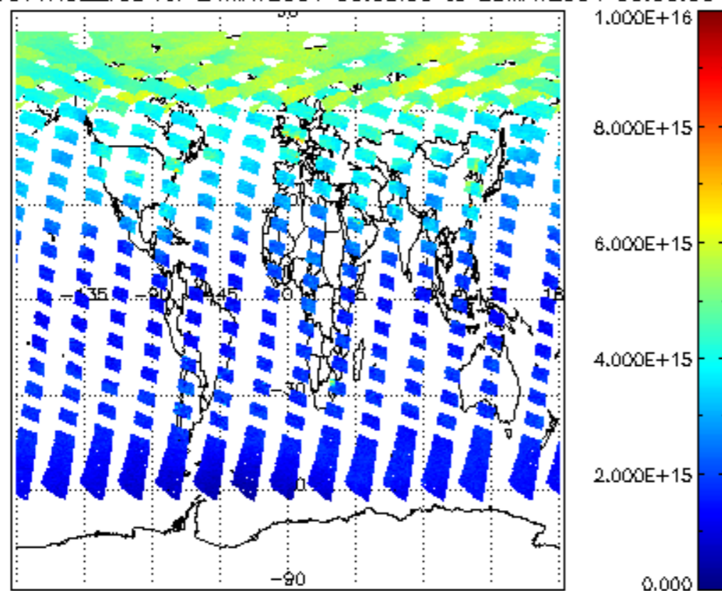
SCIOL2P_NADUV1NO2_vcd for 24MAY2004 00:00:00 to 25MAY2004 00:00:00
