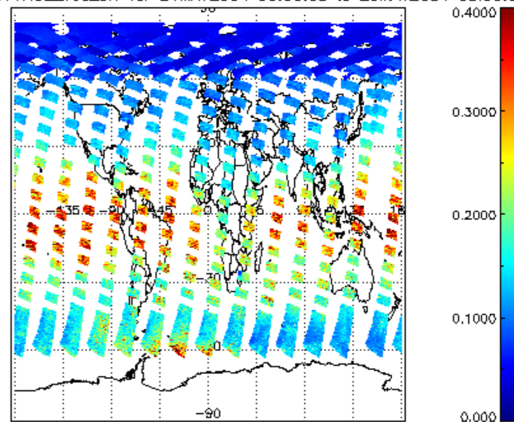
iCIOL2P_NADUV1NO2_vcd_err for 24MAY2004 00:00:00 to 25MAY2004 00:00:00
