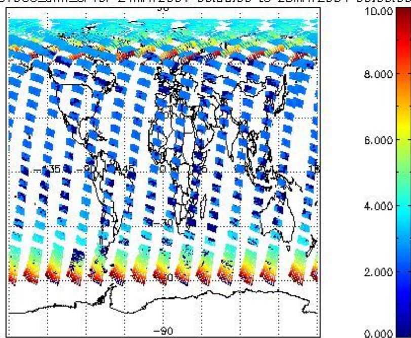
SCIOL2P_NADUV003_amf_cl for 24MAY2004 00:00:00 to 25MAY2004 00:00:00
