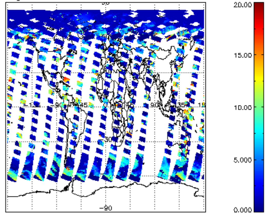
cl_top_height for 22MAY2004 00:00:00 to 23MAY2004 00:00:00
