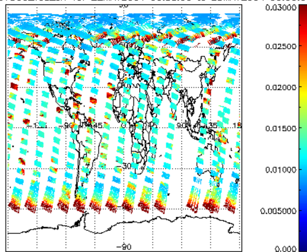
SCIOL2P_NADUV003_vcd_err for 22MAY2004 00:00:00 to 23MAY2004 00:00:00
