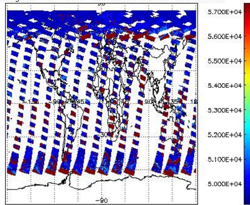
cloud_flags for 22MAY2004 00:00:00 to 23MAY2004 00:00:00
