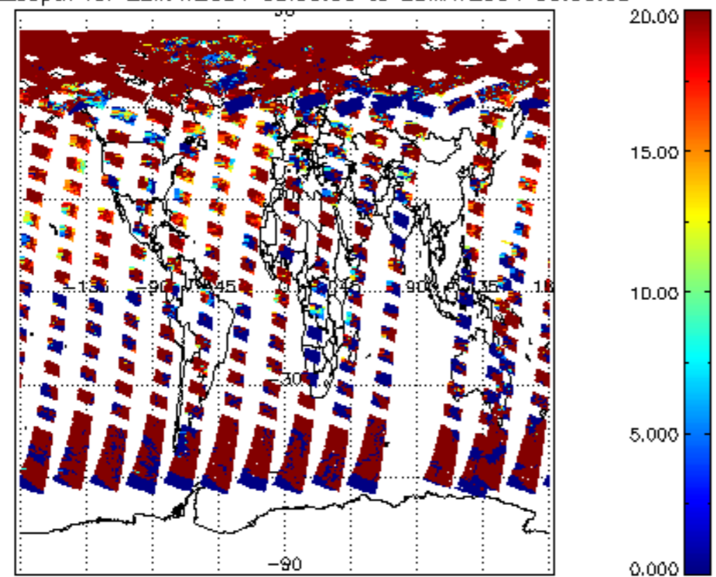
cl_opt_depth for 22MAY2004 00:00:00 to 23MAY2004 00:00:00
