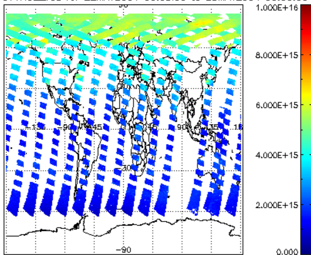
SCIOL2P_NADUV1NO2_vcd for 22MAY2004 00:00:00 to 23MAY2004 00:00:00
