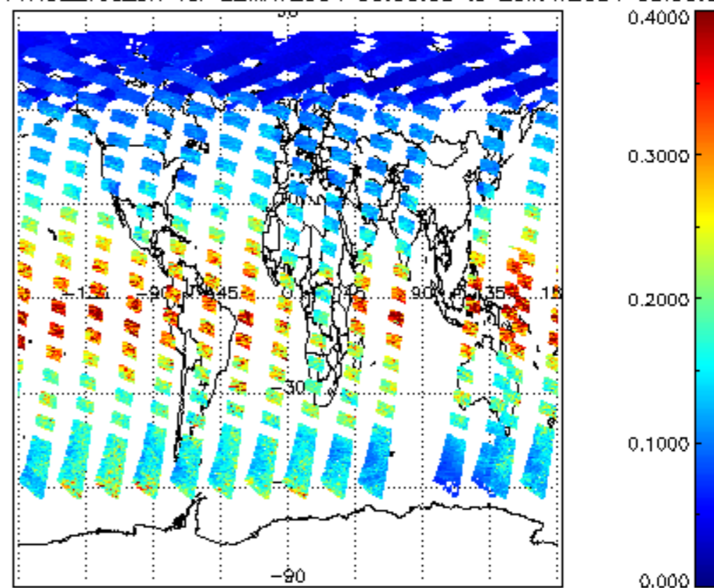
iCIOL2P_NADUV1NO2_vcd_err for 22MAY2004 00:00:00 to 23MAY2004 00:00:00
