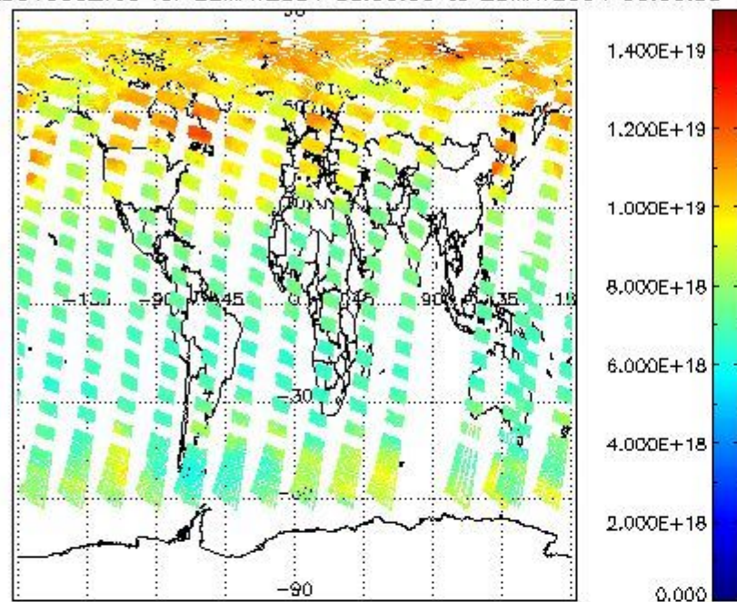
SCIOL2P_NADUV003_vcd for 22MAY2004 00:00:00 to 23MAY2004 00:00:00
