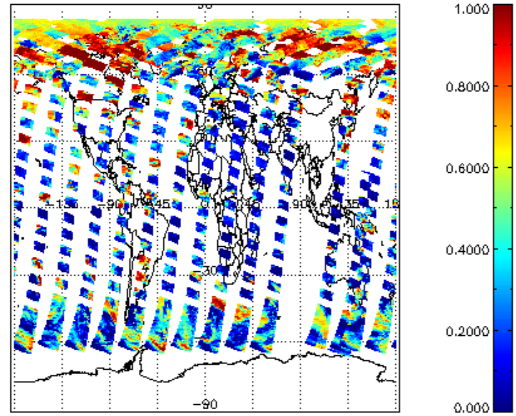
cl_frac for 22MAY2004 00:00:00 to 23MAY2004 00:00:00
