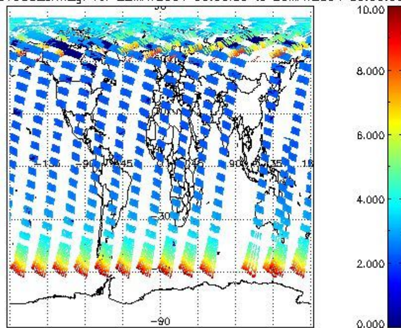
SCIOL2P_NADUV003_amf_gr for 22MAY2004 00:00:00 to 23MAY2004 00:00:00
