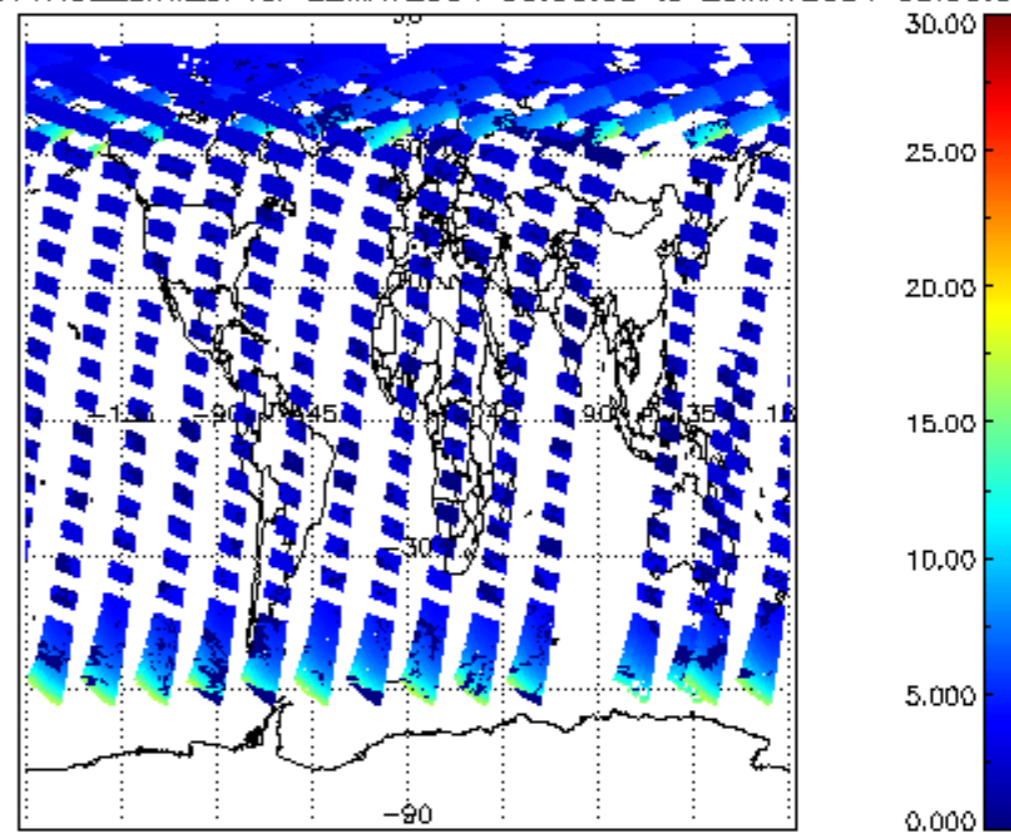
iCIOL2P_NADUV1NO2_amf_cl for 22MAY2004 00:00:00 to 23MAY2004 00:00:00
