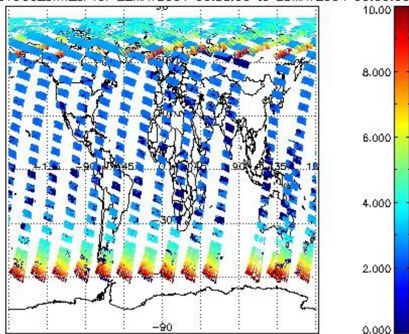
SCIOL2P_NADUV003_amf_cl for 22MAY2004 00:00:00 to 23MAY2004 00:00:00
