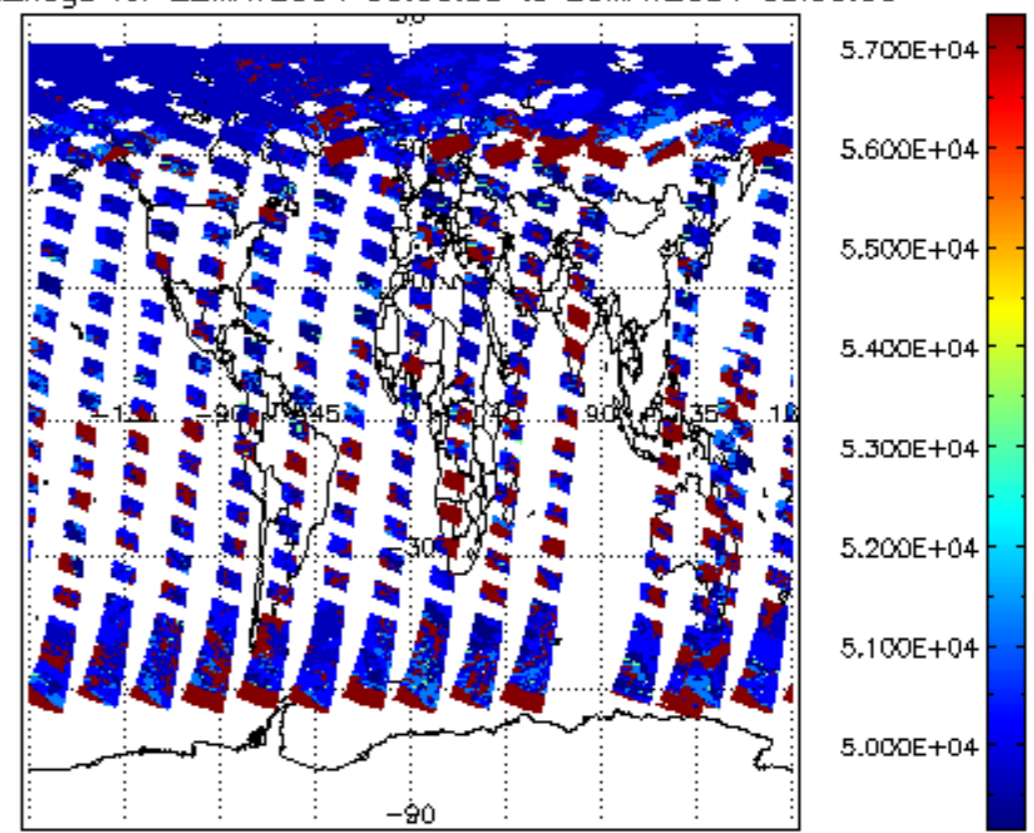
cloud_flags for 22MAY2004 00:00:00 to 23MAY2004 00:00:00
