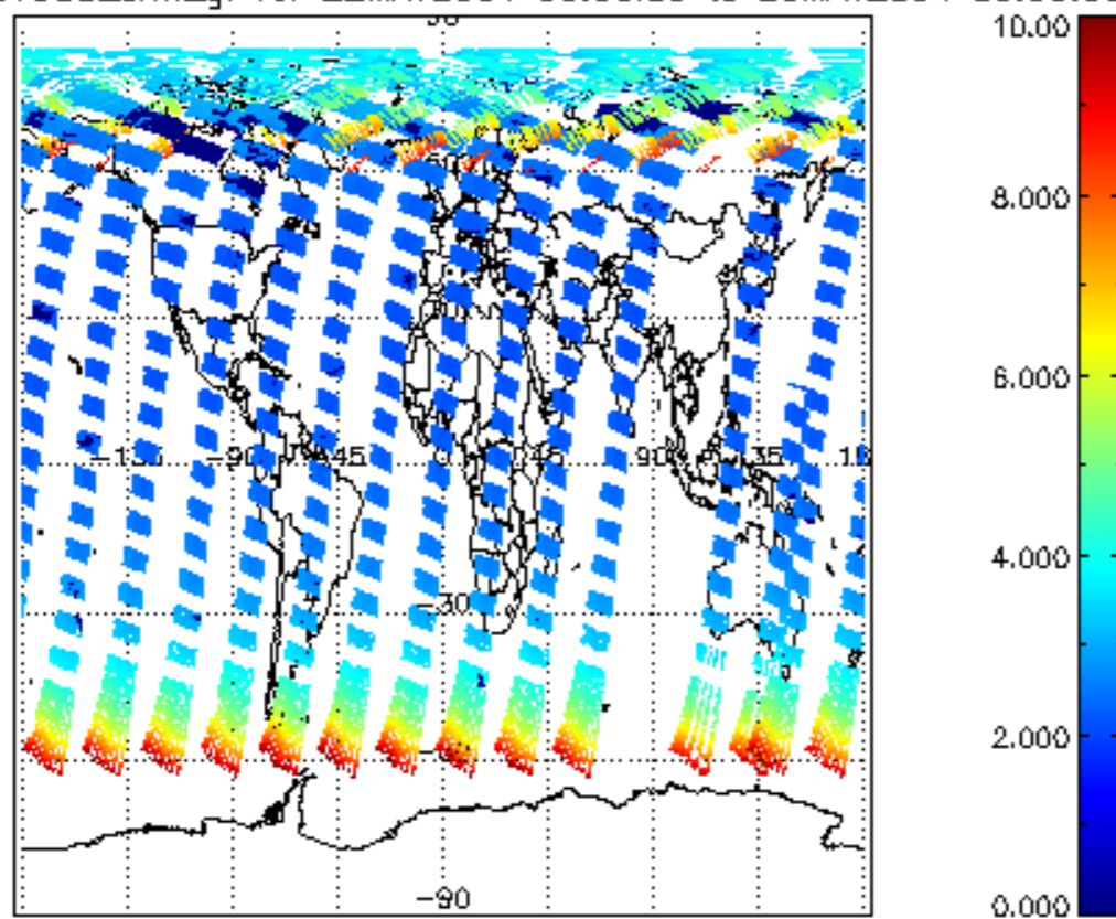
SCIOL2P_NADUV003_amf_gr for 22MAY2004 00:00:00 to 23MAY2004 00:00:00
