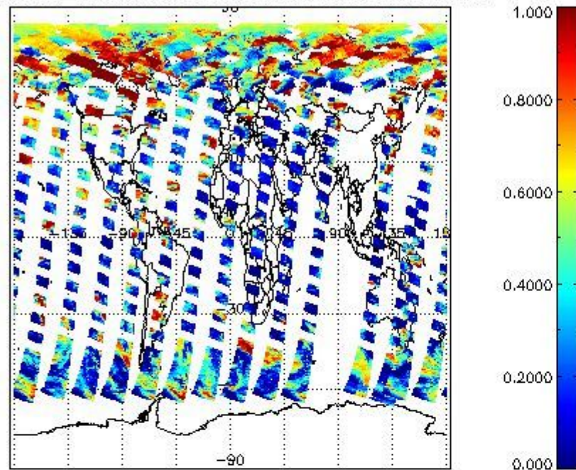
cL_frac for 22MAY2004 00:00:00 to 23MAY2004 00:00:00
