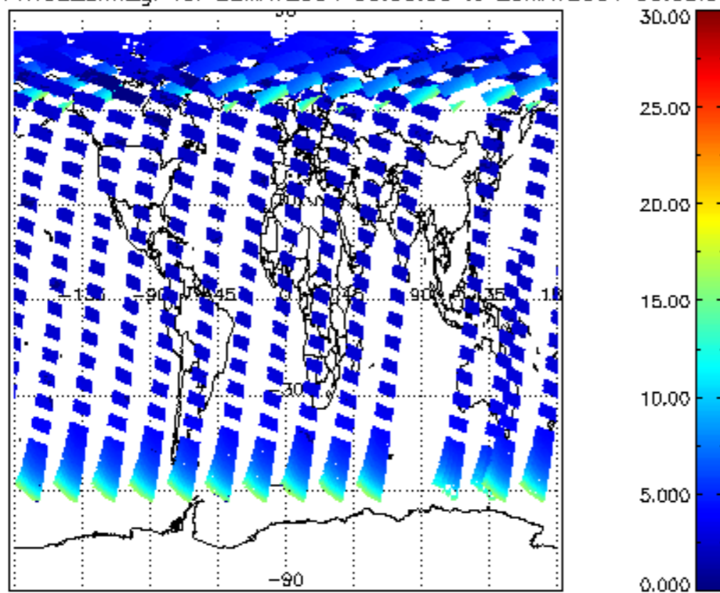
iCIOL2P_NADUV1NO2_amf_gr for 22MAY2004 00:00:00 to 23MAY2004 00:00:00
