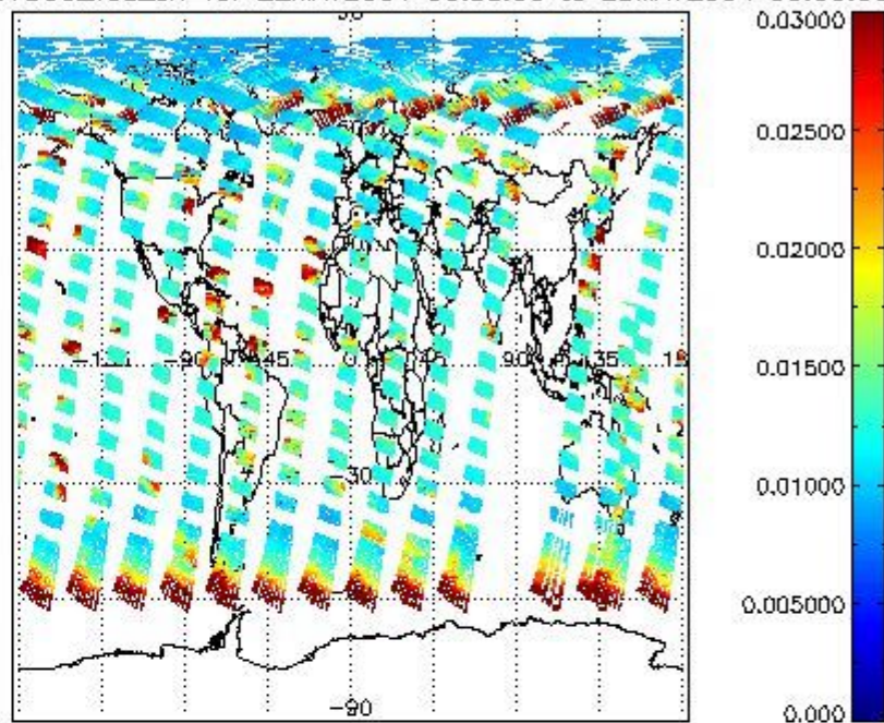
SCIOL2P_NADUV003_vcd_err for 22MAY2004 00:00:00 to 23MAY2004 00:00:00
