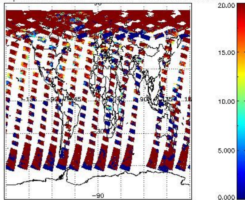
cL_opt_depth for 22MAY2004 00:00:00 to 23MAY2004 00:00:00
