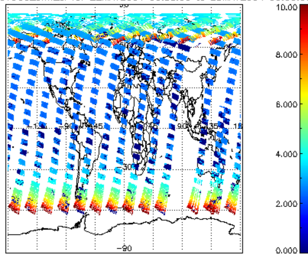
SCIOL2P_NADUV003_amf_cl for 22MAY2004 00:00:00 to 23MAY2004 00:00:00
