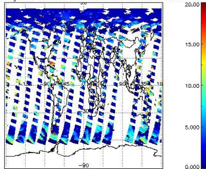
cL_top_height for 22MAY2004 00:00:00 to 23MAY2004 00:00:00
