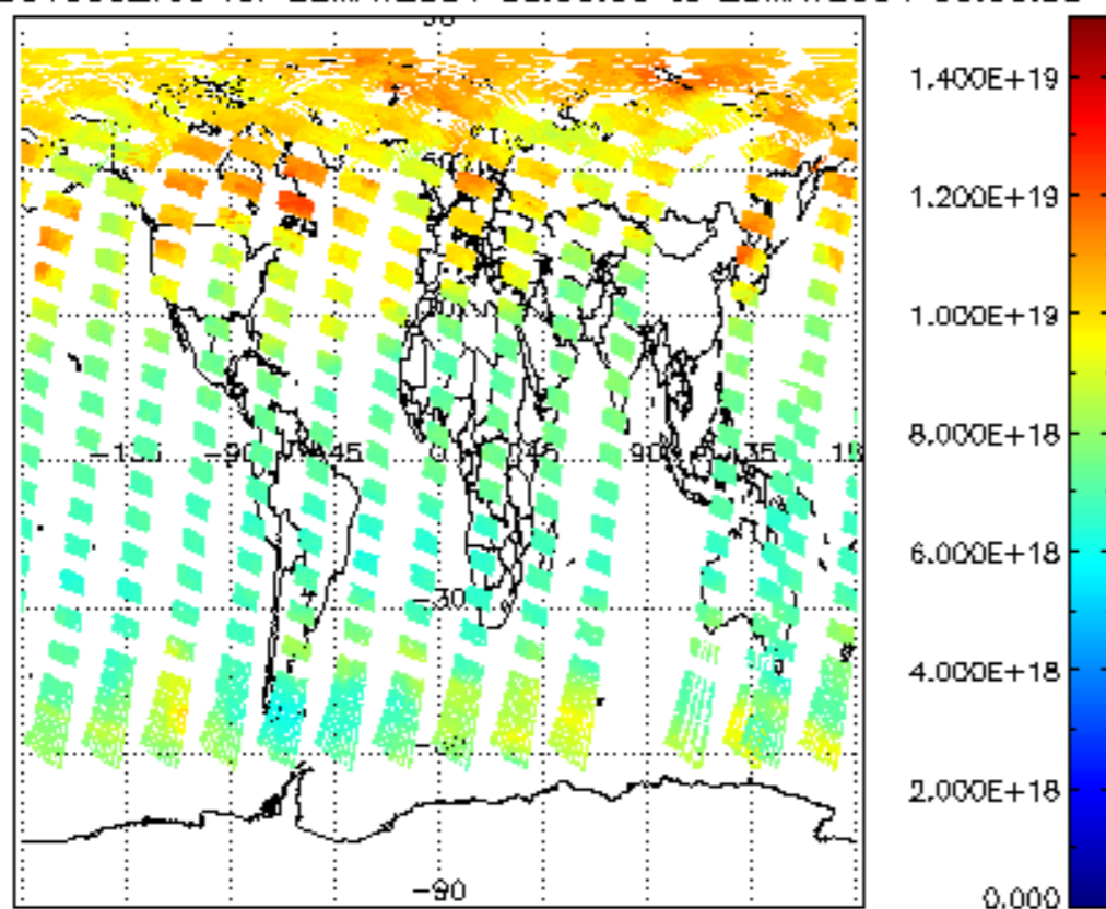
SCIOL2P_NADUV003_vcd for 22MAY2004 00:00:00 to 23MAY2004 00:00:00
