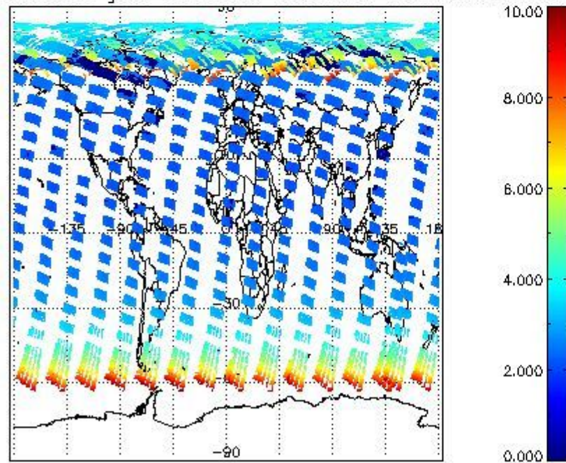
SCIOL2P_NADUV003_amf_gr for 19MAY2004 00:00:00 to 20MAY2004 00:00:00
