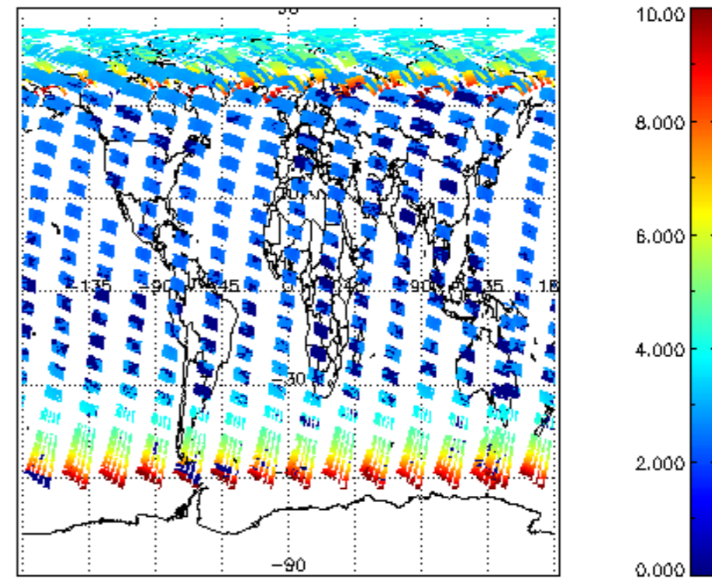
SCIOL2P_NADUV003_amf_cl for 19MAY2004 00:00:00 to 20MAY2004 00:00:00
