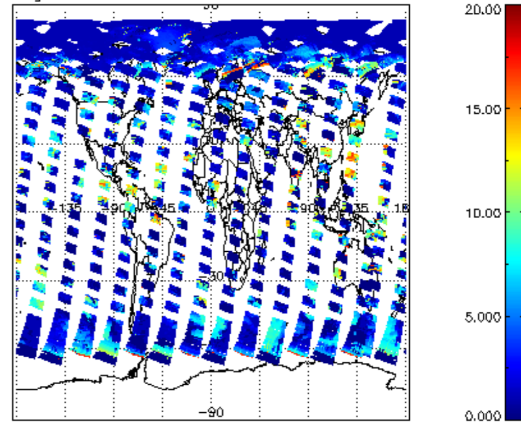
cl_top_height for 19MAY2004 00:00:00 to 20MAY2004 00:00:00
