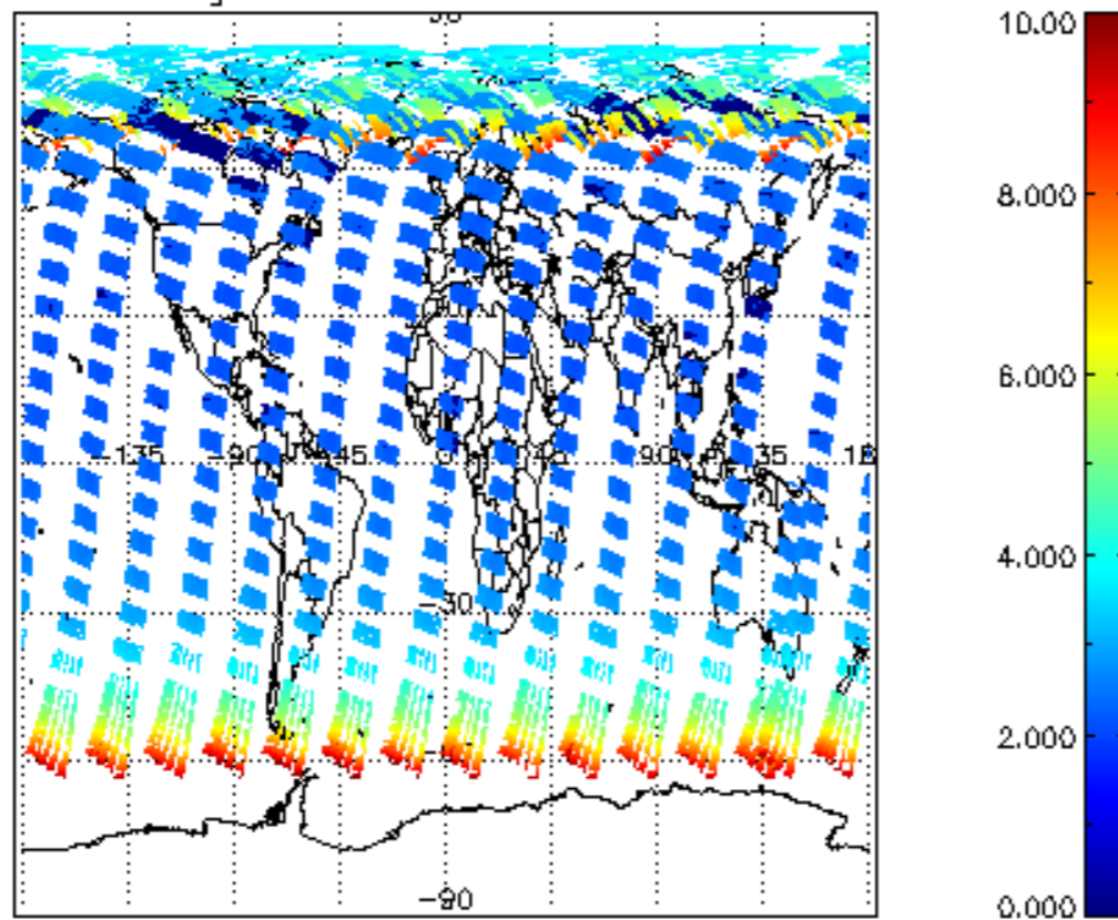
SCIOL2P_NADUV003_amf_gr for 19MAY2004 00:00:00 to 20MAY2004 00:00:00
