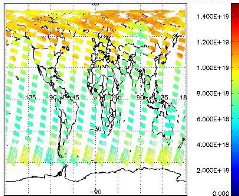
SCIOL2P_NADUV003_vcd for 19MAY2004 00:00:00 to 20MAY2004 00:00:00
