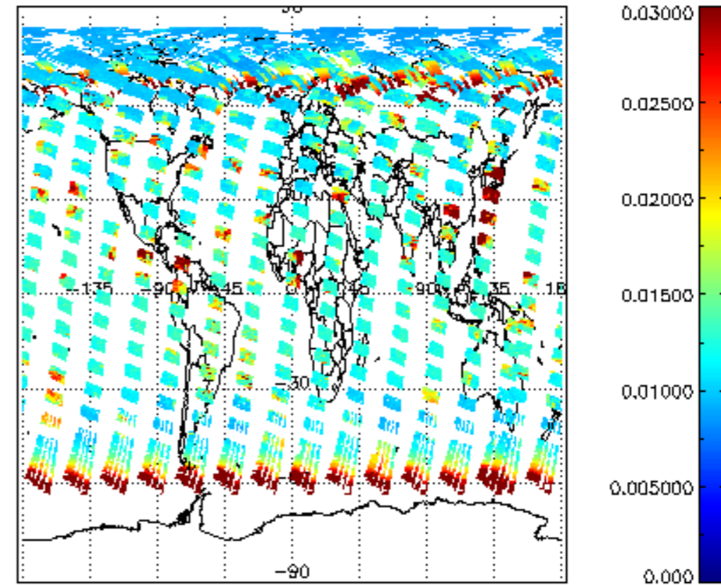
SCIOL2P_NADUV003_vcd_err for 19MAY2004 00:00:00 to 20MAY2004 00:00:00
