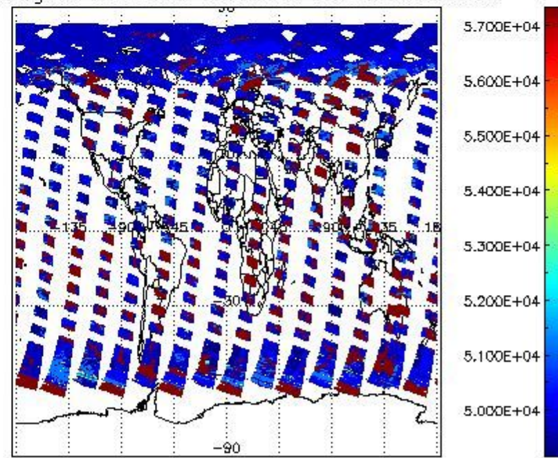
cloud_flags for 19MAY2004 00:00:00 to 20MAY2004 00:00:00
