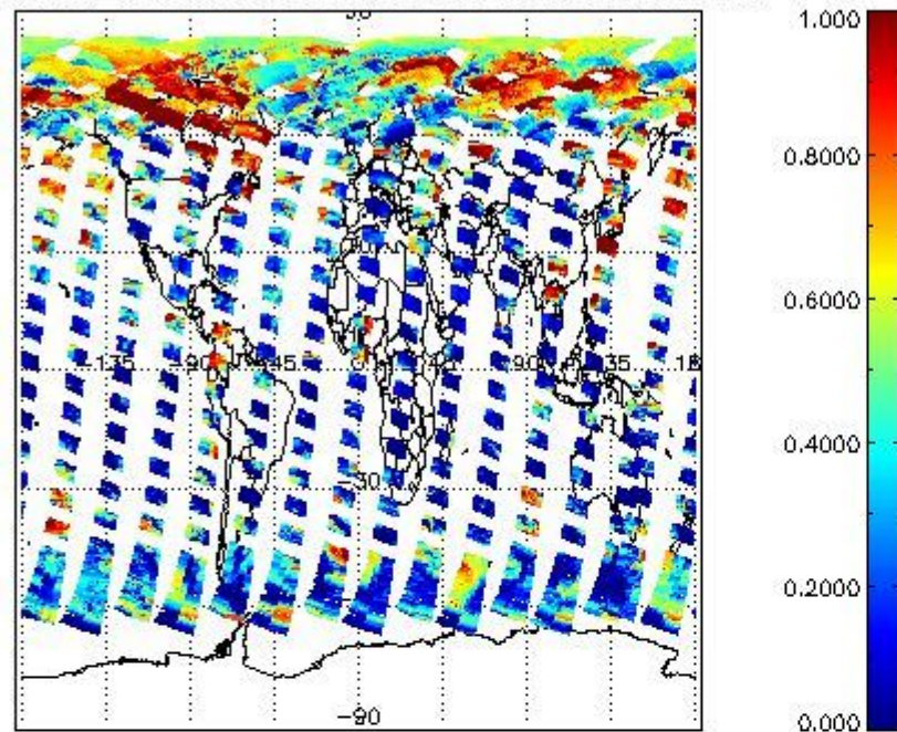
cL_frac for 19MAY2004 00:00:00 to 20MAY2004 00:00:00
