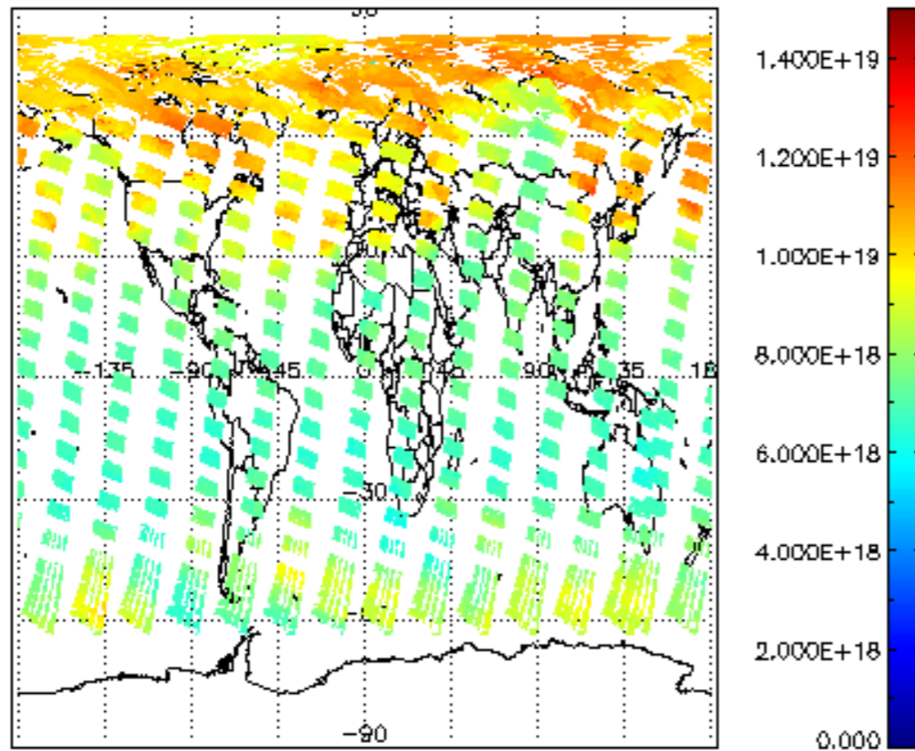
SCIOL2P_NADUV003_vcd for 19MAY2004 00:00:00 to 20MAY2004 00:00:00
