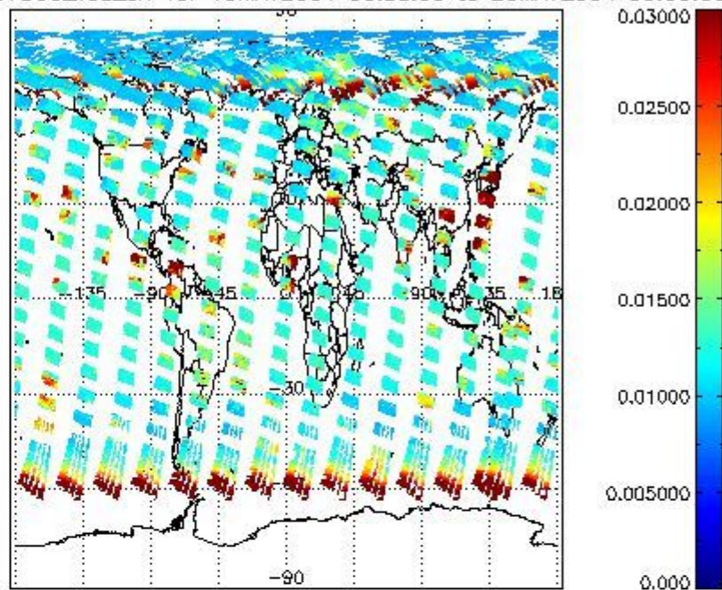
SCIOL2P_NADUV003_vcd_err for 19MAY2004 00:00:00 to 20MAY2004 00:00:00
