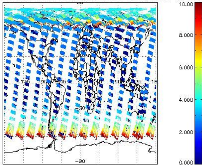
SCIOL2P_NADUV003_amf_cl for 19MAY2004 00:00:00 to 20MAY2004 00:00:00
