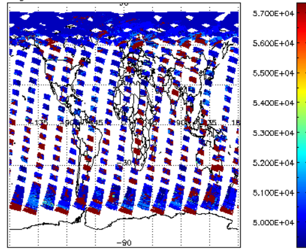
cloud_flags for 19MAY2004 00:00:00 to 20MAY2004 00:00:00
