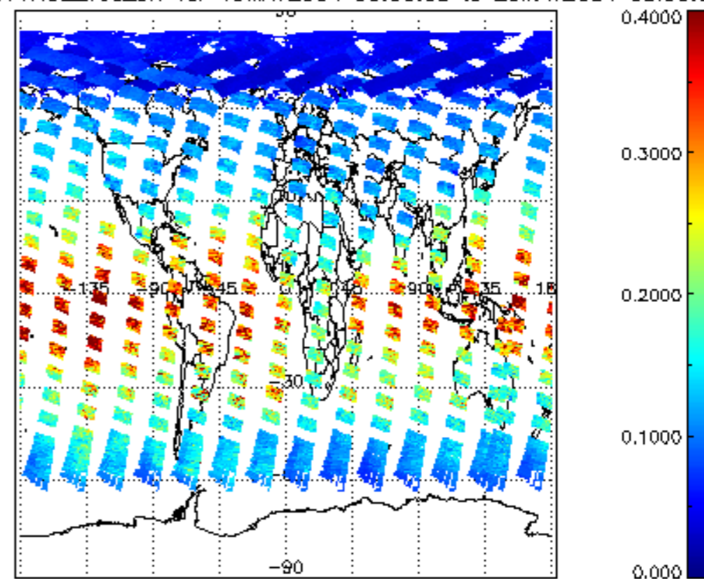
iCIOL2P_NADUV1NO2_vcd_err for 19MAY2004 00:00:00 to 20MAY2004 00:00:00
