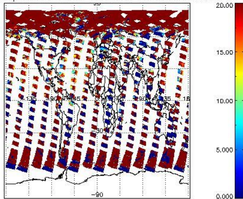
cL_opt_depth for 19MAY2004 00:00:00 to 20MAY2004 00:00:00
