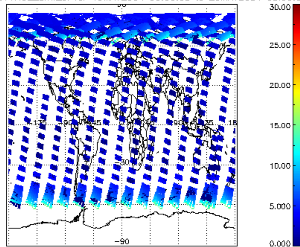
iCIOL2P_NADUV1NO2_amf_cl for 19MAY2004 00:00:00 to 20MAY2004 00:00:00
