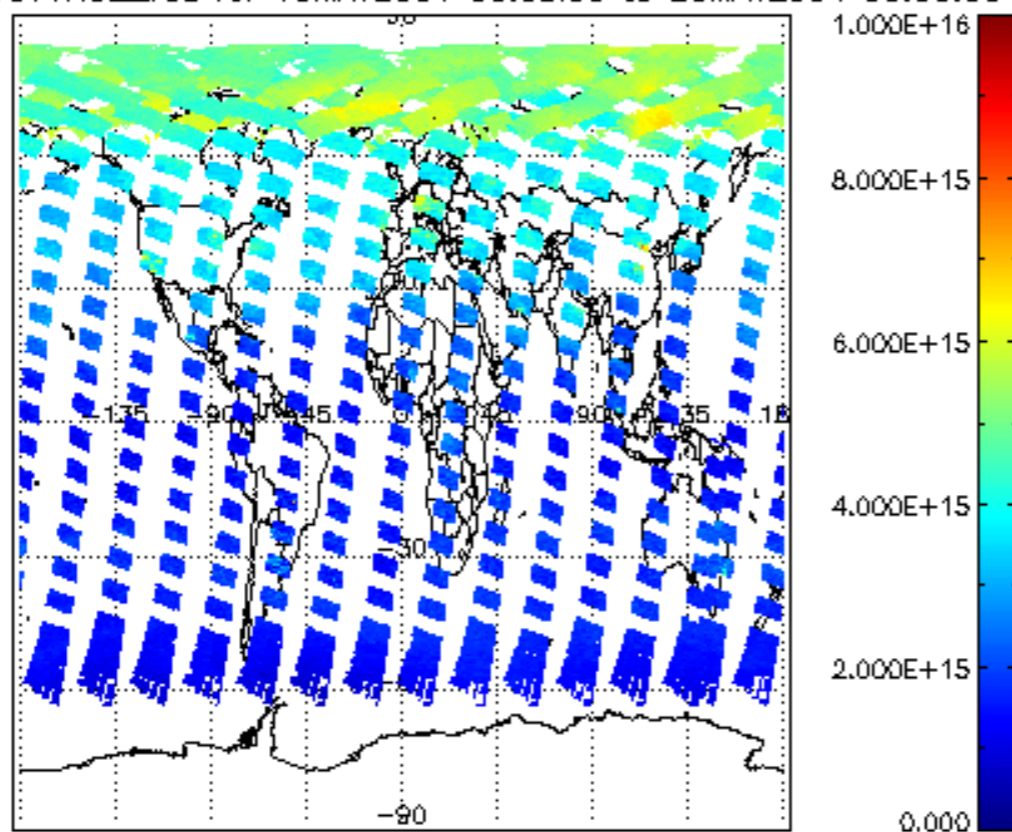
SCIOL2P_NADUV1NO2_vcd for 19MAY2004 00:00:00 to 20MAY2004 00:00:00
