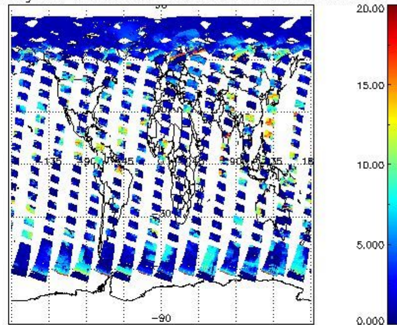
cL_top_height for 19MAY2004 00:00:00 to 20MAY2004 00:00:00
