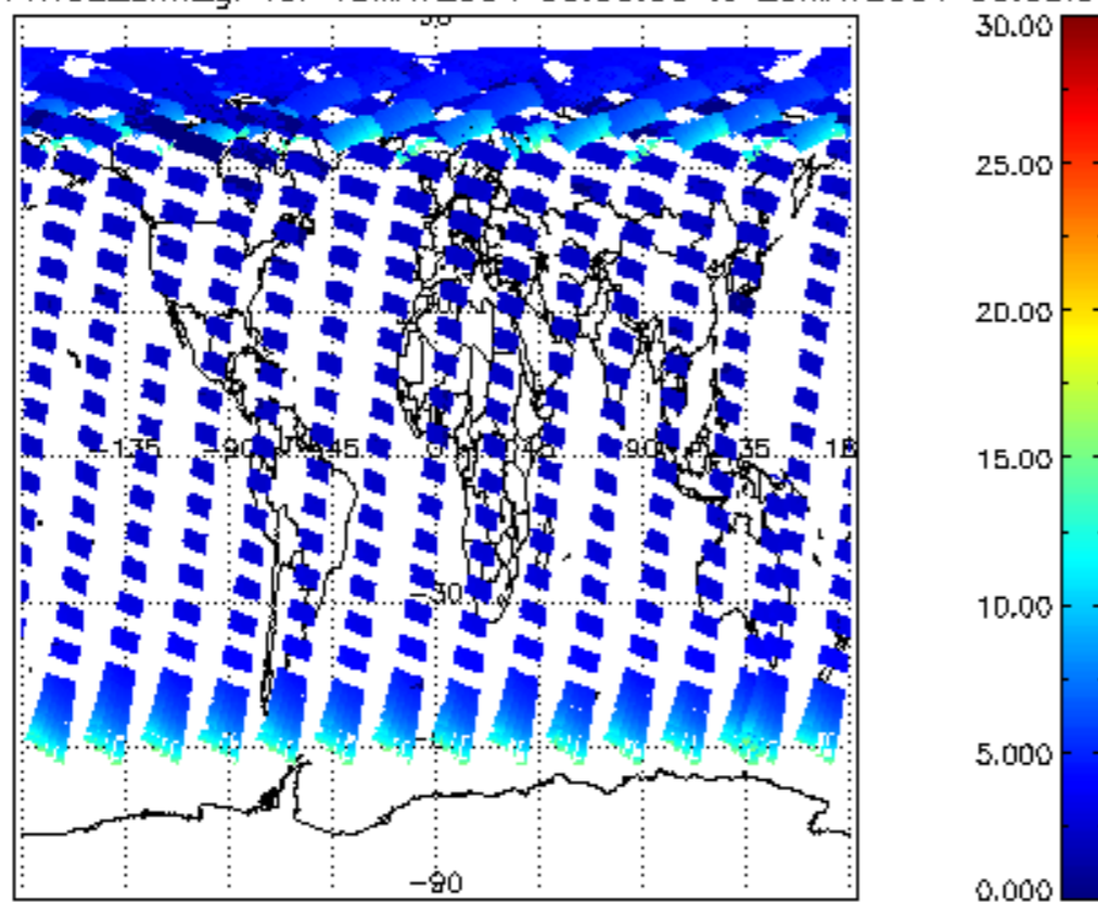
iCIOL2P_NADUV1NO2_amf_gr for 19MAY2004 00:00:00 to 20MAY2004 00:00:00
