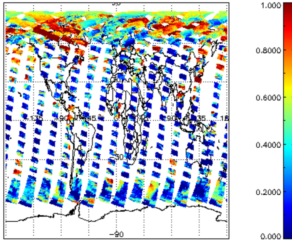
cl_frac for 19MAY2004 00:00:00 to 20MAY2004 00:00:00
