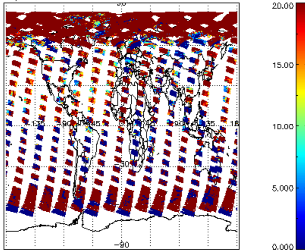
cl_opt_depth for 19MAY2004 00:00:00 to 20MAY2004 00:00:00
