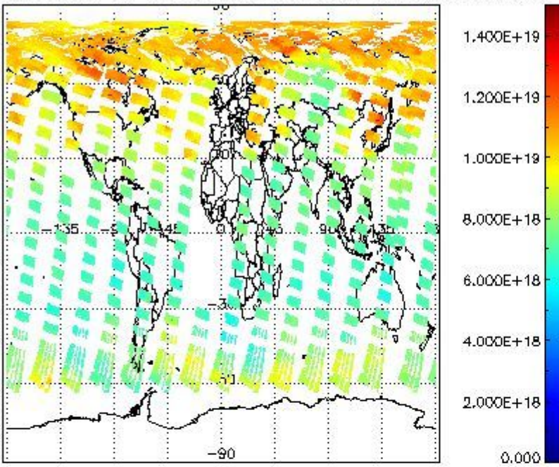
SCIOL2P_NADUV003_vcd for 18MAY2004 00:00:00 to 19MAY2004 00:00:00
