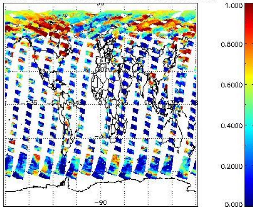
cL_frac for 18MAY2004 00:00:00 to 19MAY2004 00:00:00
