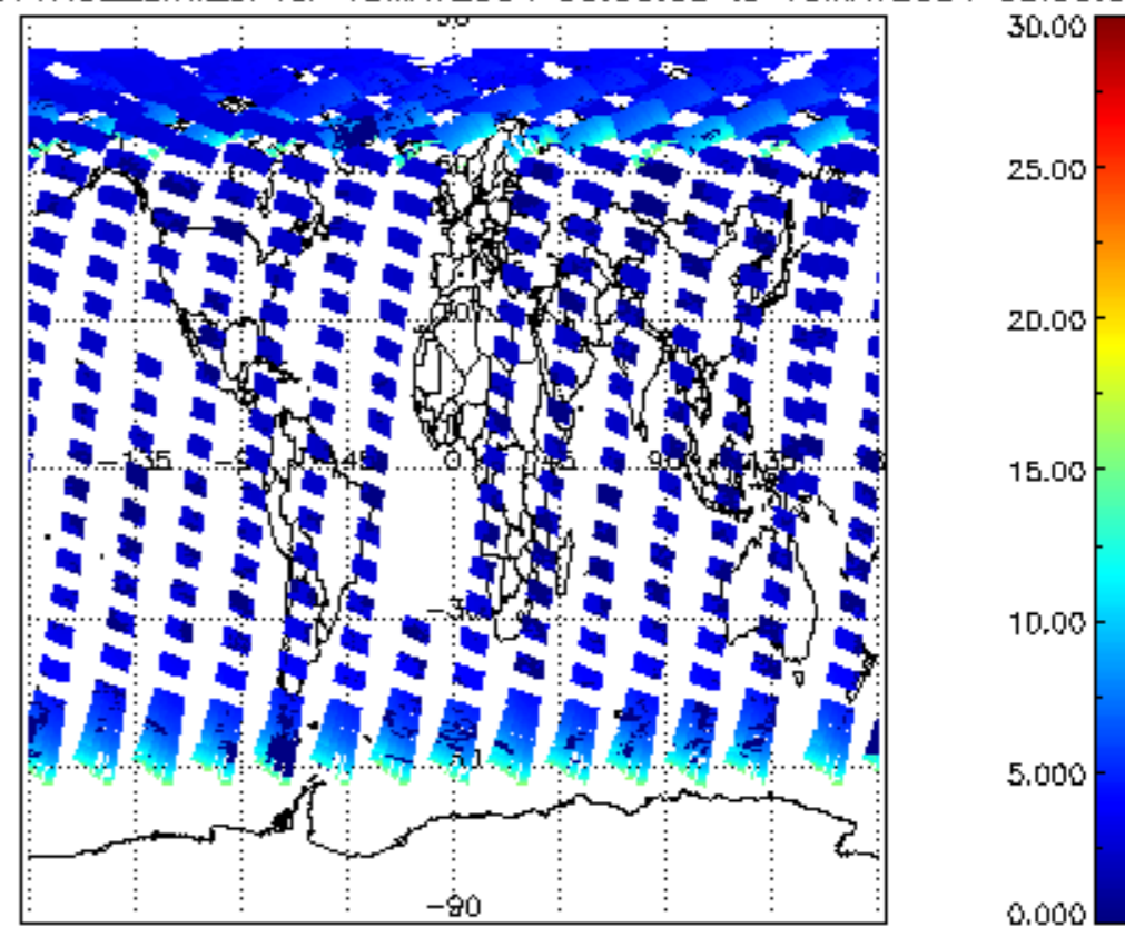
iCIOL2P_NADUV1NO2_amf_cl for 18MAY2004 00:00:00 to 19MAY2004 00:00:00
