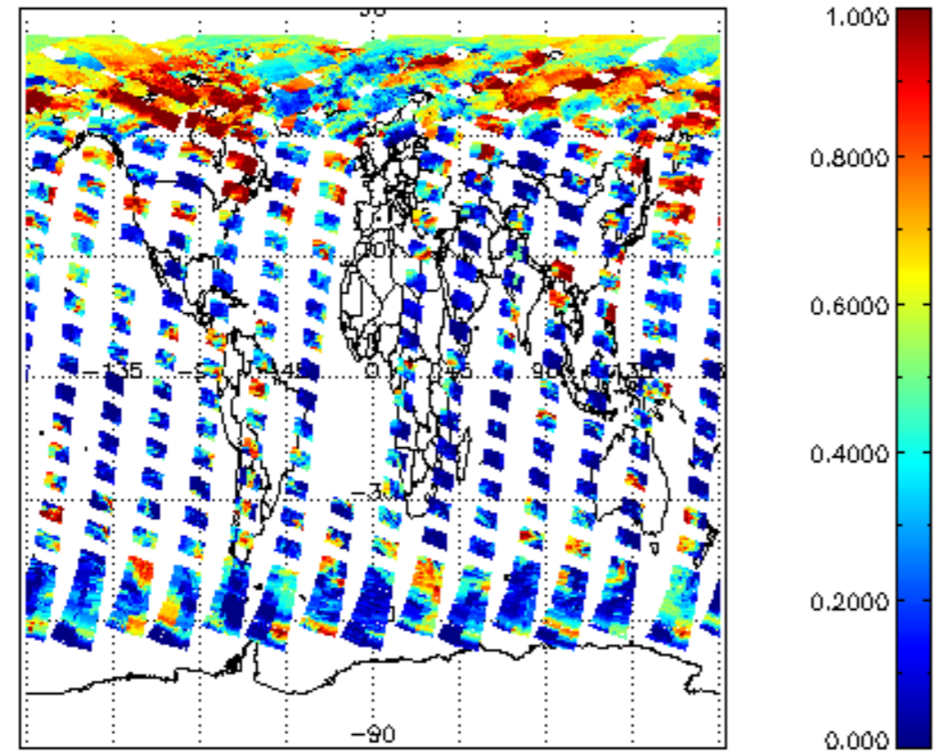
cl_frac for 18MAY2004 00:00:00 to 19MAY2004 00:00:00
