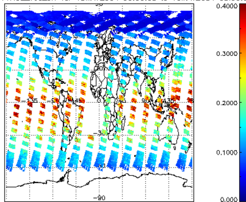
iCIOL2P_NADUV1NO2_vcd_err for 18MAY2004 00:00:00 to 19MAY2004 00:00:00
