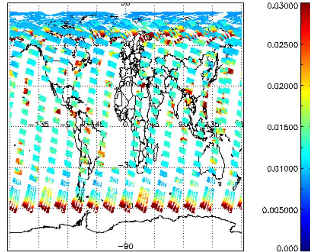
SCIOL2P_NADUV003_vcd_err for 18MAY2004 00:00:00 to 19MAY2004 00:00:00
