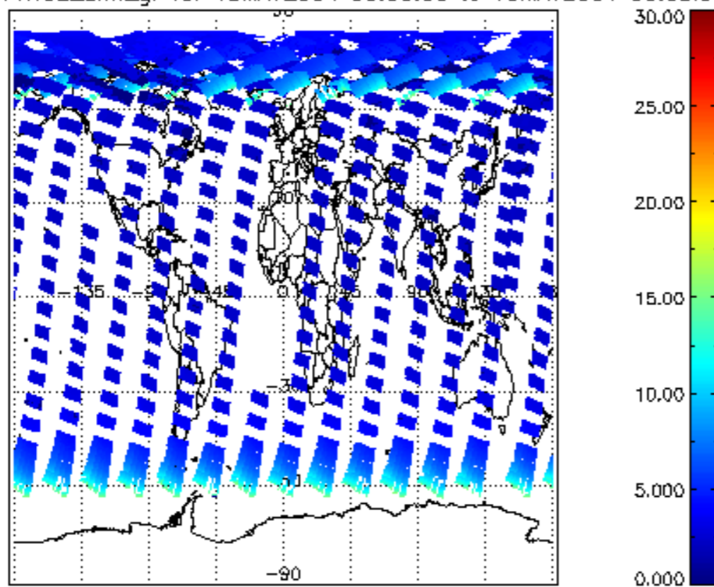
iCIOL2P_NADUV1NO2_amf_gr for 18MAY2004 00:00:00 to 19MAY2004 00:00:00
