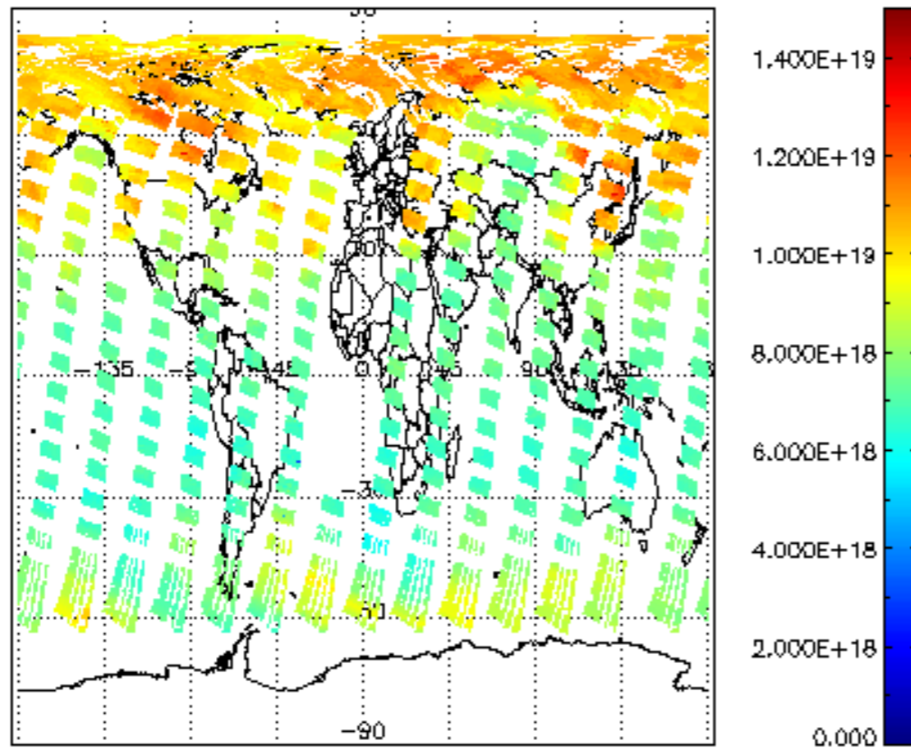
SCIOL2P_NADUV003_vcd for 18MAY2004 00:00:00 to 19MAY2004 00:00:00
