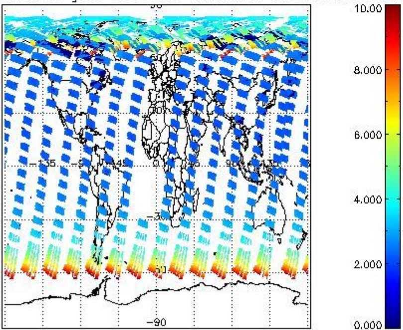
SCIOL2P_NADUV003_amf_gr for 18MAY2004 00:00:00 to 19MAY2004 00:00:00
