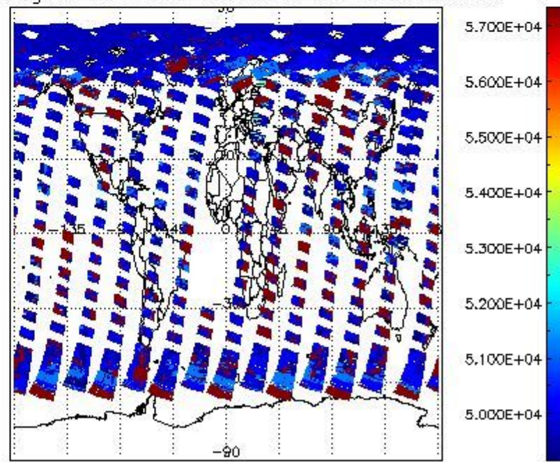
cloud_flags for 18MAY2004 00:00:00 to 19MAY2004 00:00:00
