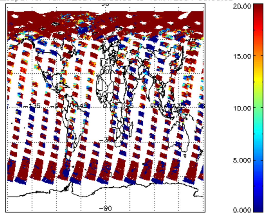
cl_opt_depth for 18MAY2004 00:00:00 to 19MAY2004 00:00:00
