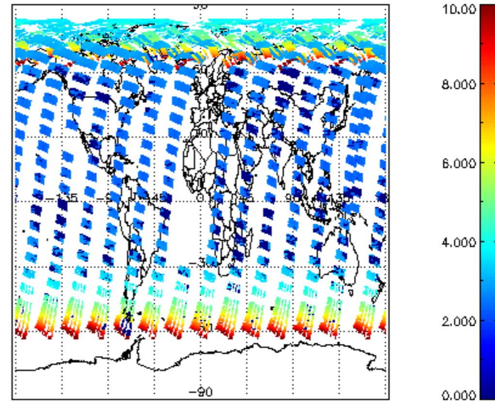
SCIOL2P_NADUV003_amf_cl for 18MAY2004 00:00:00 to 19MAY2004 00:00:00
