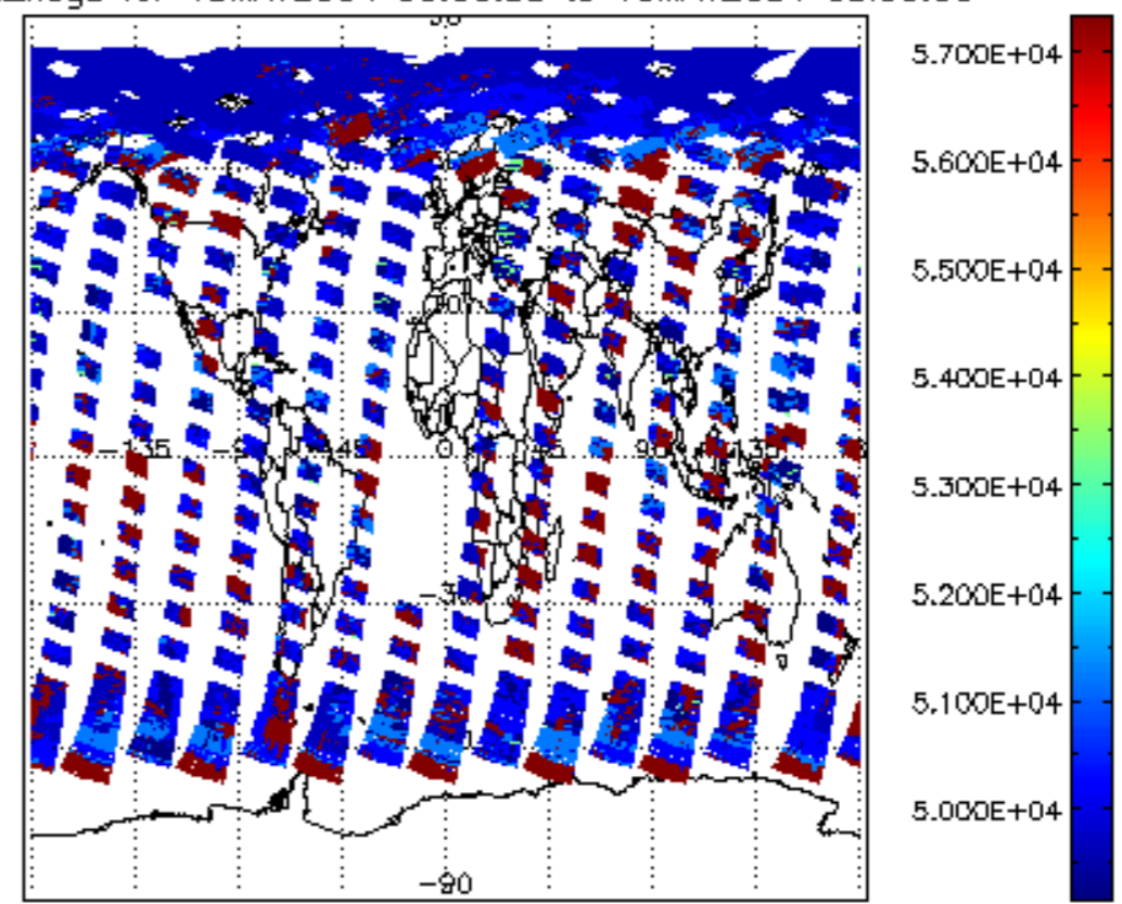
cloud_flags for 18MAY2004 00:00:00 to 19MAY2004 00:00:00
