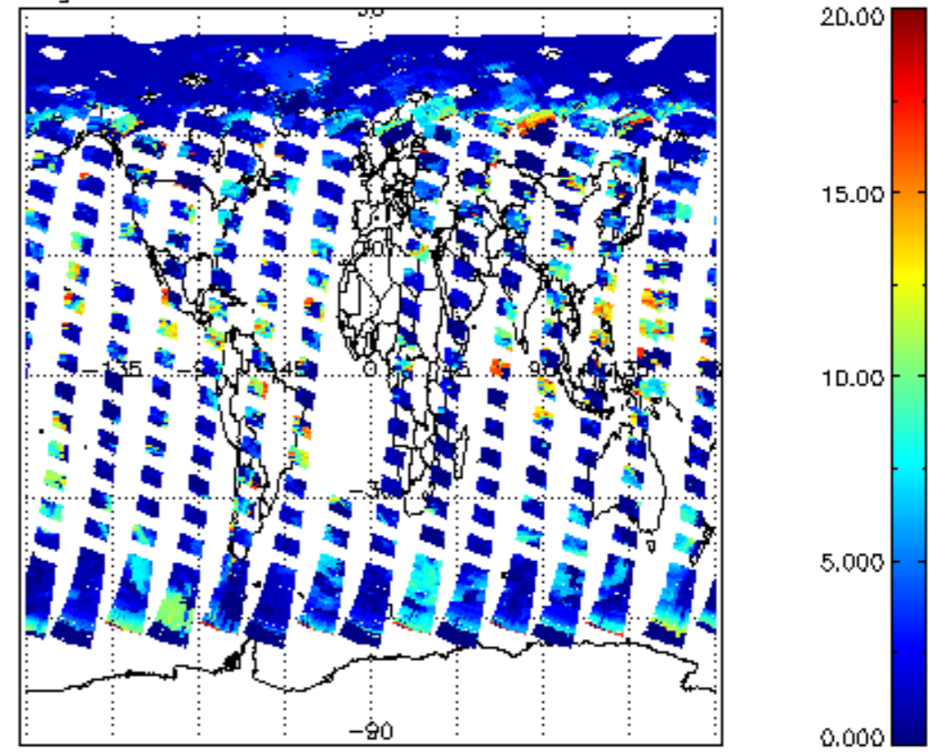
cl_top_height for 18MAY2004 00:00:00 to 19MAY2004 00:00:00
