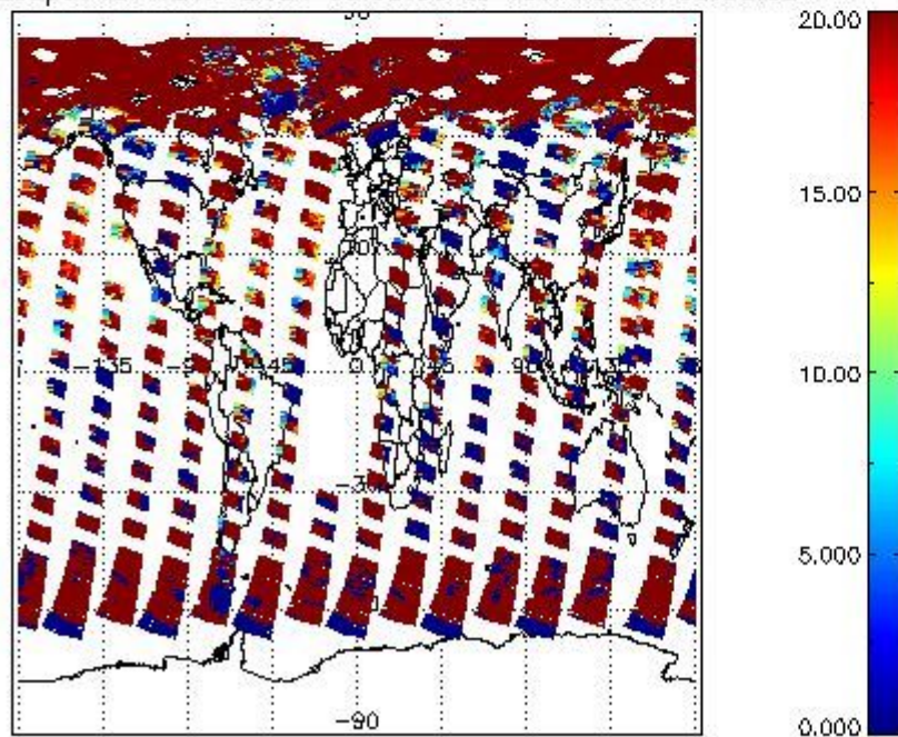
cL_opt_depth for 18MAY2004 00:00:00 to 19MAY2004 00:00:00
