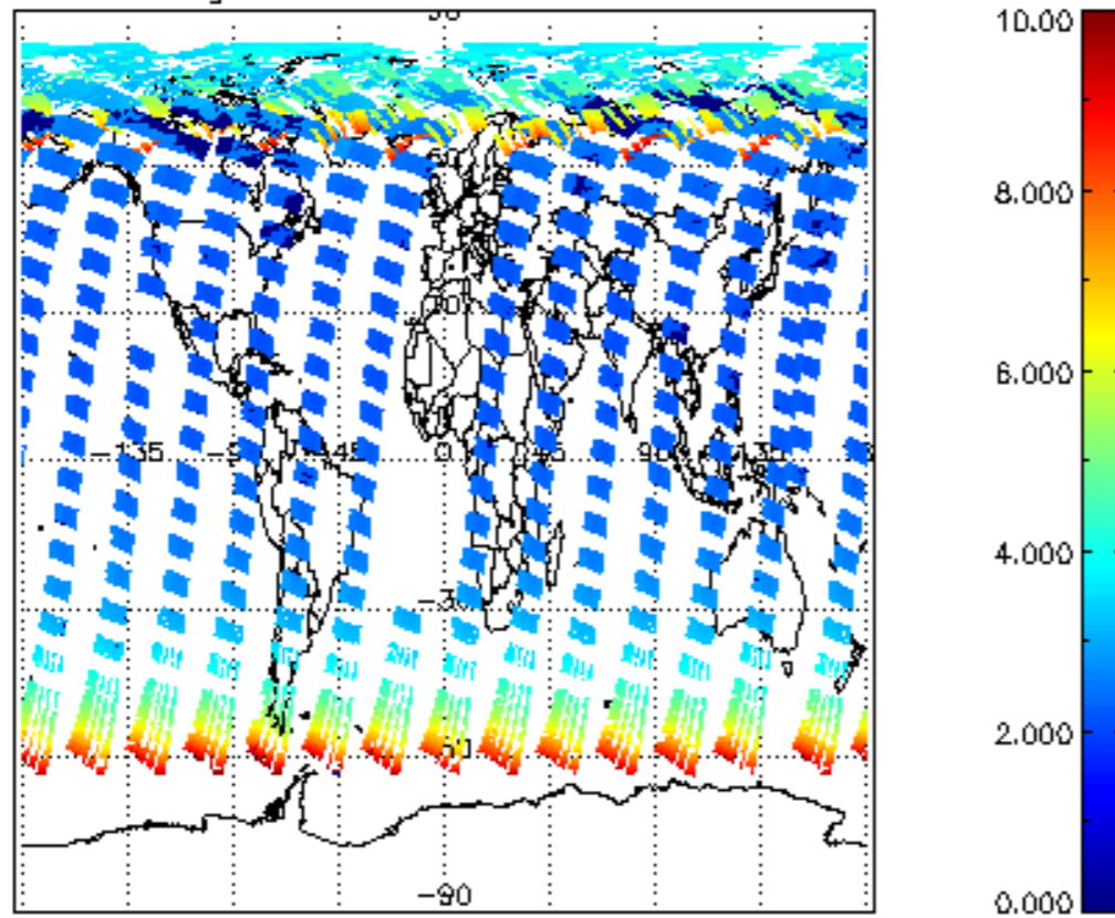
SCIOL2P_NADUV003_amf_gr for 18MAY2004 00:00:00 to 19MAY2004 00:00:00
