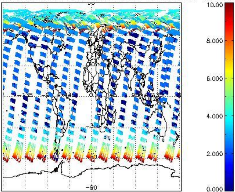
SCIOL2P_NADUV003_amf_cl for 18MAY2004 00:00:00 to 19MAY2004 00:00:00
