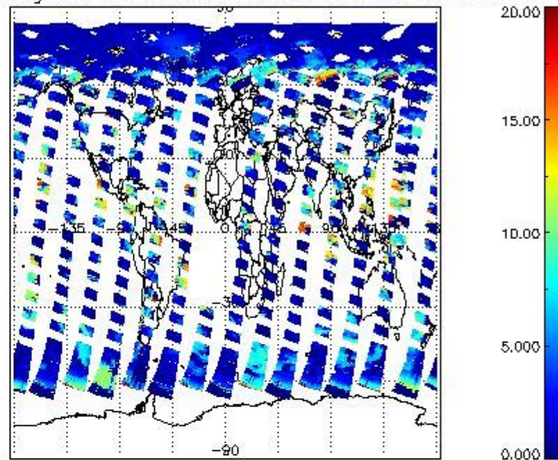
cL_top_height for 18MAY2004 00:00:00 to 19MAY2004 00:00:00
