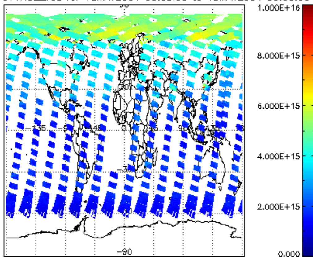
SCIOL2P_NADUV1NO2_vcd for 18MAY2004 00:00:00 to 19MAY2004 00:00:00
