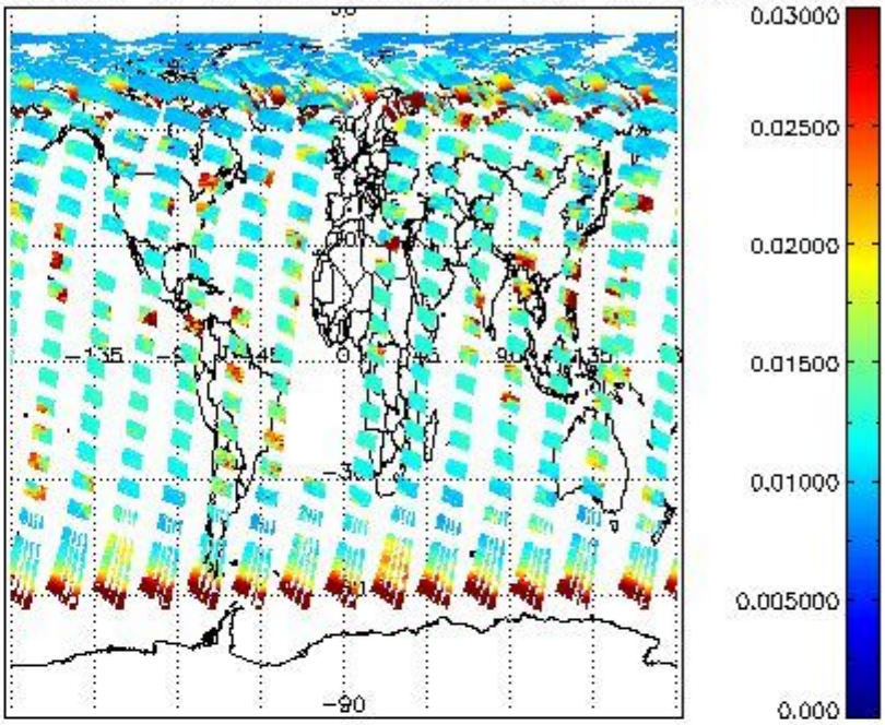
SCIOL2P_NADUV003_vcd_err for 18MAY2004 00:00:00 to 19MAY2004 00:00:00
