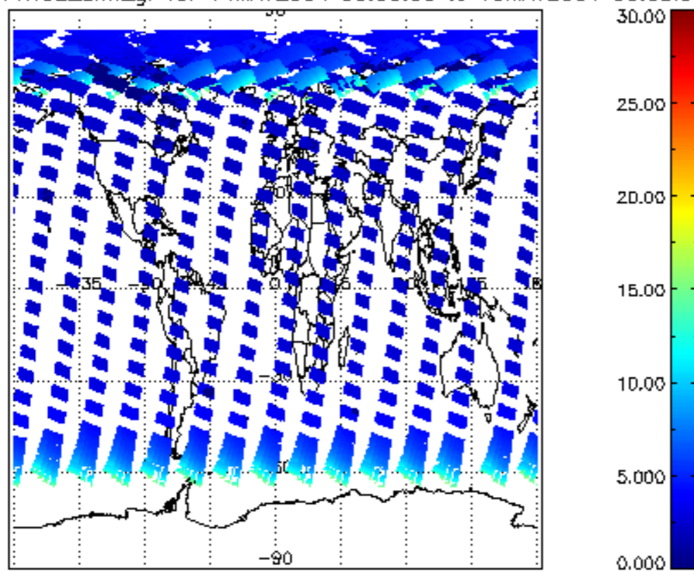
iCIOL2P_NADUV1NO2_amf_gr for 14MAY2004 00:00:00 to 15MAY2004 00:00:00
