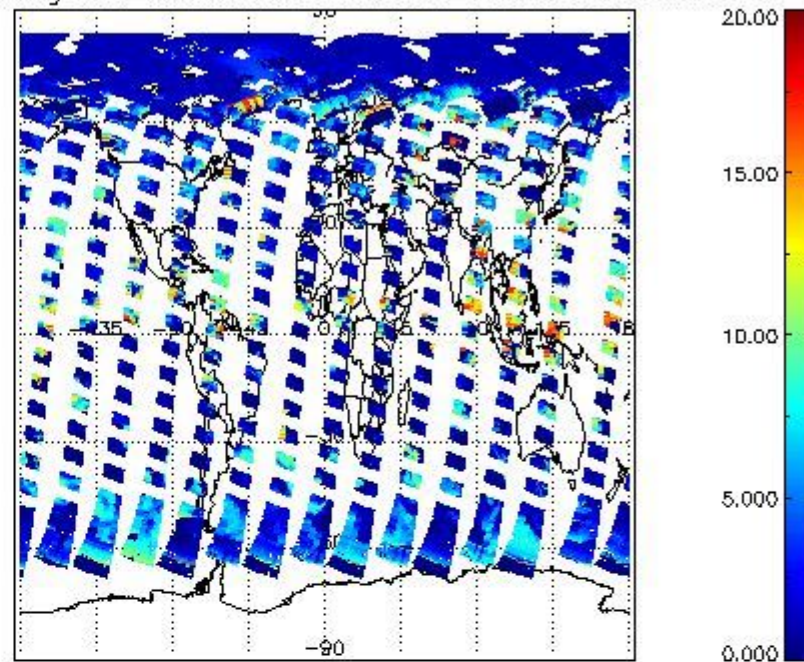
cL_top_height for 14MAY2004 00:00:00 to 15MAY2004 00:00:00
