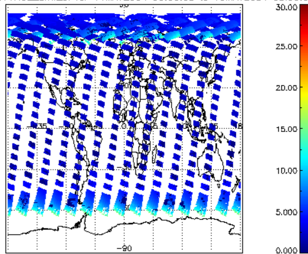
iCIOL2P_NADUV1NO2_amf_cl for 14MAY2004 00:00:00 to 15MAY2004 00:00:00
