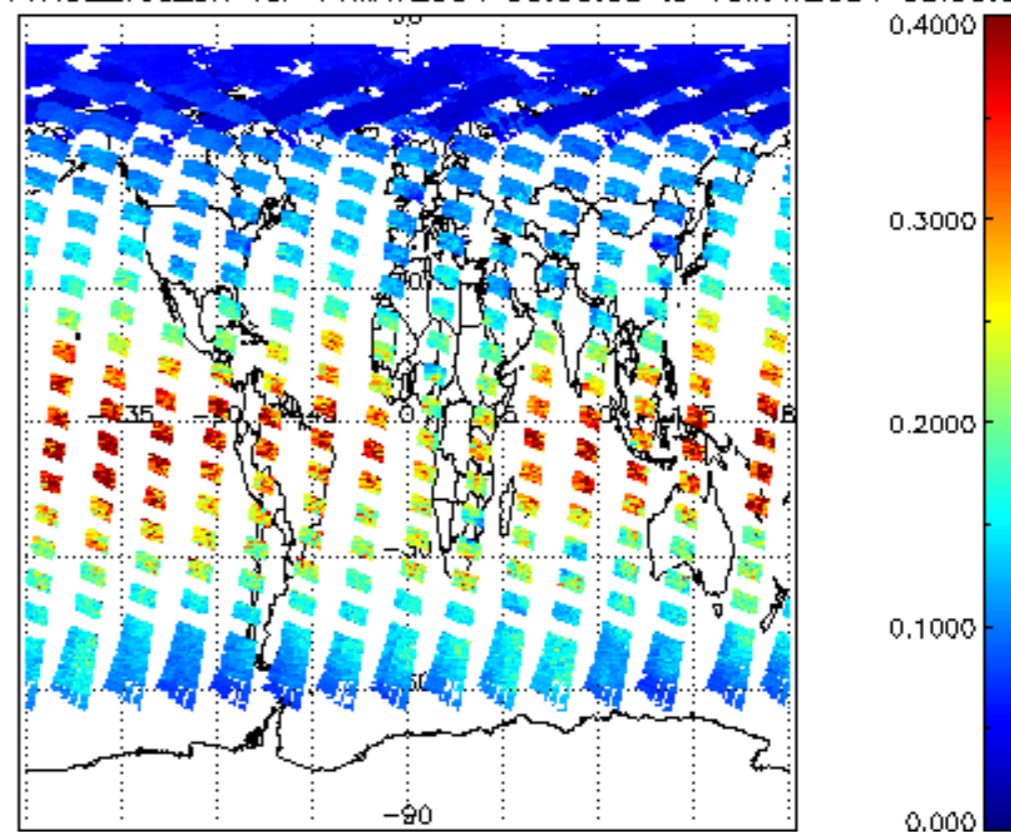
iCIOL2P_NADUV1NO2_vcd_err for 14MAY2004 00:00:00 to 15MAY2004 00:00:00
