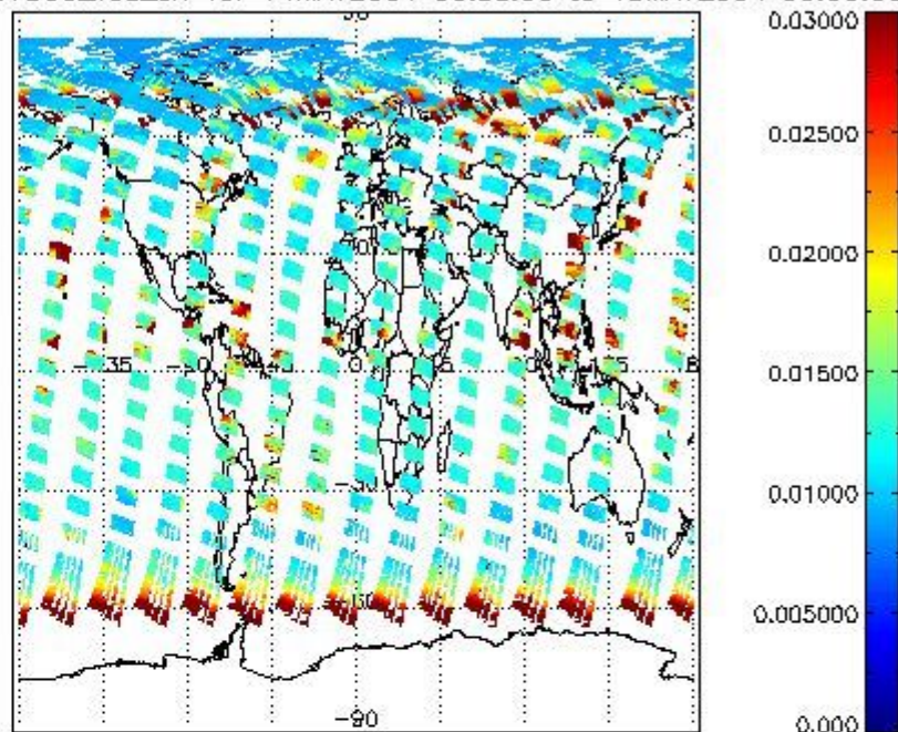
SCIOL2P_NADUV003_vcd_err for 14MAY2004 00:00:00 to 15MAY2004 00:00:00
