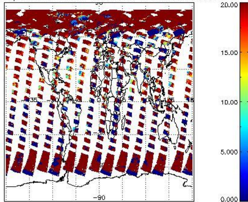
cL_opt_depth for 14MAY2004 00:00:00 to 15MAY2004 00:00:00
