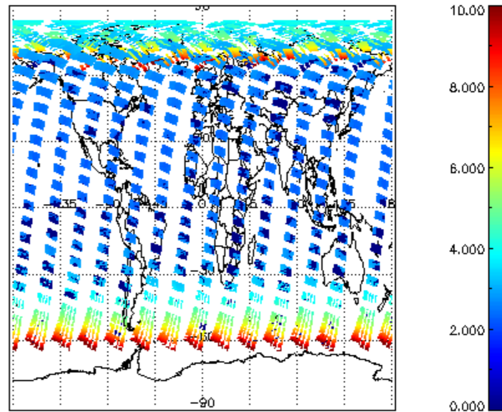
SCIOL2P_NADUV003_amf_cl for 14MAY2004 00:00:00 to 15MAY2004 00:00:00
