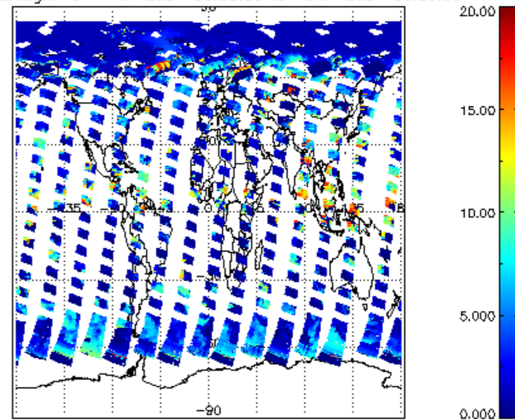
cl_top_height for 14MAY2004 00:00:00 to 15MAY2004 00:00:00
