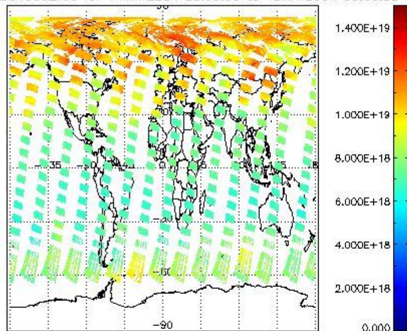
SCIOL2P_NADUV003_vcd for 14MAY2004 00:00:00 to 15MAY2004 00:00:00
