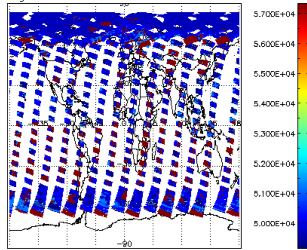
cloud_flags for 14MAY2004 00:00:00 to 15MAY2004 00:00:00
