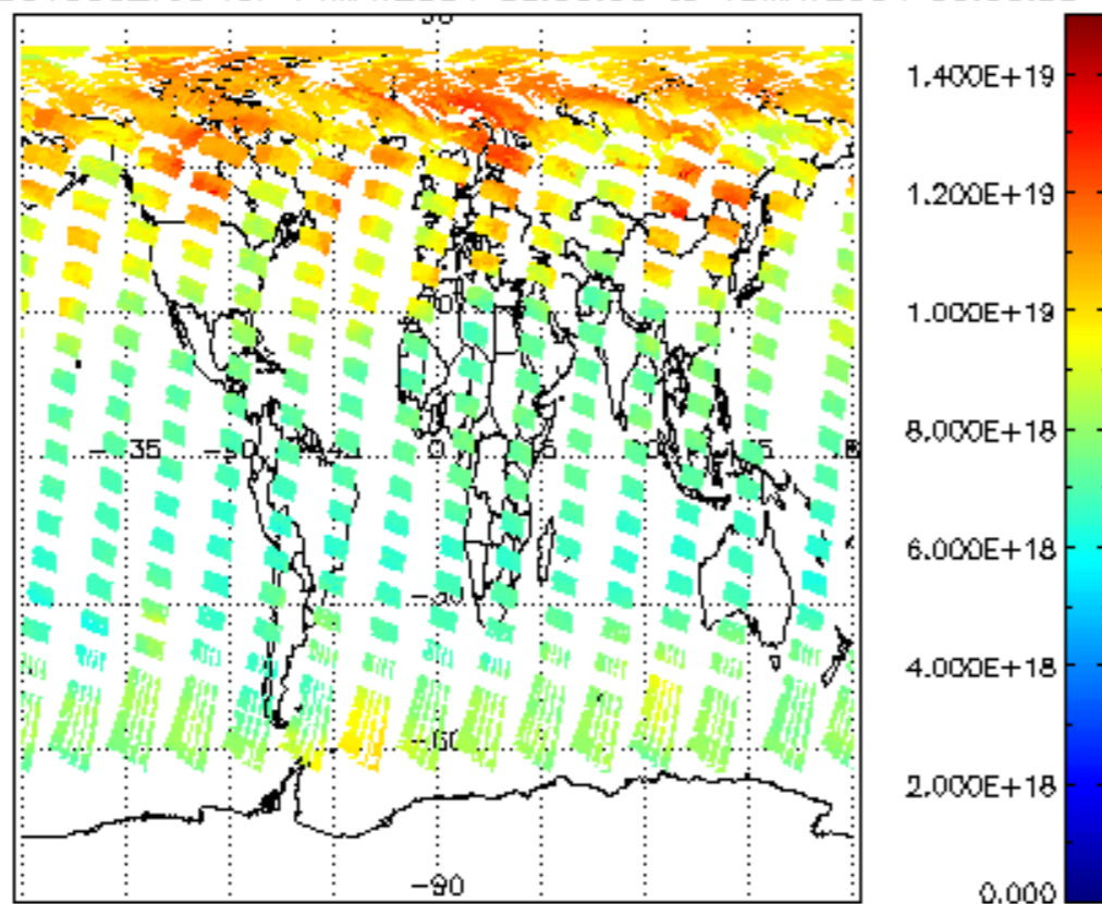
SCIOL2P_NADUV003_vcd for 14MAY2004 00:00:00 to 15MAY2004 00:00:00
