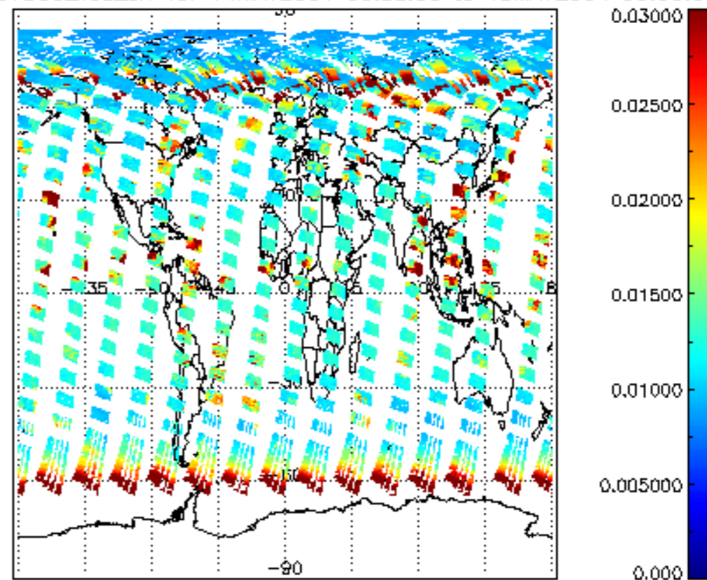
SCIOL2P_NADUV003_vcd_err for 14MAY2004 00:00:00 to 15MAY2004 00:00:00
