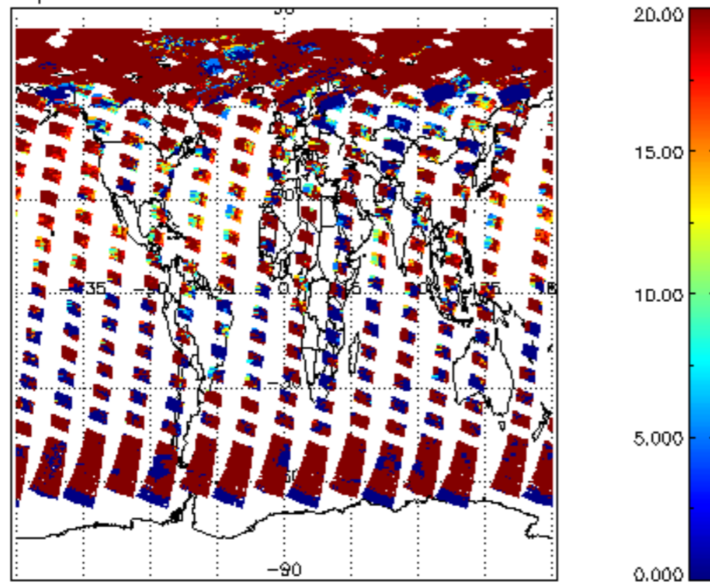
cl_opt_depth for 14MAY2004 00:00:00 to 15MAY2004 00:00:00
