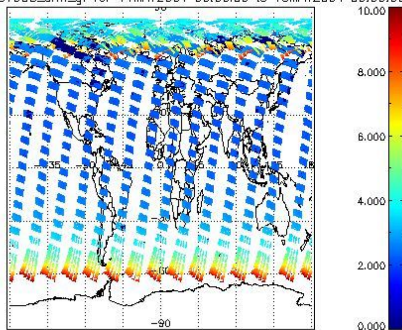
SCIOL2P_NADUV003_amf_gr for 14MAY2004 00:00:00 to 15MAY2004 00:00:00
