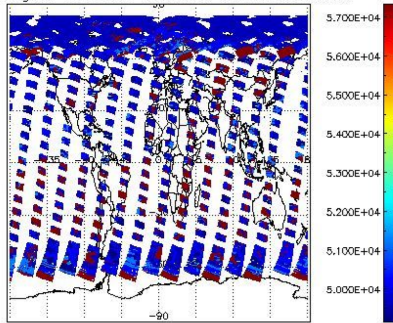
cloud_flags for 14MAY2004 00:00:00 to 15MAY2004 00:00:00
