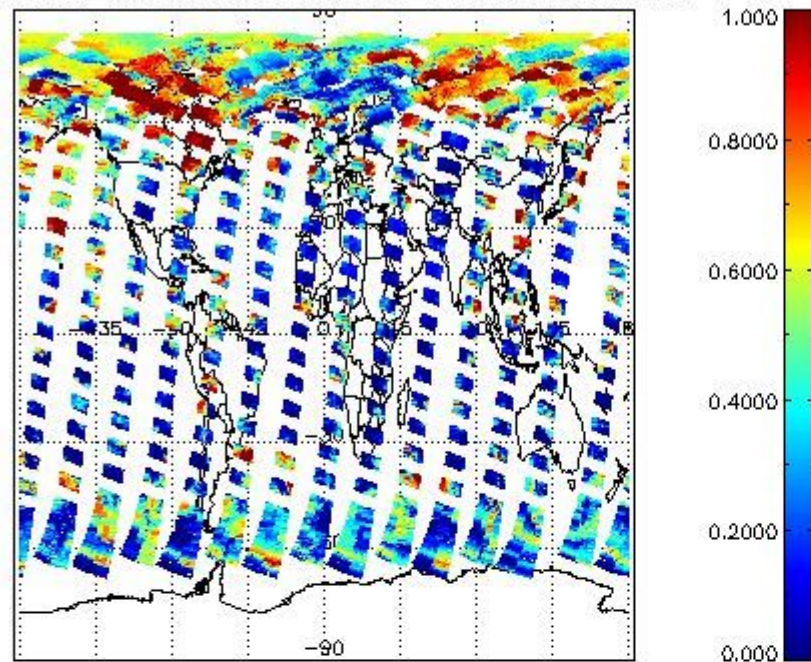
cL_frac for 14MAY2004 00:00:00 to 15MAY2004 00:00:00
