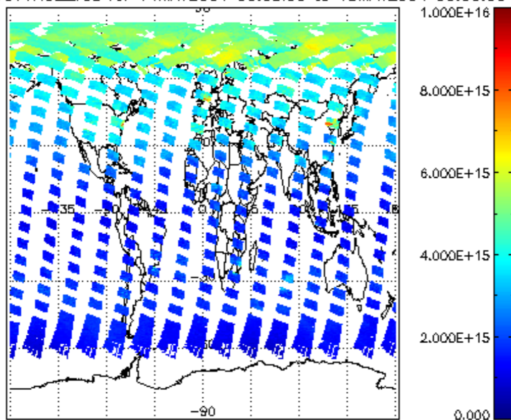
SCIOL2P_NADUV1NO2_vcd for 14MAY2004 00:00:00 to 15MAY2004 00:00:00
