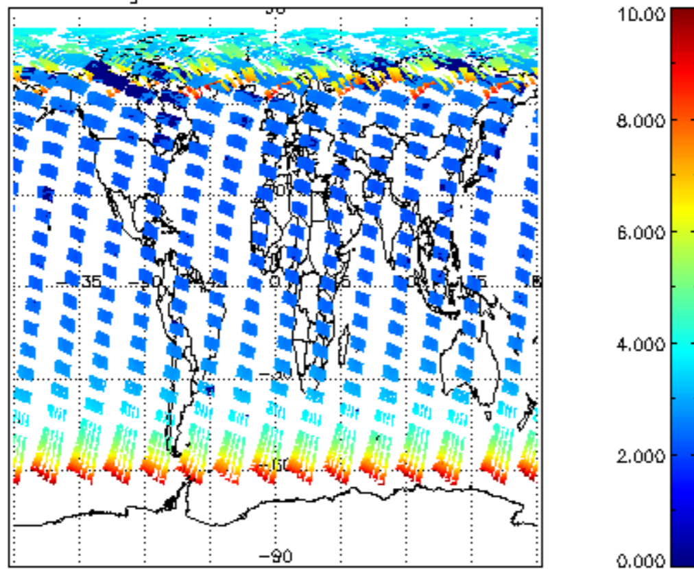
SCIOL2P_NADUV003_amf_gr for 14MAY2004 00:00:00 to 15MAY2004 00:00:00
