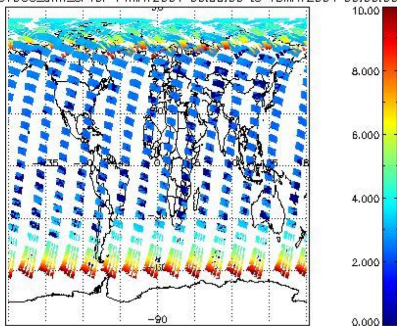
SCIOL2P_NADUV003_amf_cl for 14MAY2004 00:00:00 to 15MAY2004 00:00:00
