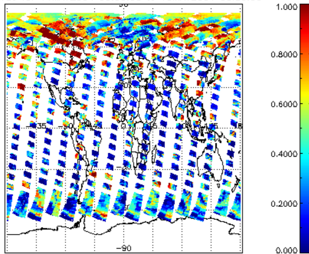
cl_frac for 14MAY2004 00:00:00 to 15MAY2004 00:00:00
