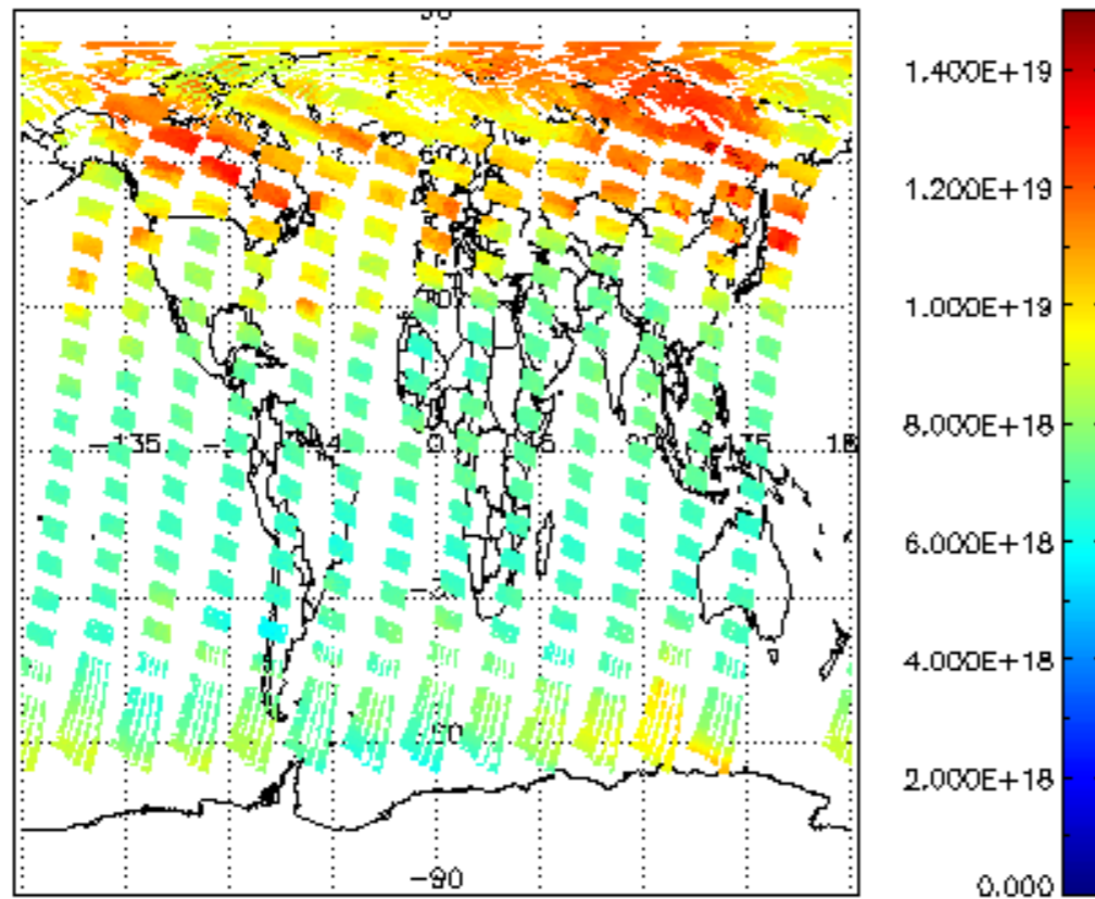
SCIOL2P_NADUV003_vcd for 08MAY2004 00:00:00 to 09MAY2004 00:00:00
