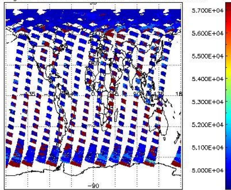
cloud_flags for 08MAY2004 00:00:00 to 09MAY2004 00:00:00
