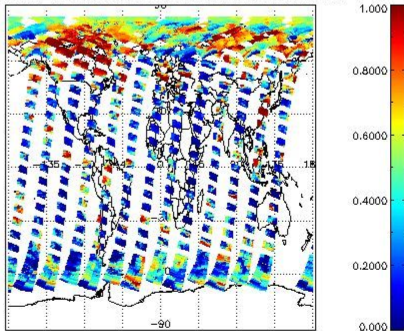
cL_frac for 08MAY2004 00:00:00 to 09MAY2004 00:00:00
