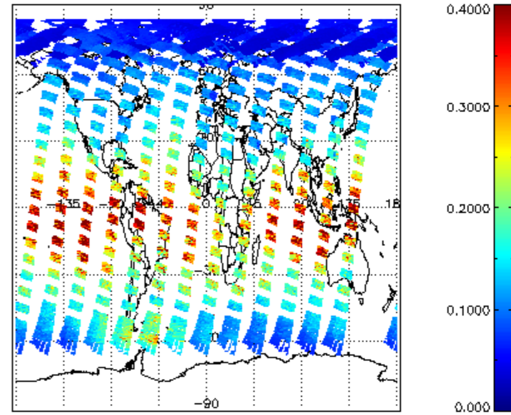
iCIOL2P_NADUV1NO2_vcd_err for 08MAY2004 00:00:00 to 09MAY2004 00:00:00
