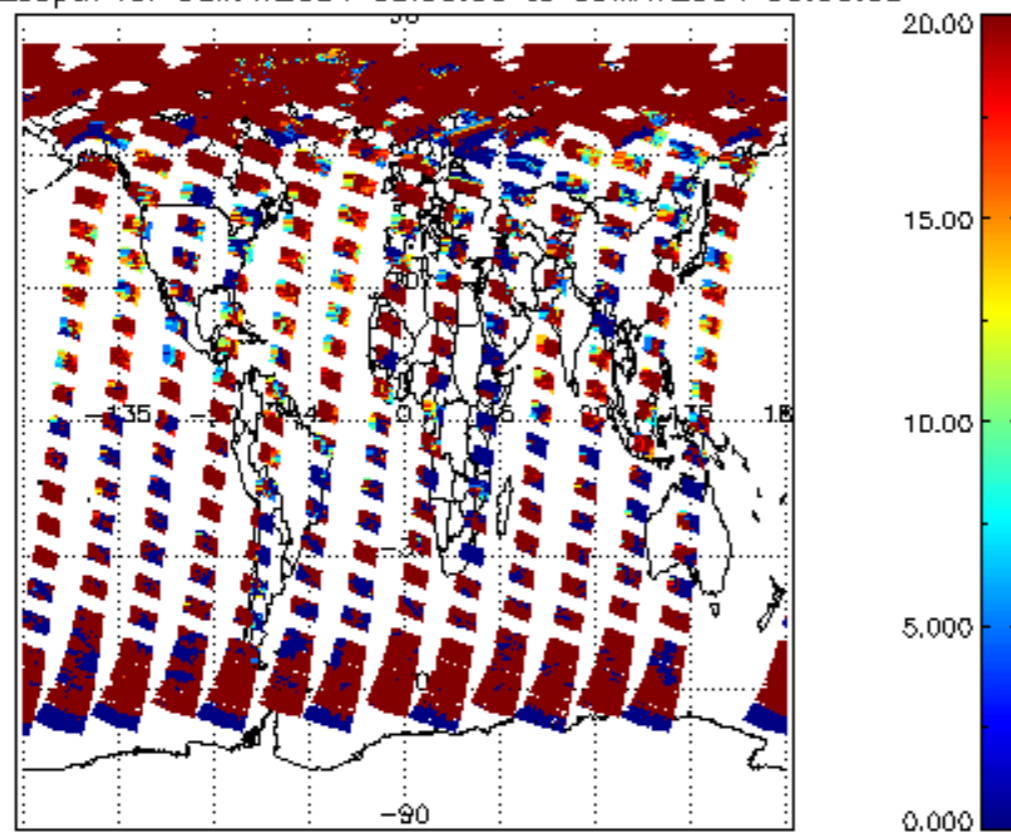
cl_opt_depth for 08MAY2004 00:00:00 to 09MAY2004 00:00:00
