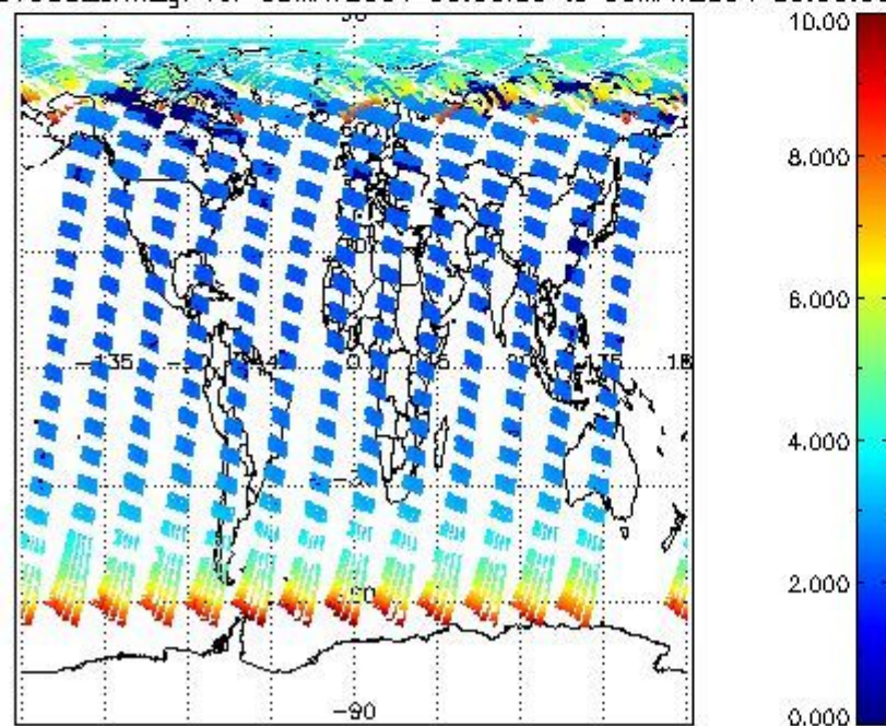
SCIOL2P_NADUV003_amf_gr for 08MAY2004 00:00:00 to 09MAY2004 00:00:00
