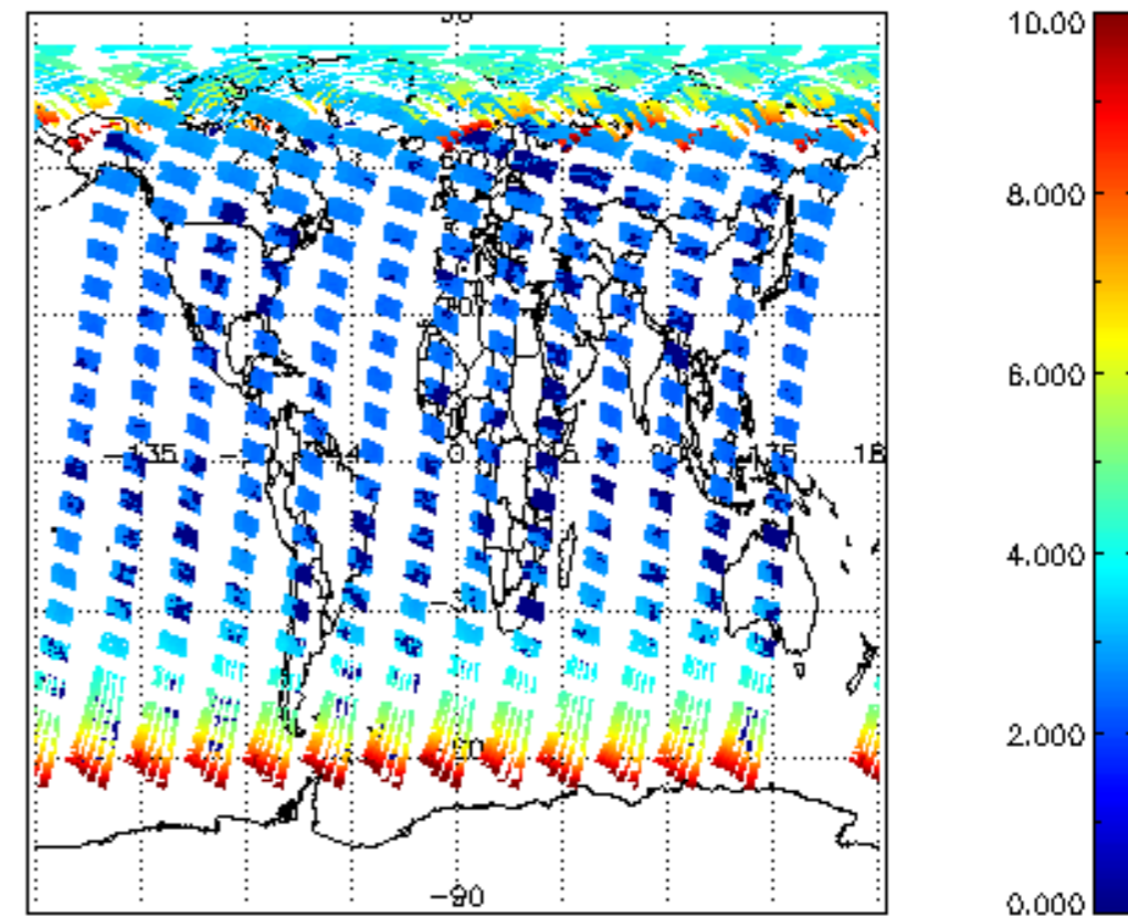
SCIOL2P_NADUV003_amf_cl for 08MAY2004 00:00:00 to 09MAY2004 00:00:00
