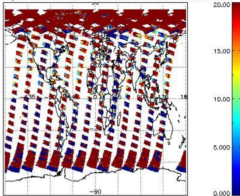
cL_opt_depth for 08MAY2004 00:00:00 to 09MAY2004 00:00:00
