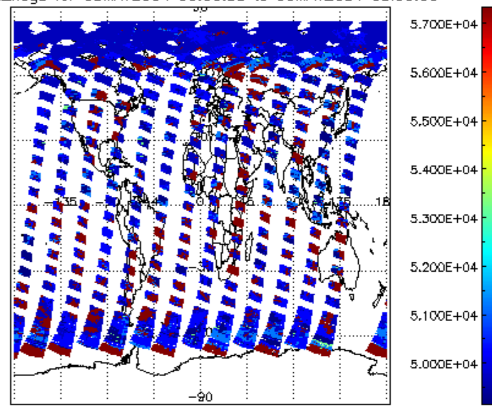
cloud_flags for 08MAY2004 00:00:00 to 09MAY2004 00:00:00
