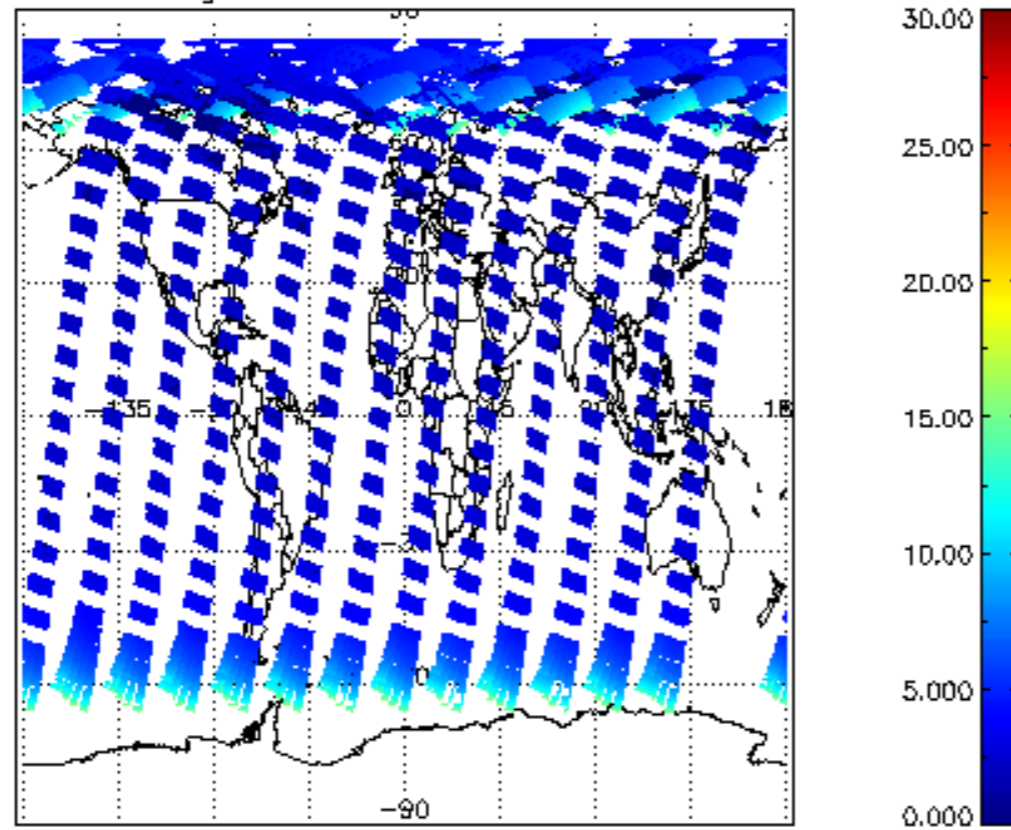
iCIOL2P_NADUV1NO2_amf_gr for 08MAY2004 00:00:00 to 09MAY2004 00:00:00
