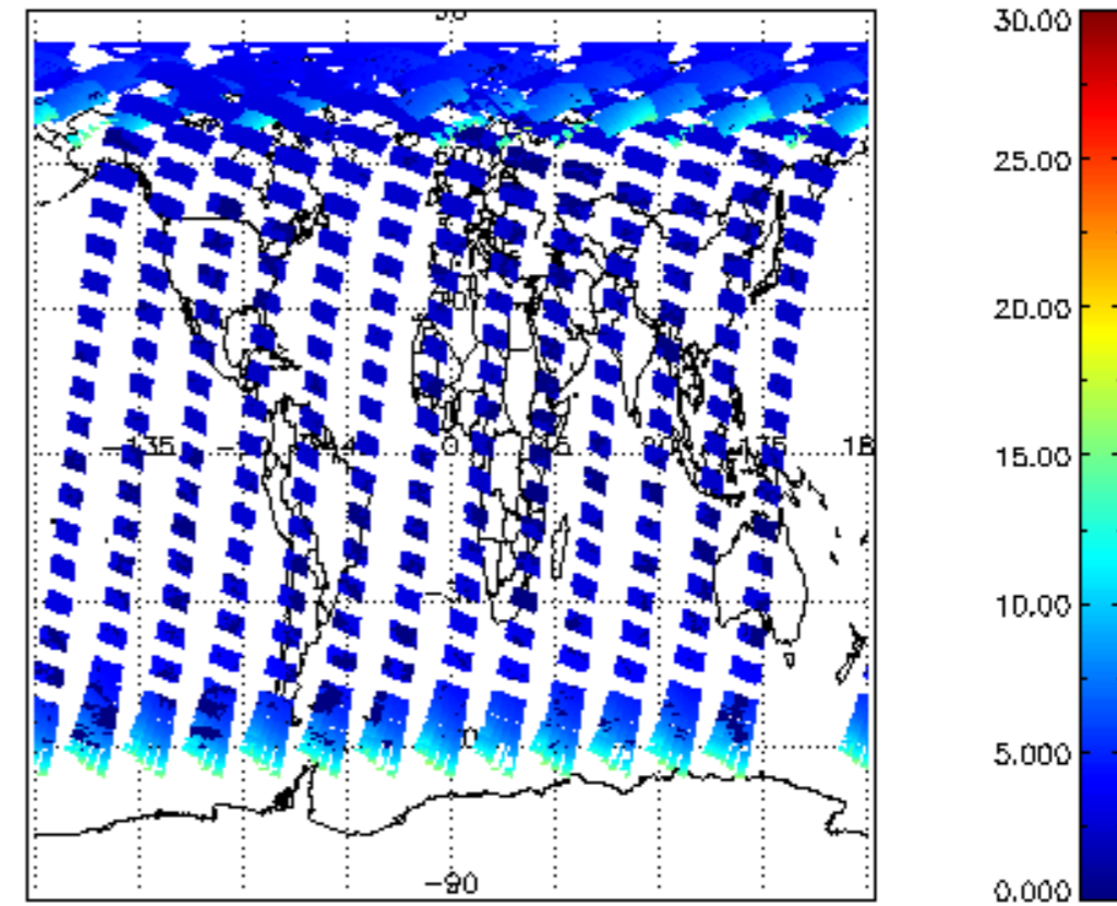
iCIOL2P_NADUV1NO2_amf_cl for 08MAY2004 00:00:00 to 09MAY2004 00:00:00
