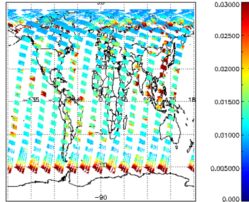
SCIOL2P_NADUV003_vcd_err for 08MAY2004 00:00:00 to 09MAY2004 00:00:00
