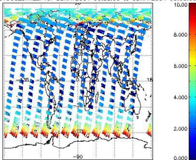
SCIOL2P_NADUV003_amf_cl for 08MAY2004 00:00:00 to 09MAY2004 00:00:00
