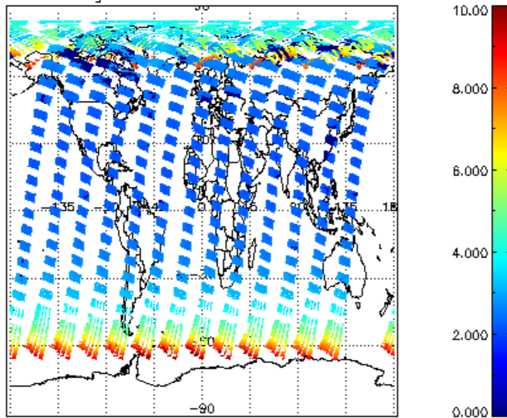
SCIOL2P_NADUV003_amf_gr for 08MAY2004 00:00:00 to 09MAY2004 00:00:00
