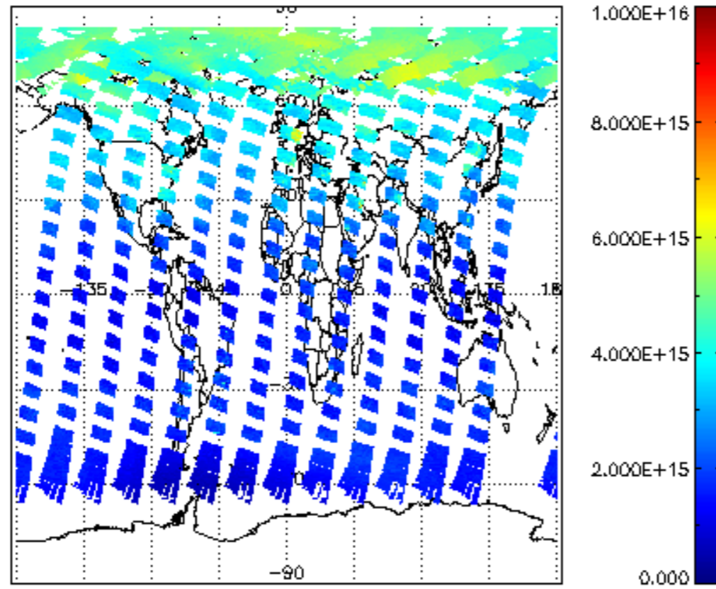
SCIOL2P_NADUV1NO2_vcd for 08MAY2004 00:00:00 to 09MAY2004 00:00:00
