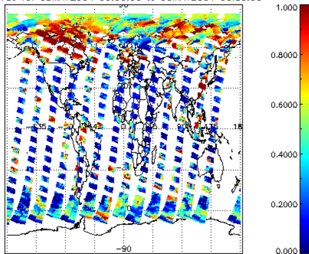
cl_frac for 08MAY2004 00:00:00 to 09MAY2004 00:00:00
