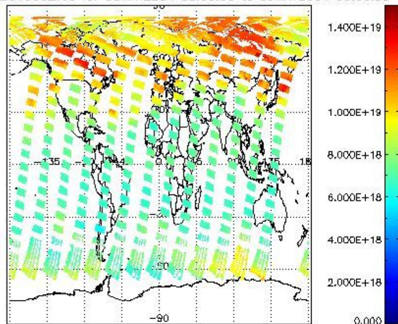
SCIOL2P_NADUV003_vcd for 08MAY2004 00:00:00 to 09MAY2004 00:00:00
