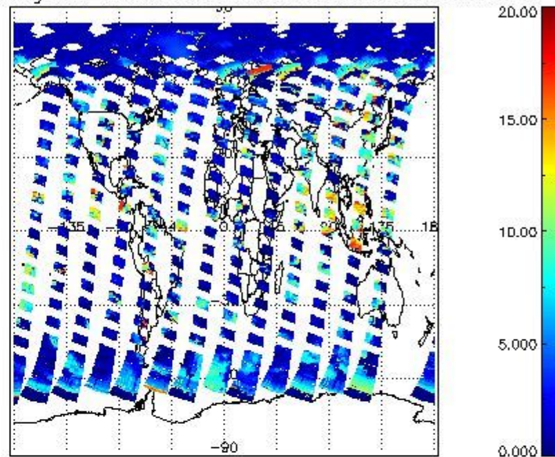
cL_top_height for 08MAY2004 00:00:00 to 09MAY2004 00:00:00
