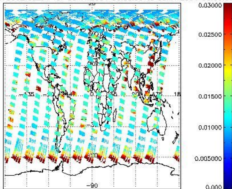
SCIOL2P_NADUV003_vcd_err for 08MAY2004 00:00:00 to 09MAY2004 00:00:00
