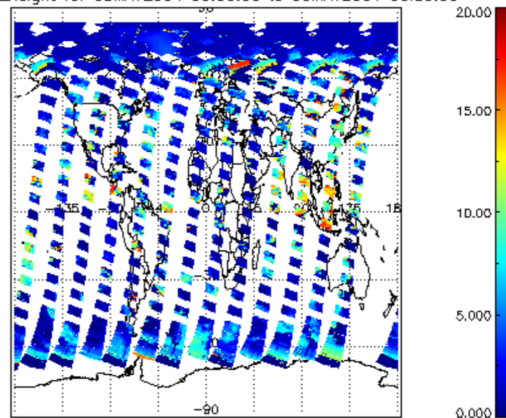
cl_top_height for 08MAY2004 00:00:00 to 09MAY2004 00:00:00
