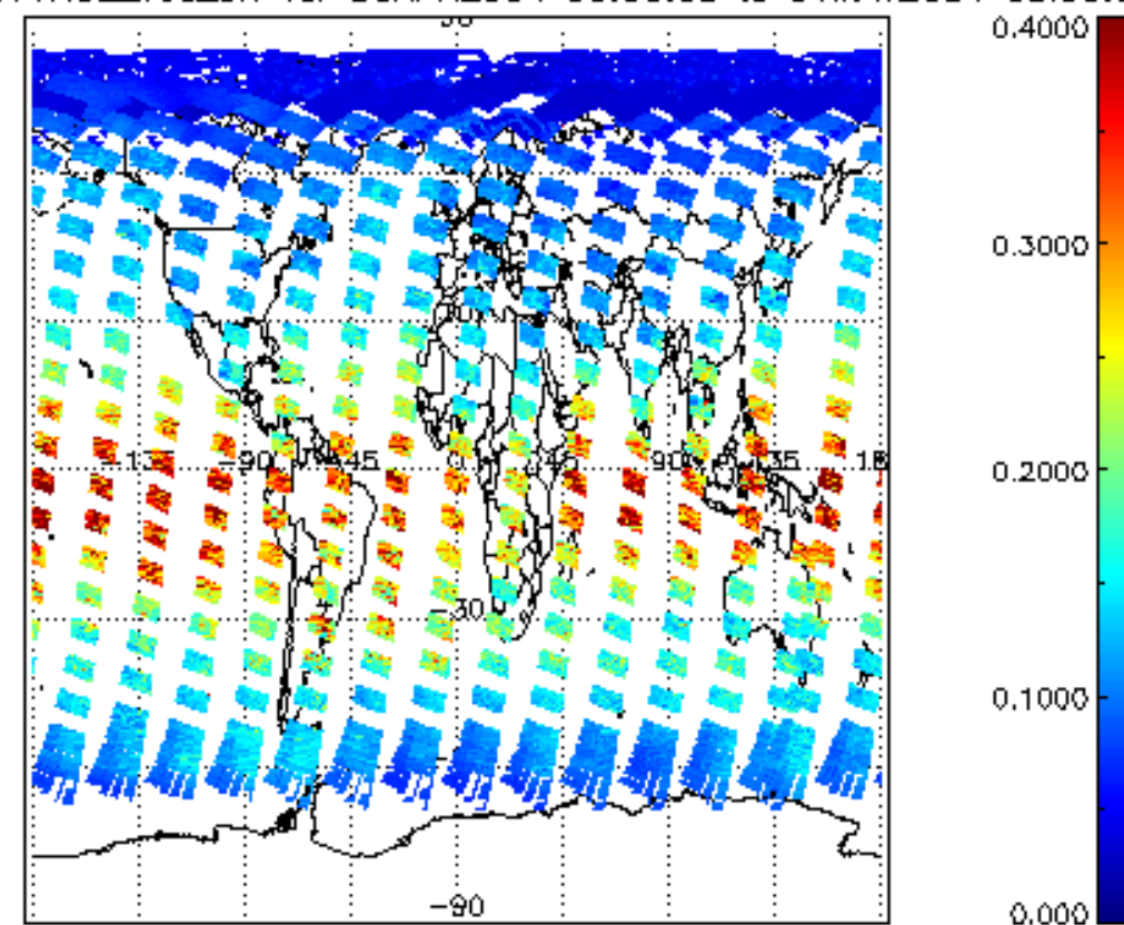
iCIOL2P_NADUV1NO2_vcd_err for 30APR2004 00:00:00 to 01MAY2004 00:00:00
