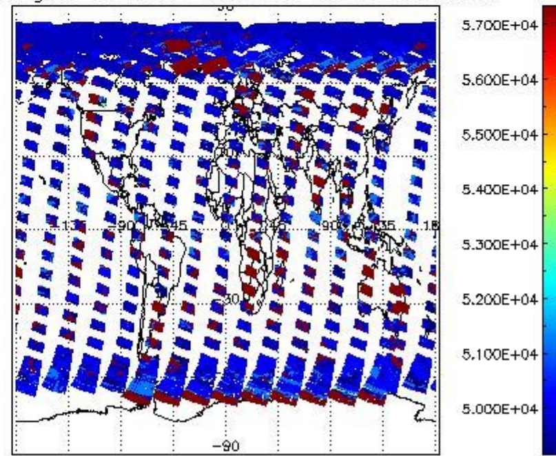
cloud_flags for 30APR2004 00:00:00 to 01MAY2004 00:00:00
