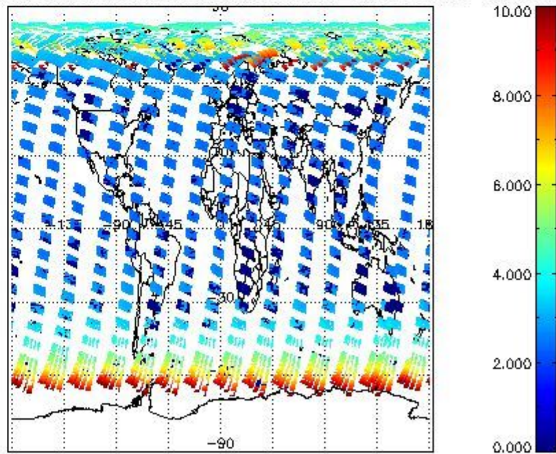
SCIOL2P_NADUV003_amf_cl for 30APR2004 00:00:00 to 01MAY2004 00:00:00
