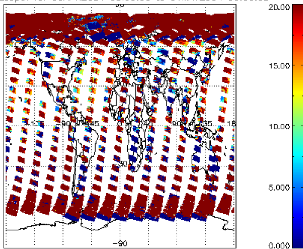
cl_opt_depth for 30APR2004 00:00:00 to 01MAY2004 00:00:00
