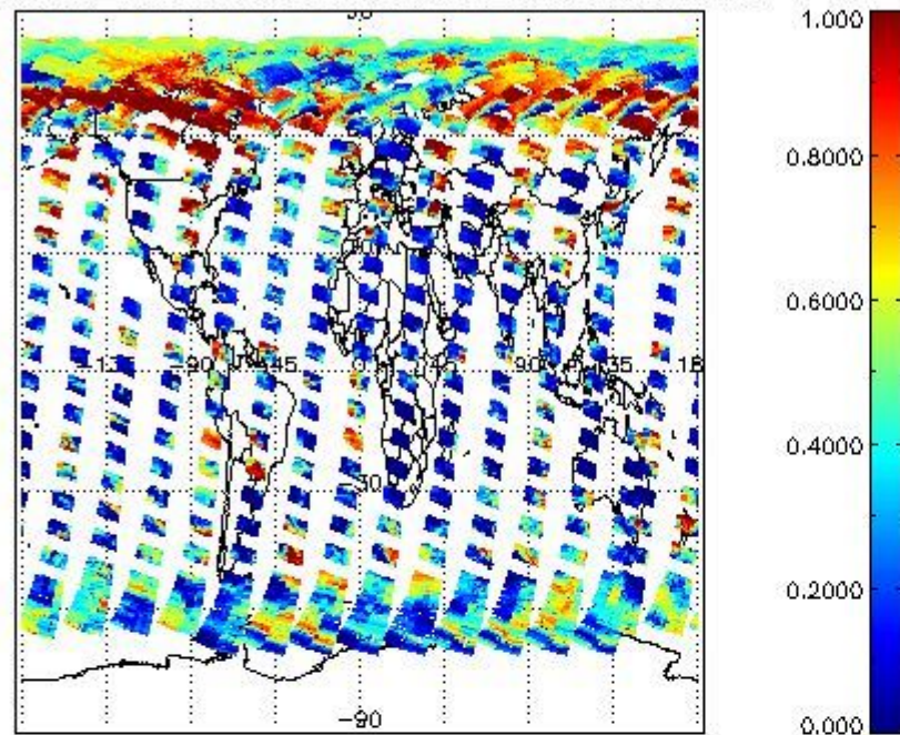
cL_frac for 30APR2004 00:00:00 to 01MAY2004 00:00:00
