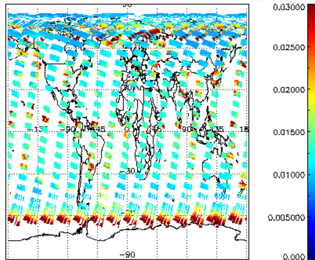
SCIOL2P_NADUV003_vcd_err for 30APR2004 00:00:00 to 01MAY2004 00:00:00
