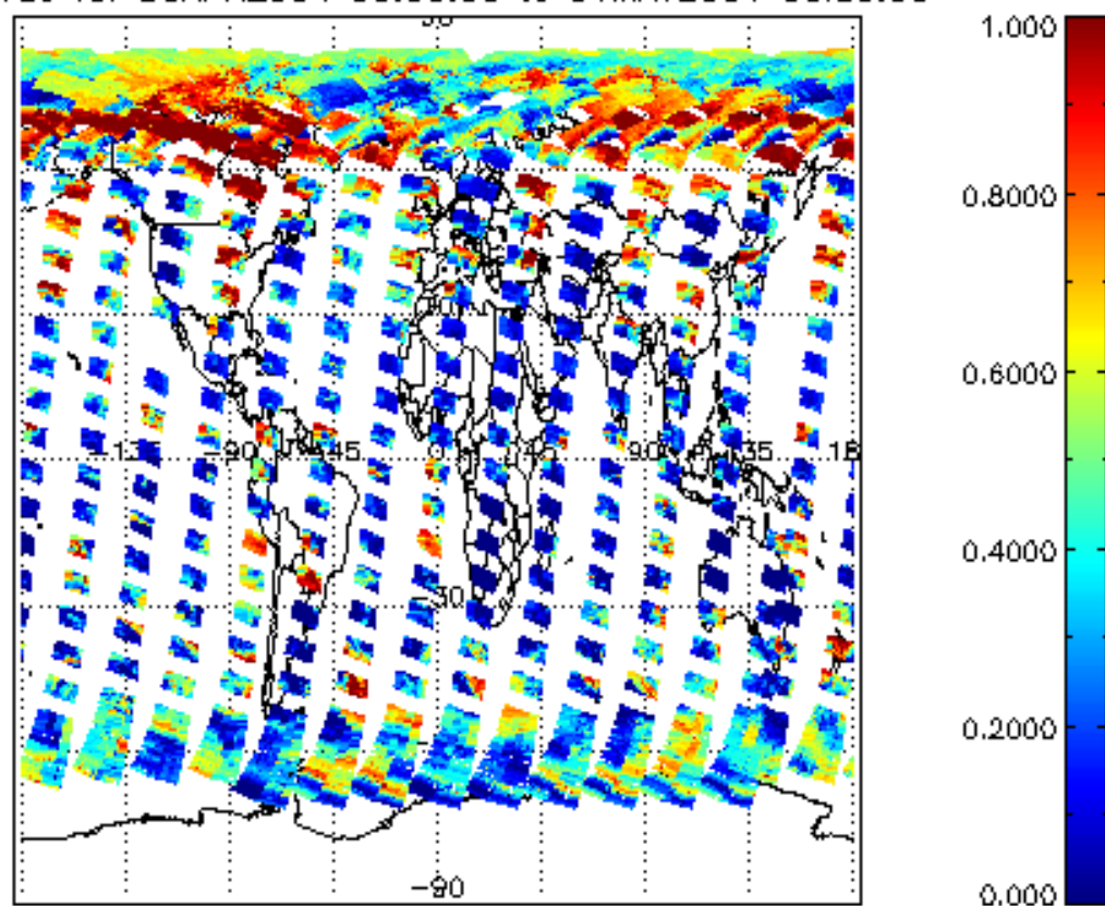
cl_frac for 30APR2004 00:00:00 to 01MAY2004 00:00:00
