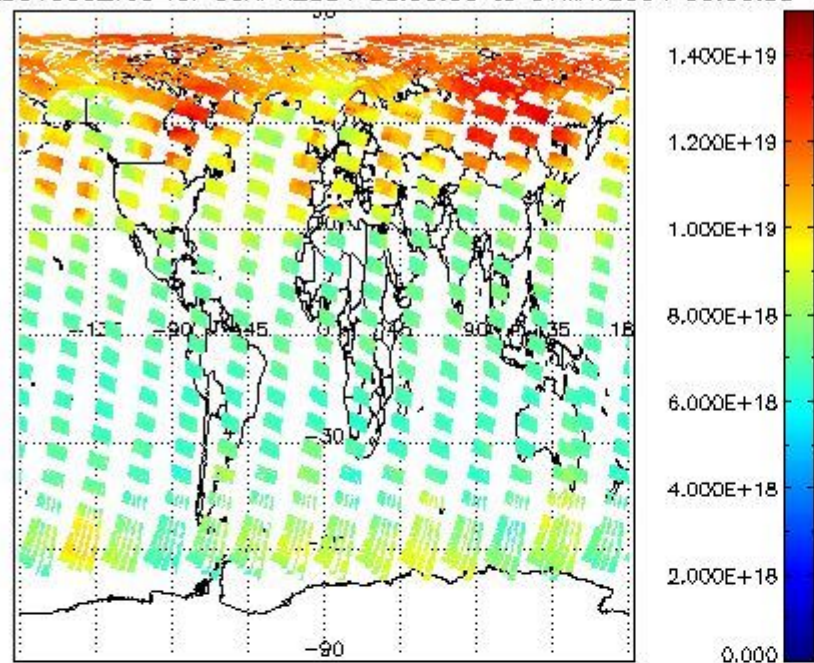
SCIOL2P_NADUV003_vcd for 30APR2004 00:00:00 to 01MAY2004 00:00:00
