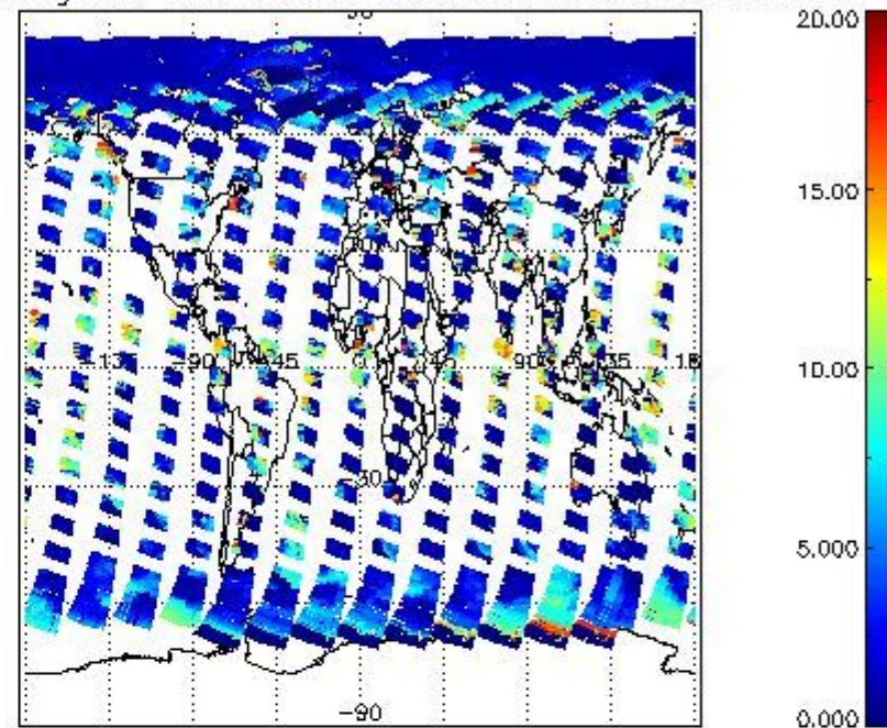
cL_top_height for 30APR2004 00:00:00 to 01MAY2004 00:00:00
