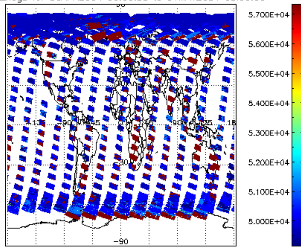
cloud_flags for 30APR2004 00:00:00 to 01MAY2004 00:00:00
