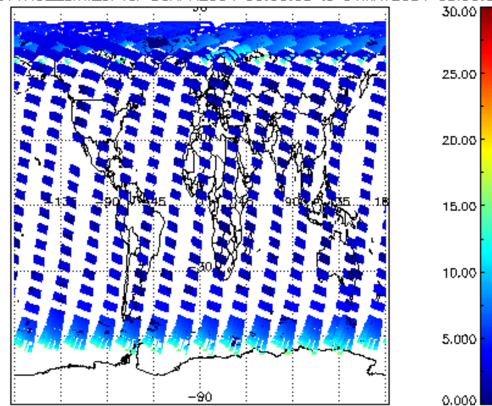
iCIOL2P_NADUV1NO2_amf_cl for 30APR2004 00:00:00 to 01MAY2004 00:00:00
