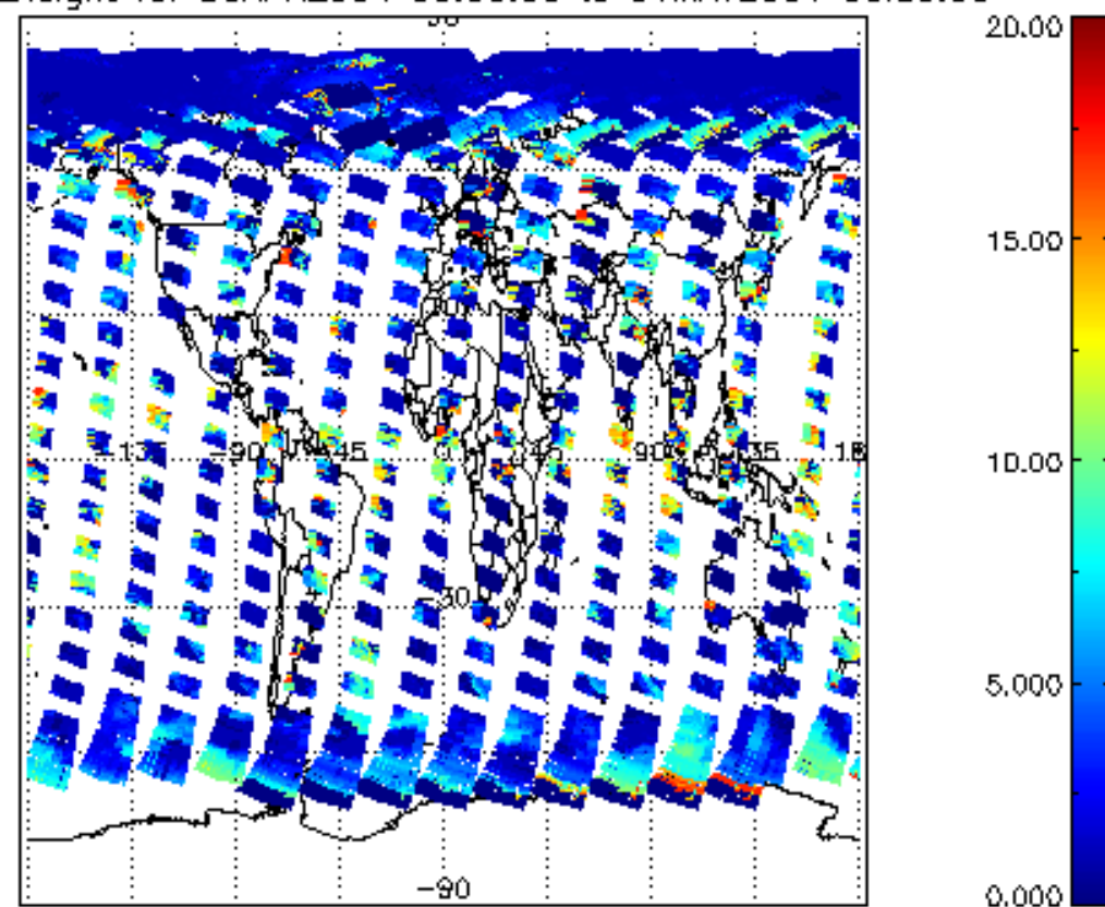
cl_top_height for 30APR2004 00:00:00 to 01MAY2004 00:00:00
