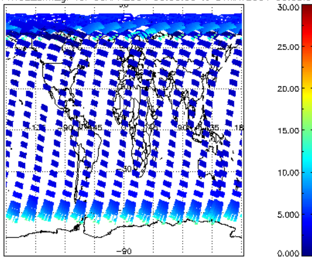
iCIOL2P_NADUV1NO2_amf_gr for 30APR2004 00:00:00 to 01MAY2004 00:00:00
