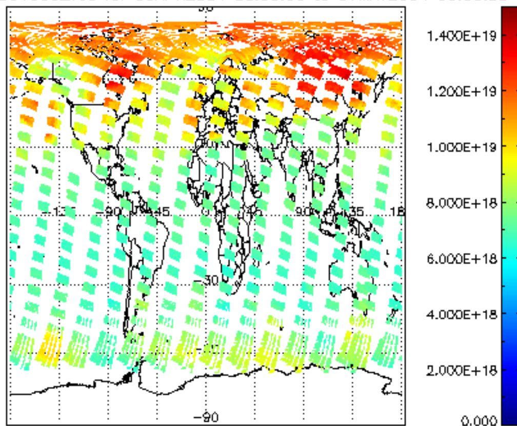
SCIOL2P_NADUV003_vcd for 30APR2004 00:00:00 to 01MAY2004 00:00:00
