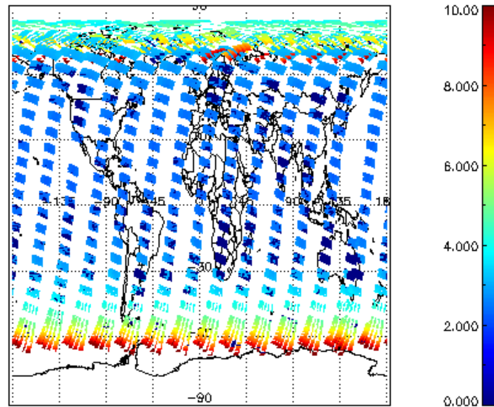
SCIOL2P_NADUV003_amf_cl for 30APR2004 00:00:00 to 01MAY2004 00:00:00
