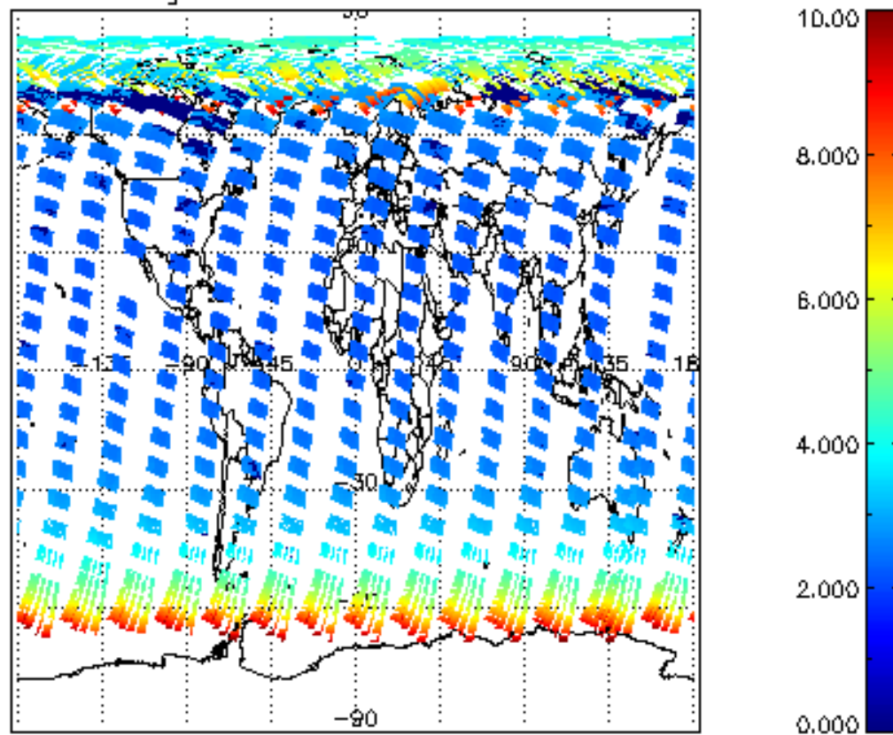
SCIOL2P_NADUV003_amf_gr for 30APR2004 00:00:00 to 01MAY2004 00:00:00
