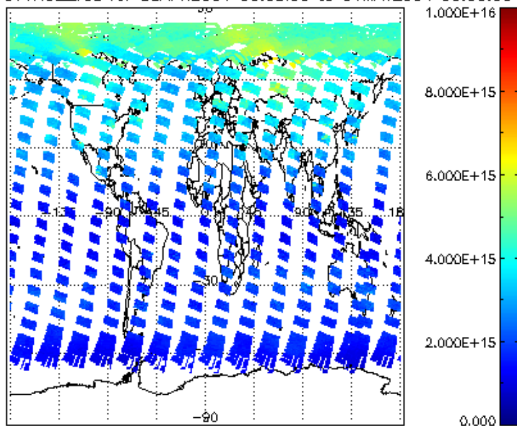
SCIOL2P_NADUV1NO2_vcd for 30APR2004 00:00:00 to 01MAY2004 00:00:00
