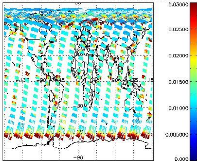
SCIOL2P_NADUV003_vcd_err for 30APR2004 00:00:00 to 01MAY2004 00:00:00
