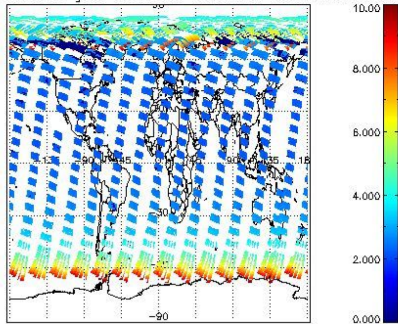
SCIOL2P_NADUV003_amf_gr for 30APR2004 00:00:00 to 01MAY2004 00:00:00
