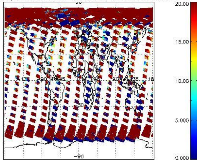
cL_opt_depth for 30APR2004 00:00:00 to 01MAY2004 00:00:00
