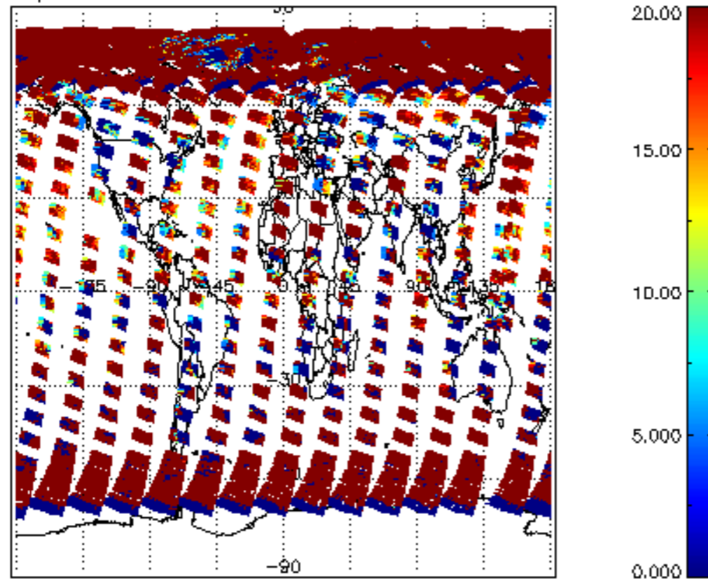
cl_opt_depth for 29APR2004 00:00:00 to 30APR2004 00:00:00
