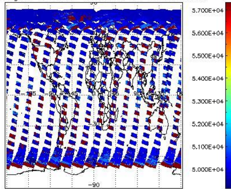
cloud_flags for 29APR2004 00:00:00 to 30APR2004 00:00:00
