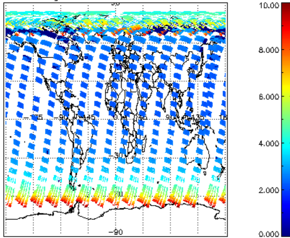
SCIOL2P_NADUV003_amf_gr for 29APR2004 00:00:00 to 30APR2004 00:00:00
