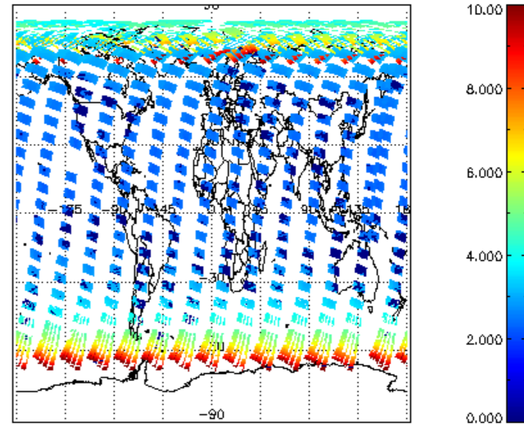
SCIOL2P_NADUV003_amf_cl for 29APR2004 00:00:00 to 30APR2004 00:00:00
