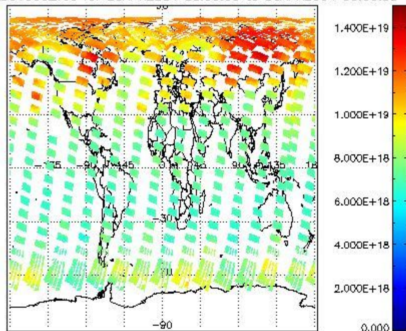
SCIOL2P_NADUV003_vcd for 29APR2004 00:00:00 to 30APR2004 00:00:00
