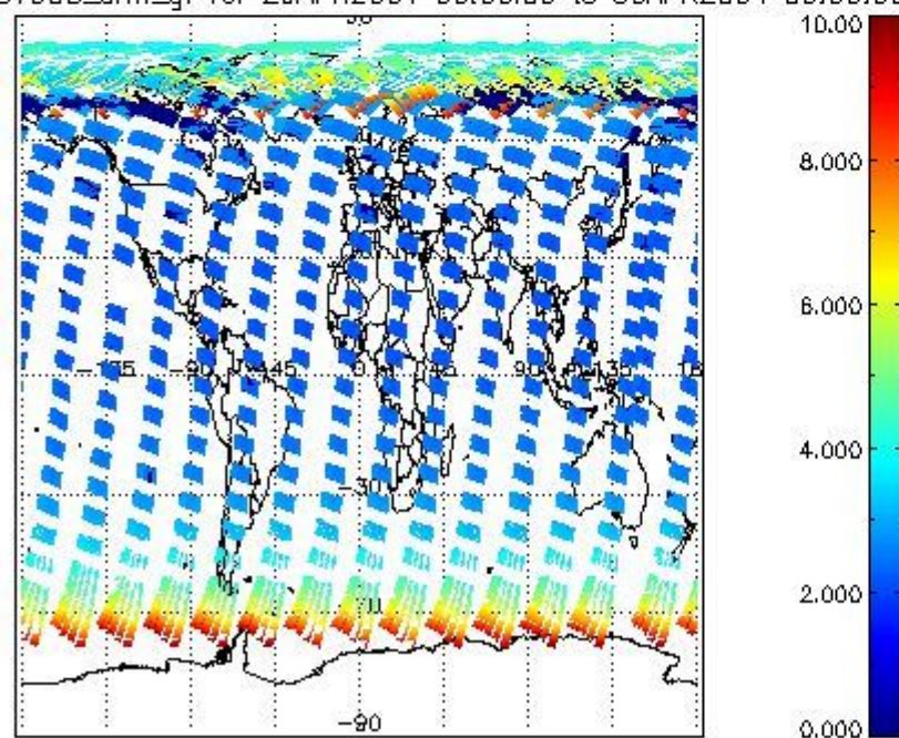
SCIOL2P_NADUV003_amf_gr for 29APR2004 00:00:00 to 30APR2004 00:00:00
