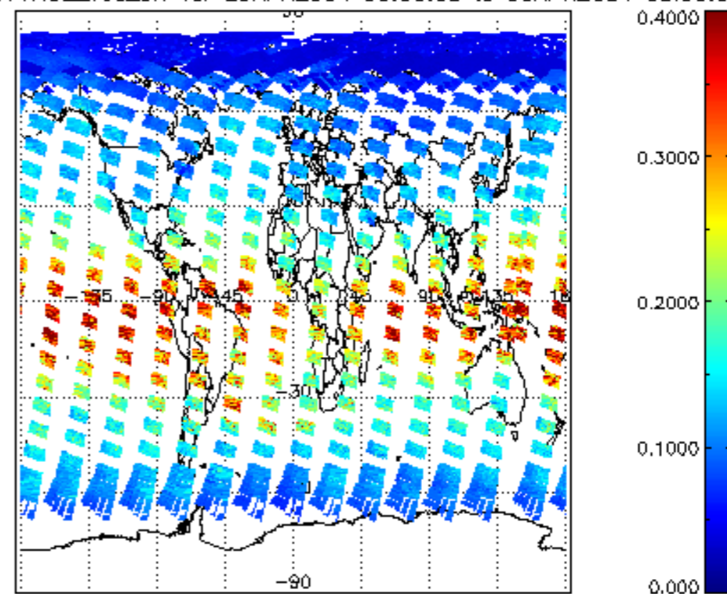
iCIOL2P_NADUV1NO2_vcd_err for 29APR2004 00:00:00 to 30APR2004 00:00:00
