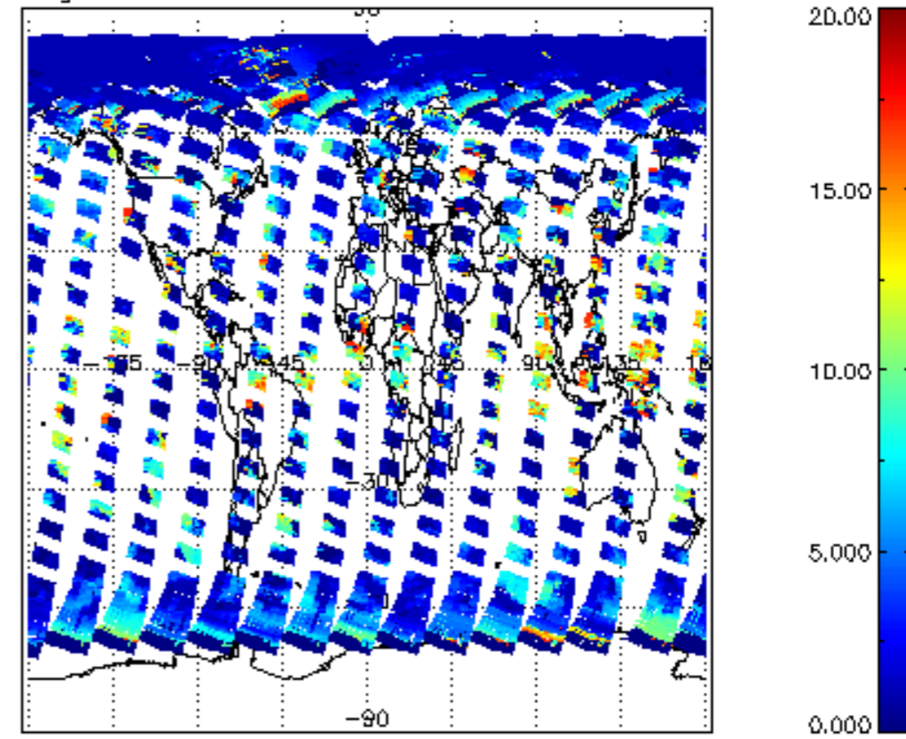
cl_top_height for 29APR2004 00:00:00 to 30APR2004 00:00:00
