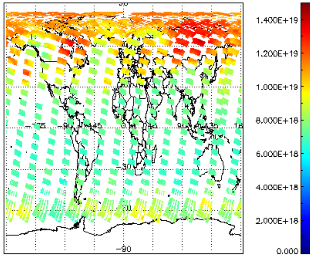
SCIOL2P_NADUV003_vcd for 29APR2004 00:00:00 to 30APR2004 00:00:00
