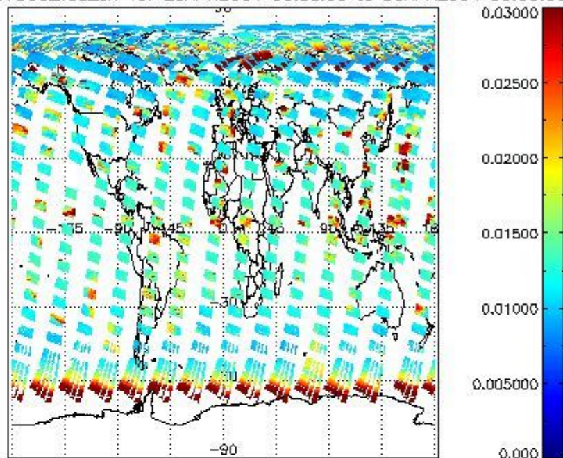
SCIOL2P_NADUV003_vcd_err for 29APR2004 00:00:00 to 30APR2004 00:00:00
