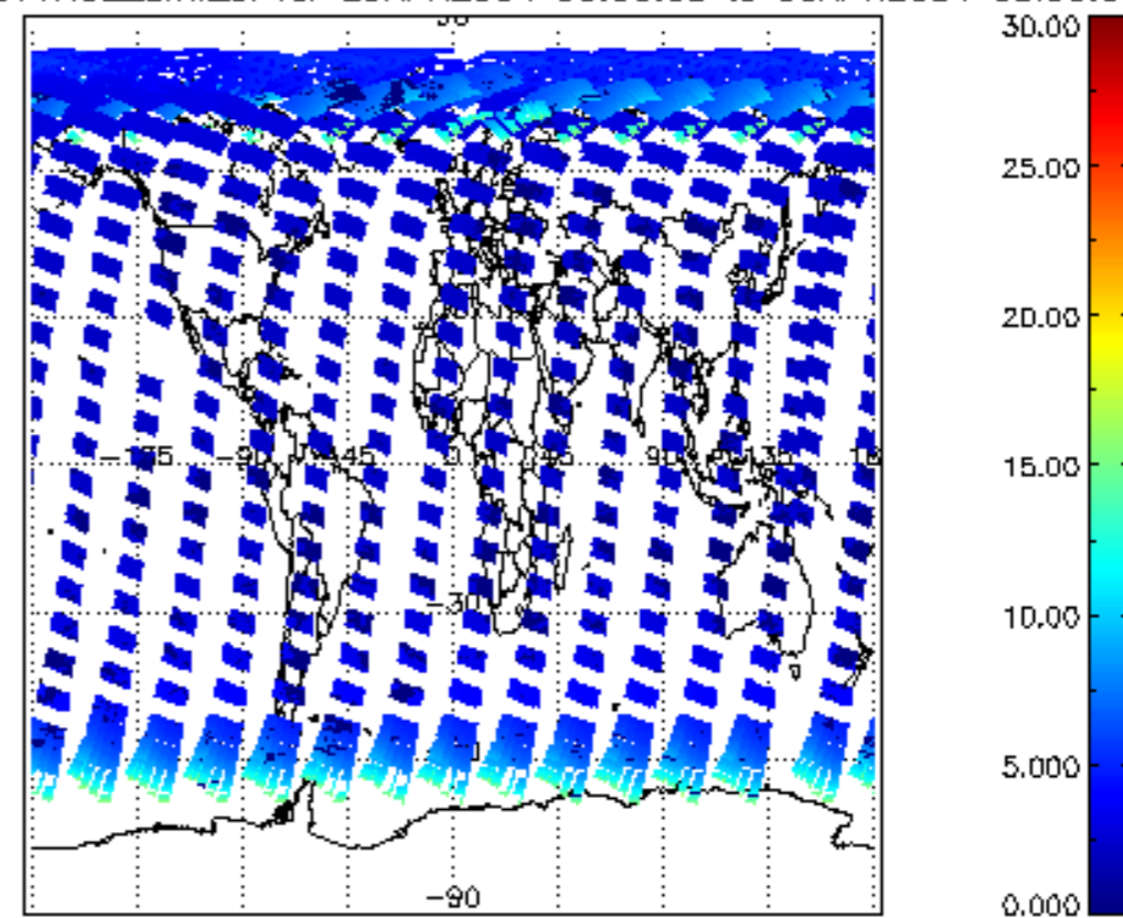
iCIOL2P_NADUV1NO2_amf_cl for 29APR2004 00:00:00 to 30APR2004 00:00:00
