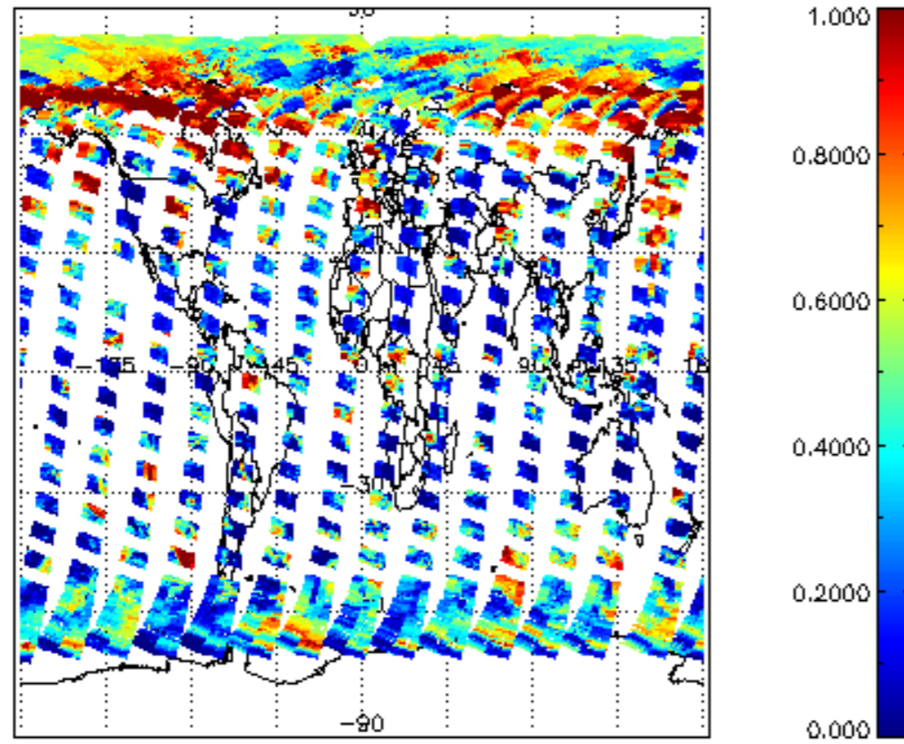
cl_frac for 29APR2004 00:00:00 to 30APR2004 00:00:00
