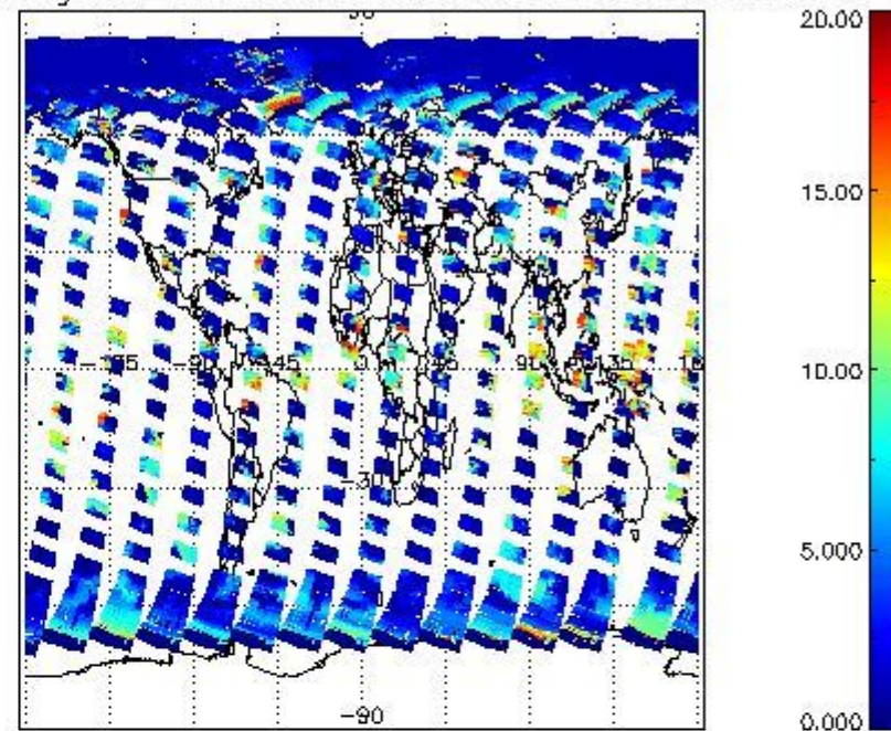
cL_top_height for 29APR2004 00:00:00 to 30APR2004 00:00:00
