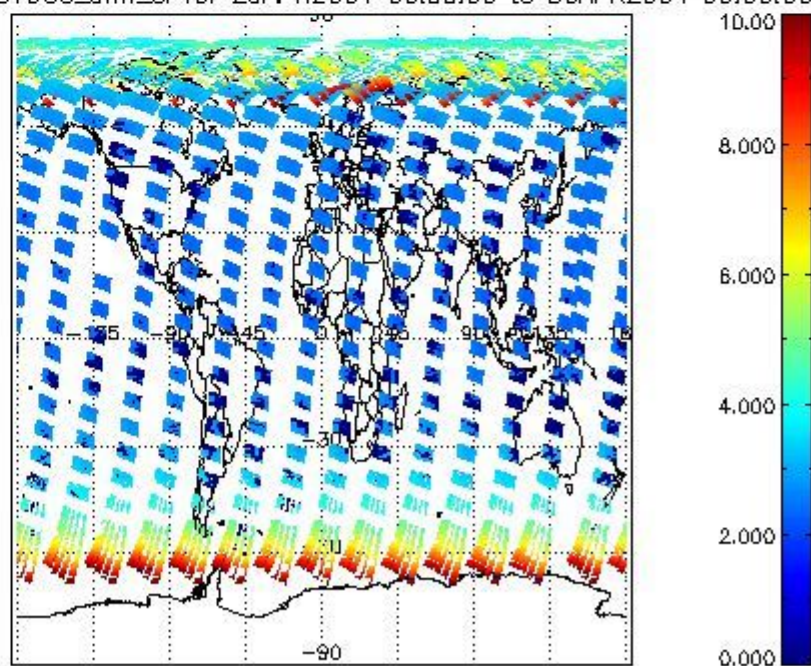
SCIOL2P_NADUV003_amf_cl for 29APR2004 00:00:00 to 30APR2004 00:00:00
