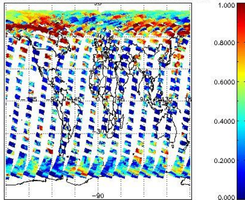
cL_frac for 29APR2004 00:00:00 to 30APR2004 00:00:00
