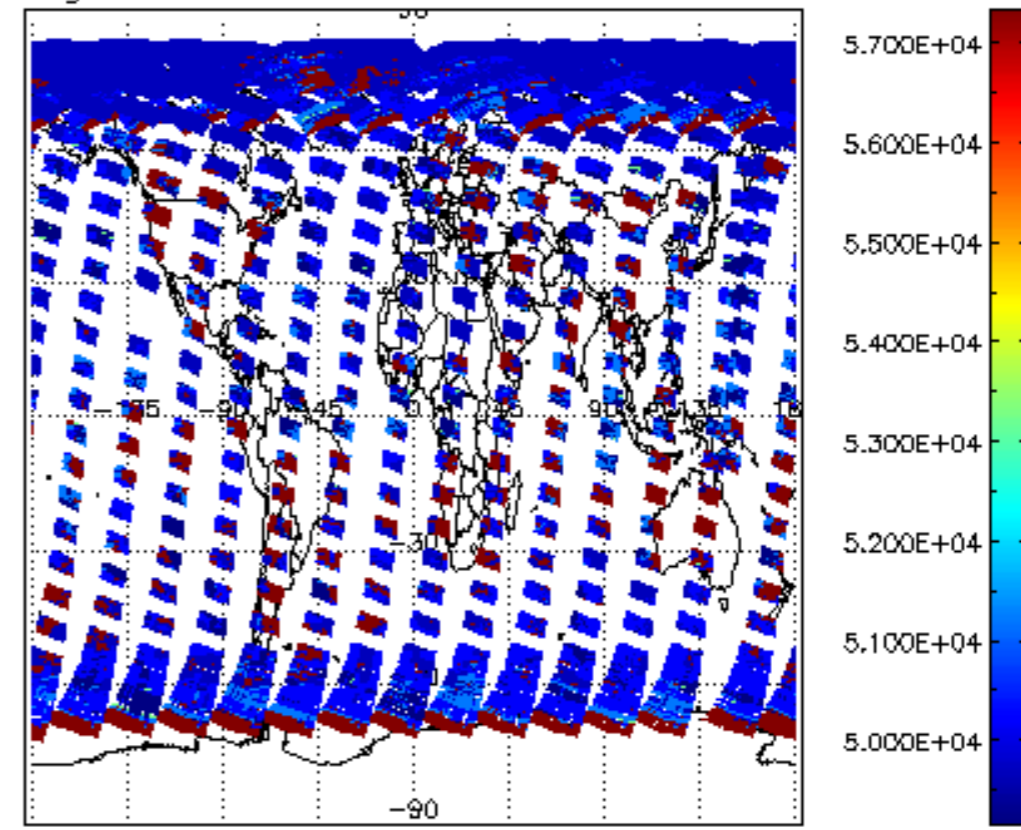
cloud_flags for 29APR2004 00:00:00 to 30APR2004 00:00:00
