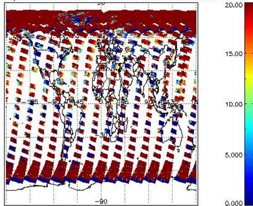
cL_opt_depth for 29APR2004 00:00:00 to 30APR2004 00:00:00
