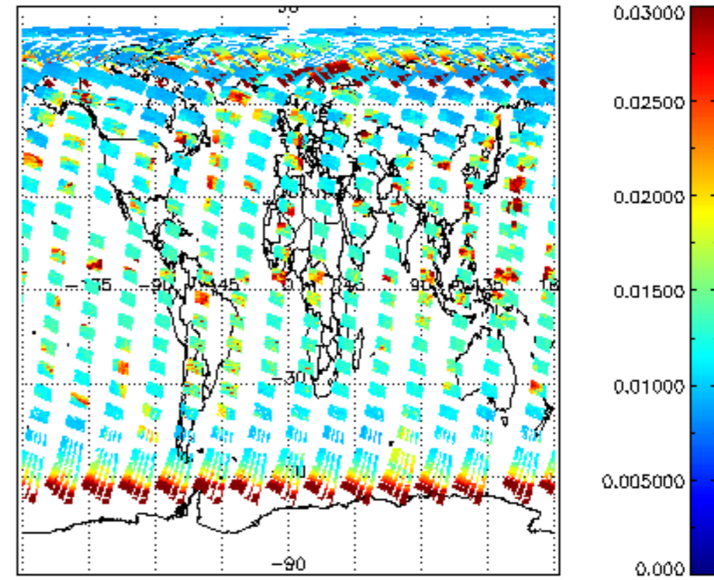
SCIOL2P_NADUV003_vcd_err for 29APR2004 00:00:00 to 30APR2004 00:00:00
