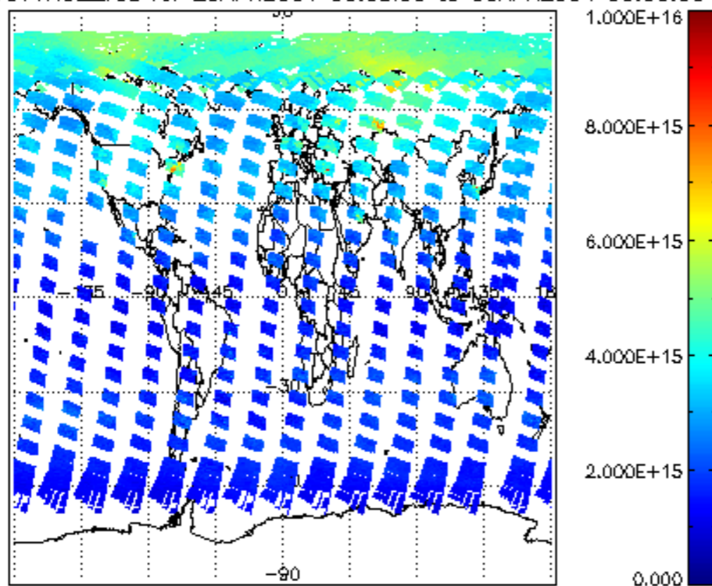
SCIOL2P_NADUV1NO2_vcd for 29APR2004 00:00:00 to 30APR2004 00:00:00
