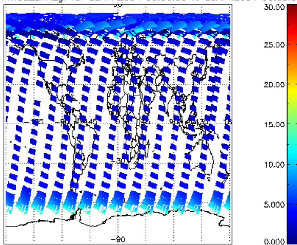
iCIOL2P_NADUV1NO2_amf_gr for 29APR2004 00:00:00 to 30APR2004 00:00:00
