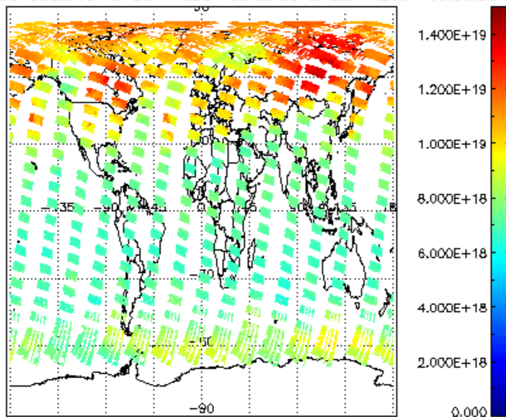
SCIOL2P_NADUV003_vcd for 28APR2004 00:00:00 to 29APR2004 00:00:00
