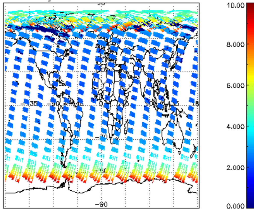
SCIOL2P_NADUV003_amf_gr for 28APR2004 00:00:00 to 29APR2004 00:00:00
