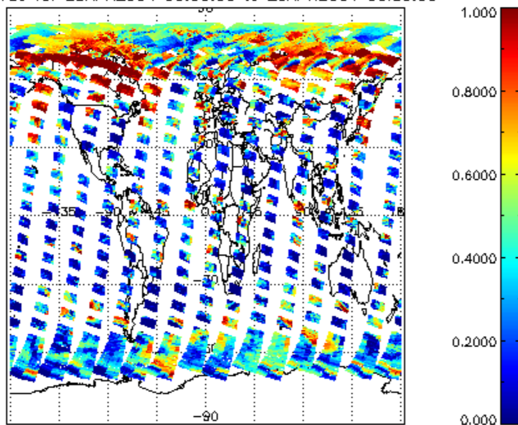
cl_frac for 28APR2004 00:00:00 to 29APR2004 00:00:00
