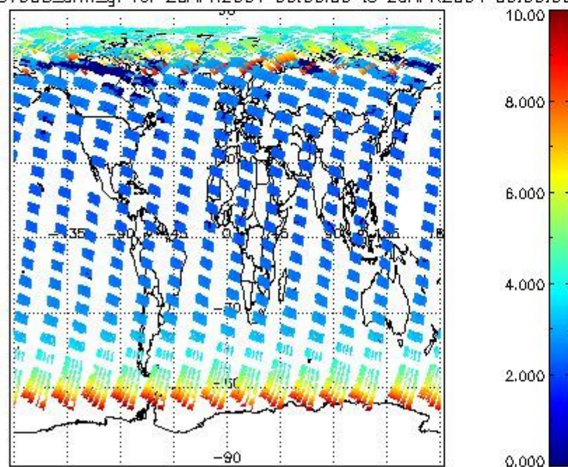
SCIOL2P_NADUV003_amf_gr for 28APR2004 00:00:00 to 29APR2004 00:00:00
