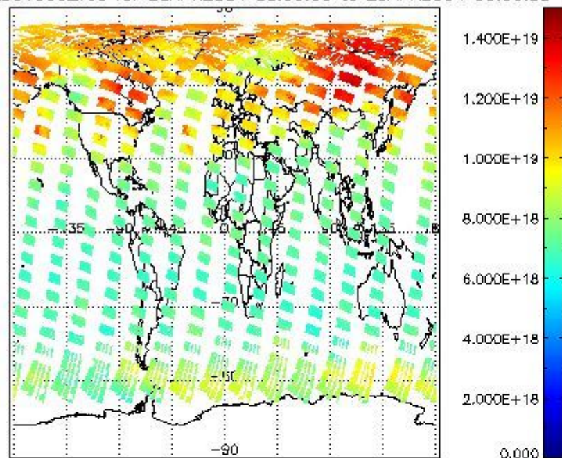
SCIOL2P_NADUV003_vcd for 28APR2004 00:00:00 to 29APR2004 00:00:00
