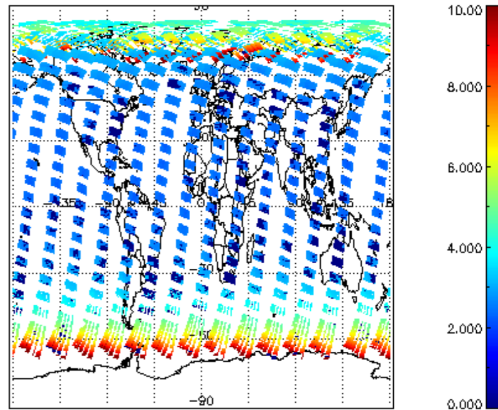
SCIOL2P_NADUV003_amf_cl for 28APR2004 00:00:00 to 29APR2004 00:00:00
