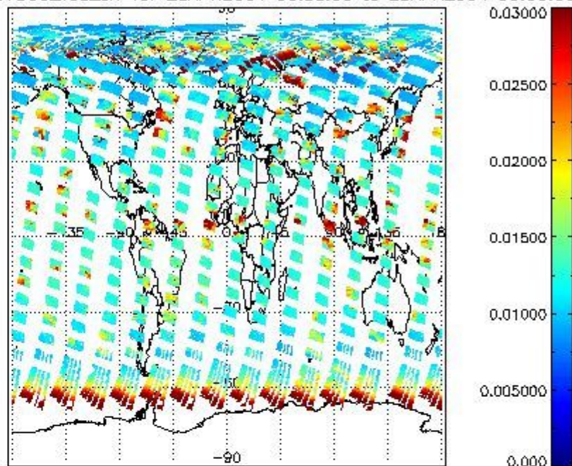
SCIOL2P_NADUV003_vcd_err for 28APR2004 00:00:00 to 29APR2004 00:00:00
