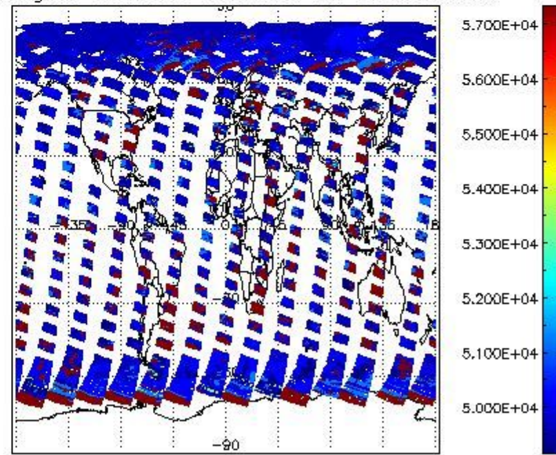
cloud_flags for 28APR2004 00:00:00 to 29APR2004 00:00:00
