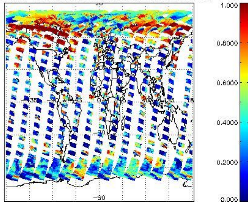
cL_frac for 28APR2004 00:00:00 to 29APR2004 00:00:00
