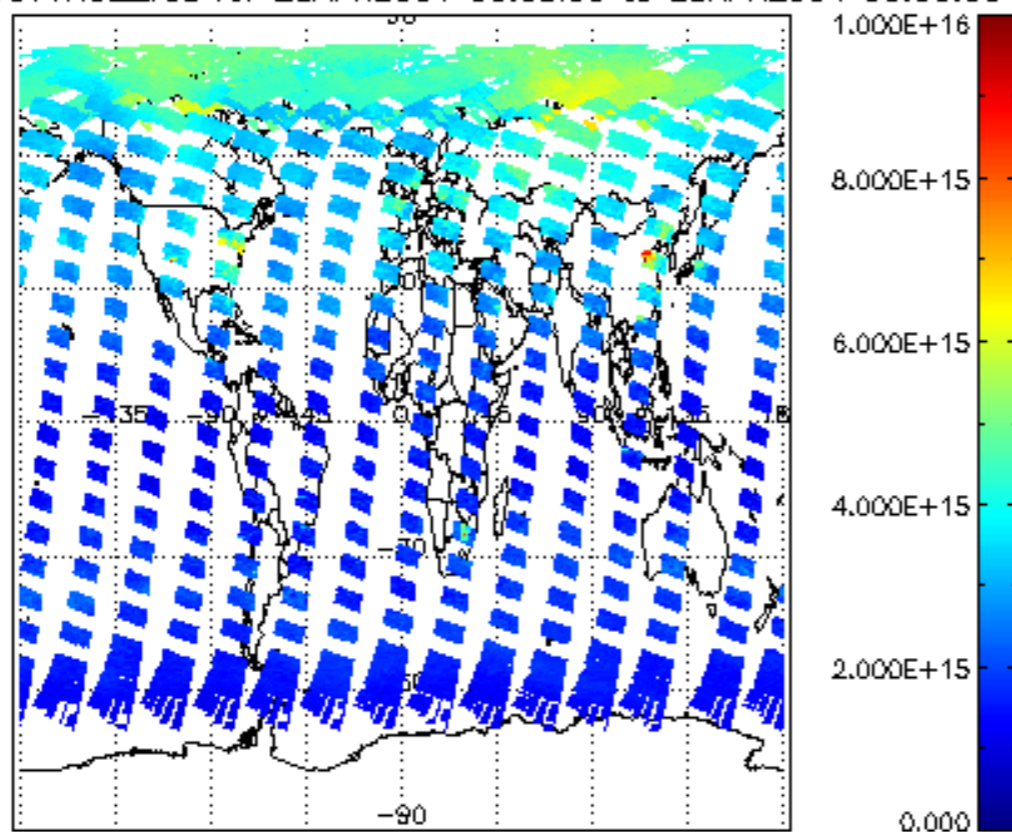
SCIOL2P_NADUV1NO2_vcd for 28APR2004 00:00:00 to 29APR2004 00:00:00
