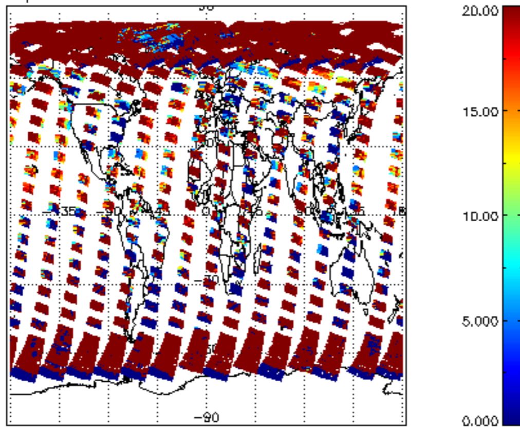
cl_opt_depth for 28APR2004 00:00:00 to 29APR2004 00:00:00
