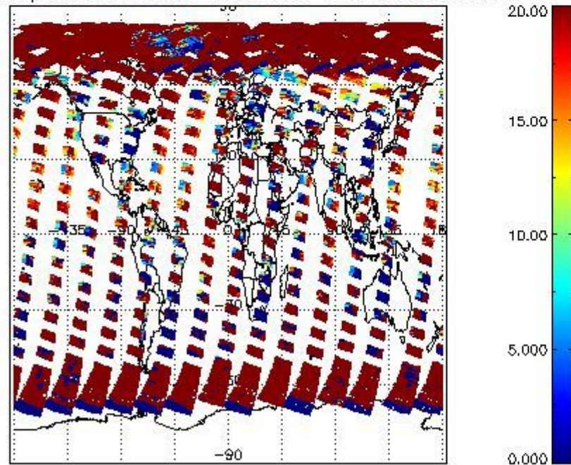
cL_opt_depth for 28APR2004 00:00:00 to 29APR2004 00:00:00
