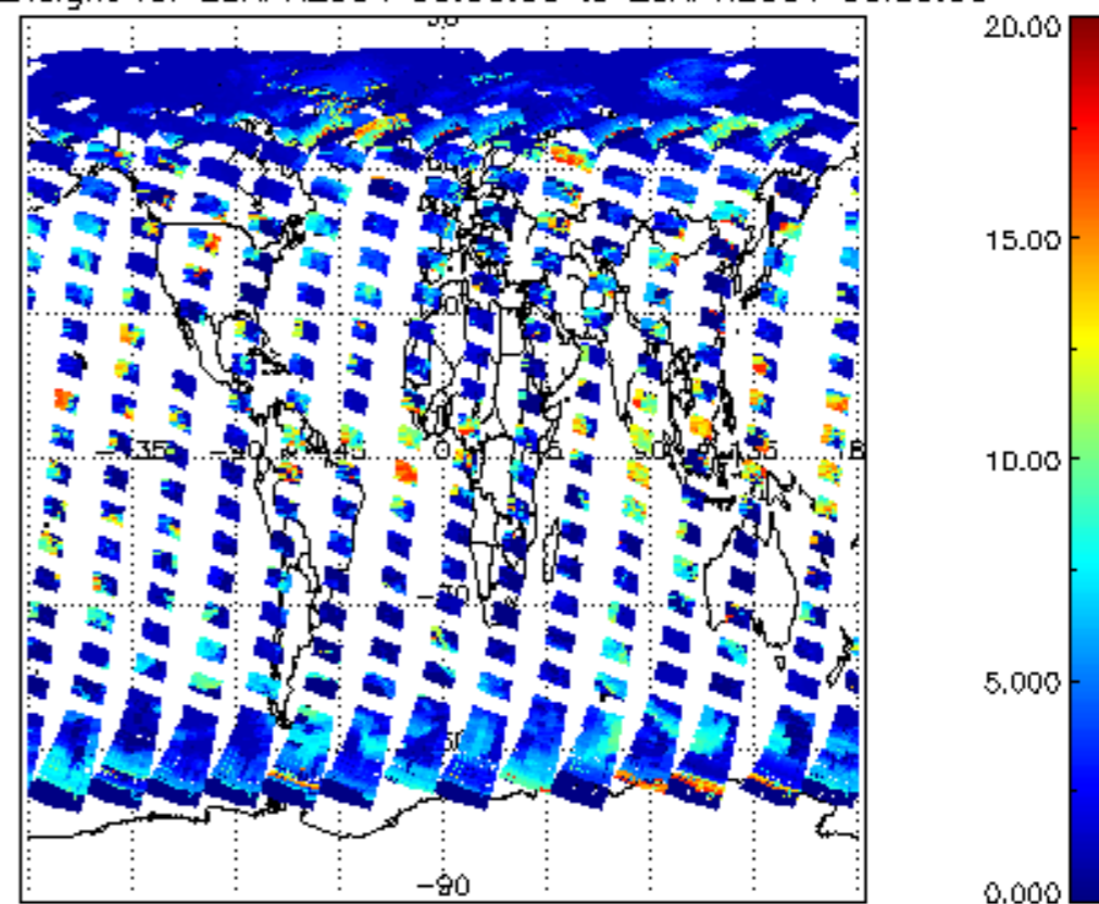
cl_top_height for 28APR2004 00:00:00 to 29APR2004 00:00:00
