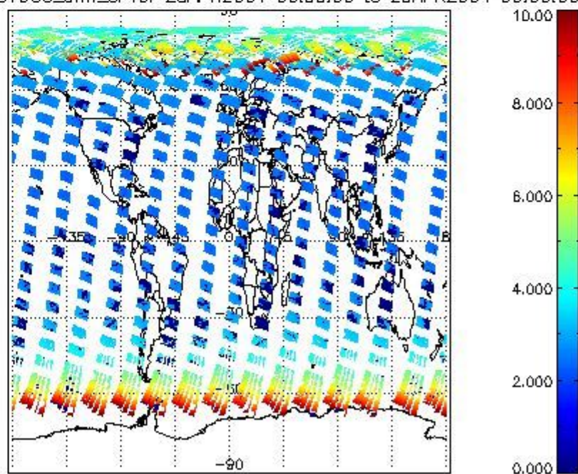
SCIOL2P_NADUV003_amf_cl for 28APR2004 00:00:00 to 29APR2004 00:00:00
