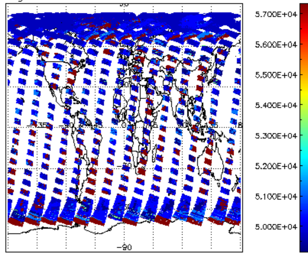
cloud_flags for 28APR2004 00:00:00 to 29APR2004 00:00:00
