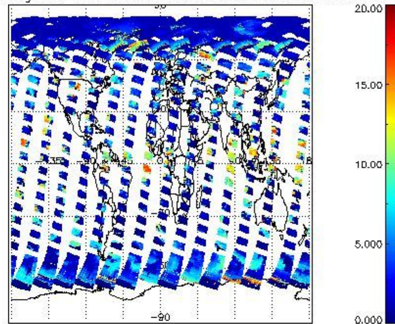
cL_top_height for 28APR2004 00:00:00 to 29APR2004 00:00:00
