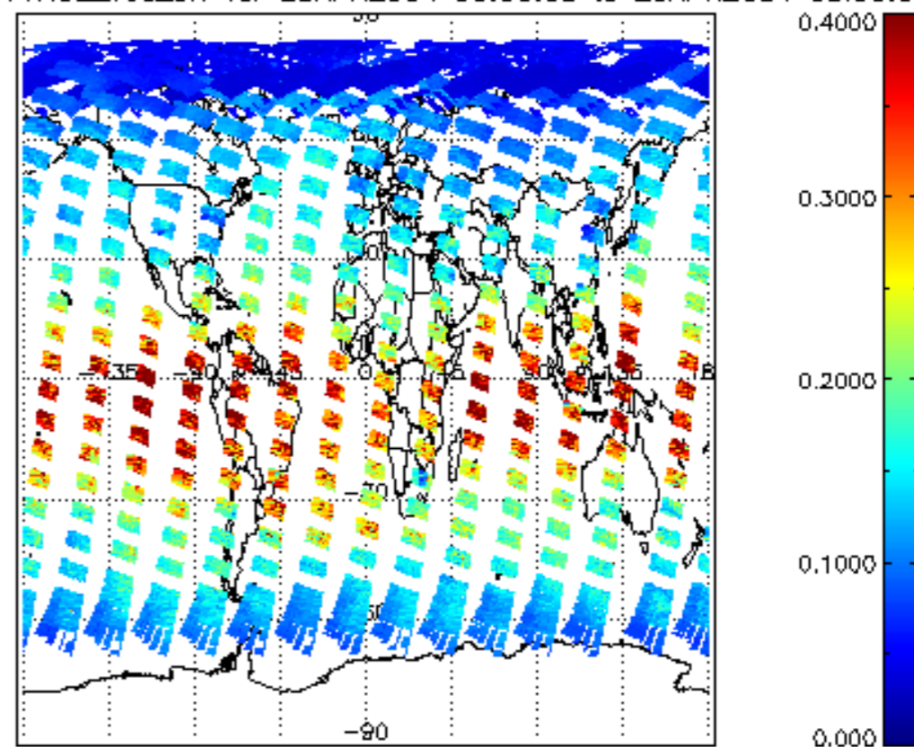
iCIOL2P_NADUV1NO2_vcd_err for 28APR2004 00:00:00 to 29APR2004 00:00:00
