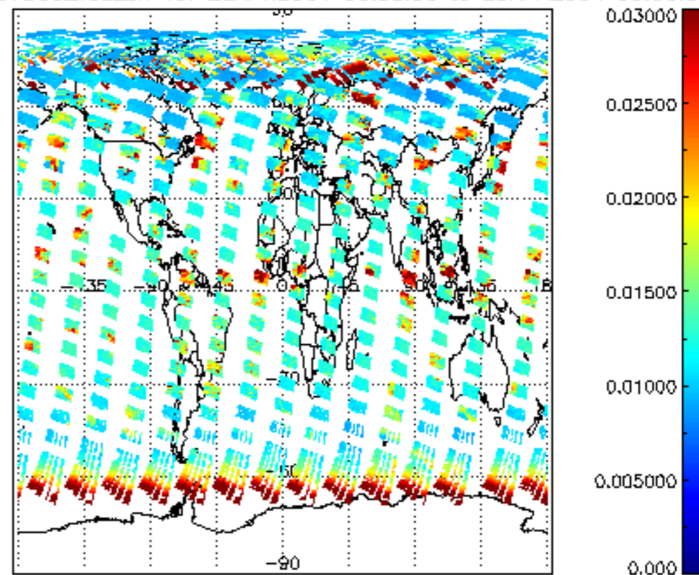
SCIOL2P_NADUV003_vcd_err for 28APR2004 00:00:00 to 29APR2004 00:00:00
