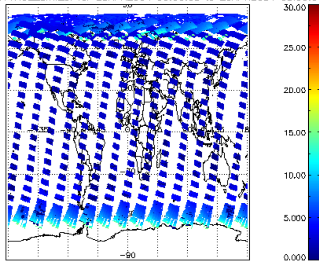
iCIOL2P_NADUV1NO2_amf_cl for 28APR2004 00:00:00 to 29APR2004 00:00:00
