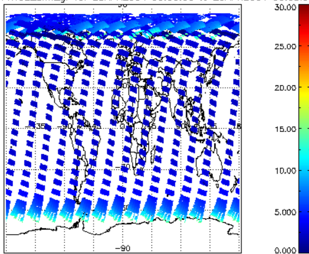
iCIOL2P_NADUV1NO2_amf_gr for 28APR2004 00:00:00 to 29APR2004 00:00:00
