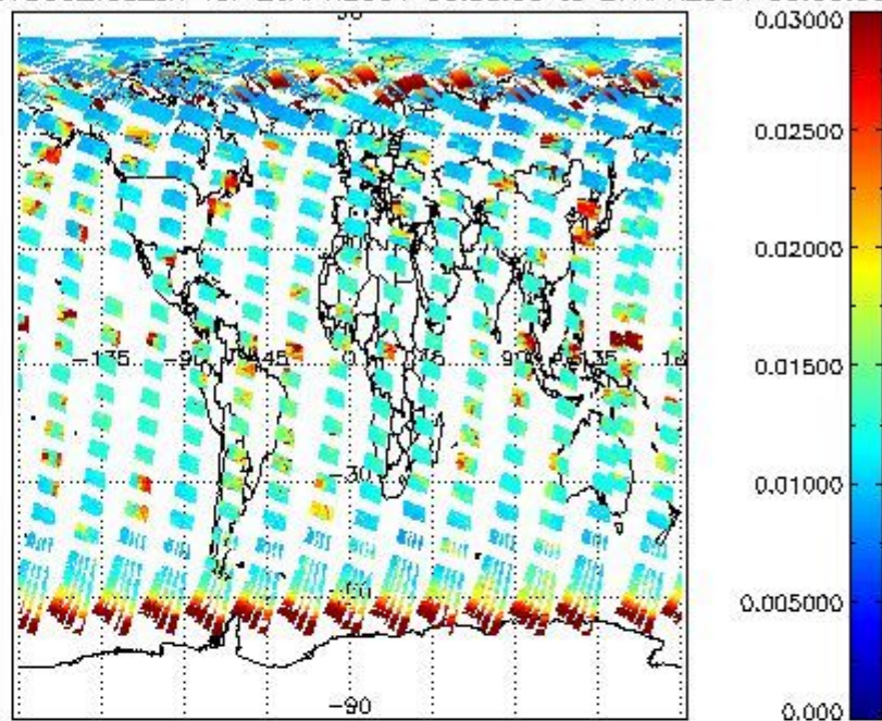
SCIOL2P_NADUV003_vcd_err for 26APR2004 00:00:00 to 27APR2004 00:00:00
