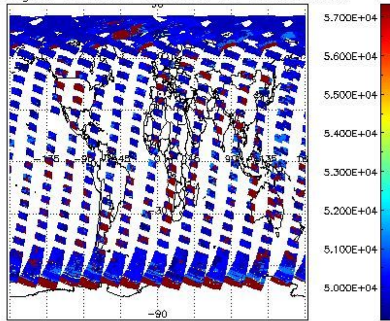
cloud_flags for 26APR2004 00:00:00 to 27APR2004 00:00:00
