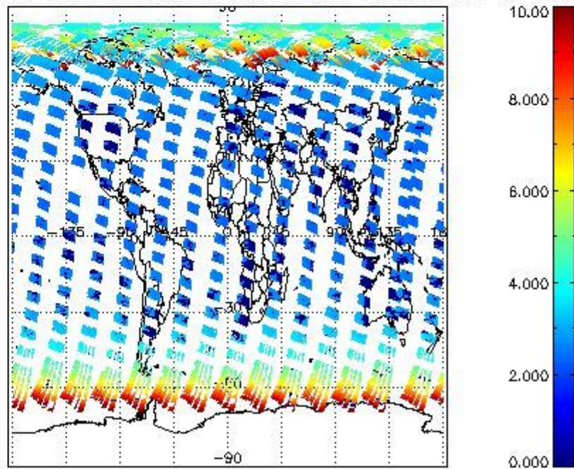
SCIOL2P_NADUV003_amf_cl for 26APR2004 00:00:00 to 27APR2004 00:00:00
