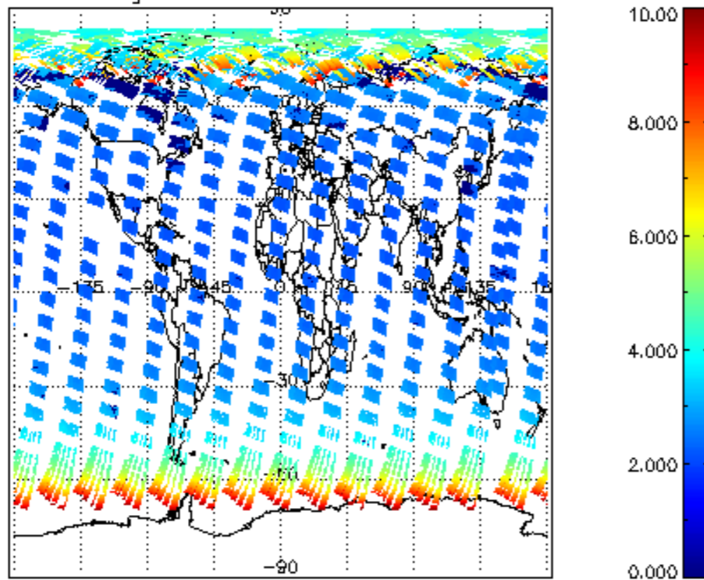
SCIOL2P_NADUV003_amf_gr for 26APR2004 00:00:00 to 27APR2004 00:00:00
