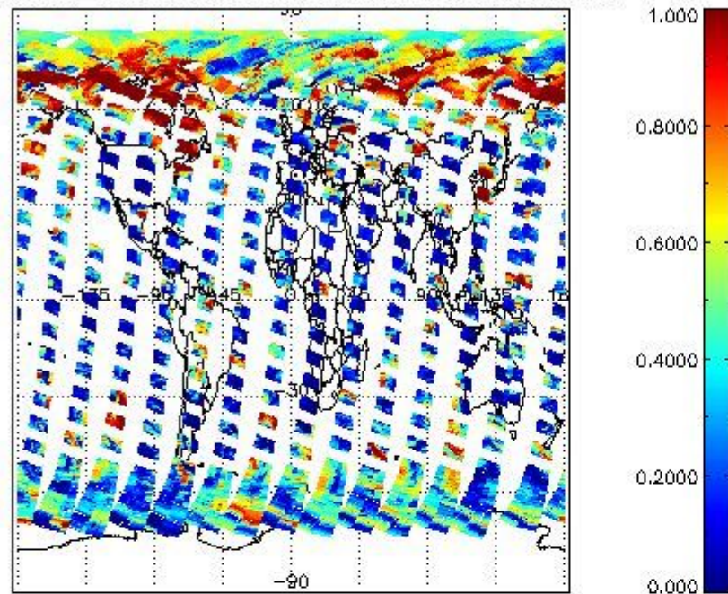
cL_frac for 26APR2004 00:00:00 to 27APR2004 00:00:00
