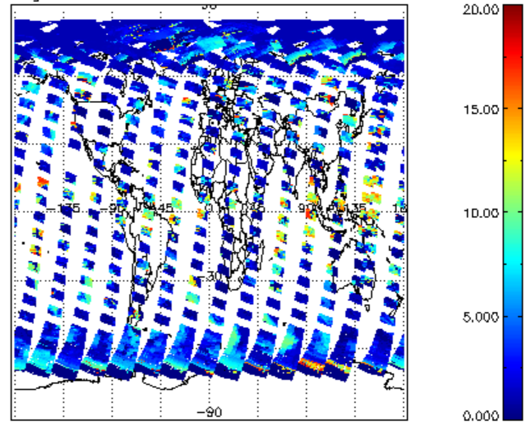
cl_top_height for 26APR2004 00:00:00 to 27APR2004 00:00:00
