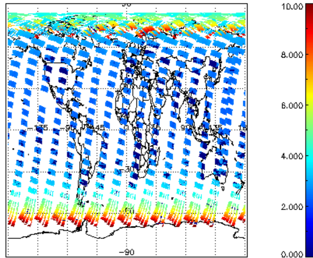
SCIOL2P_NADUV003_amf_cl for 26APR2004 00:00:00 to 27APR2004 00:00:00
