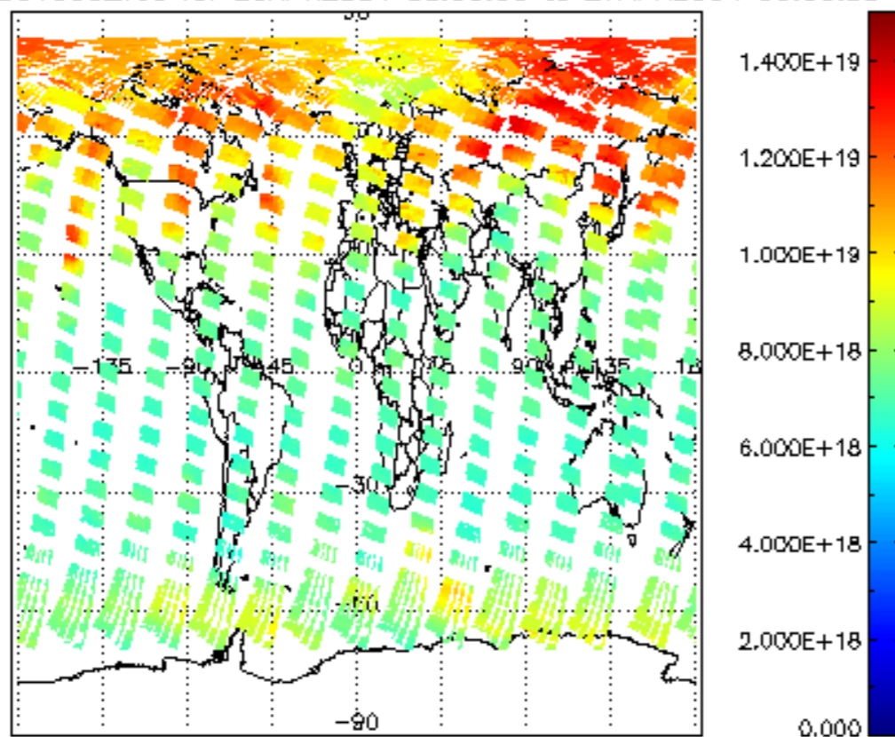
SCIOL2P_NADUV003_vcd for 26APR2004 00:00:00 to 27APR2004 00:00:00
