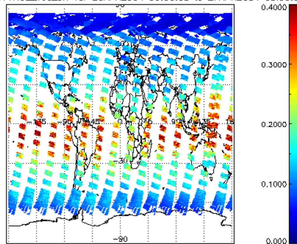
iCIOL2P_NADUV1NO2_vcd_err for 26APR2004 00:00:00 to 27APR2004 00:00:00
