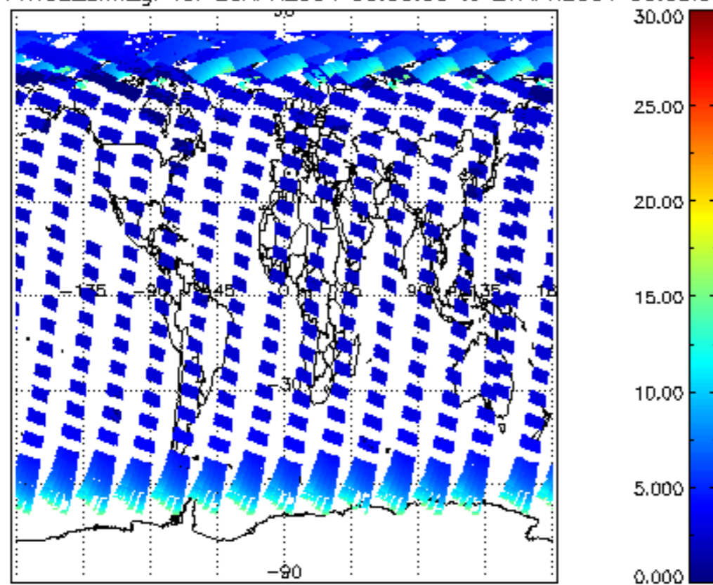
iCIOL2P_NADUV1NO2_amf_gr for 26APR2004 00:00:00 to 27APR2004 00:00:00
