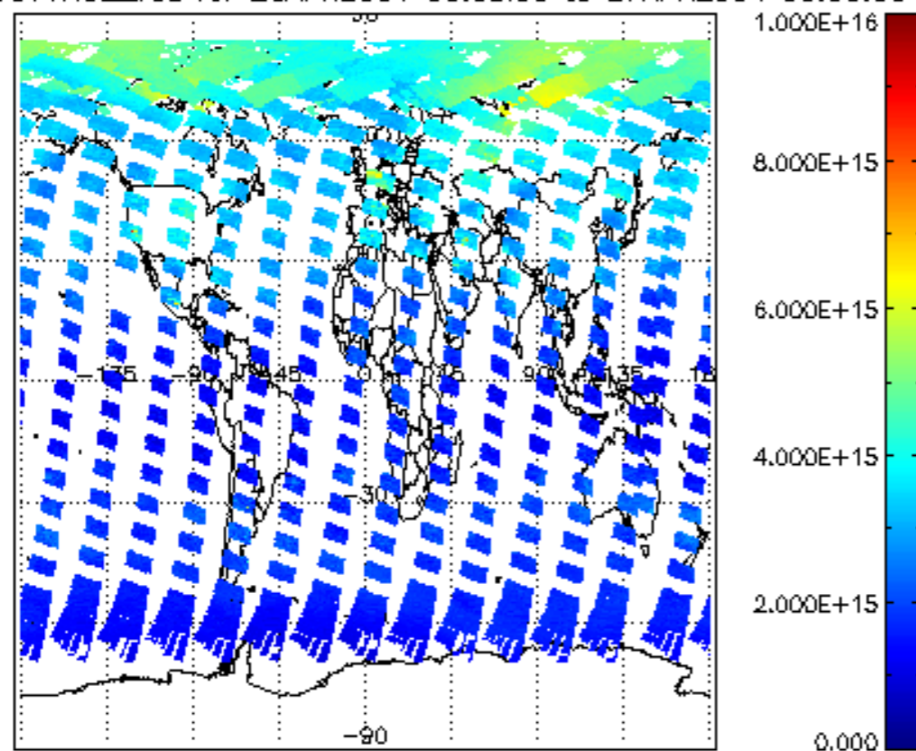
SCIOL2P_NADUV1NO2_vcd for 26APR2004 00:00:00 to 27APR2004 00:00:00
