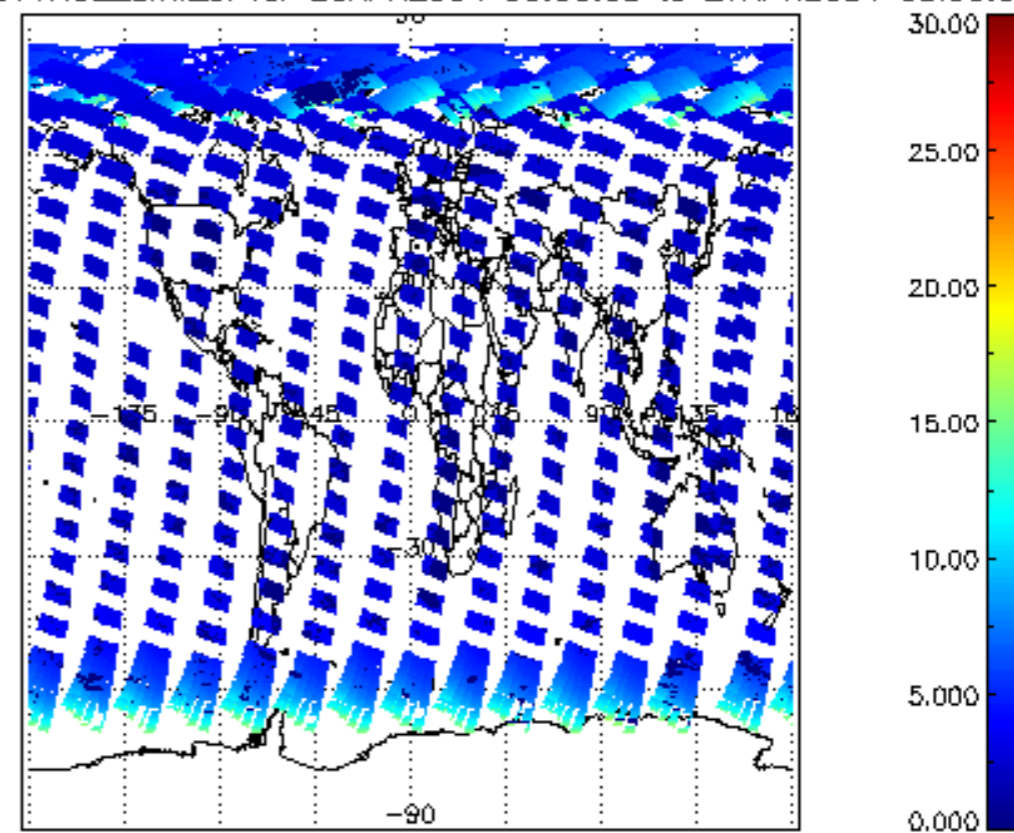
iCIOL2P_NADUV1NO2_amf_cl for 26APR2004 00:00:00 to 27APR2004 00:00:00
