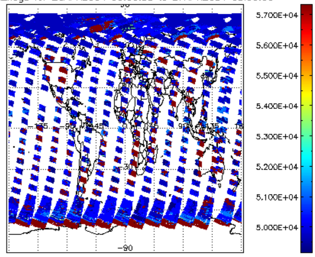
cloud_flags for 26APR2004 00:00:00 to 27APR2004 00:00:00
