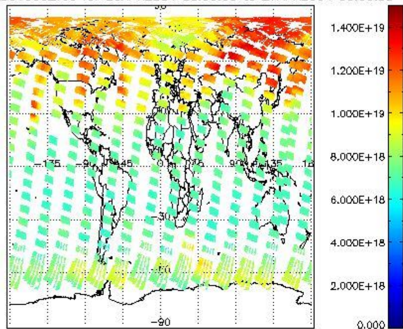
SCIOL2P_NADUV003_vcd for 26APR2004 00:00:00 to 27APR2004 00:00:00
