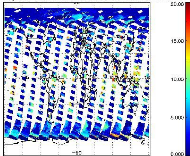
cL_top_height for 26APR2004 00:00:00 to 27APR2004 00:00:00
