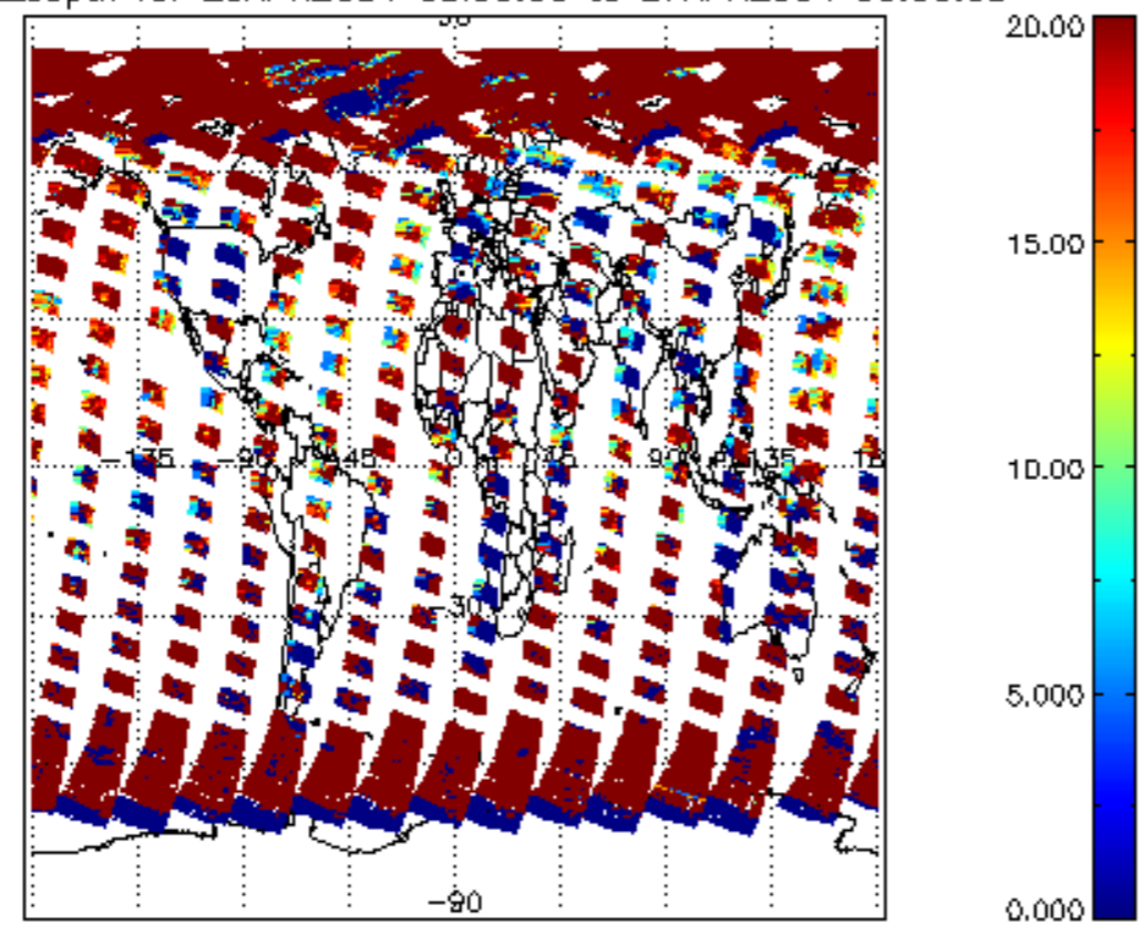
cl_opt_depth for 26APR2004 00:00:00 to 27APR2004 00:00:00
