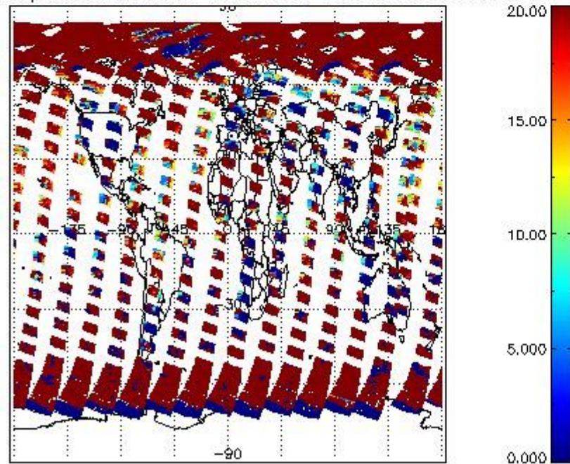
cL_opt_depth for 26APR2004 00:00:00 to 27APR2004 00:00:00
