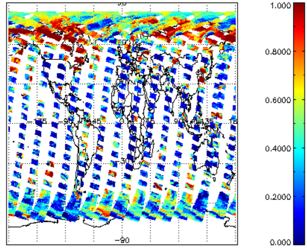
cl_frac for 26APR2004 00:00:00 to 27APR2004 00:00:00
