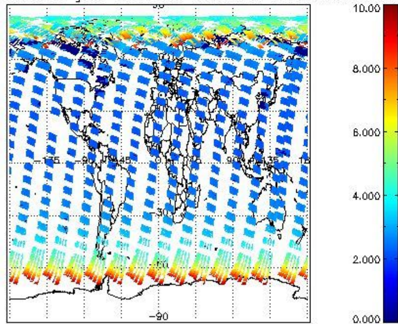
SCIOL2P_NADUV003_amf_gr for 26APR2004 00:00:00 to 27APR2004 00:00:00
