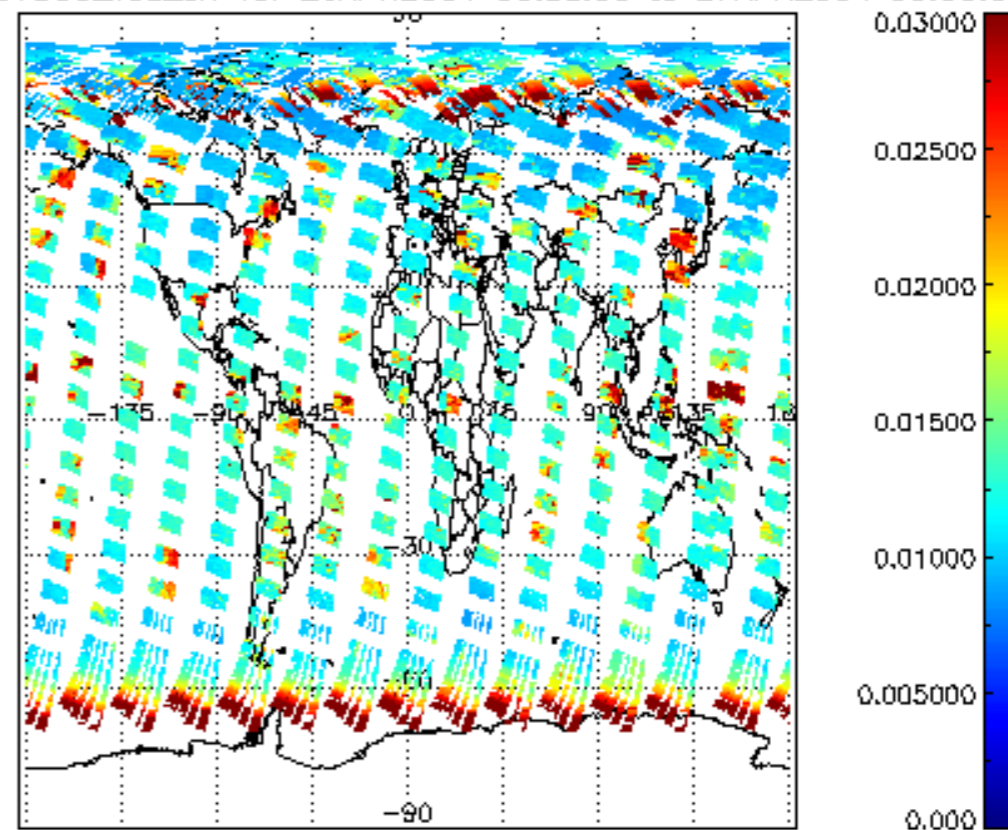
SCIOL2P_NADUV003_vcd_err for 26APR2004 00:00:00 to 27APR2004 00:00:00
