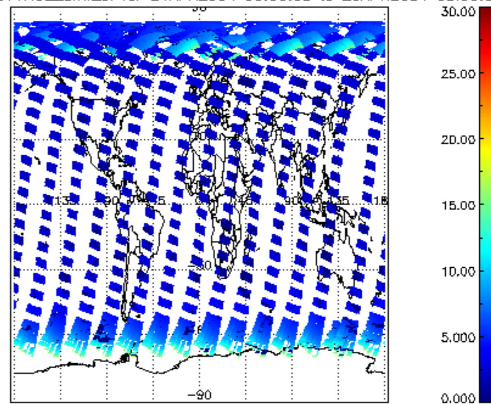
iCIOL2P_NADUV1NO2_amf_cl for 24APR2004 00:00:00 to 25APR2004 00:00:00
