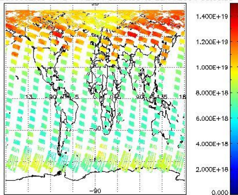
SCIOL2P_NADUV003_vcd for 24APR2004 00:00:00 to 25APR2004 00:00:00
