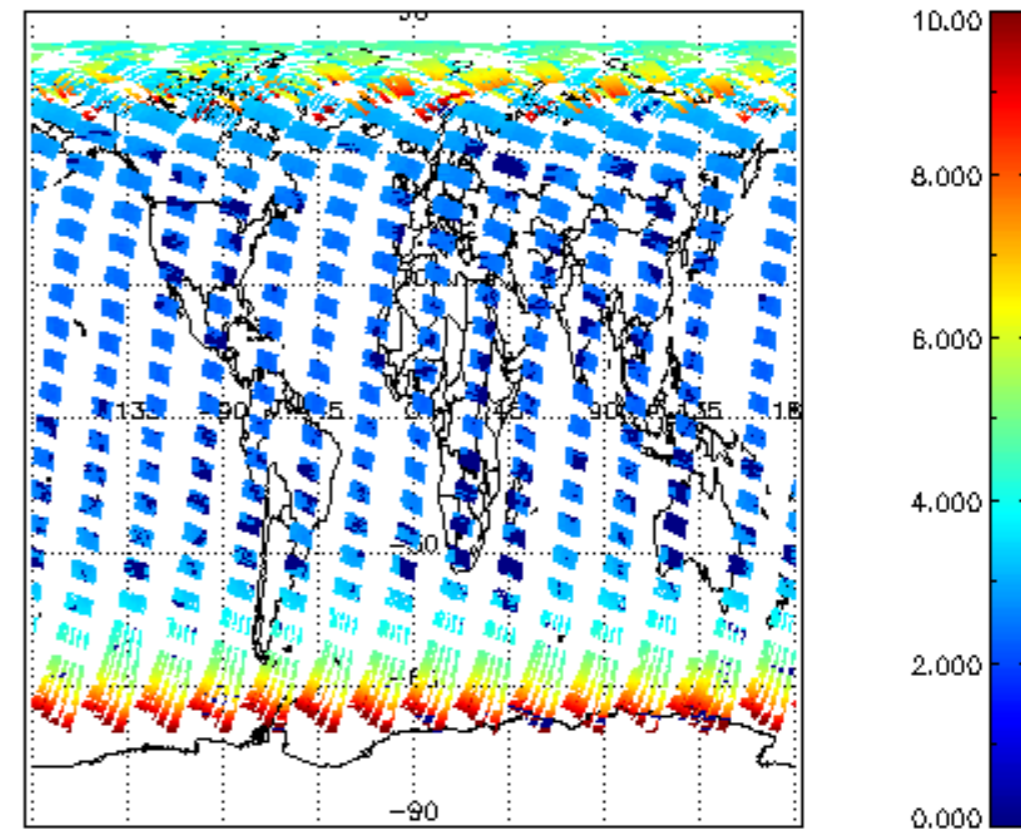
SCIOL2P_NADUV003_amf_cl for 24APR2004 00:00:00 to 25APR2004 00:00:00
