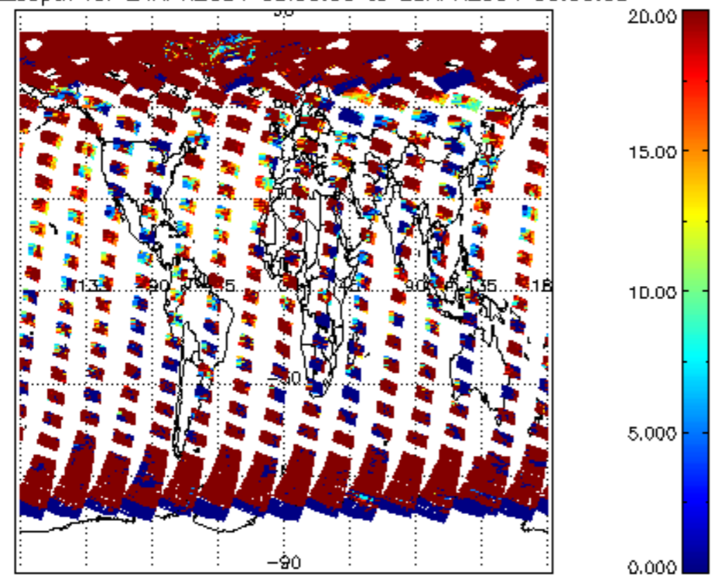
cl_opt_depth for 24APR2004 00:00:00 to 25APR2004 00:00:00
