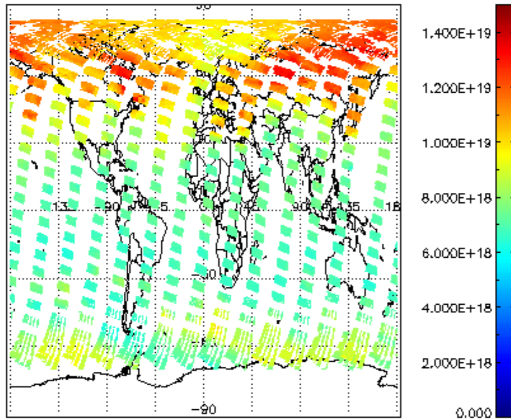
SCIOL2P_NADUV003_vcd for 24APR2004 00:00:00 to 25APR2004 00:00:00
