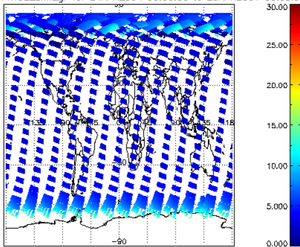
iCIOL2P_NADUV1NO2_amf_gr for 24APR2004 00:00:00 to 25APR2004 00:00:00
