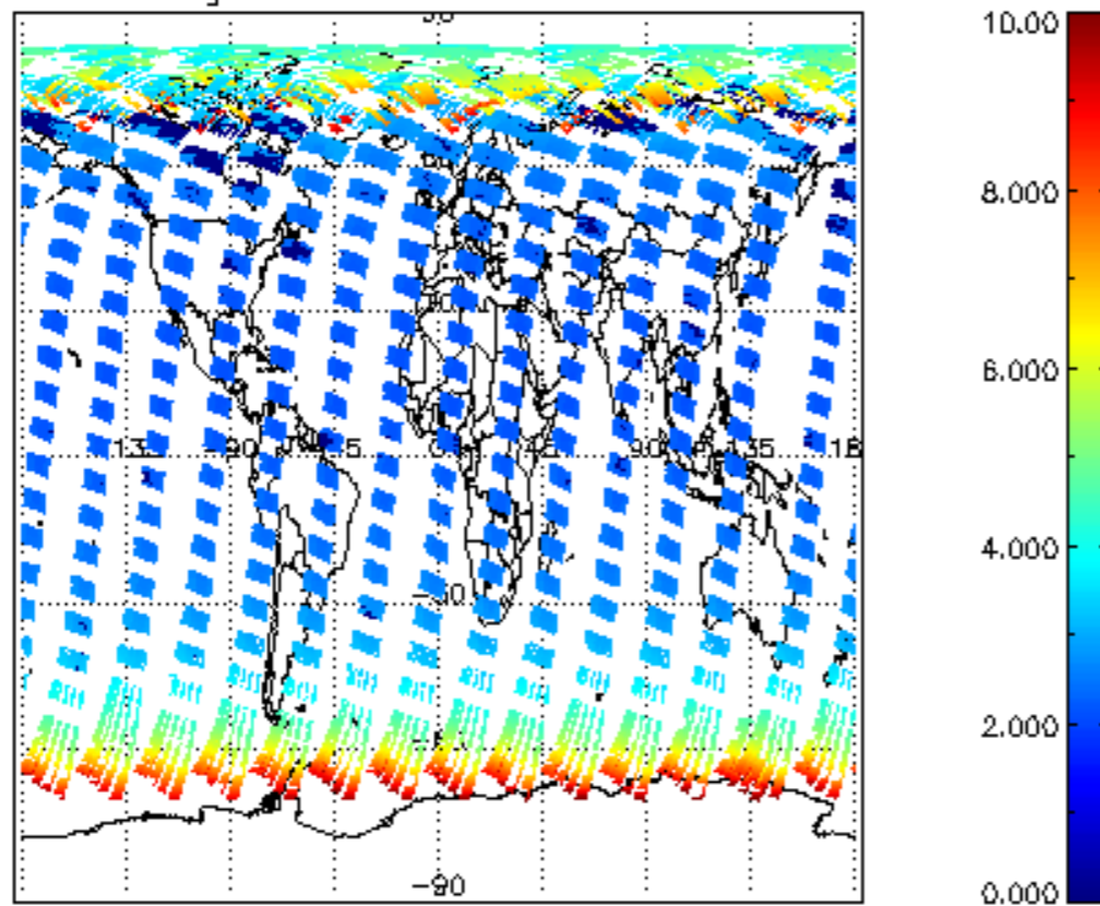
SCIOL2P_NADUV003_amf_gr for 24APR2004 00:00:00 to 25APR2004 00:00:00
