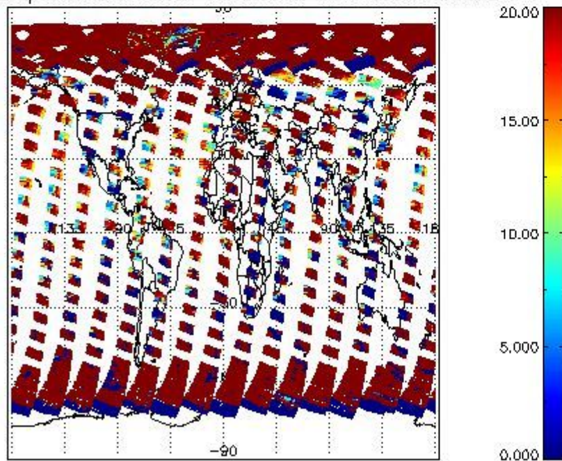
cL_opt_depth for 24APR2004 00:00:00 to 25APR2004 00:00:00
