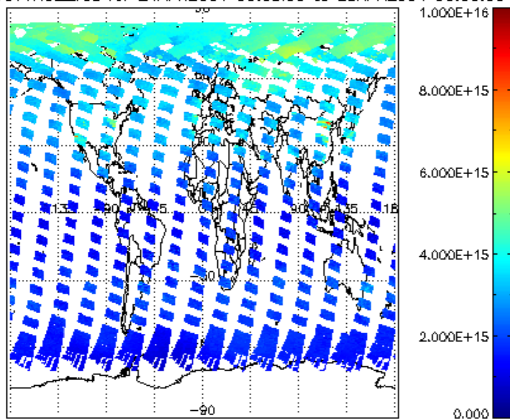
SCIOL2P_NADUV1NO2_vcd for 24APR2004 00:00:00 to 25APR2004 00:00:00
