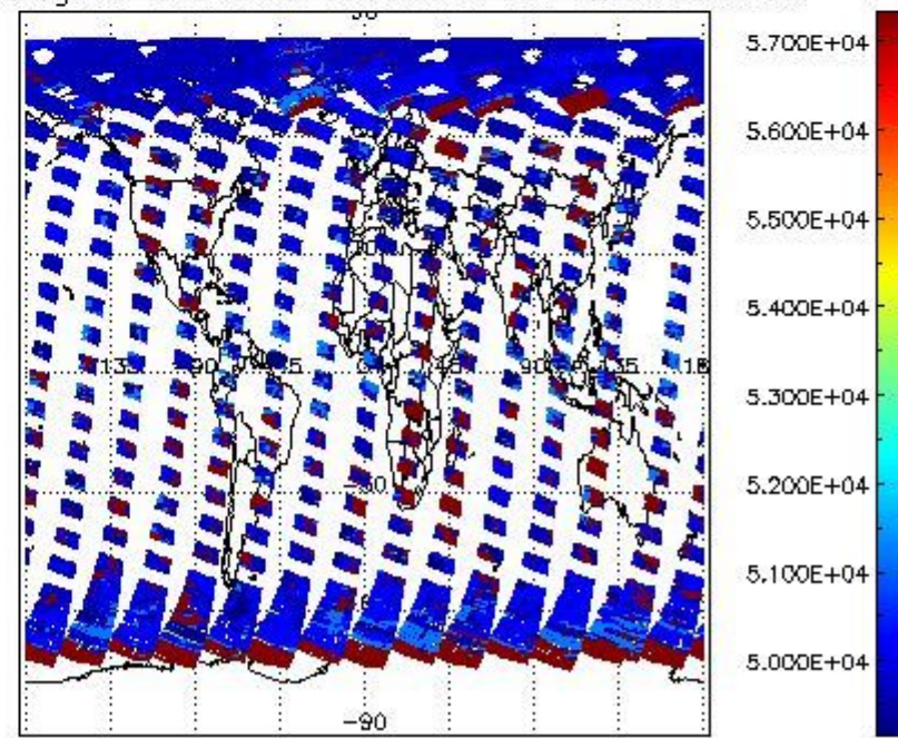
cloud_flags for 24APR2004 00:00:00 to 25APR2004 00:00:00
