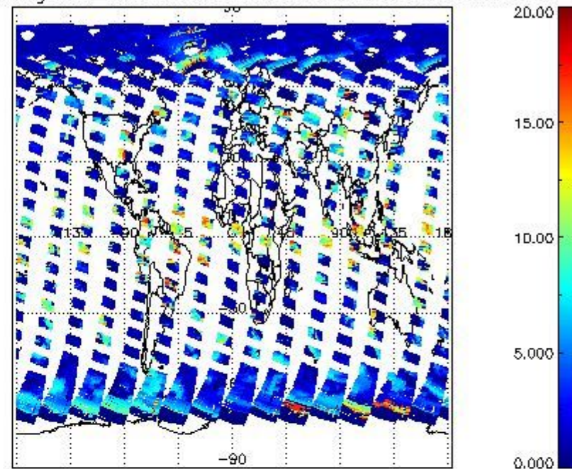
cL_top_height for 24APR2004 00:00:00 to 25APR2004 00:00:00
