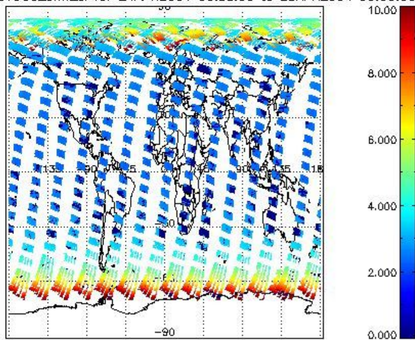
SCIOL2P_NADUV003_amf_cl for 24APR2004 00:00:00 to 25APR2004 00:00:00
