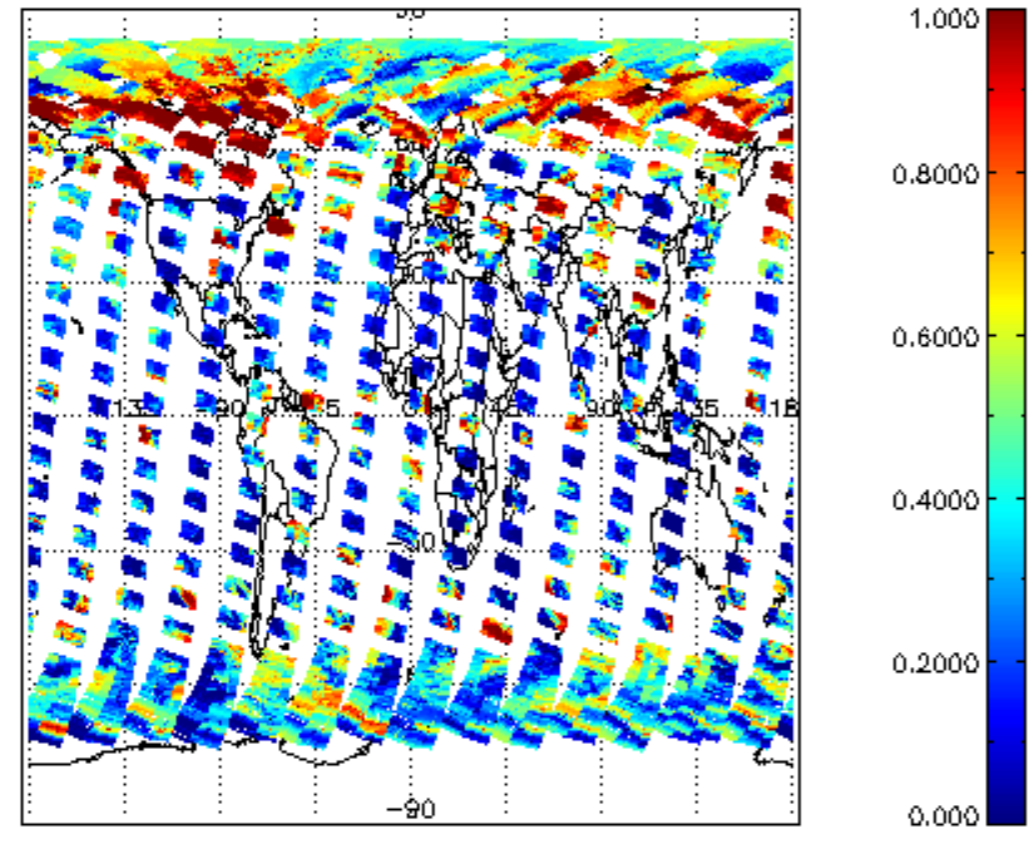
cl_frac for 24APR2004 00:00:00 to 25APR2004 00:00:00
