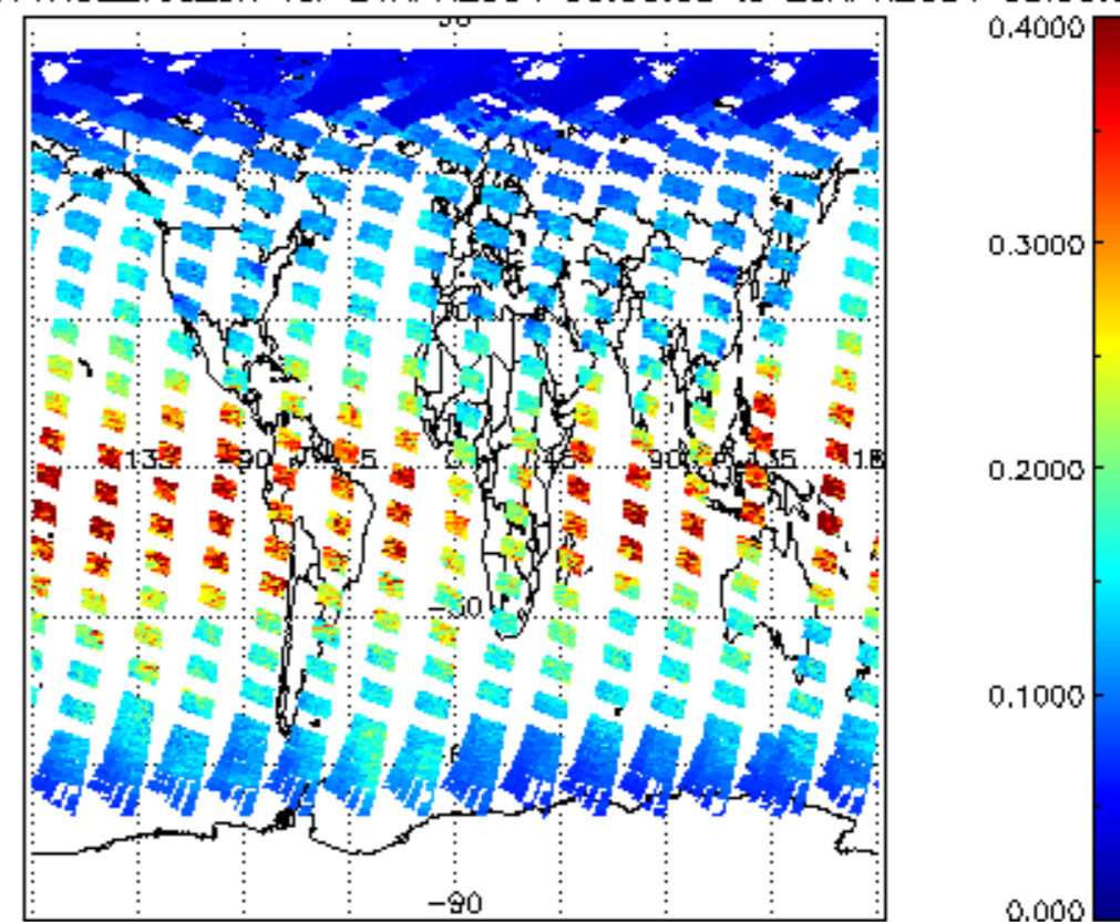
iCIOL2P_NADUV1NO2_vcd_err for 24APR2004 00:00:00 to 25APR2004 00:00:00
