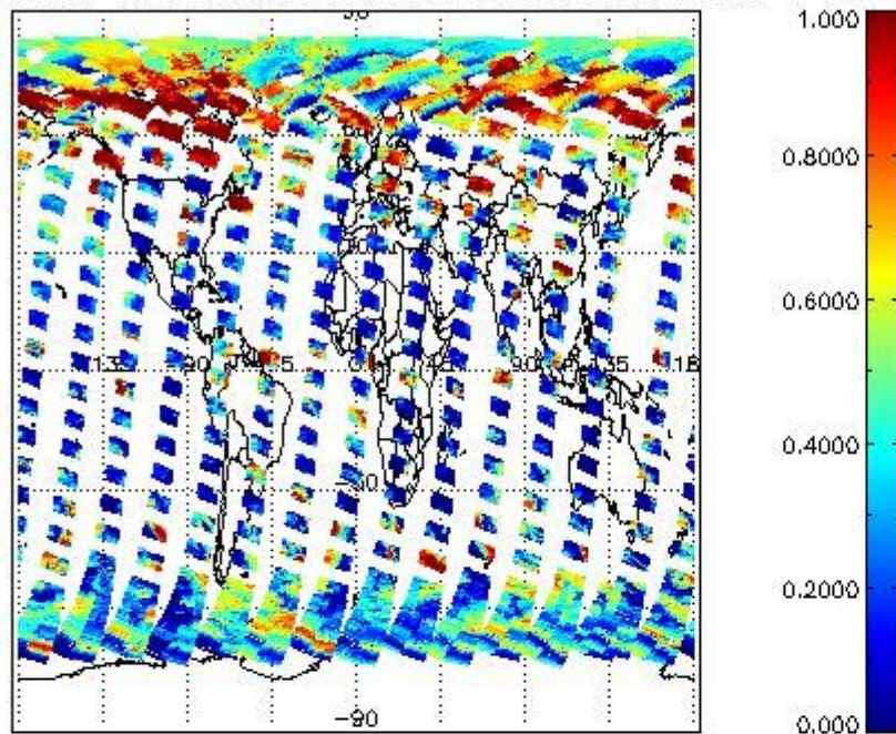
cL_frac for 24APR2004 00:00:00 to 25APR2004 00:00:00
