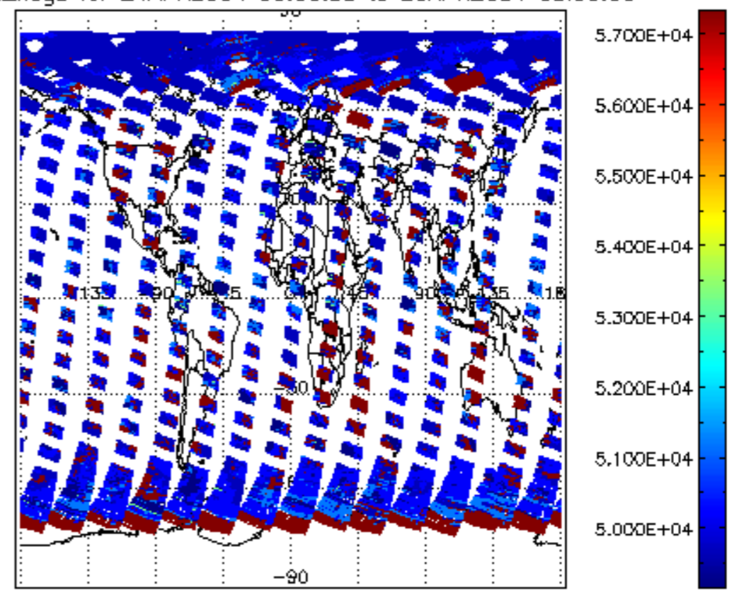
cloud_flags for 24APR2004 00:00:00 to 25APR2004 00:00:00
