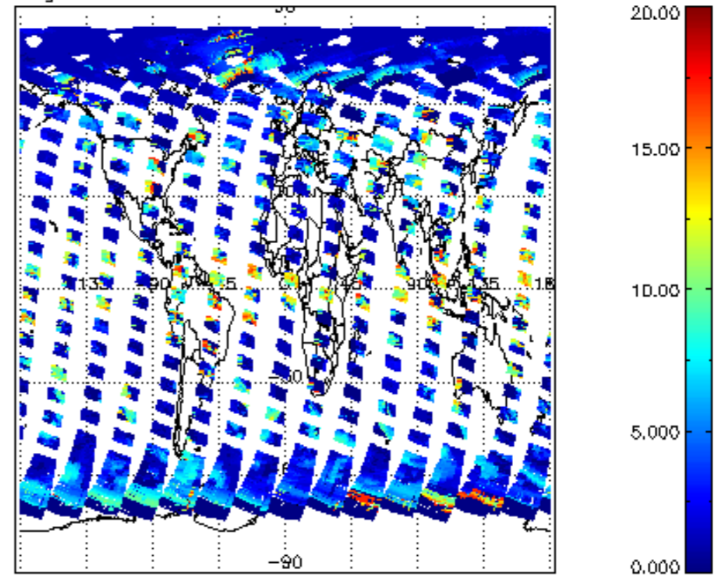
cl_top_height for 24APR2004 00:00:00 to 25APR2004 00:00:00
