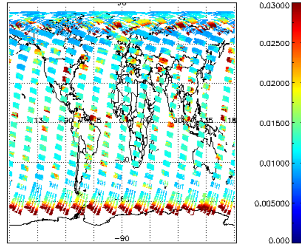
SCIOL2P_NADUV003_vcd_err for 24APR2004 00:00:00 to 25APR2004 00:00:00
