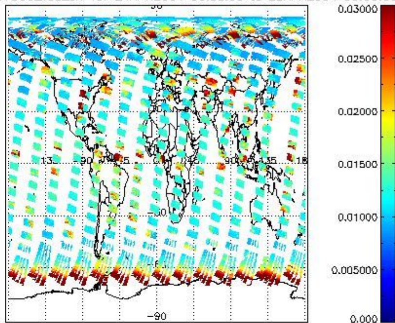
SCIOL2P_NADUV003_vcd_err for 24APR2004 00:00:00 to 25APR2004 00:00:00
