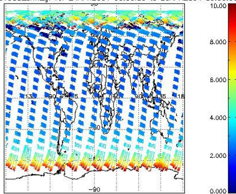
SCIOL2P_NADUV003_amf_gr for 24APR2004 00:00:00 to 25APR2004 00:00:00
