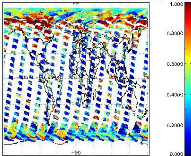
cL_frac for 22APR2004 00:00:00 to 23APR2004 00:00:00
