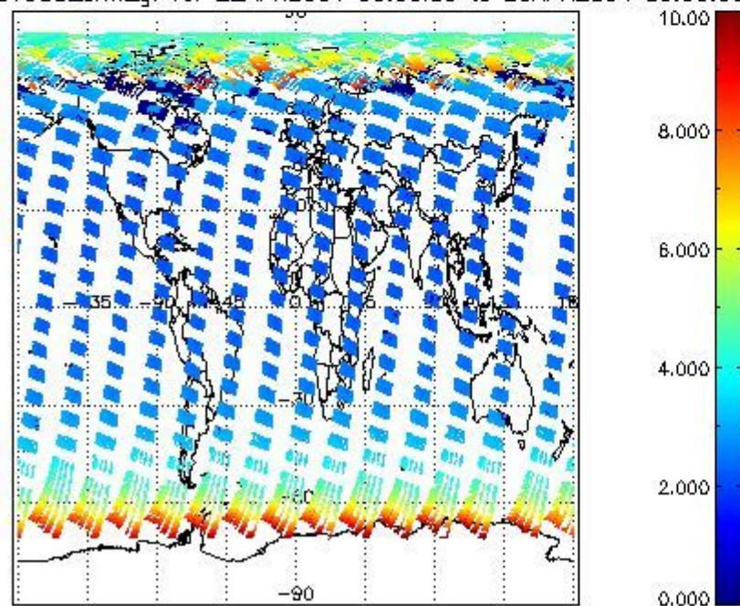
SCIOL2P_NADUV003_amf_gr for 22APR2004 00:00:00 to 23APR2004 00:00:00
