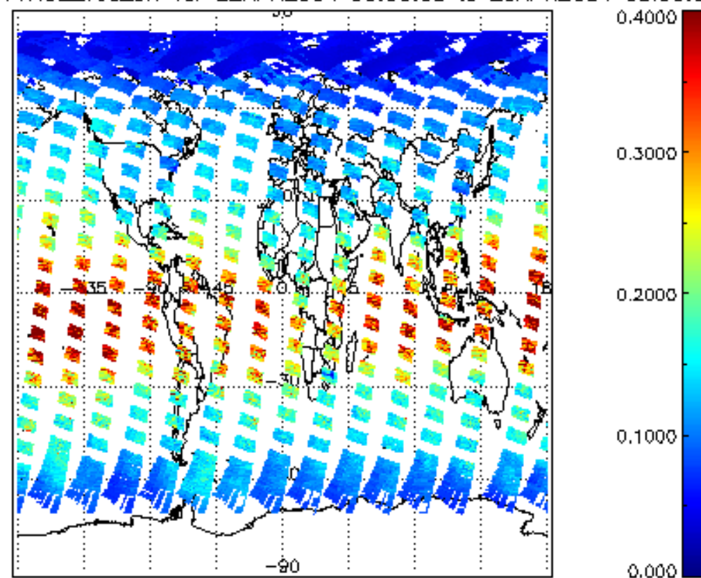
iCIOL2P_NADUV1NO2_vcd_err for 22APR2004 00:00:00 to 23APR2004 00:00:00
