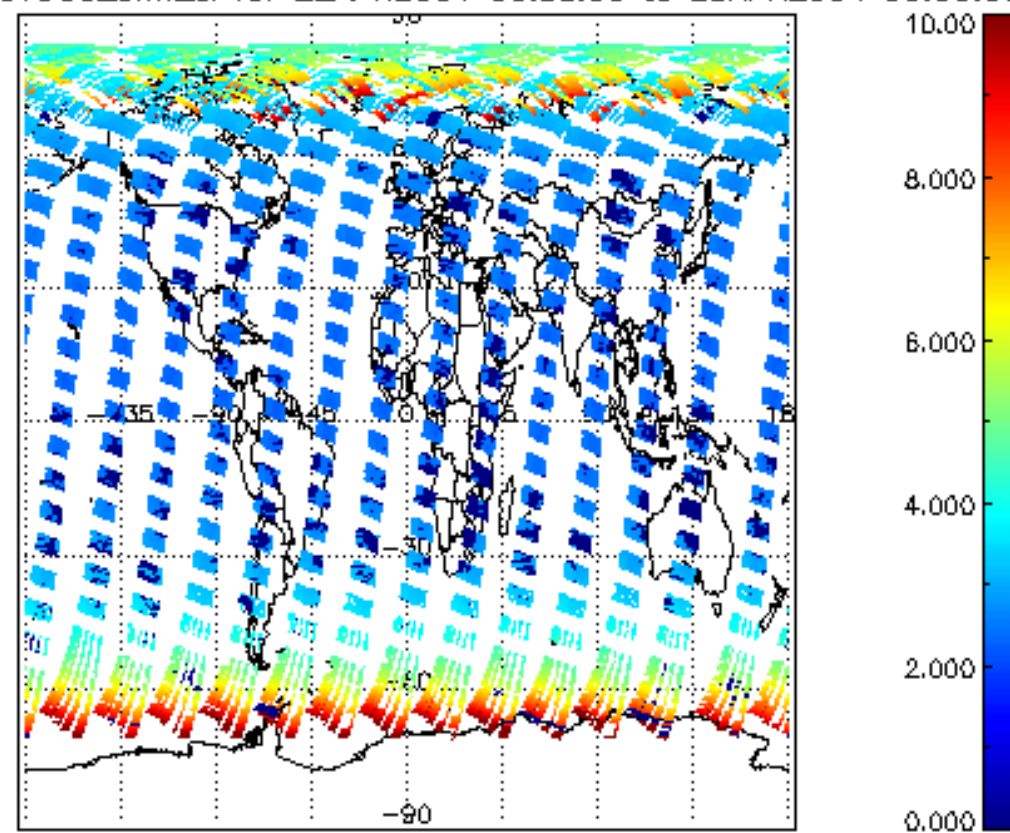
SCIOL2P_NADUV003_amf_cl for 22APR2004 00:00:00 to 23APR2004 00:00:00
