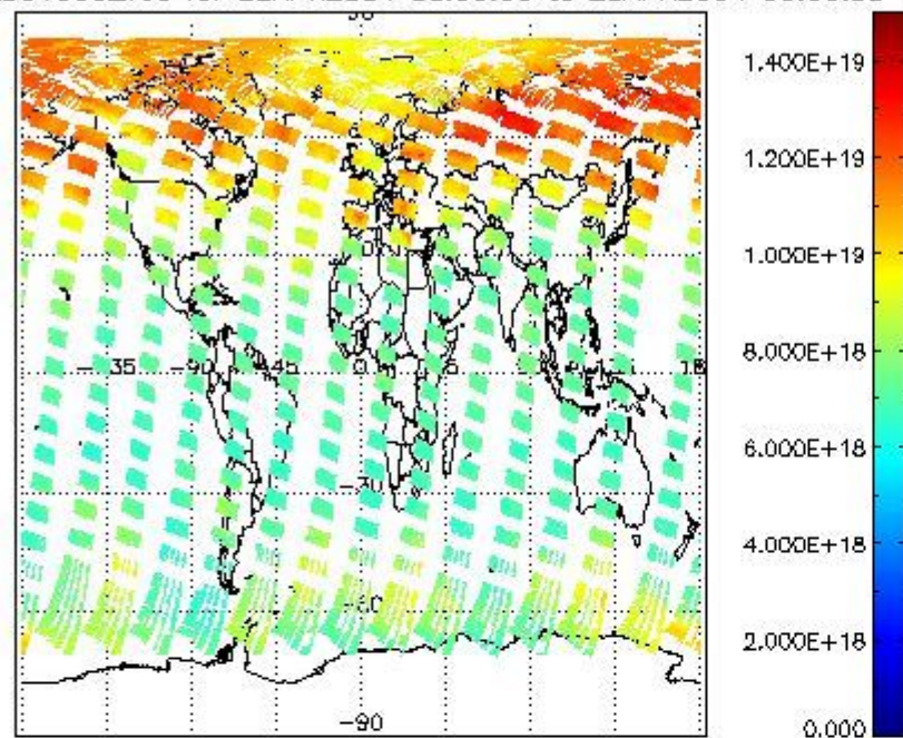
SCIOL2P_NADUV003_vcd for 22APR2004 00:00:00 to 23APR2004 00:00:00
