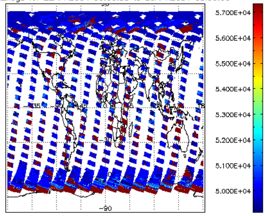
cloud_flags for 22APR2004 00:00:00 to 23APR2004 00:00:00
