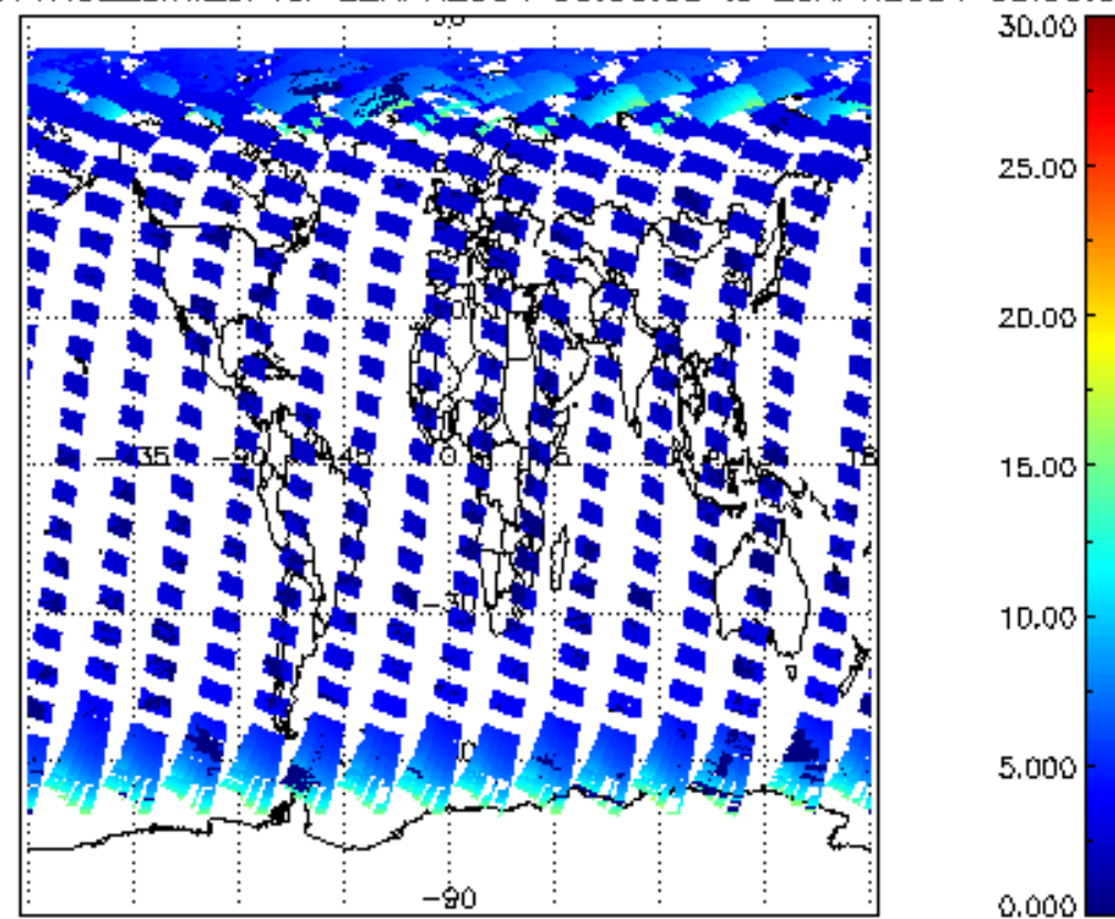
iCIOL2P_NADUV1NO2_amf_cl for 22APR2004 00:00:00 to 23APR2004 00:00:00
