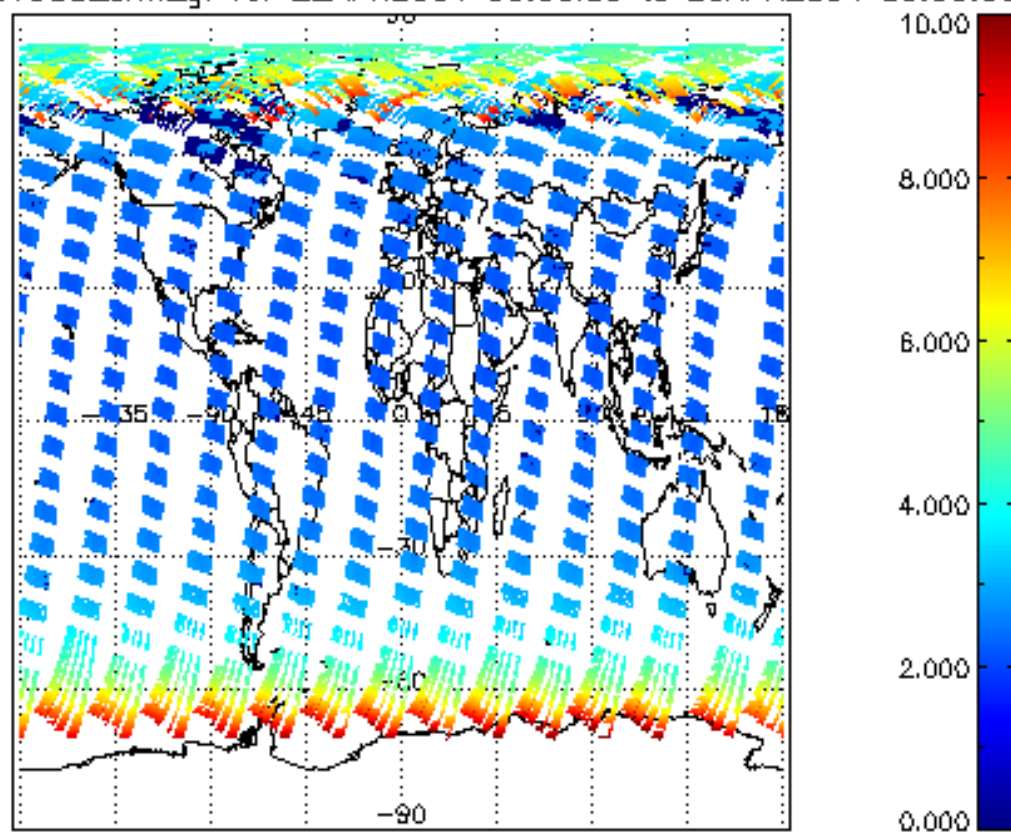
SCIOL2P_NADUV003_amf_gr for 22APR2004 00:00:00 to 23APR2004 00:00:00
