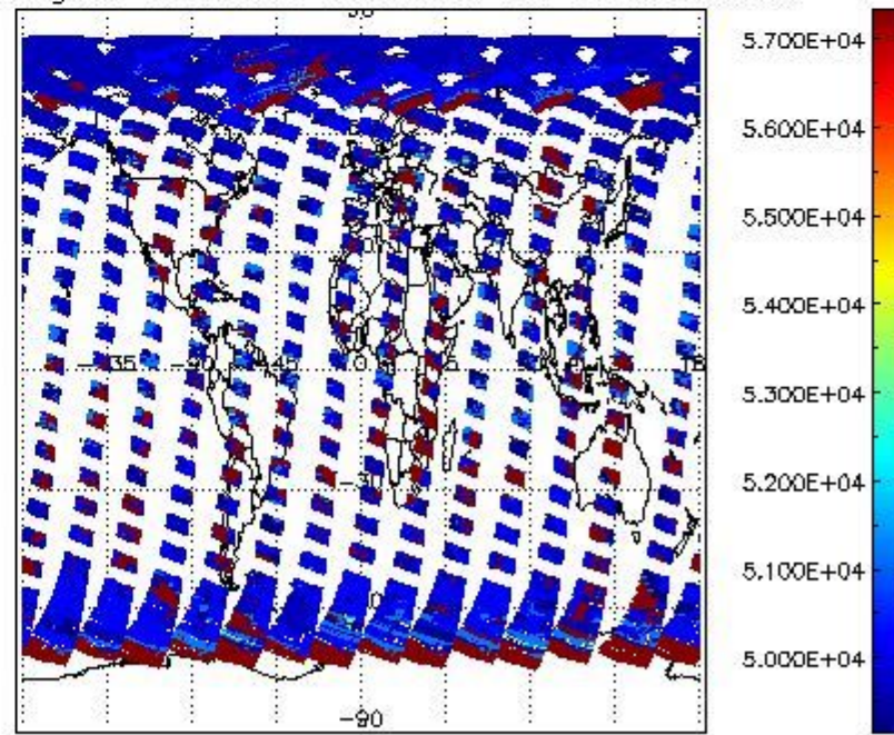
cloud_flags for 22APR2004 00:00:00 to 23APR2004 00:00:00
