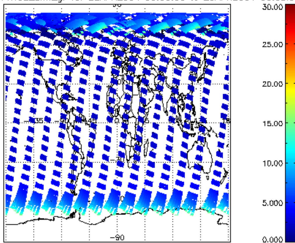
iCIOL2P_NADUV1NO2_amf_gr for 22APR2004 00:00:00 to 23APR2004 00:00:00
