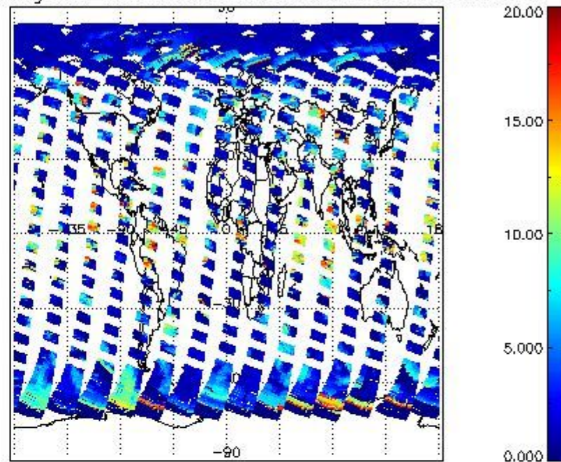
cL_top_height for 22APR2004 00:00:00 to 23APR2004 00:00:00
