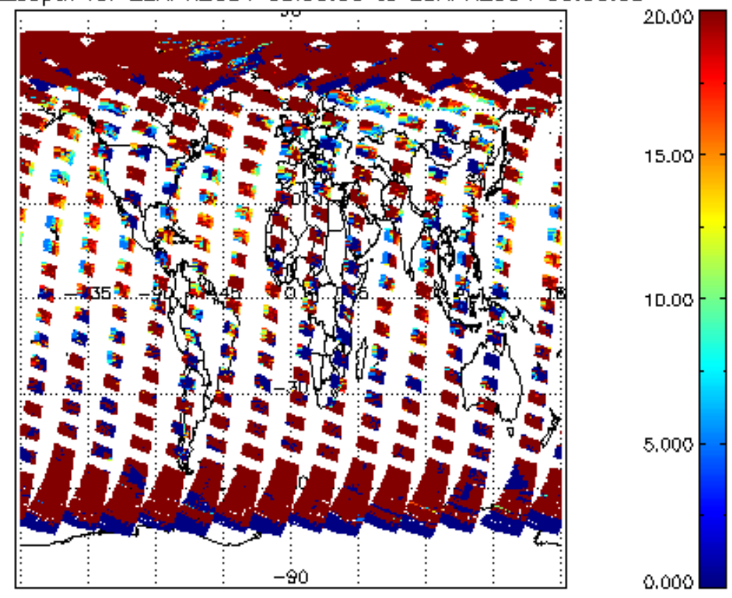
cl_opt_depth for 22APR2004 00:00:00 to 23APR2004 00:00:00
