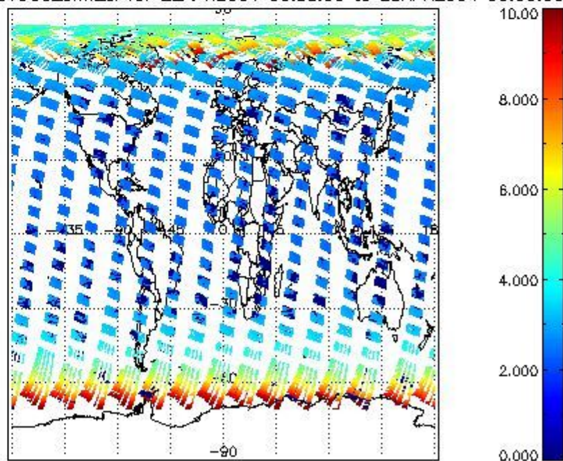
SCIOL2P_NADUV003_amf_cl for 22APR2004 00:00:00 to 23APR2004 00:00:00
