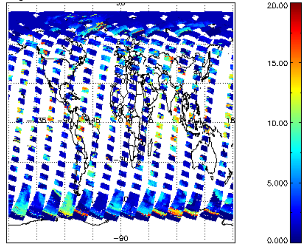
cl_top_height for 22APR2004 00:00:00 to 23APR2004 00:00:00
