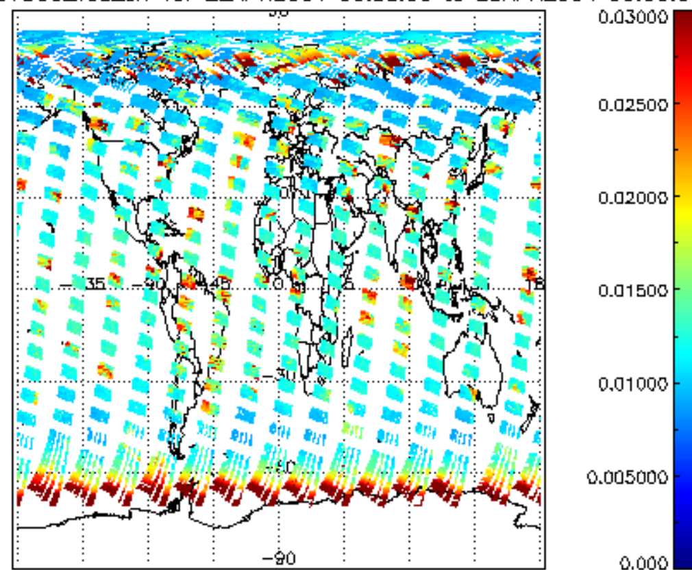
SCIOL2P_NADUV003_vcd_err for 22APR2004 00:00:00 to 23APR2004 00:00:00
