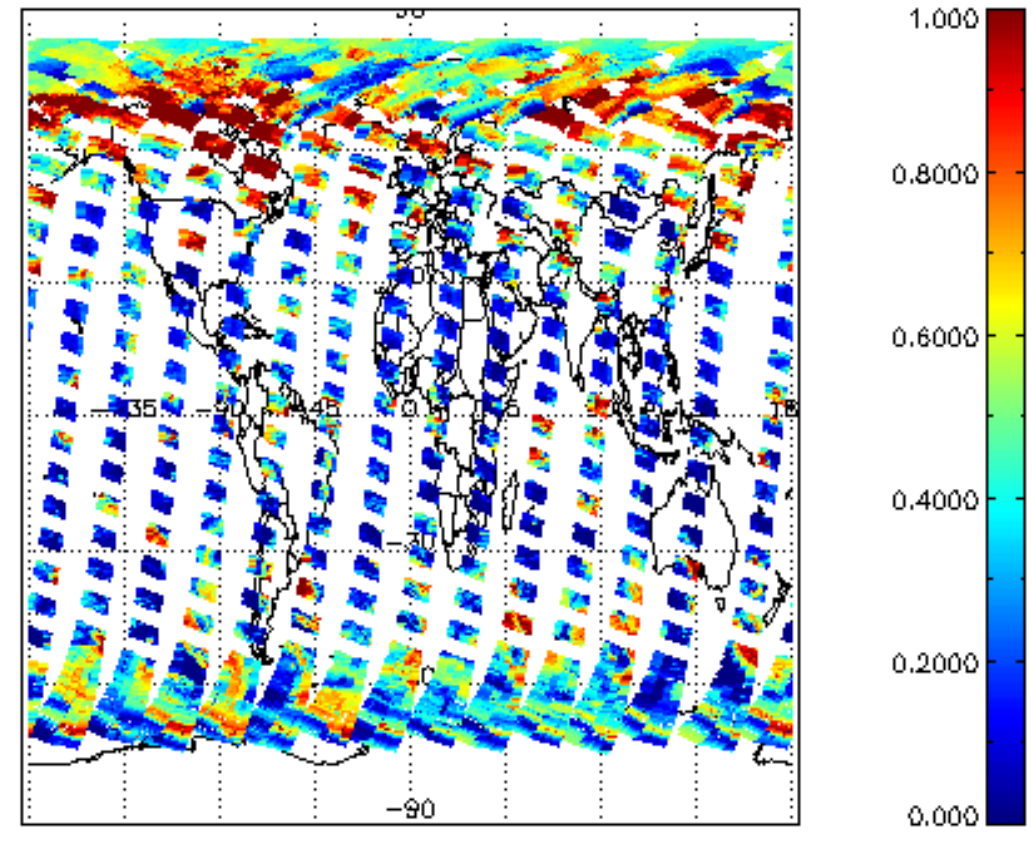
cl_frac for 22APR2004 00:00:00 to 23APR2004 00:00:00
