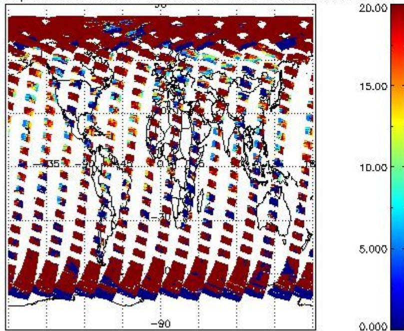
cL_opt_depth for 22APR2004 00:00:00 to 23APR2004 00:00:00
