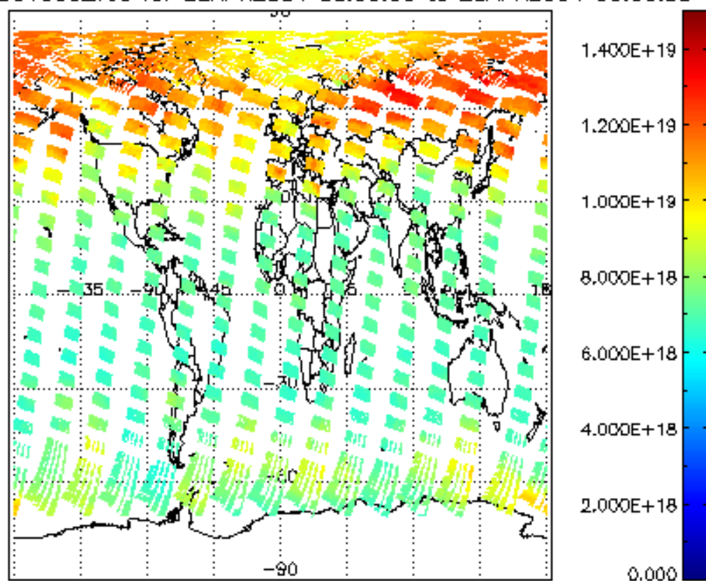
SCIOL2P_NADUV003_vcd for 22APR2004 00:00:00 to 23APR2004 00:00:00
