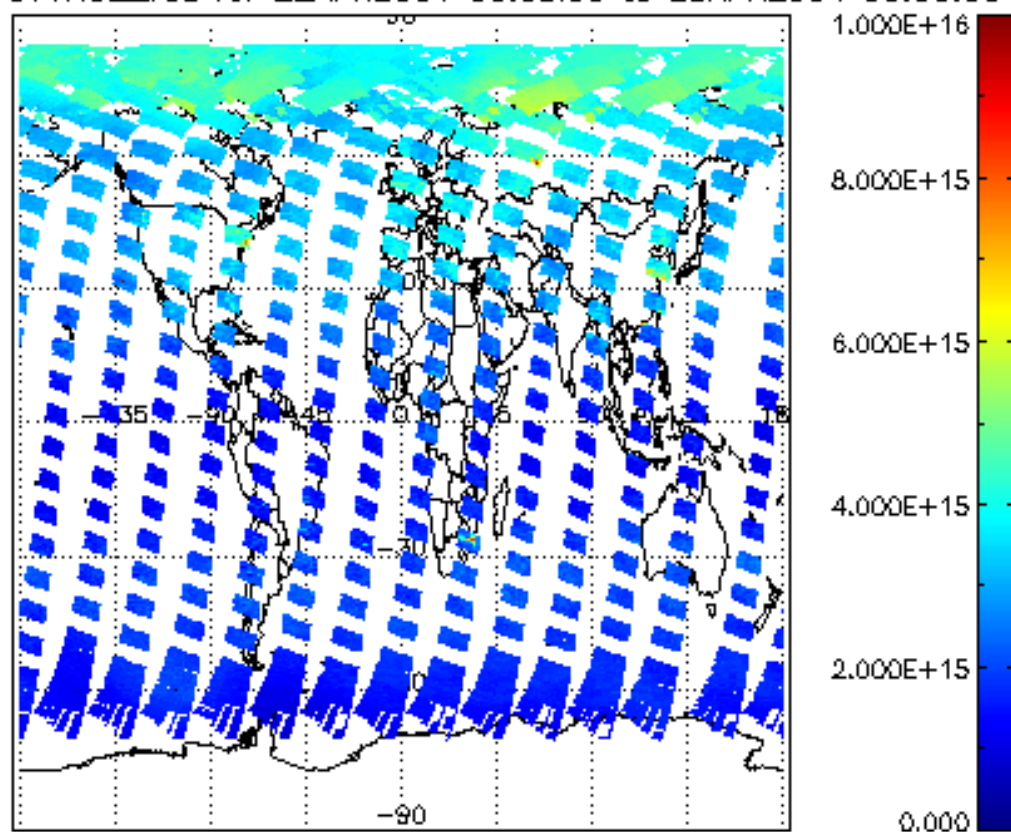
SCIOL2P_NADUV1NO2_vcd for 22APR2004 00:00:00 to 23APR2004 00:00:00
