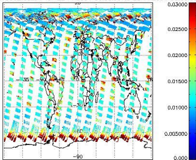
SCIOL2P_NADUV003_vcd_err for 22APR2004 00:00:00 to 23APR2004 00:00:00
