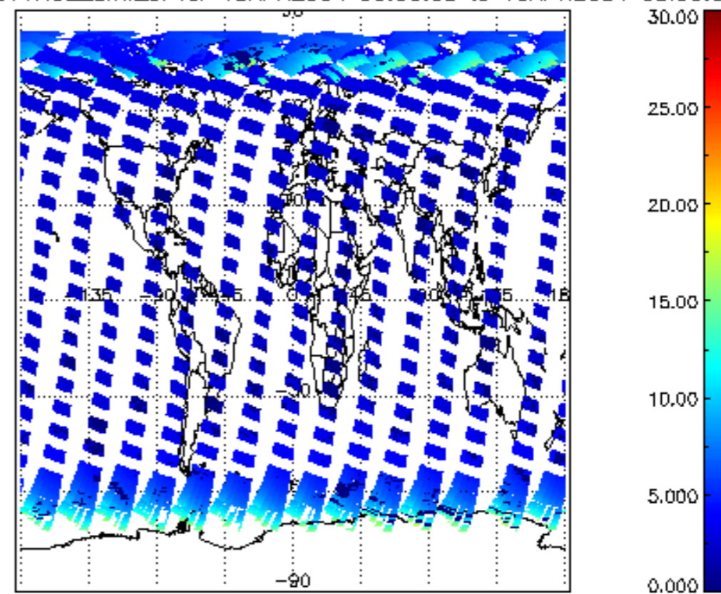
iCIOL2P_NADUV1NO2_amf_cl for 18APR2004 00:00:00 to 19APR2004 00:00:00
