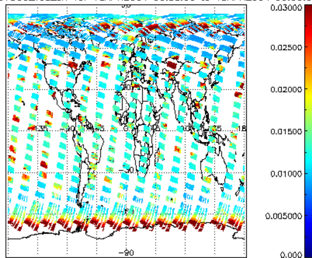
SCIOL2P_NADUV003_vcd_err for 18APR2004 00:00:00 to 19APR2004 00:00:00
