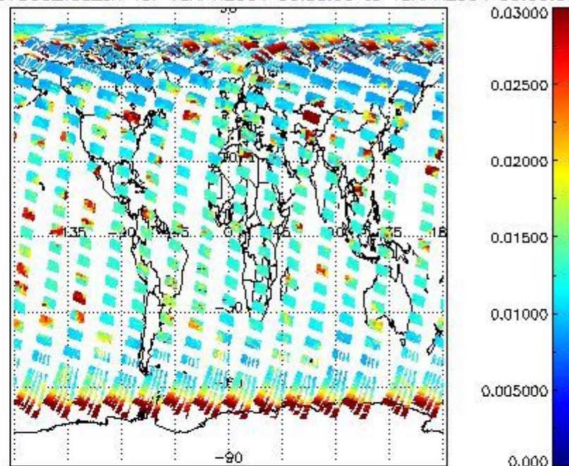
SCIOL2P_NADUV003_vcd_err for 18APR2004 00:00:00 to 19APR2004 00:00:00
