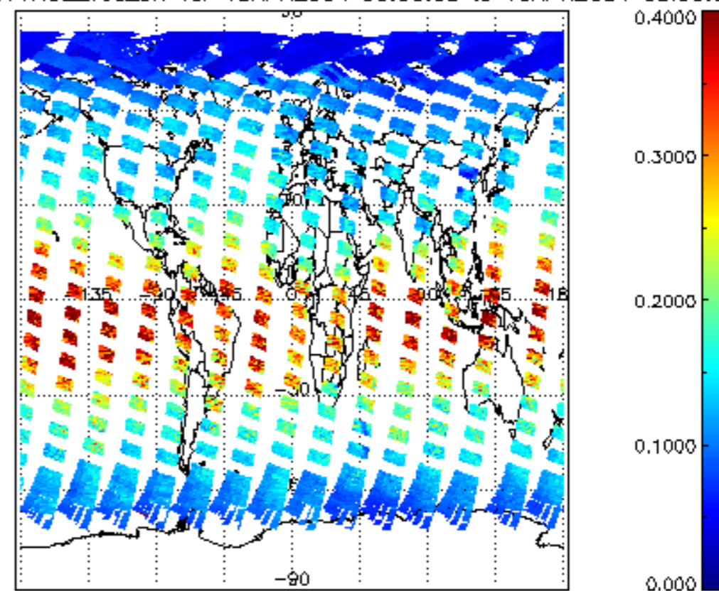
iCIOL2P_NADUV1NO2_vcd_err for 18APR2004 00:00:00 to 19APR2004 00:00:00
