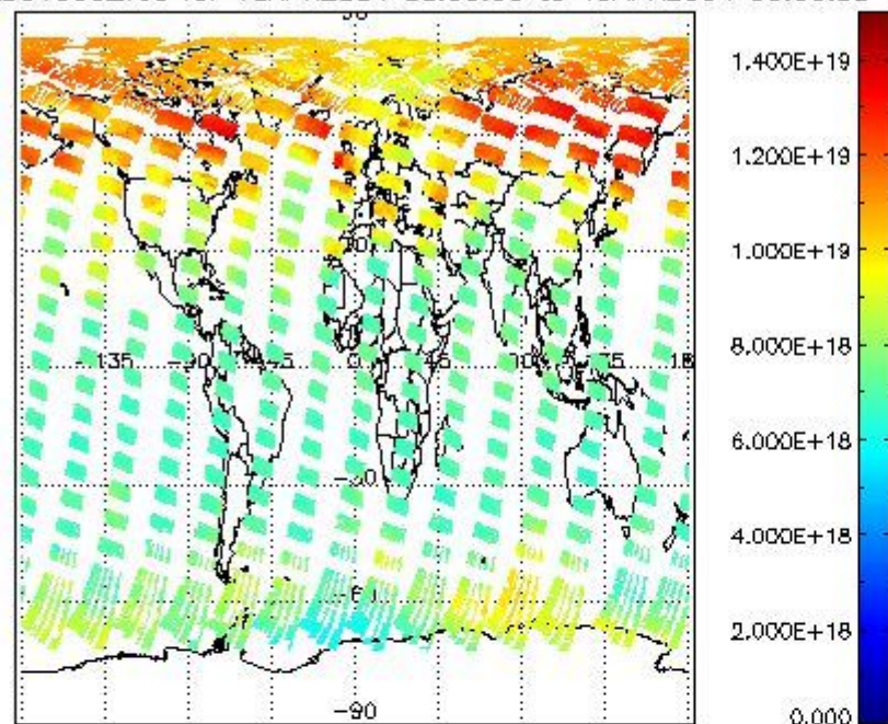
SCIOL2P_NADUV003_vcd for 18APR2004 00:00:00 to 19APR2004 00:00:00
