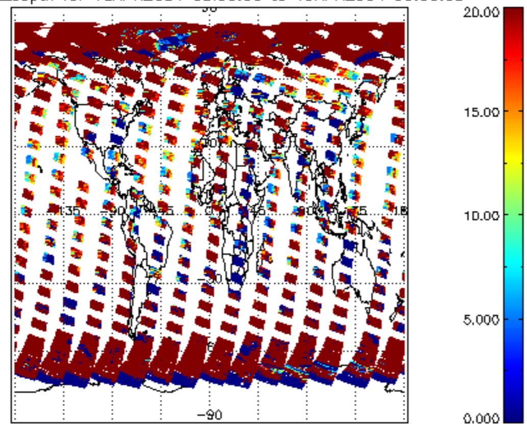
cl_opt_depth for 18APR2004 00:00:00 to 19APR2004 00:00:00
