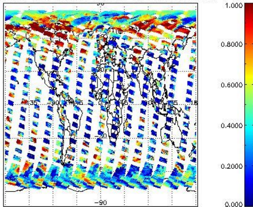
cL_frac for 18APR2004 00:00:00 to 19APR2004 00:00:00
