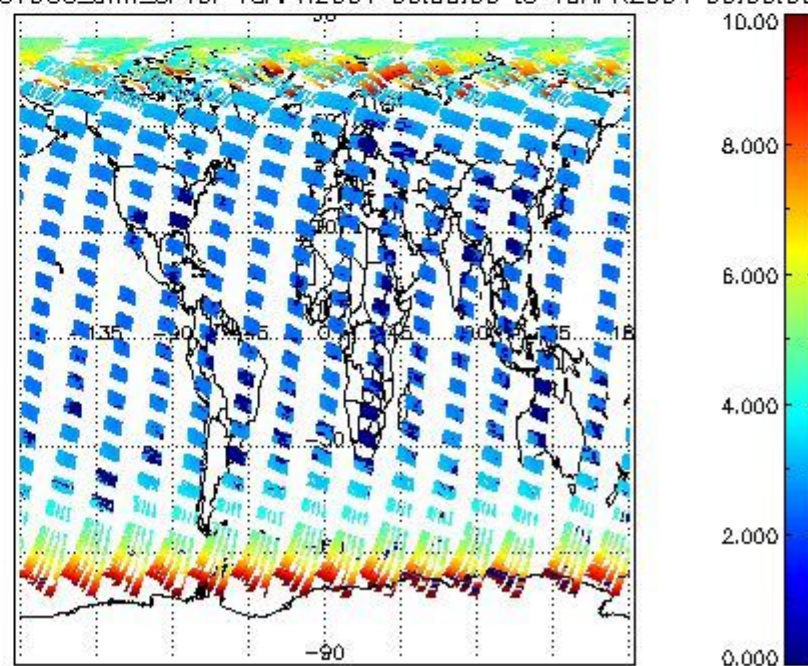
SCIOL2P_NADUV003_amf_cl for 18APR2004 00:00:00 to 19APR2004 00:00:00
