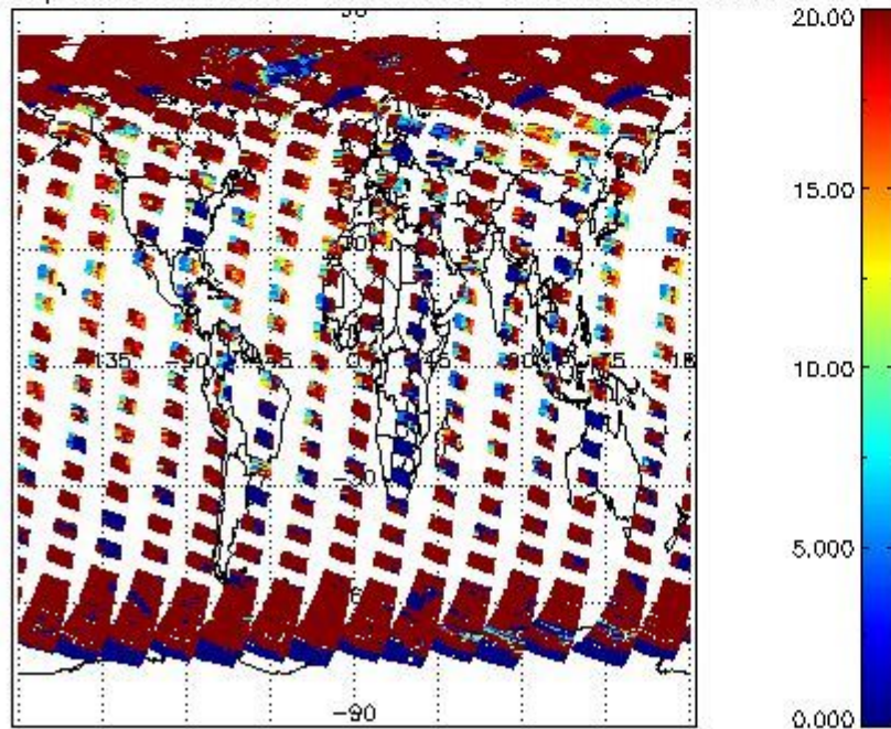
cL_opt_depth for 18APR2004 00:00:00 to 19APR2004 00:00:00
