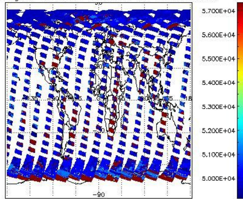
cloud_flags for 18APR2004 00:00:00 to 19APR2004 00:00:00
