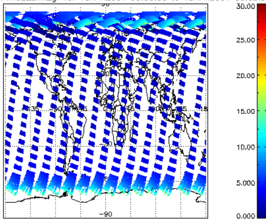
iCIOL2P_NADUV1NO2_amf_gr for 18APR2004 00:00:00 to 19APR2004 00:00:00
