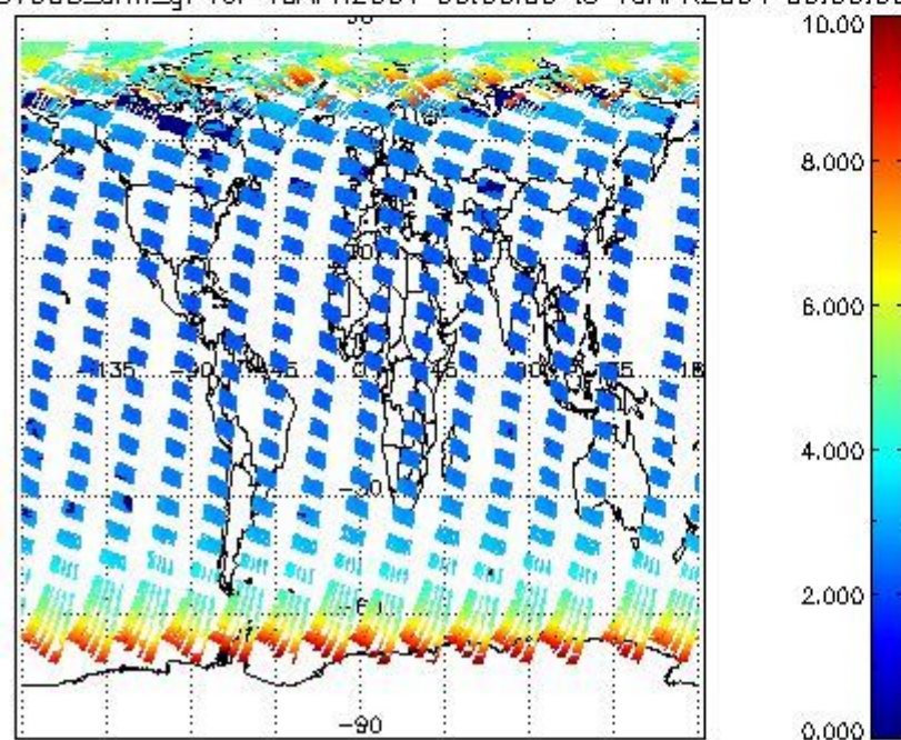
SCIOL2P_NADUV003_amf_gr for 18APR2004 00:00:00 to 19APR2004 00:00:00
