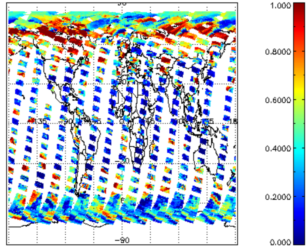
cl_frac for 18APR2004 00:00:00 to 19APR2004 00:00:00
