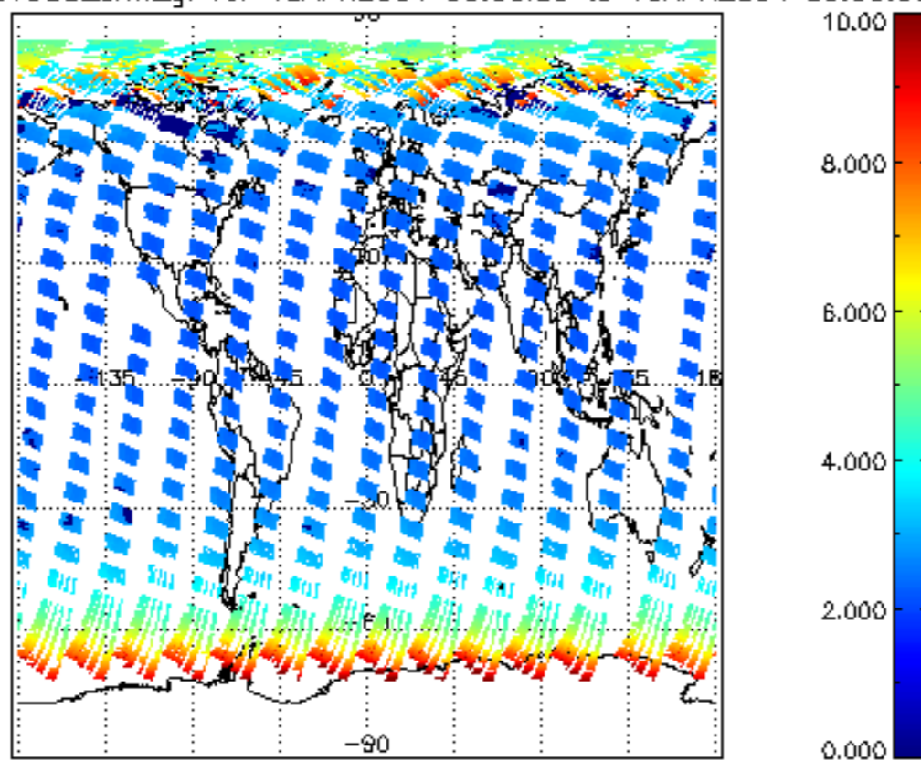
SCIOL2P_NADUV003_amf_gr for 18APR2004 00:00:00 to 19APR2004 00:00:00
