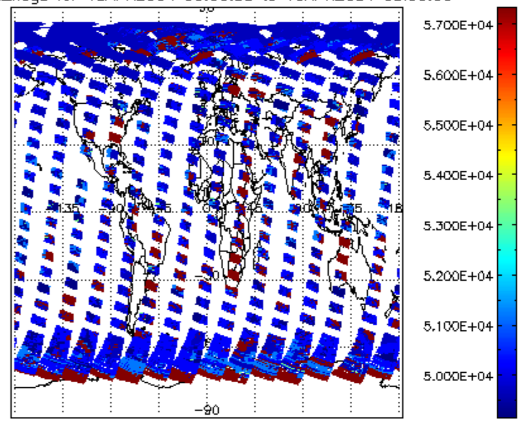
cloud_flags for 18APR2004 00:00:00 to 19APR2004 00:00:00
