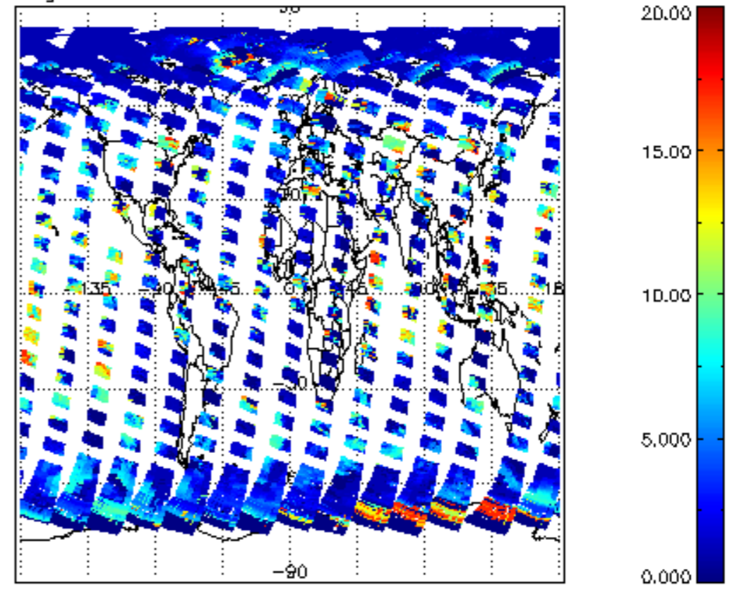
cl_top_height for 18APR2004 00:00:00 to 19APR2004 00:00:00
