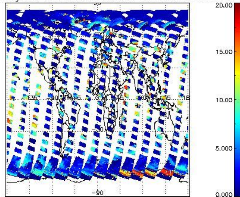
cL_top_height for 18APR2004 00:00:00 to 19APR2004 00:00:00
