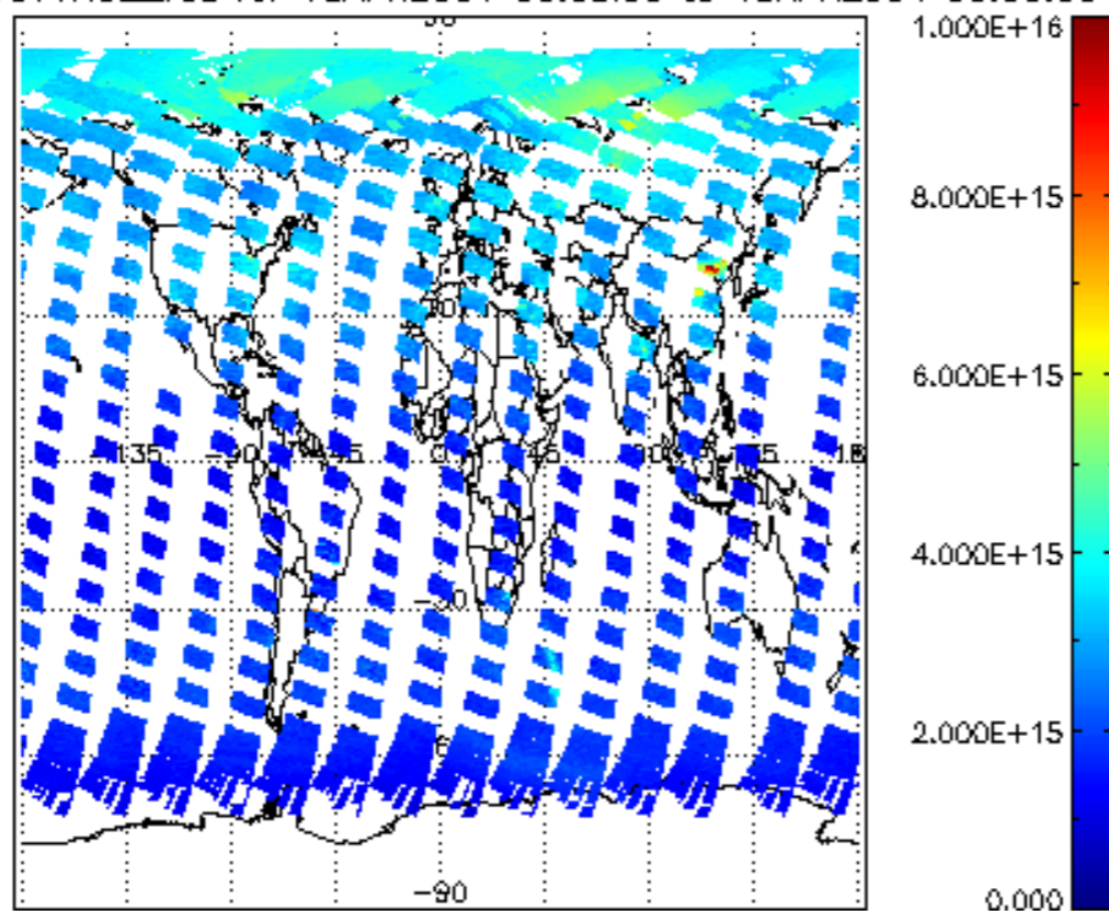
SCIOL2P_NADUV1NO2_vcd for 18APR2004 00:00:00 to 19APR2004 00:00:00
