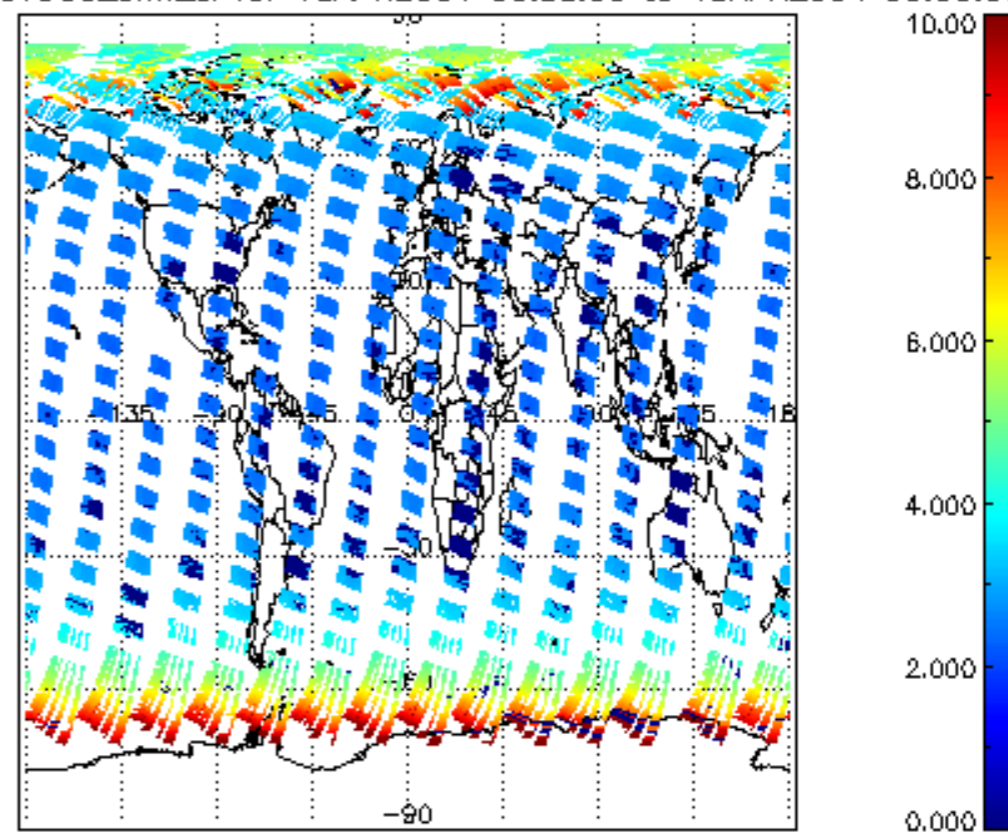
SCIOL2P_NADUV003_amf_cl for 18APR2004 00:00:00 to 19APR2004 00:00:00
