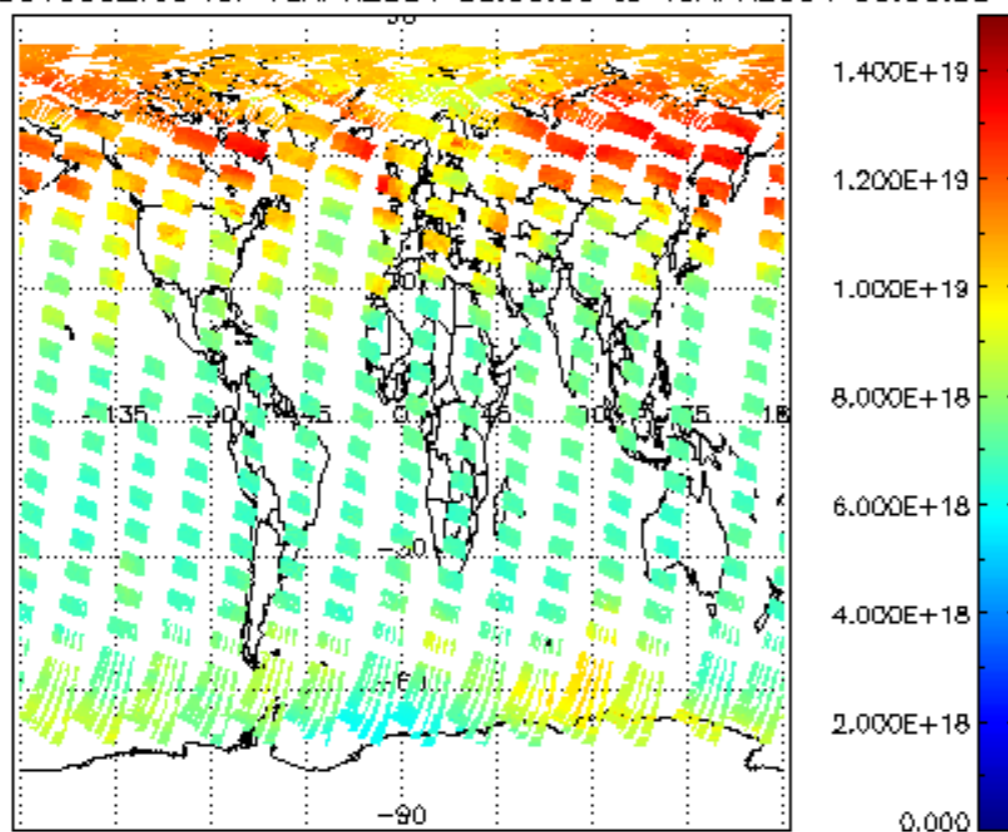
SCIOL2P_NADUV003_vcd for 18APR2004 00:00:00 to 19APR2004 00:00:00
