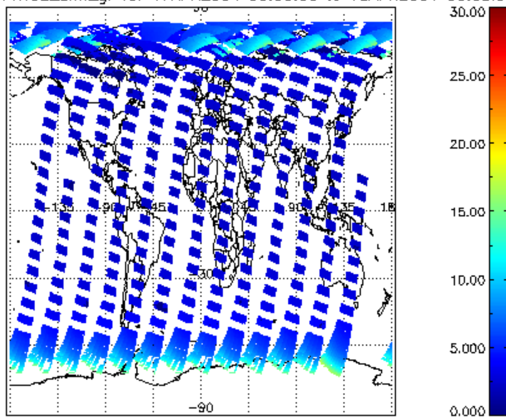
iCIOL2P_NADUV1NO2_amf_gr for 17APR2004 00:00:00 to 18APR2004 00:00:00
