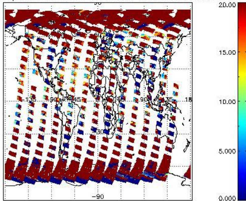
cLopt_depth for 17APR2004 00:00:00 to 18APR2004 00:00:00
