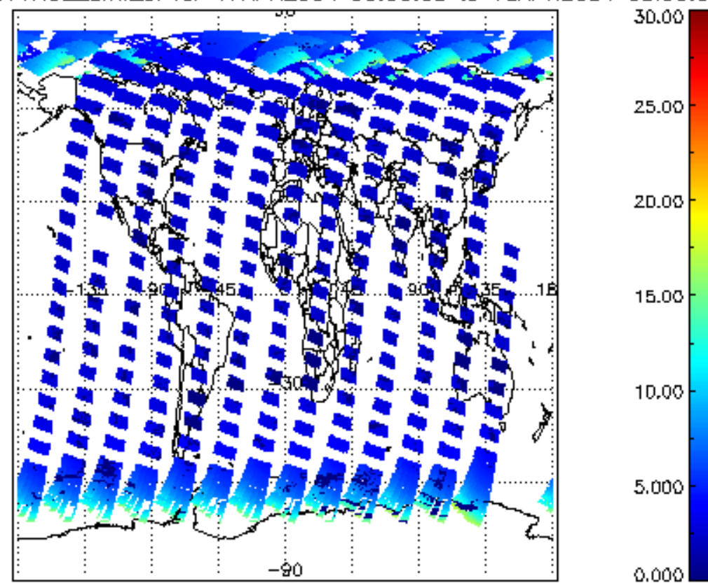
iCIOL2P_NADUV1NO2_amf_cl for 17APR2004 00:00:00 to 18APR2004 00:00:00
