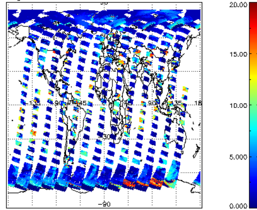
cl_top_height for 17APR2004 00:00:00 to 18APR2004 00:00:00
