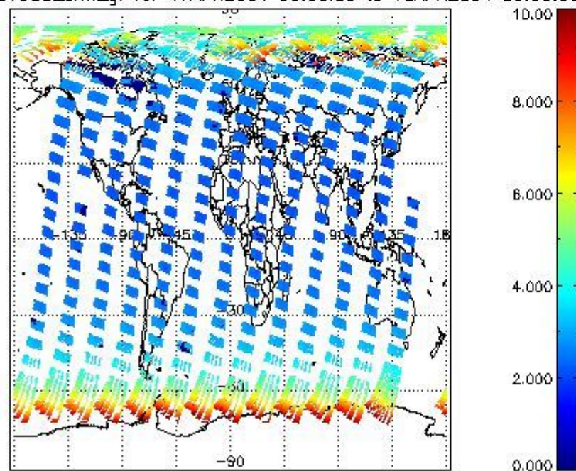
SCIOL2P_NADUV003_amf_gr for 17APR2004 00:00:00 to 18APR2004 00:00:00
