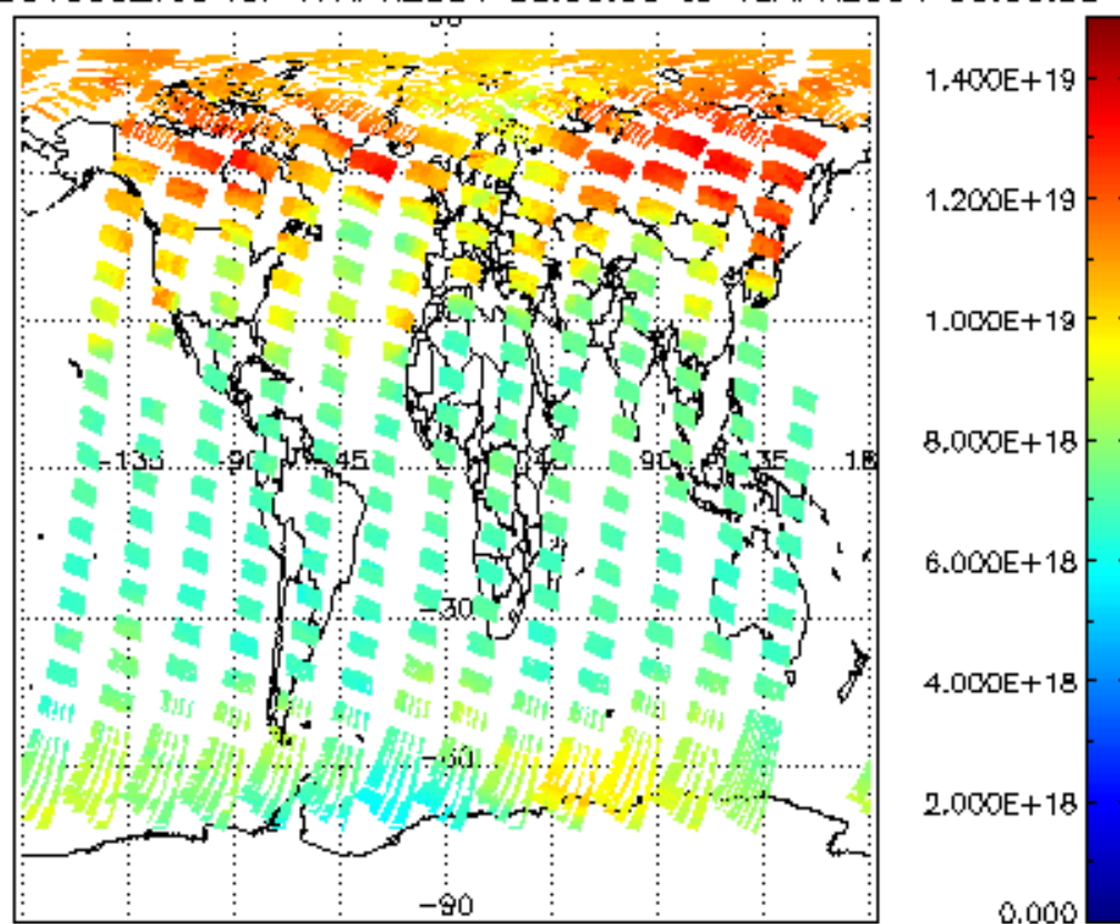
SCIOL2P_NADUV003_vcd for 17APR2004 00:00:00 to 18APR2004 00:00:00
