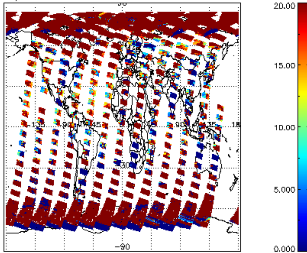
cl_opt_depth for 17APR2004 00:00:00 to 18APR2004 00:00:00
