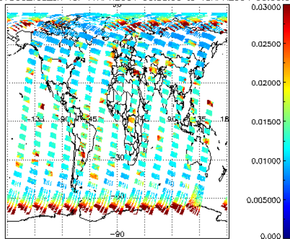
SCIOL2P_NADUV003_vcd_err for 17APR2004 00:00:00 to 18APR2004 00:00:00
