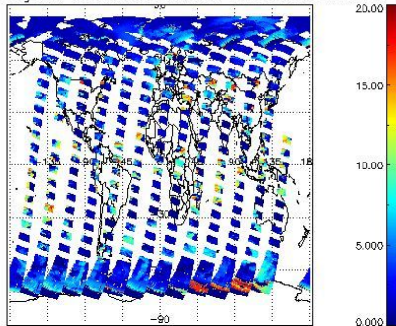
cL_top_height for 17APR2004 00:00:00 to 18APR2004 00:00:00
