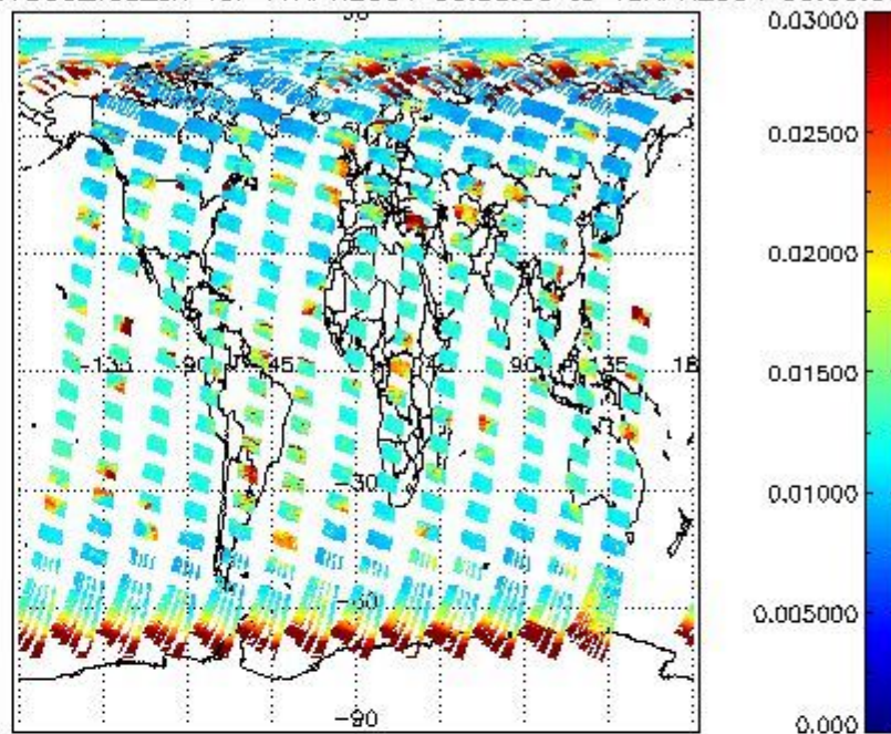
SCIOL2P_NADUV003_vcd_err for 17APR2004 00:00:00 to 18APR2004 00:00:00
