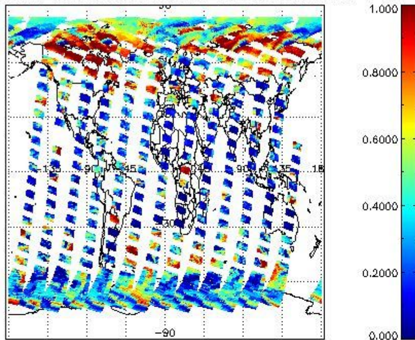
cLfrac for 17APR2004 00:00:00 to 18APR2004 00:00:00
