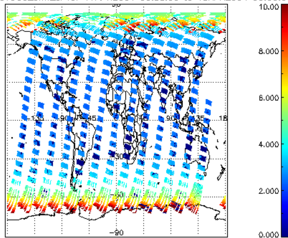
SCIOL2P_NADUV003_amf_cl for 17APR2004 00:00:00 to 18APR2004 00:00:00
