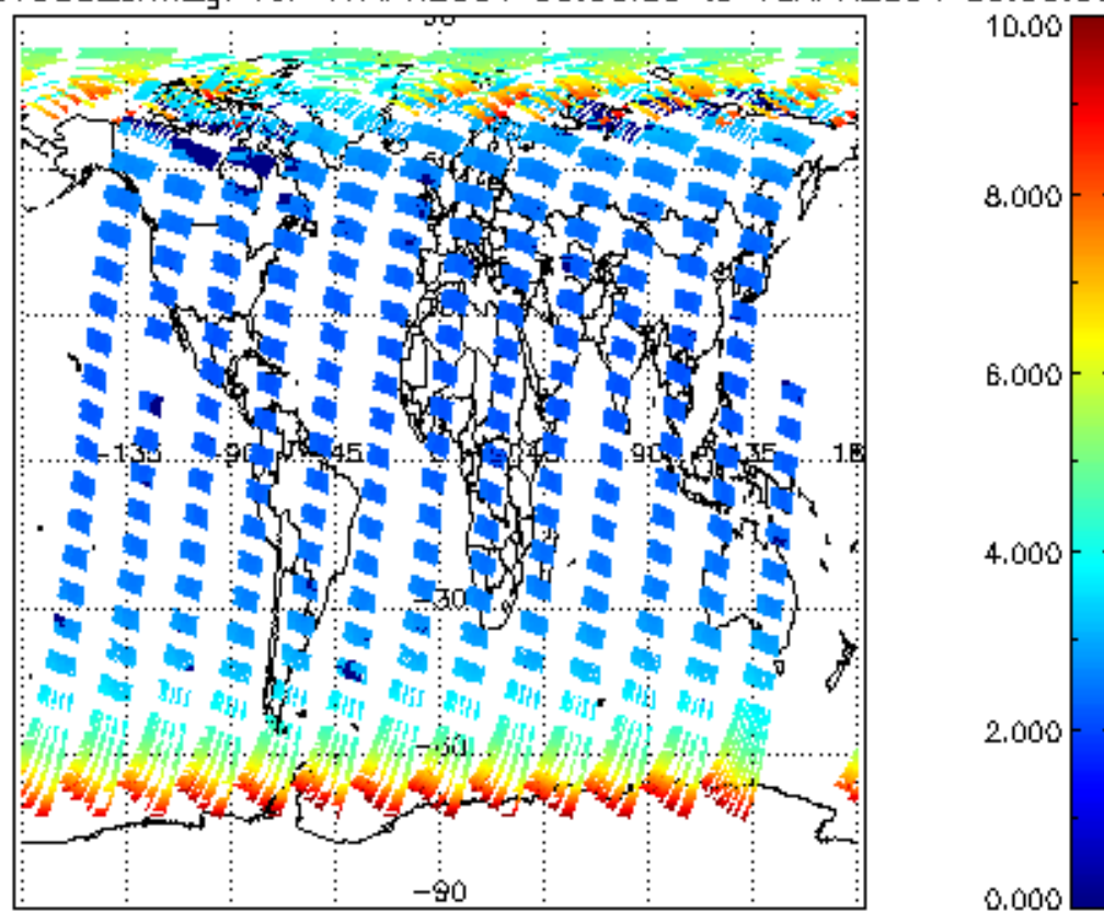
SCIOL2P_NADUV003_amf_gr for 17APR2004 00:00:00 to 18APR2004 00:00:00
