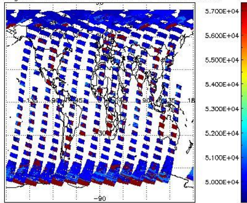
cloud_flags for 17APR2004 00:00:00 to 18APR2004 00:00:00
