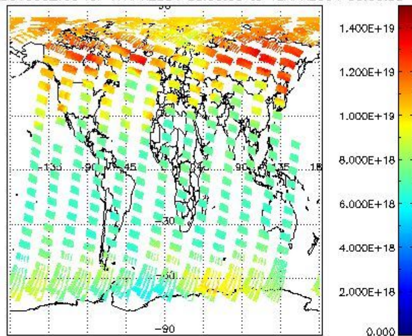
SCIOL2P_NADUV003_vcd for 17APR2004 00:00:00 to 18APR2004 00:00:00
