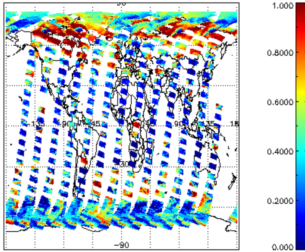
cl_frac for 17APR2004 00:00:00 to 18APR2004 00:00:00
