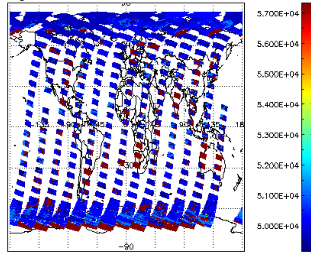
cloud_flags for 17APR2004 00:00:00 to 18APR2004 00:00:00
