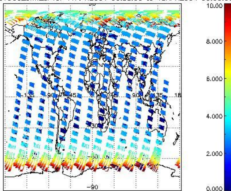
SCIOL2P_NADUV003_amf_cl for 17APR2004 00:00:00 to 18APR2004 00:00:00
