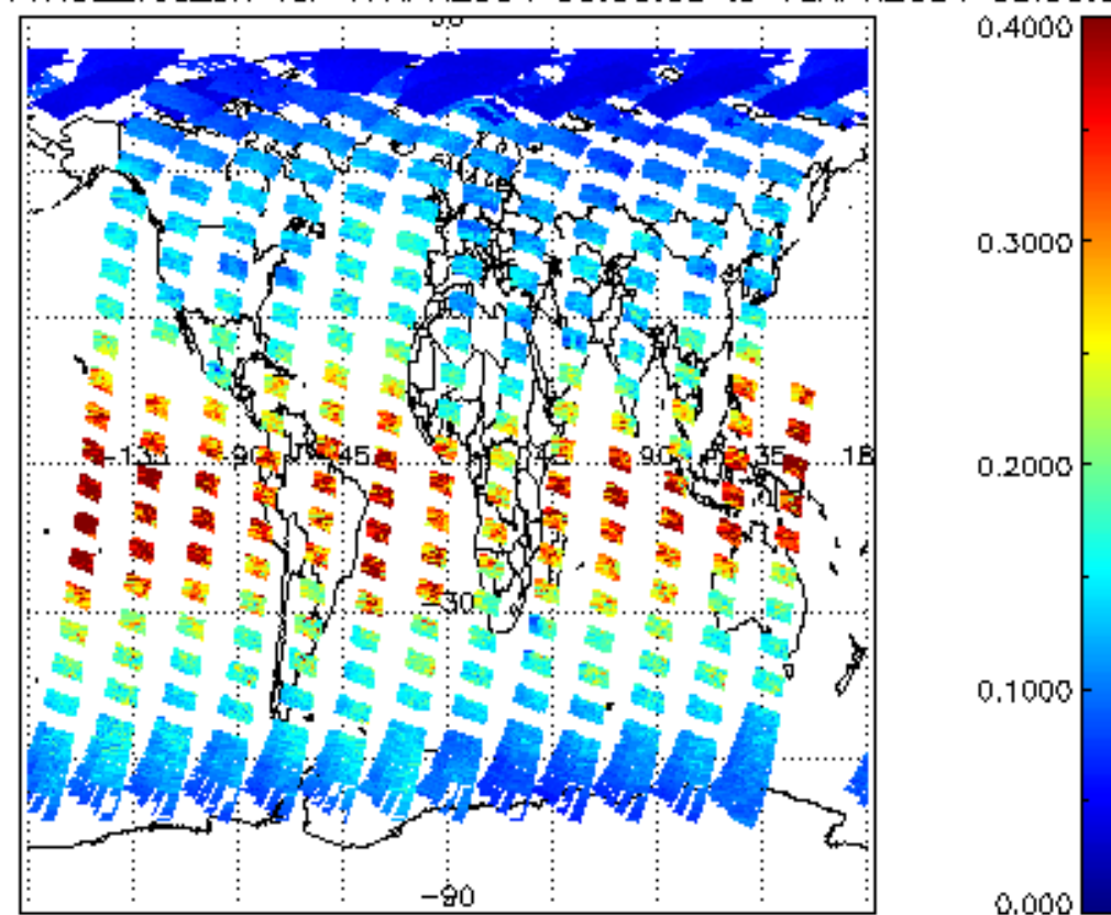
iCIOL2P_NADUV1NO2_vcd_err for 17APR2004 00:00:00 to 18APR2004 00:00:00
