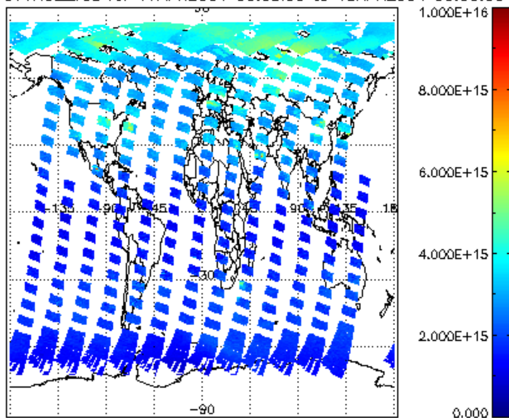
SCIOL2P_NADUV1NO2_vcd for 17APR2004 00:00:00 to 18APR2004 00:00:00
